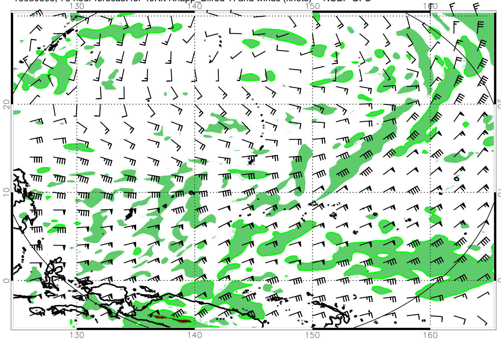
16080606, 78 hour forecast for 49Kft Knapp_Ellrod TI and winds (knots) -- NCEP GFS
