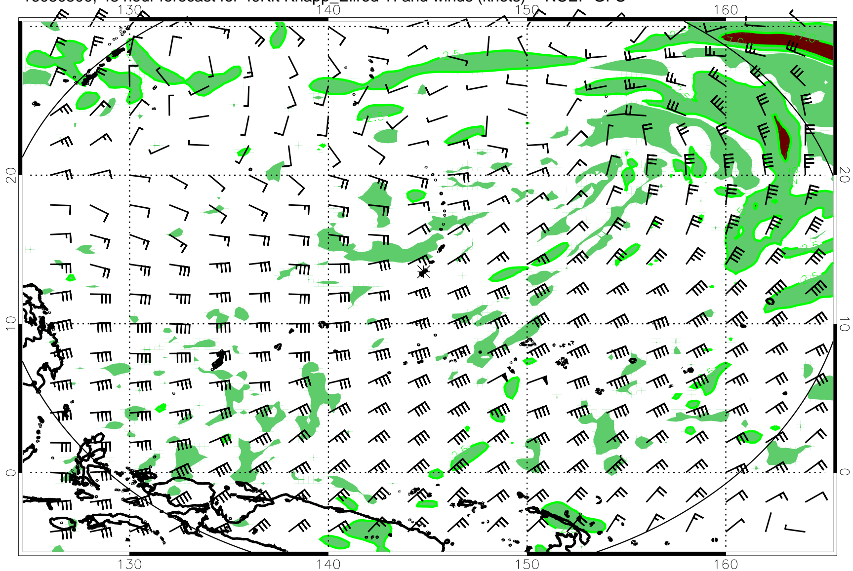
16080500, 48 hour forecast for 49Kft Knapp_Ellrod TI and winds (knots) -- NCEP GFS
