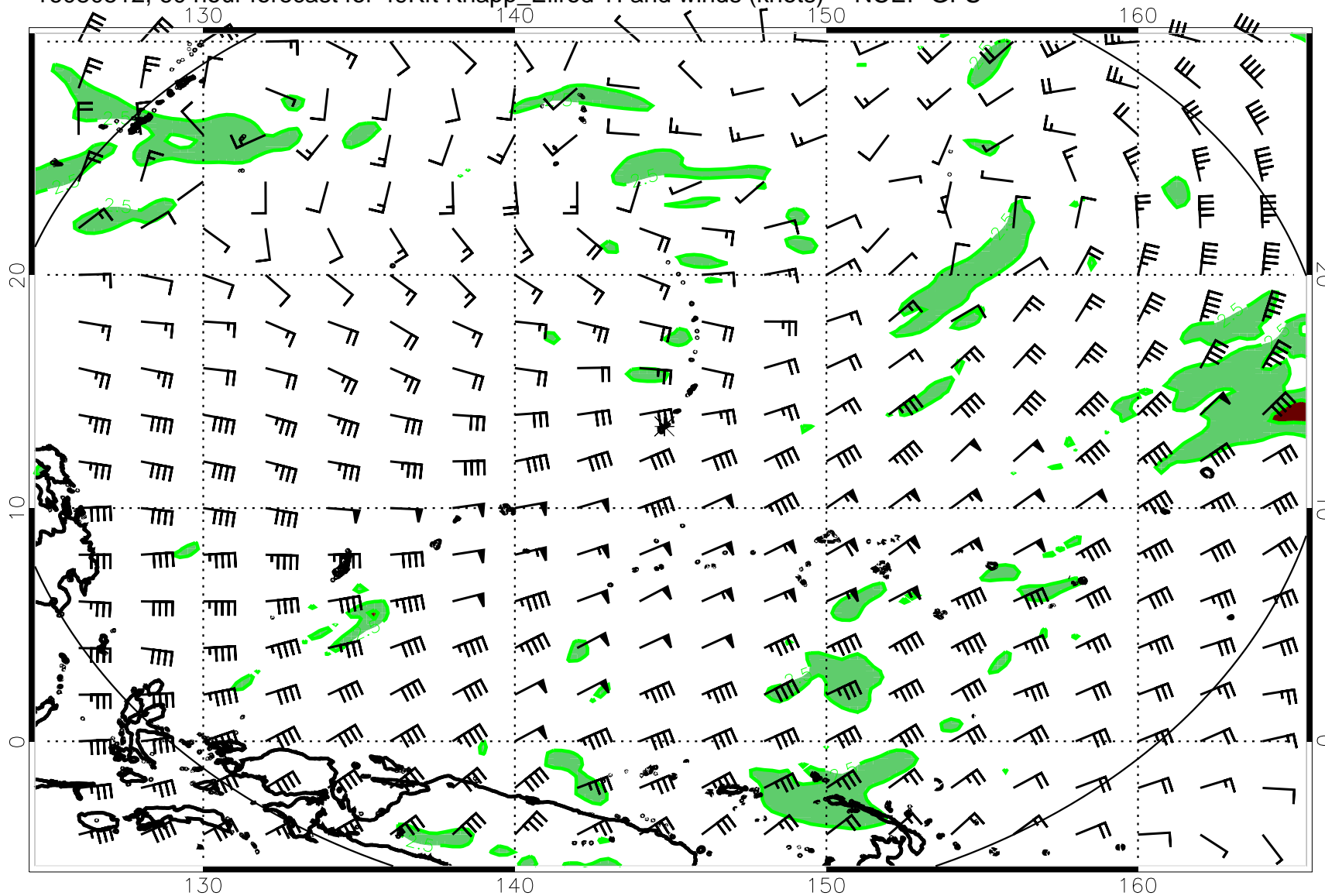
16080512, 60 hour forecast for 49Kft Knapp_Ellrod TI and winds (knots) -- NCEP GFS
