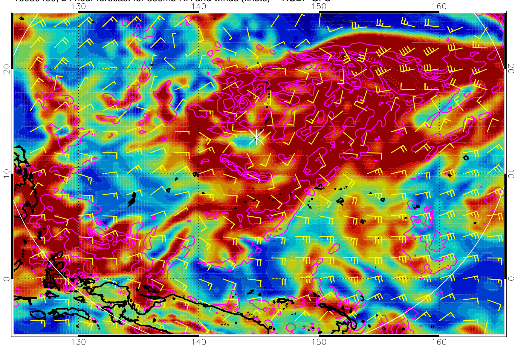
16080400, 24 hour forecast for 300mb RH and winds (knots) -- NCEP GFS
