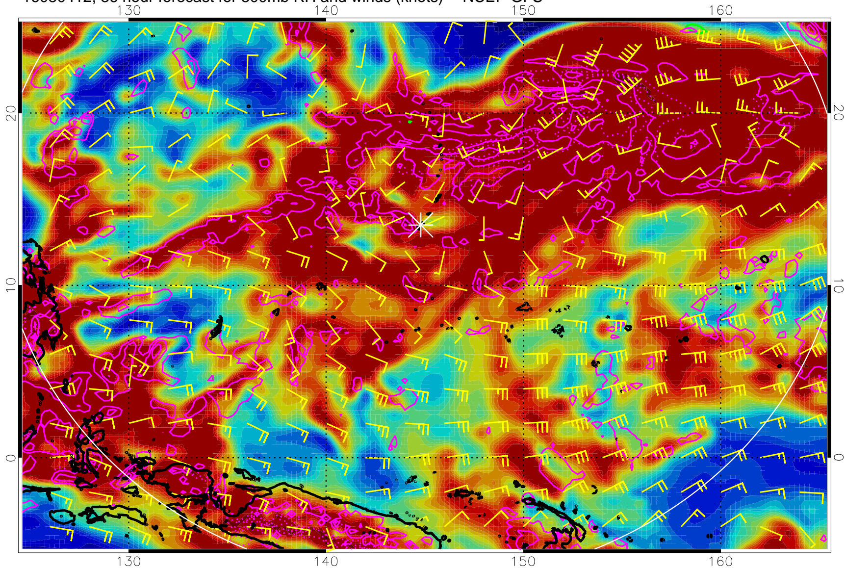
16080412, 36 hour forecast for 300mb RH and winds (knots) -- NCEP GFS
