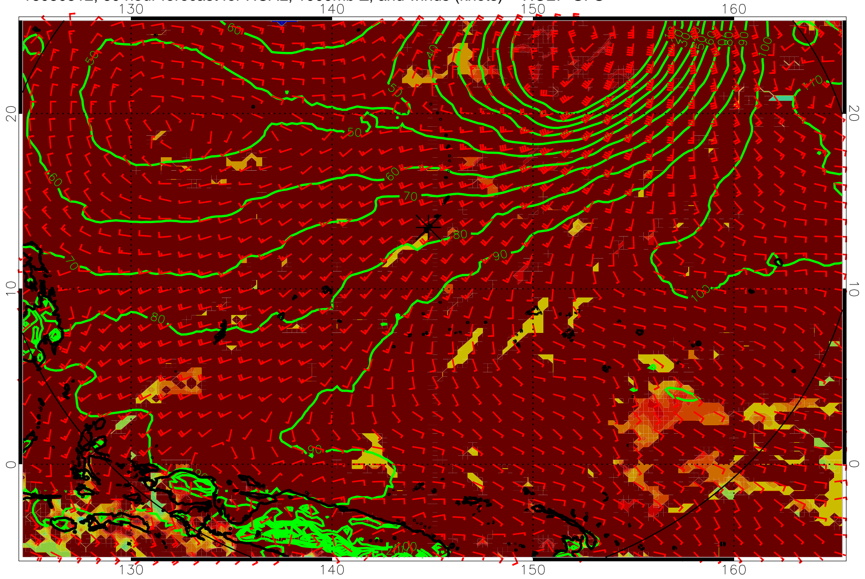
16080512, 60 hour forecast for HCAL, 1000mb Z, and winds (knots) -- NCEP GFS
