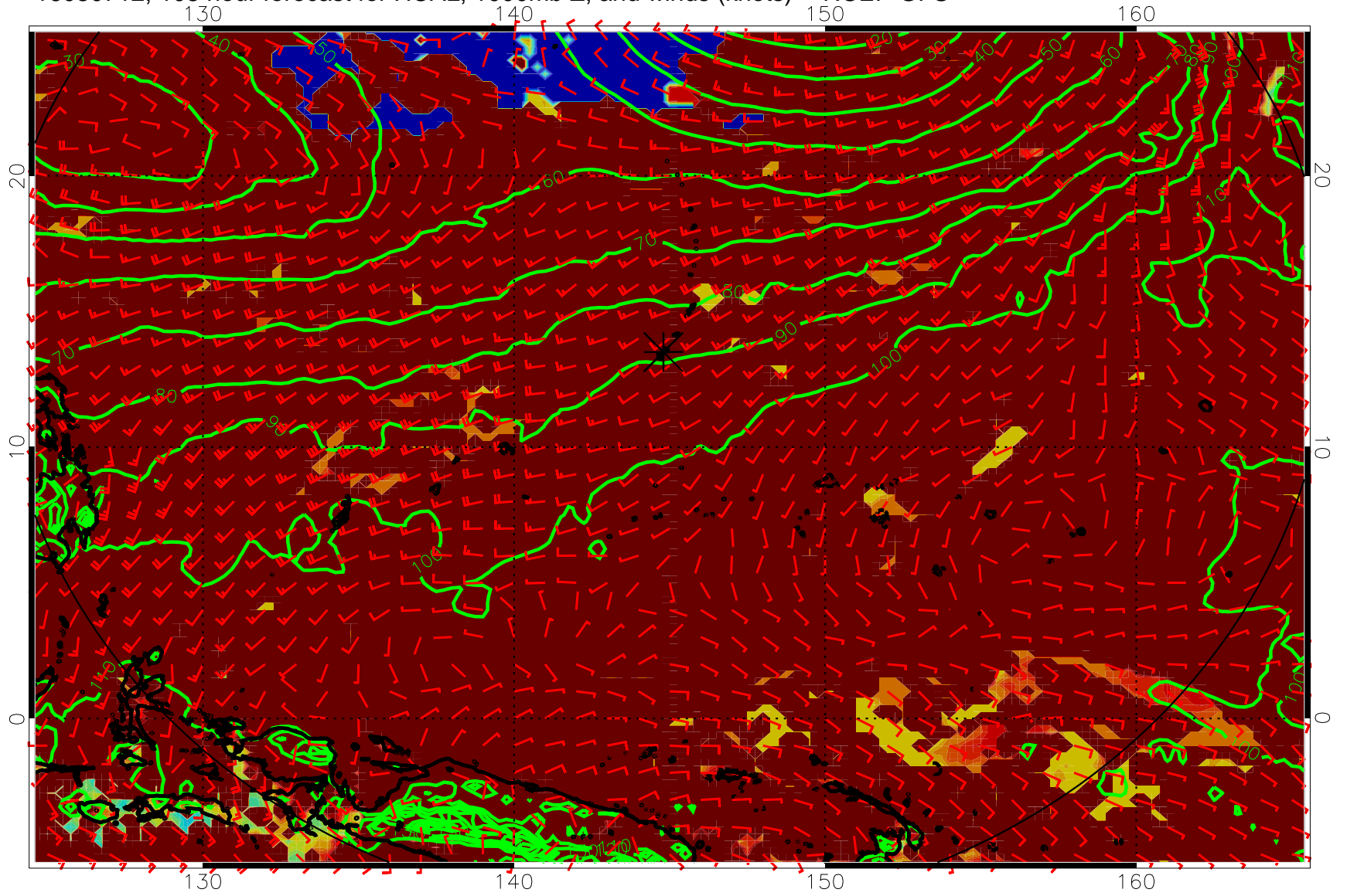
16080712, 108 hour forecast for HCAL, 1000mb Z, and winds (knots) -- NCEP GFS
