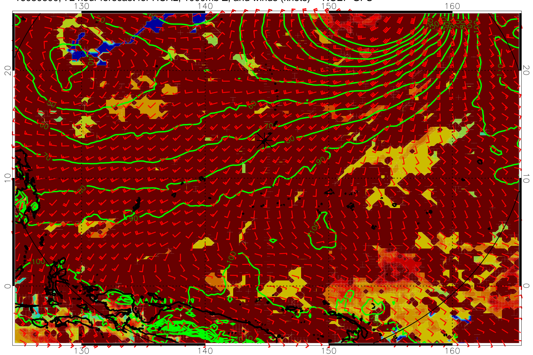
16080600, 72 hour forecast for HCAL, 1000mb Z, and winds (knots) -- NCEP GFS
