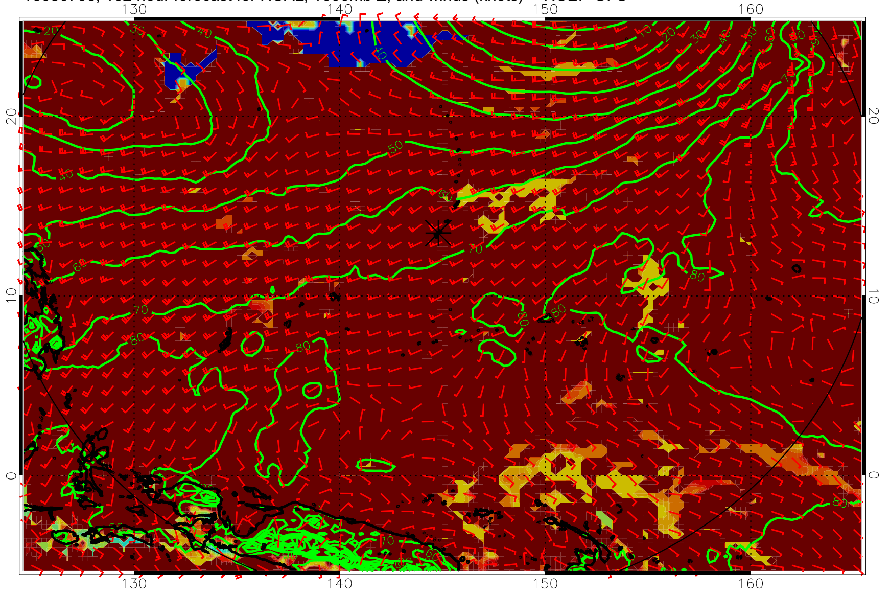
16080706, 102 hour forecast for HCAL, 1000mb Z, and winds (knots) -- NCEP GFS
