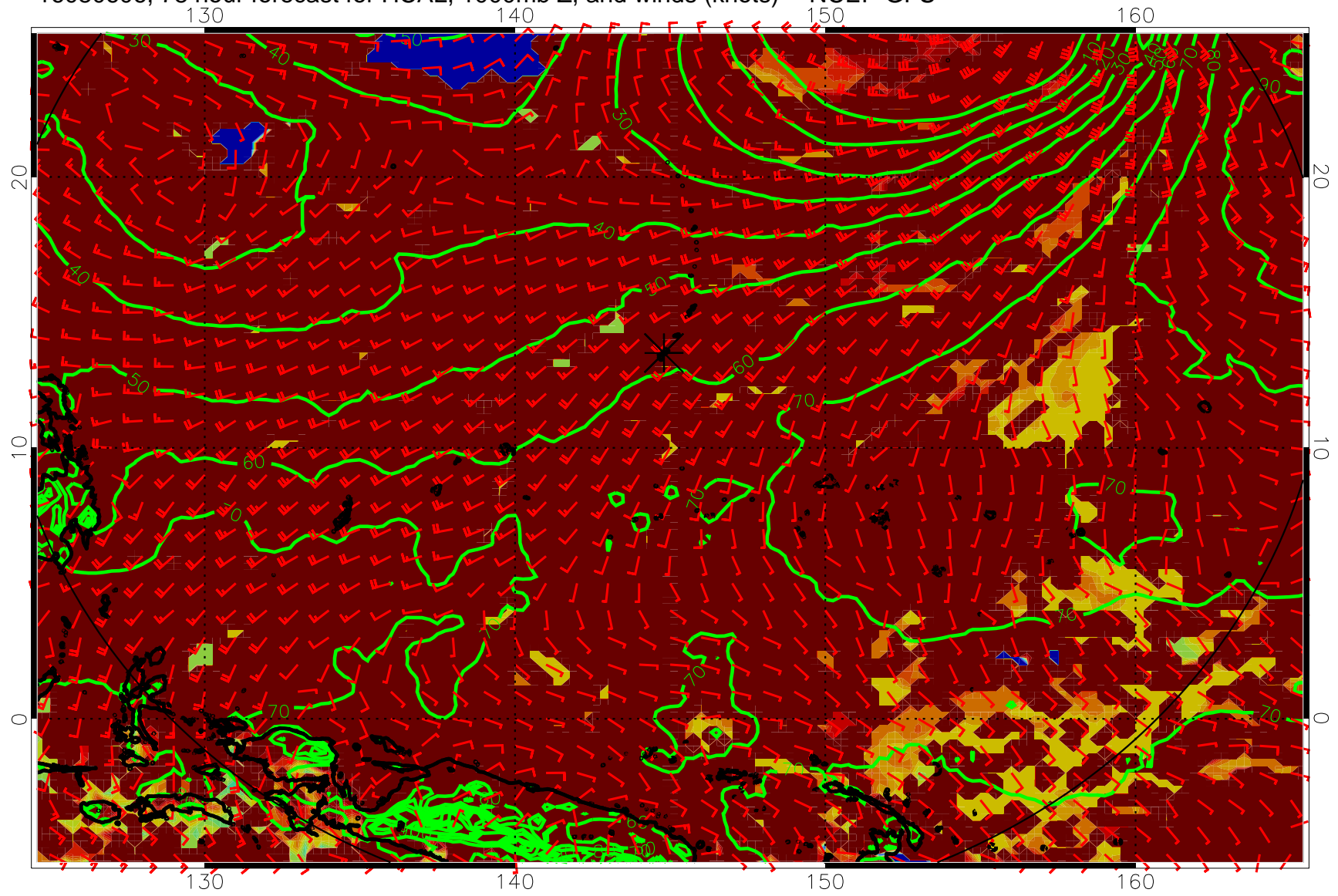
16080606, 78 hour forecast for HCAL, 1000mb Z, and winds (knots) -- NCEP GFS
