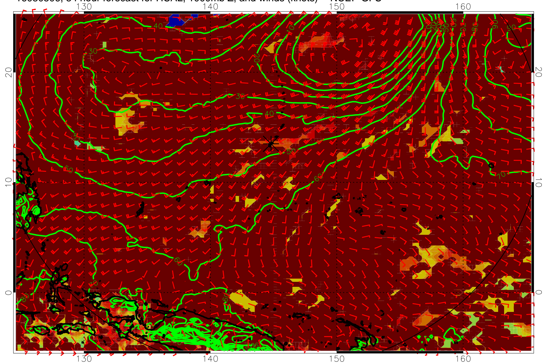
16080506, 54 hour forecast for HCAL, 1000mb Z, and winds (knots) -- NCEP GFS
