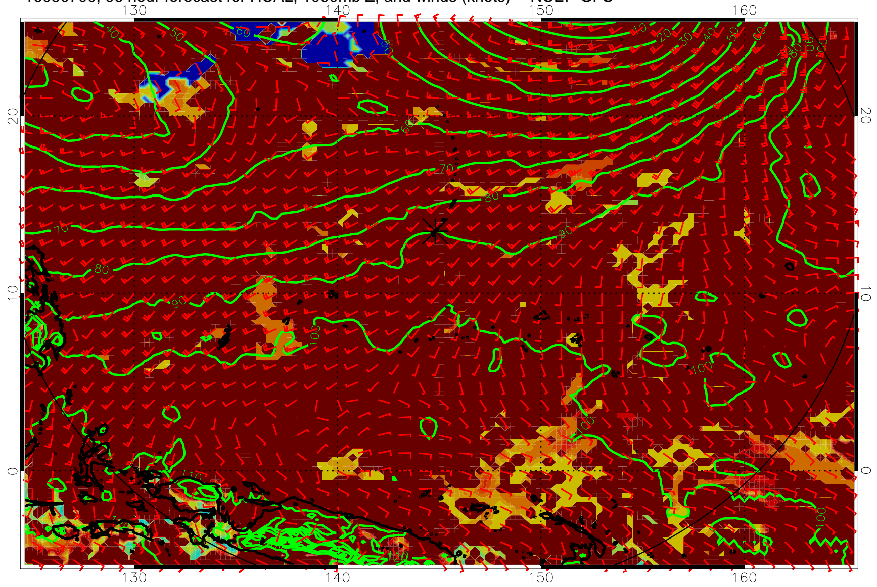
16080700, 96 hour forecast for HCAL, 1000mb Z, and winds (knots) -- NCEP GFS
