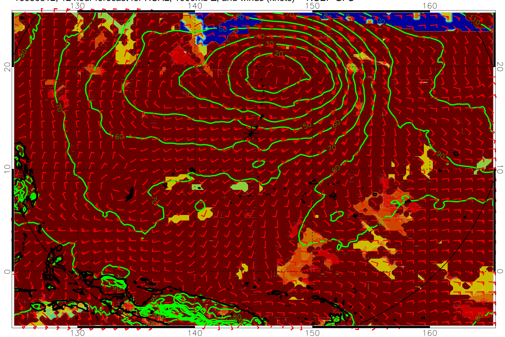
16080312, 12 hour forecast for HCAL, 1000mb Z, and winds (knots) -- NCEP GFS
