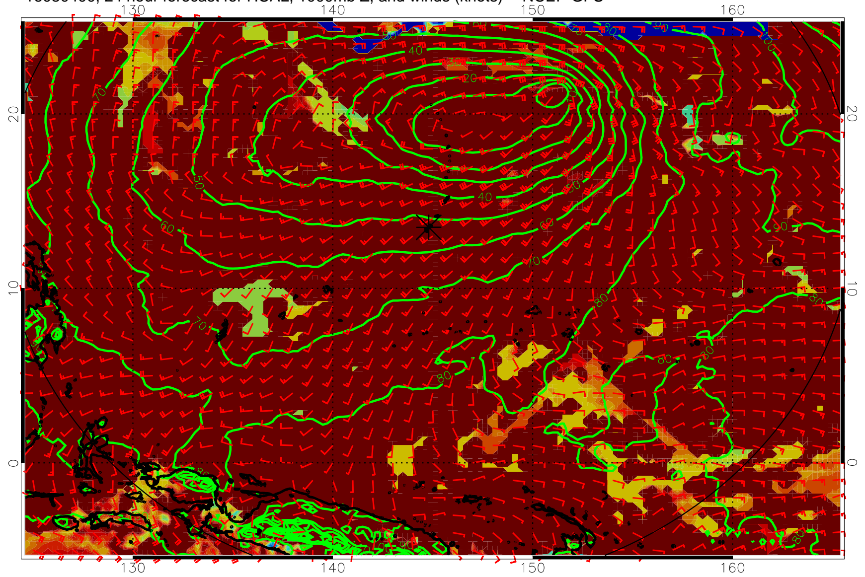
16080400, 24 hour forecast for HCAL, 1000mb Z, and winds (knots) -- NCEP GFS
