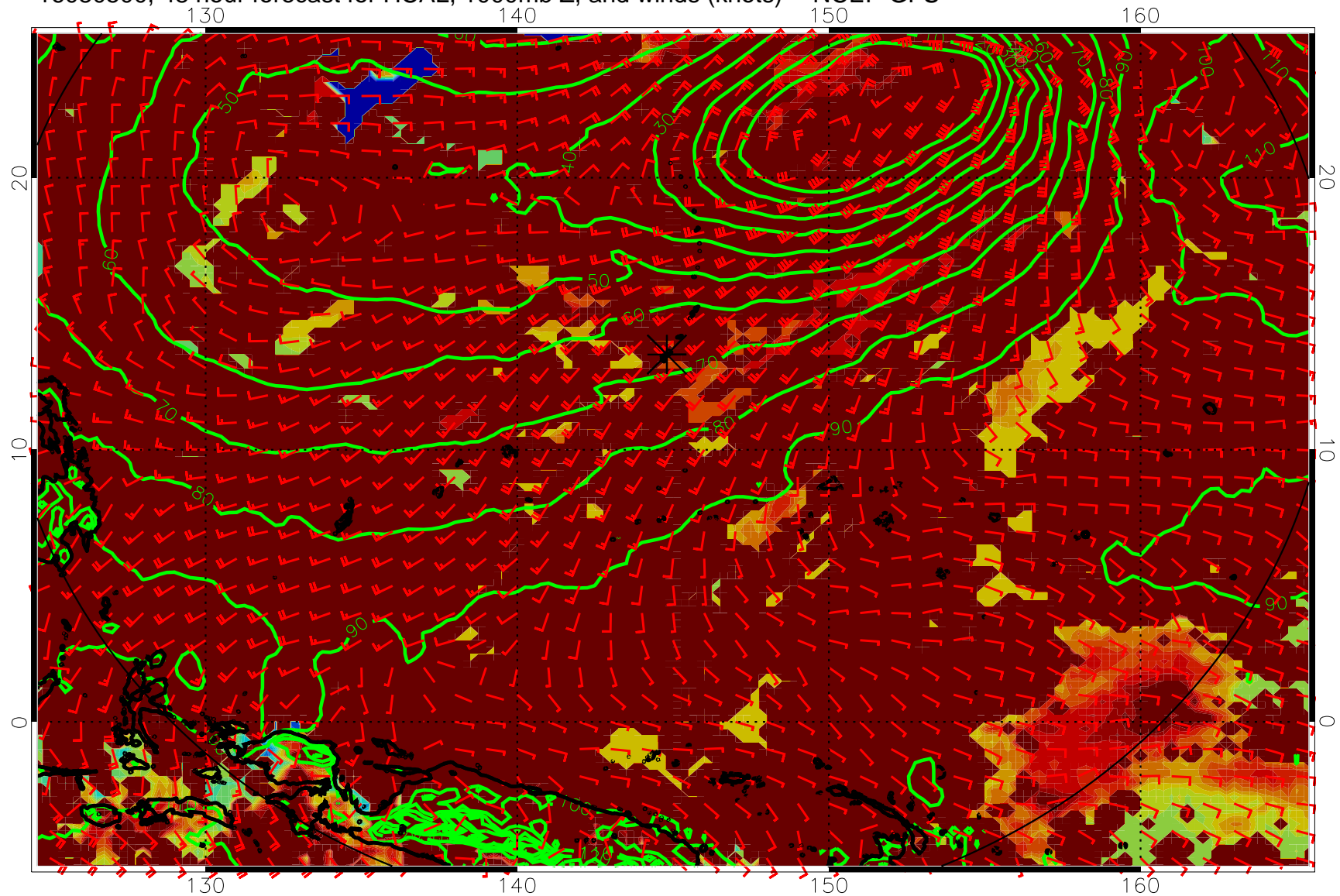
16080500, 48 hour forecast for HCAL, 1000mb Z, and winds (knots) -- NCEP GFS
