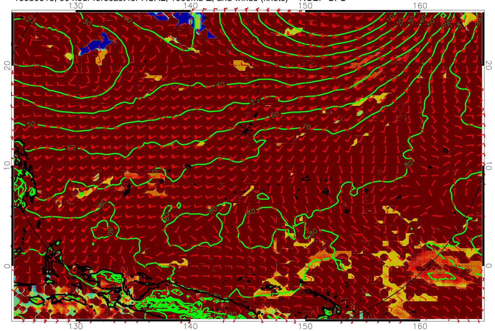
16080618, 90 hour forecast for HCAL, 1000mb Z, and winds (knots) -- NCEP GFS
