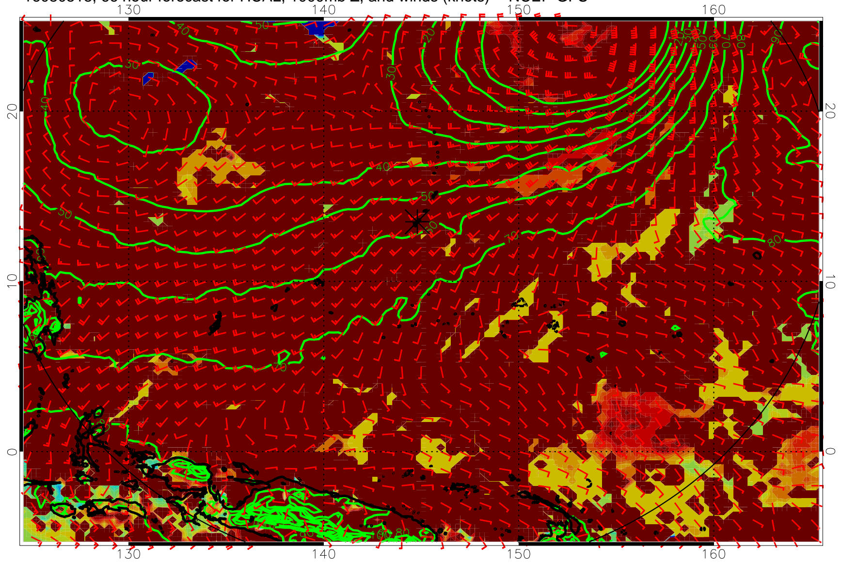
16080518, 66 hour forecast for HCAL, 1000mb Z, and winds (knots) -- NCEP GFS
