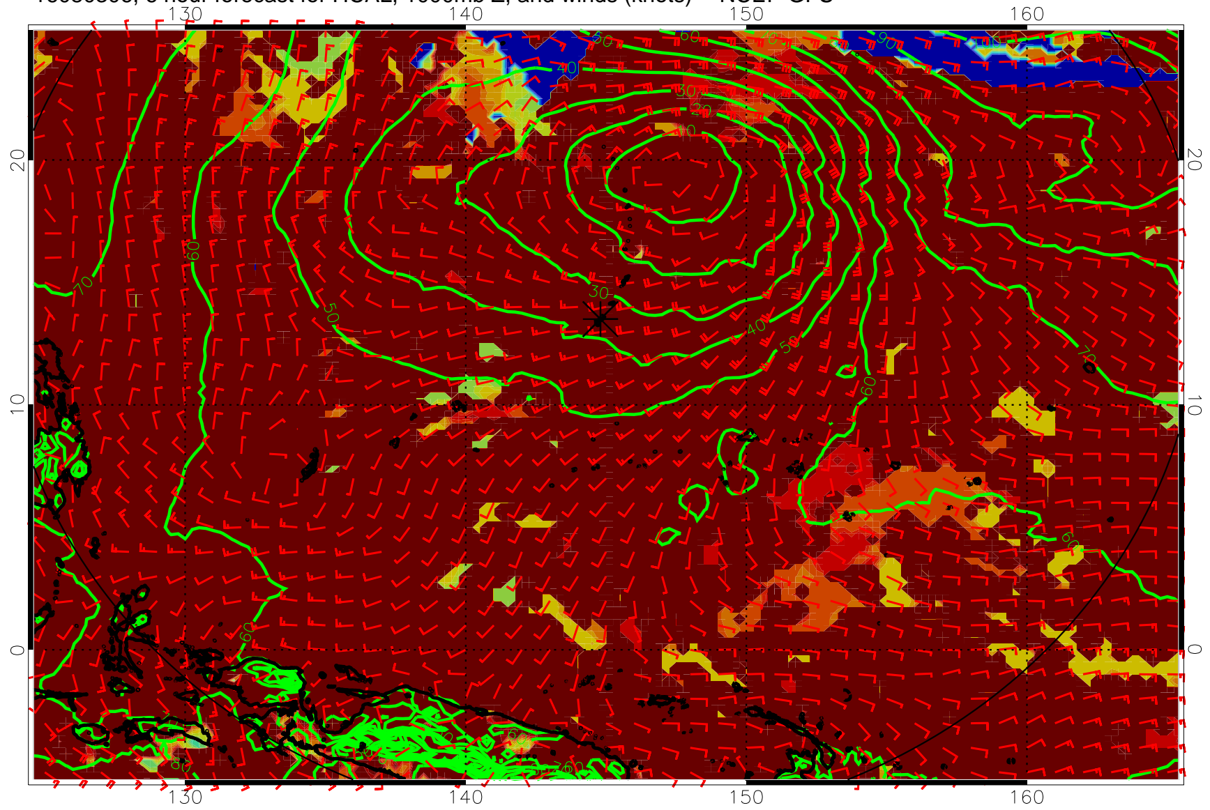
16080306, 6 hour forecast for HCAL, 1000mb Z, and winds (knots) -- NCEP GFS
