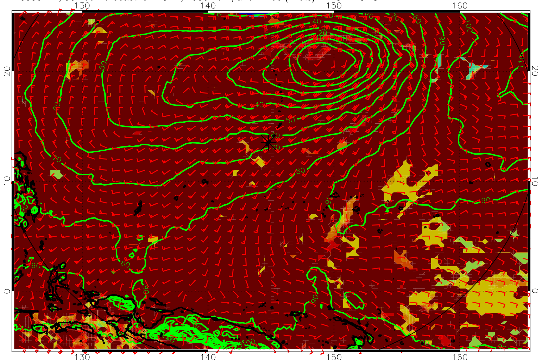
16080412, 36 hour forecast for HCAL, 1000mb Z, and winds (knots) -- NCEP GFS
