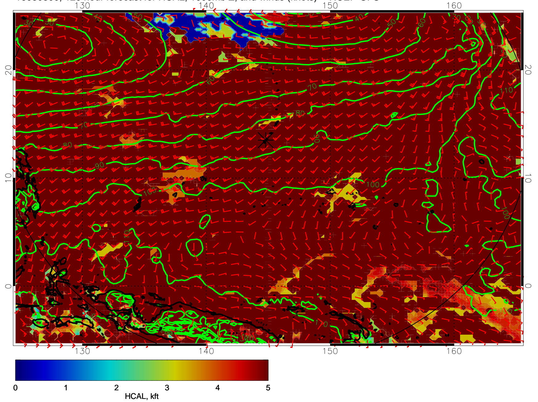
16080800, 120 hour forecast for HCAL, 1000mb Z, and winds (knots) -- NCEP GFS
