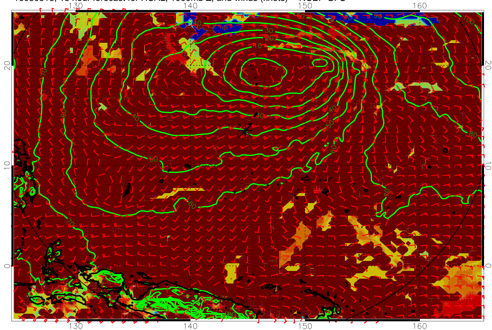
16080318, 18 hour forecast for HCAL, 1000mb Z, and winds (knots) -- NCEP GFS
