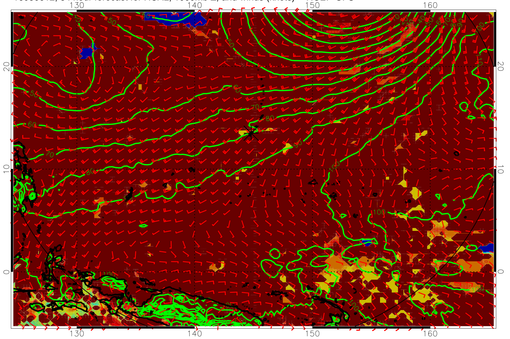
16080612, 84 hour forecast for HCAL, 1000mb Z, and winds (knots) -- NCEP GFS
