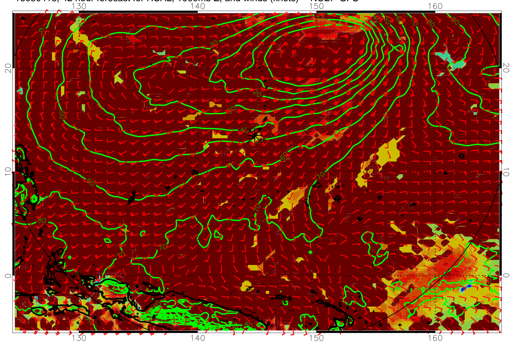
16080418, 42 hour forecast for HCAL, 1000mb Z, and winds (knots) -- NCEP GFS
