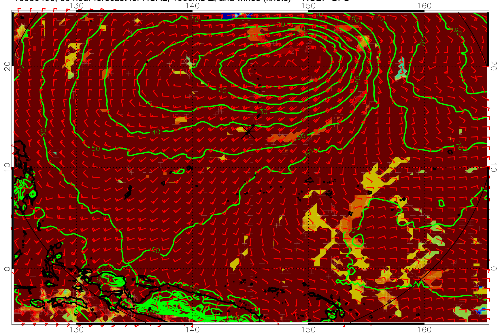
16080406, 30 hour forecast for HCAL, 1000mb Z, and winds (knots) -- NCEP GFS
