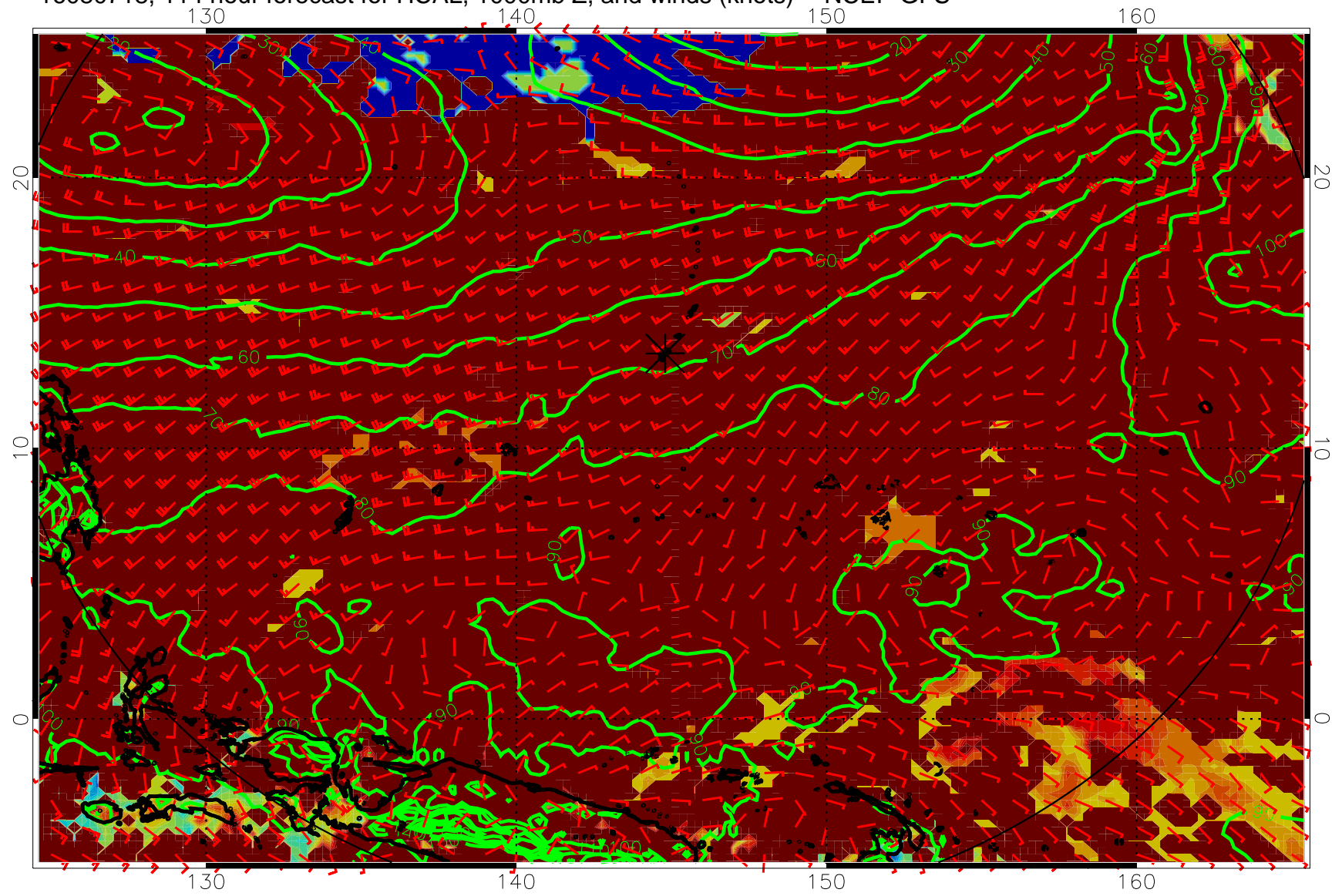
16080718, 114 hour forecast for HCAL, 1000mb Z, and winds (knots) -- NCEP GFS
