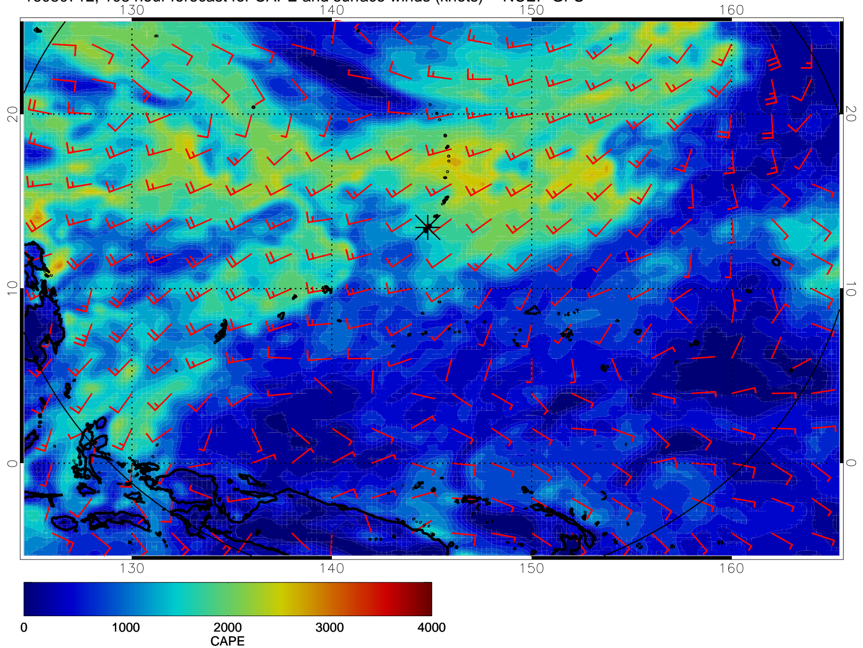
16080712, 108 hour forecast for CAPE and surface winds (knots) -- NCEP GFS
