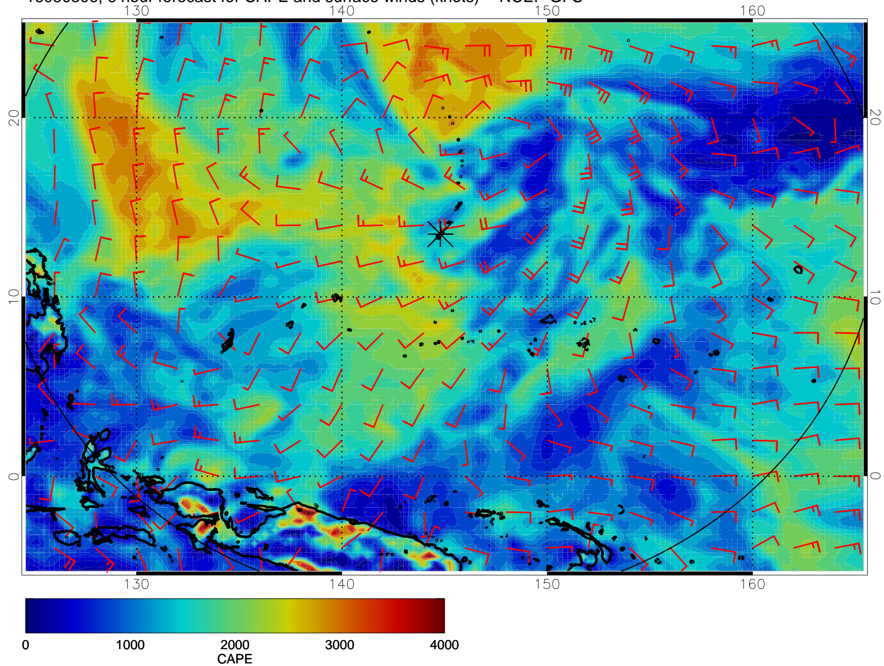
16080306, 6 hour forecast for CAPE and surface winds (knots) -- NCEP GFS
