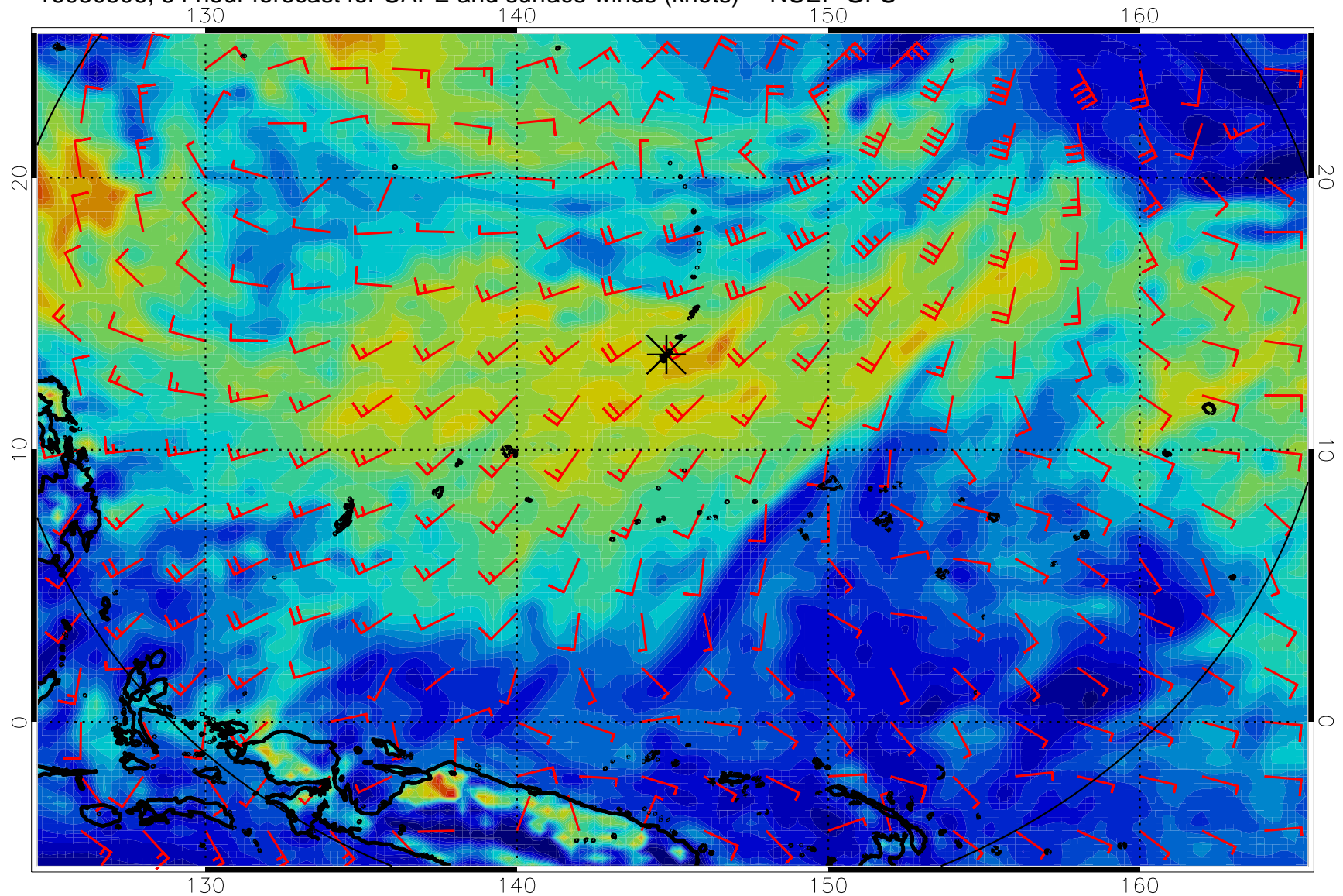
16080506, 54 hour forecast for CAPE and surface winds (knots) -- NCEP GFS
