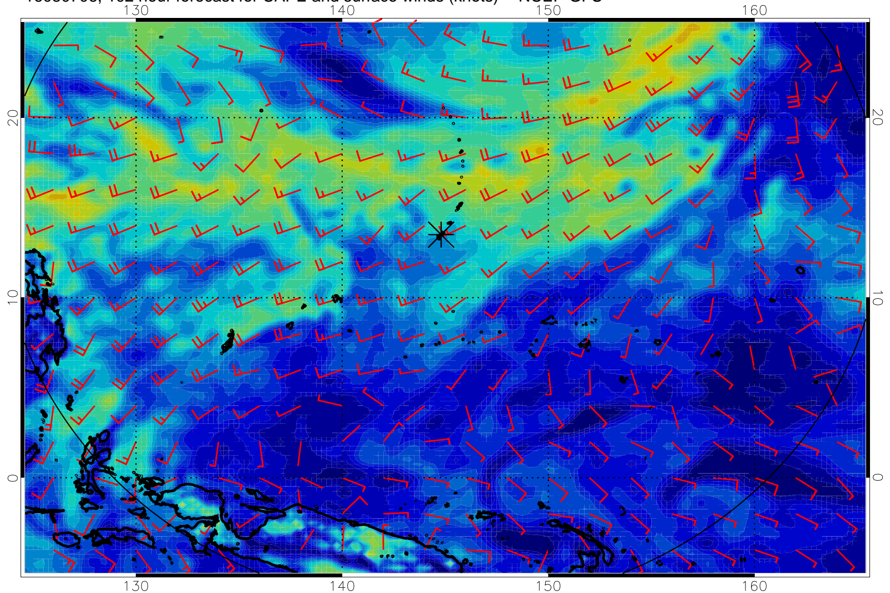
16080706, 102 hour forecast for CAPE and surface winds (knots) -- NCEP GFS
