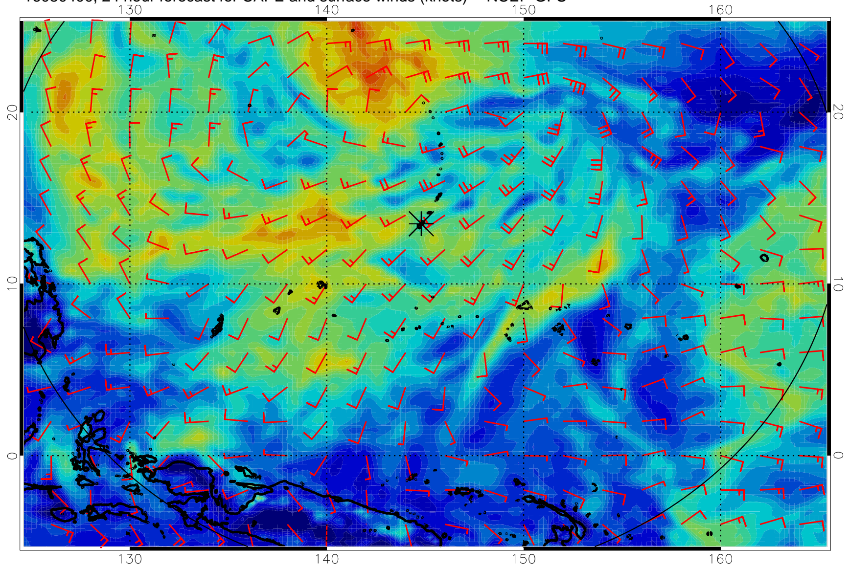
16080400, 24 hour forecast for CAPE and surface winds (knots) -- NCEP GFS
