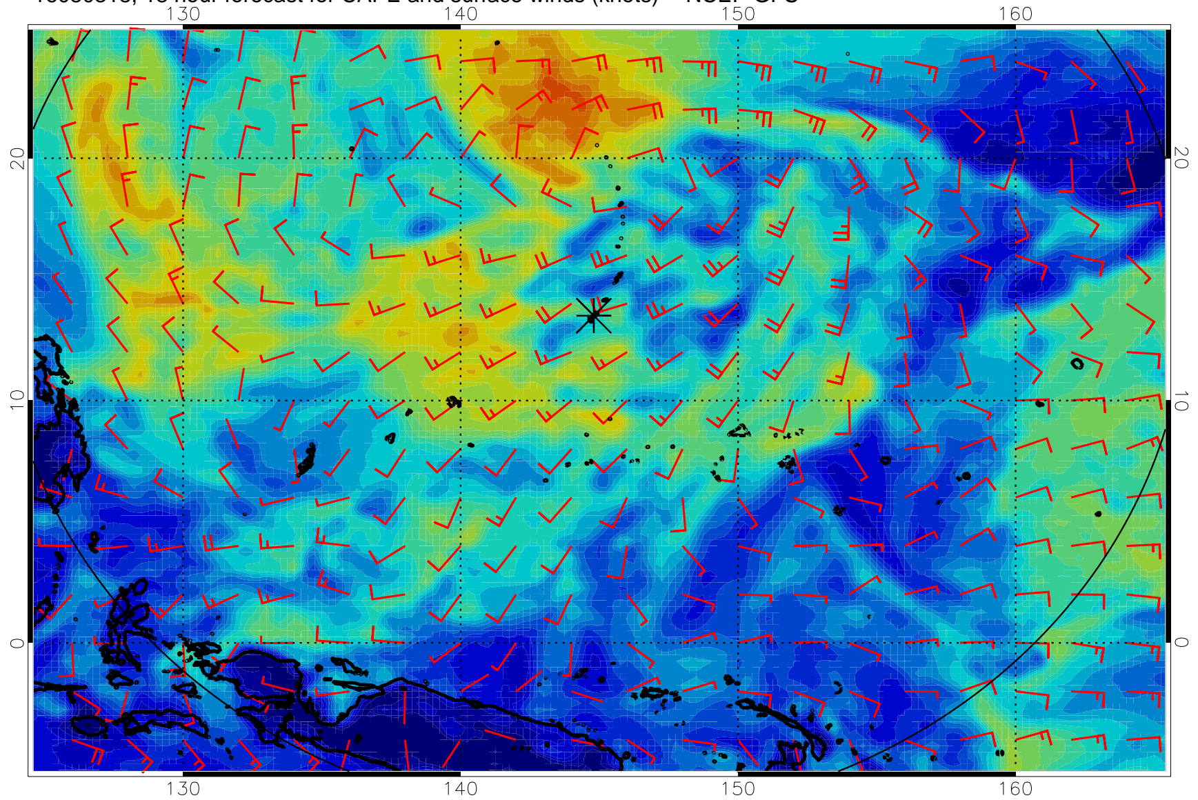
16080318, 18 hour forecast for CAPE and surface winds (knots) -- NCEP GFS
