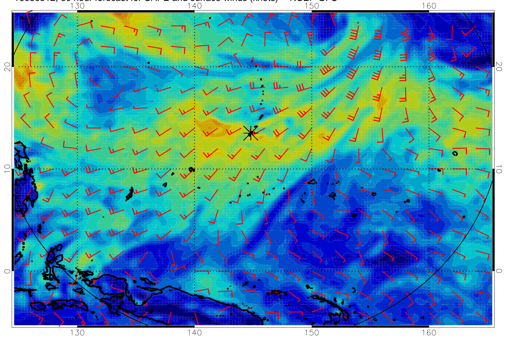
16080512, 60 hour forecast for CAPE and surface winds (knots) -- NCEP GFS
