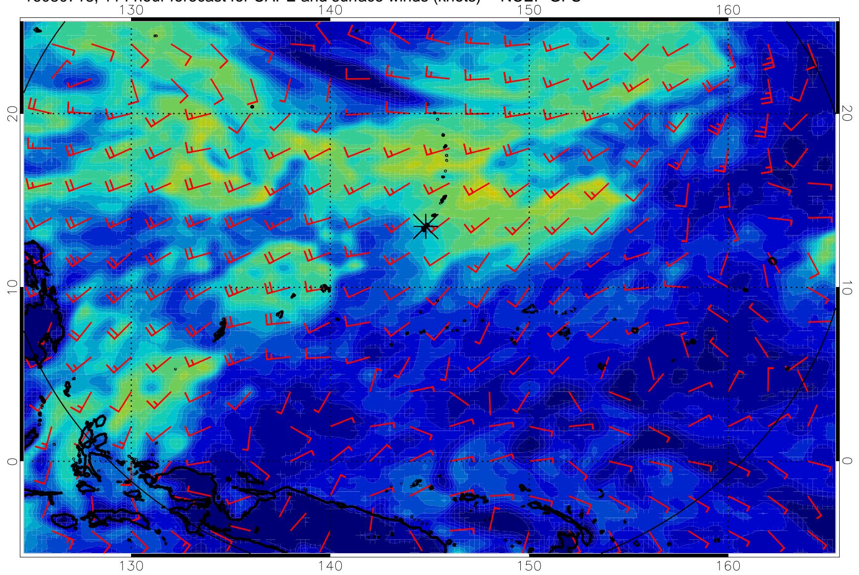
16080718, 114 hour forecast for CAPE and surface winds (knots) -- NCEP GFS
