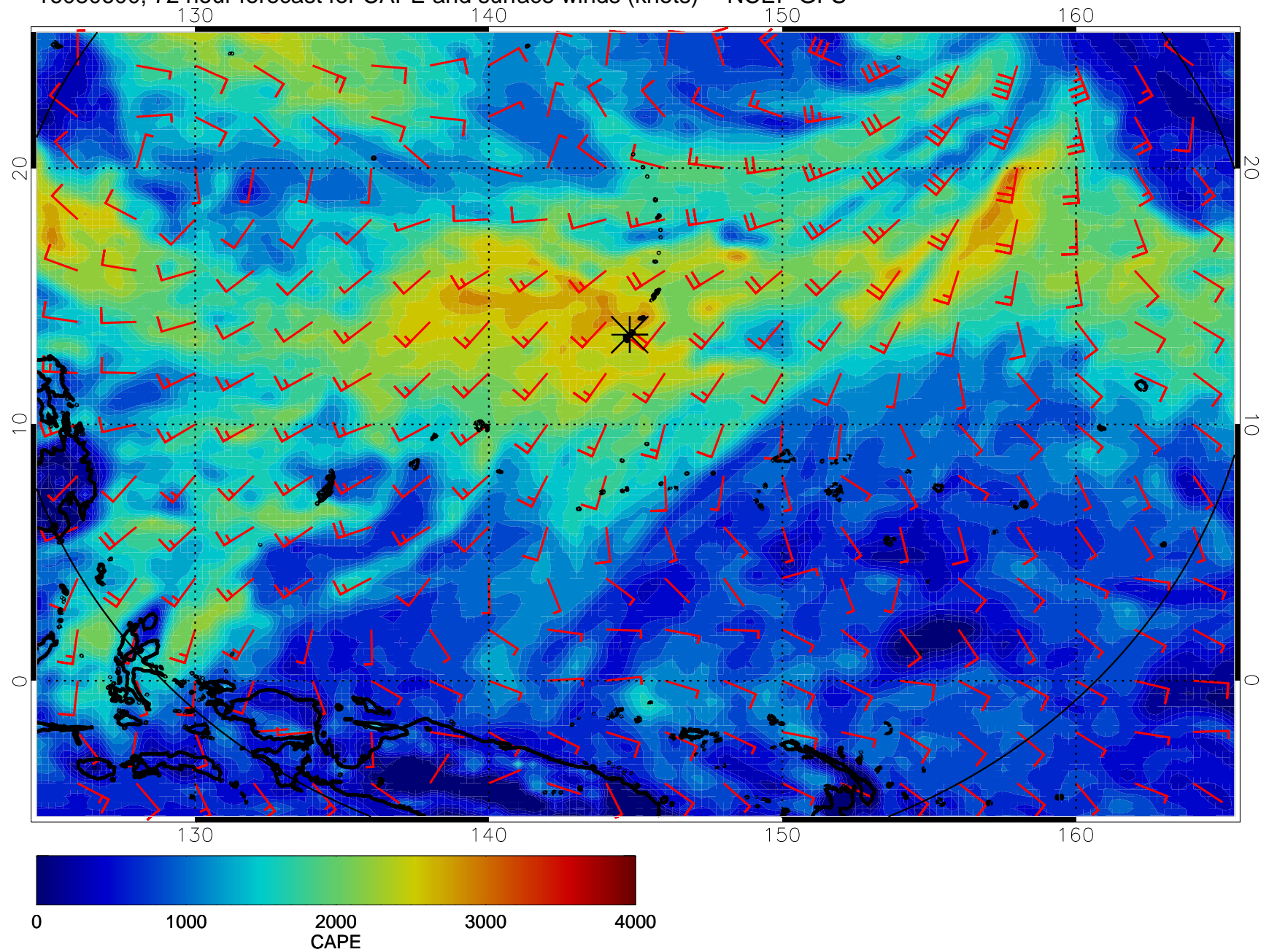
16080600, 72 hour forecast for CAPE and surface winds (knots) -- NCEP GFS
