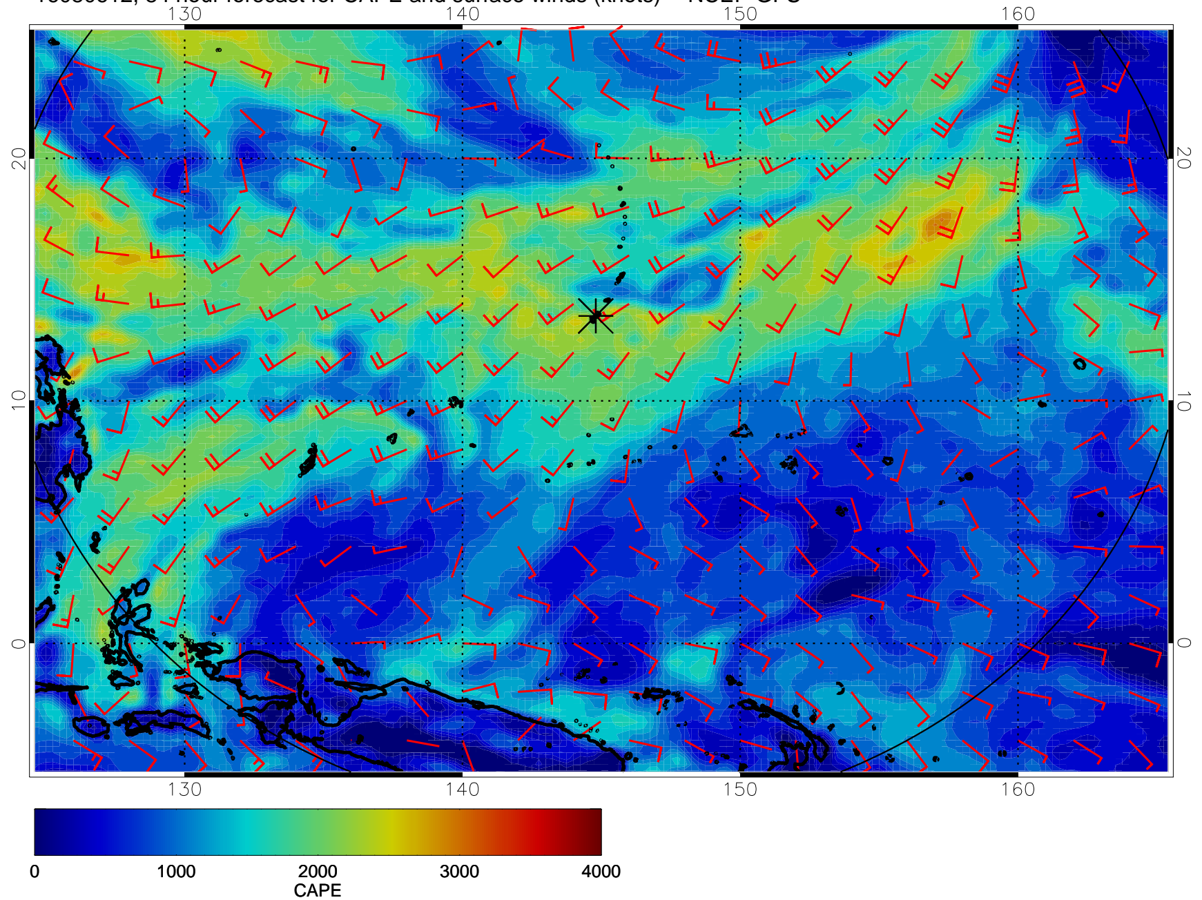
16080612, 84 hour forecast for CAPE and surface winds (knots) -- NCEP GFS
