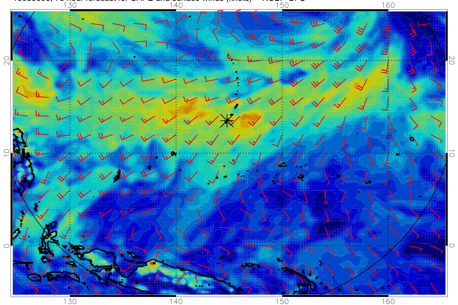
16080606, 78 hour forecast for CAPE and surface winds (knots) -- NCEP GFS
