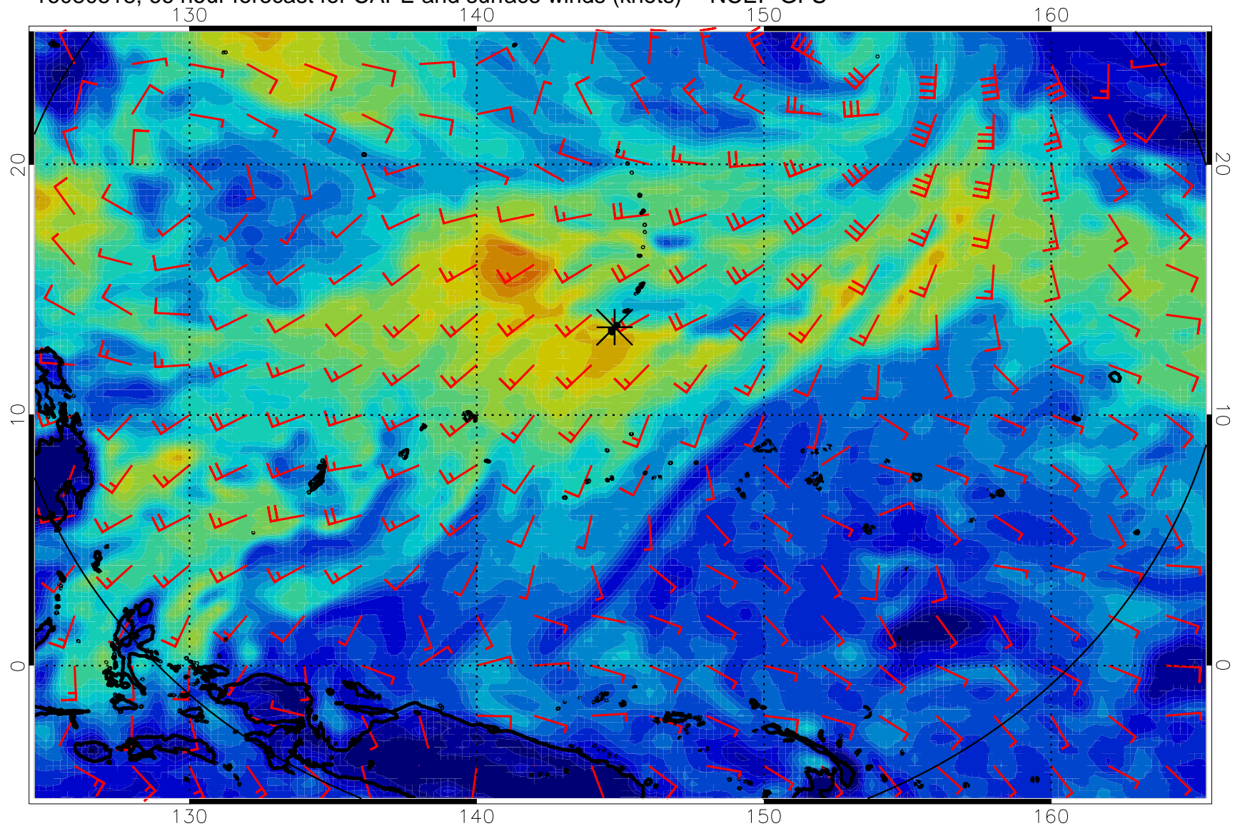
16080518, 66 hour forecast for CAPE and surface winds (knots) -- NCEP GFS
