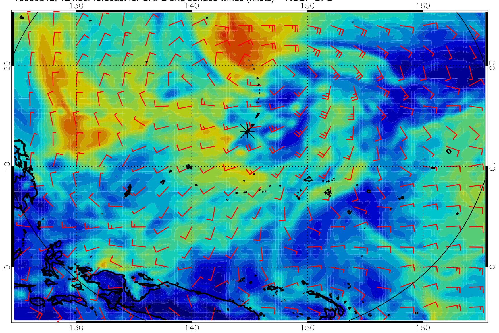
16080312, 12 hour forecast for CAPE and surface winds (knots) -- NCEP GFS
