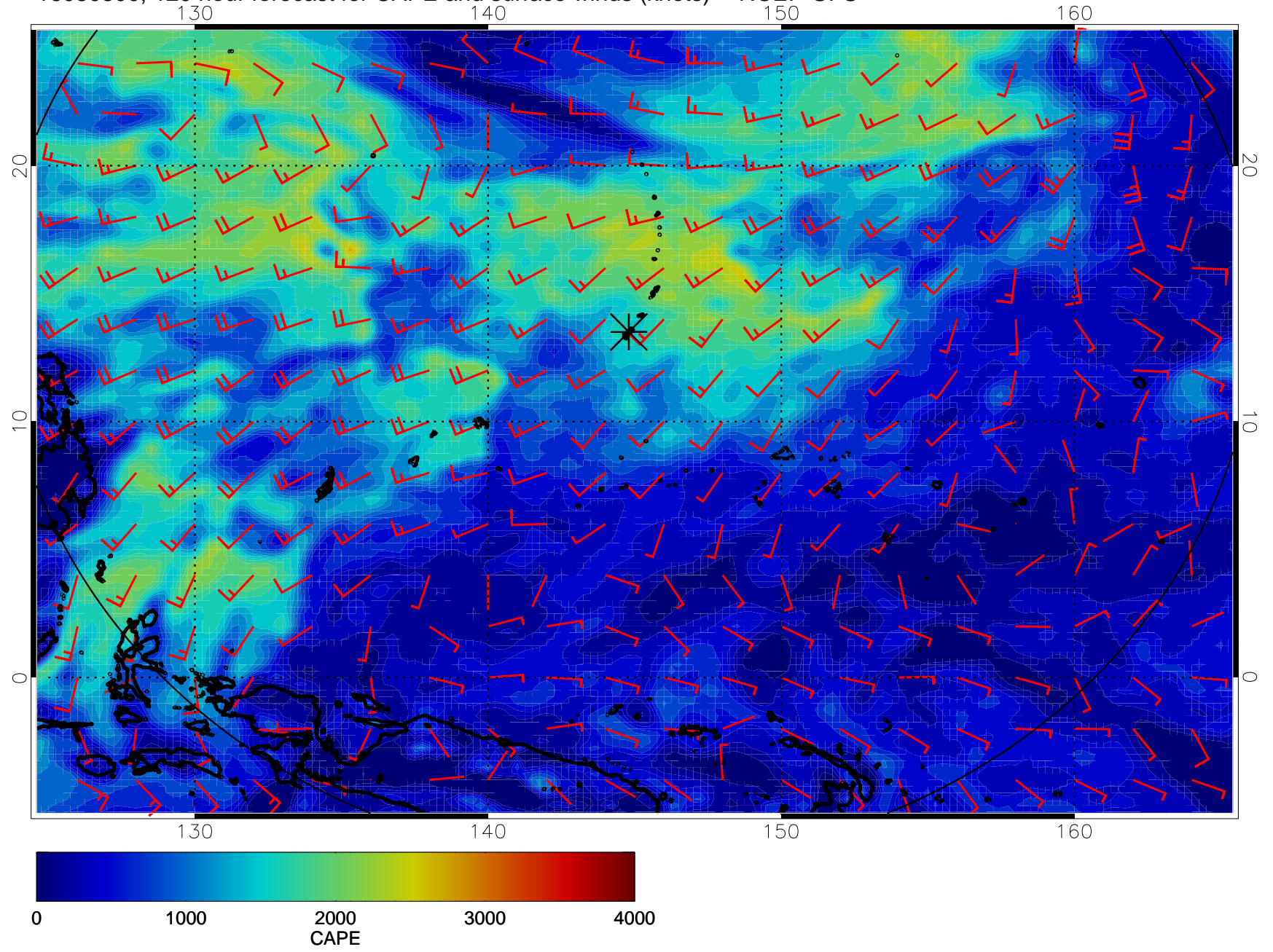
16080800, 120 hour forecast for CAPE and surface winds (knots) -- NCEP GFS
