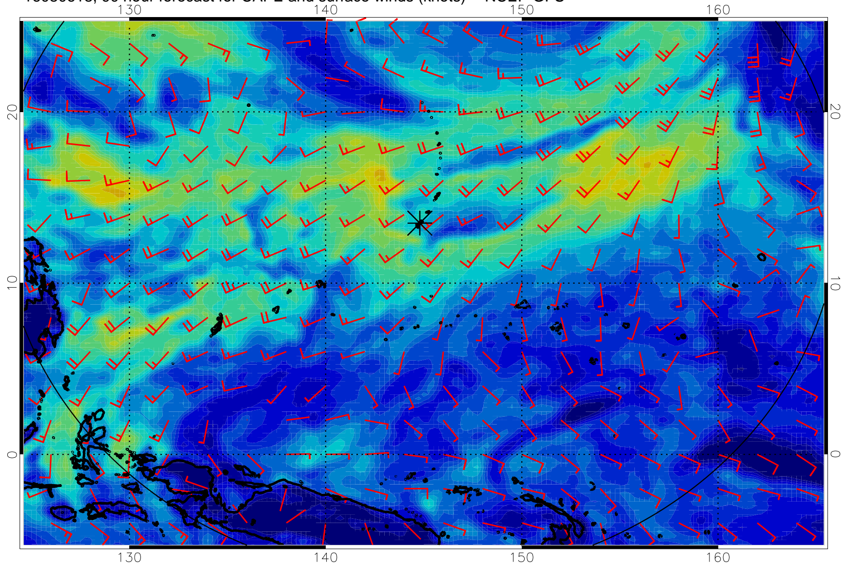
16080618, 90 hour forecast for CAPE and surface winds (knots) -- NCEP GFS
