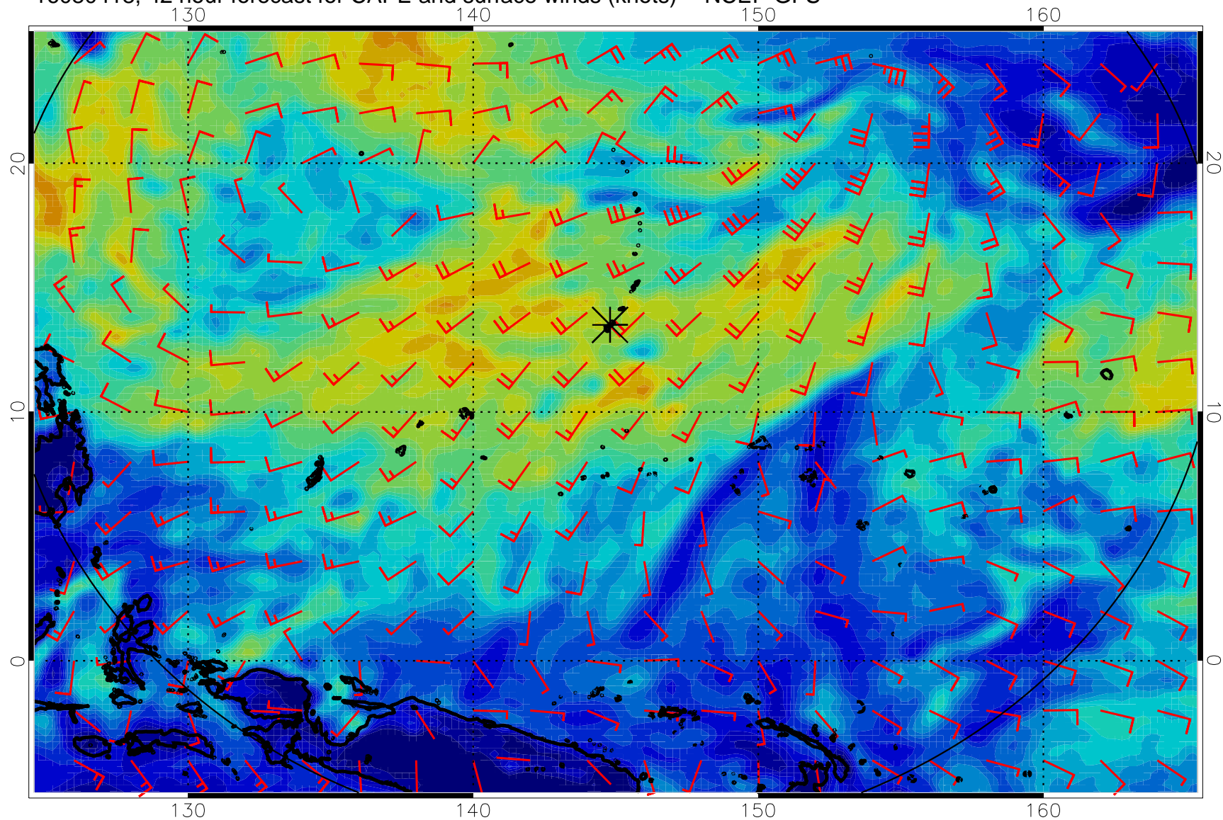
16080418, 42 hour forecast for CAPE and surface winds (knots) -- NCEP GFS
