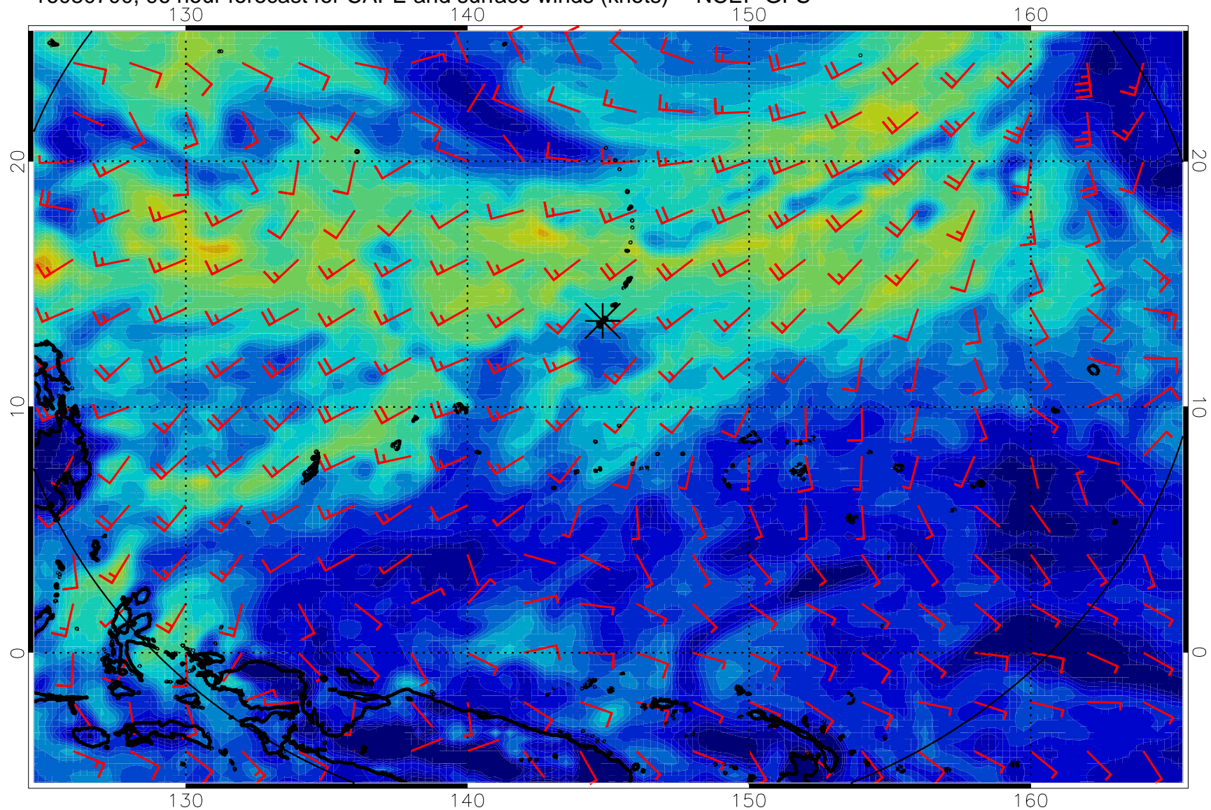
16080700, 96 hour forecast for CAPE and surface winds (knots) -- NCEP GFS
