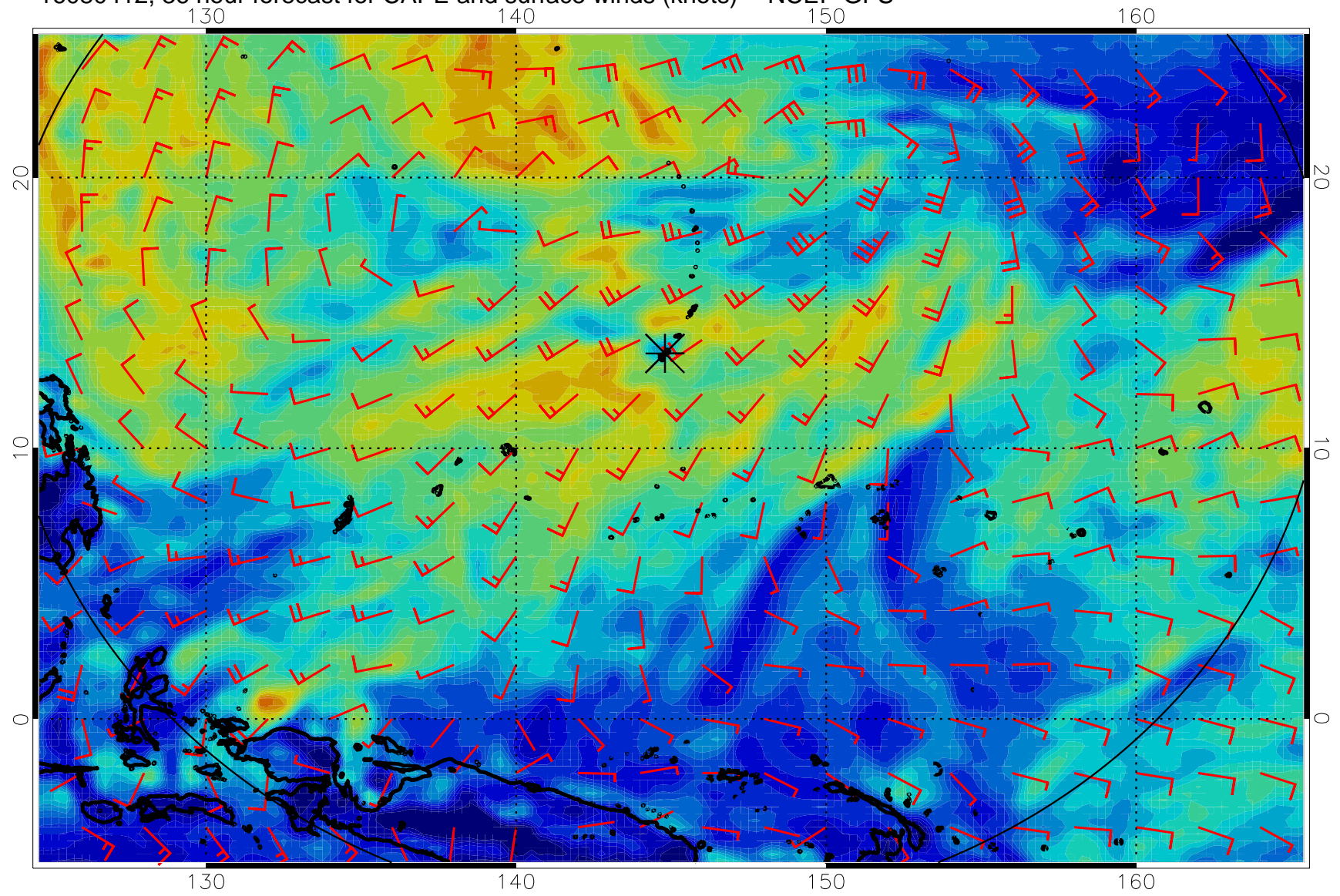
16080412, 36 hour forecast for CAPE and surface winds (knots) -- NCEP GFS
