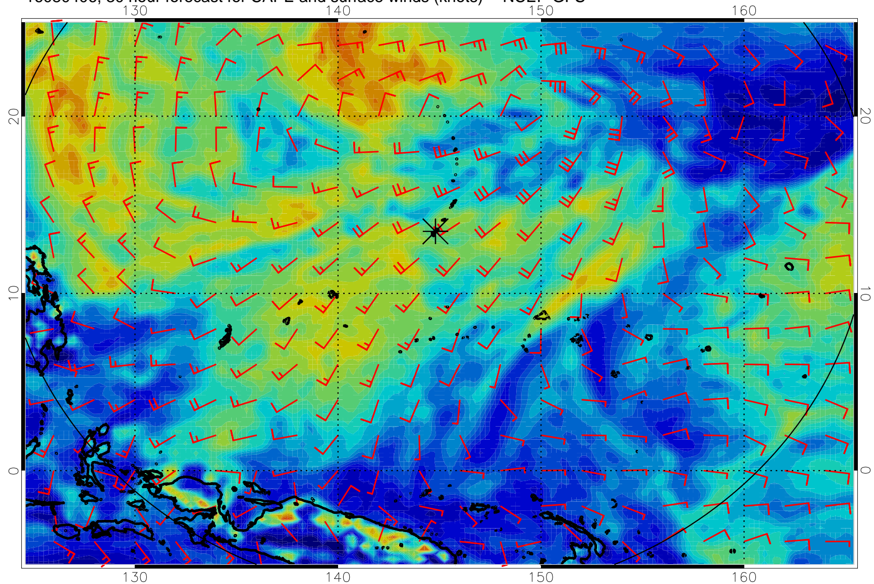
16080406, 30 hour forecast for CAPE and surface winds (knots) -- NCEP GFS
