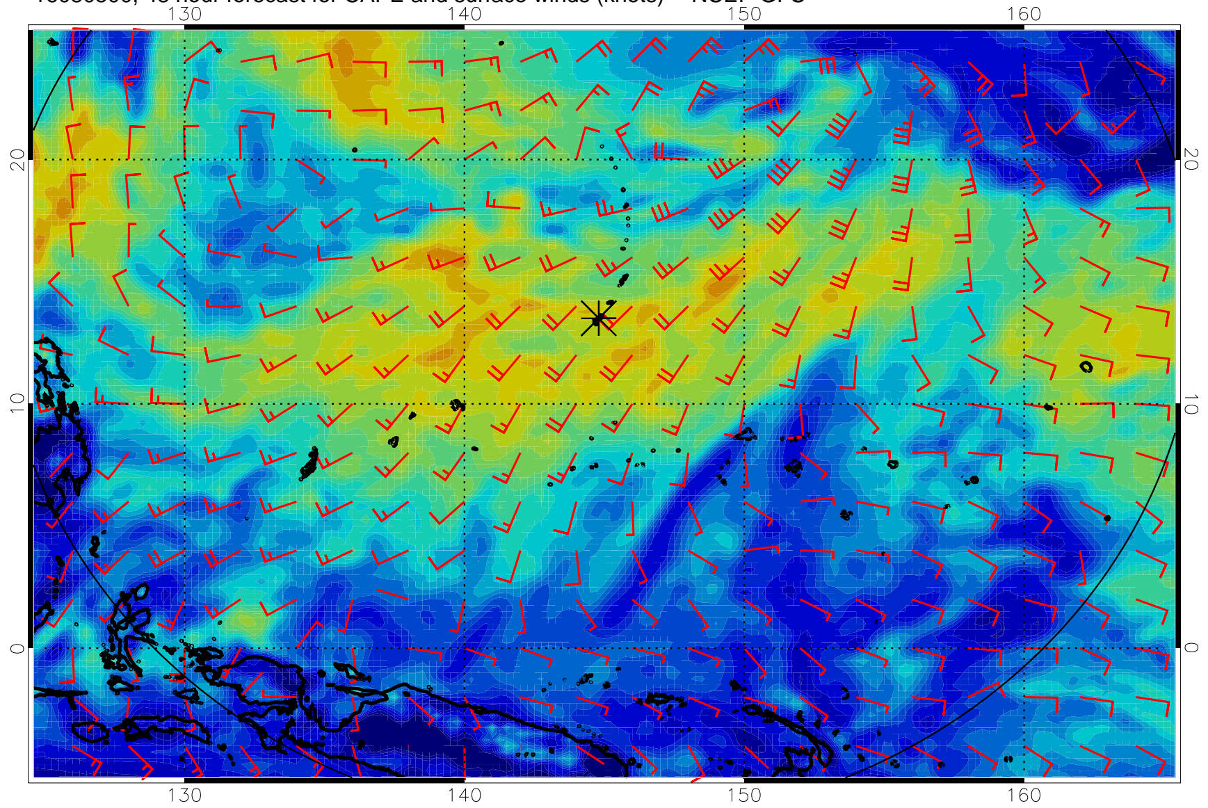
16080500, 48 hour forecast for CAPE and surface winds (knots) -- NCEP GFS
