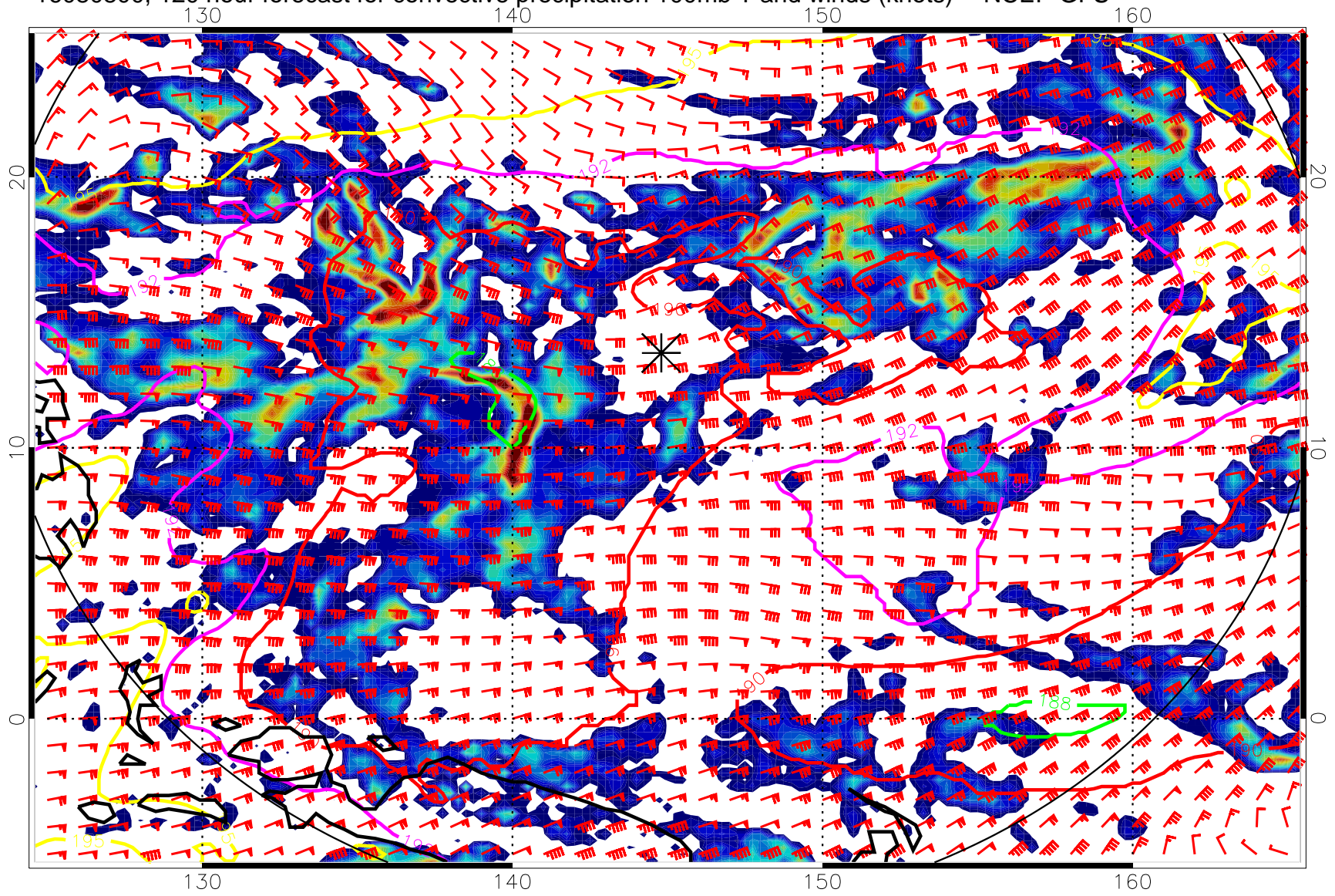
16080800, 120 hour forecast for convective precipitation 100mb T and winds (knots) -- NCEP GFS
