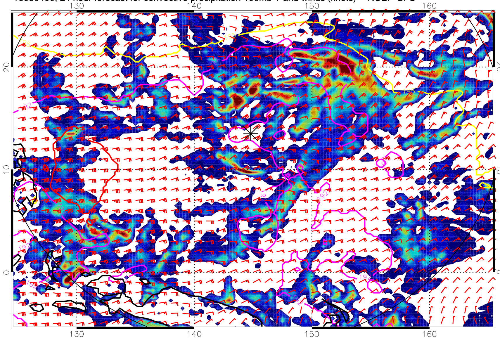
16080400, 24 hour forecast for convective precipitation 100mb T and winds (knots) -- NCEP GFS
