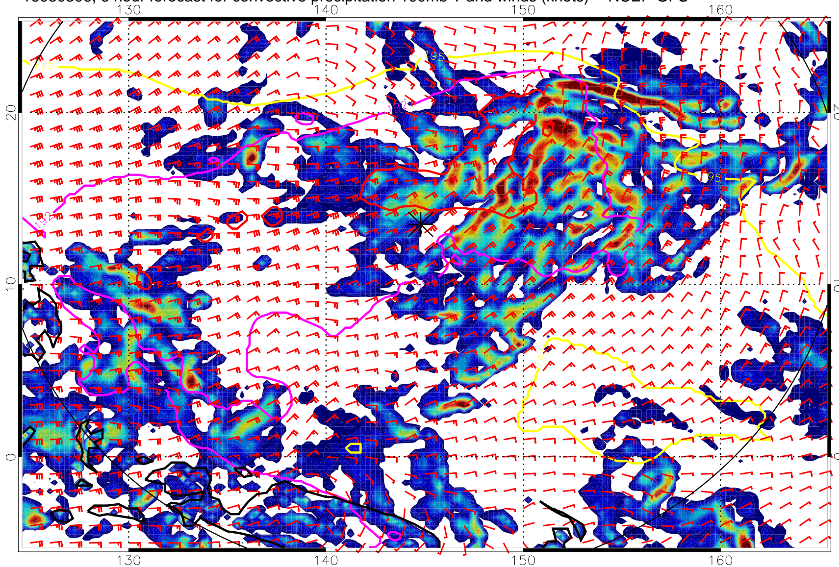
16080306, 6 hour forecast for convective precipitation 100mb T and winds (knots) -- NCEP GFS
