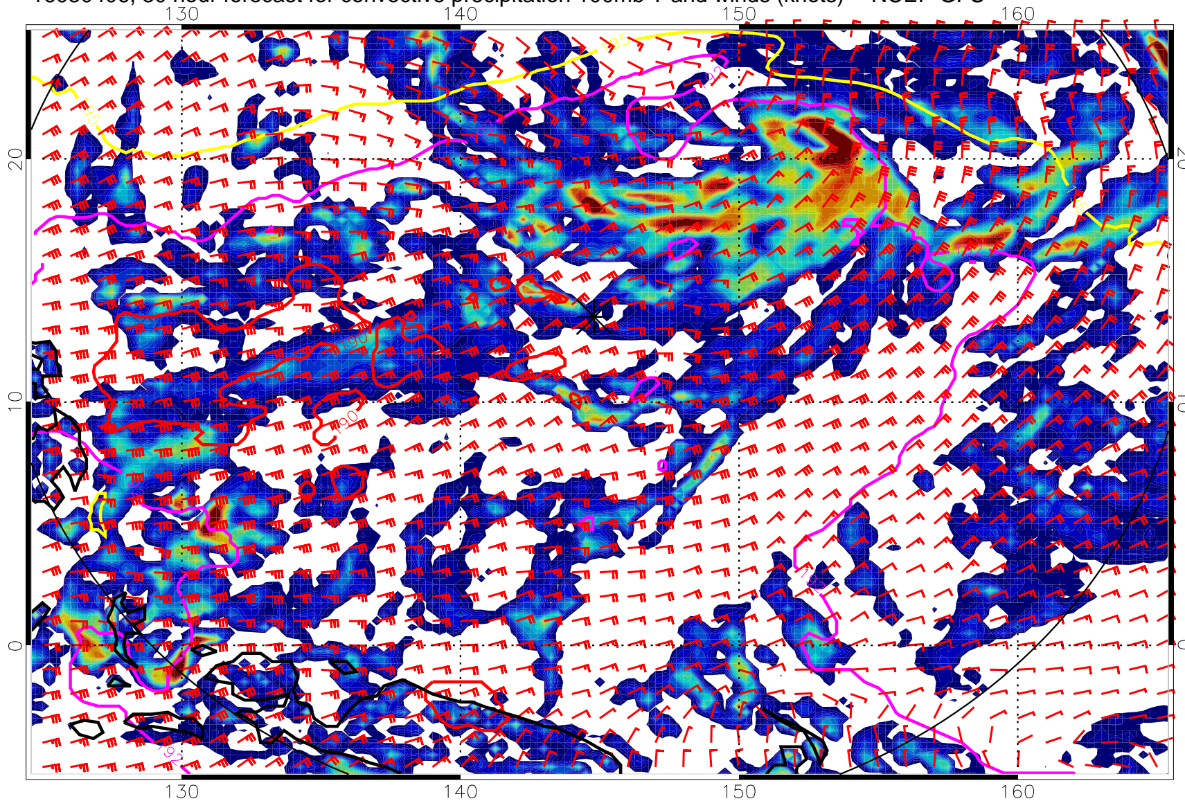
16080406, 30 hour forecast for convective precipitation 100mb T and winds (knots) -- NCEP GFS
