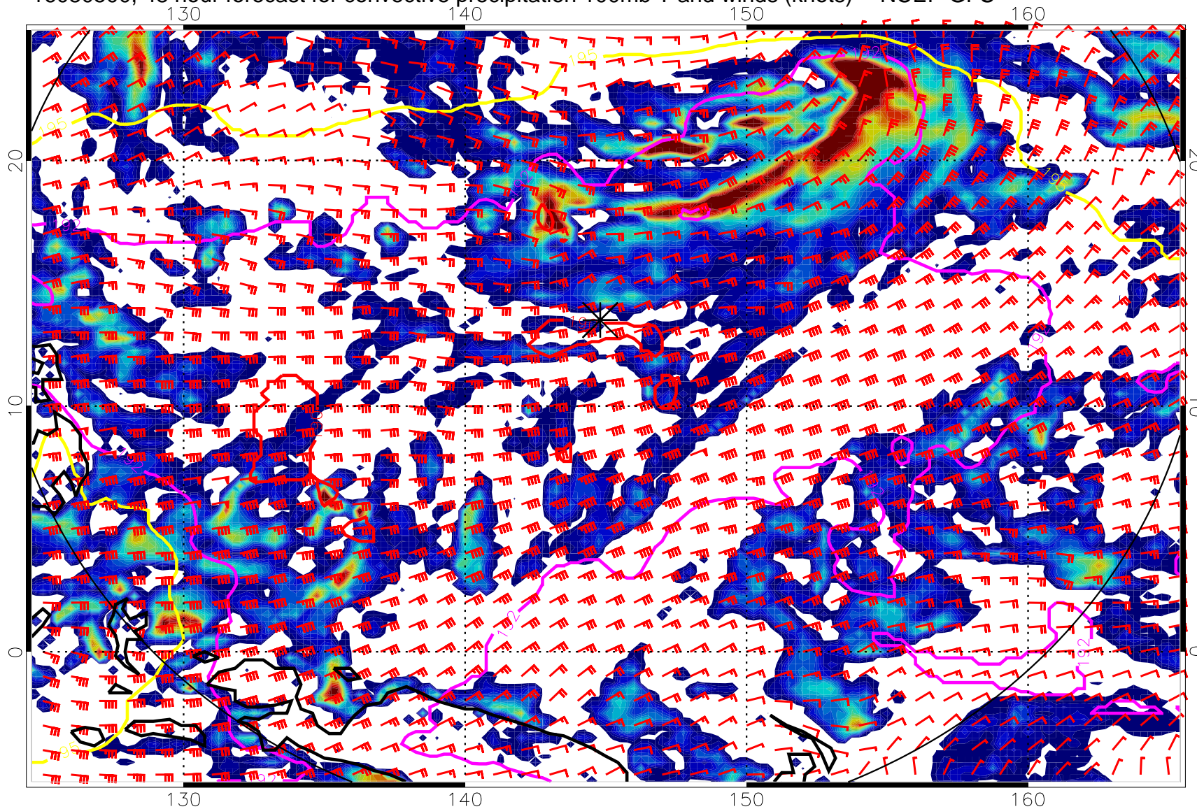
16080500, 48 hour forecast for convective precipitation 100mb T and winds (knots) -- NCEP GFS
