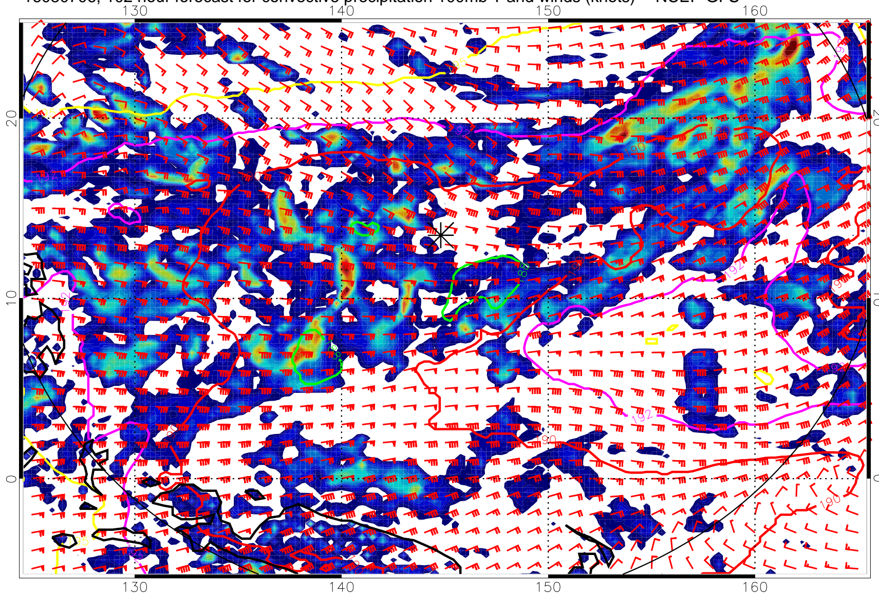
16080706, 102 hour forecast for convective precipitation 100mb T and winds (knots) -- NCEP GFS
