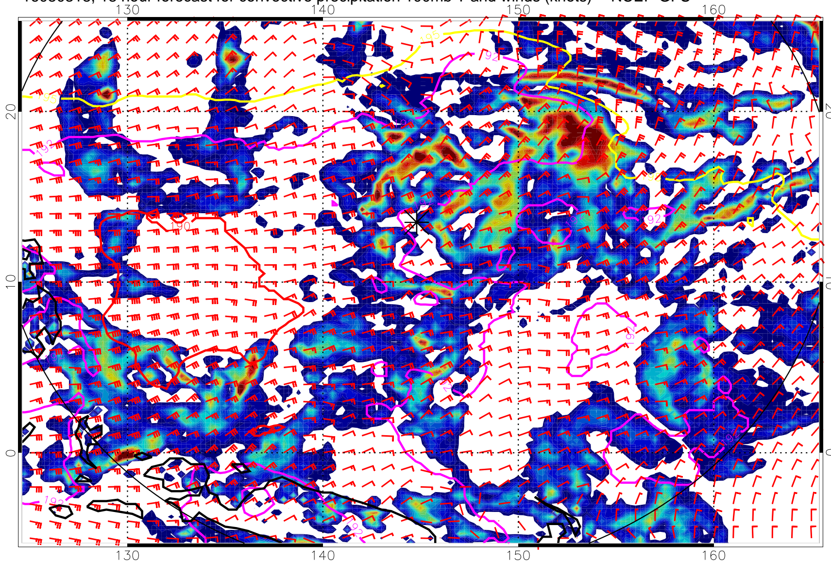
16080318, 18 hour forecast for convective precipitation 100mb T and winds (knots) -- NCEP GFS
