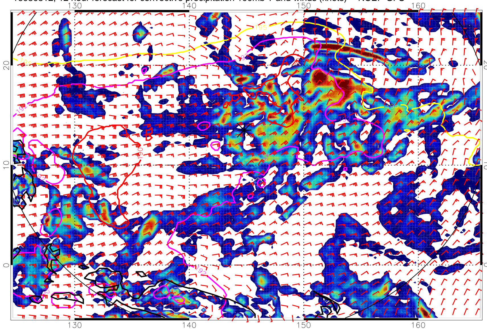
16080312, 12 hour forecast for convective precipitation 100mb T and winds (knots) -- NCEP GFS
