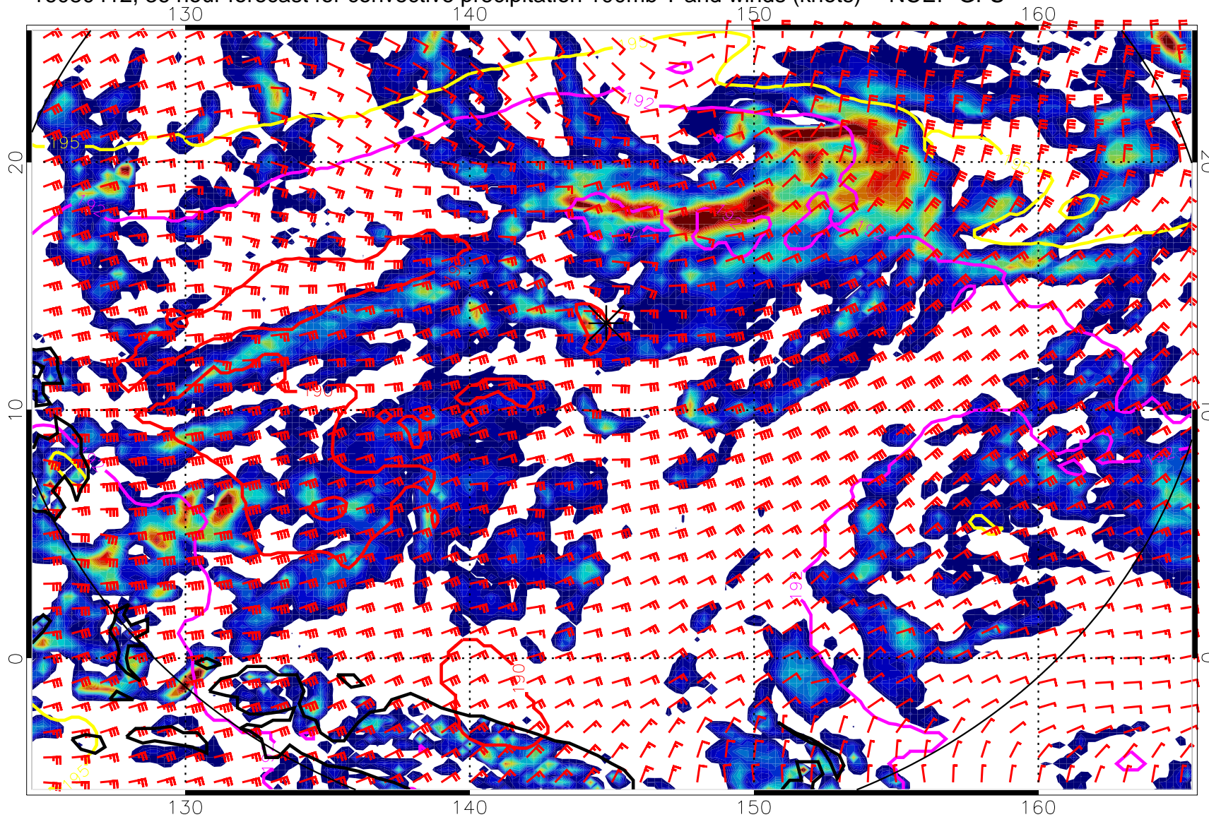
16080412, 36 hour forecast for convective precipitation 100mb T and winds (knots) -- NCEP GFS
