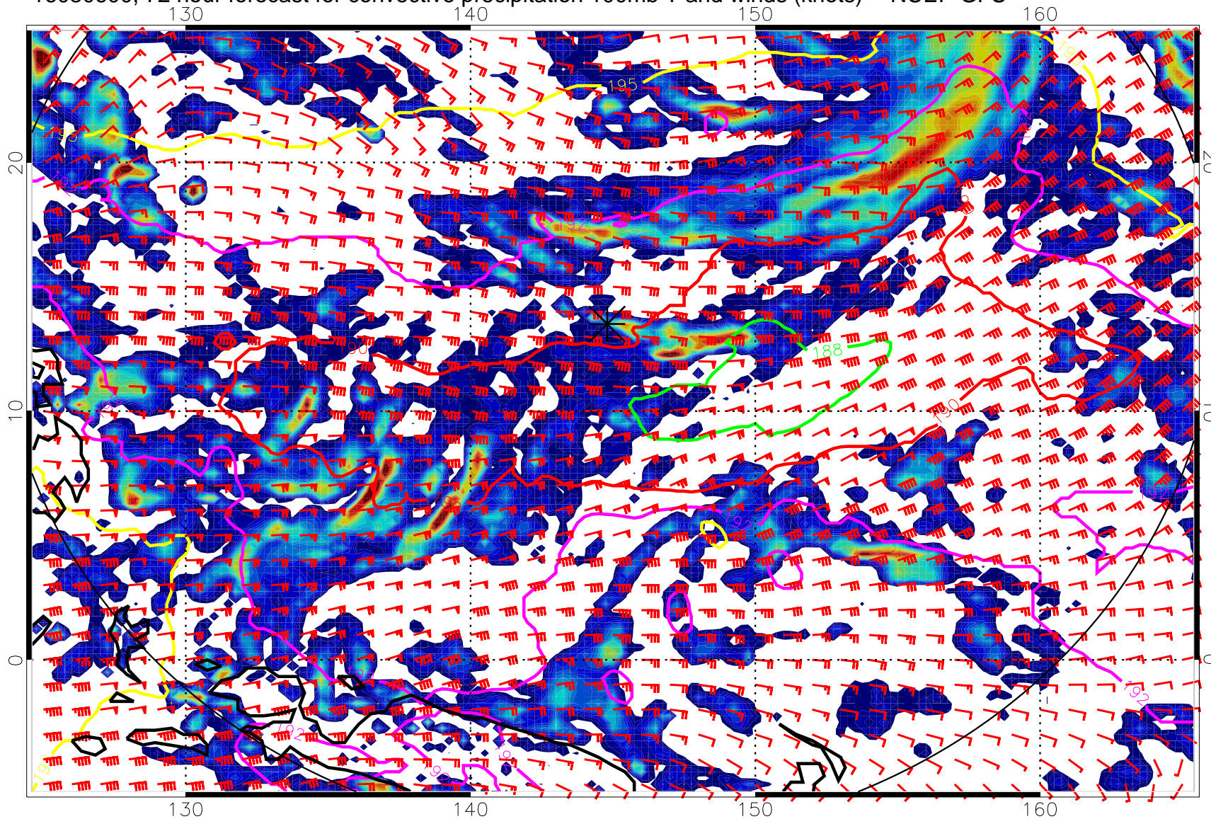
16080600, 72 hour forecast for convective precipitation 100mb T and winds (knots) -- NCEP GFS
