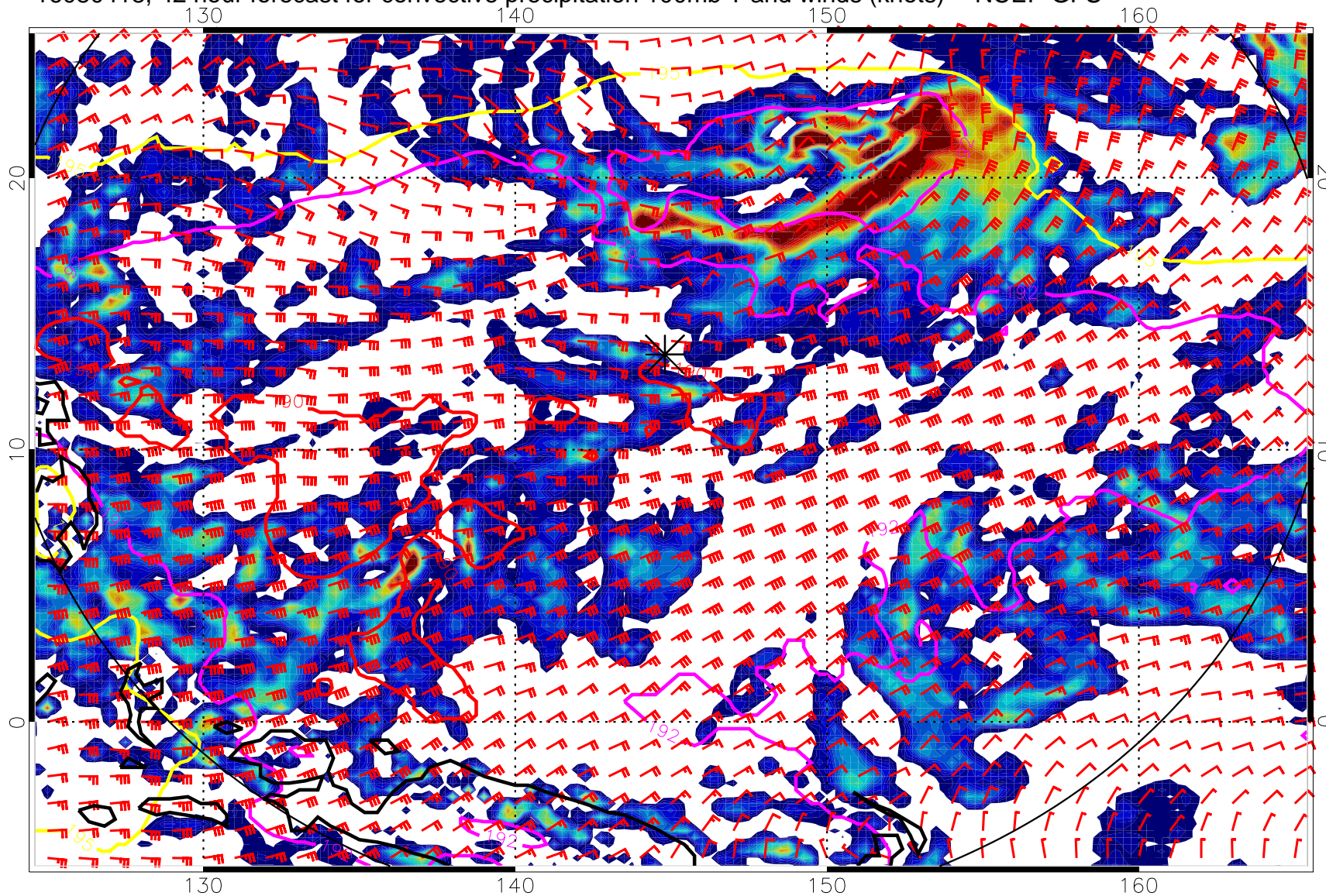
16080418, 42 hour forecast for convective precipitation 100mb T and winds (knots) -- NCEP GFS
