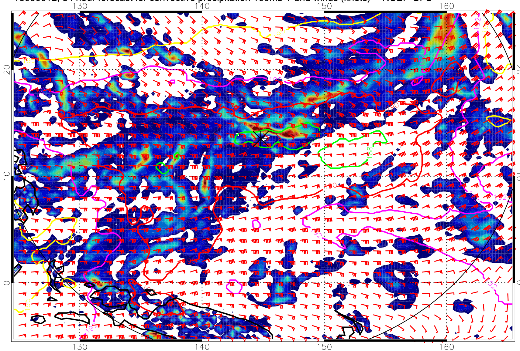
16080612, 84 hour forecast for convective precipitation 100mb T and winds (knots) -- NCEP GFS
