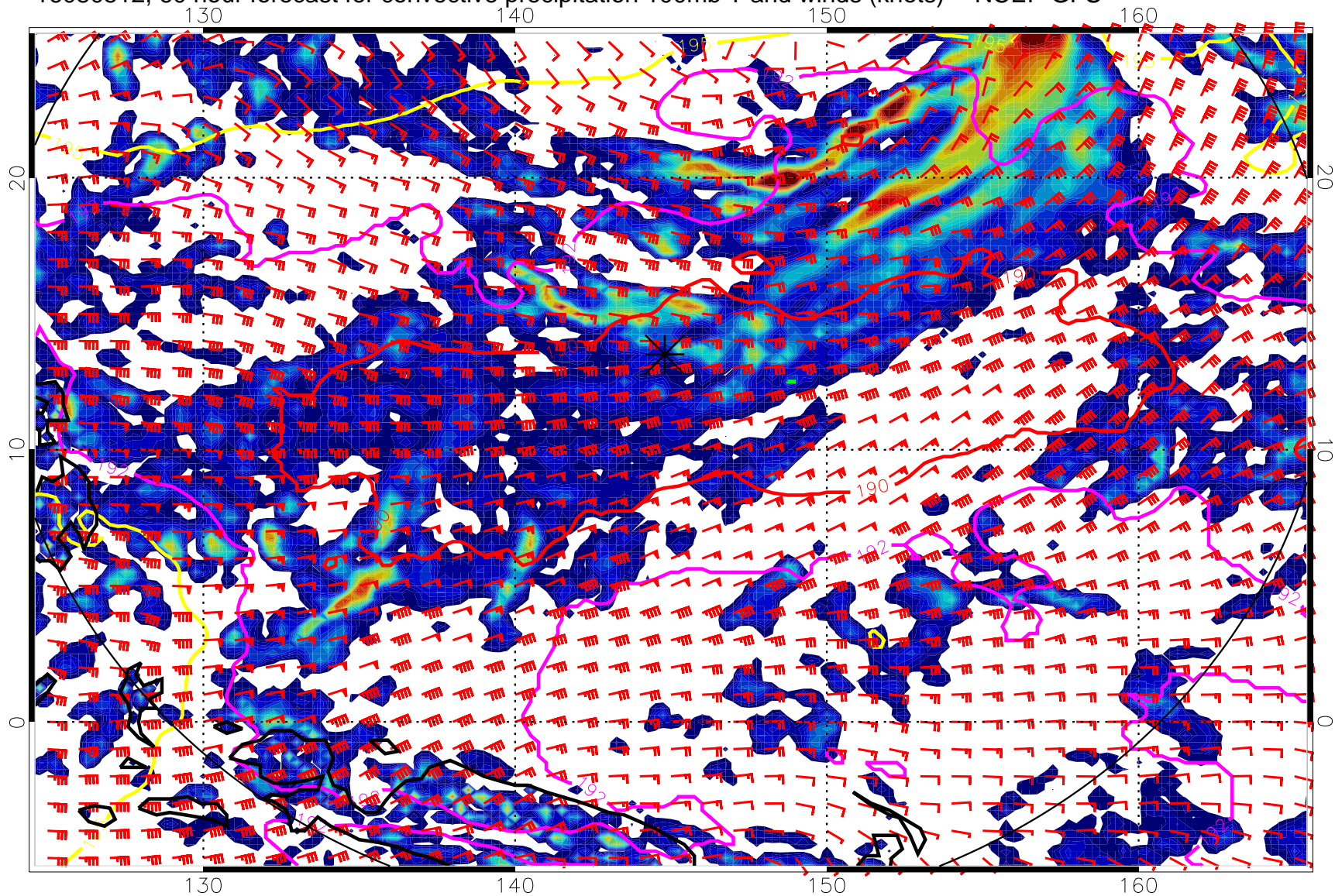
16080512, 60 hour forecast for convective precipitation 100mb T and winds (knots) -- NCEP GFS
