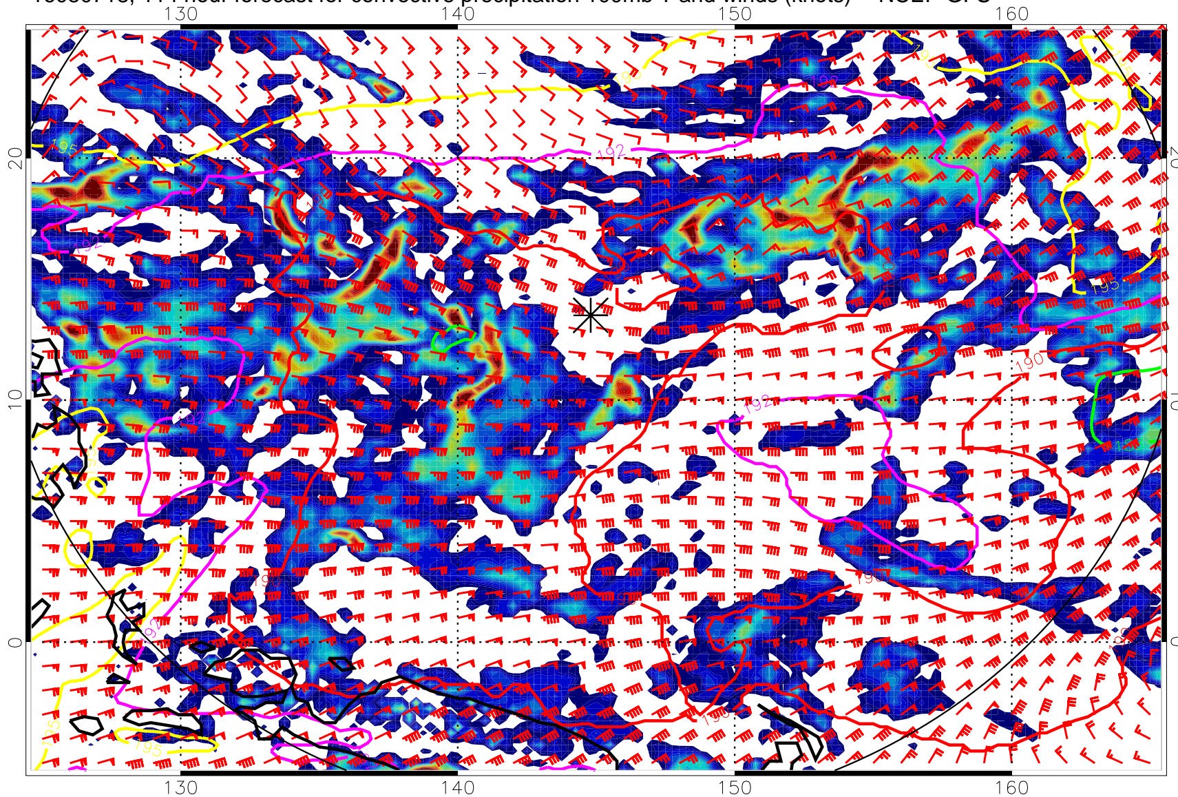
16080718, 114 hour forecast for convective precipitation 100mb T and winds (knots) -- NCEP GFS
