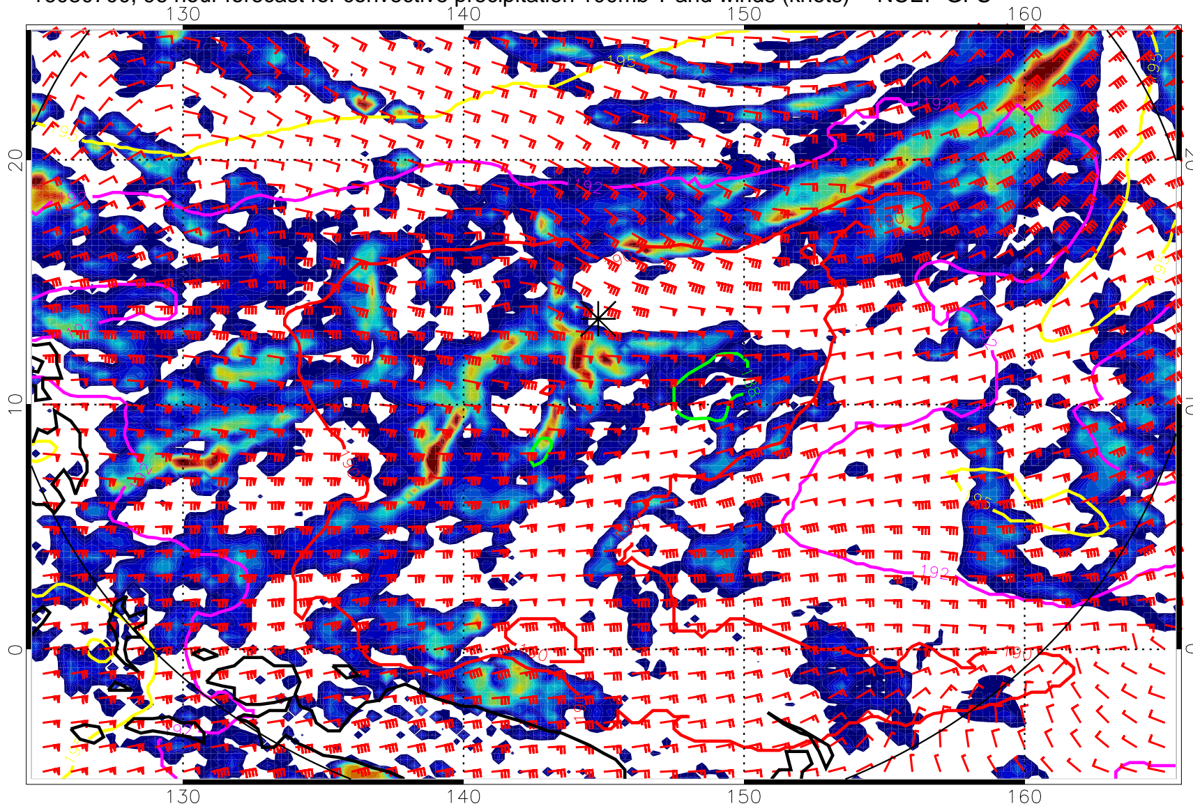
16080700, 96 hour forecast for convective precipitation 100mb T and winds (knots) -- NCEP GFS
