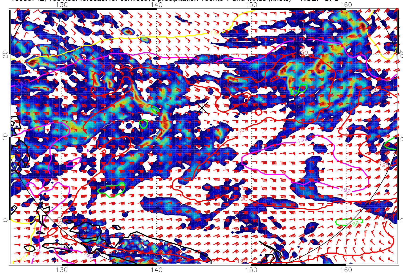
16080712, 108 hour forecast for convective precipitation 100mb T and winds (knots) -- NCEP GFS
