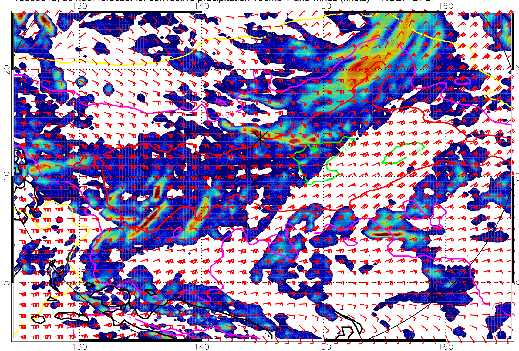
16080518, 66 hour forecast for convective precipitation 100mb T and winds (knots) -- NCEP GFS
