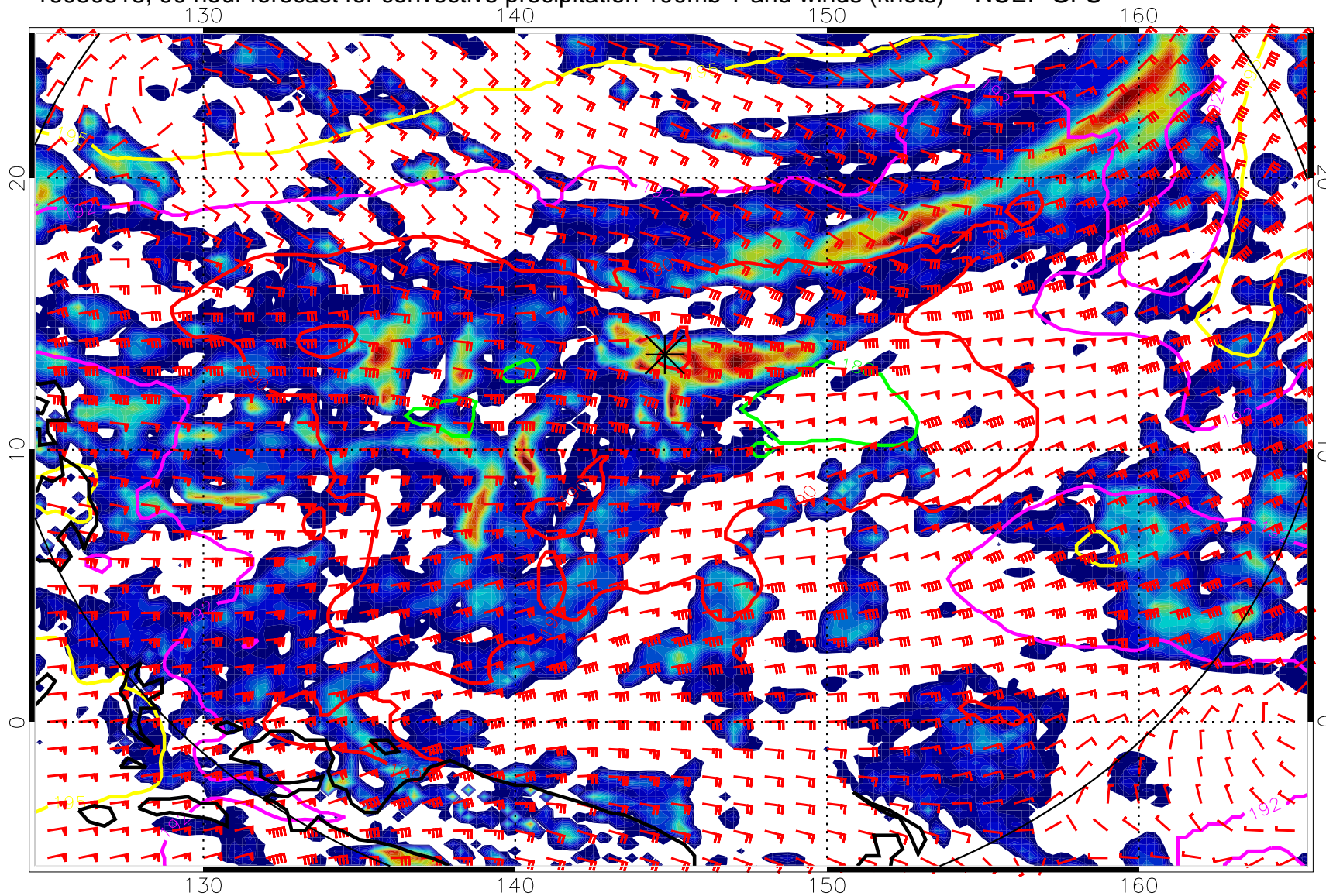
16080618, 90 hour forecast for convective precipitation 100mb T and winds (knots) -- NCEP GFS
