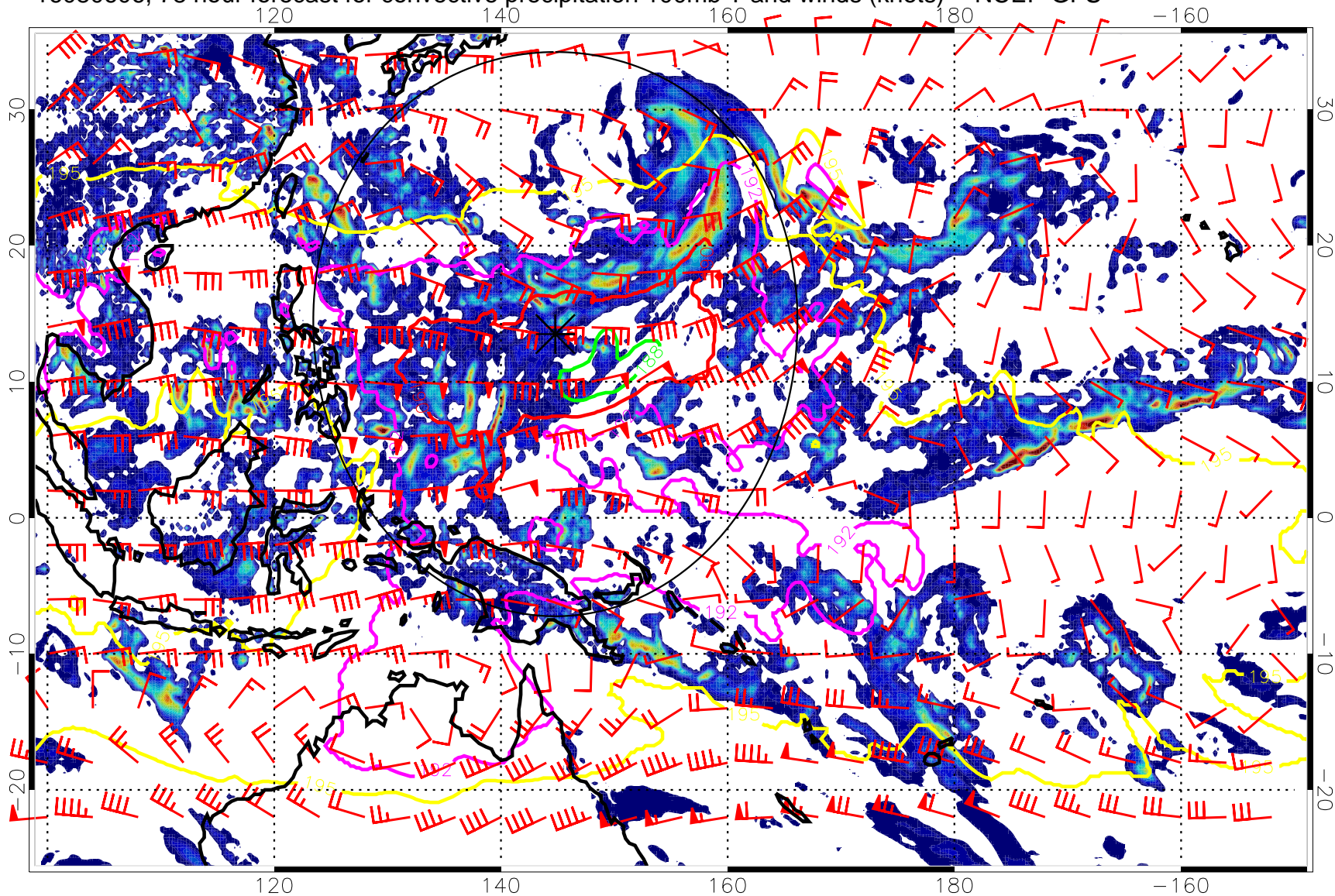
16080606, 78 hour forecast for convective precipitation 100mb T and winds (knots) -- NCEP GFS
