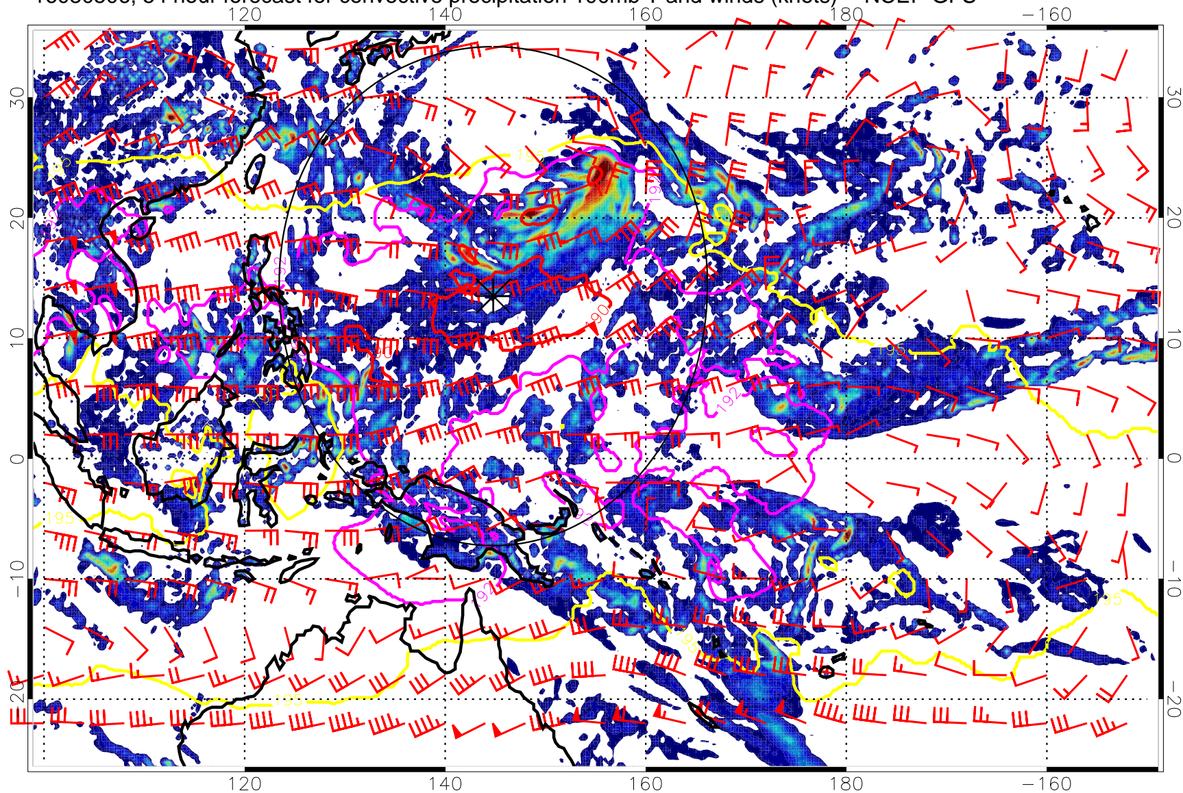
16080506, 54 hour forecast for convective precipitation 100mb T and winds (knots) -- NCEP GFS
