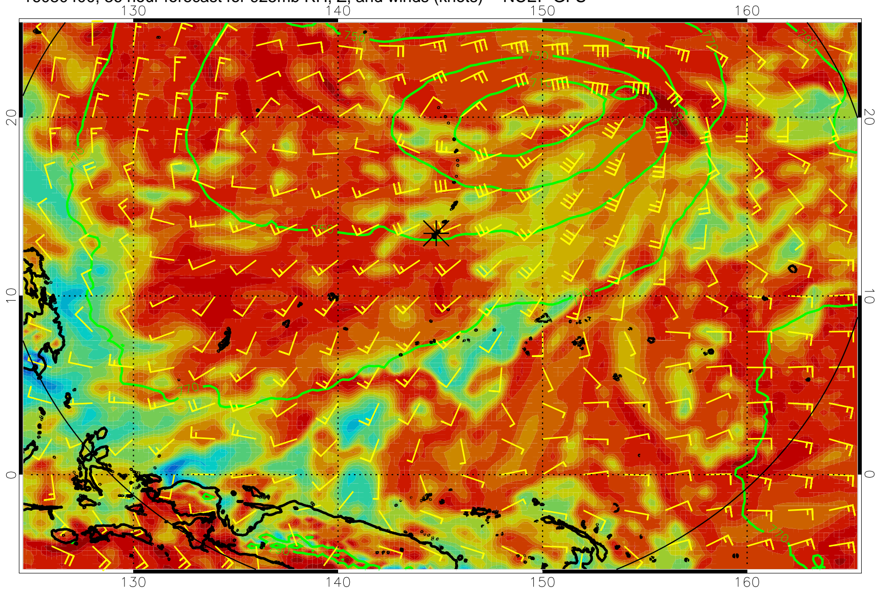
16080400, 36 hour forecast for 925mb RH, Z, and winds (knots) -- NCEP GFS
