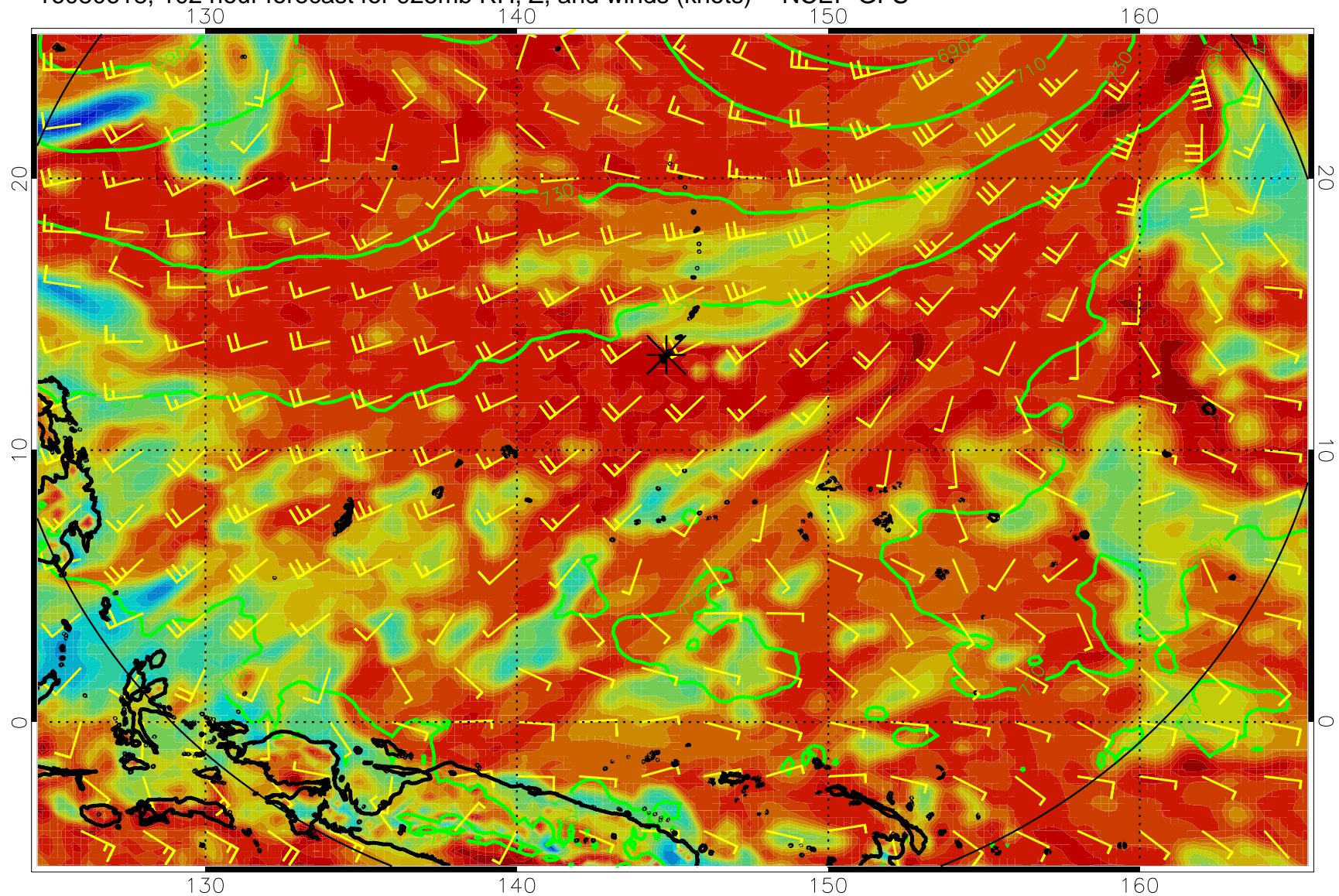
16080618, 102 hour forecast for 925mb RH, Z, and winds (knots) -- NCEP GFS
