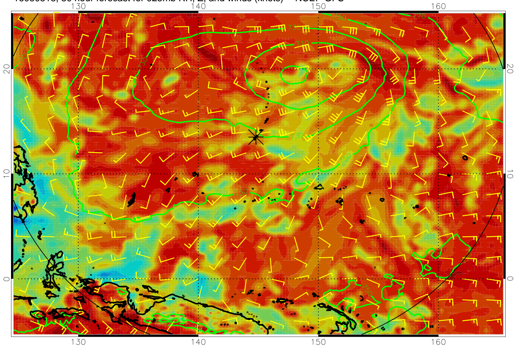
16080318, 30 hour forecast for 925mb RH, Z, and winds (knots) -- NCEP GFS
