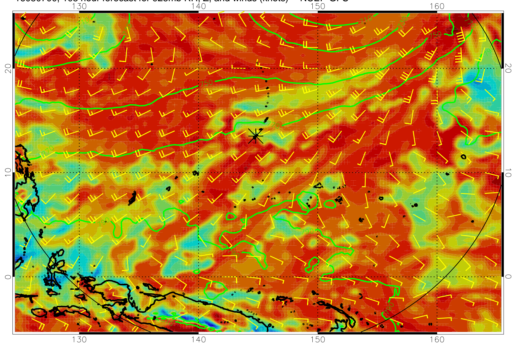
16080700, 108 hour forecast for 925mb RH, Z, and winds (knots) -- NCEP GFS
