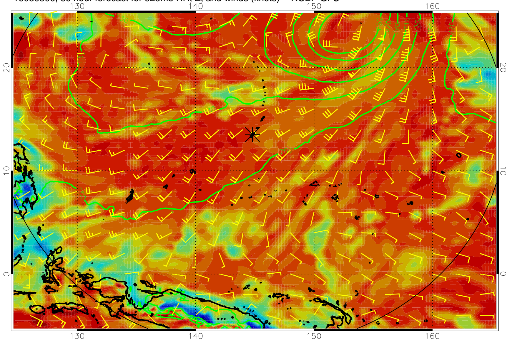
16080506, 66 hour forecast for 925mb RH, Z, and winds (knots) -- NCEP GFS
