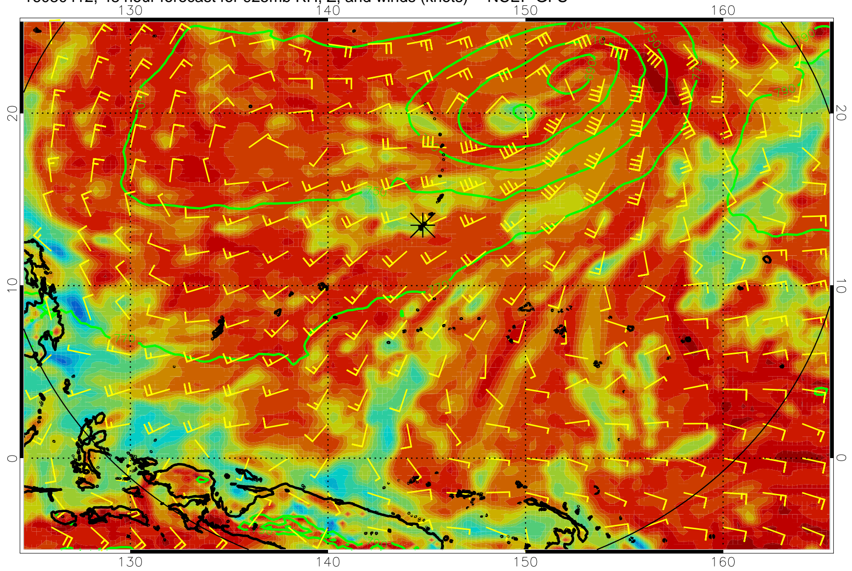
16080412, 48 hour forecast for 925mb RH, Z, and winds (knots) -- NCEP GFS
