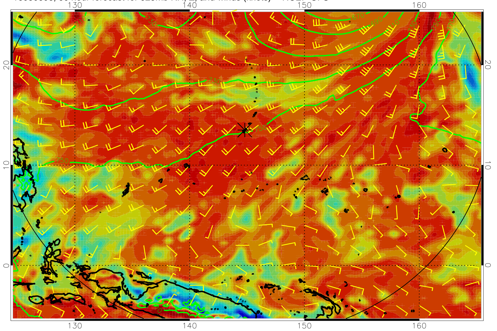
16080606, 90 hour forecast for 925mb RH, Z, and winds (knots) -- NCEP GFS
