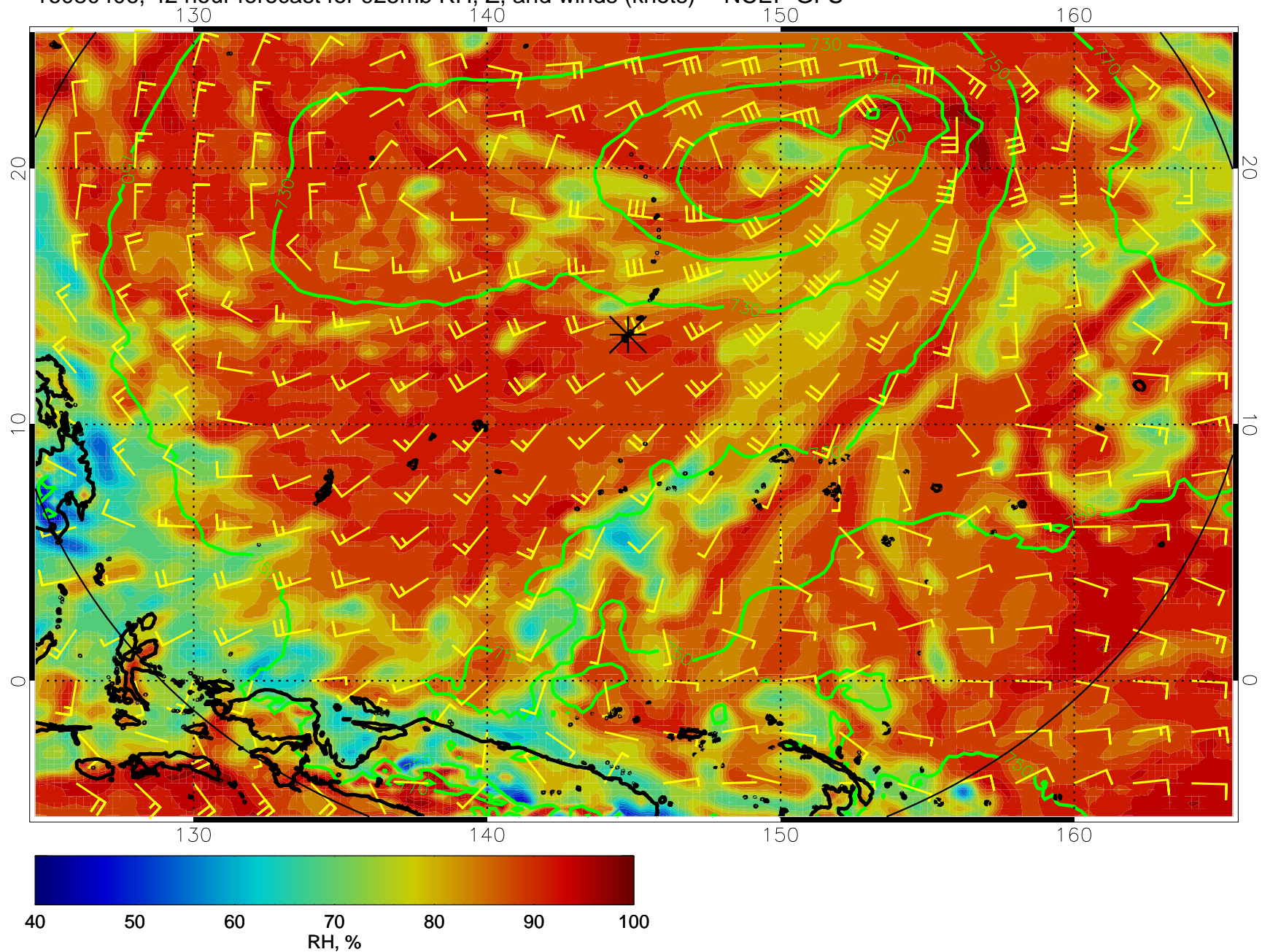
16080406, 42 hour forecast for 925mb RH, Z, and winds (knots) -- NCEP GFS
