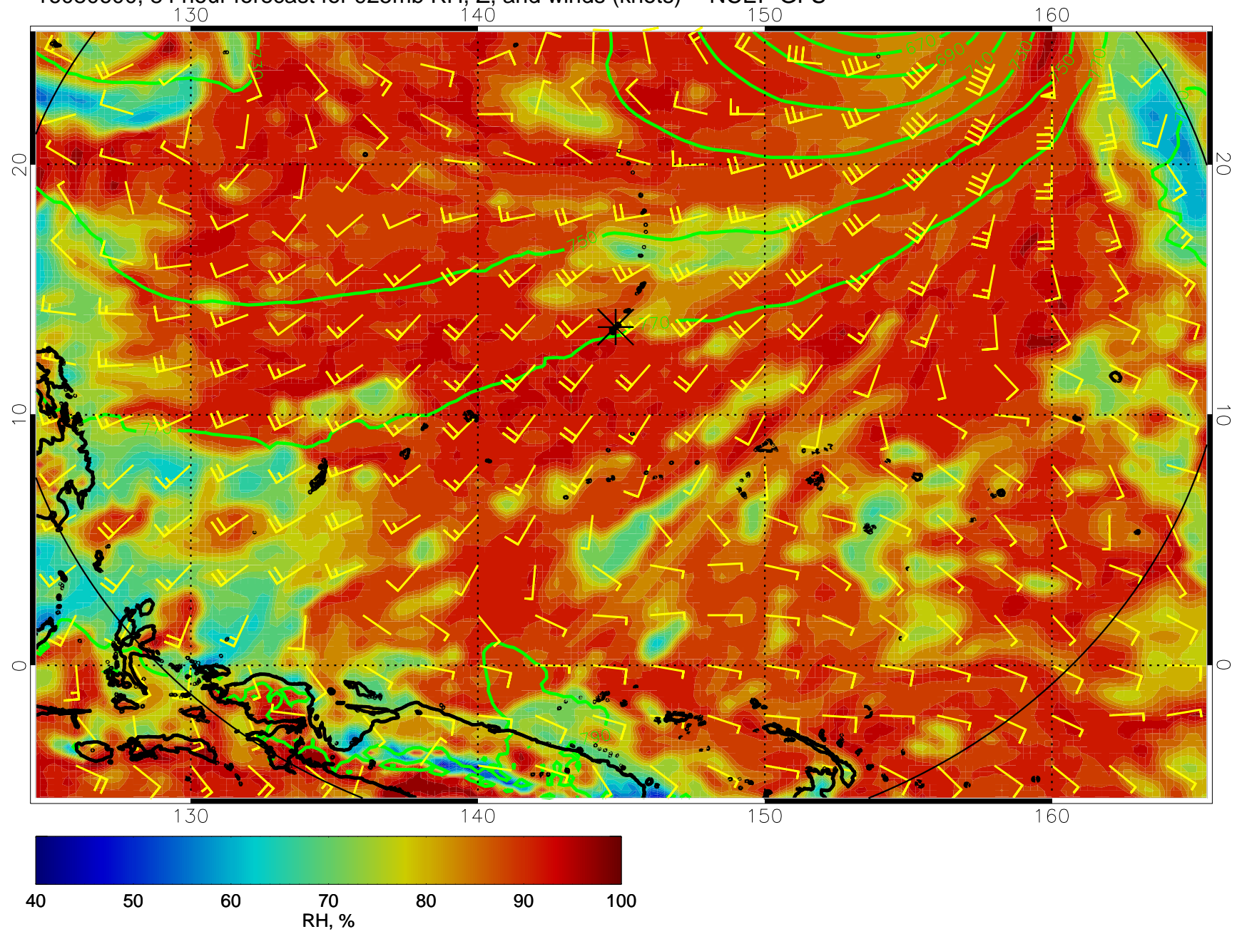
16080600, 84 hour forecast for 925mb RH, Z, and winds (knots) -- NCEP GFS
