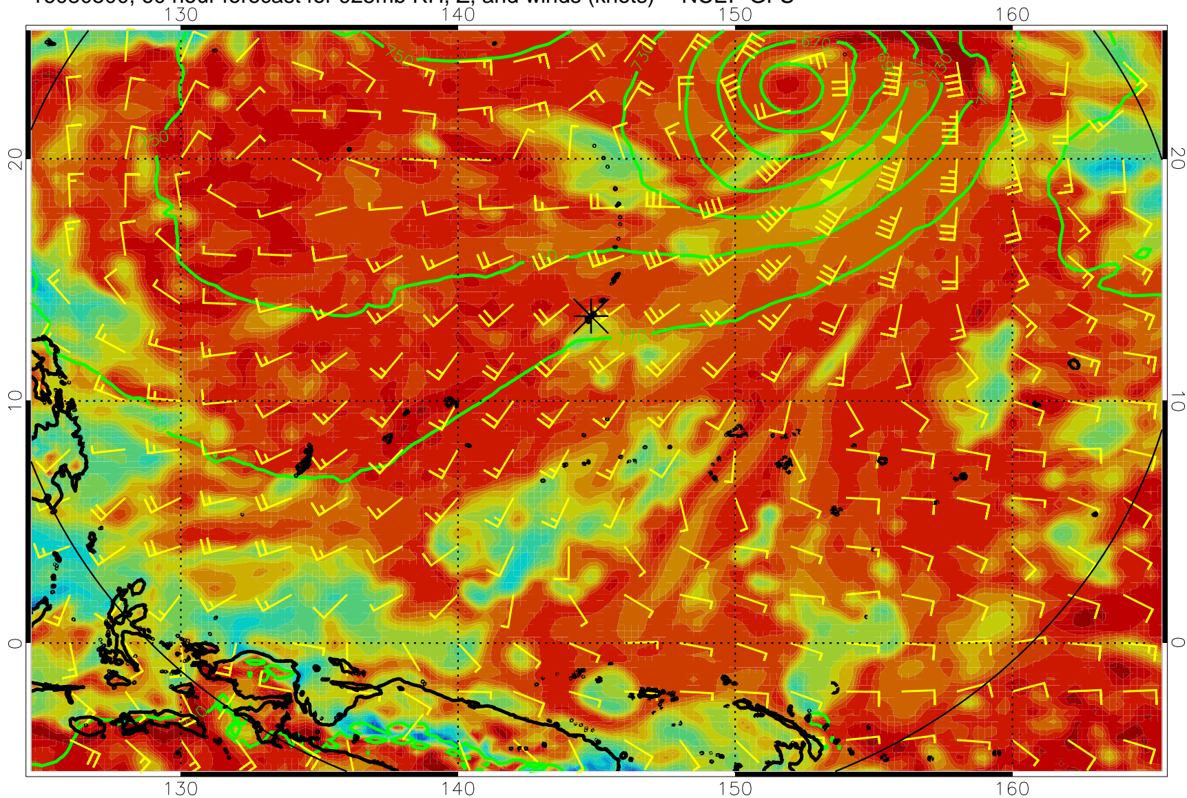
16080500, 60 hour forecast for 925mb RH, Z, and winds (knots) -- NCEP GFS
