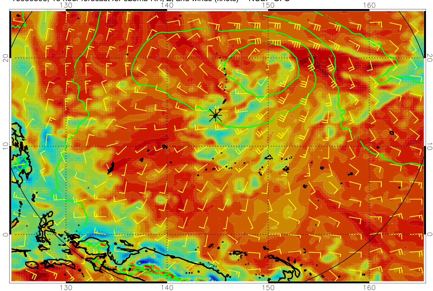
16080306, 18 hour forecast for 925mb RH, Z, and winds (knots) -- NCEP GFS
