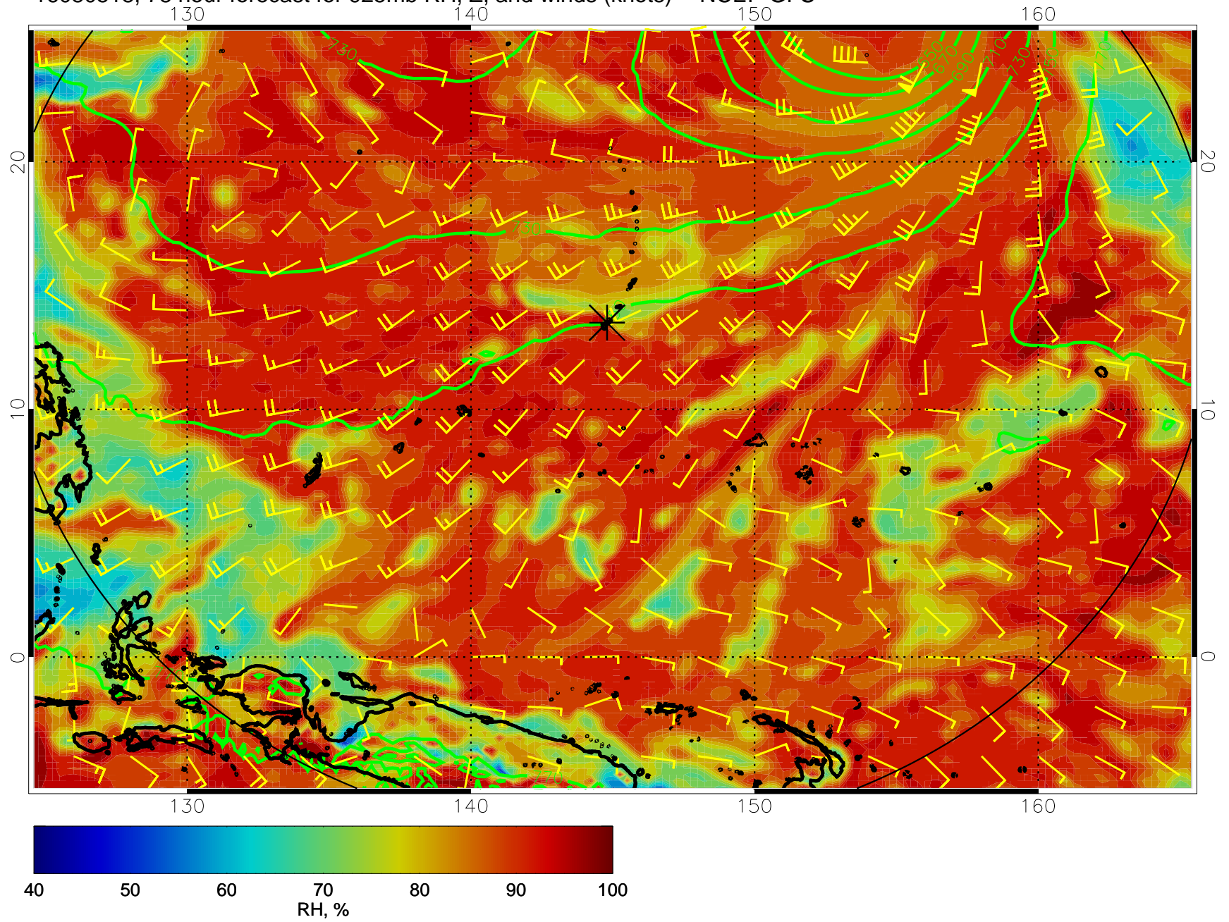
16080518, 78 hour forecast for 925mb RH, Z, and winds (knots) -- NCEP GFS
