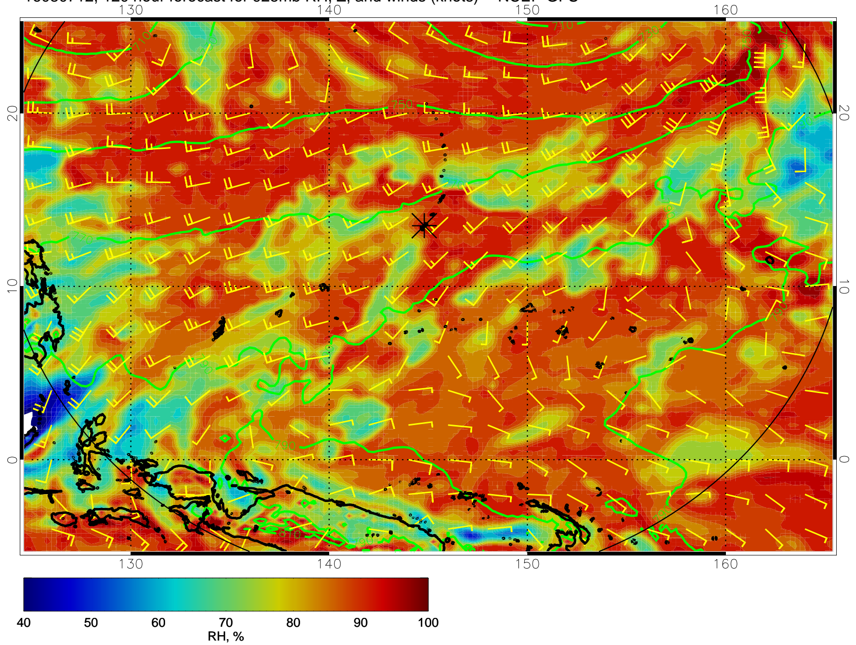
16080712, 120 hour forecast for 925mb RH, Z, and winds (knots) -- NCEP GFS
