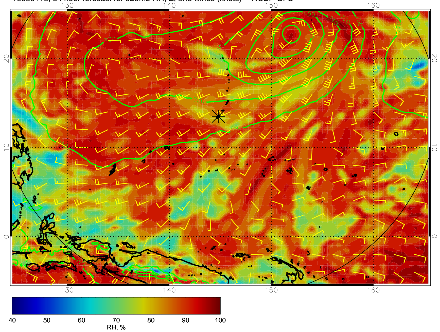
16080418, 54 hour forecast for 925mb RH, Z, and winds (knots) -- NCEP GFS
