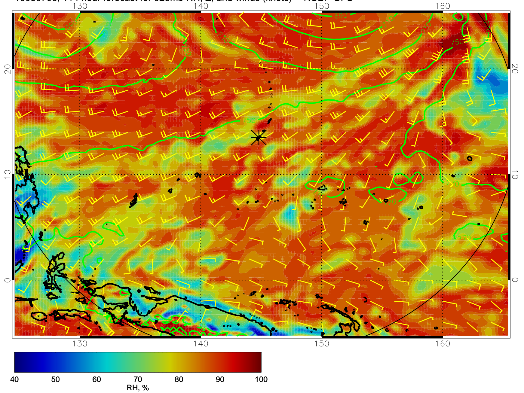
16080706, 114 hour forecast for 925mb RH, Z, and winds (knots) -- NCEP GFS
