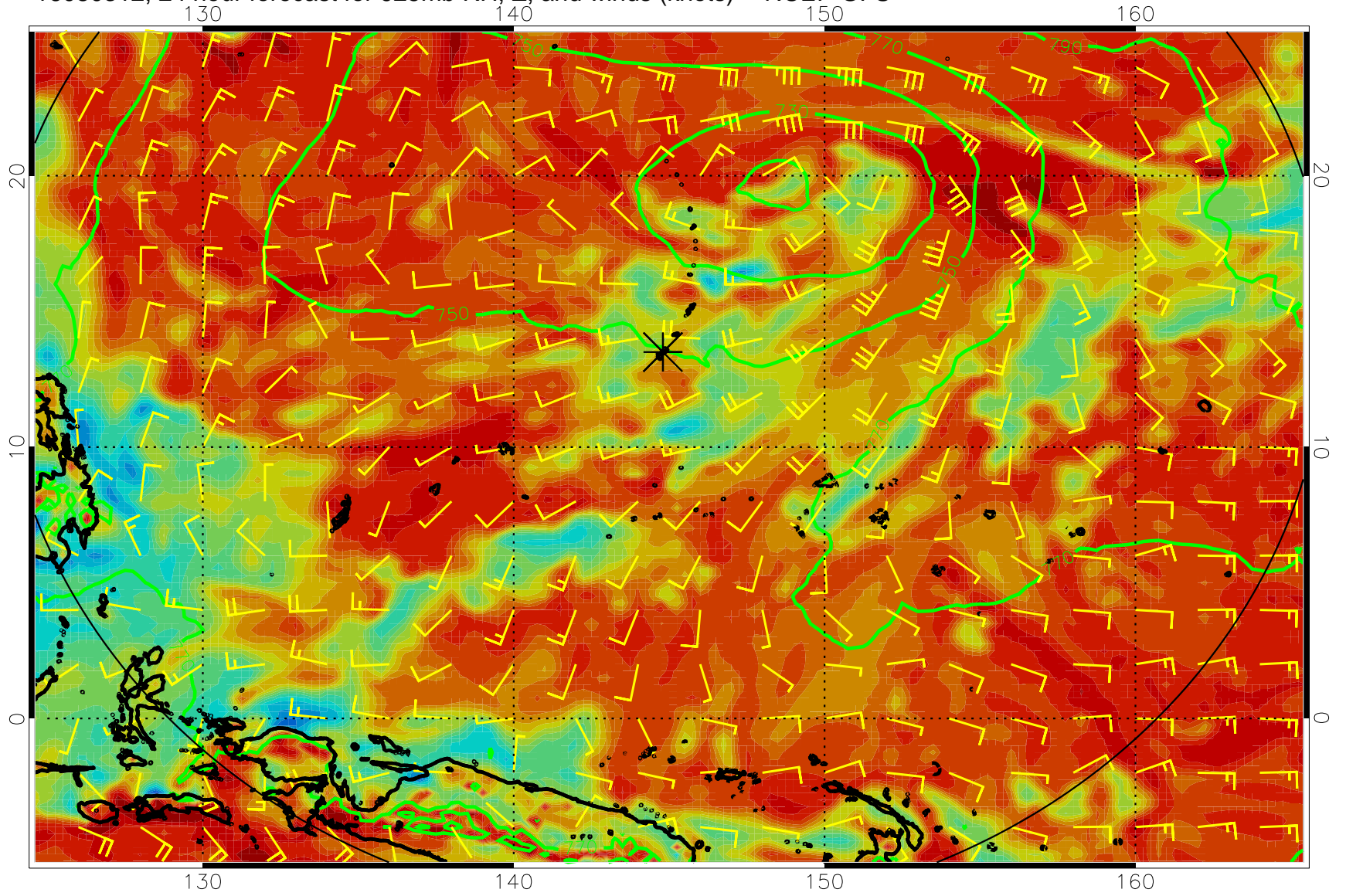
16080312, 24 hour forecast for 925mb RH, Z, and winds (knots) -- NCEP GFS
