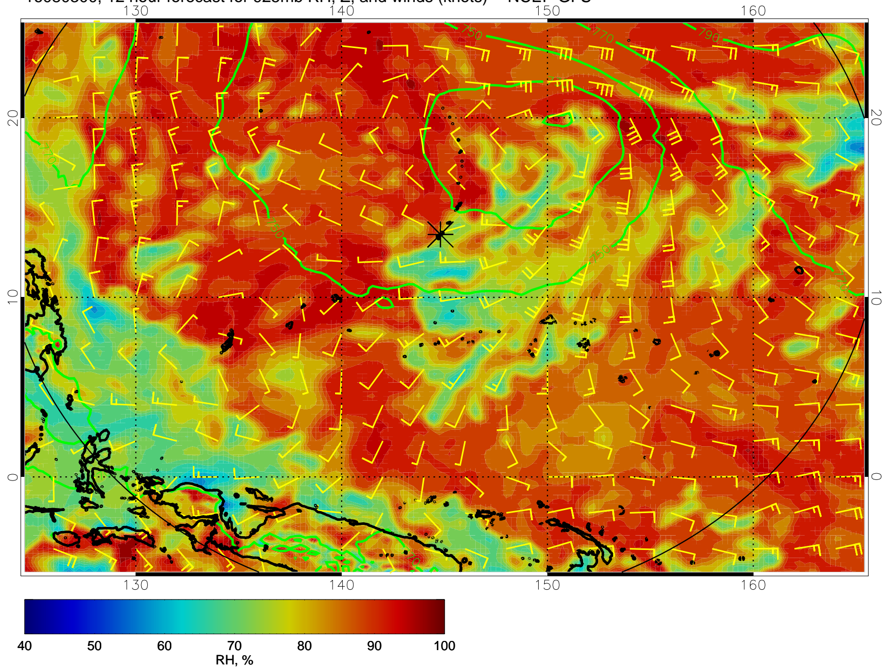
16080300, 12 hour forecast for 925mb RH, Z, and winds (knots) -- NCEP GFS
