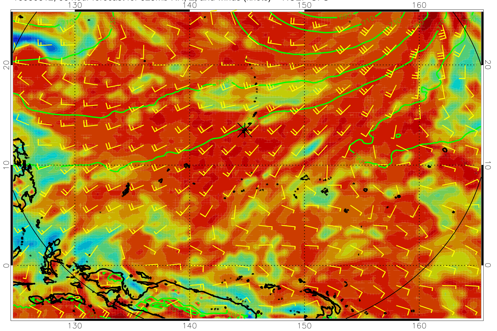
16080612, 96 hour forecast for 925mb RH, Z, and winds (knots) -- NCEP GFS
