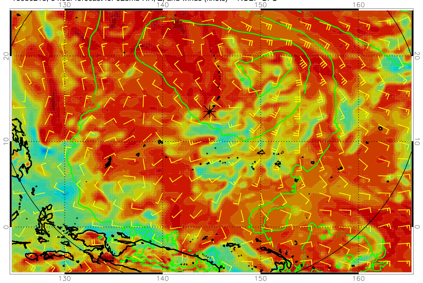
16080218, 6 hour forecast for 925mb RH, Z, and winds (knots) -- NCEP GFS
