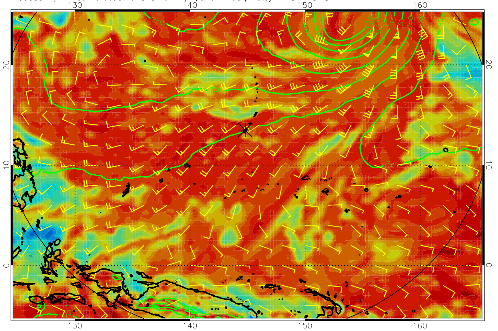
16080512, 72 hour forecast for 925mb RH, Z, and winds (knots) -- NCEP GFS
