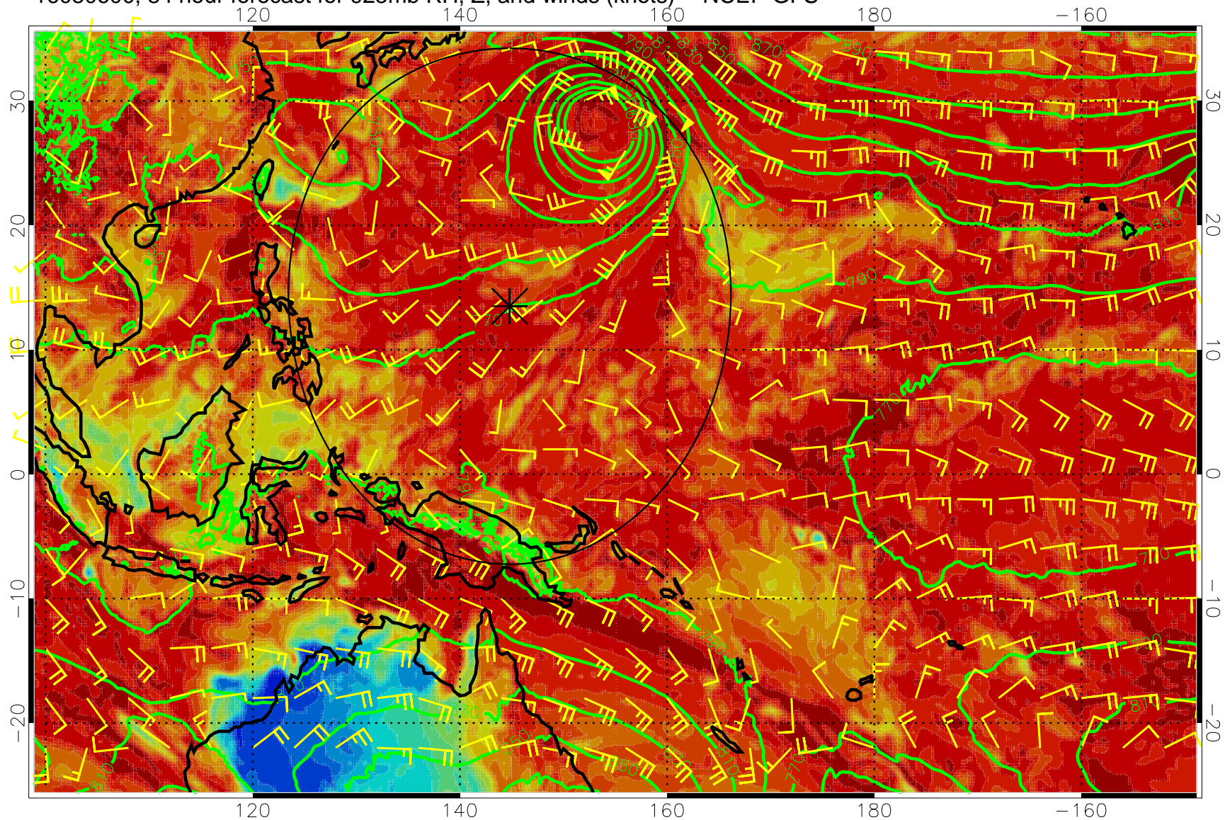
16080600, 84 hour forecast for 925mb RH, Z, and winds (knots) -- NCEP GFS
