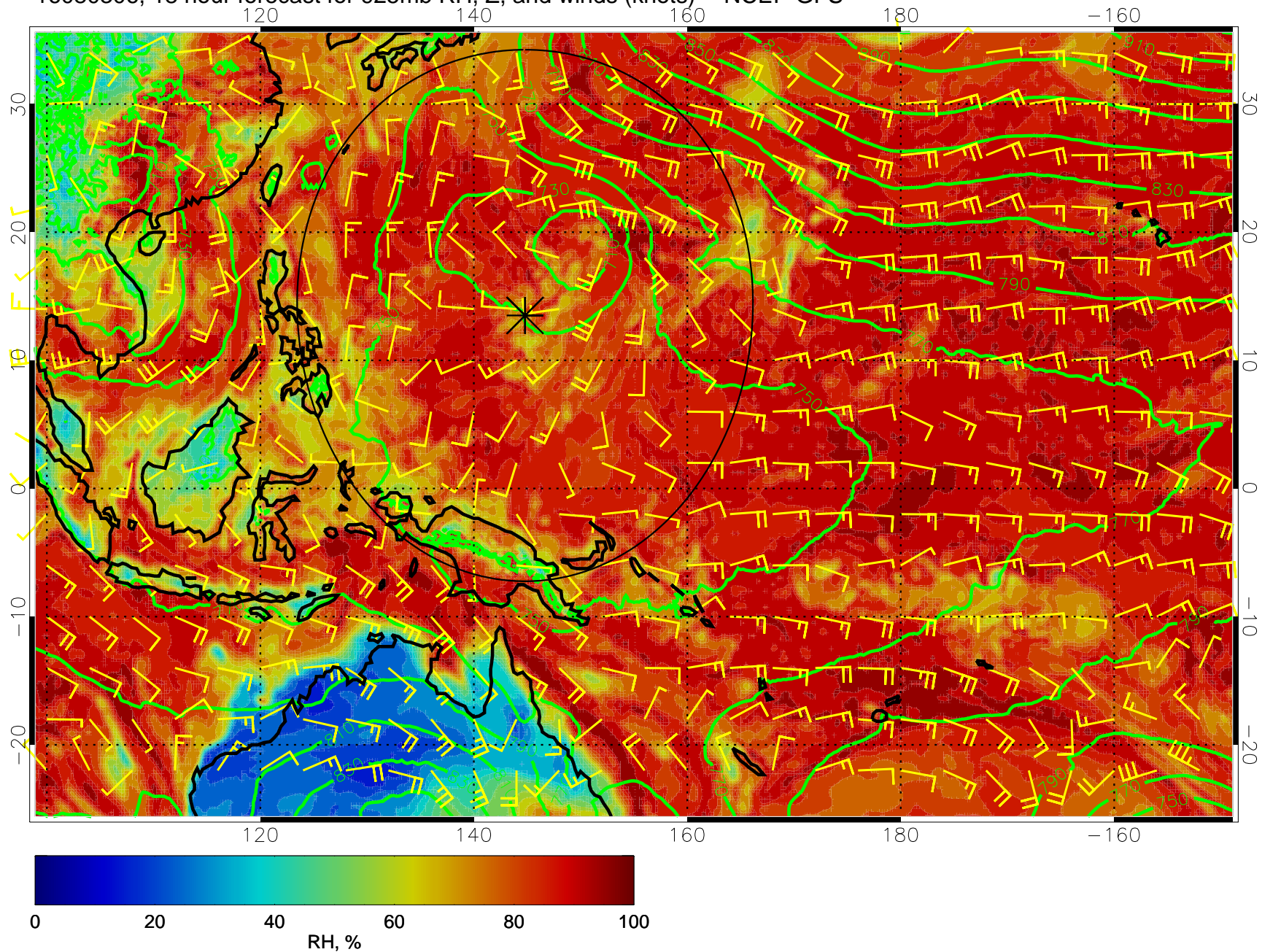
16080306, 18 hour forecast for 925mb RH, Z, and winds (knots) -- NCEP GFS
