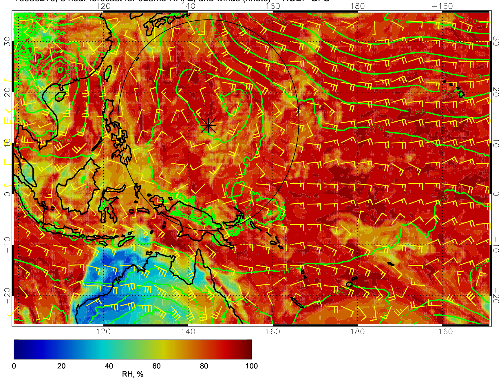
16080218, 6 hour forecast for 925mb RH, Z, and winds (knots) -- NCEP GFS
