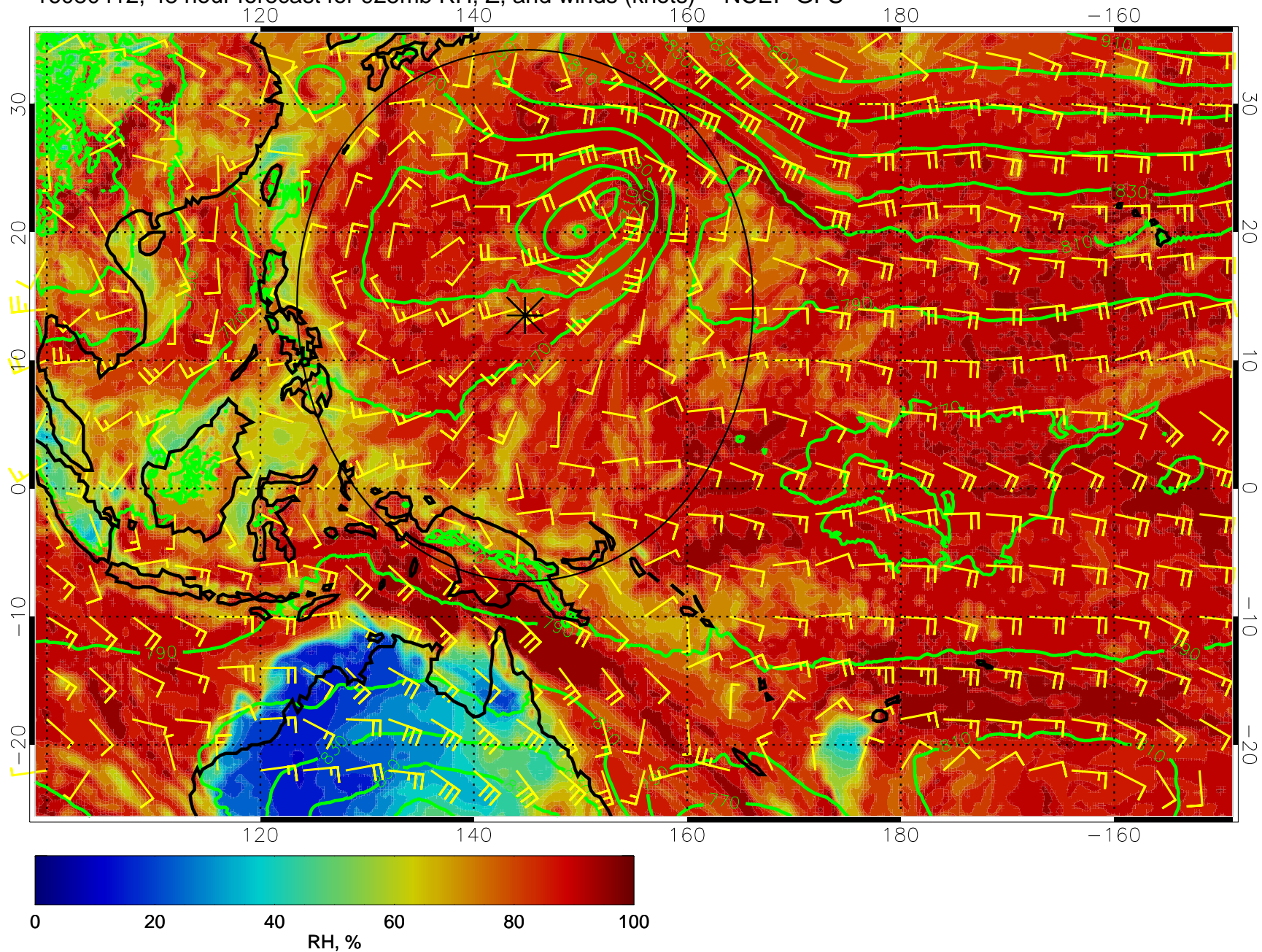
16080412, 48 hour forecast for 925mb RH, Z, and winds (knots) -- NCEP GFS
