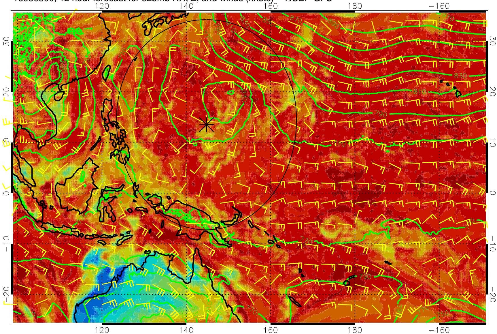
16080300, 12 hour forecast for 925mb RH, Z, and winds (knots) -- NCEP GFS
