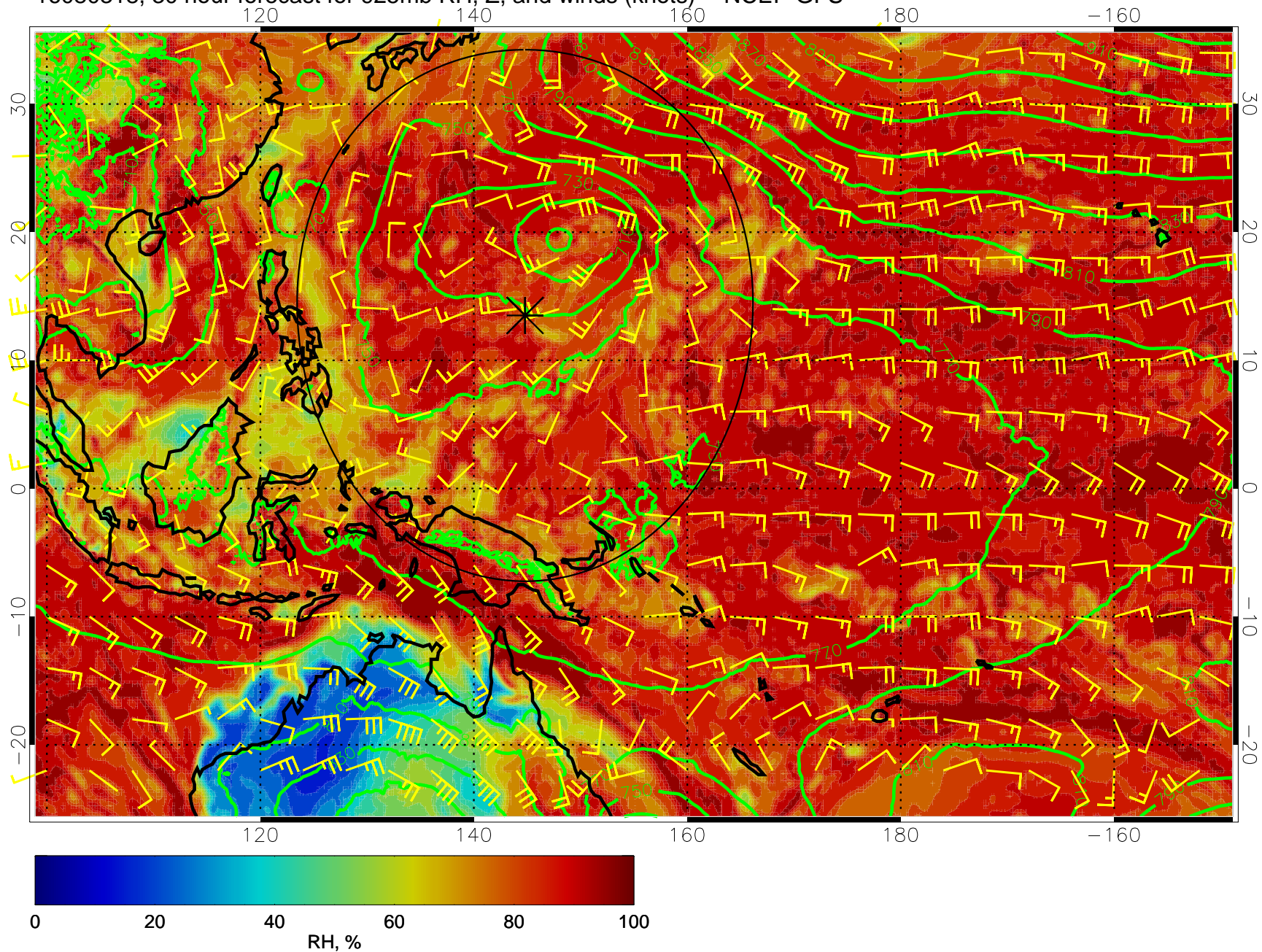
16080318, 30 hour forecast for 925mb RH, Z, and winds (knots) -- NCEP GFS
