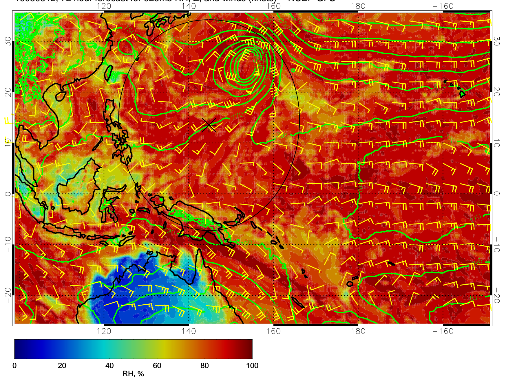
16080512, 72 hour forecast for 925mb RH, Z, and winds (knots) -- NCEP GFS
