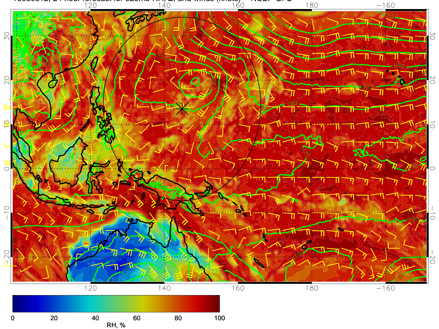
16080312, 24 hour forecast for 925mb RH, Z, and winds (knots) -- NCEP GFS
