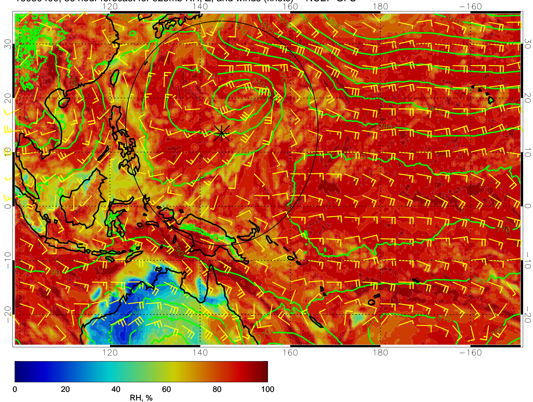
16080400, 36 hour forecast for 925mb RH, Z, and winds (knots) -- NCEP GFS
