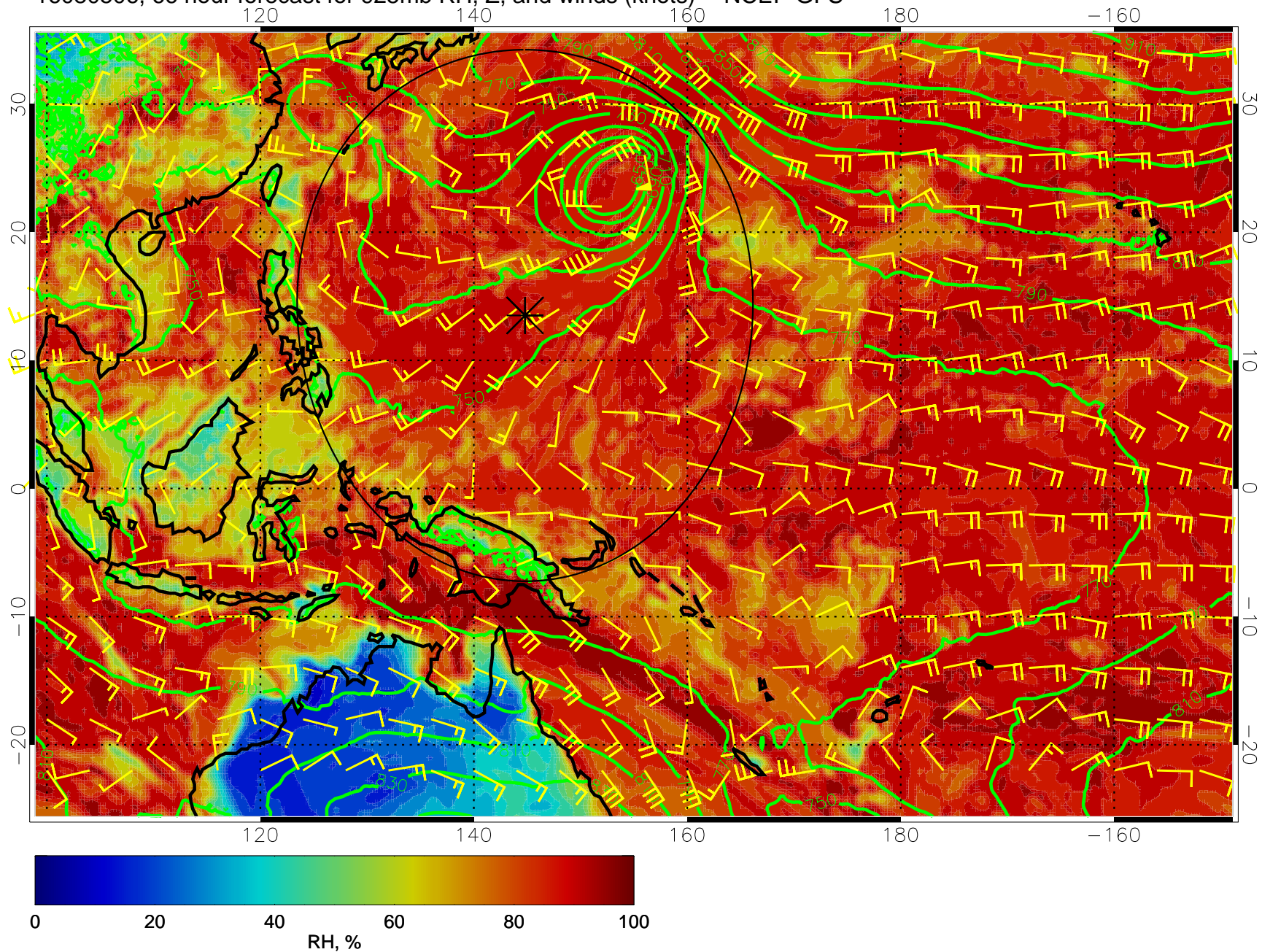
16080506, 66 hour forecast for 925mb RH, Z, and winds (knots) -- NCEP GFS
