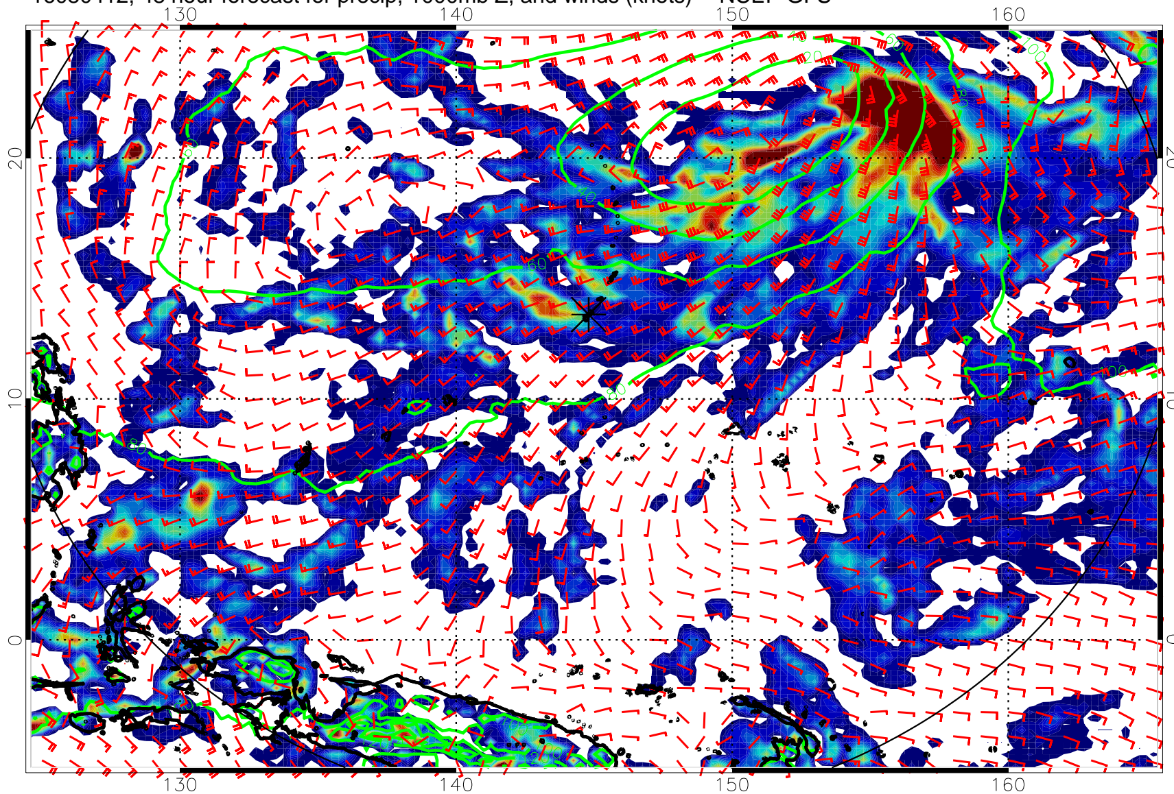
16080412, 48 hour forecast for precip, 1000mb Z, and winds (knots) -- NCEP GFS
