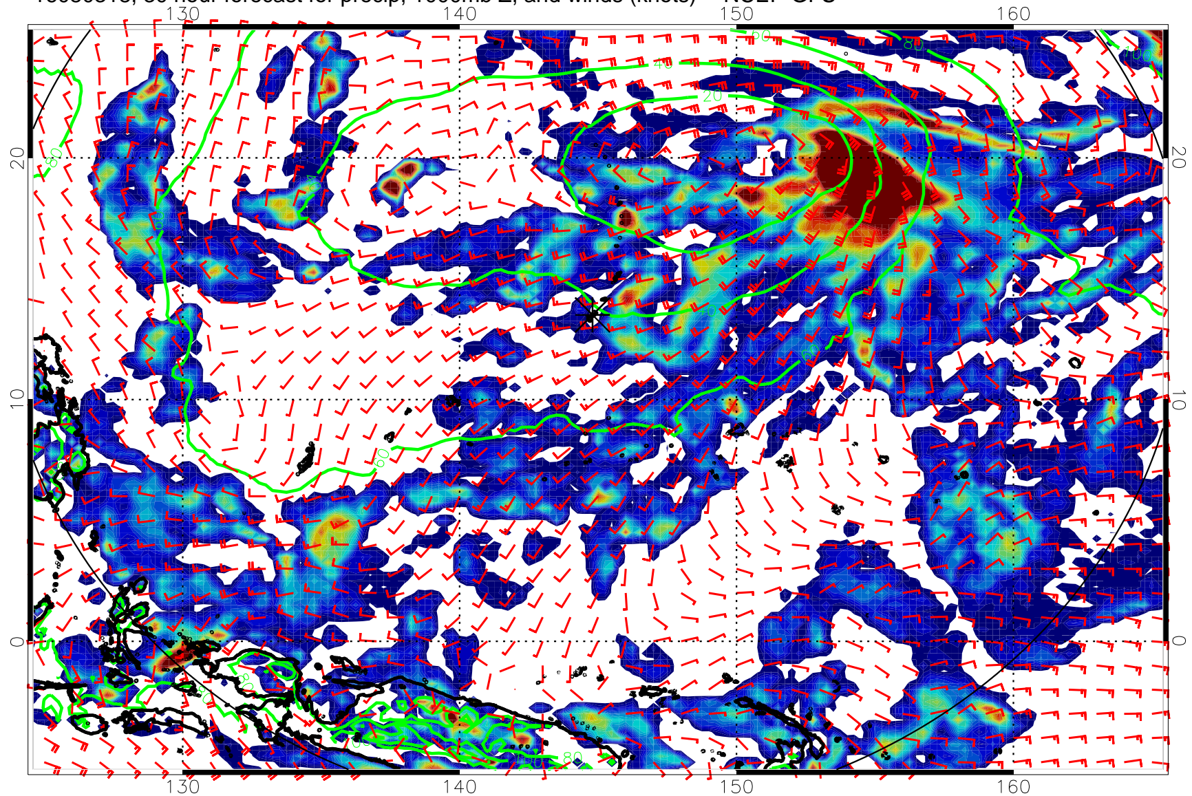
16080318, 30 hour forecast for precip, 1000mb Z, and winds (knots) -- NCEP GFS
