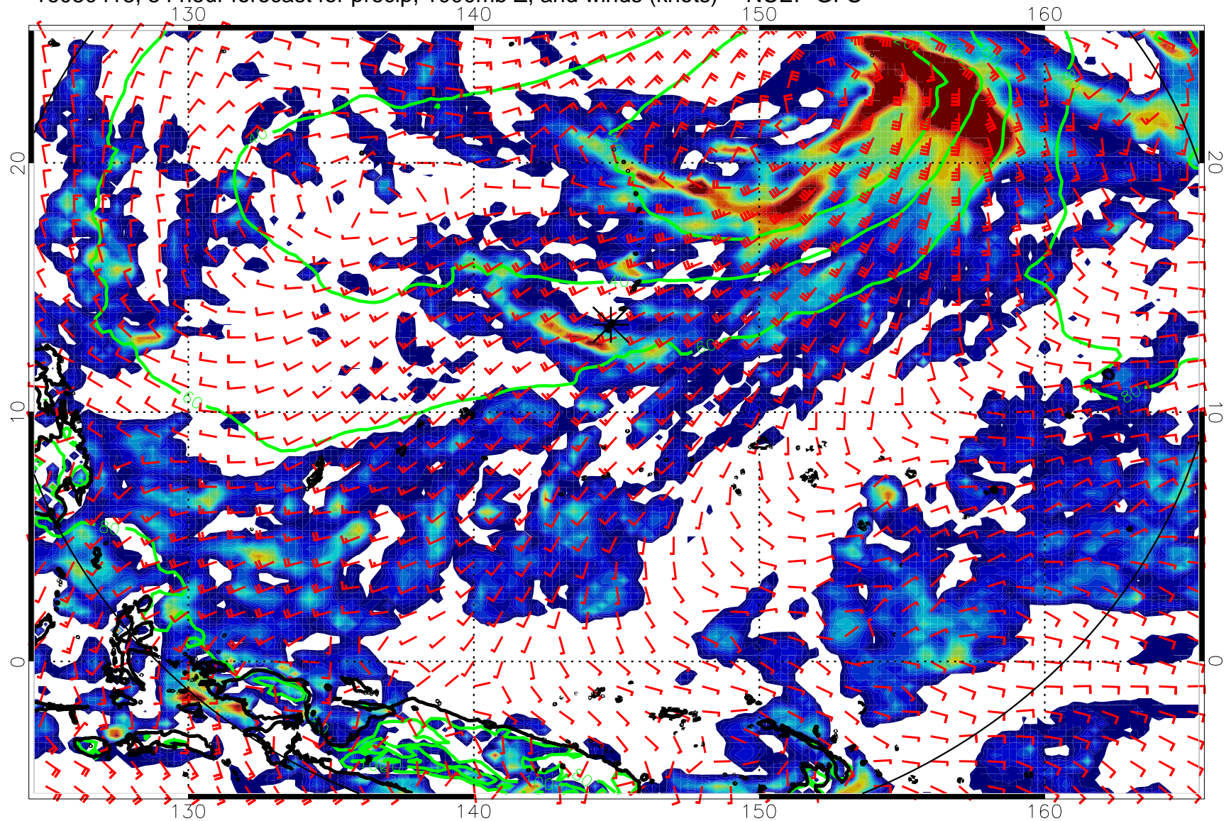
16080418, 54 hour forecast for precip, 1000mb Z, and winds (knots) -- NCEP GFS
