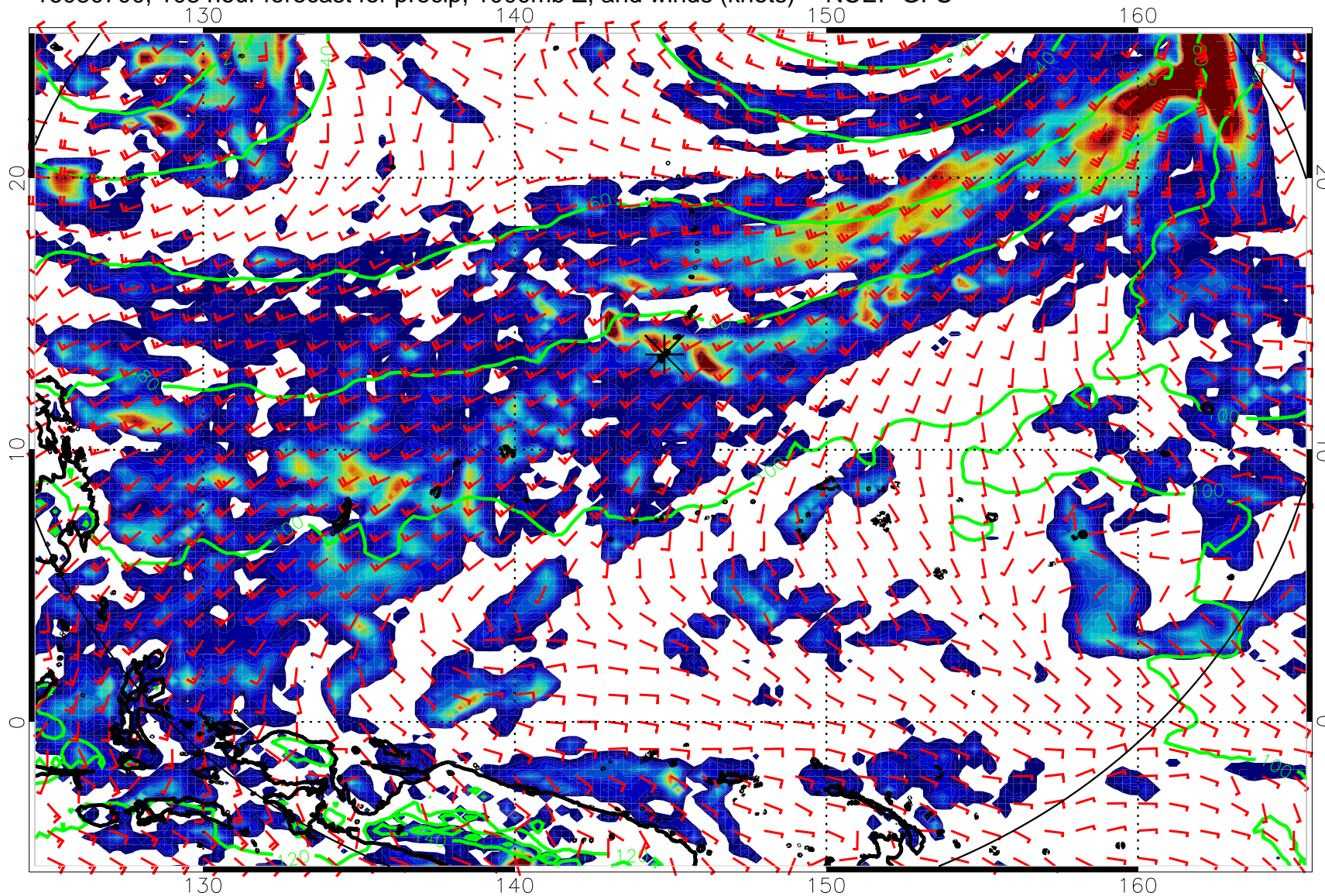
16080700, 108 hour forecast for precip, 1000mb Z, and winds (knots) -- NCEP GFS
