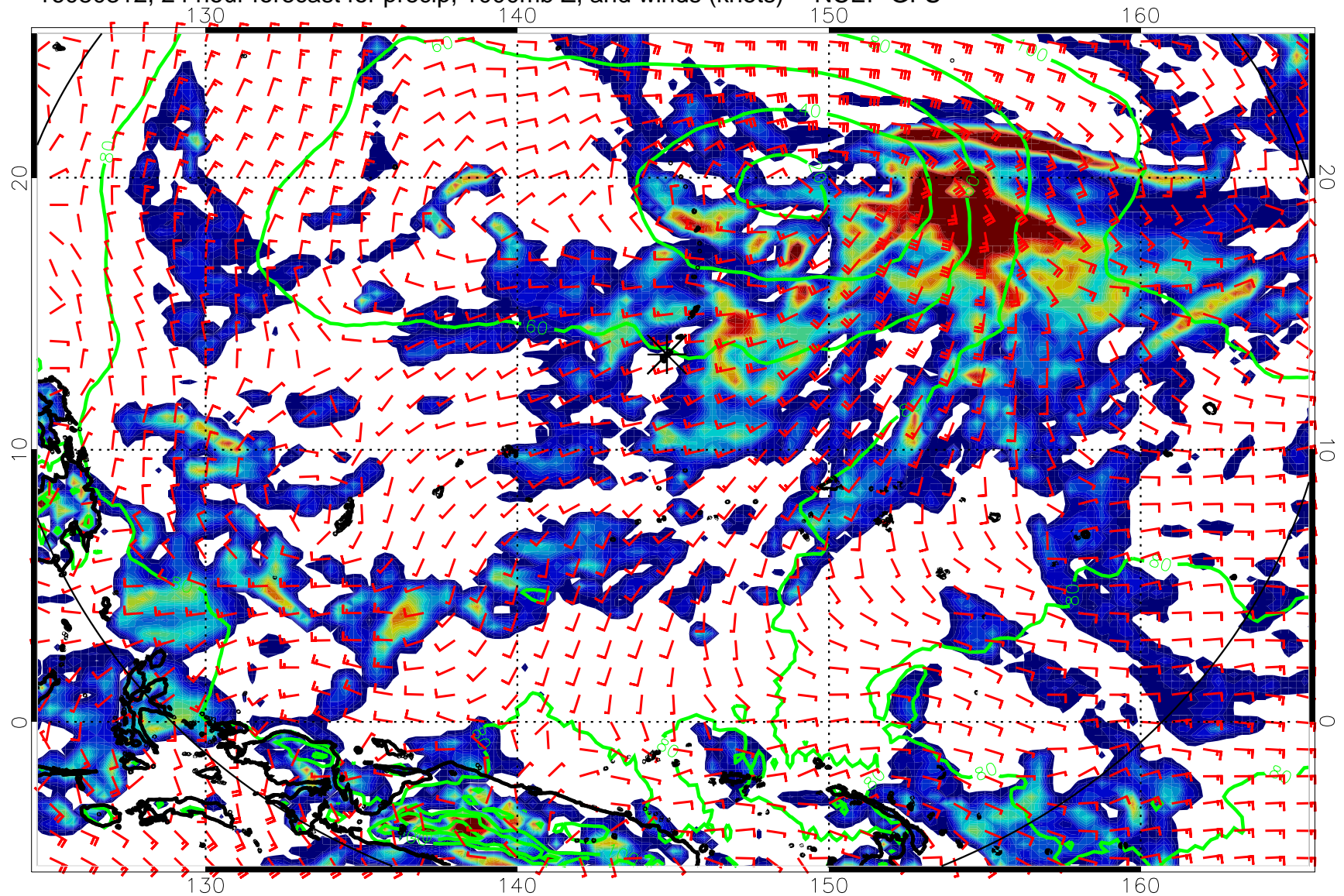
16080312, 24 hour forecast for precip, 1000mb Z, and winds (knots) -- NCEP GFS
