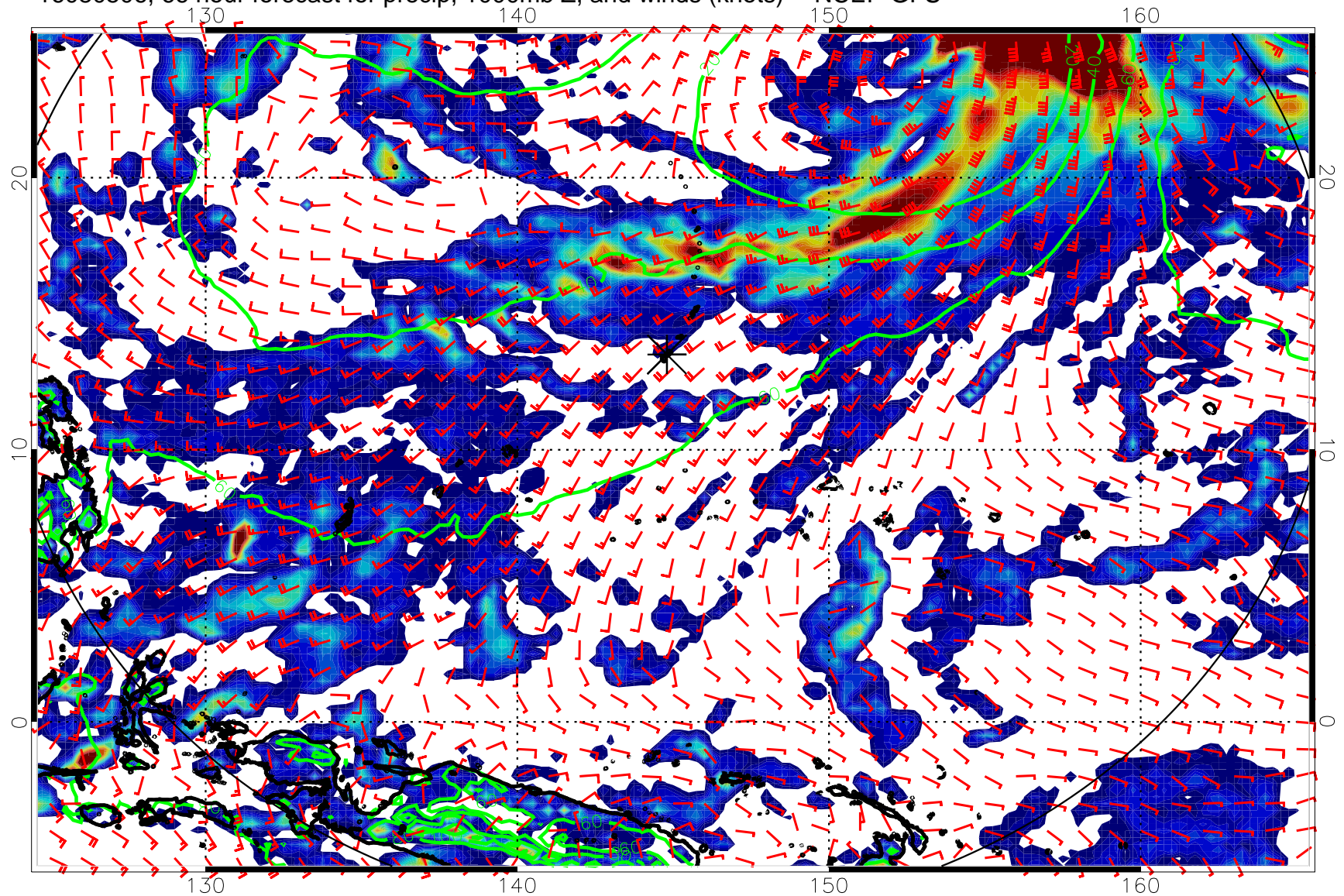
16080506, 66 hour forecast for precip, 1000mb Z, and winds (knots) -- NCEP GFS
