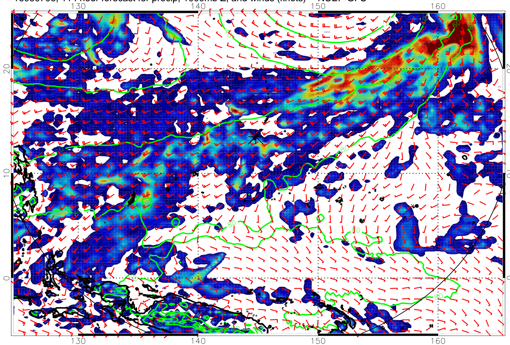
16080706, 114 hour forecast for precip, 1000mb Z, and winds (knots) -- NCEP GFS
