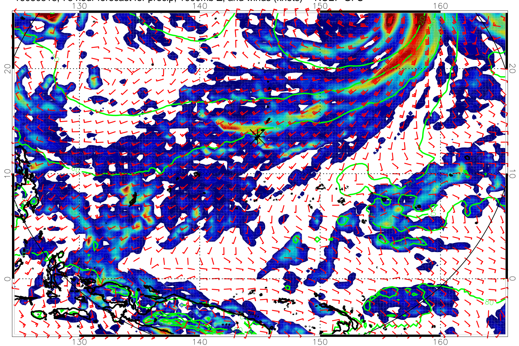
16080518, 78 hour forecast for precip, 1000mb Z, and winds (knots) -- NCEP GFS
