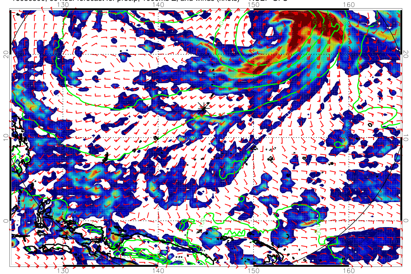
16080500, 60 hour forecast for precip, 1000mb Z, and winds (knots) -- NCEP GFS
