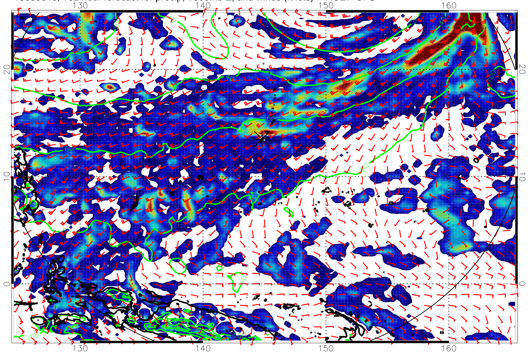
16080618, 102 hour forecast for precip, 1000mb Z, and winds (knots) -- NCEP GFS
