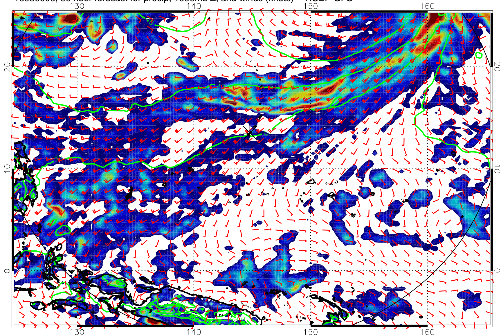
16080606, 90 hour forecast for precip, 1000mb Z, and winds (knots) -- NCEP GFS
