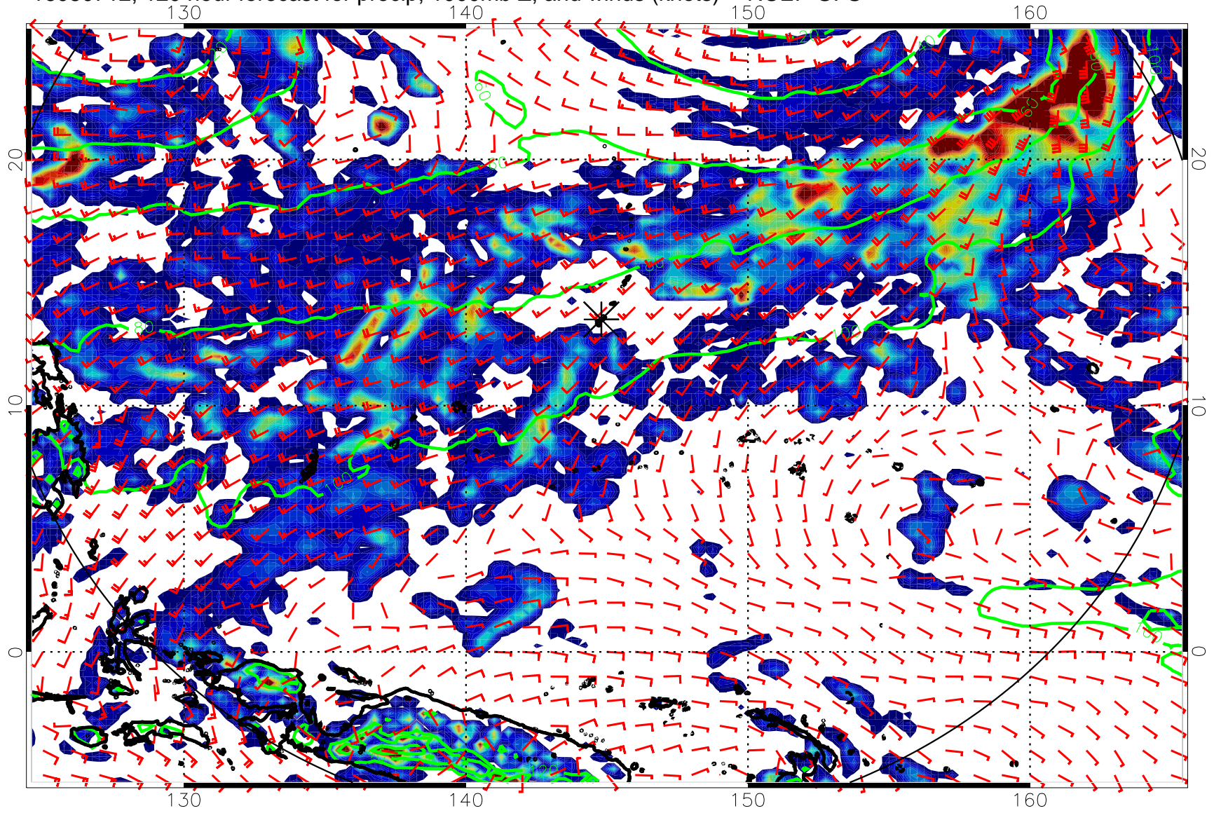
16080712, 120 hour forecast for precip, 1000mb Z, and winds (knots) -- NCEP GFS
