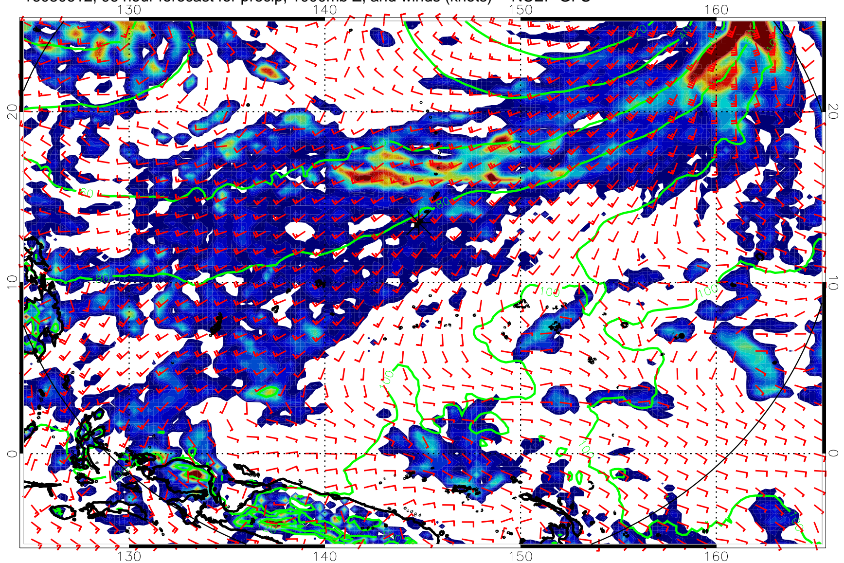
16080612, 96 hour forecast for precip, 1000mb Z, and winds (knots) -- NCEP GFS
