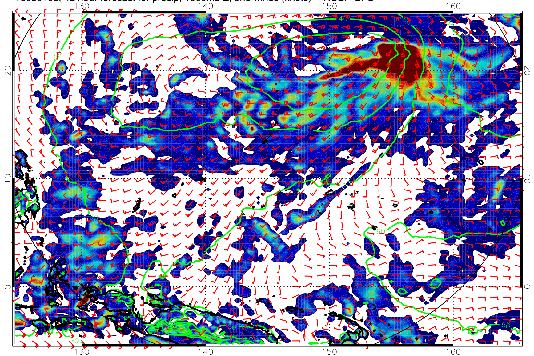
16080406, 42 hour forecast for precip, 1000mb Z, and winds (knots) -- NCEP GFS
