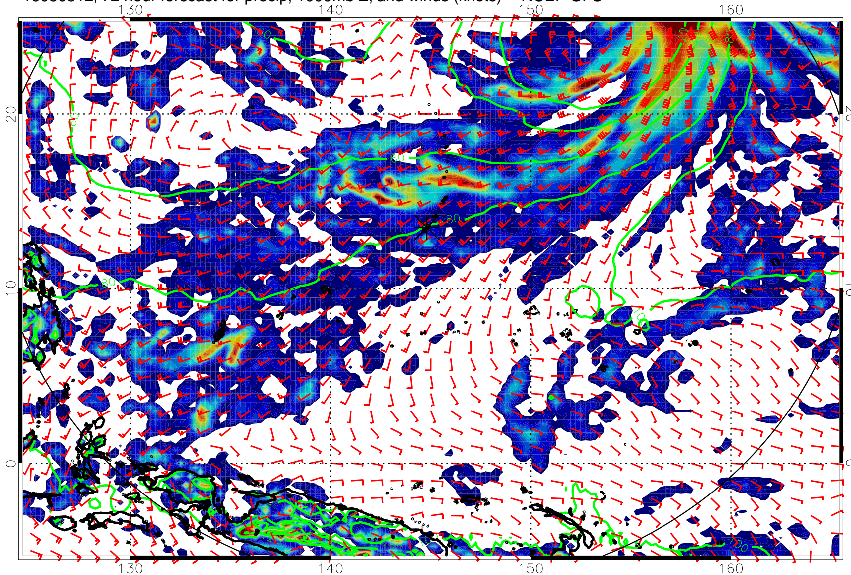
16080512, 72 hour forecast for precip, 1000mb Z, and winds (knots) -- NCEP GFS
