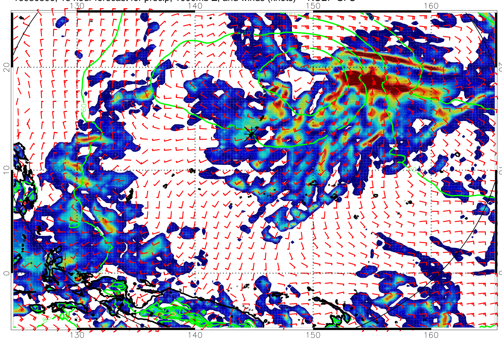
16080306, 18 hour forecast for precip, 1000mb Z, and winds (knots) -- NCEP GFS
