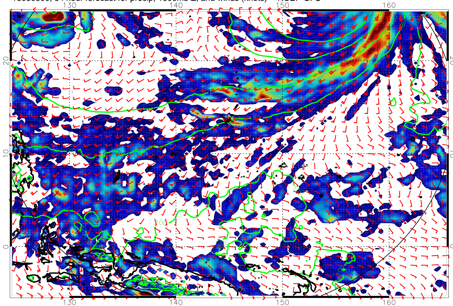
16080600, 84 hour forecast for precip, 1000mb Z, and winds (knots) -- NCEP GFS
