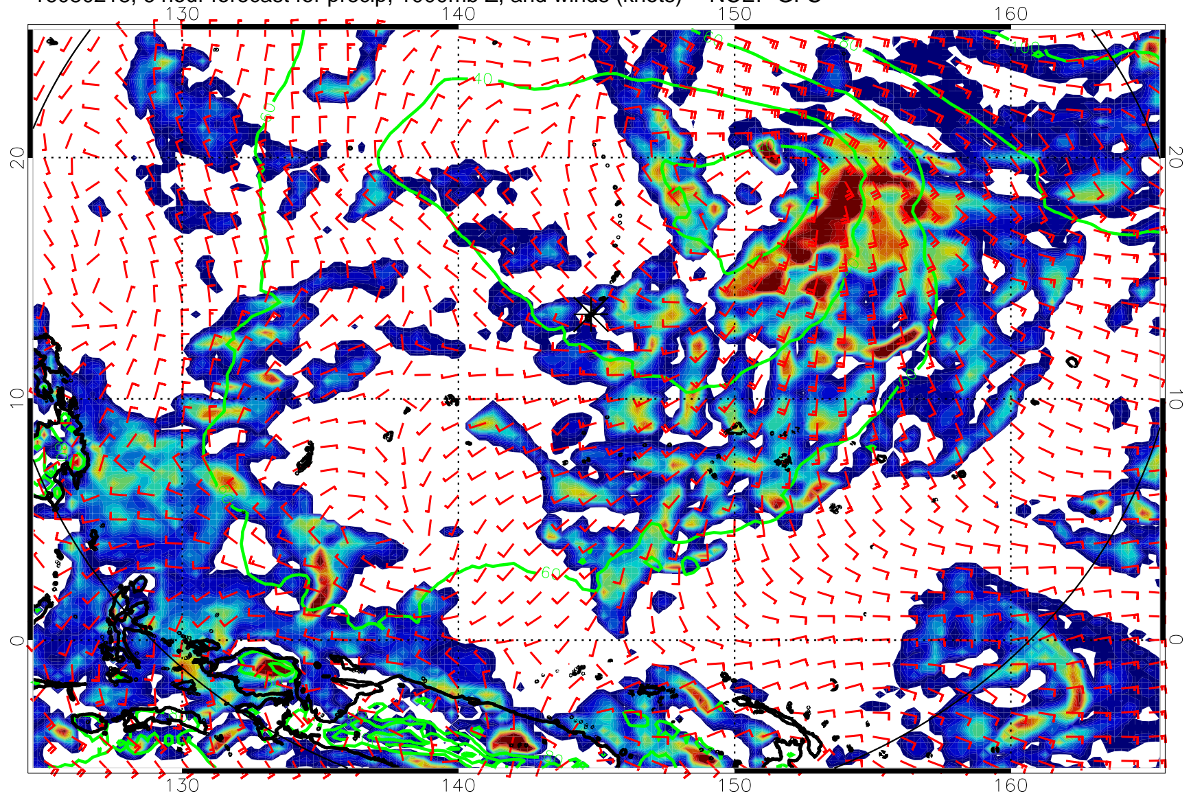
16080218, 6 hour forecast for precip, 1000mb Z, and winds (knots) -- NCEP GFS
