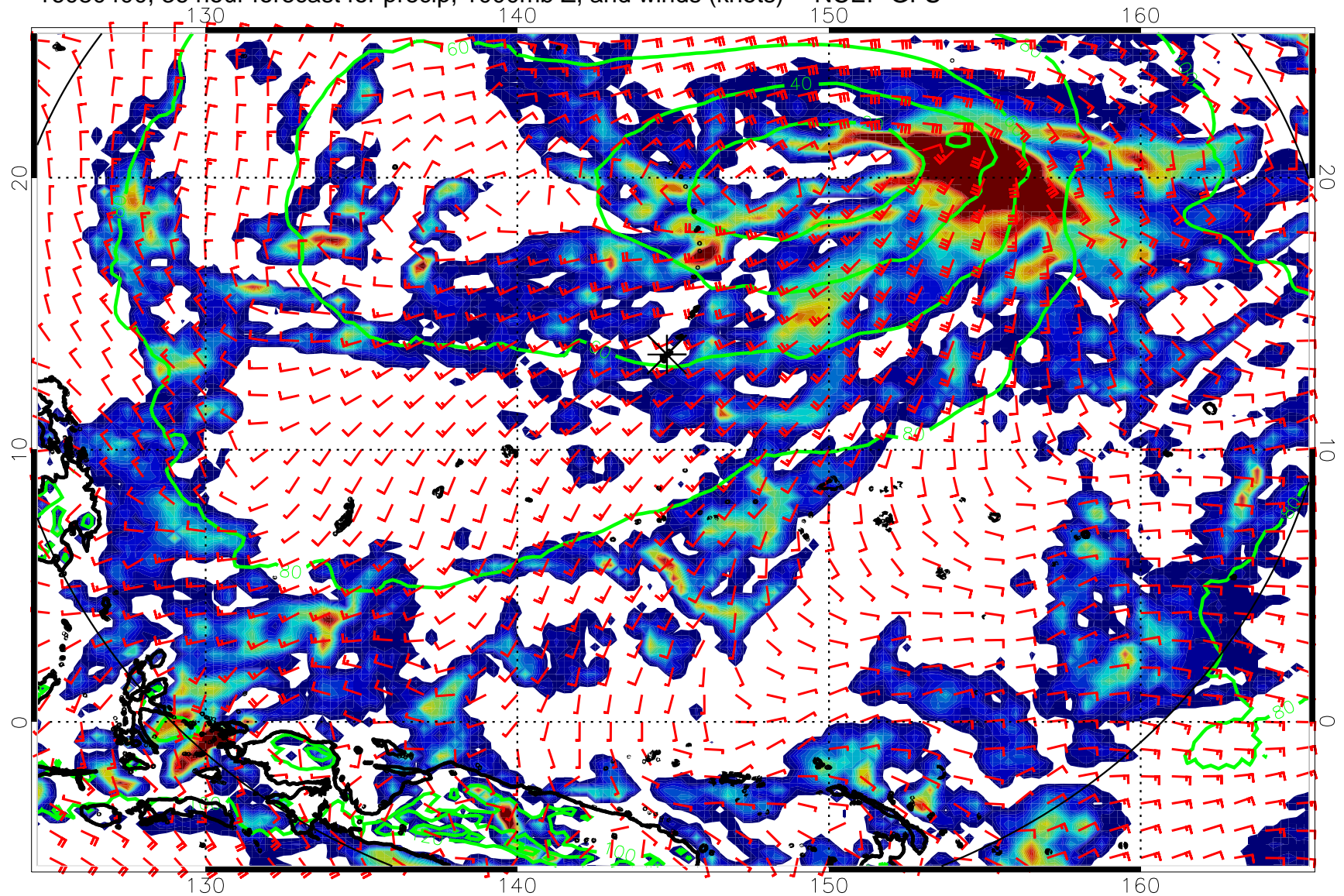
16080400, 36 hour forecast for precip, 1000mb Z, and winds (knots) -- NCEP GFS
