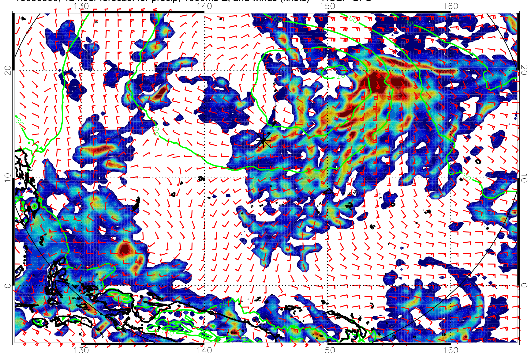
16080300, 12 hour forecast for precip, 1000mb Z, and winds (knots) -- NCEP GFS
