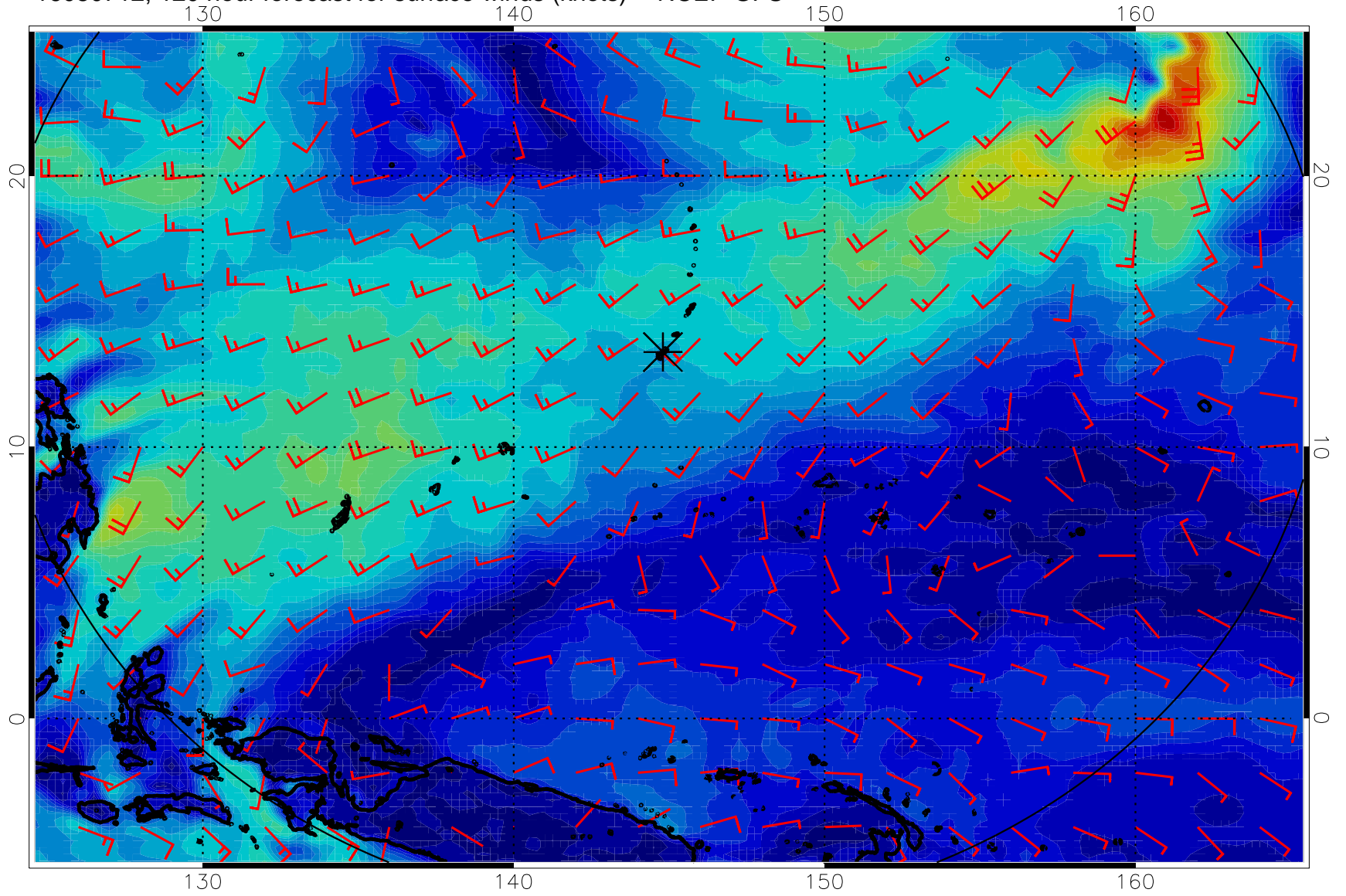
16080712, 120 hour forecast for surface winds (knots) -- NCEP GFS
