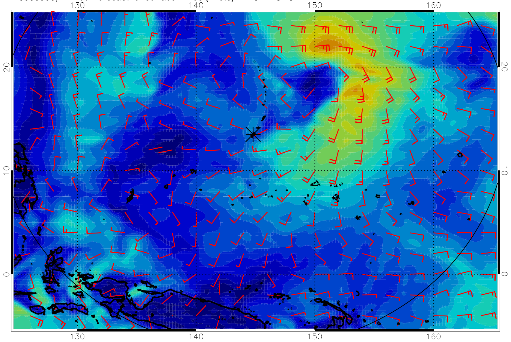
16080300, 12 hour forecast for surface winds (knots) -- NCEP GFS
