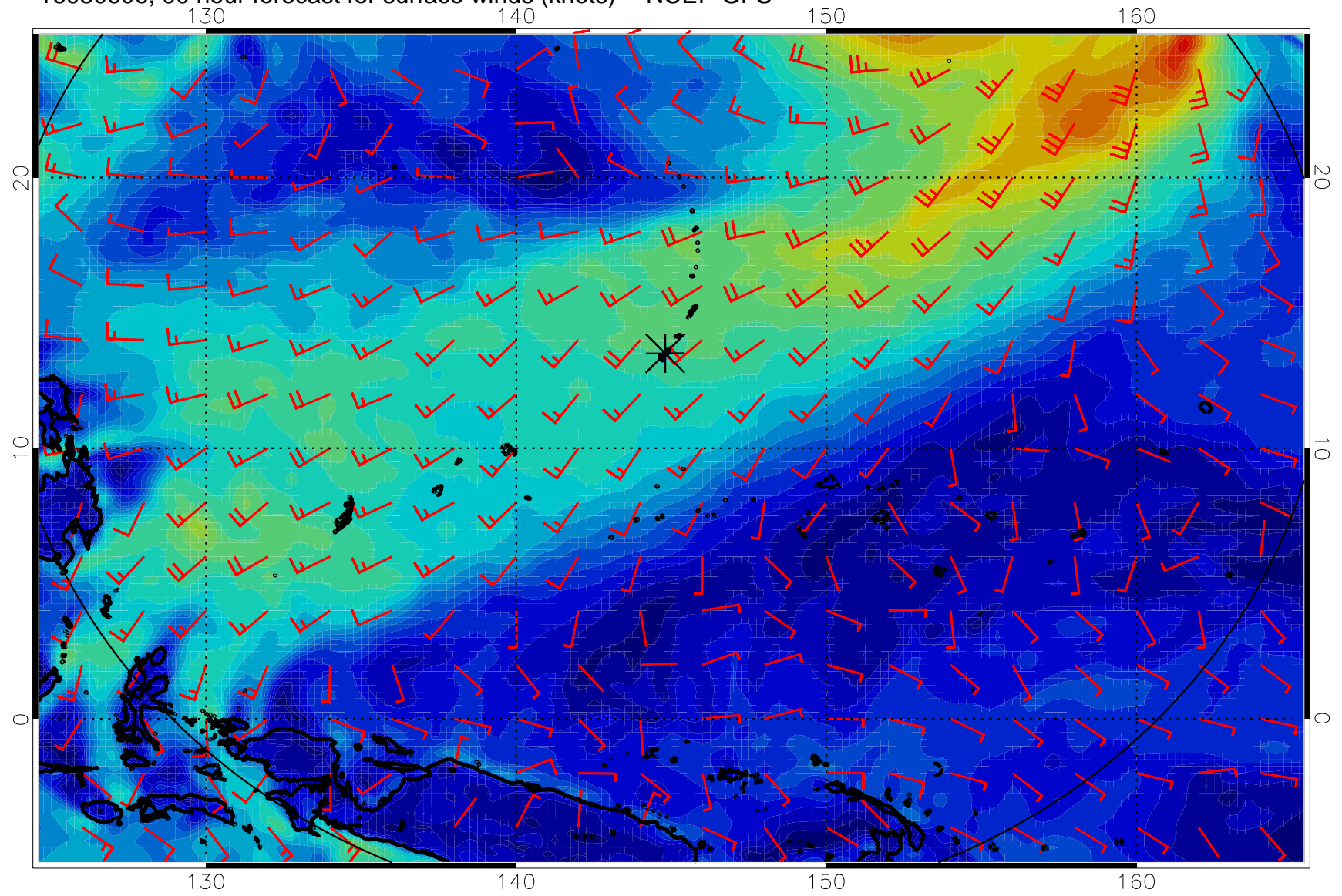
16080606, 90 hour forecast for surface winds (knots) -- NCEP GFS
