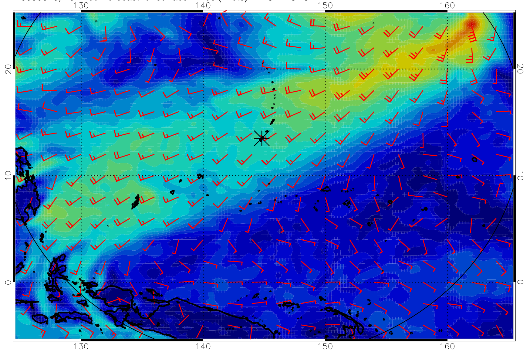
16080618, 102 hour forecast for surface winds (knots) -- NCEP GFS
