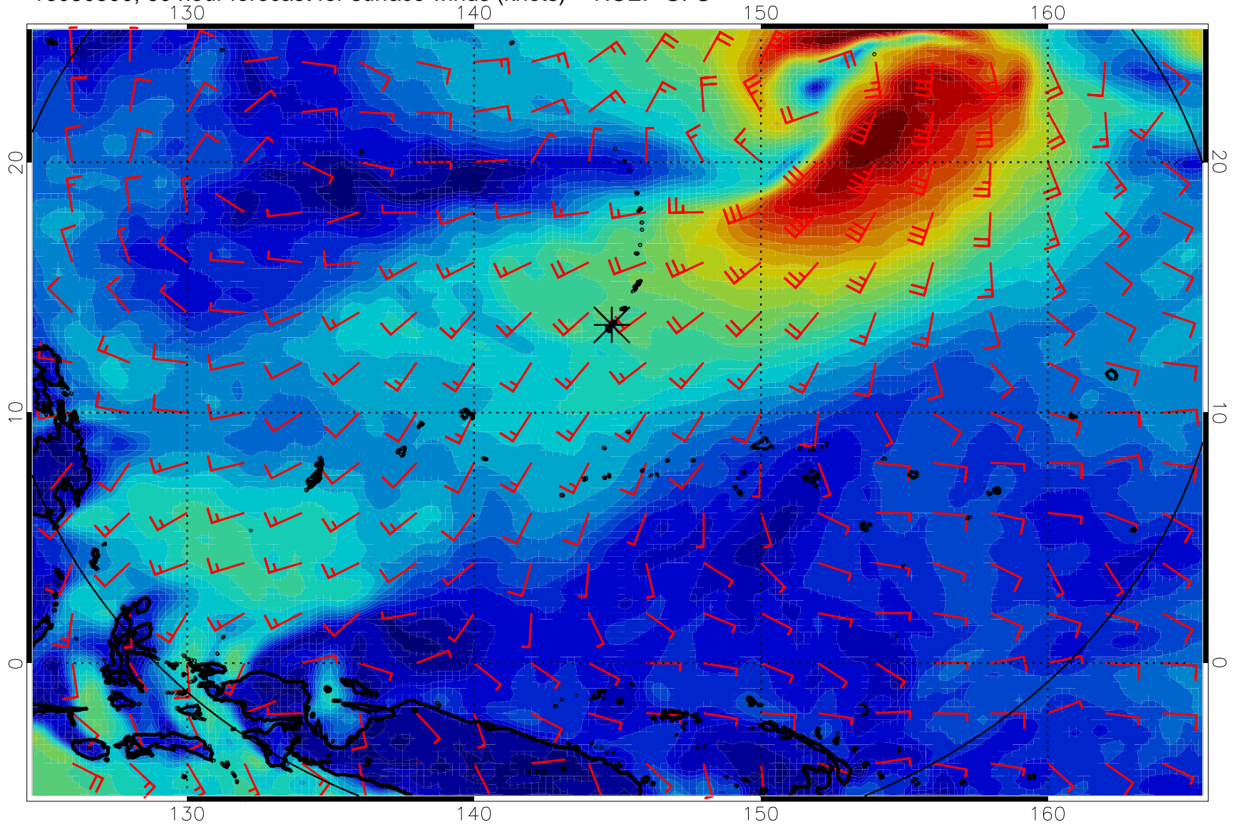
16080500, 60 hour forecast for surface winds (knots) -- NCEP GFS
