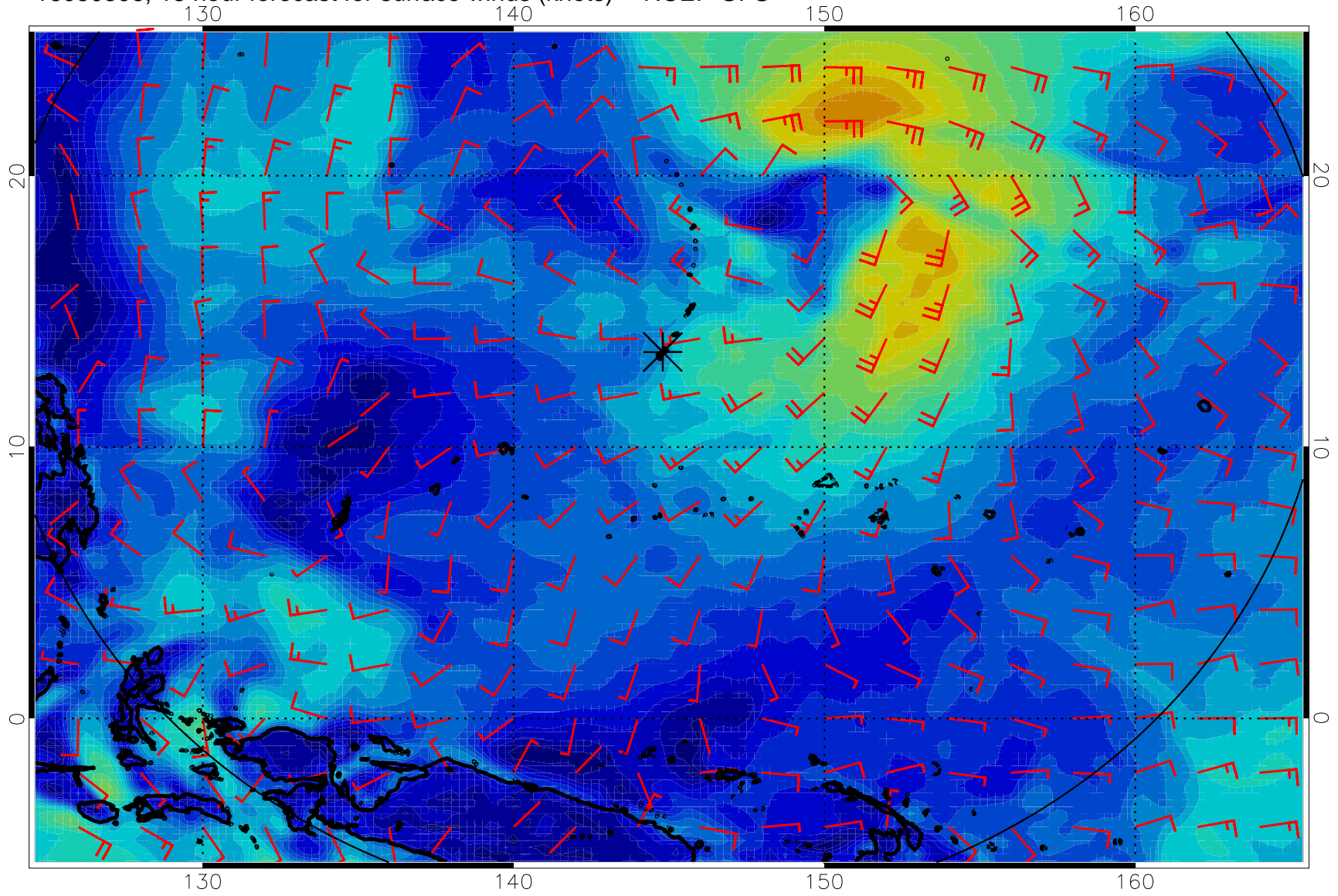
16080306, 18 hour forecast for surface winds (knots) -- NCEP GFS
