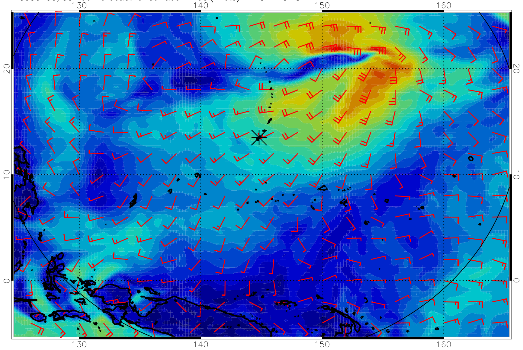
16080400, 36 hour forecast for surface winds (knots) -- NCEP GFS
