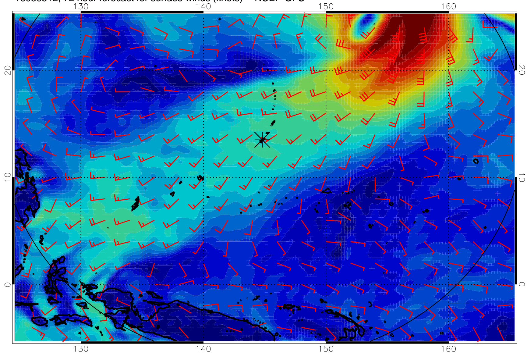
16080512, 72 hour forecast for surface winds (knots) -- NCEP GFS
