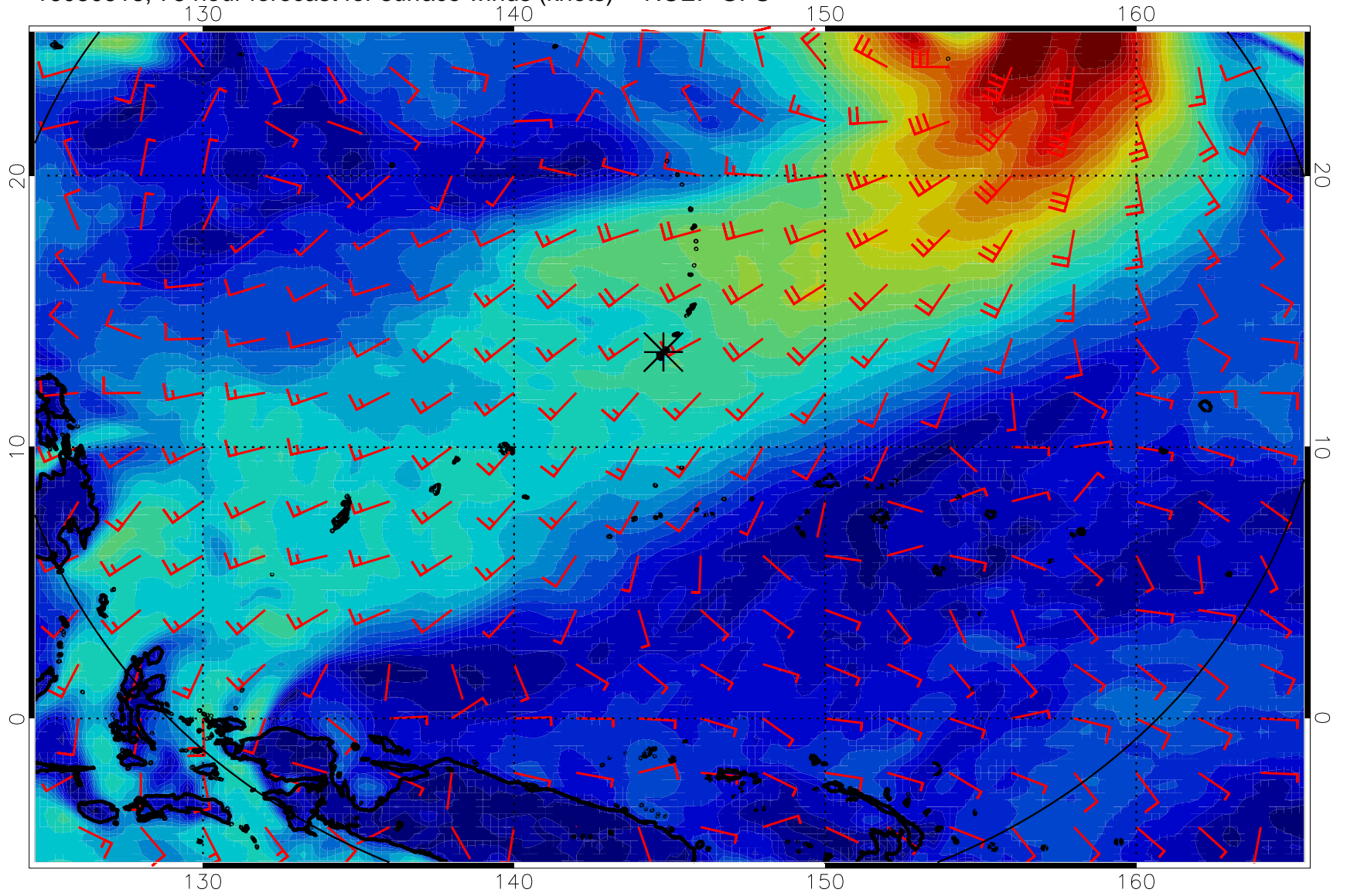
16080518, 78 hour forecast for surface winds (knots) -- NCEP GFS
