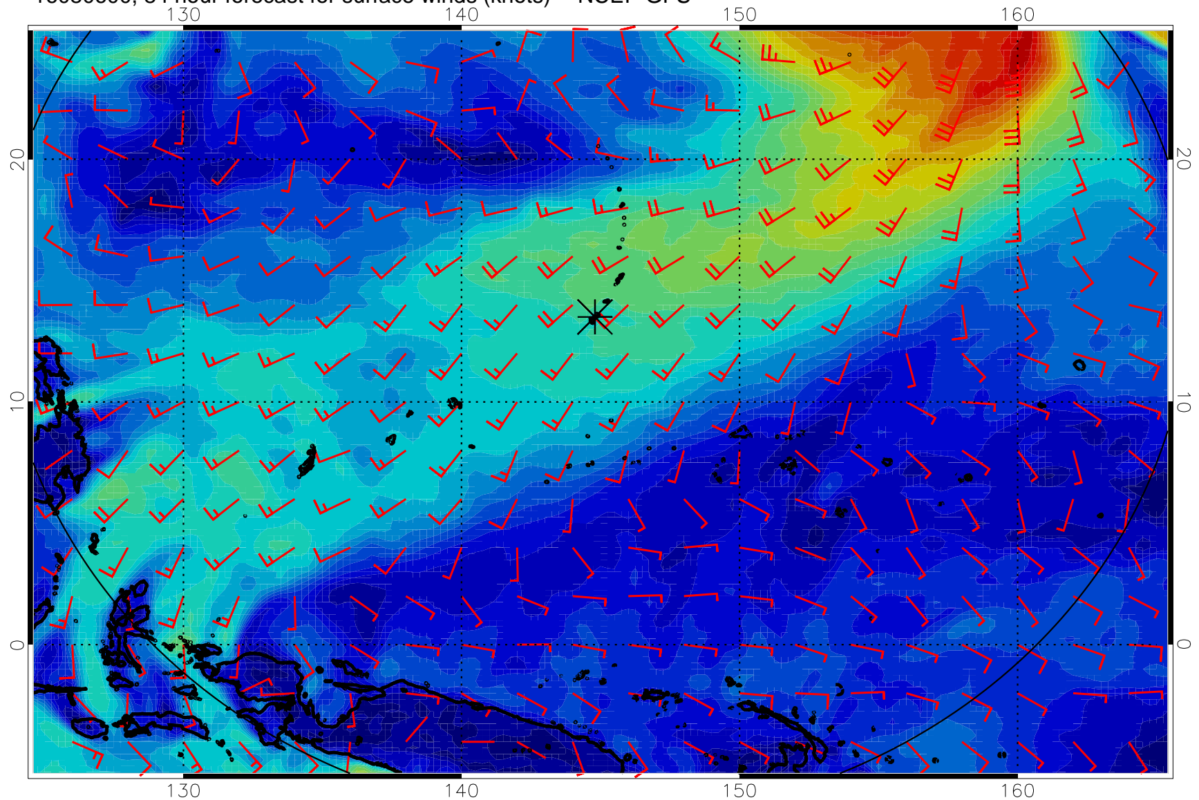
16080600, 84 hour forecast for surface winds (knots) -- NCEP GFS
