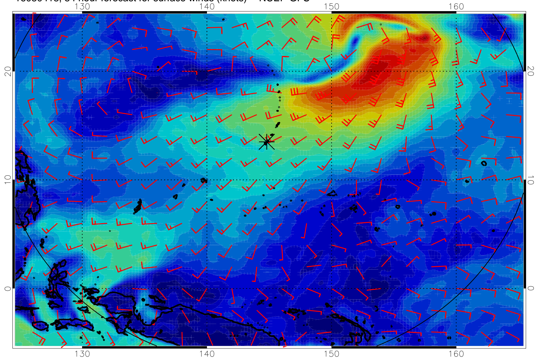
16080418, 54 hour forecast for surface winds (knots) -- NCEP GFS
