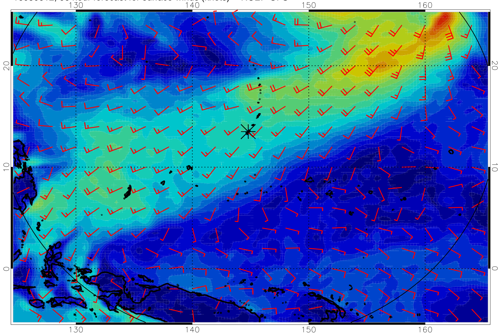
16080612, 96 hour forecast for surface winds (knots) -- NCEP GFS
