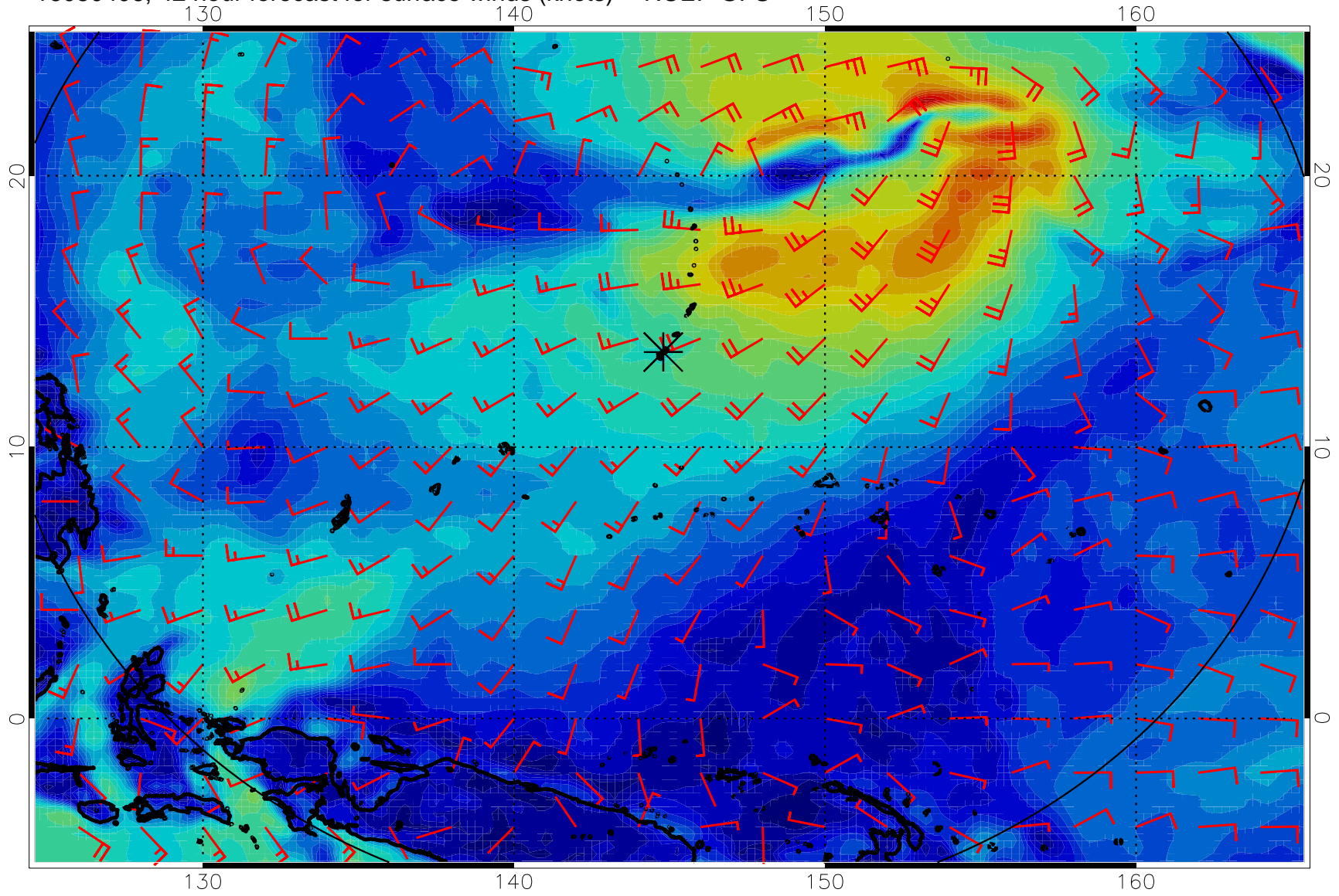
16080406, 42 hour forecast for surface winds (knots) -- NCEP GFS
