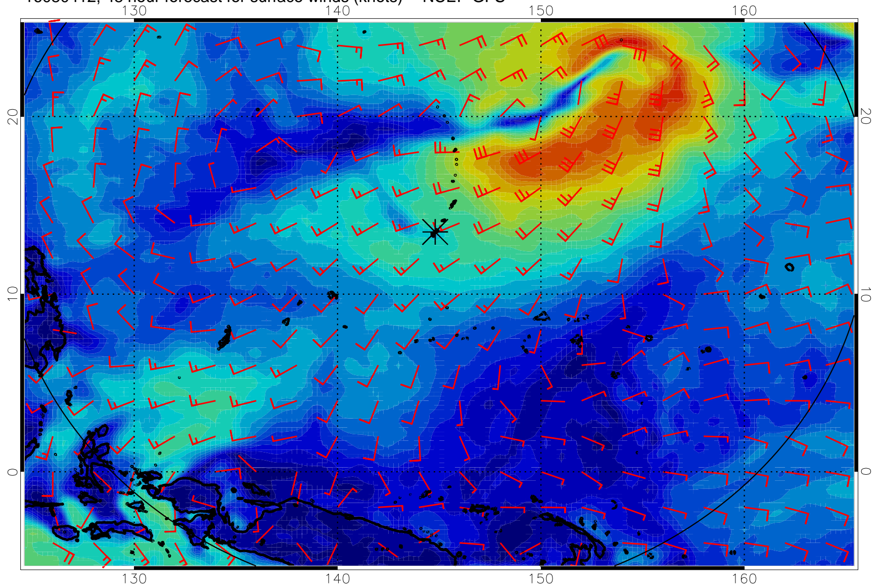
16080412, 48 hour forecast for surface winds (knots) -- NCEP GFS
