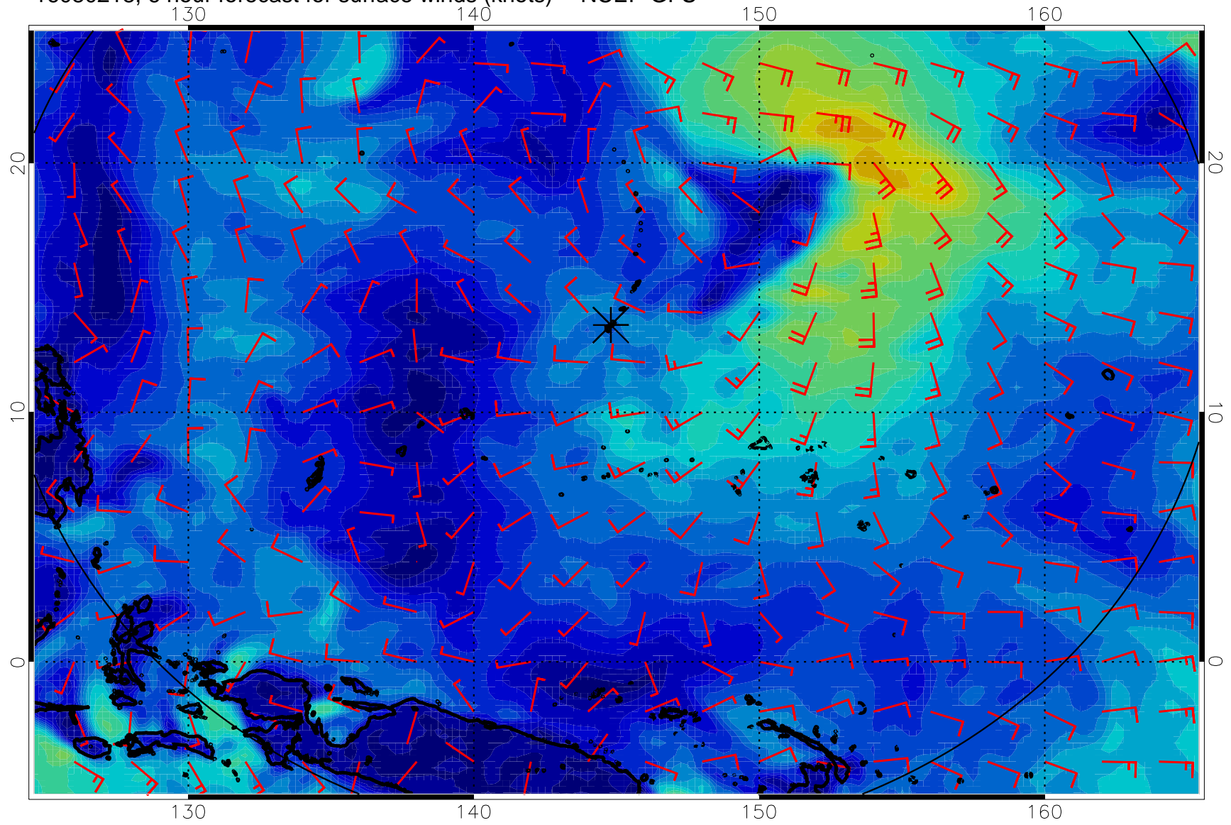
16080218, 6 hour forecast for surface winds (knots) -- NCEP GFS
