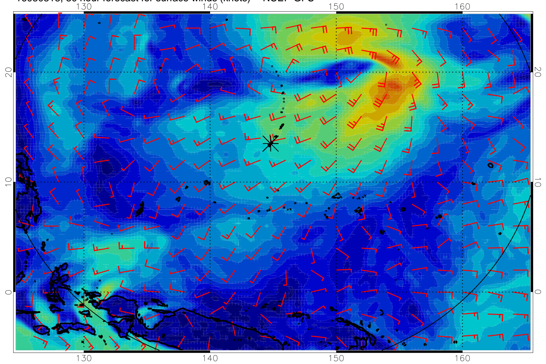
16080318, 30 hour forecast for surface winds (knots) -- NCEP GFS
