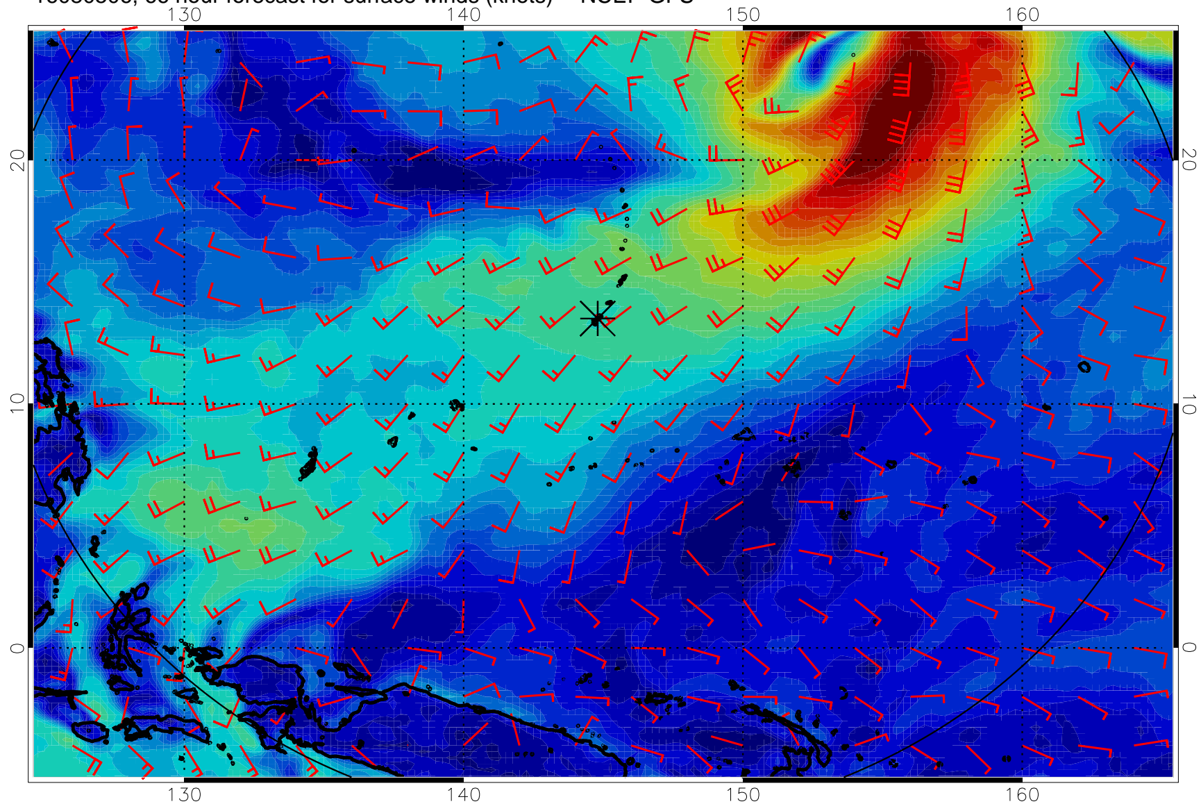
16080506, 66 hour forecast for surface winds (knots) -- NCEP GFS
