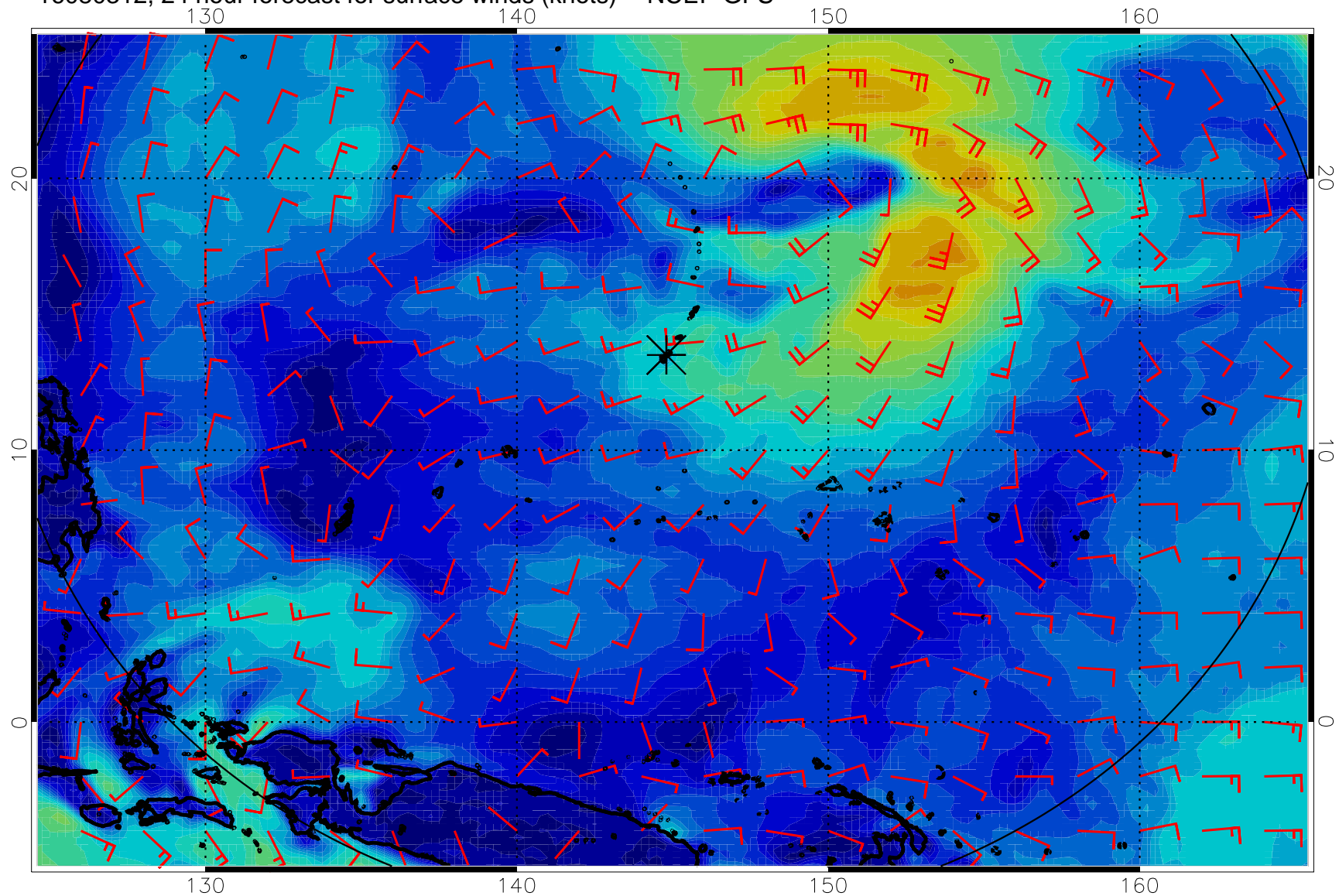
16080312, 24 hour forecast for surface winds (knots) -- NCEP GFS
