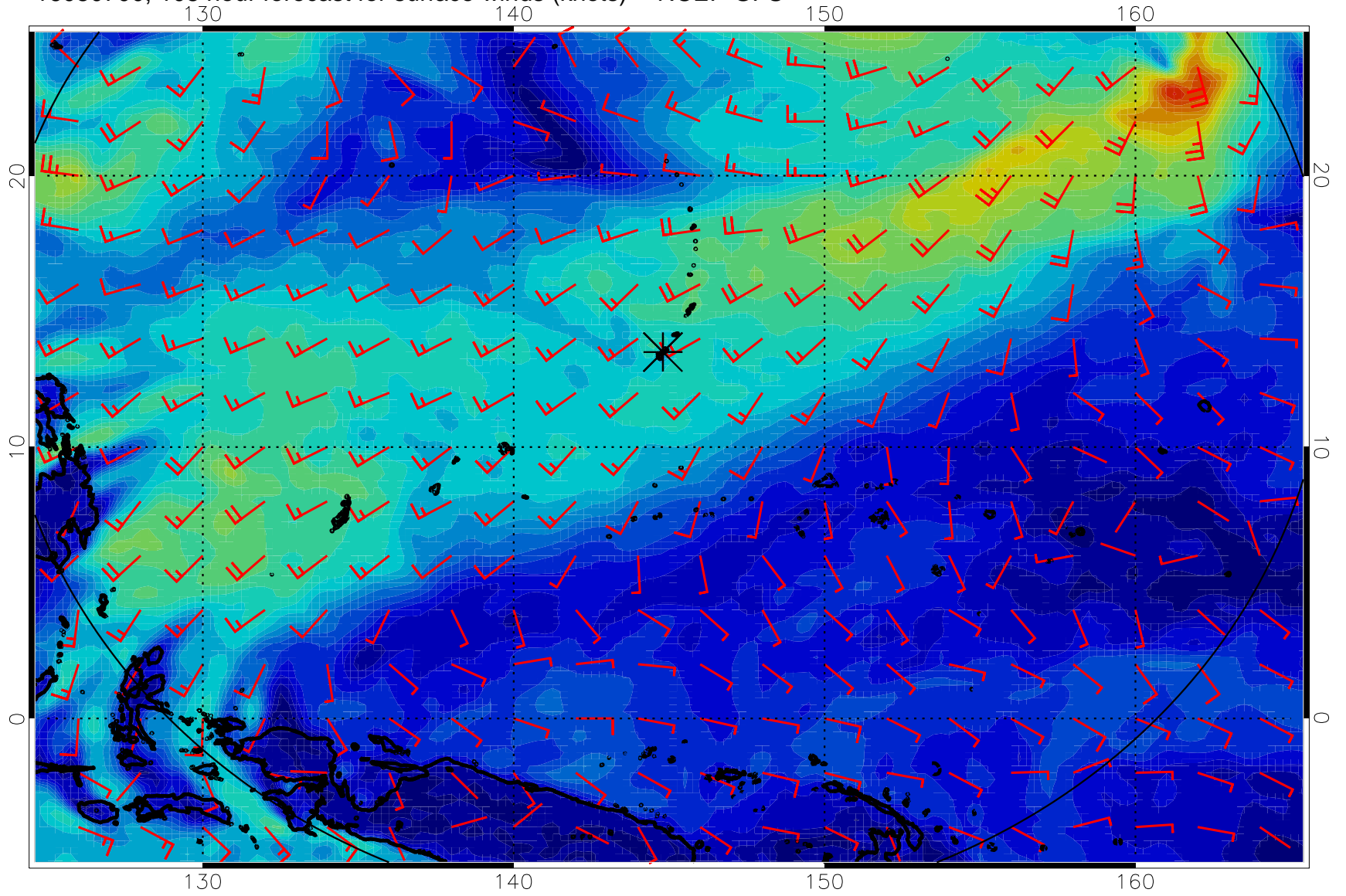
16080700, 108 hour forecast for surface winds (knots) -- NCEP GFS
