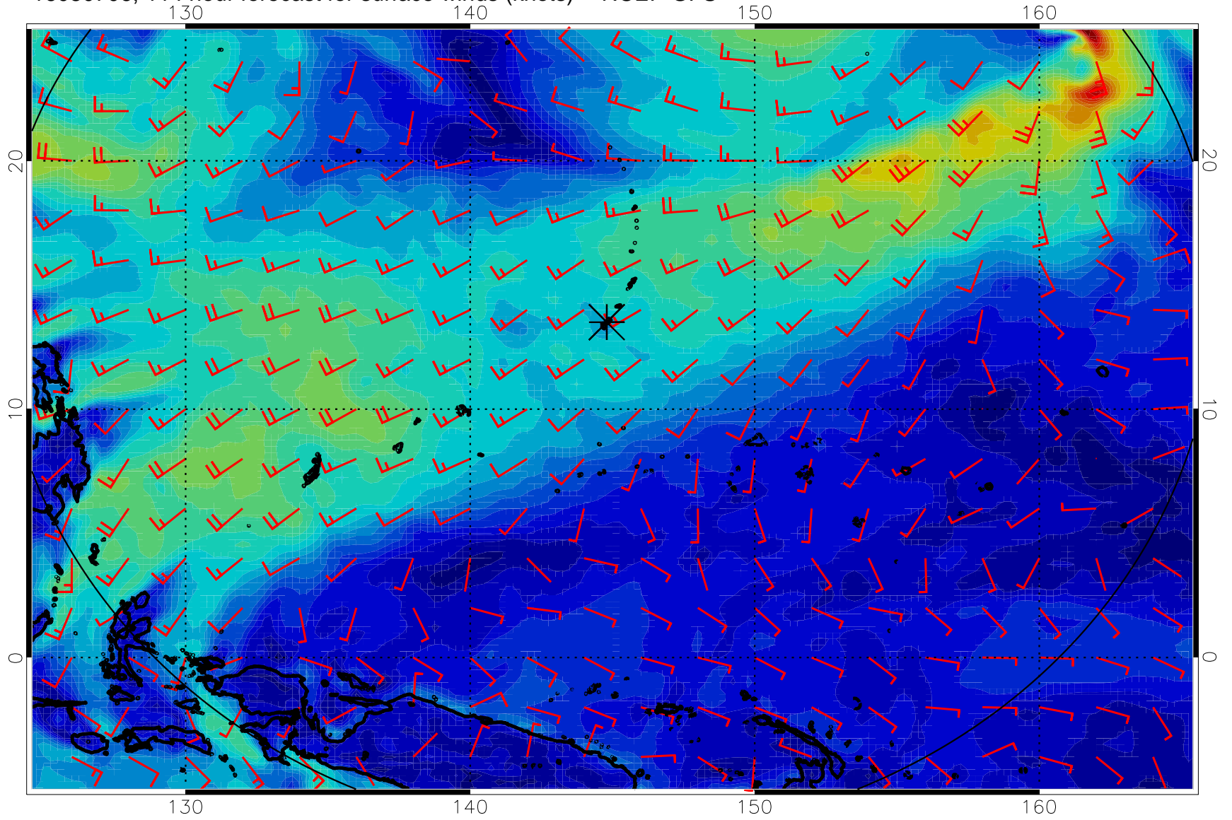
16080706, 114 hour forecast for surface winds (knots) -- NCEP GFS
