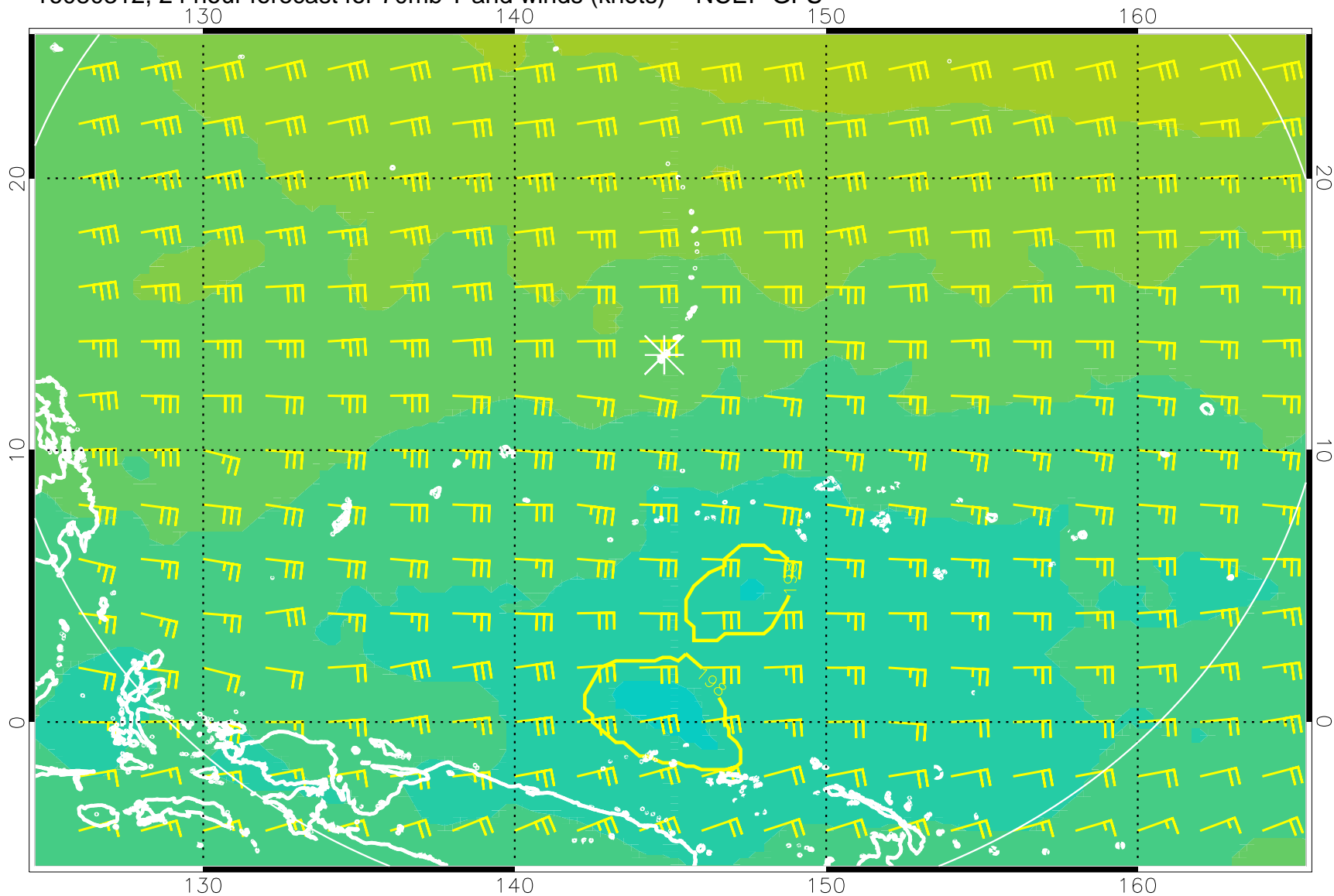
16080312, 24 hour forecast for 70mb T and winds (knots) -- NCEP GFS
