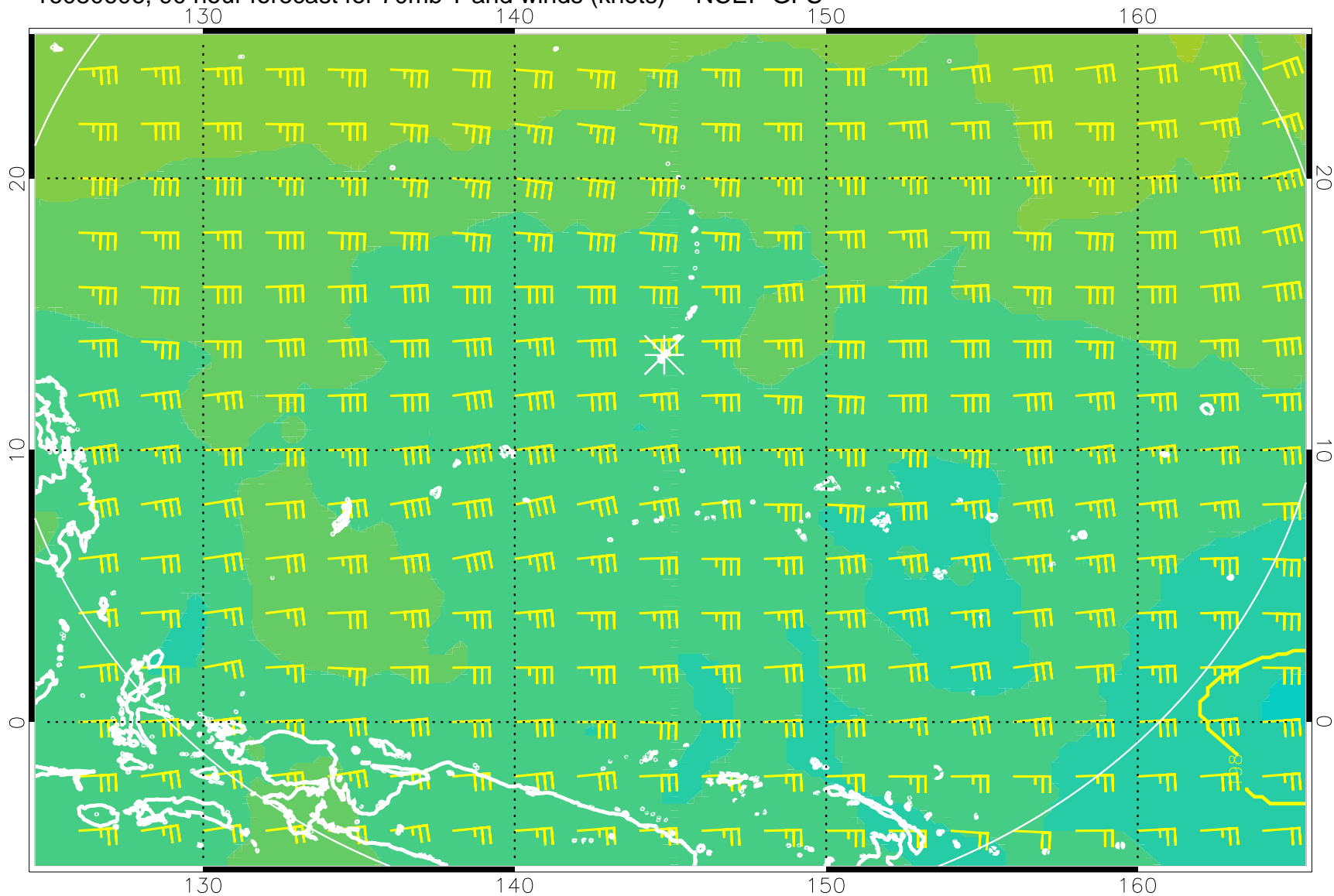
16080606, 90 hour forecast for 70mb T and winds (knots) -- NCEP GFS
