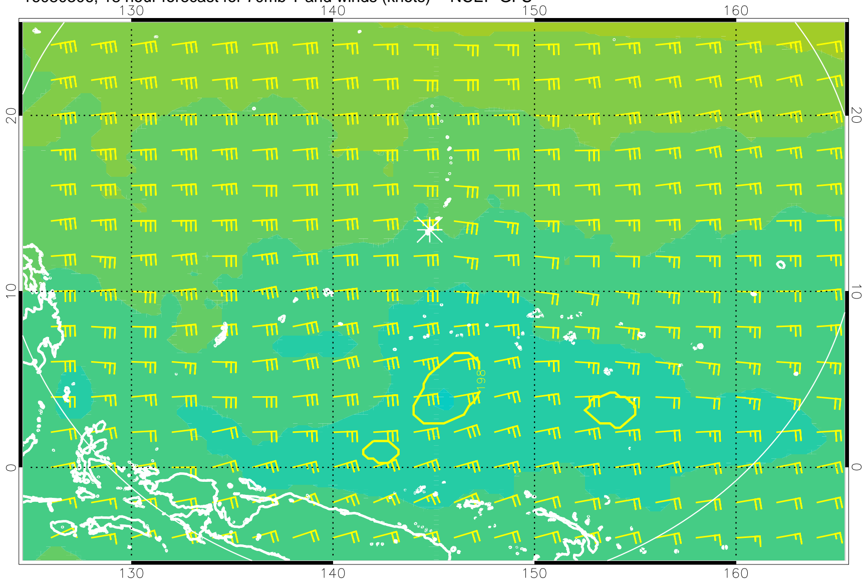
16080306, 18 hour forecast for 70mb T and winds (knots) -- NCEP GFS
