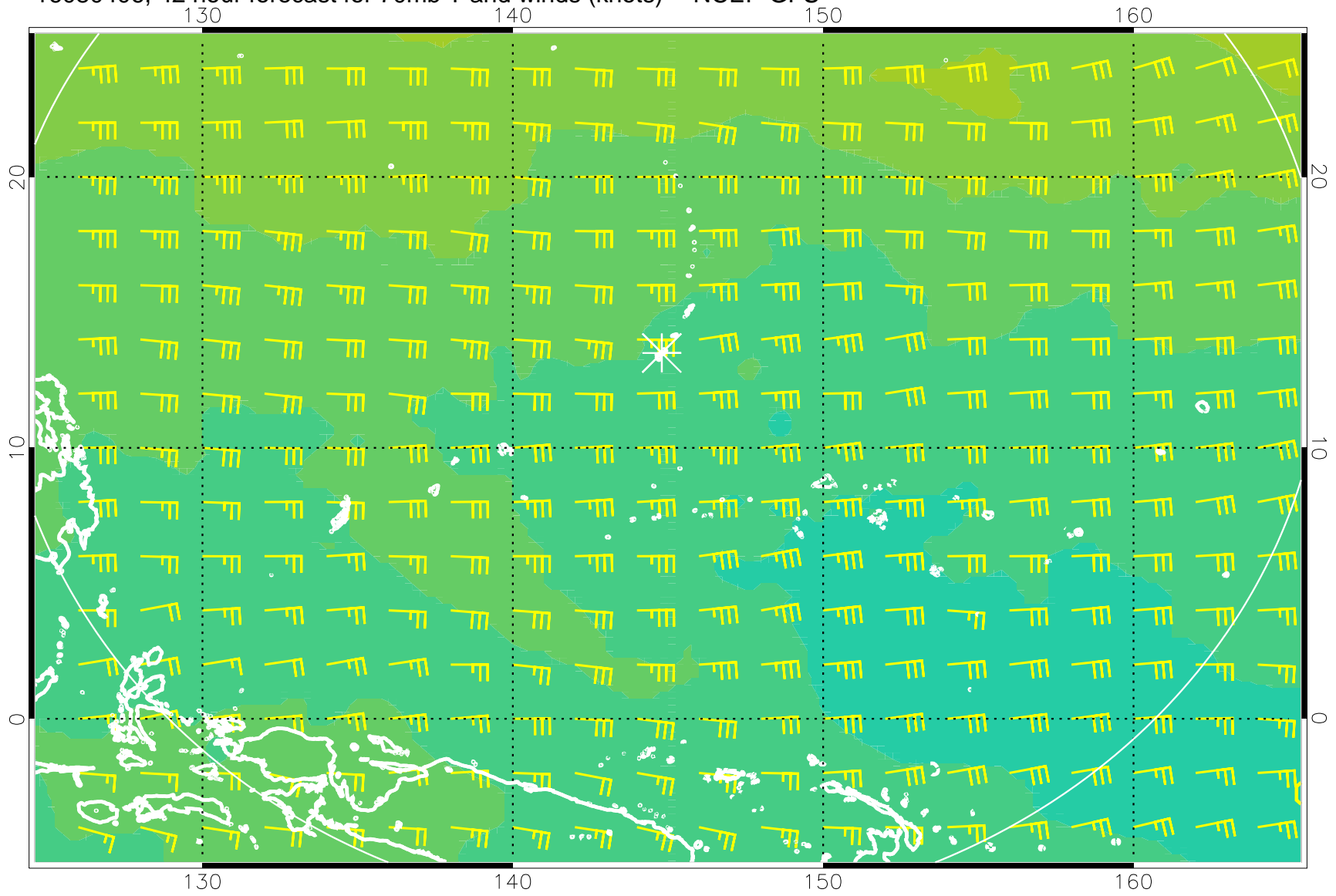
16080406, 42 hour forecast for 70mb T and winds (knots) -- NCEP GFS
