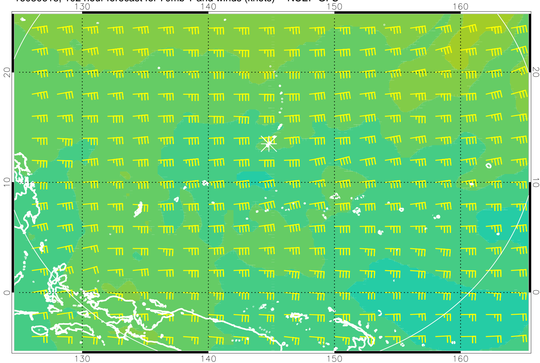
16080618, 102 hour forecast for 70mb T and winds (knots) -- NCEP GFS
