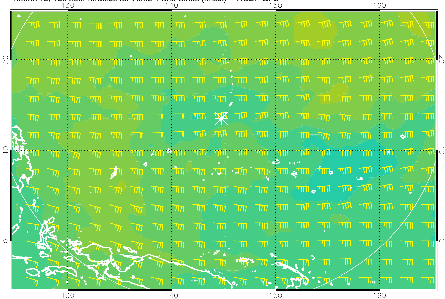
16080712, 120 hour forecast for 70mb T and winds (knots) -- NCEP GFS
