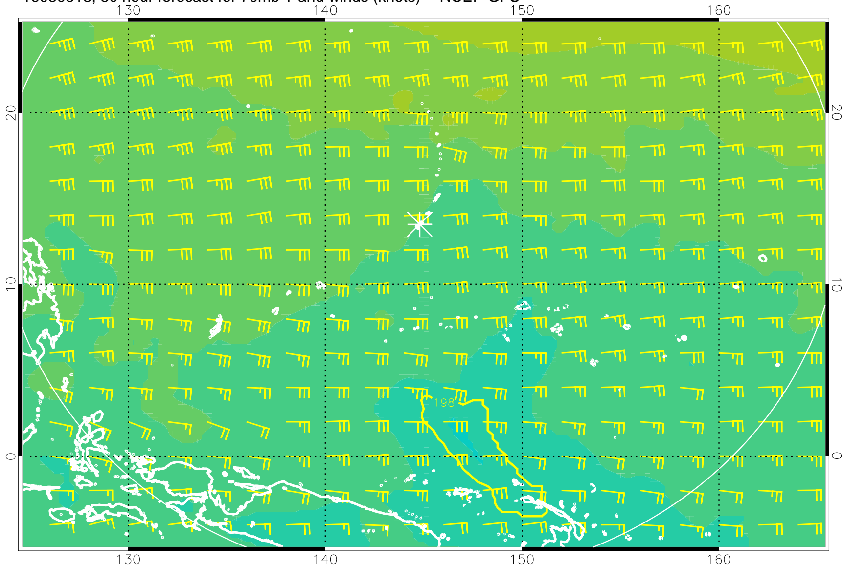
16080318, 30 hour forecast for 70mb T and winds (knots) -- NCEP GFS
