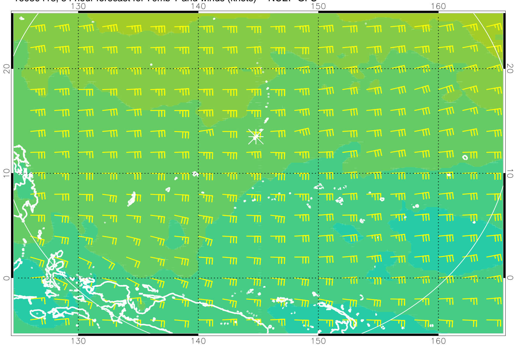
16080418, 54 hour forecast for 70mb T and winds (knots) -- NCEP GFS
