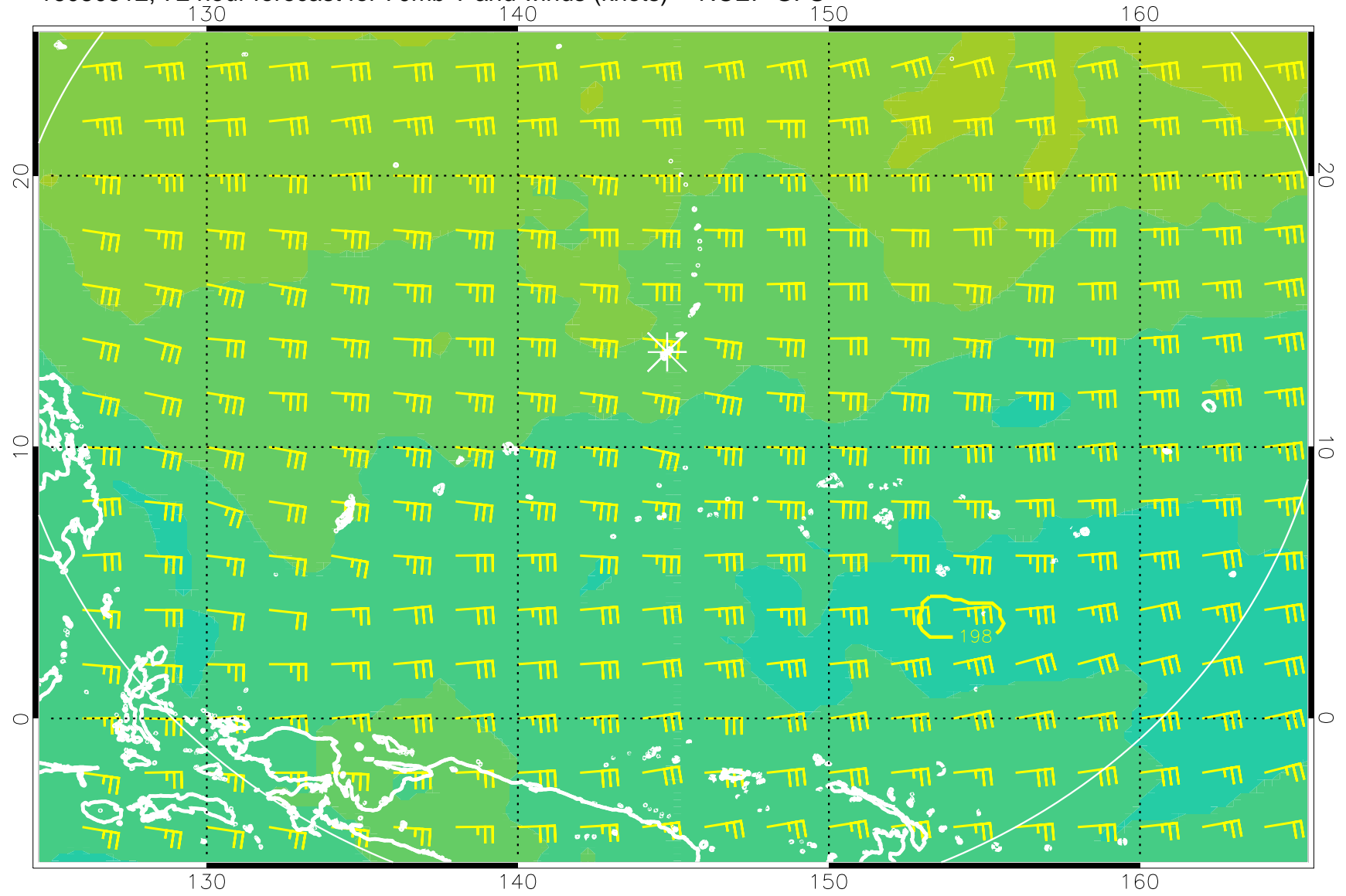
16080512, 72 hour forecast for 70mb T and winds (knots) -- NCEP GFS
