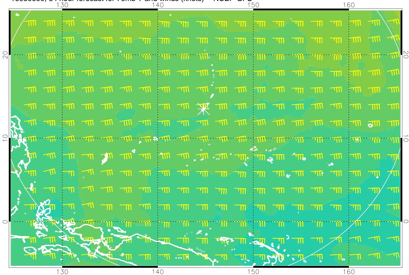
16080600, 84 hour forecast for 70mb T and winds (knots) -- NCEP GFS
