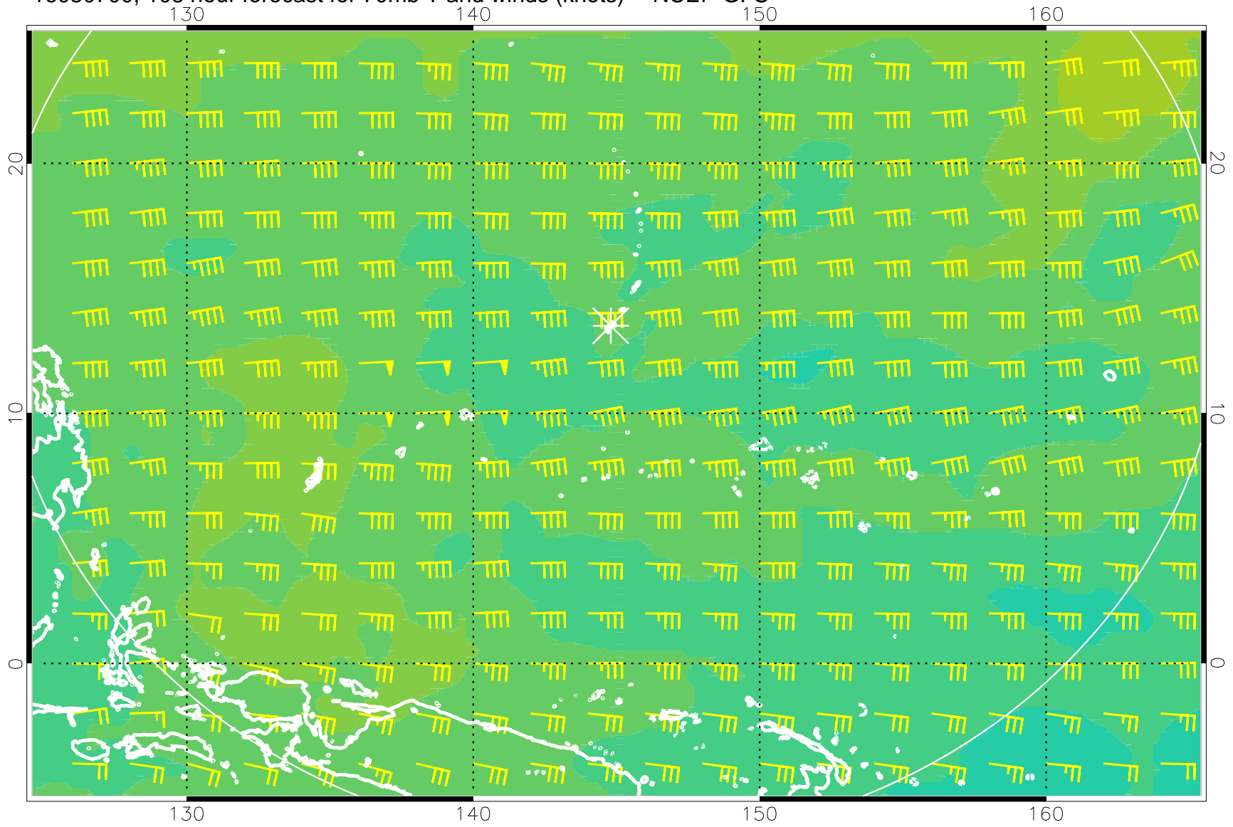
16080700, 108 hour forecast for 70mb T and winds (knots) -- NCEP GFS
