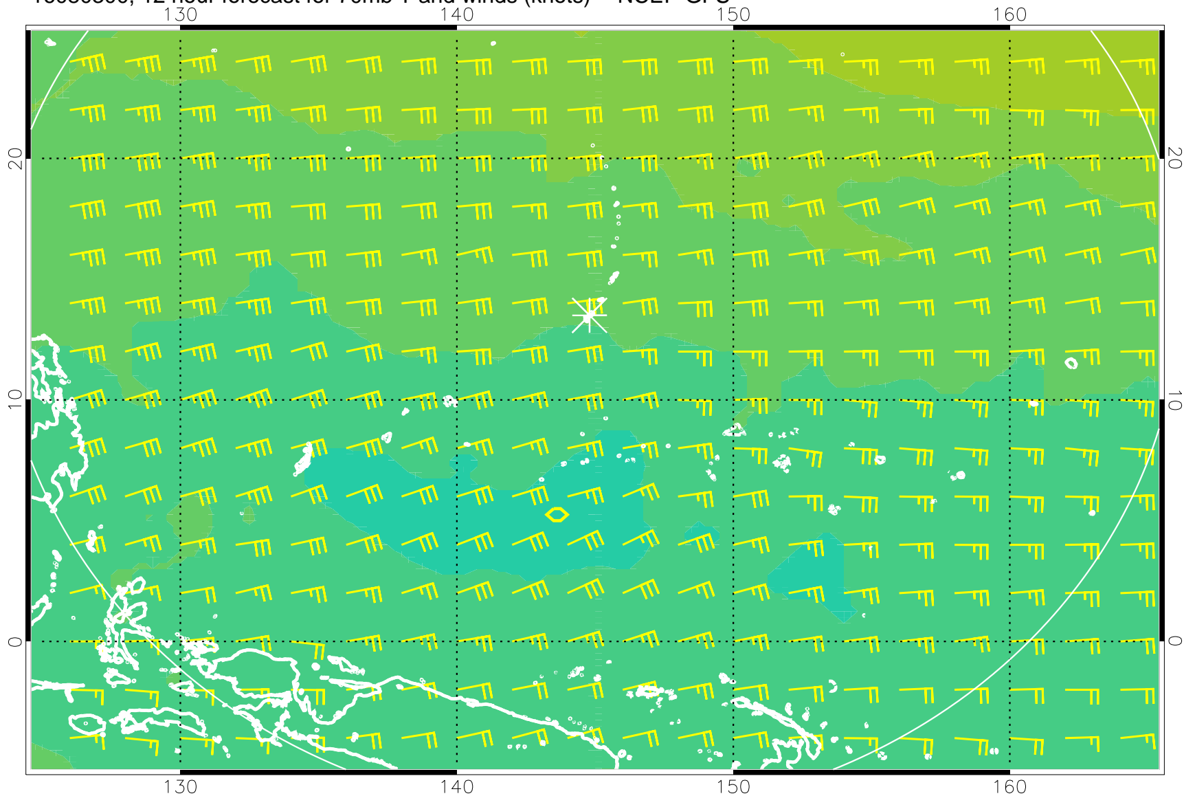
16080300, 12 hour forecast for 70mb T and winds (knots) -- NCEP GFS
