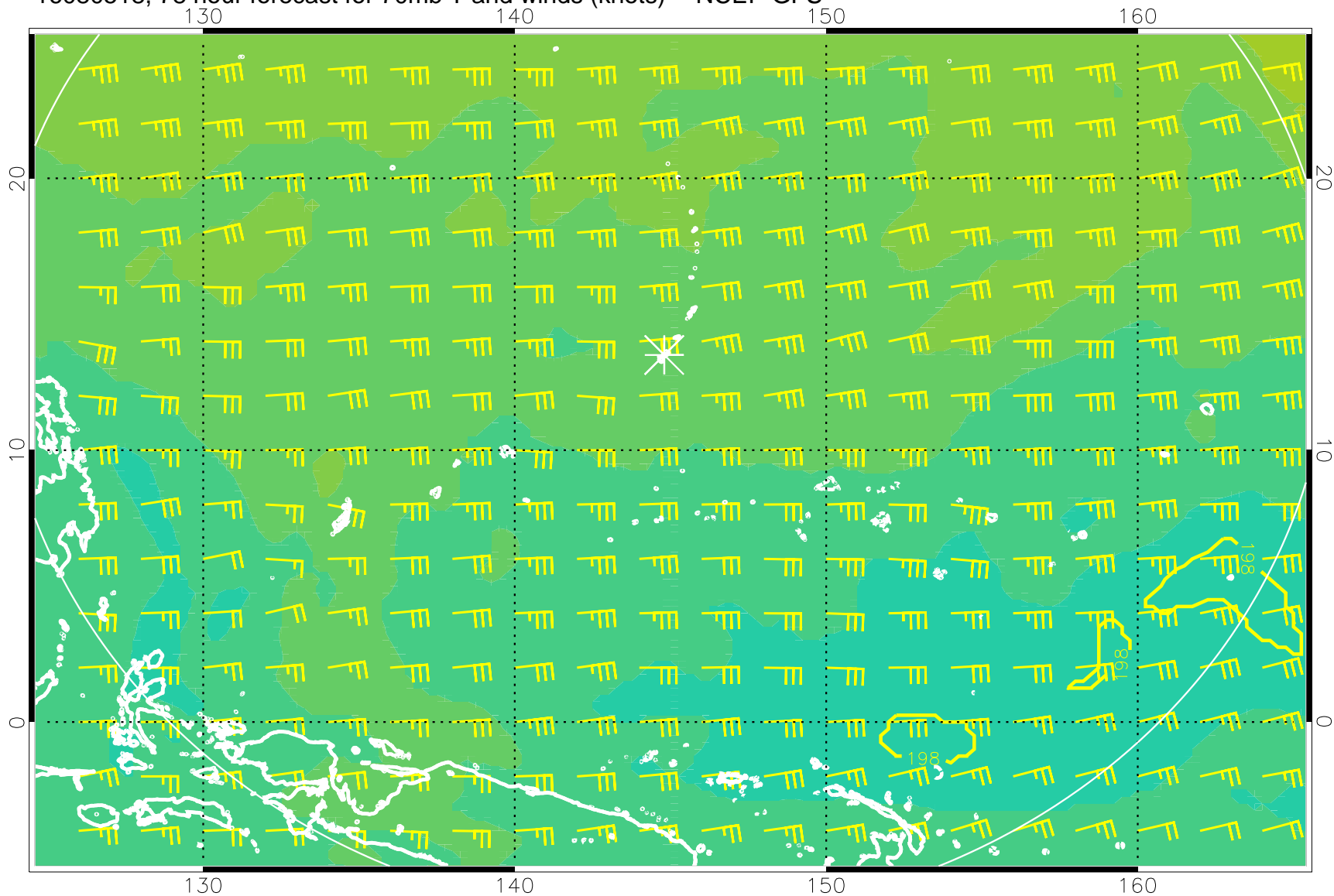
16080518, 78 hour forecast for 70mb T and winds (knots) -- NCEP GFS
