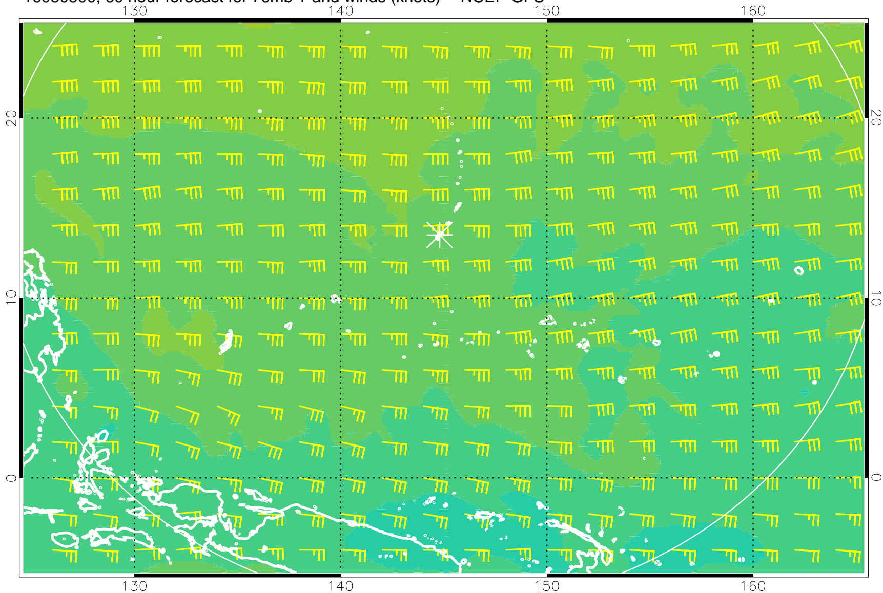
16080500, 60 hour forecast for 70mb T and winds (knots) -- NCEP GFS
