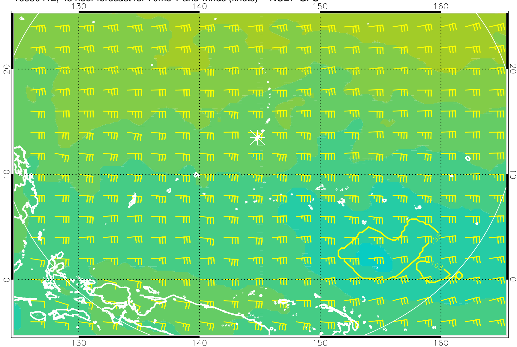
16080412, 48 hour forecast for 70mb T and winds (knots) -- NCEP GFS
