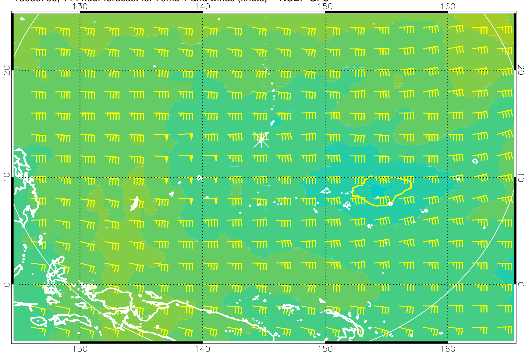
16080706, 114 hour forecast for 70mb T and winds (knots) -- NCEP GFS
