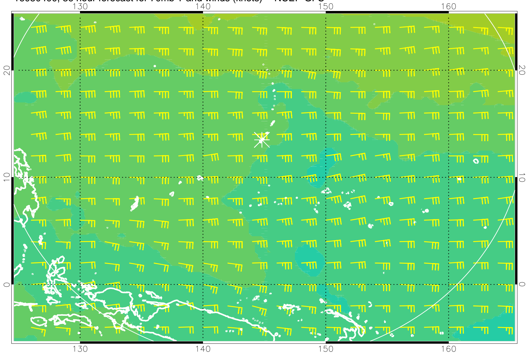
16080400, 36 hour forecast for 70mb T and winds (knots) -- NCEP GFS
