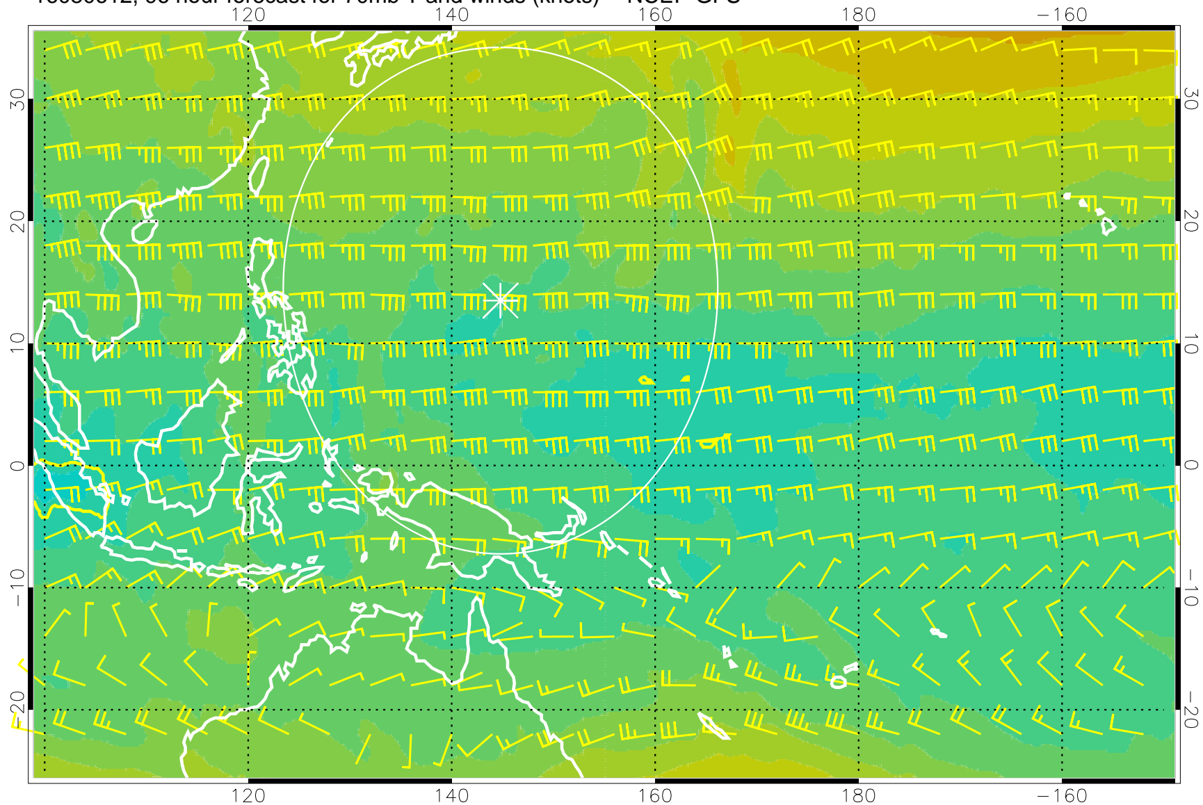
16080612, 96 hour forecast for 70mb T and winds (knots) -- NCEP GFS
