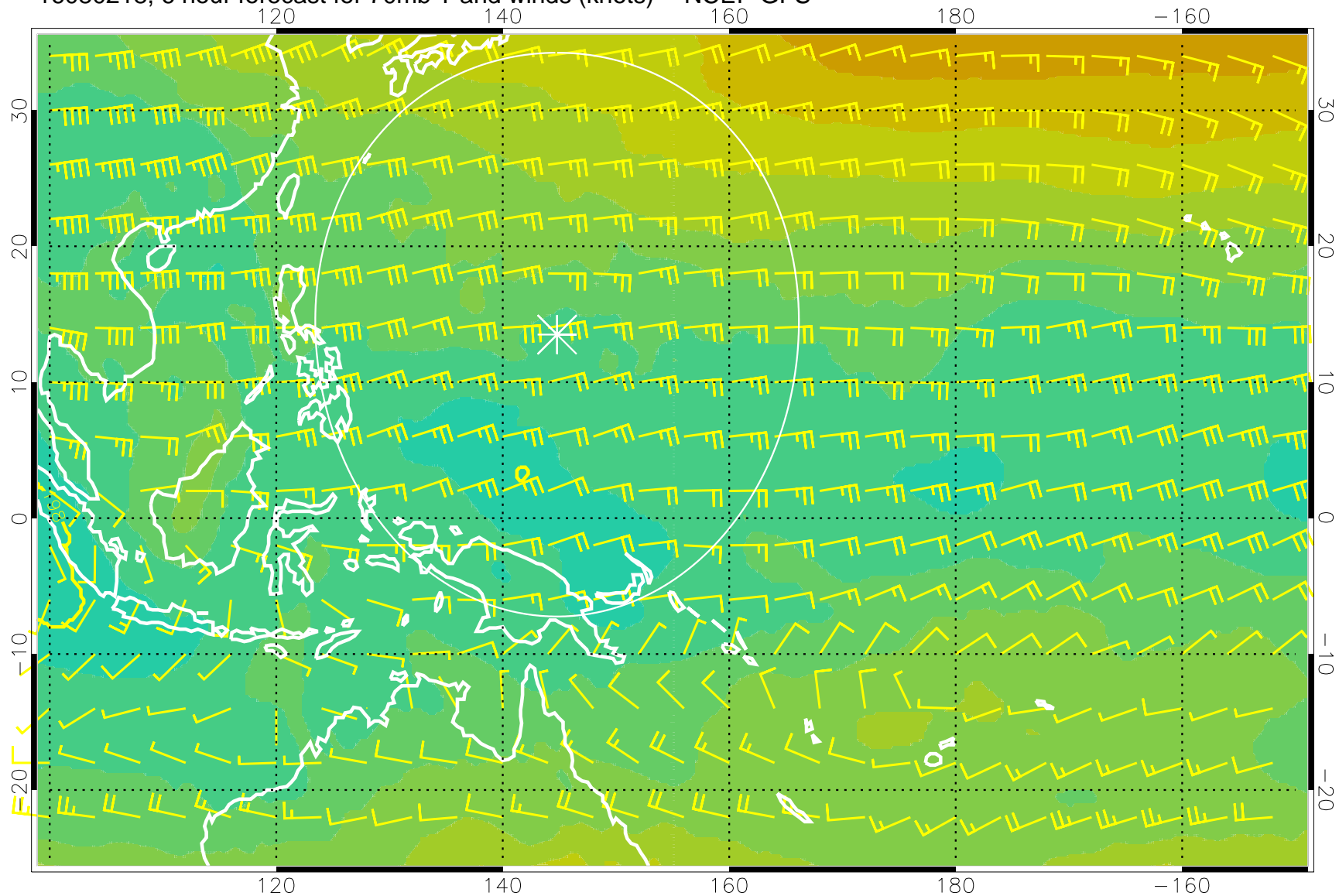
16080218, 6 hour forecast for 70mb T and winds (knots) -- NCEP GFS
