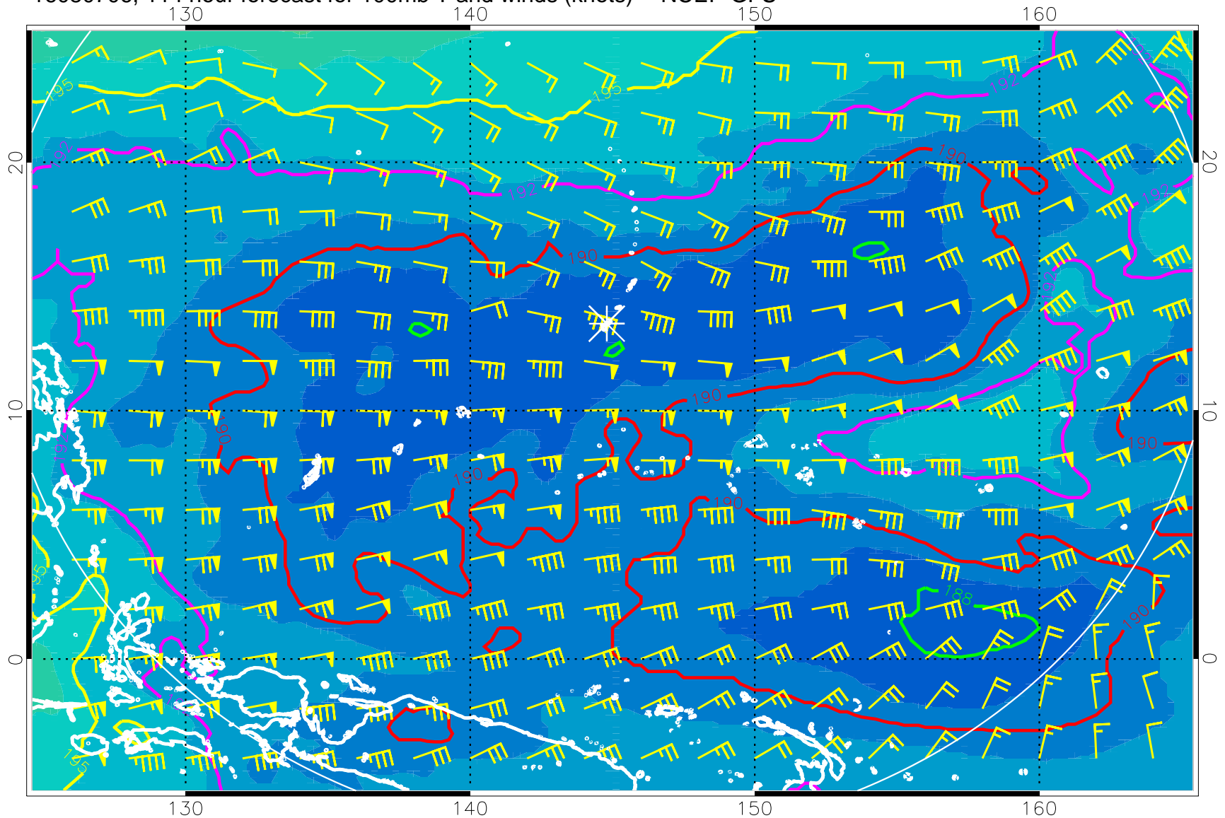
16080706, 114 hour forecast for 100mb T and winds (knots) -- NCEP GFS
