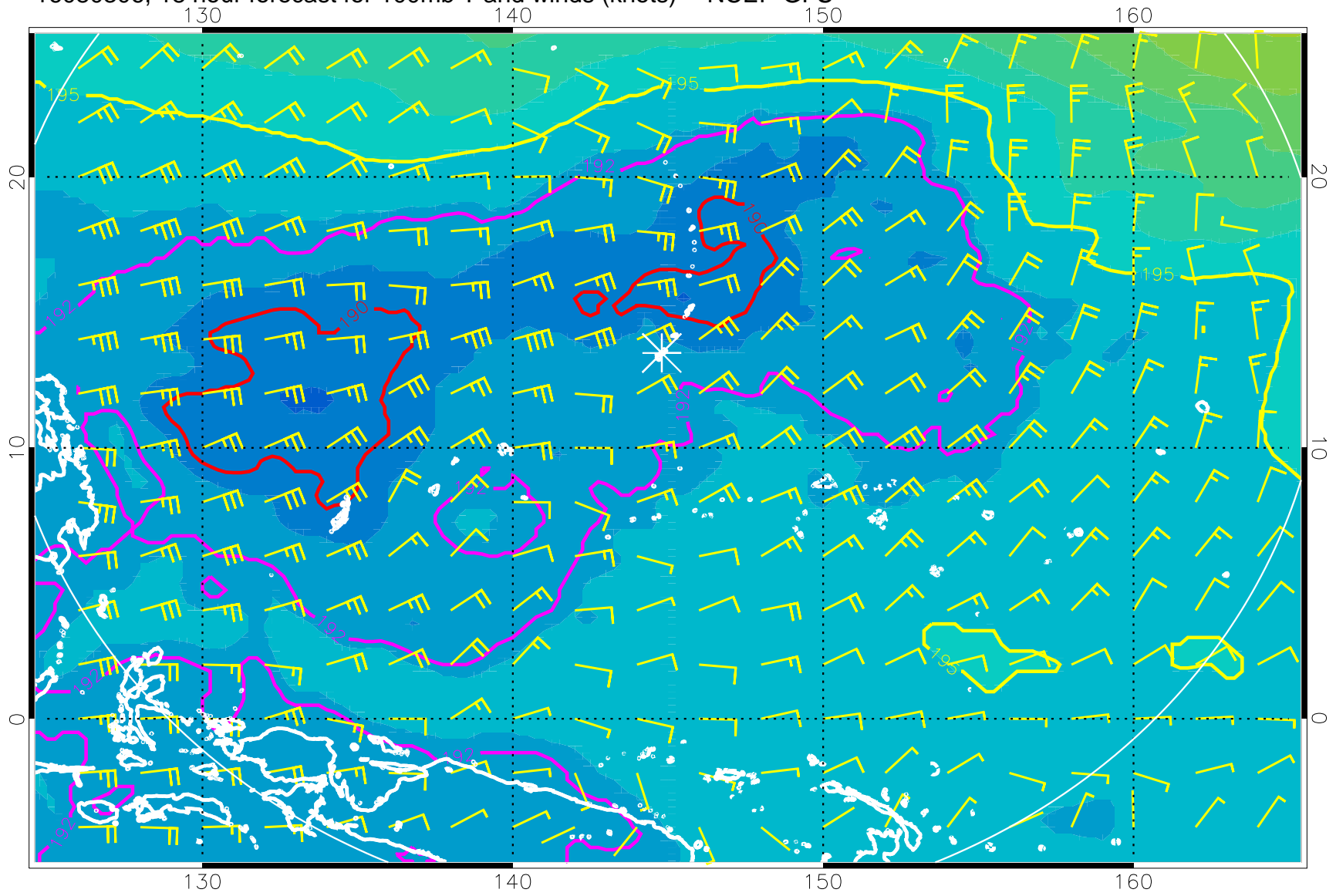
16080306, 18 hour forecast for 100mb T and winds (knots) -- NCEP GFS
