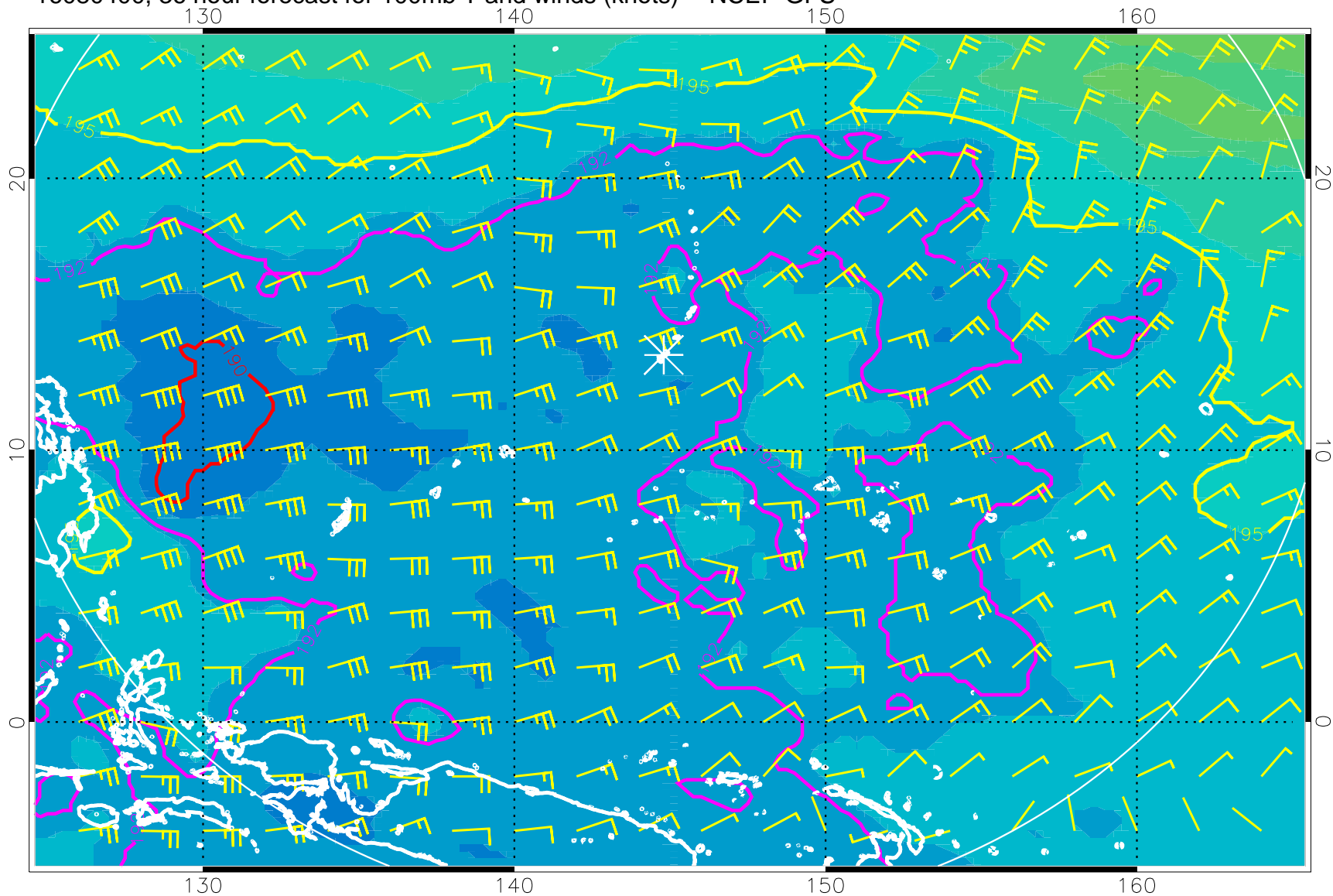
16080400, 36 hour forecast for 100mb T and winds (knots) -- NCEP GFS
