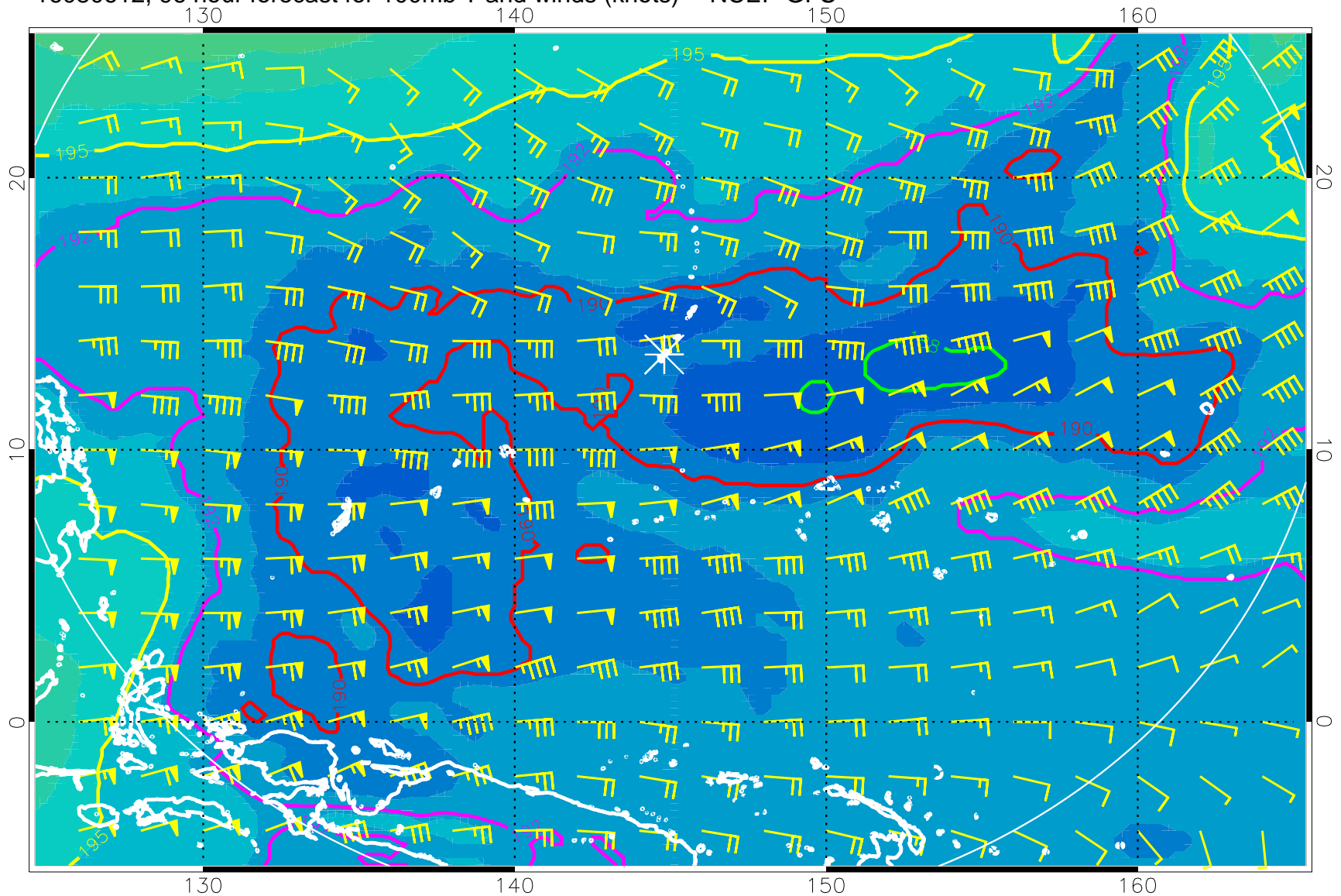
16080612, 96 hour forecast for 100mb T and winds (knots) -- NCEP GFS
