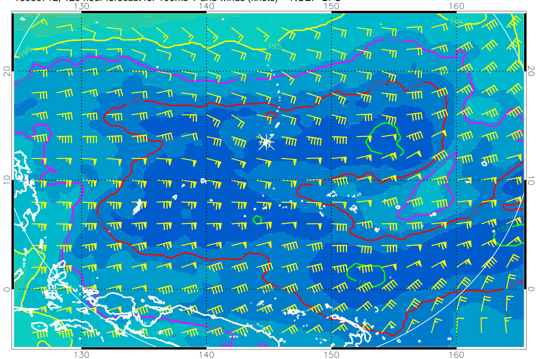
16080712, 120 hour forecast for 100mb T and winds (knots) -- NCEP GFS
