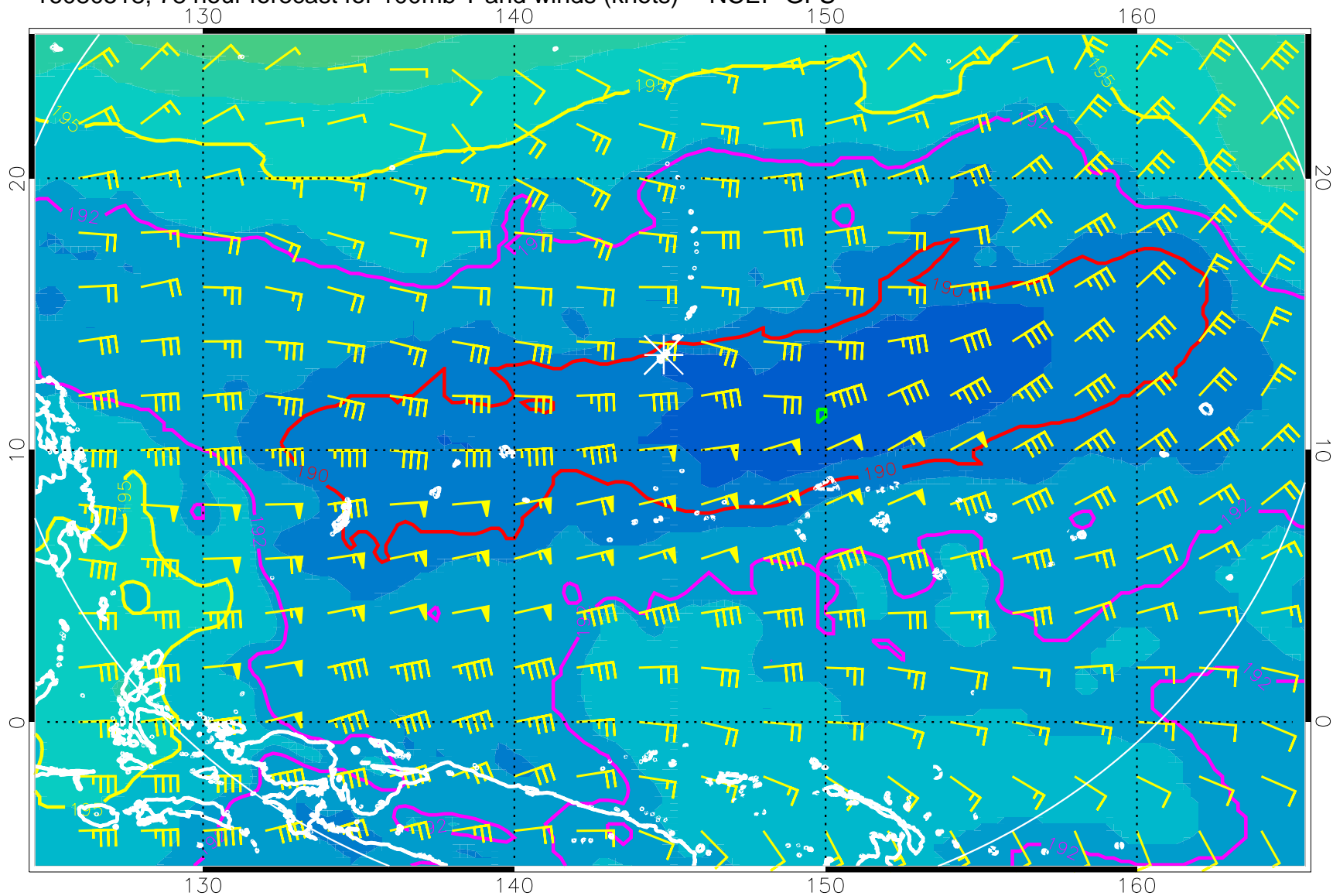
16080518, 78 hour forecast for 100mb T and winds (knots) -- NCEP GFS
