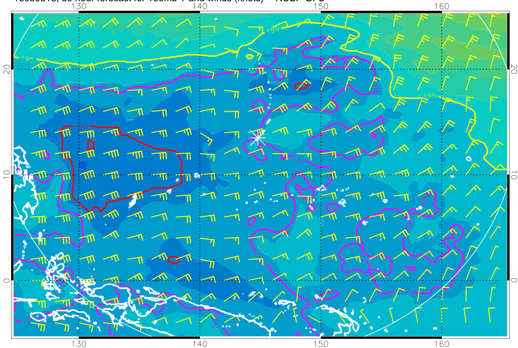
16080318, 30 hour forecast for 100mb T and winds (knots) -- NCEP GFS
