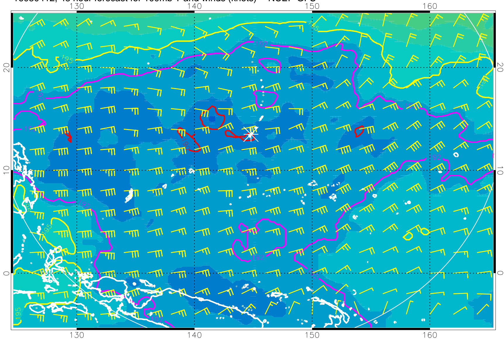
16080412, 48 hour forecast for 100mb T and winds (knots) -- NCEP GFS
