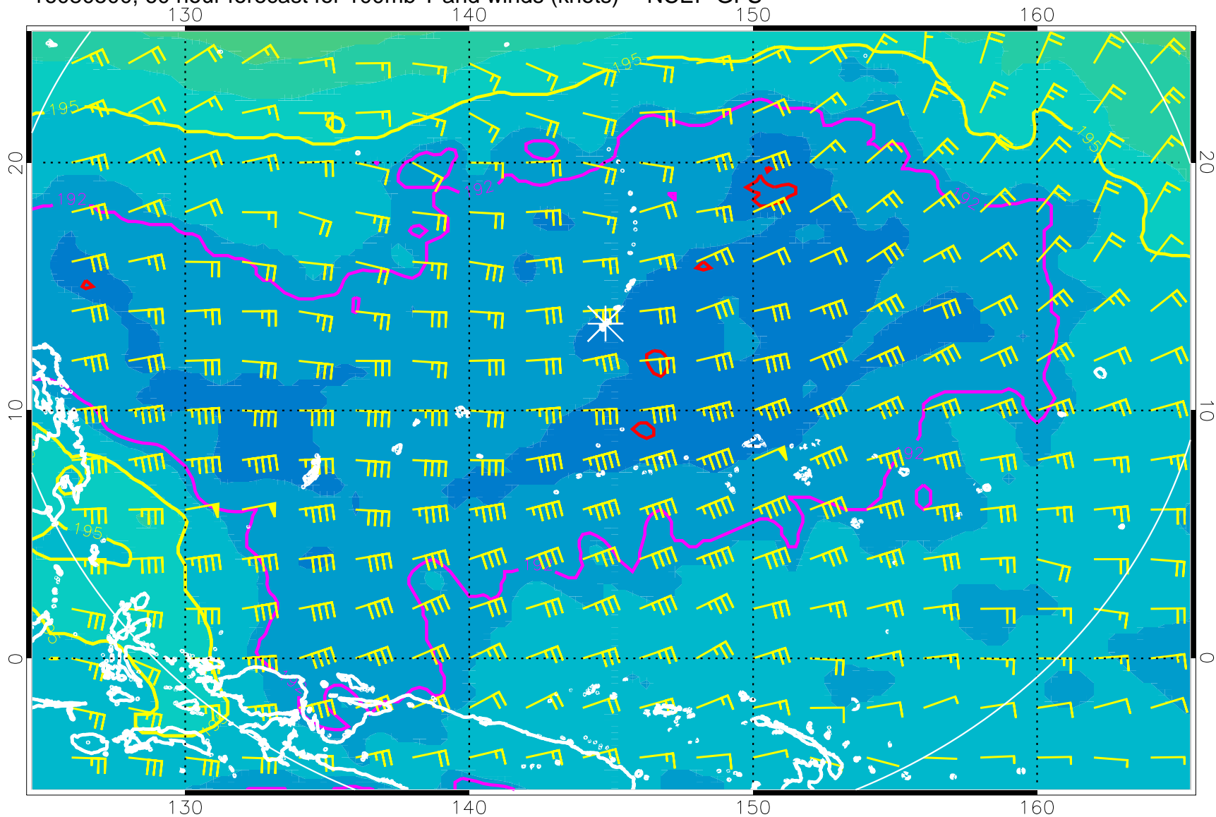
16080500, 60 hour forecast for 100mb T and winds (knots) -- NCEP GFS
