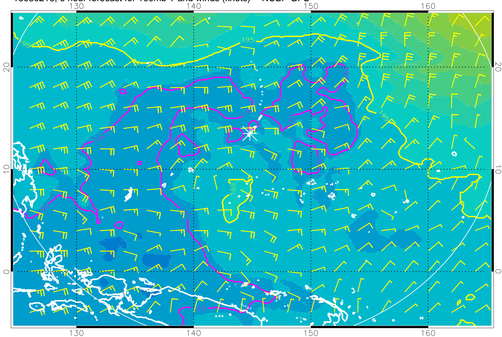
16080218, 6 hour forecast for 100mb T and winds (knots) -- NCEP GFS
