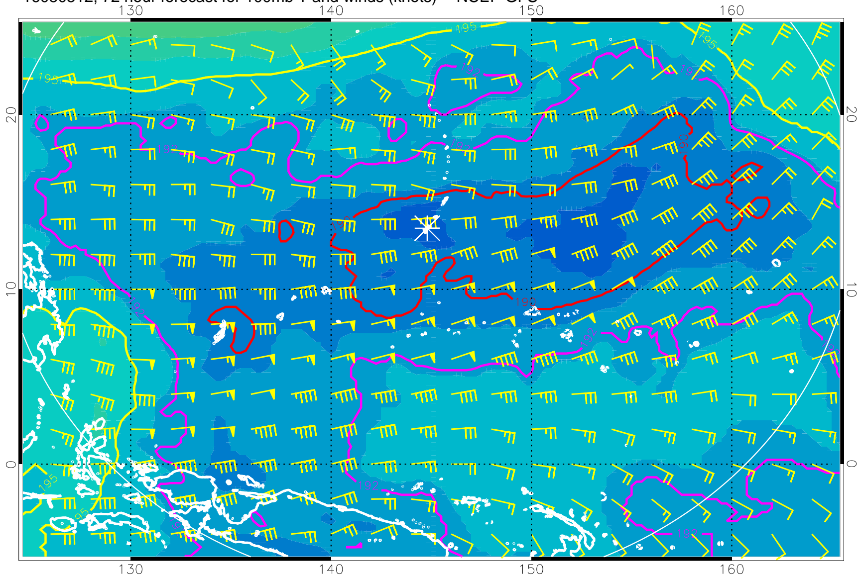
16080512, 72 hour forecast for 100mb T and winds (knots) -- NCEP GFS
