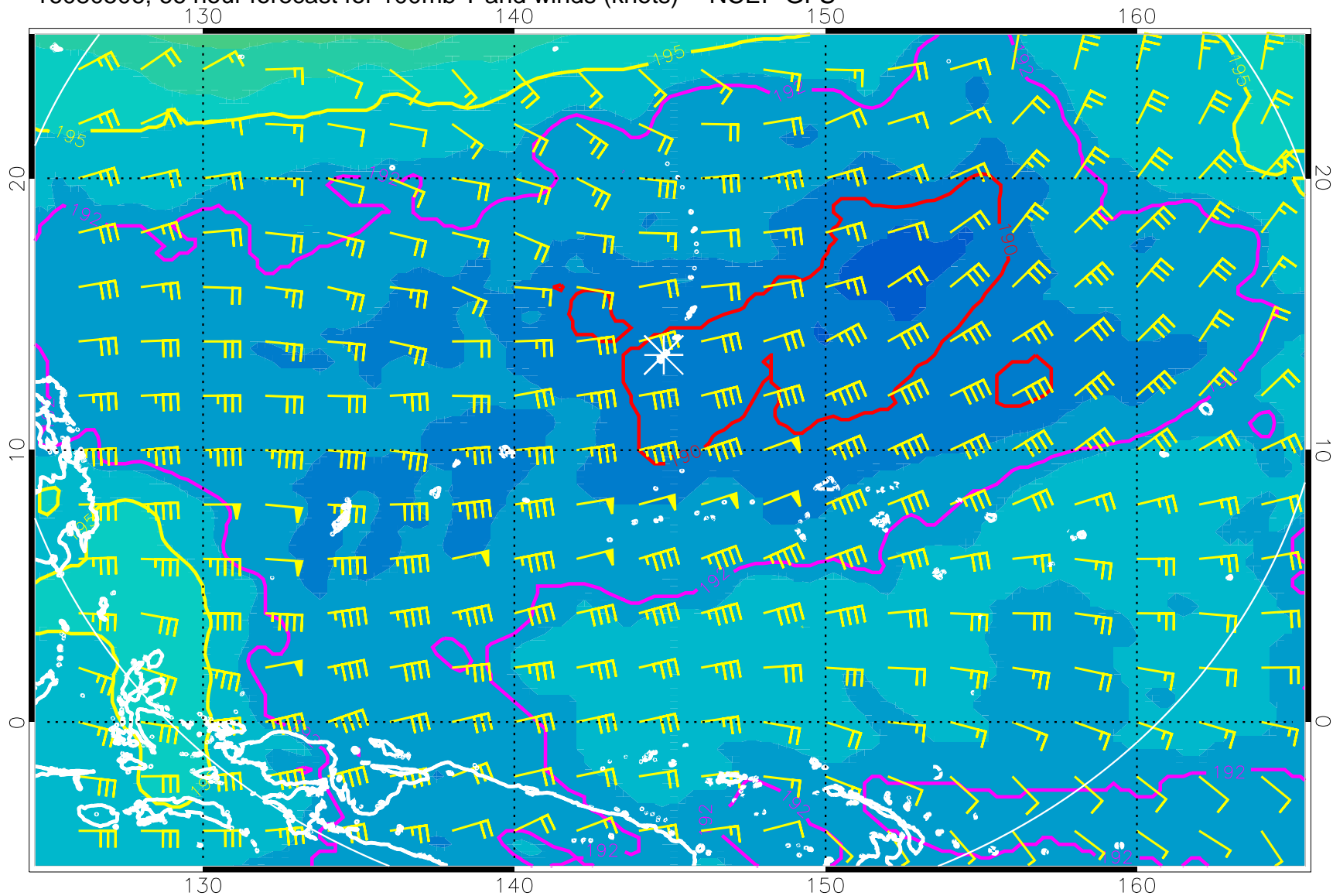
16080506, 66 hour forecast for 100mb T and winds (knots) -- NCEP GFS
