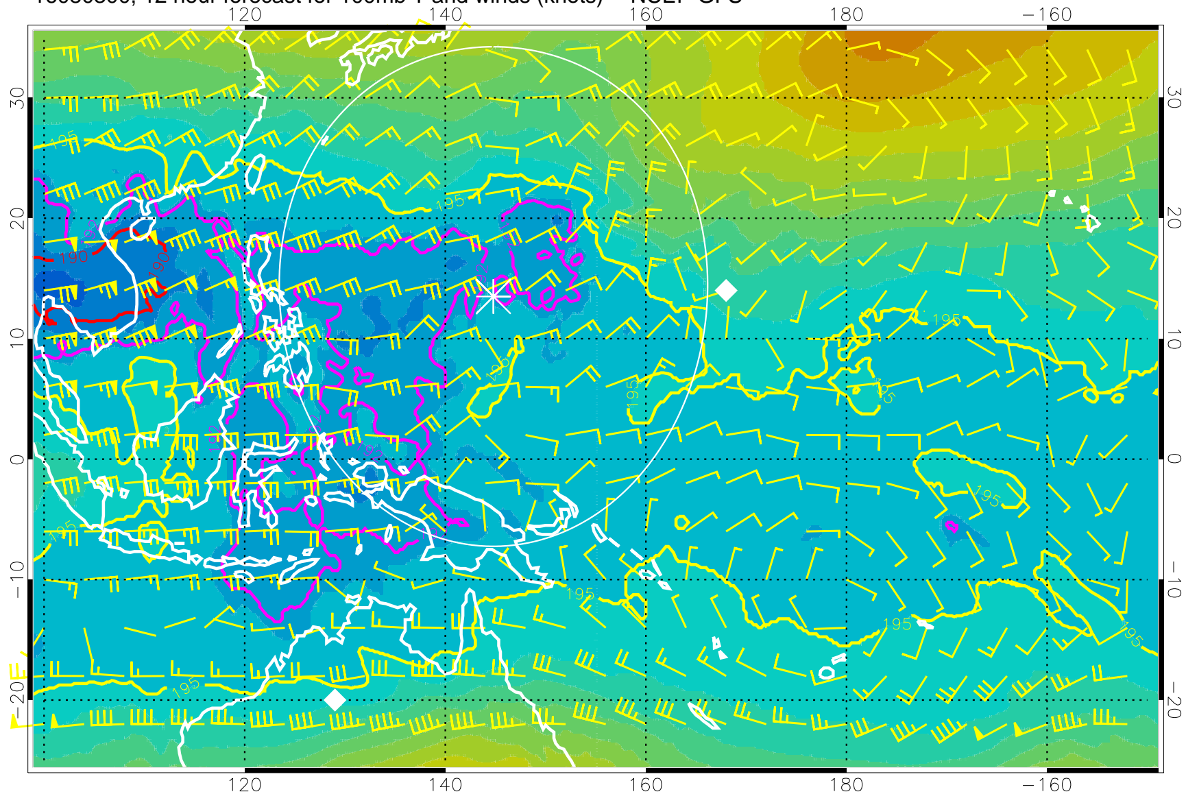
16080300, 12 hour forecast for 100mb T and winds (knots) -- NCEP GFS
