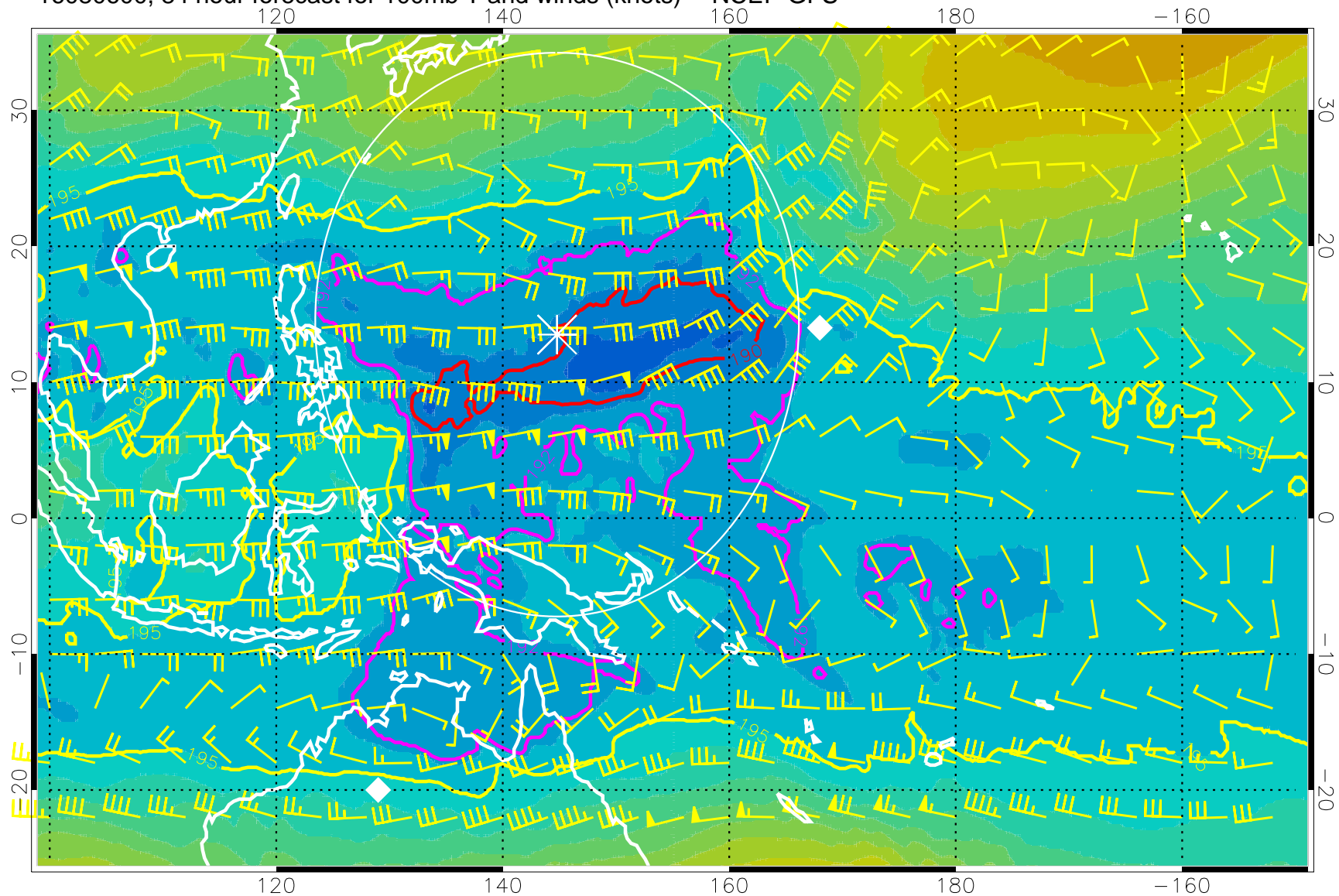
16080600, 84 hour forecast for 100mb T and winds (knots) -- NCEP GFS
