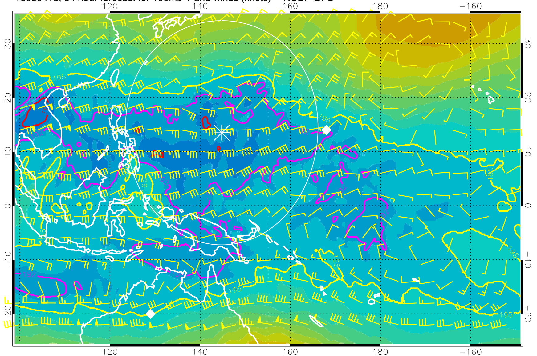
16080418, 54 hour forecast for 100mb T and winds (knots) -- NCEP GFS
