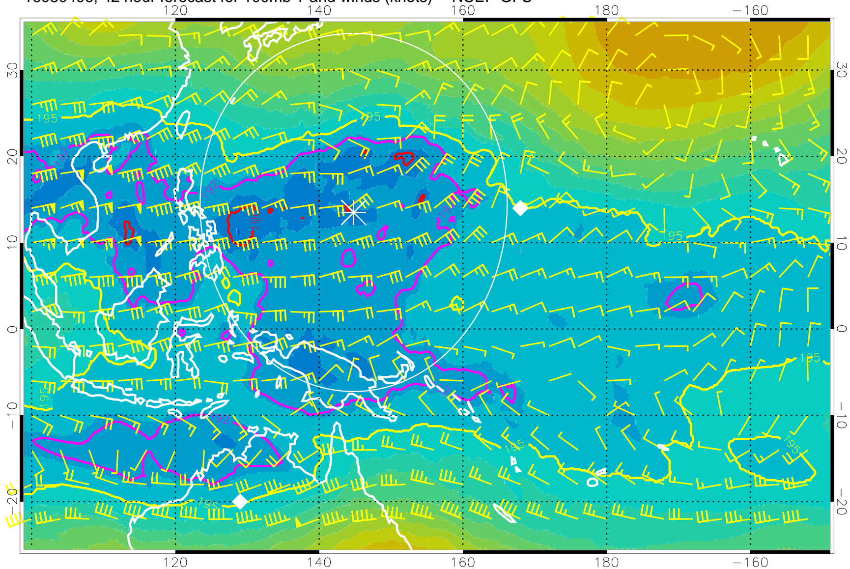
16080406, 42 hour forecast for 100mb T and winds (knots) -- NCEP GFS
