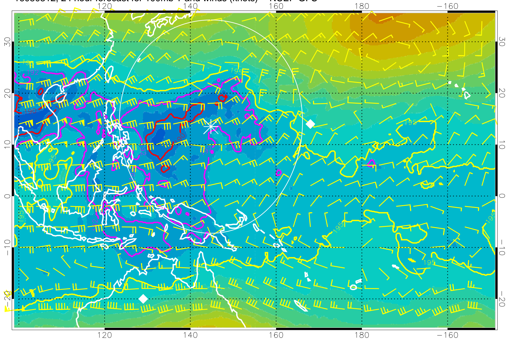
16080312, 24 hour forecast for 100mb T and winds (knots) -- NCEP GFS
