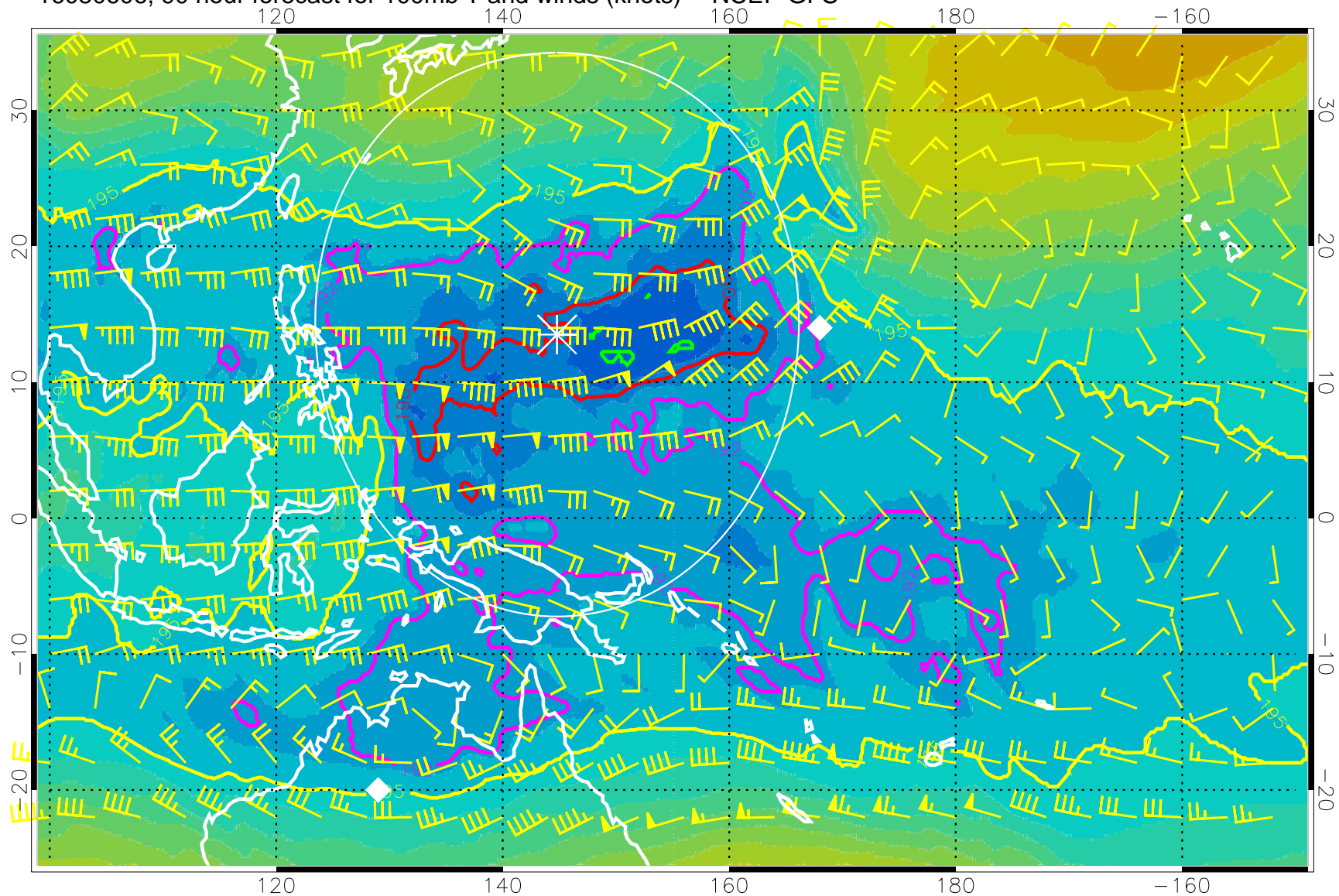
16080606, 90 hour forecast for 100mb T and winds (knots) -- NCEP GFS
