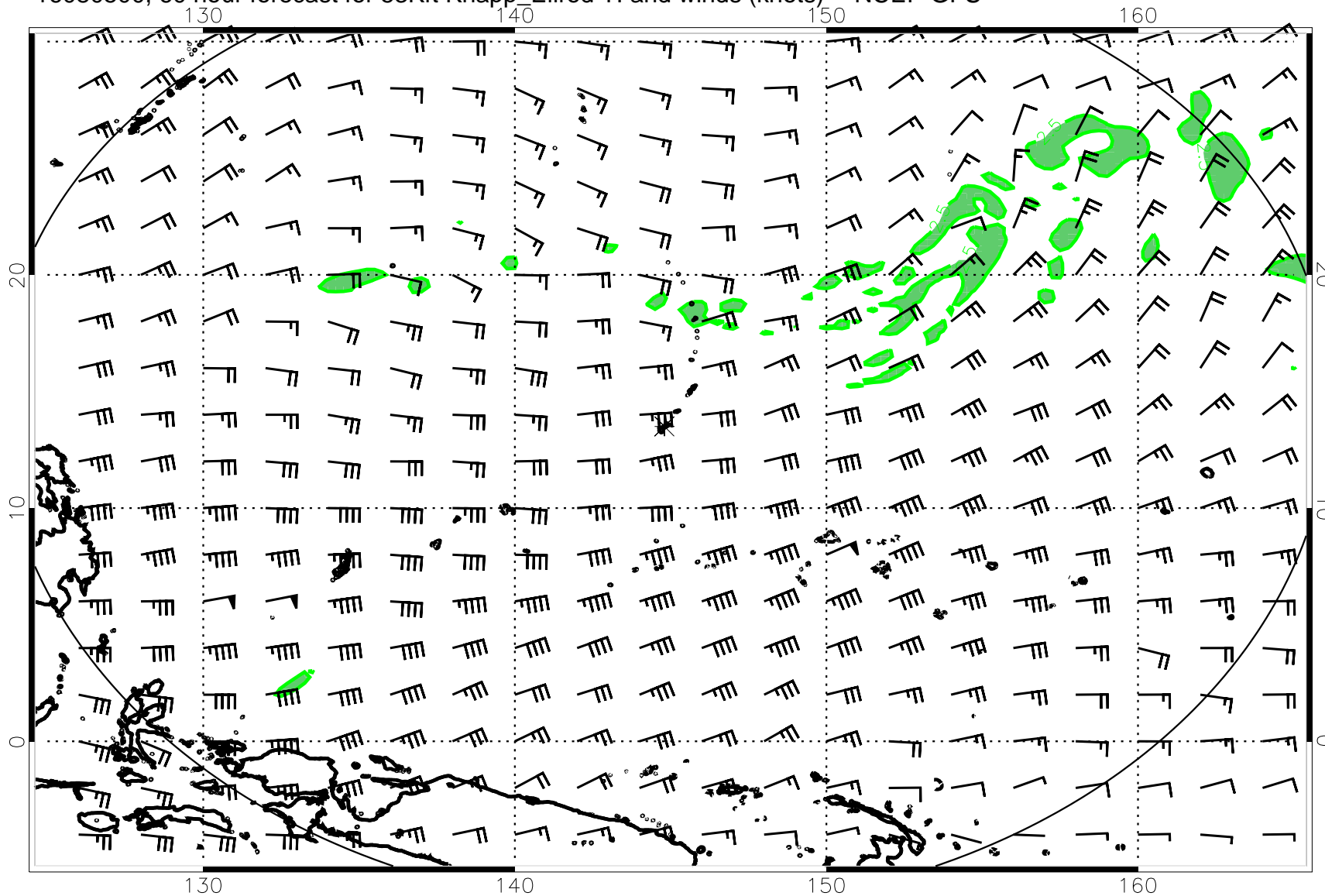
16080500, 60 hour forecast for 53Kft Knapp_Ellrod TI and winds (knots) -- NCEP GFS
