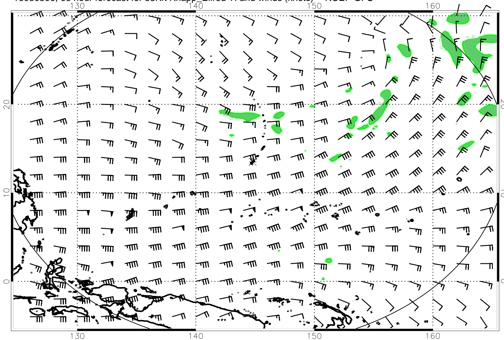
16080506, 66 hour forecast for 53Kft Knapp_Ellrod TI and winds (knots) -- NCEP GFS
