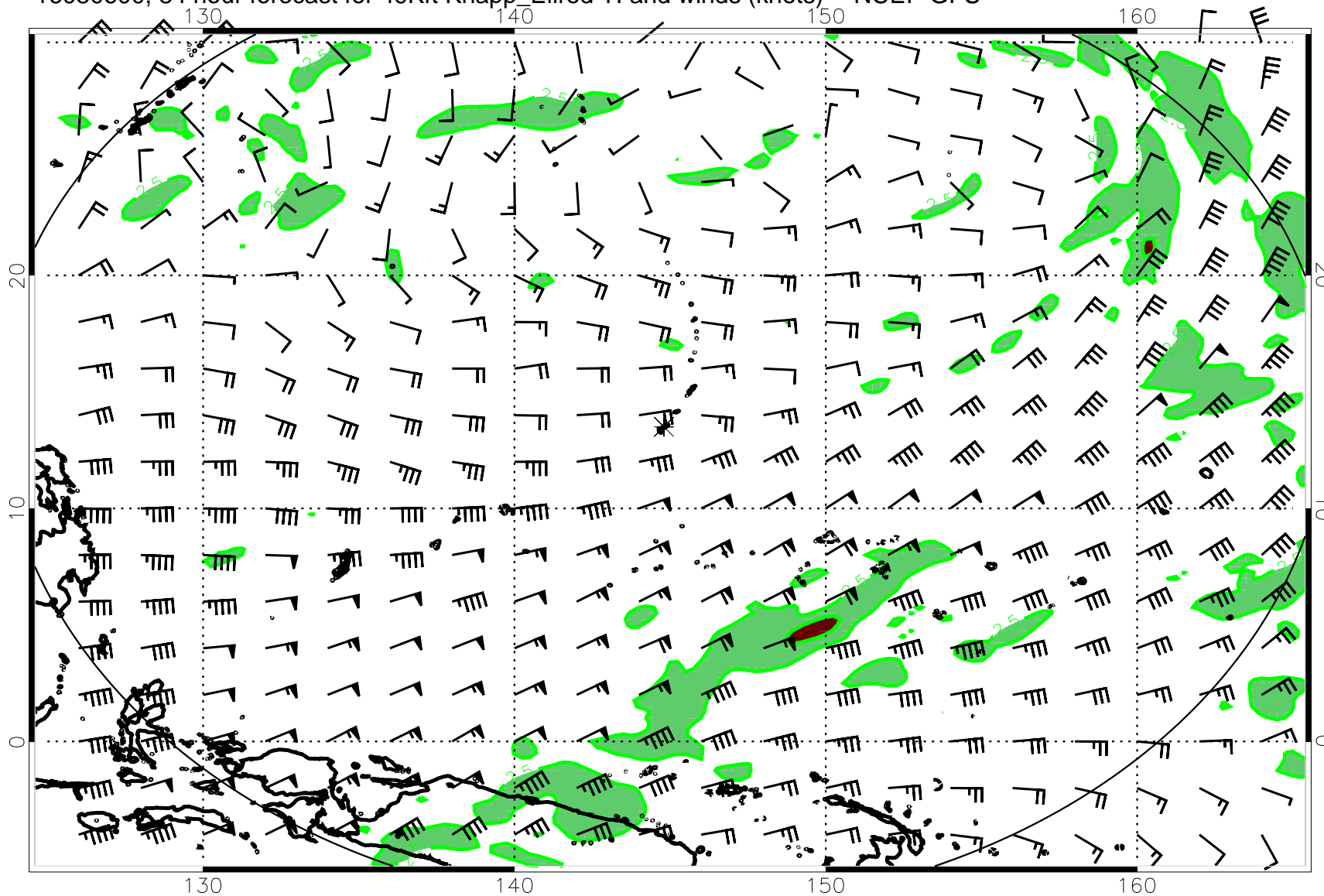
16080600, 84 hour forecast for 49Kft Knapp_Ellrod TI and winds (knots) -- NCEP GFS
