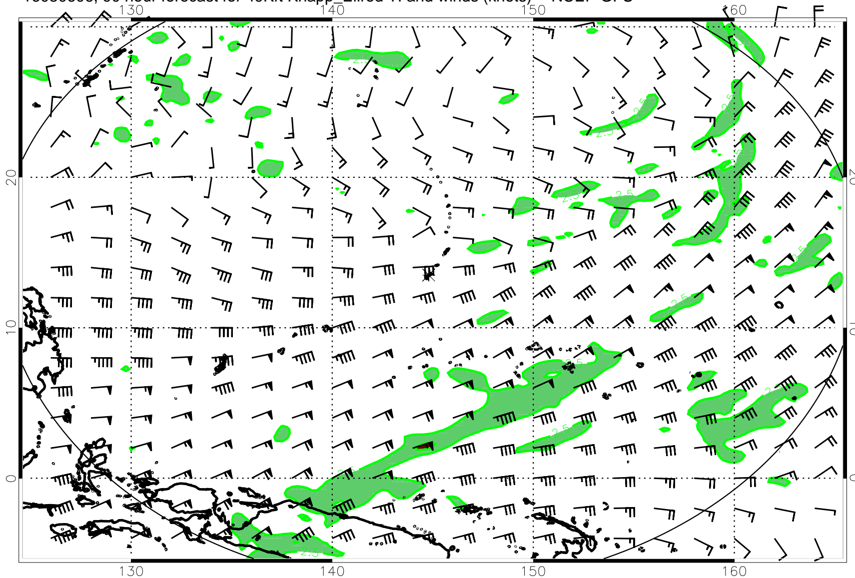
16080606, 90 hour forecast for 49Kft Knapp_Ellrod TI and winds (knots) -- NCEP GFS
