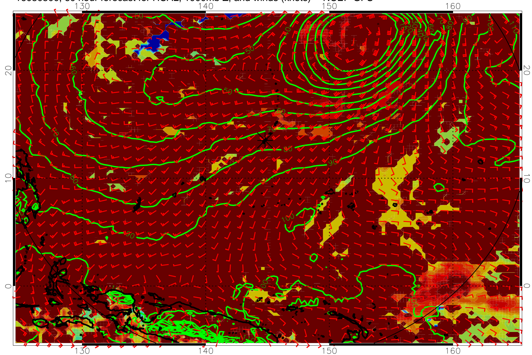
16080500, 60 hour forecast for HCAL, 1000mb Z, and winds (knots) -- NCEP GFS
