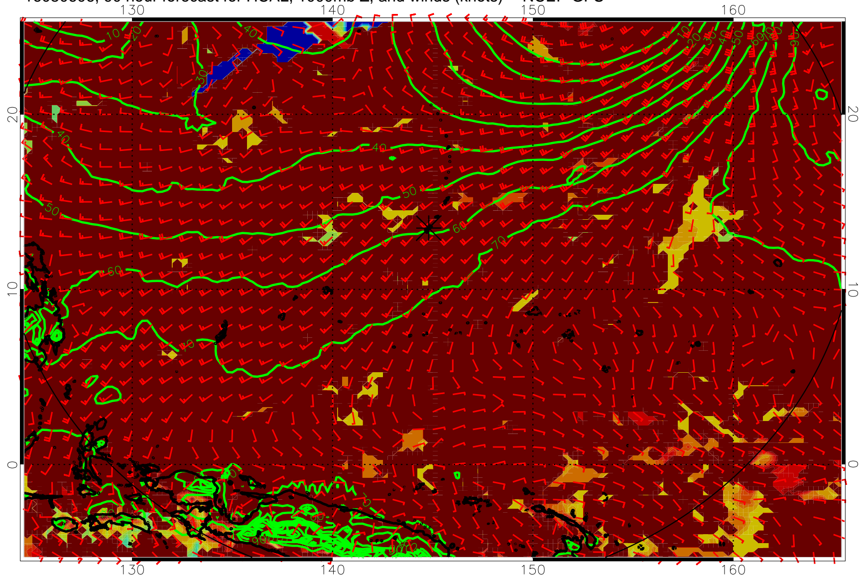
16080606, 90 hour forecast for HCAL, 1000mb Z, and winds (knots) -- NCEP GFS
