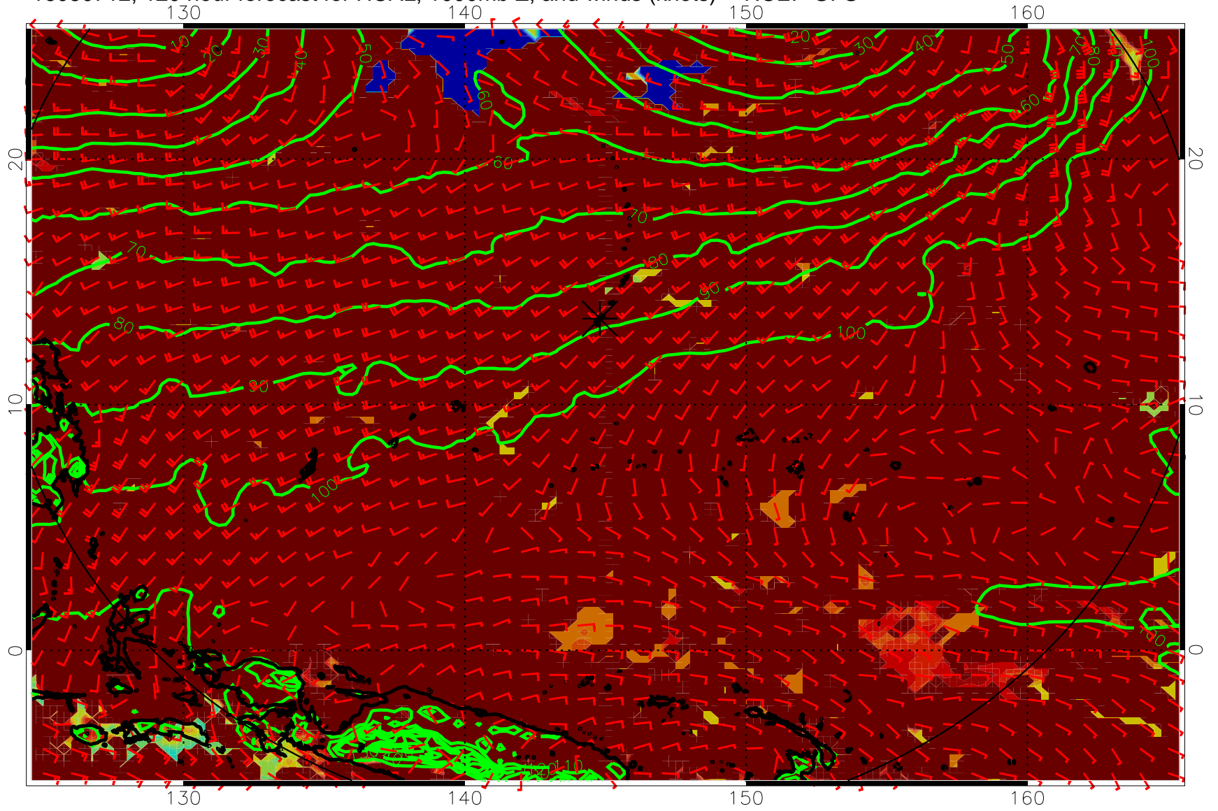
16080712, 120 hour forecast for HCAL, 1000mb Z, and winds (knots) -- NCEP GFS
