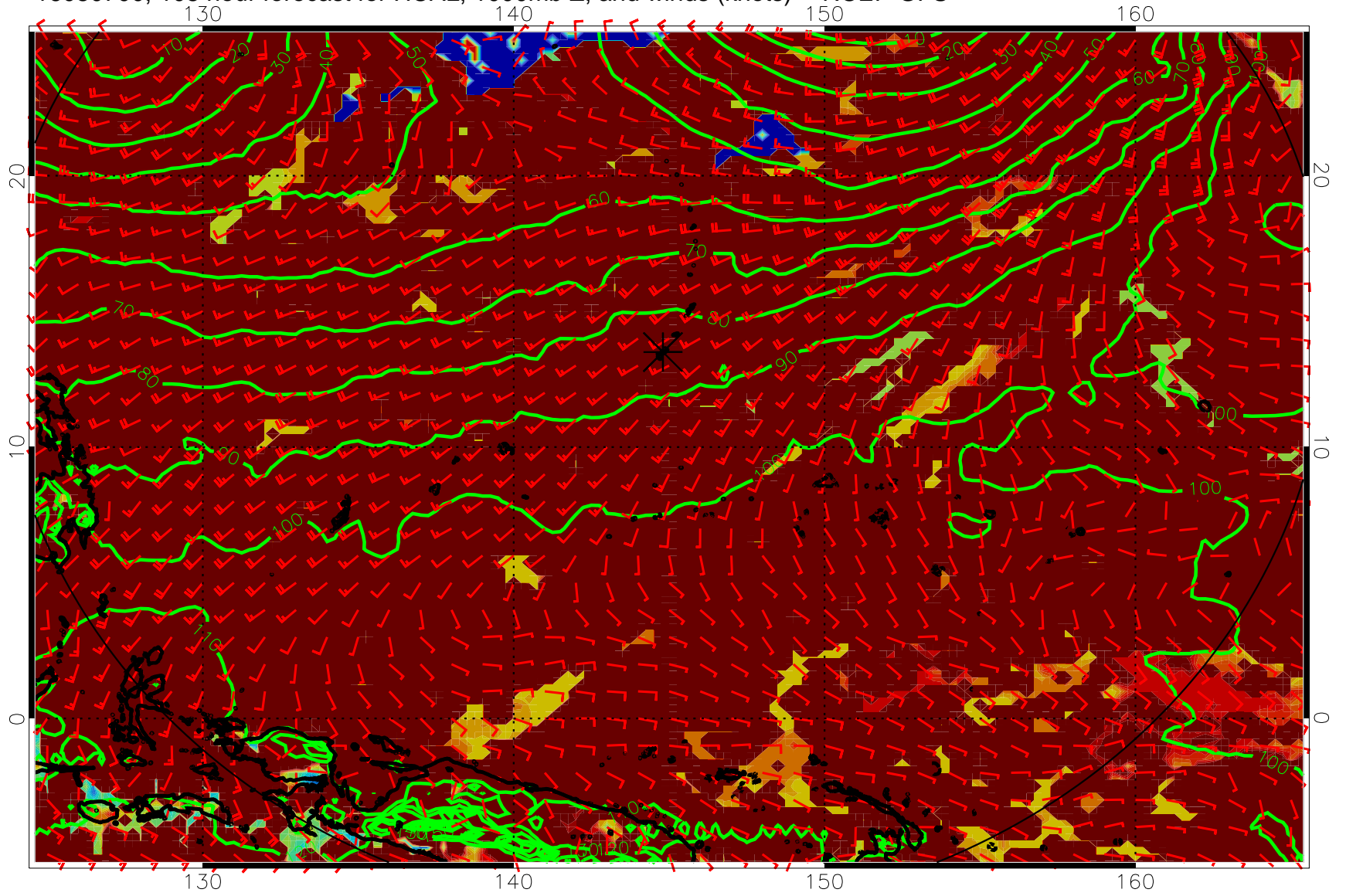
16080700, 108 hour forecast for HCAL, 1000mb Z, and winds (knots) -- NCEP GFS
