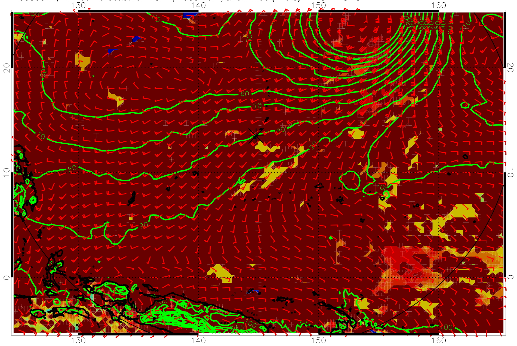
16080512, 72 hour forecast for HCAL, 1000mb Z, and winds (knots) -- NCEP GFS
