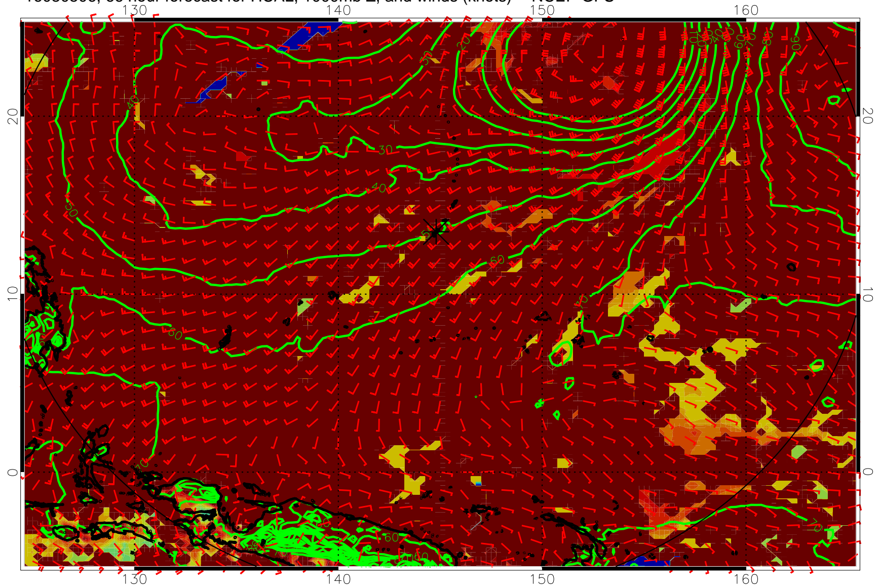
16080506, 66 hour forecast for HCAL, 1000mb Z, and winds (knots) -- NCEP GFS
