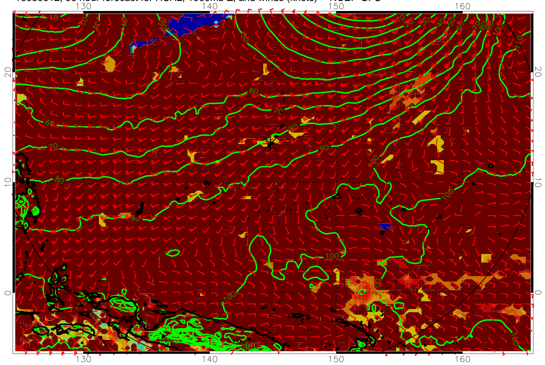
16080612, 96 hour forecast for HCAL, 1000mb Z, and winds (knots) -- NCEP GFS
