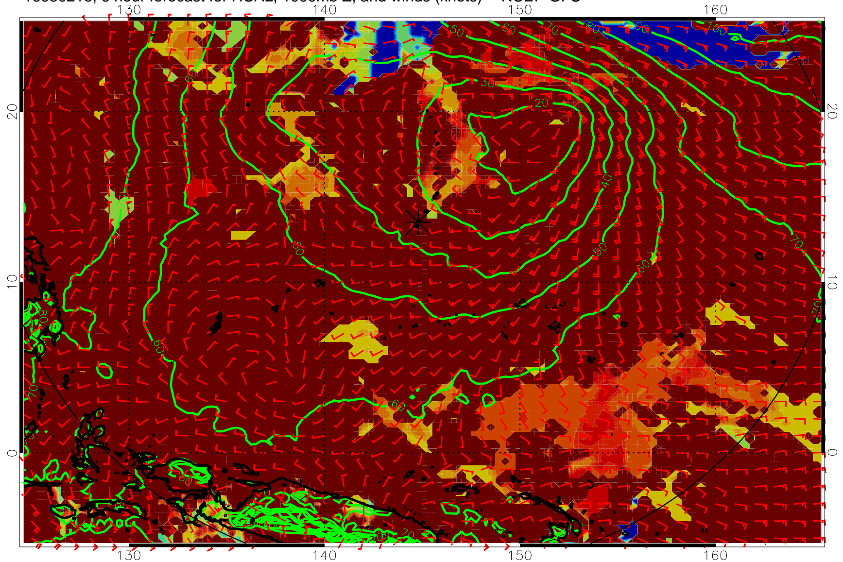
16080218, 6 hour forecast for HCAL, 1000mb Z, and winds (knots) -- NCEP GFS
