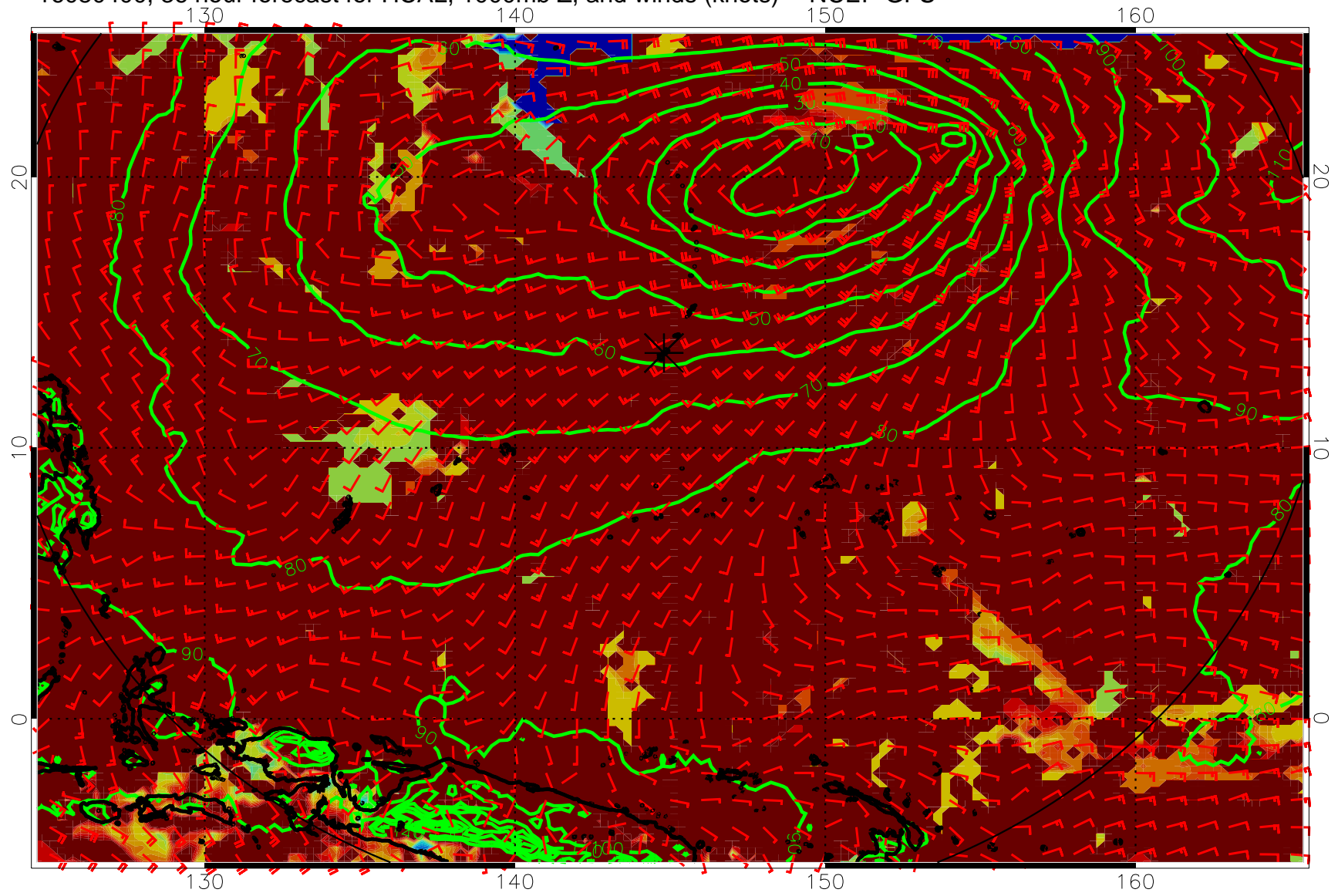
16080400, 36 hour forecast for HCAL, 1000mb Z, and winds (knots) -- NCEP GFS
