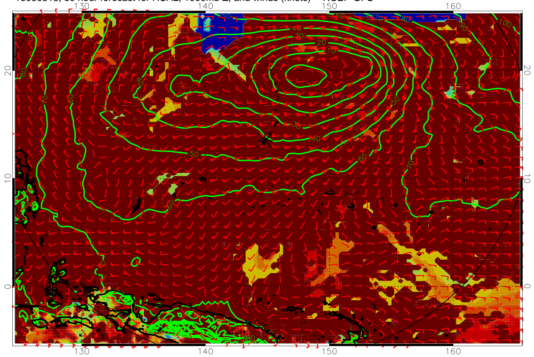
16080318, 30 hour forecast for HCAL, 1000mb Z, and winds (knots) -- NCEP GFS
