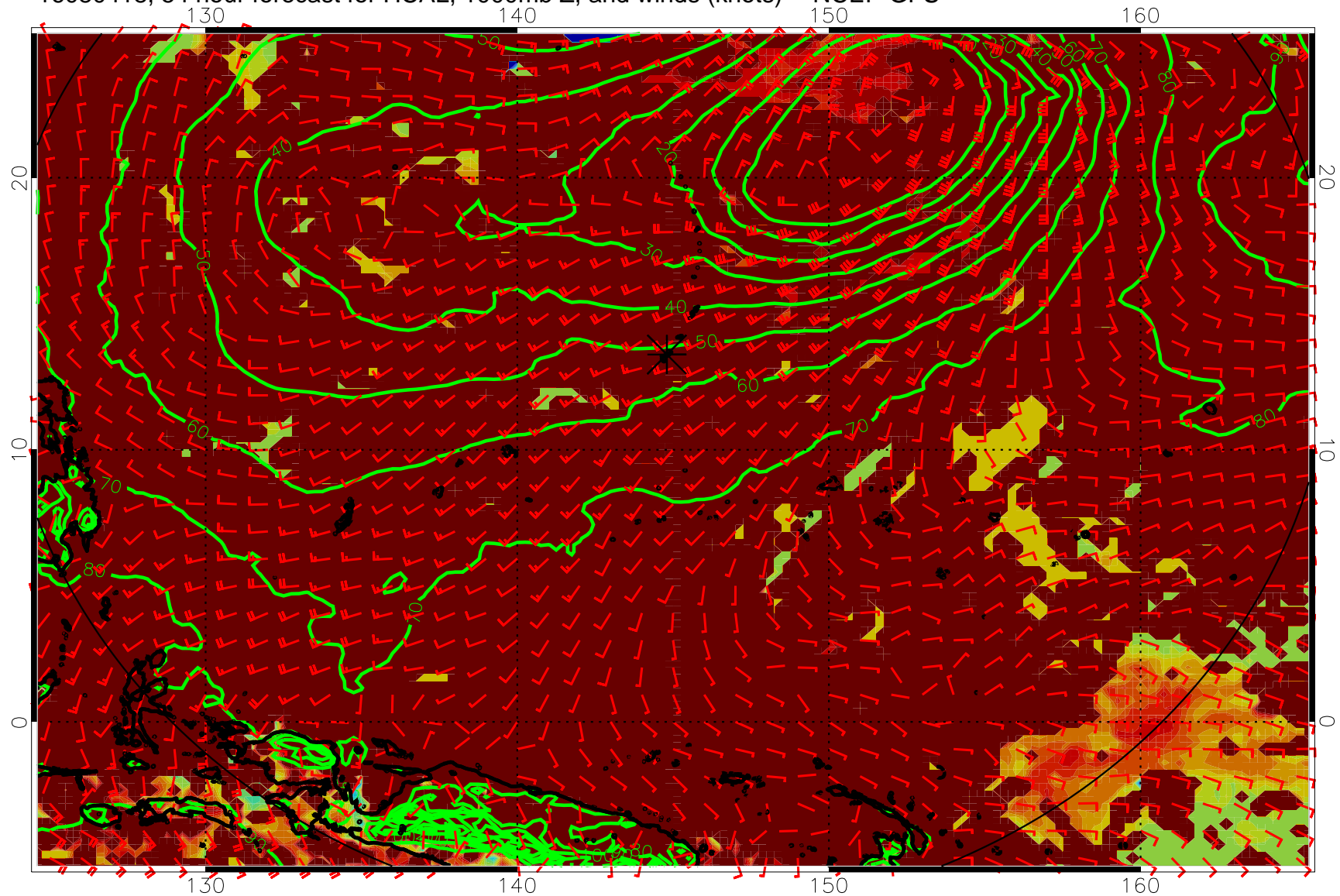
16080418, 54 hour forecast for HCAL, 1000mb Z, and winds (knots) -- NCEP GFS
