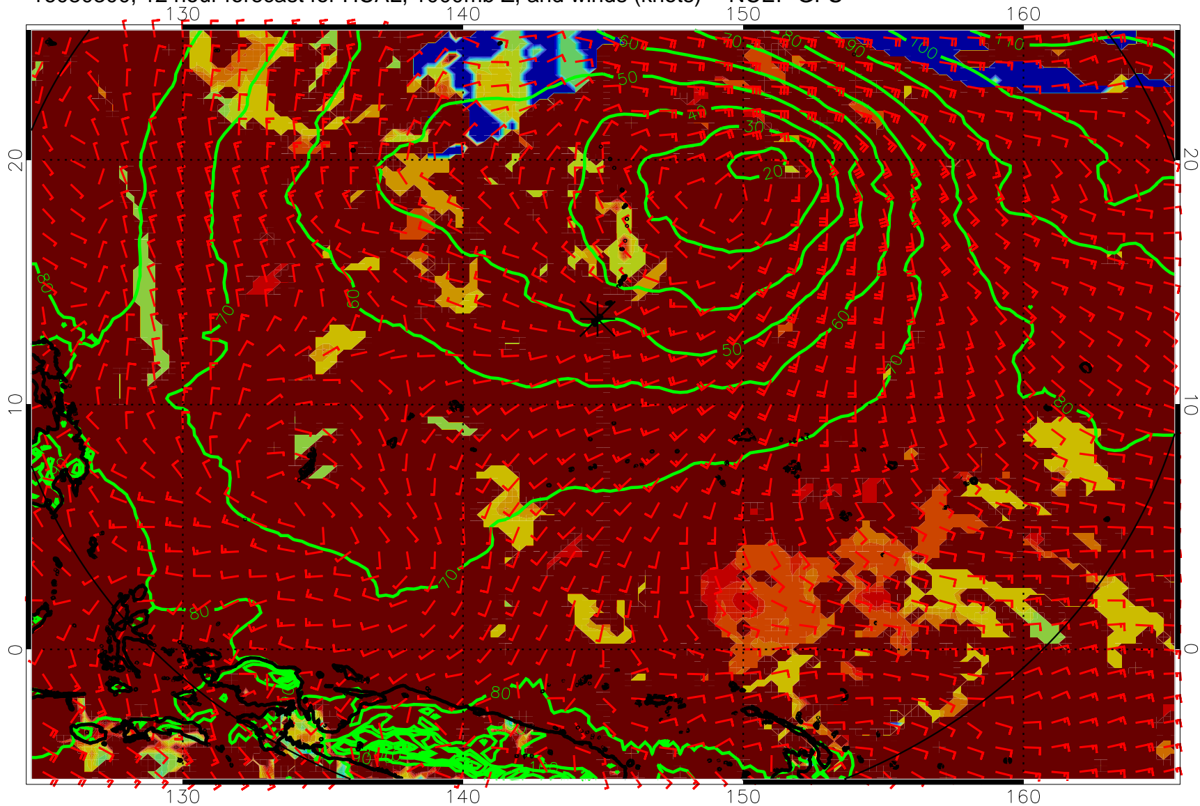
16080300, 12 hour forecast for HCAL, 1000mb Z, and winds (knots) -- NCEP GFS
