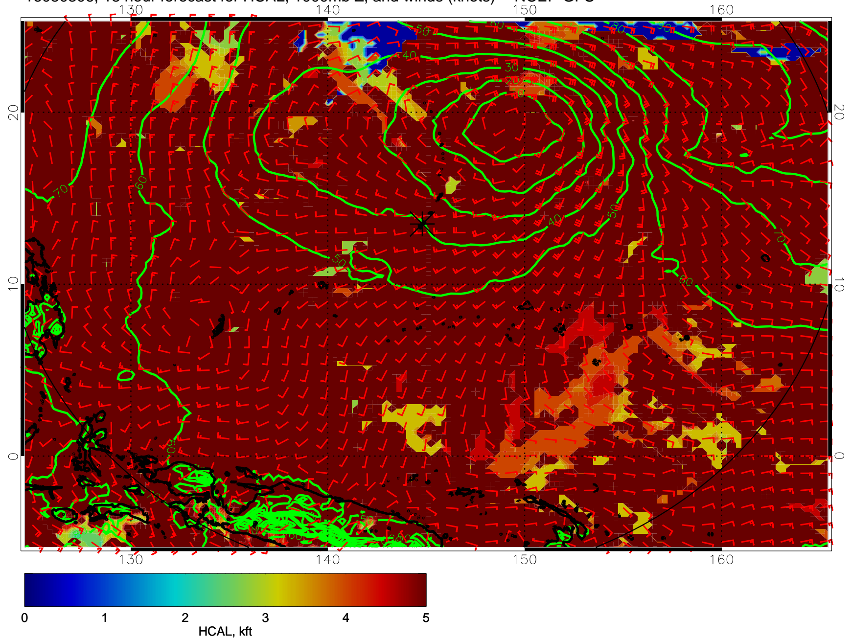
16080306, 18 hour forecast for HCAL, 1000mb Z, and winds (knots) -- NCEP GFS
