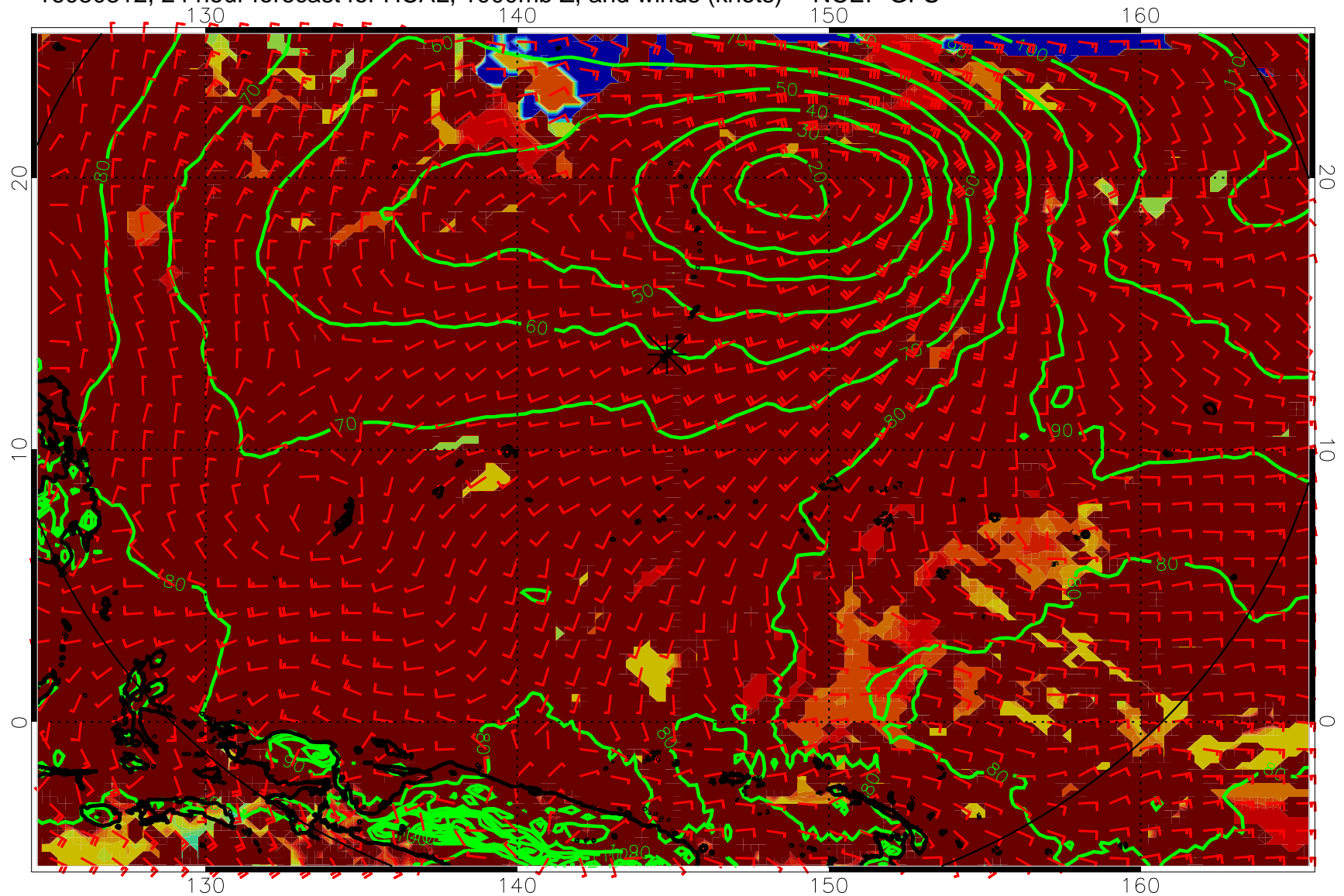
16080312, 24 hour forecast for HCAL, 1000mb Z, and winds (knots) -- NCEP GFS
