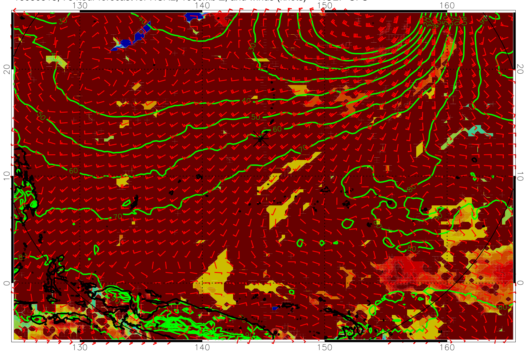
16080518, 78 hour forecast for HCAL, 1000mb Z, and winds (knots) -- NCEP GFS
