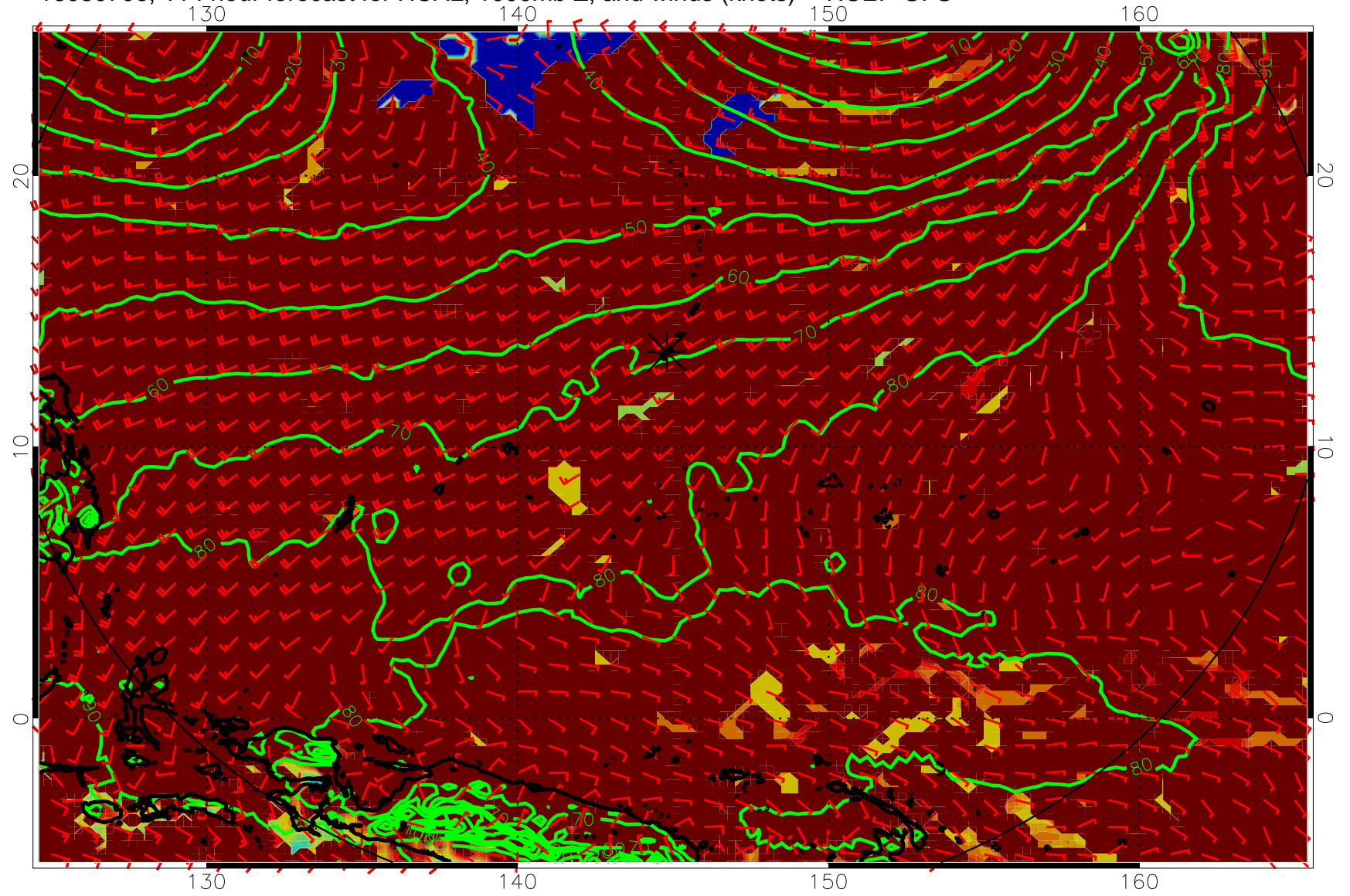
16080706, 114 hour forecast for HCAL, 1000mb Z, and winds (knots) -- NCEP GFS
