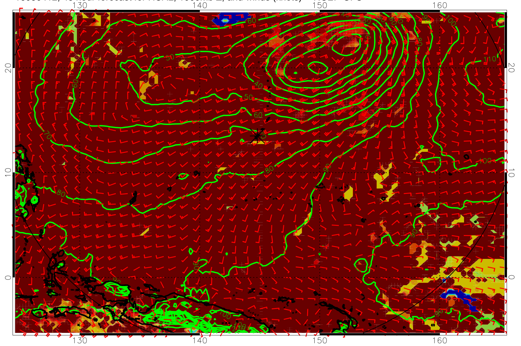
16080412, 48 hour forecast for HCAL, 1000mb Z, and winds (knots) -- NCEP GFS
