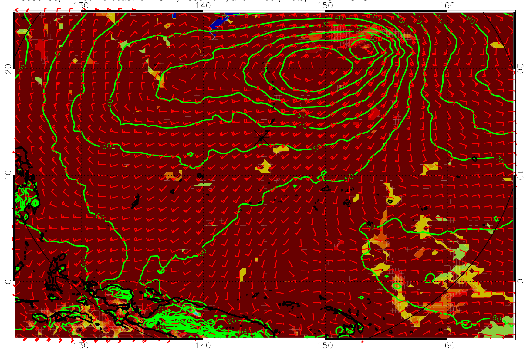
16080406, 42 hour forecast for HCAL, 1000mb Z, and winds (knots) -- NCEP GFS
