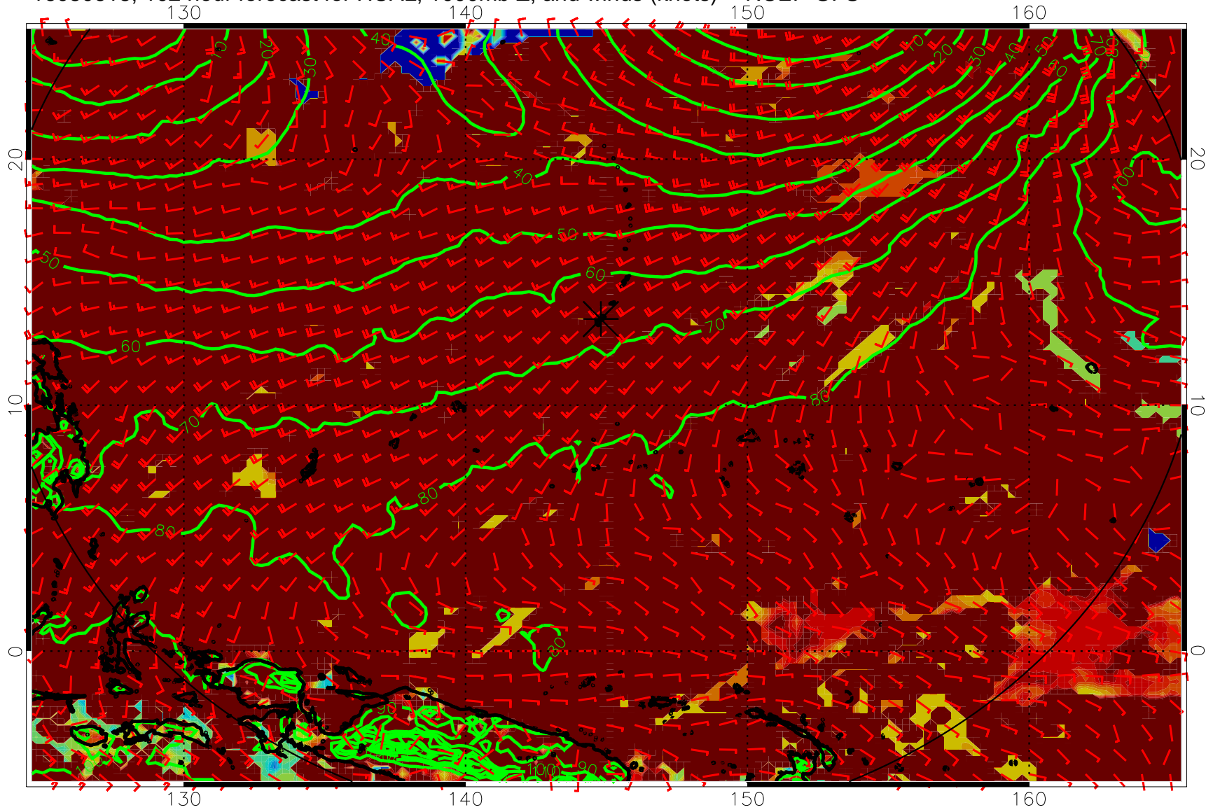
16080618, 102 hour forecast for HCAL, 1000mb Z, and winds (knots) -- NCEP GFS
