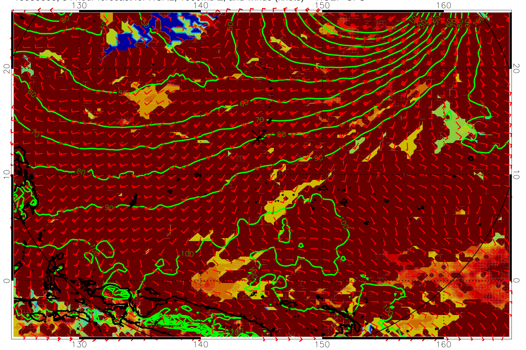
16080600, 84 hour forecast for HCAL, 1000mb Z, and winds (knots) -- NCEP GFS
