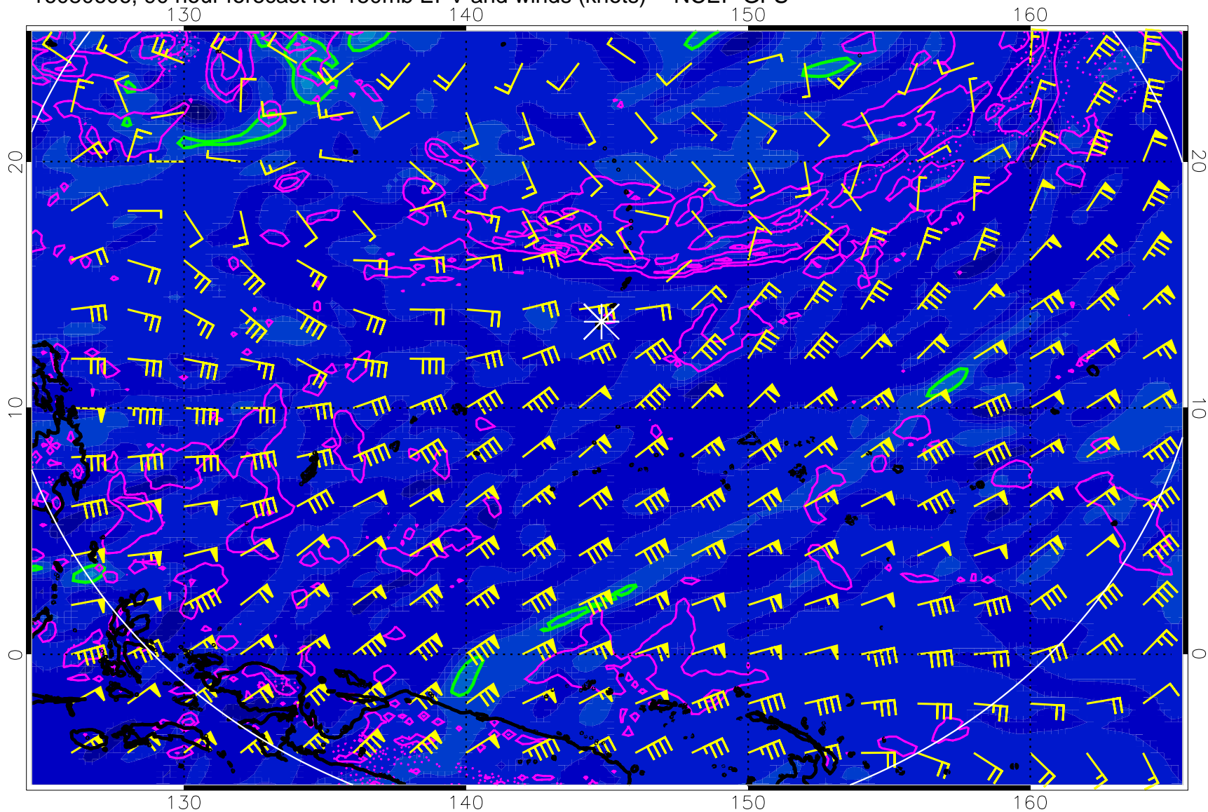
16080606, 90 hour forecast for 150mb EPV and winds (knots) -- NCEP GFS
