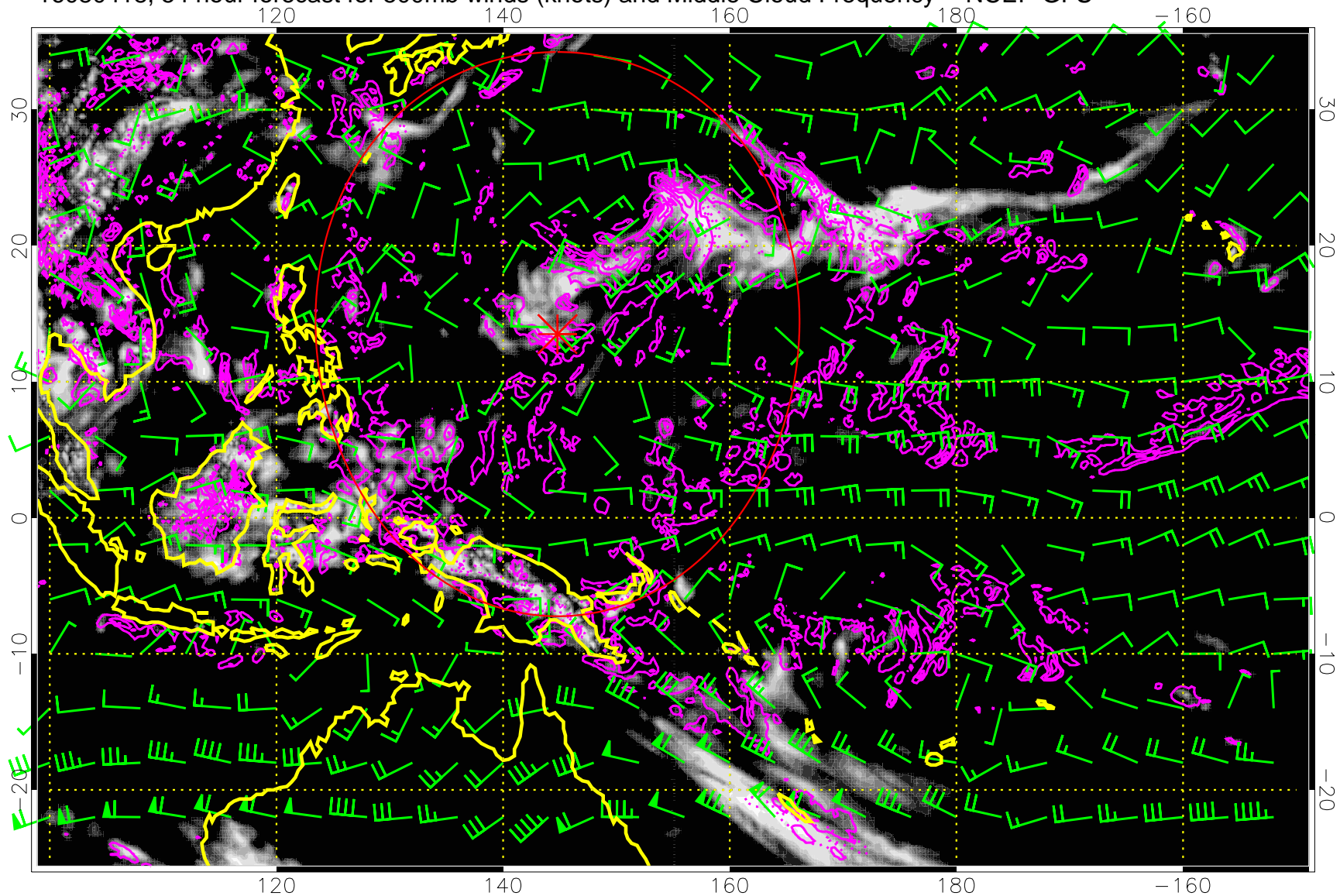
16080418, 54 hour forecast for 500mb winds (knots) and Middle Cloud Frequency -- NCEP GFS
