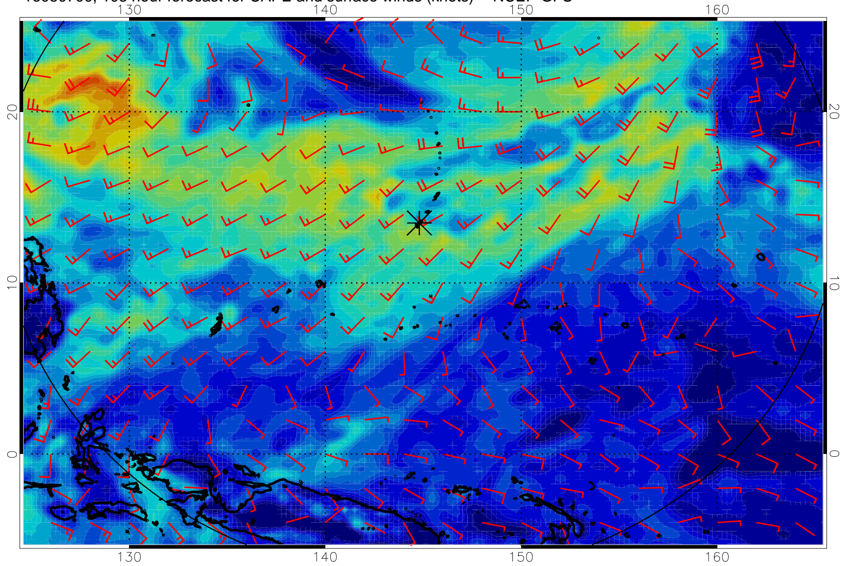
16080700, 108 hour forecast for CAPE and surface winds (knots) -- NCEP GFS
