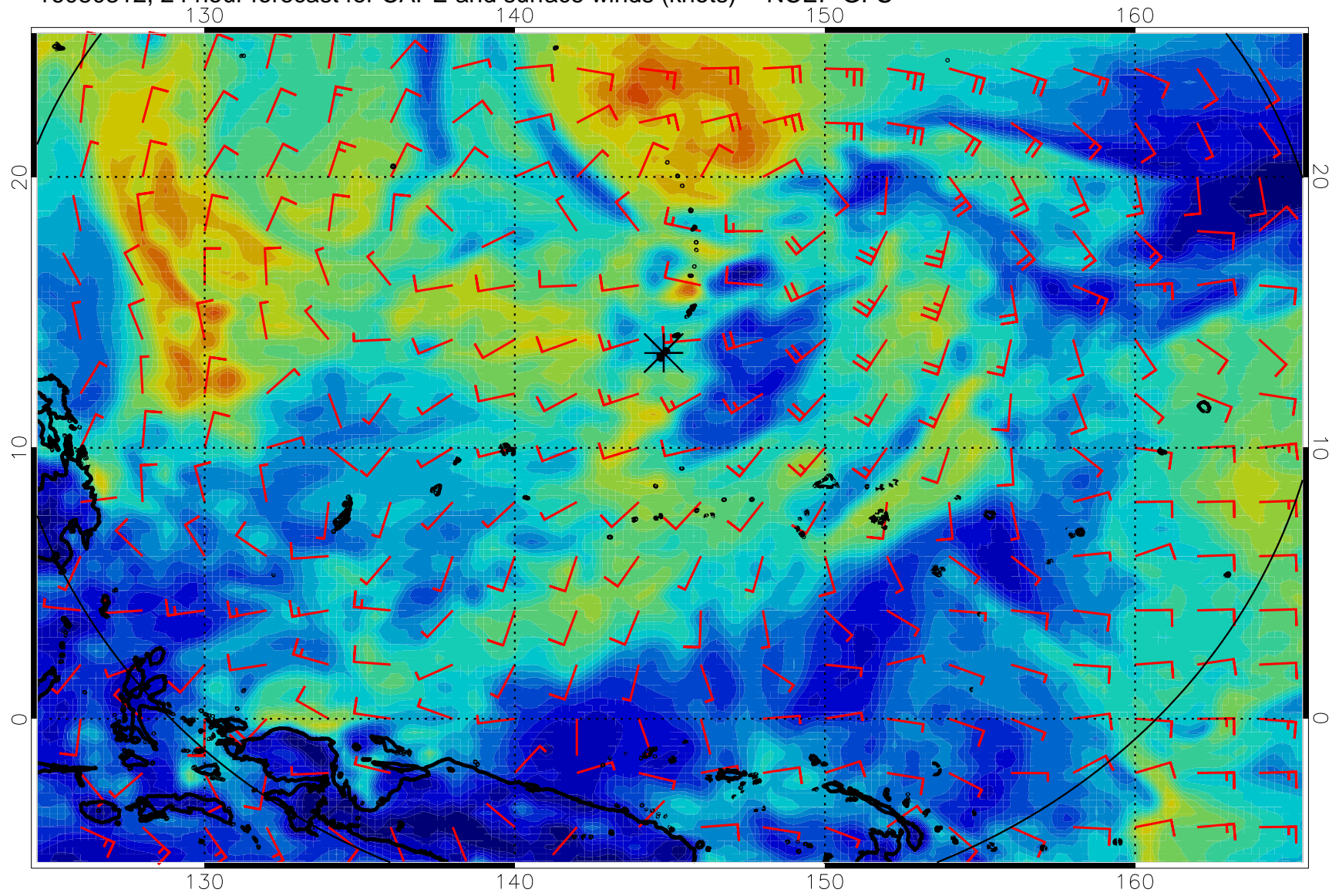
16080312, 24 hour forecast for CAPE and surface winds (knots) -- NCEP GFS
