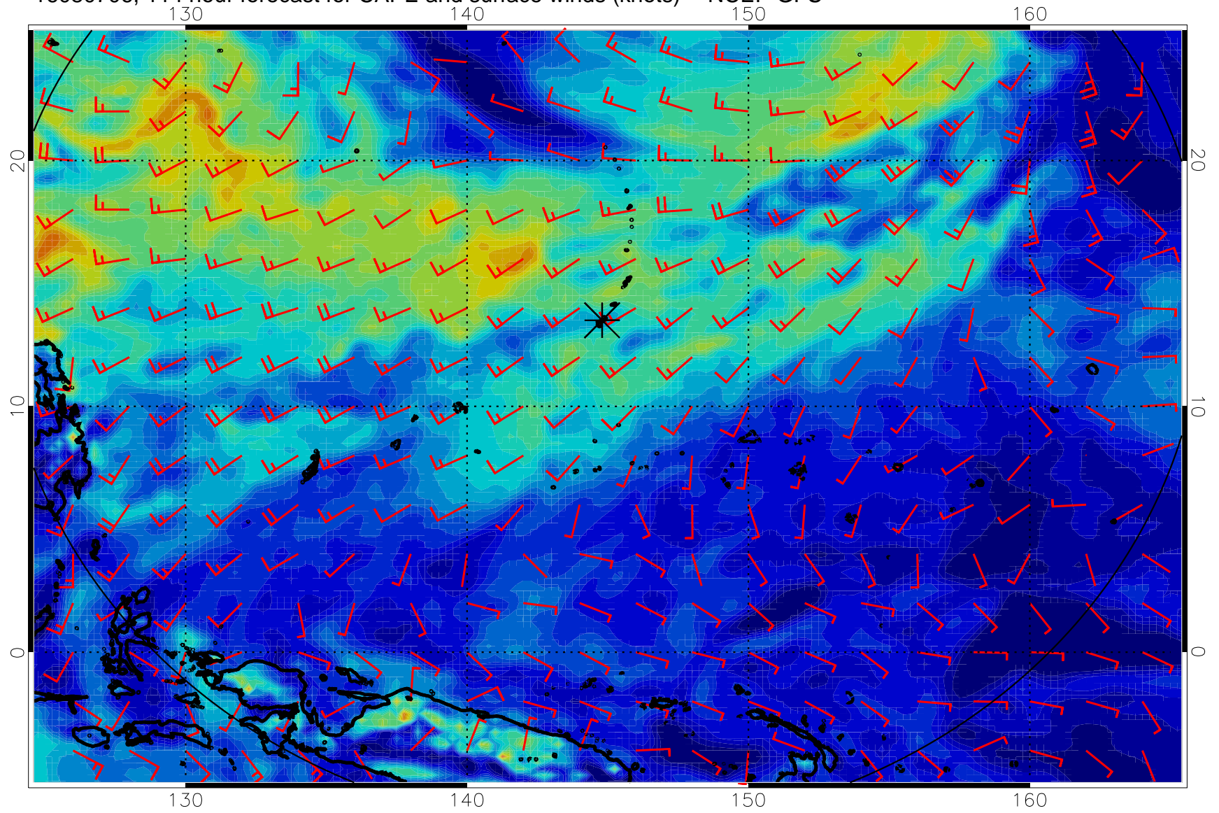
16080706, 114 hour forecast for CAPE and surface winds (knots) -- NCEP GFS
