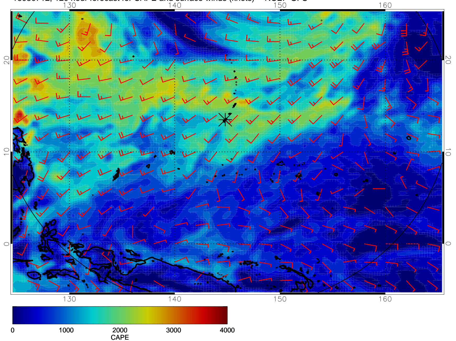
16080712, 120 hour forecast for CAPE and surface winds (knots) -- NCEP GFS
