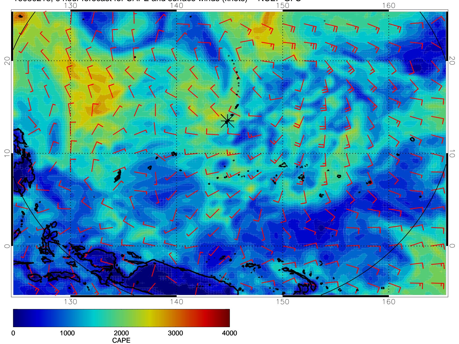
16080218, 6 hour forecast for CAPE and surface winds (knots) -- NCEP GFS
