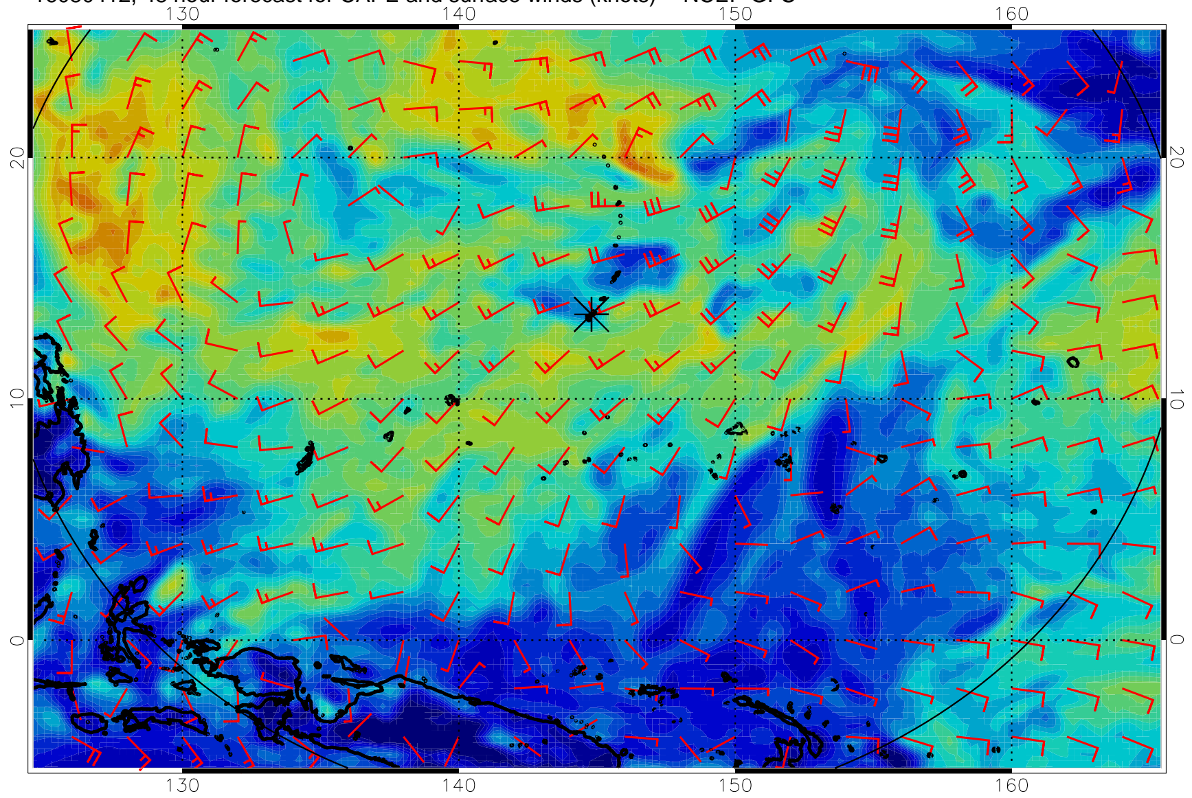
16080412, 48 hour forecast for CAPE and surface winds (knots) -- NCEP GFS
