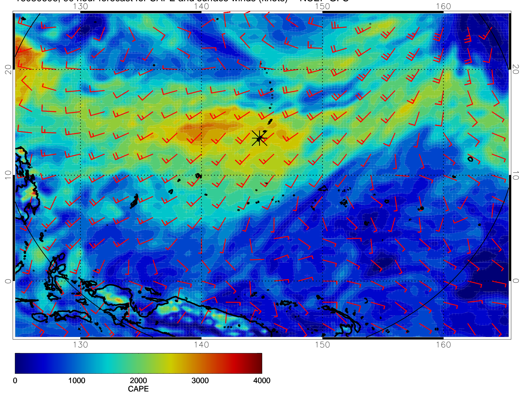
16080606, 90 hour forecast for CAPE and surface winds (knots) -- NCEP GFS
