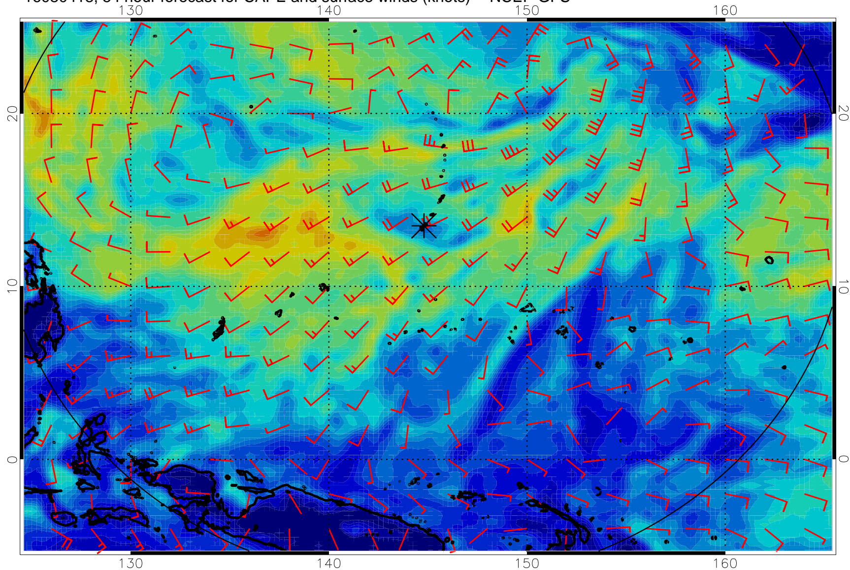
16080418, 54 hour forecast for CAPE and surface winds (knots) -- NCEP GFS
