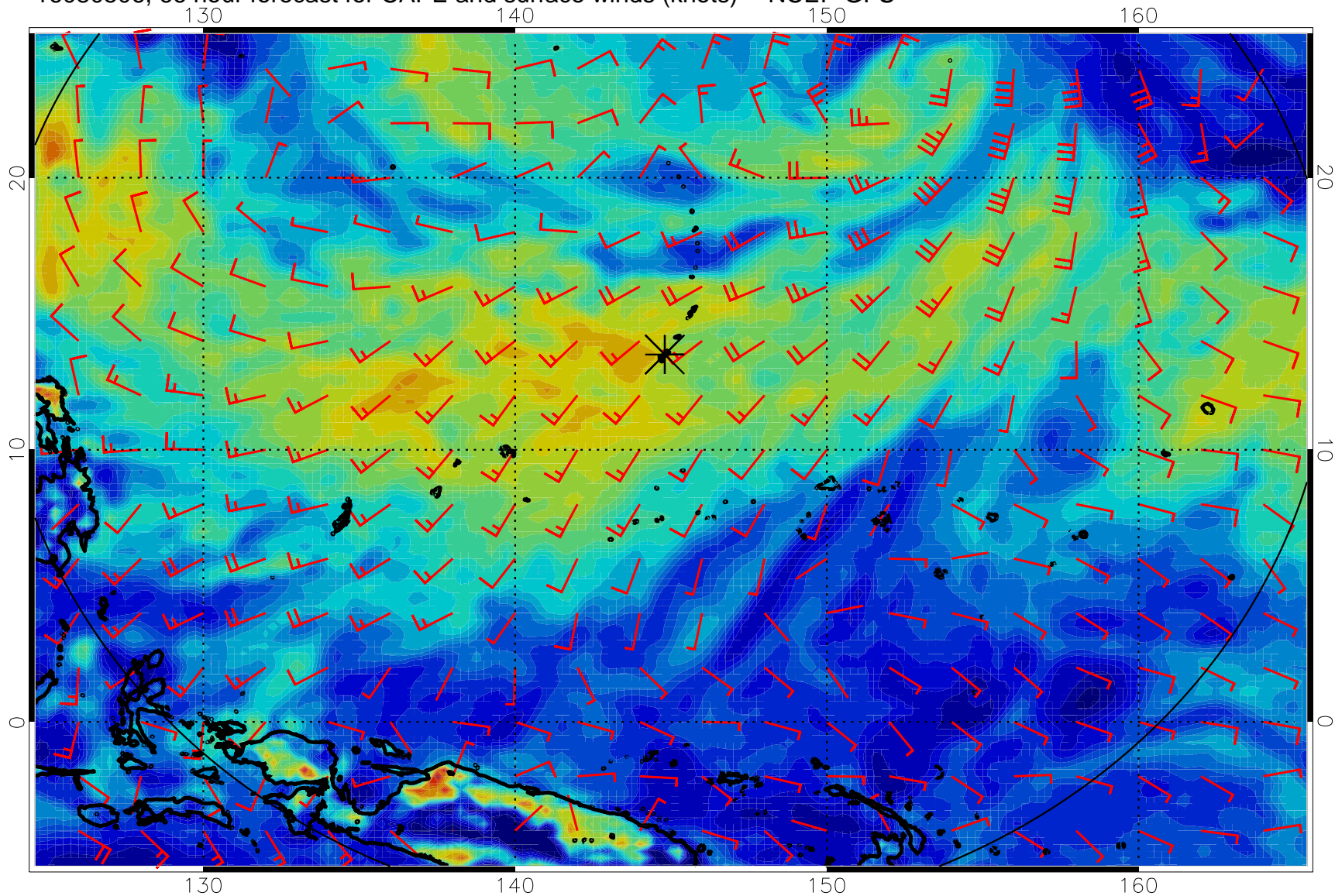
16080506, 66 hour forecast for CAPE and surface winds (knots) -- NCEP GFS
