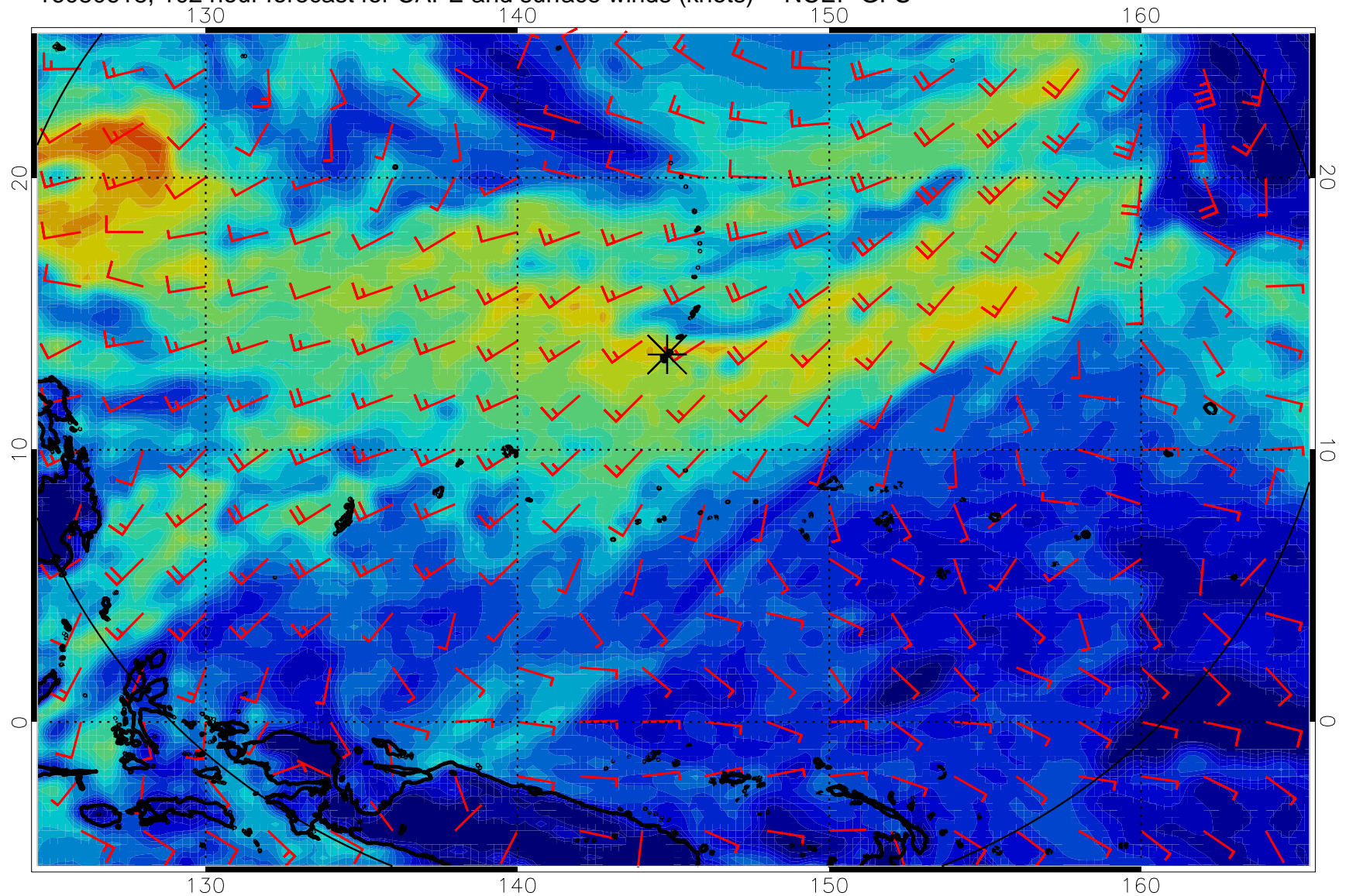
16080618, 102 hour forecast for CAPE and surface winds (knots) -- NCEP GFS
