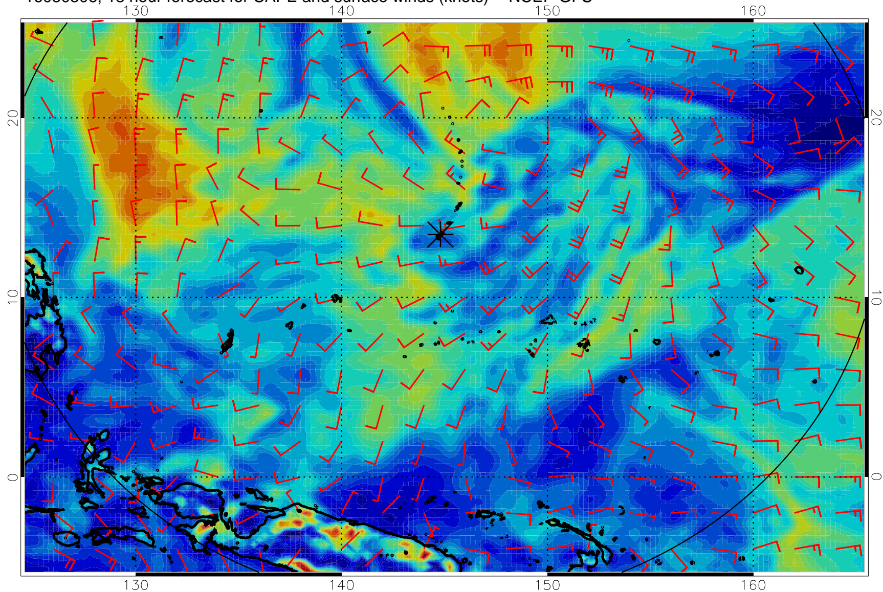
16080306, 18 hour forecast for CAPE and surface winds (knots) -- NCEP GFS
