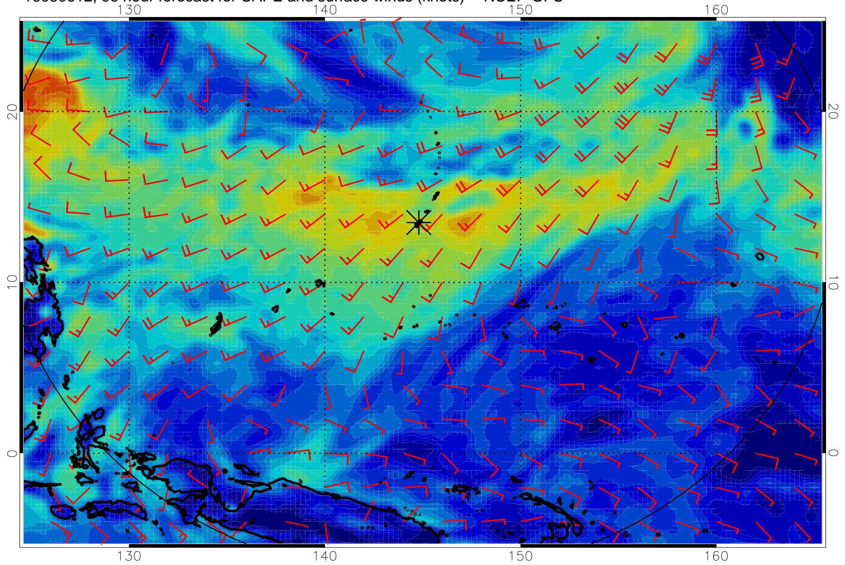
16080612, 96 hour forecast for CAPE and surface winds (knots) -- NCEP GFS
