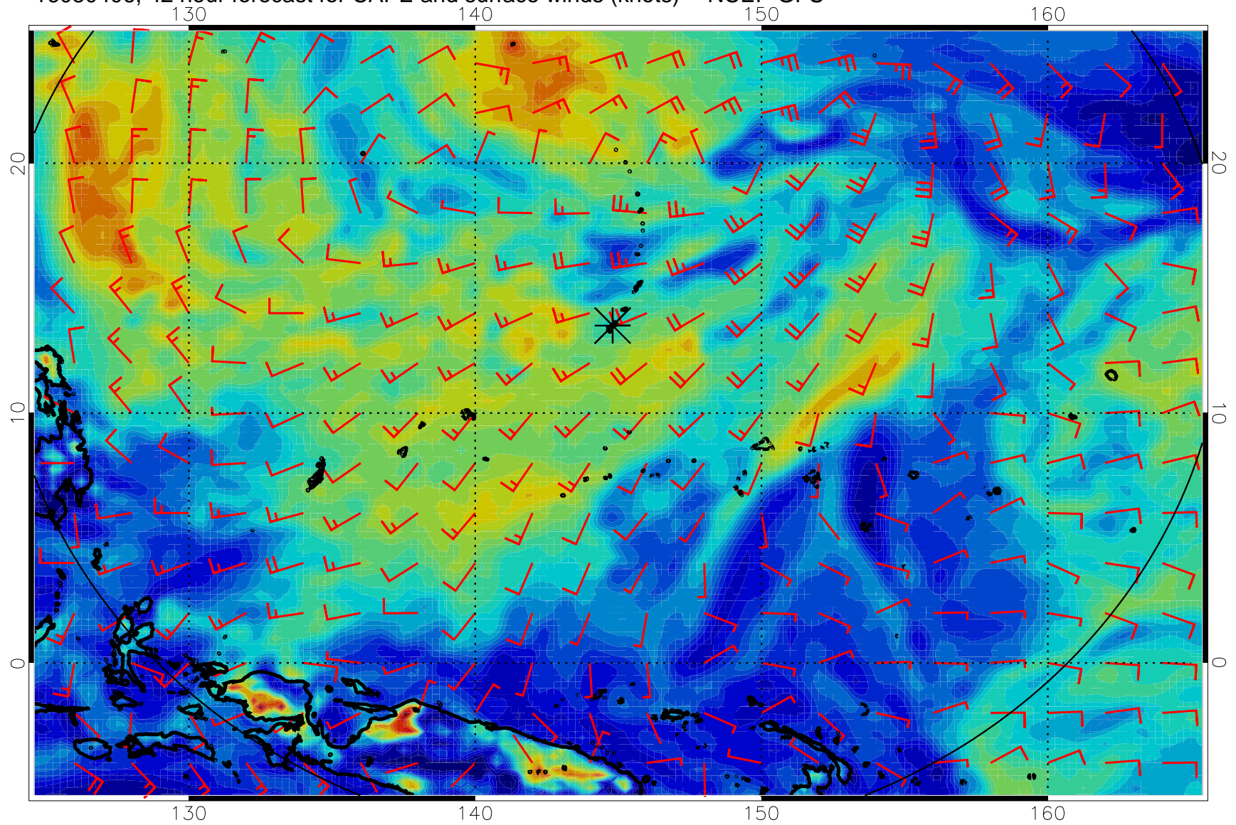
16080406, 42 hour forecast for CAPE and surface winds (knots) -- NCEP GFS
