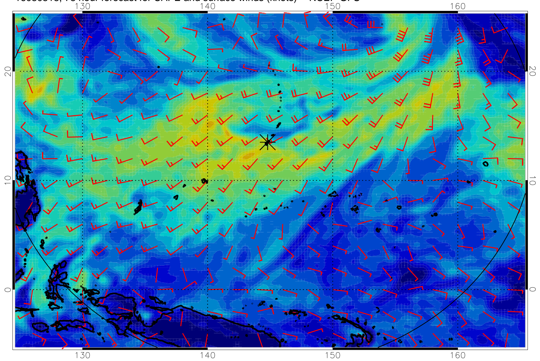
16080518, 78 hour forecast for CAPE and surface winds (knots) -- NCEP GFS
