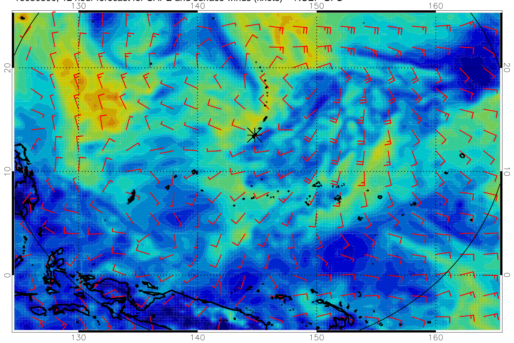
16080300, 12 hour forecast for CAPE and surface winds (knots) -- NCEP GFS
