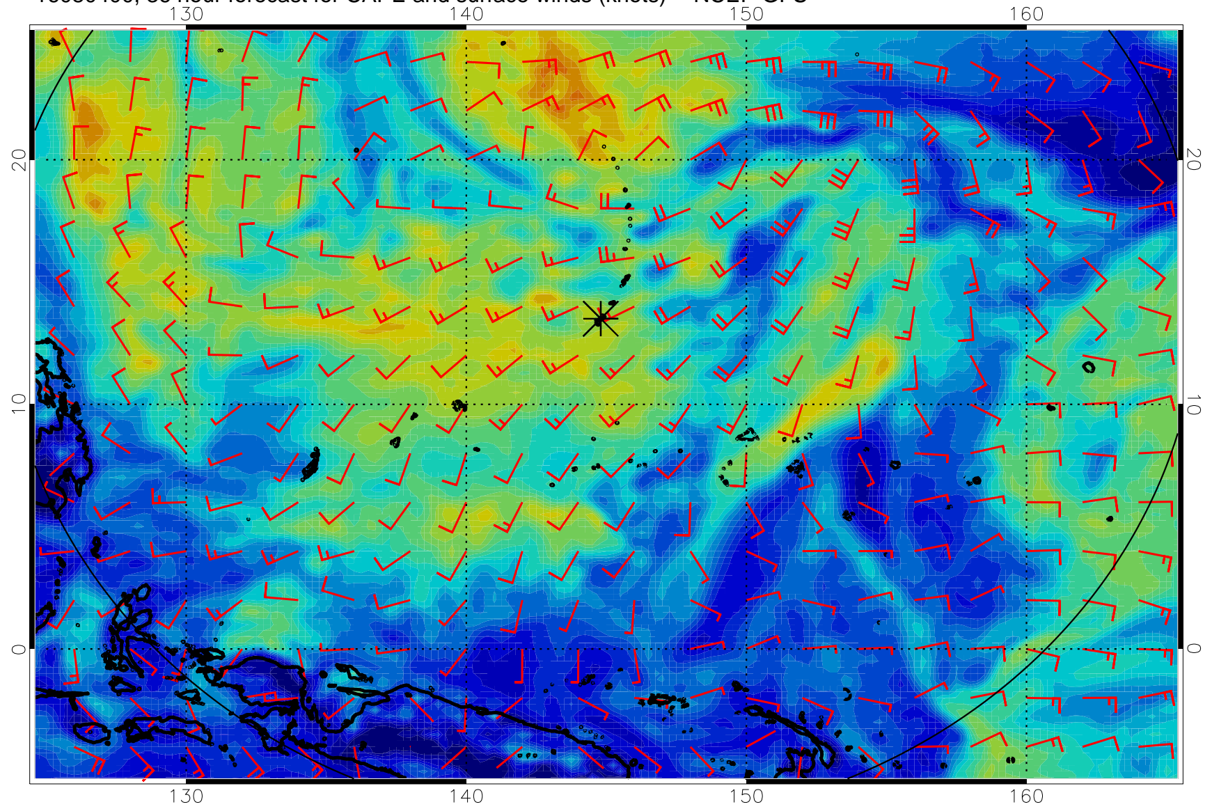
16080400, 36 hour forecast for CAPE and surface winds (knots) -- NCEP GFS
