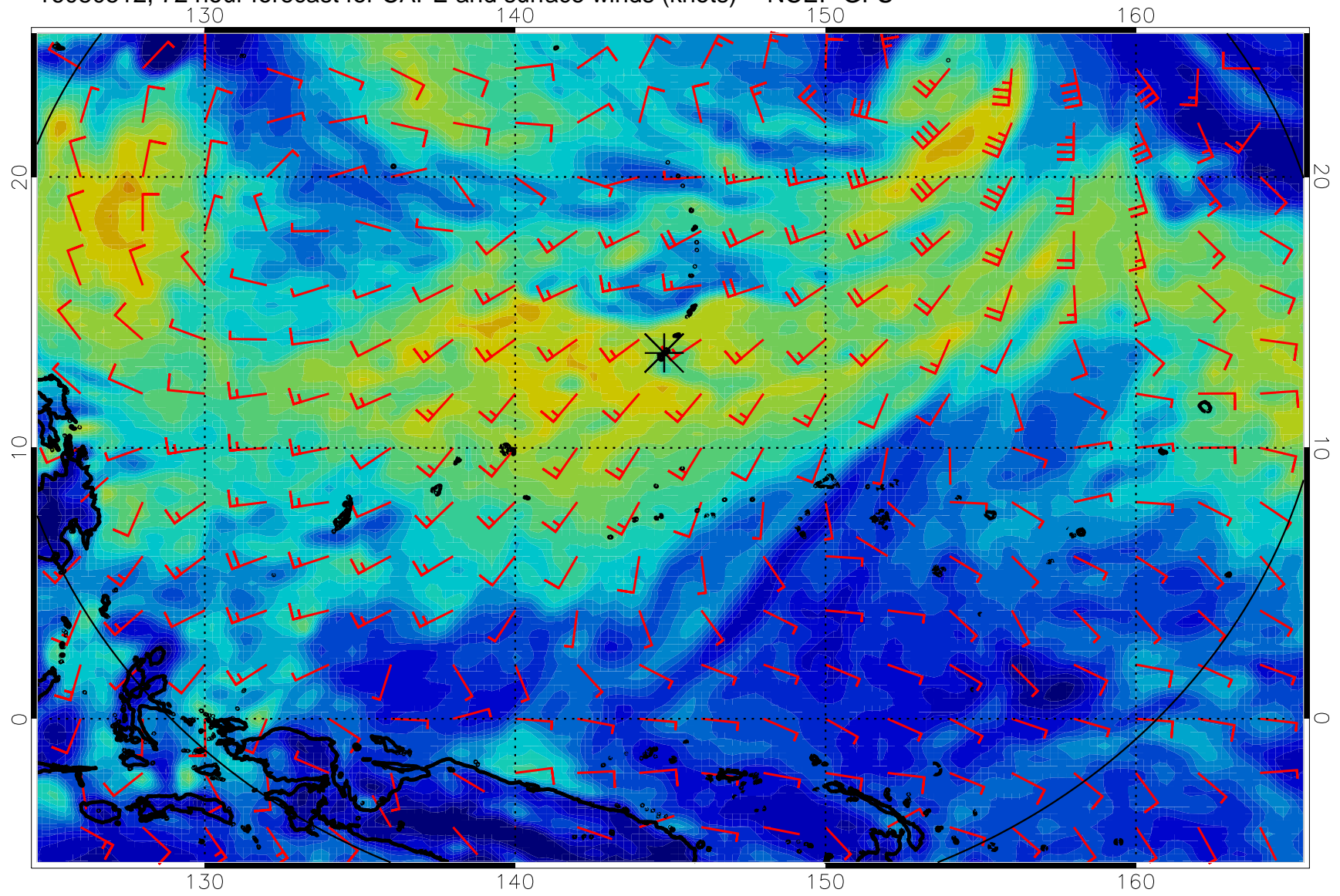
16080512, 72 hour forecast for CAPE and surface winds (knots) -- NCEP GFS
