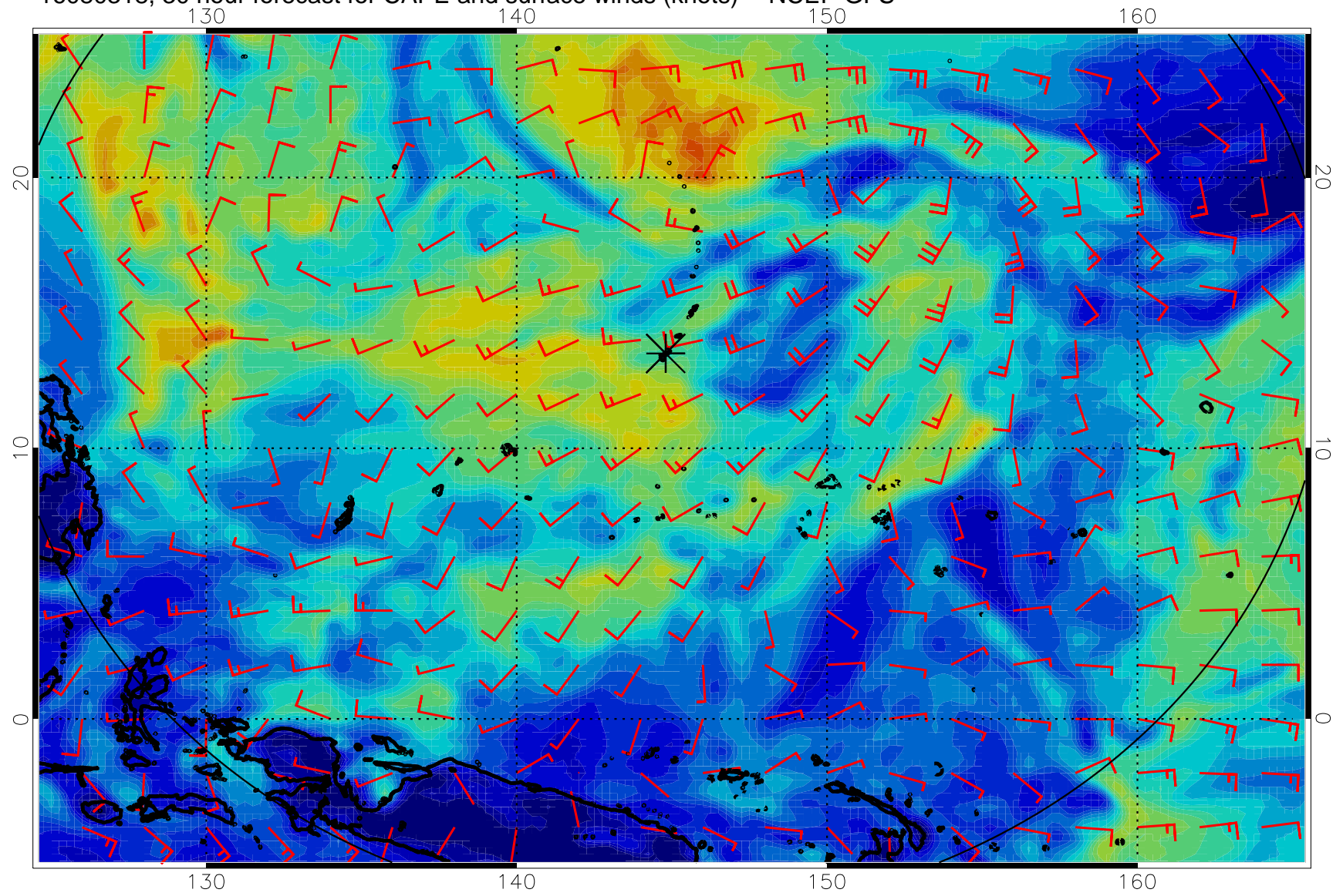
16080318, 30 hour forecast for CAPE and surface winds (knots) -- NCEP GFS
