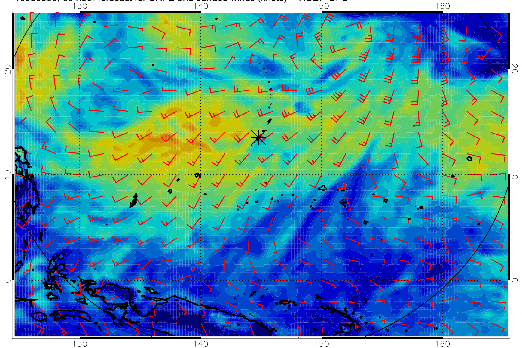
16080500, 60 hour forecast for CAPE and surface winds (knots) -- NCEP GFS
