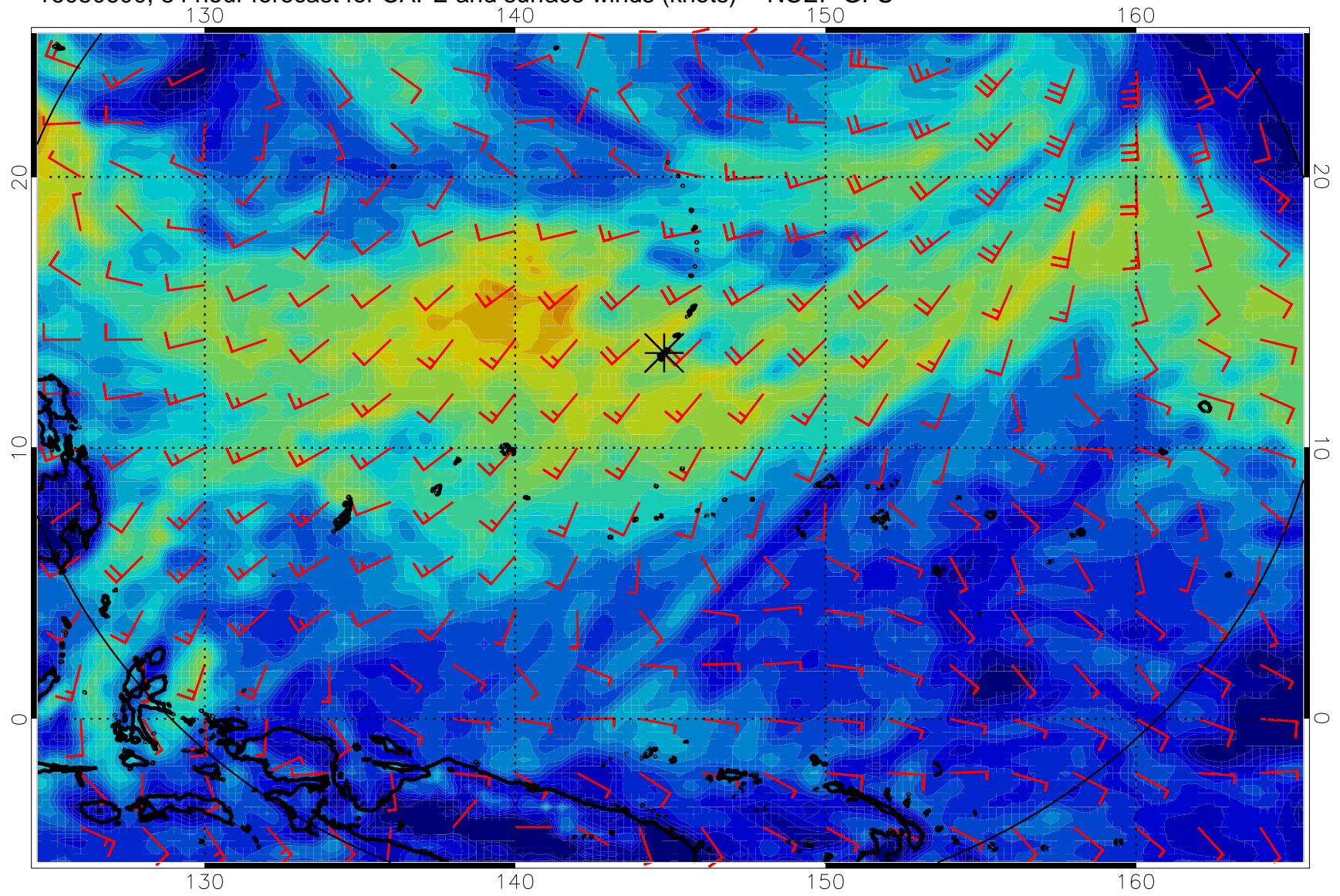
16080600, 84 hour forecast for CAPE and surface winds (knots) -- NCEP GFS
