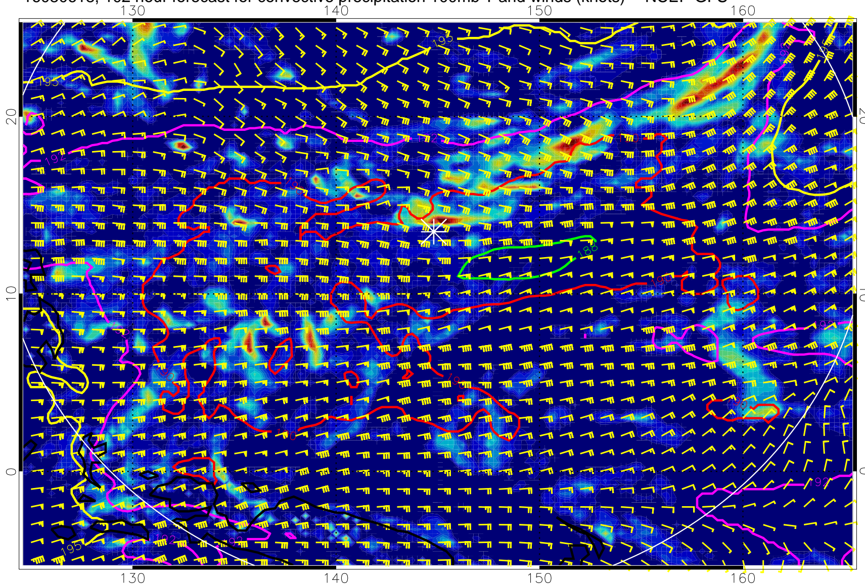
16080618, 102 hour forecast for convective precipitation 100mb T and winds (knots) -- NCEP GFS
