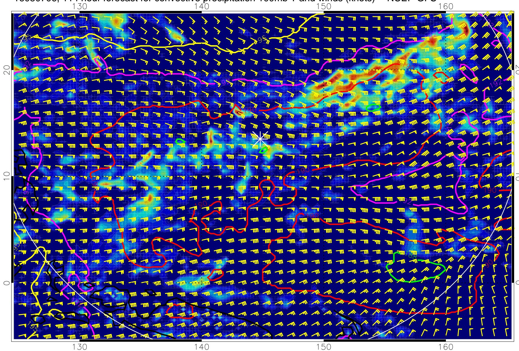
16080706, 114 hour forecast for convective precipitation 100mb T and winds (knots) -- NCEP GFS
