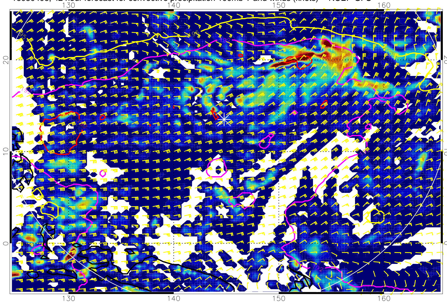
16080406, 42 hour forecast for convective precipitation 100mb T and winds (knots) -- NCEP GFS
