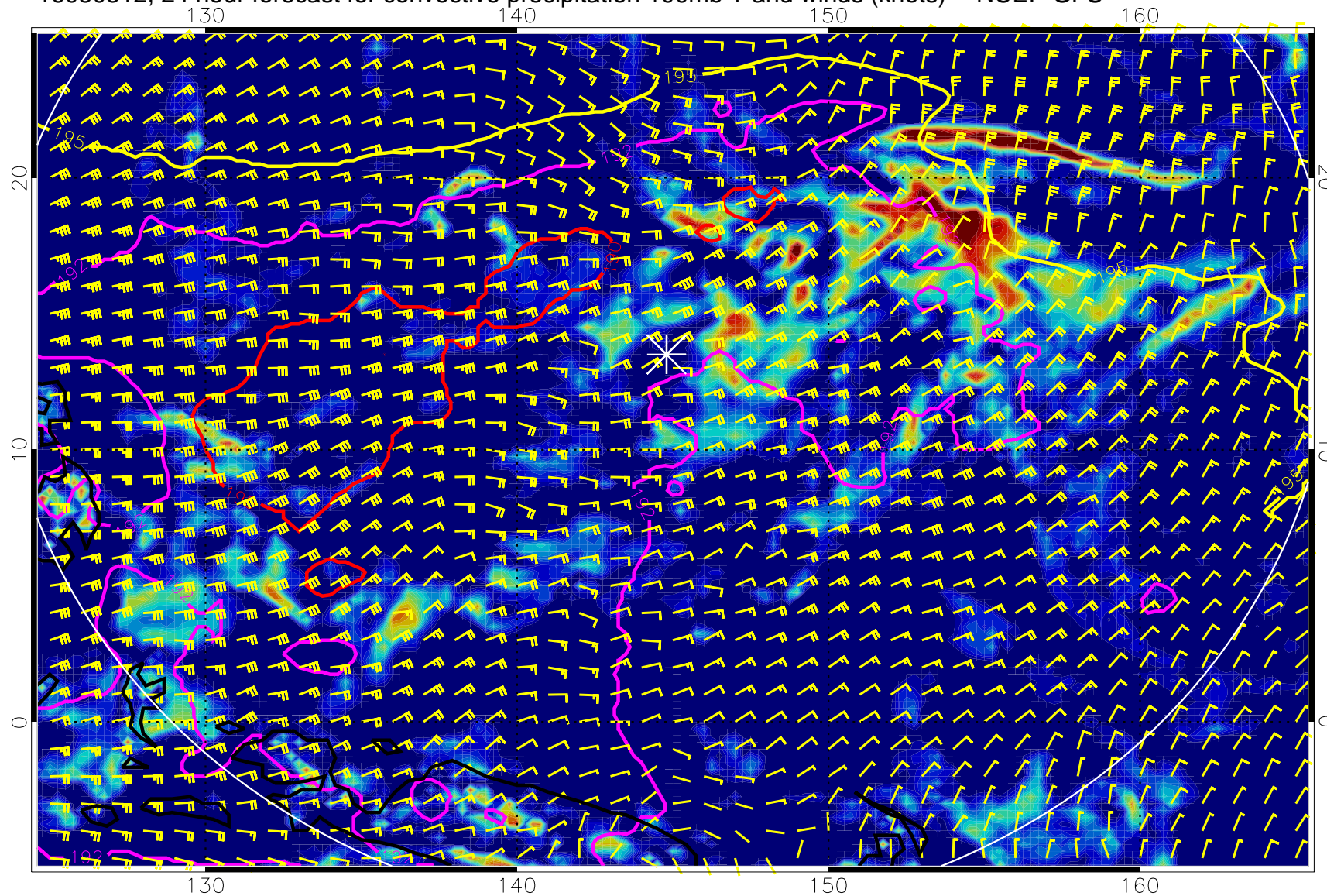
16080312, 24 hour forecast for convective precipitation 100mb T and winds (knots) -- NCEP GFS
