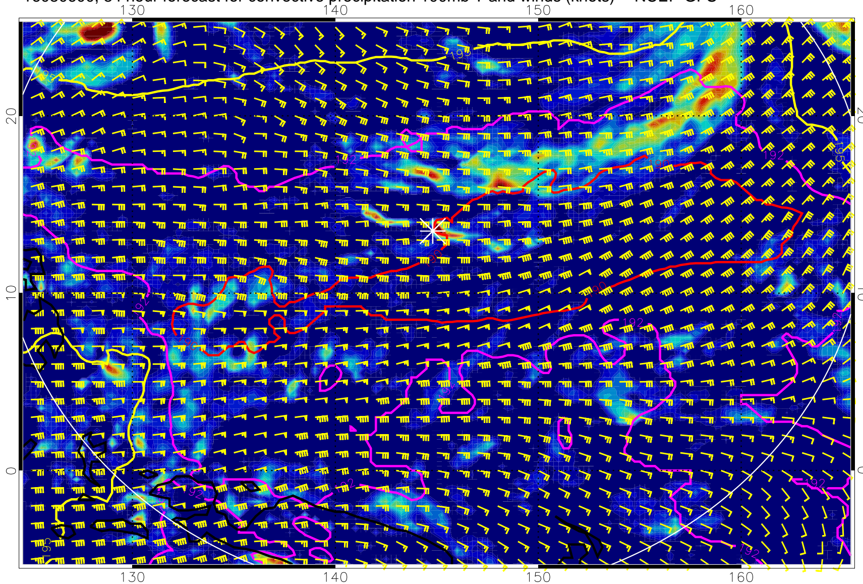
16080600, 84 hour forecast for convective precipitation 100mb T and winds (knots) -- NCEP GFS
