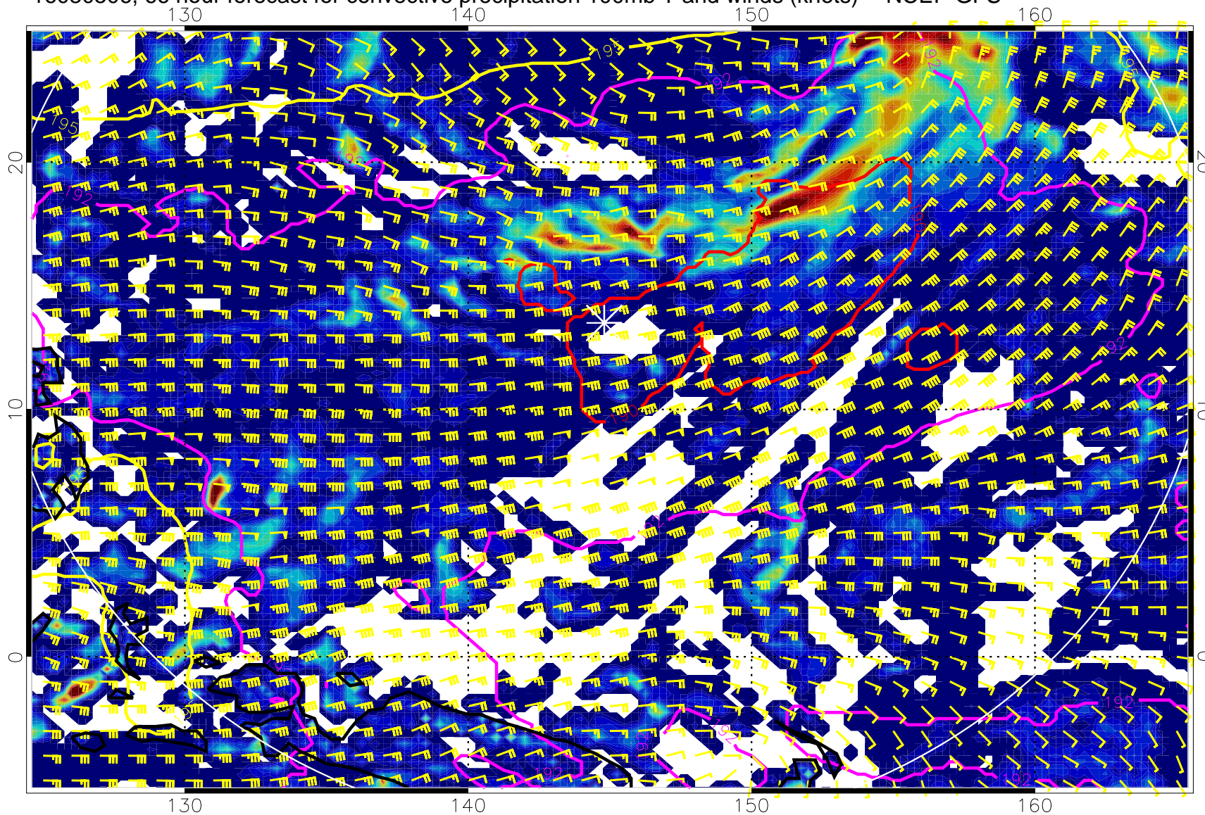
16080506, 66 hour forecast for convective precipitation 100mb T and winds (knots) -- NCEP GFS
