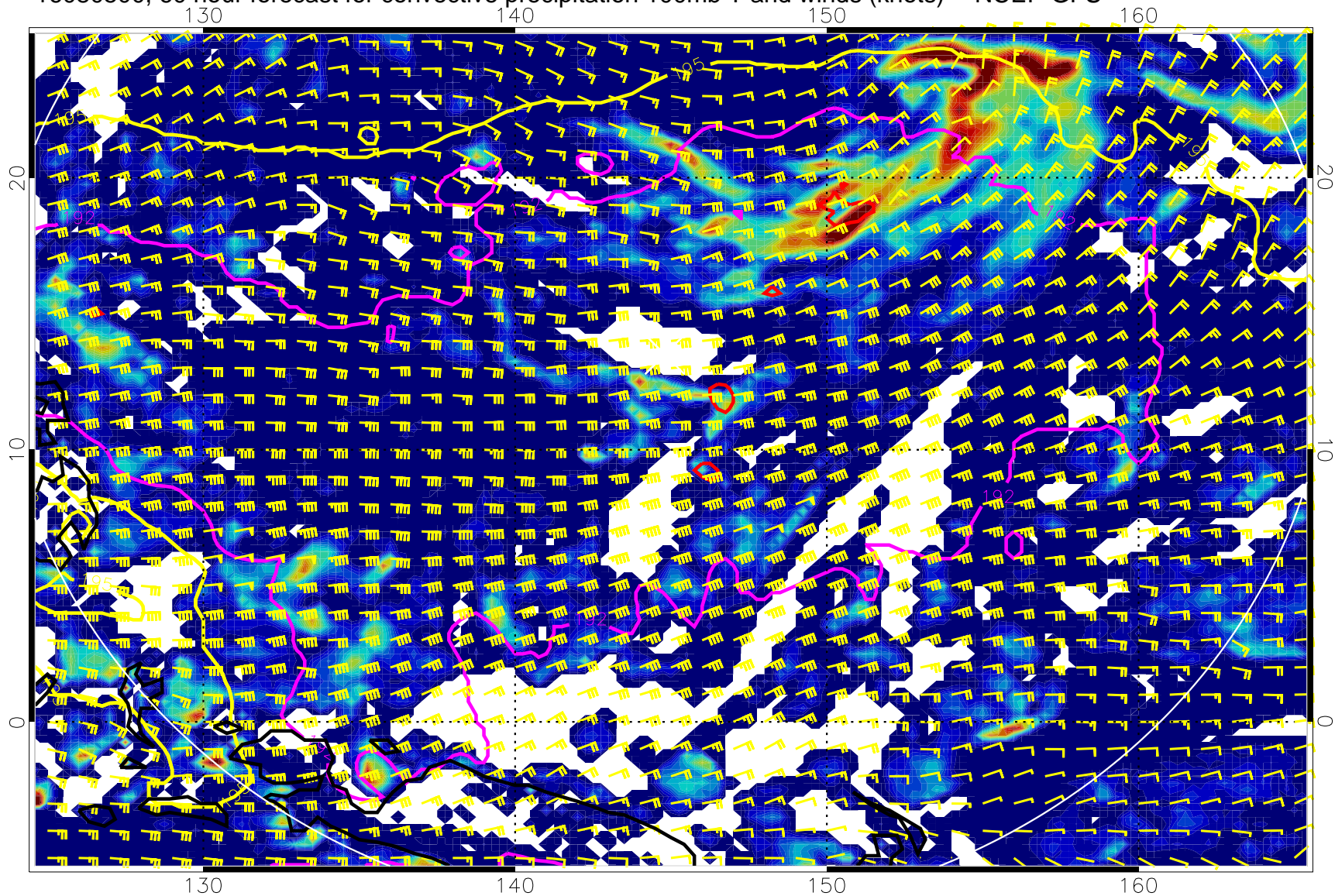
16080500, 60 hour forecast for convective precipitation 100mb T and winds (knots) -- NCEP GFS
