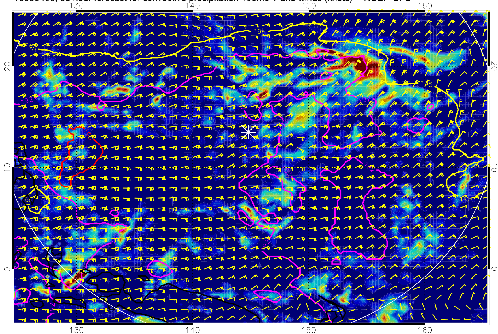
16080400, 36 hour forecast for convective precipitation 100mb T and winds (knots) -- NCEP GFS
