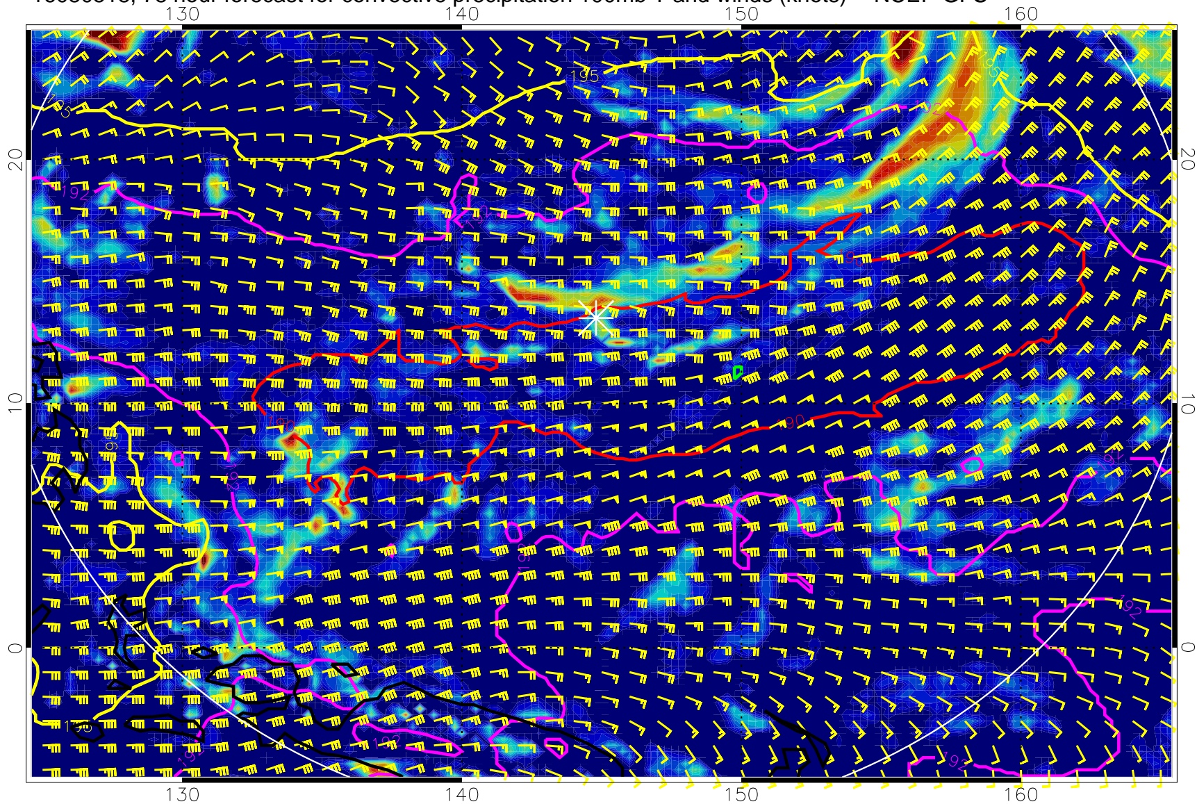
16080518, 78 hour forecast for convective precipitation 100mb T and winds (knots) -- NCEP GFS
