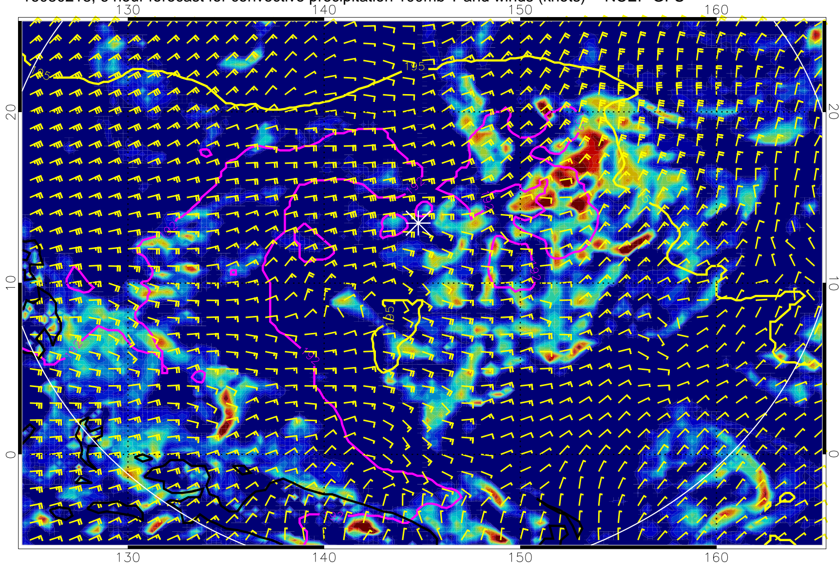
16080218, 6 hour forecast for convective precipitation 100mb T and winds (knots) -- NCEP GFS
