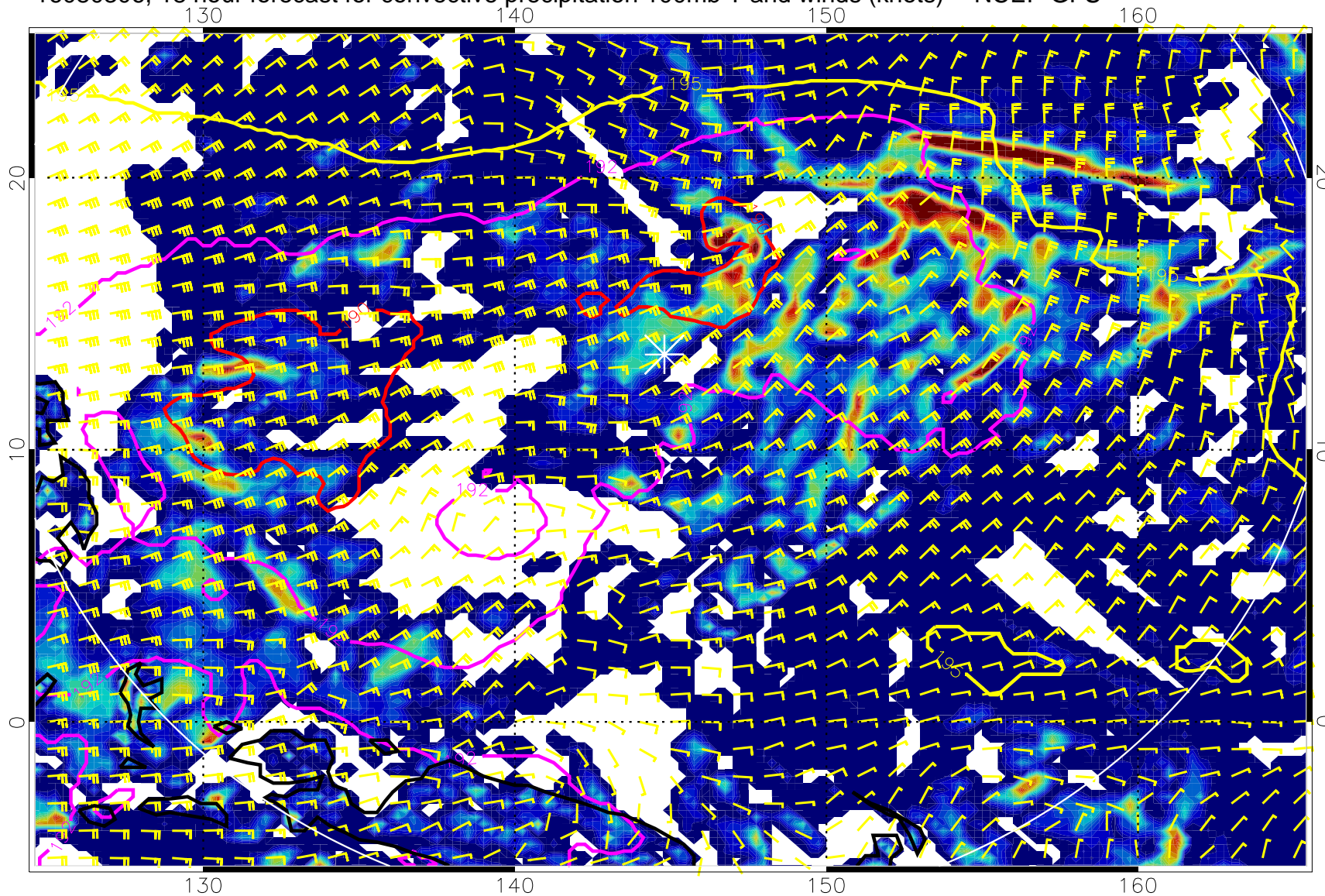
16080306, 18 hour forecast for convective precipitation 100mb T and winds (knots) -- NCEP GFS
