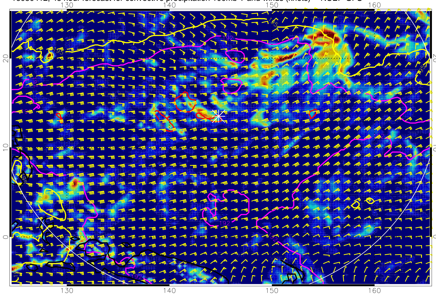
16080412, 48 hour forecast for convective precipitation 100mb T and winds (knots) -- NCEP GFS
