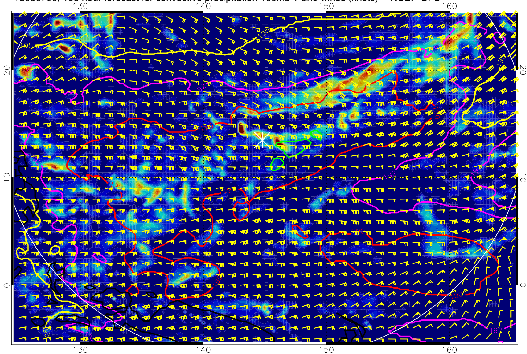
16080700, 108 hour forecast for convective precipitation 100mb T and winds (knots) -- NCEP GFS
