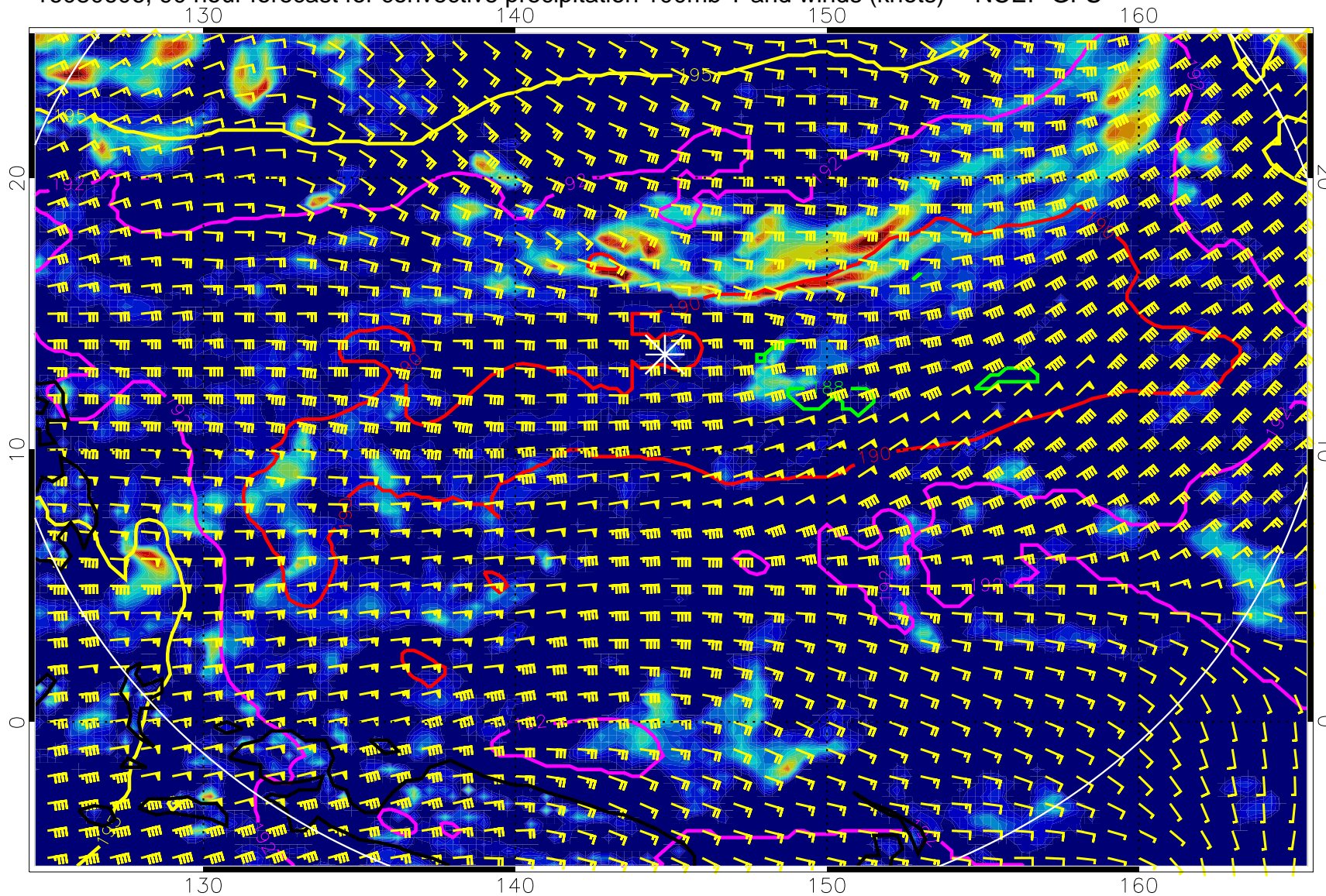
16080606, 90 hour forecast for convective precipitation 100mb T and winds (knots) -- NCEP GFS
