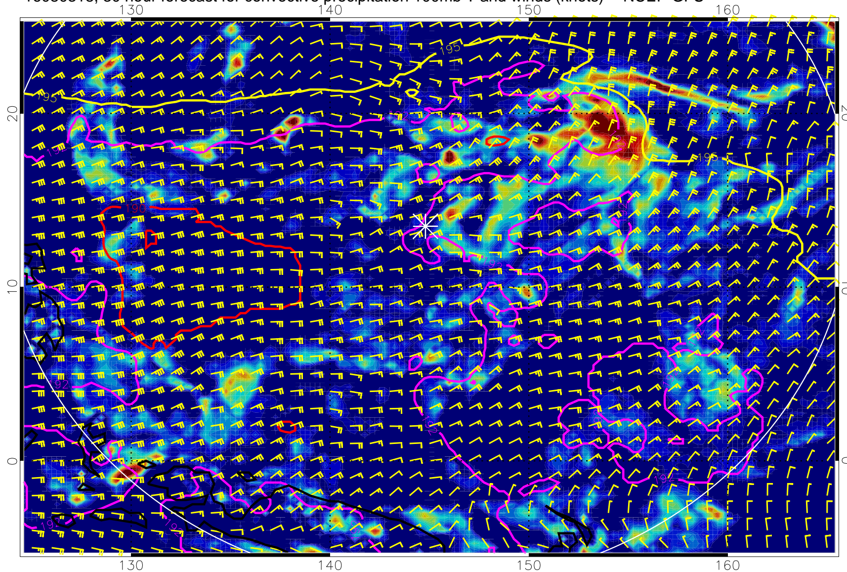
16080318, 30 hour forecast for convective precipitation 100mb T and winds (knots) -- NCEP GFS
