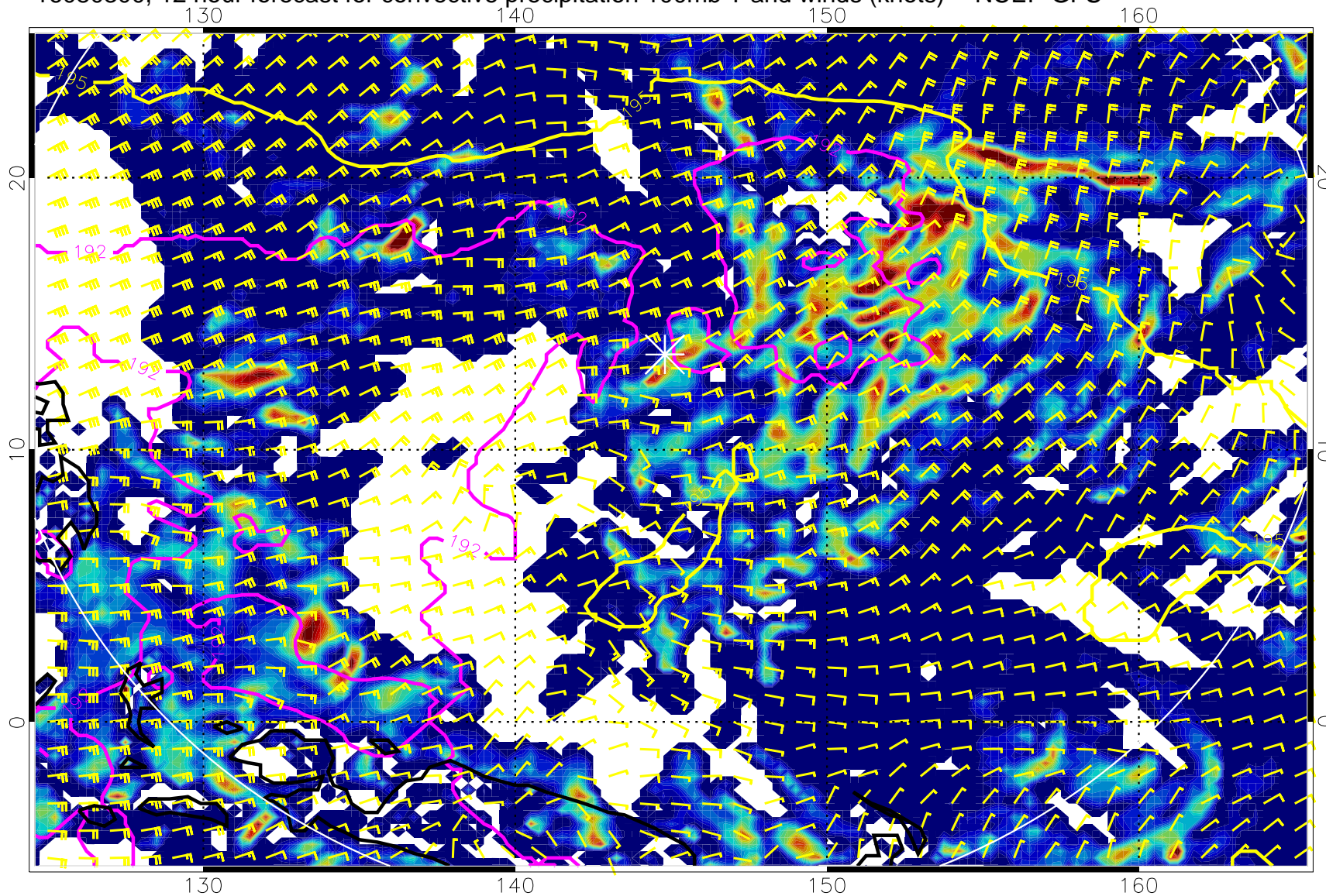
16080300, 12 hour forecast for convective precipitation 100mb T and winds (knots) -- NCEP GFS
