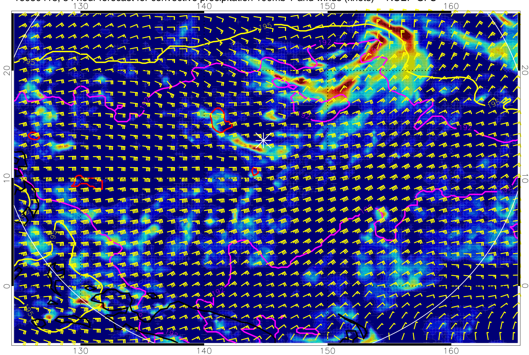
16080418, 54 hour forecast for convective precipitation 100mb T and winds (knots) -- NCEP GFS
