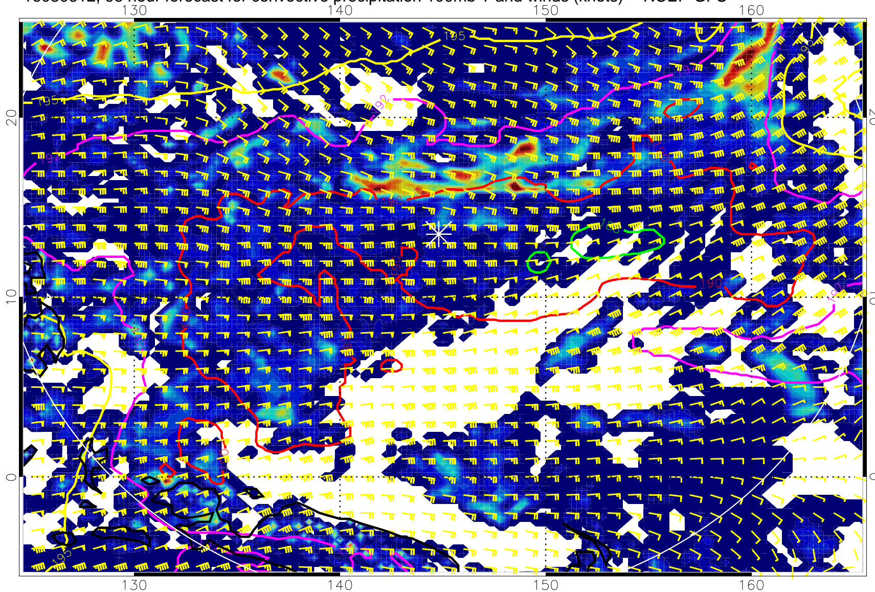
16080612, 96 hour forecast for convective precipitation 100mb T and winds (knots) -- NCEP GFS
