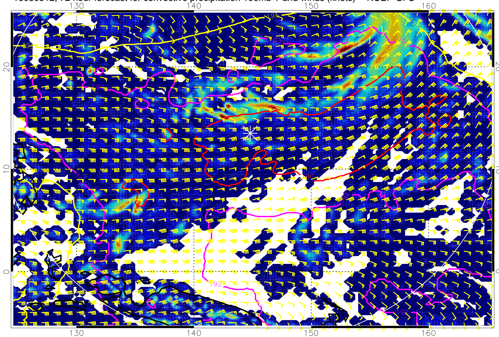
16080512, 72 hour forecast for convective precipitation 100mb T and winds (knots) -- NCEP GFS
