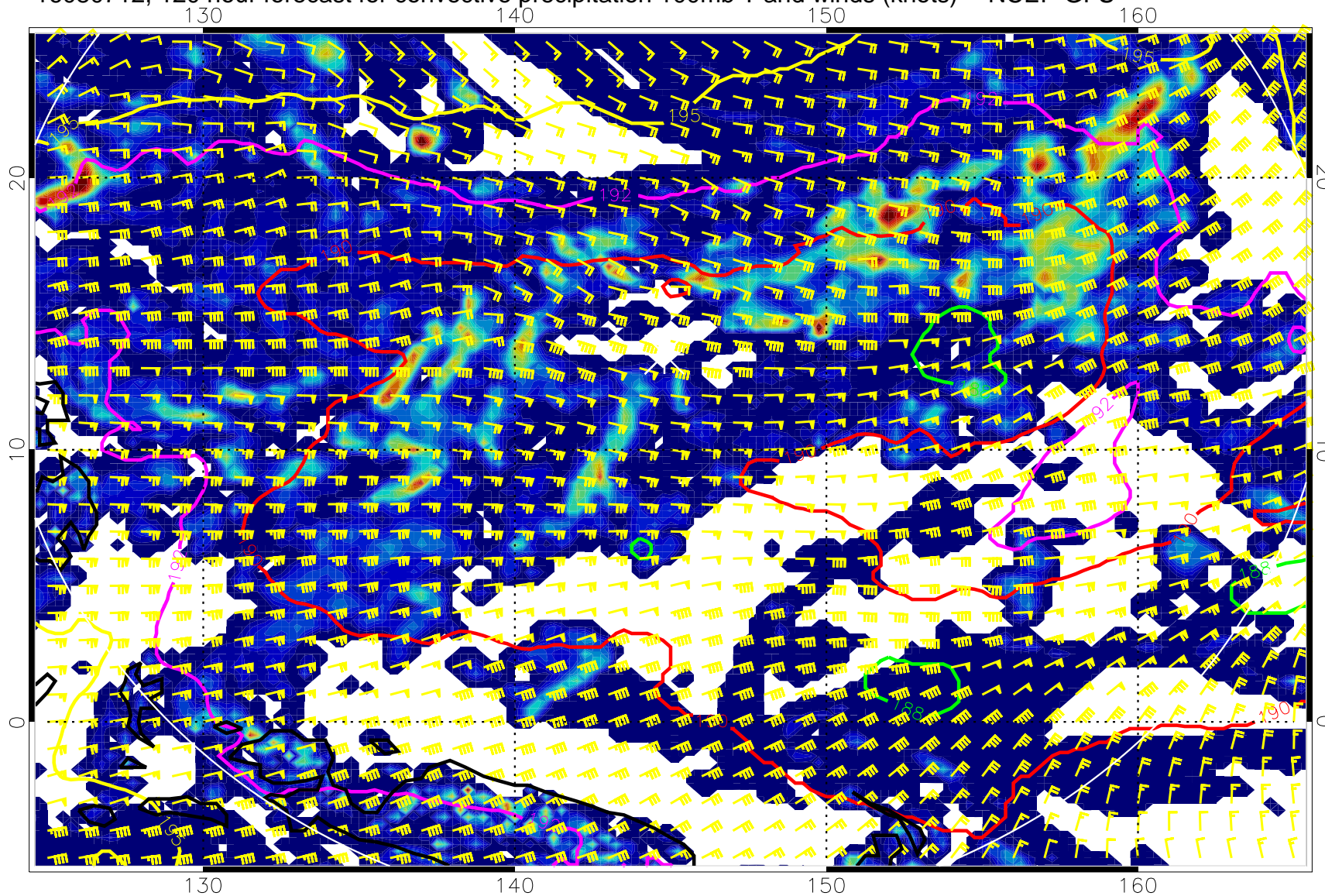
16080712, 120 hour forecast for convective precipitation 100mb T and winds (knots) -- NCEP GFS
