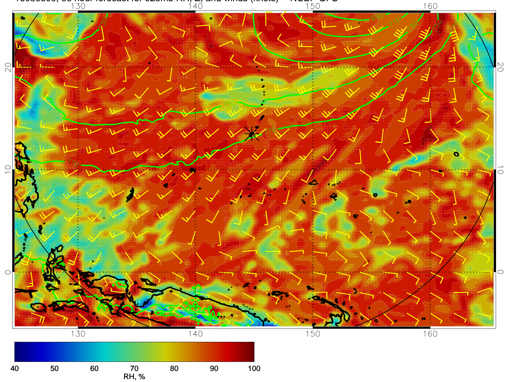
16080600, 96 hour forecast for 925mb RH, Z, and winds (knots) -- NCEP GFS
