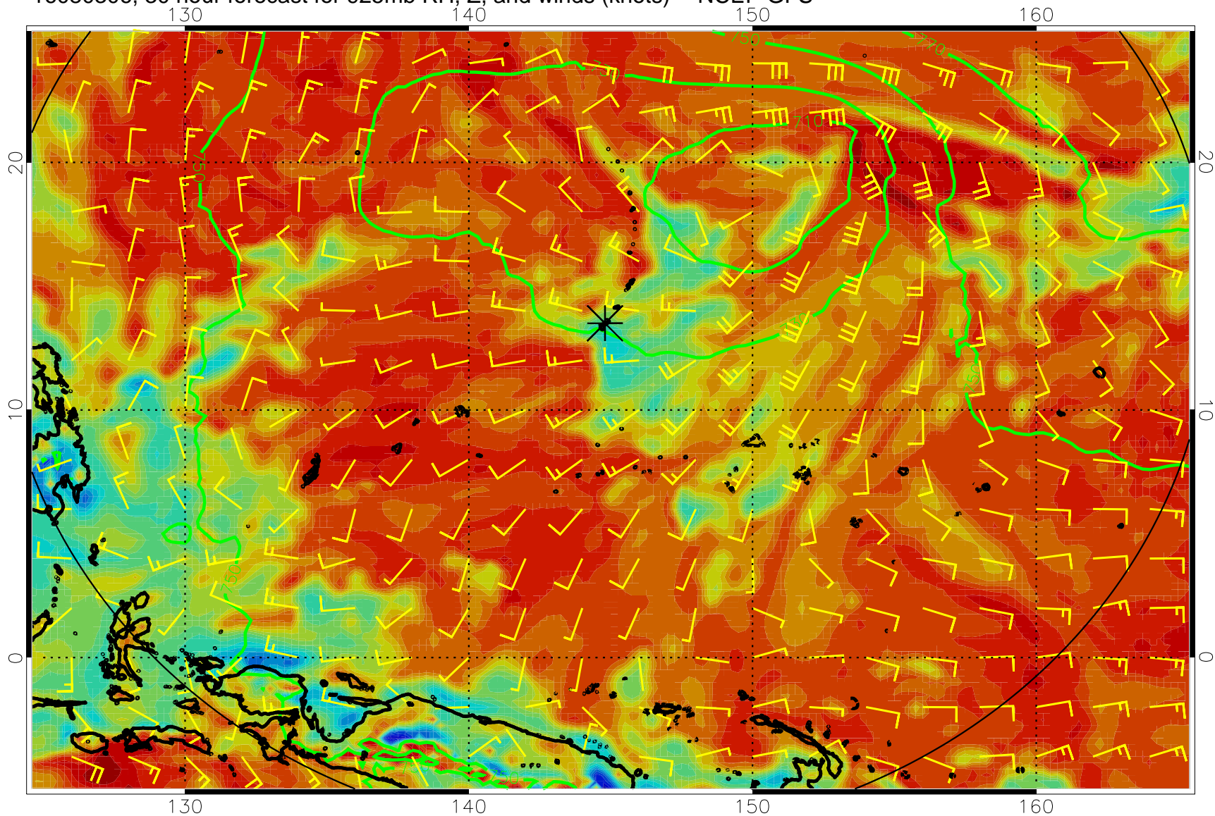
16080306, 30 hour forecast for 925mb RH, Z, and winds (knots) -- NCEP GFS
