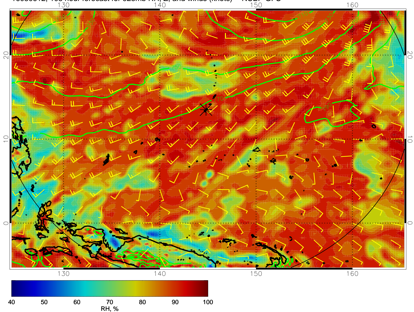
16080612, 108 hour forecast for 925mb RH, Z, and winds (knots) -- NCEP GFS
