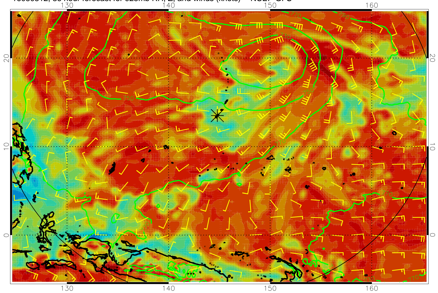
16080312, 36 hour forecast for 925mb RH, Z, and winds (knots) -- NCEP GFS
