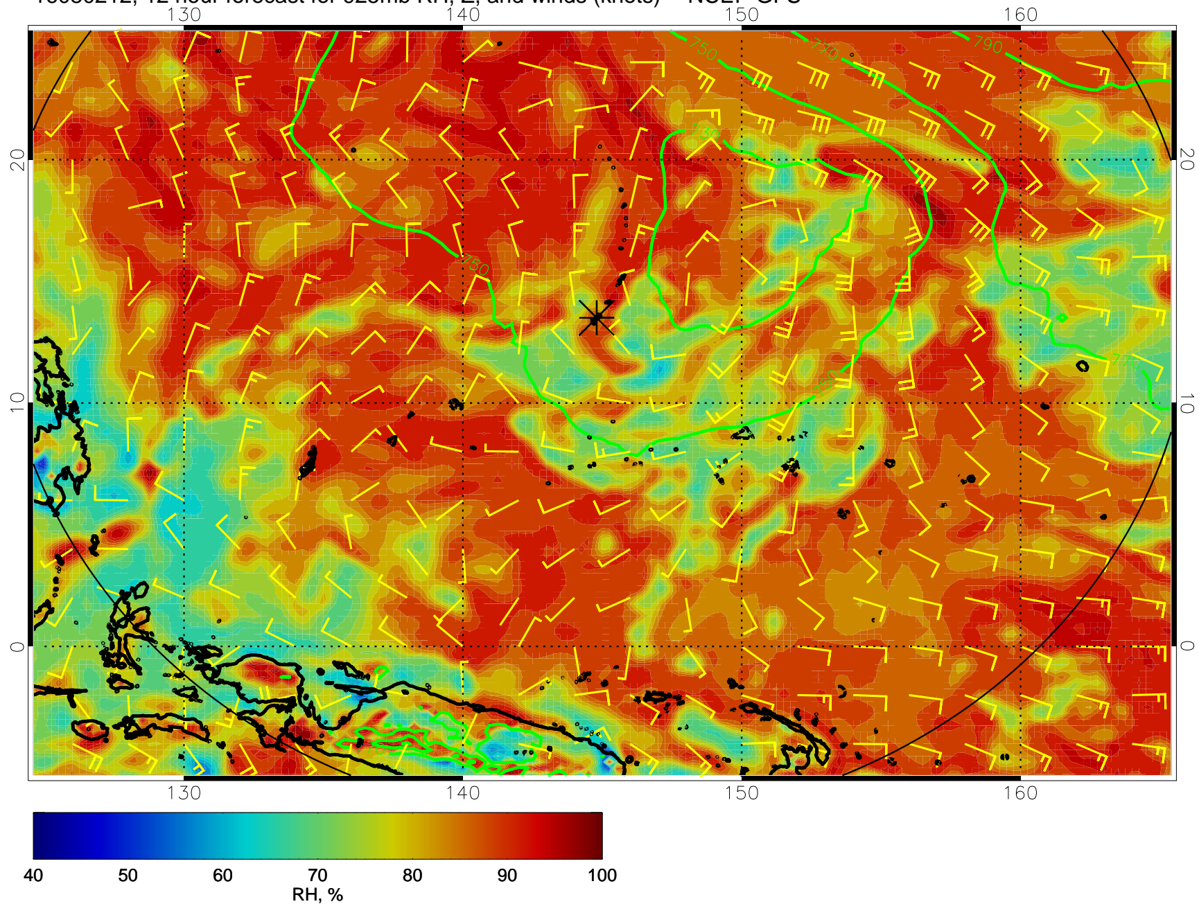
16080212, 12 hour forecast for 925mb RH, Z, and winds (knots) -- NCEP GFS
