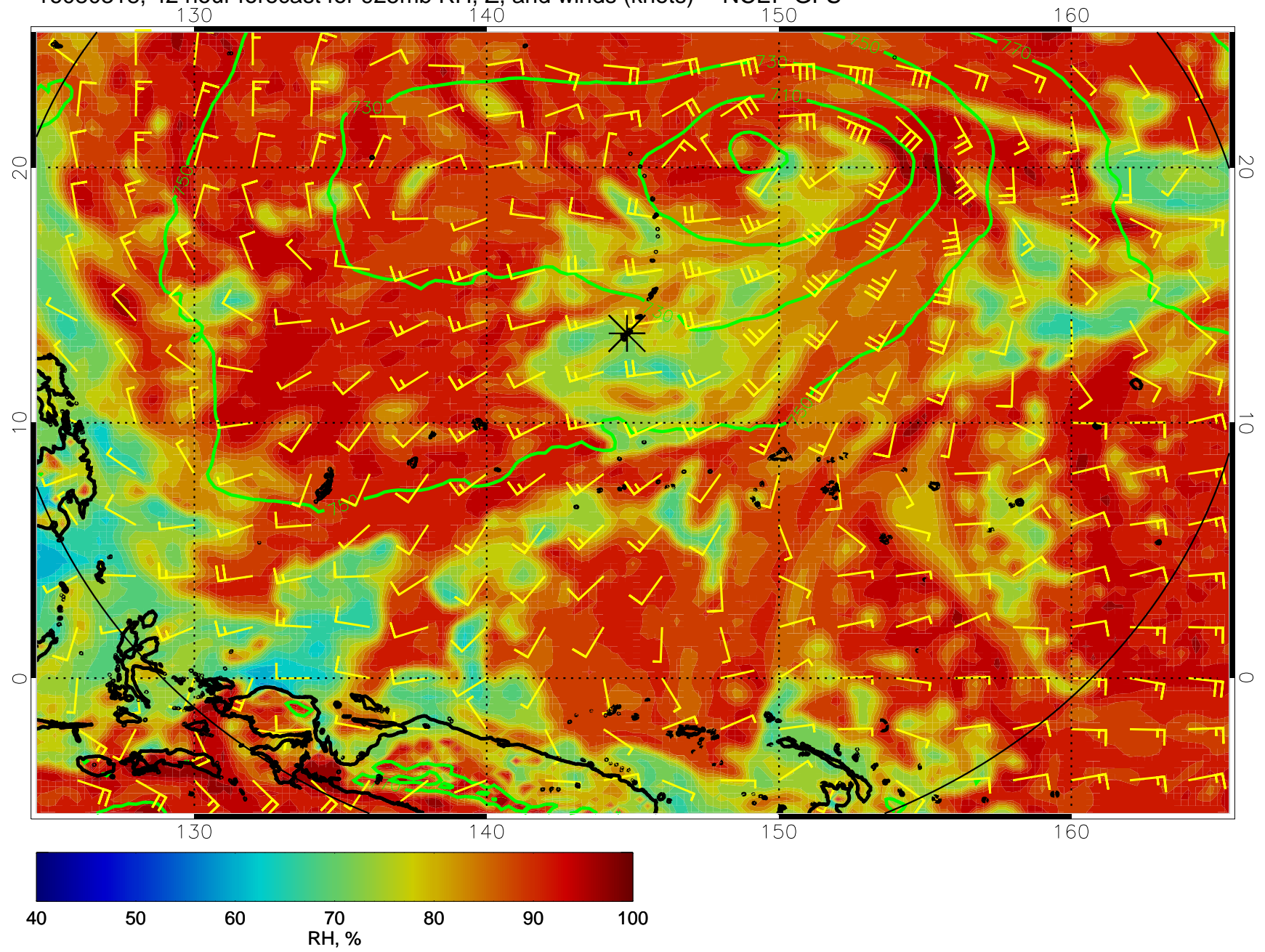
16080318, 42 hour forecast for 925mb RH, Z, and winds (knots) -- NCEP GFS
