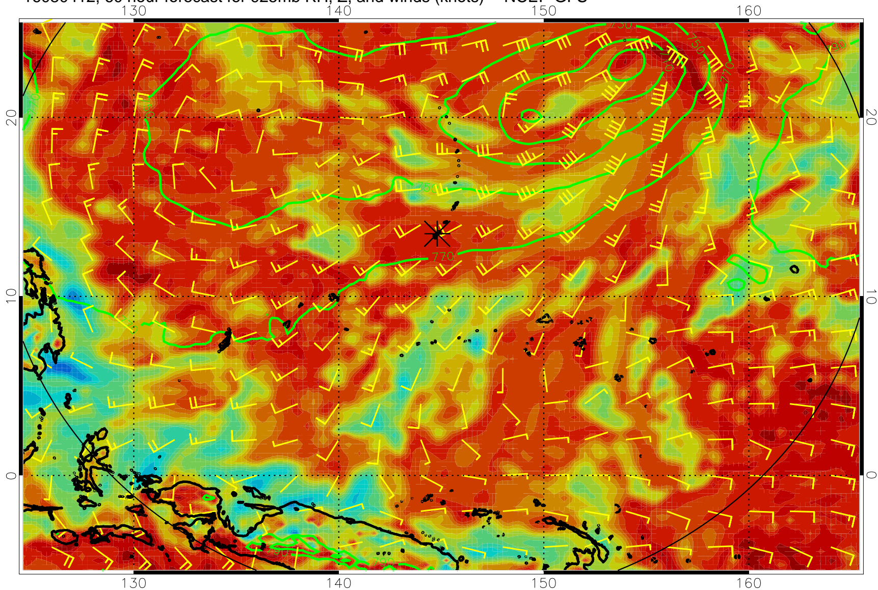
16080412, 60 hour forecast for 925mb RH, Z, and winds (knots) -- NCEP GFS
