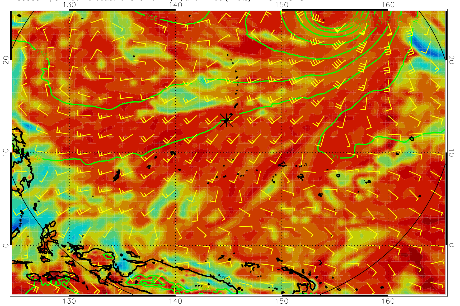
16080512, 84 hour forecast for 925mb RH, Z, and winds (knots) -- NCEP GFS
