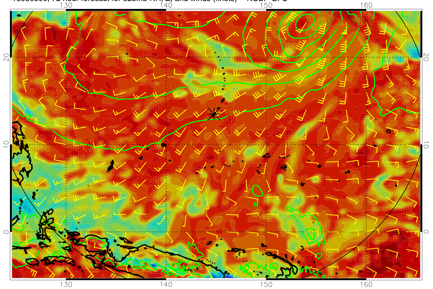
16080500, 72 hour forecast for 925mb RH, Z, and winds (knots) -- NCEP GFS
