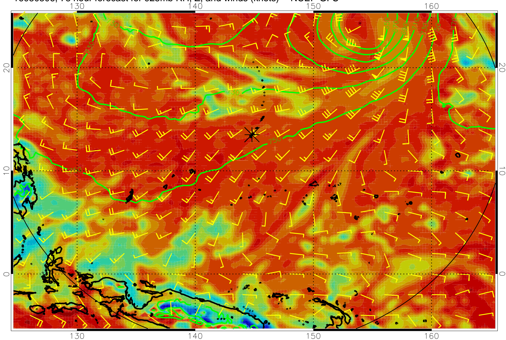
16080506, 78 hour forecast for 925mb RH, Z, and winds (knots) -- NCEP GFS
