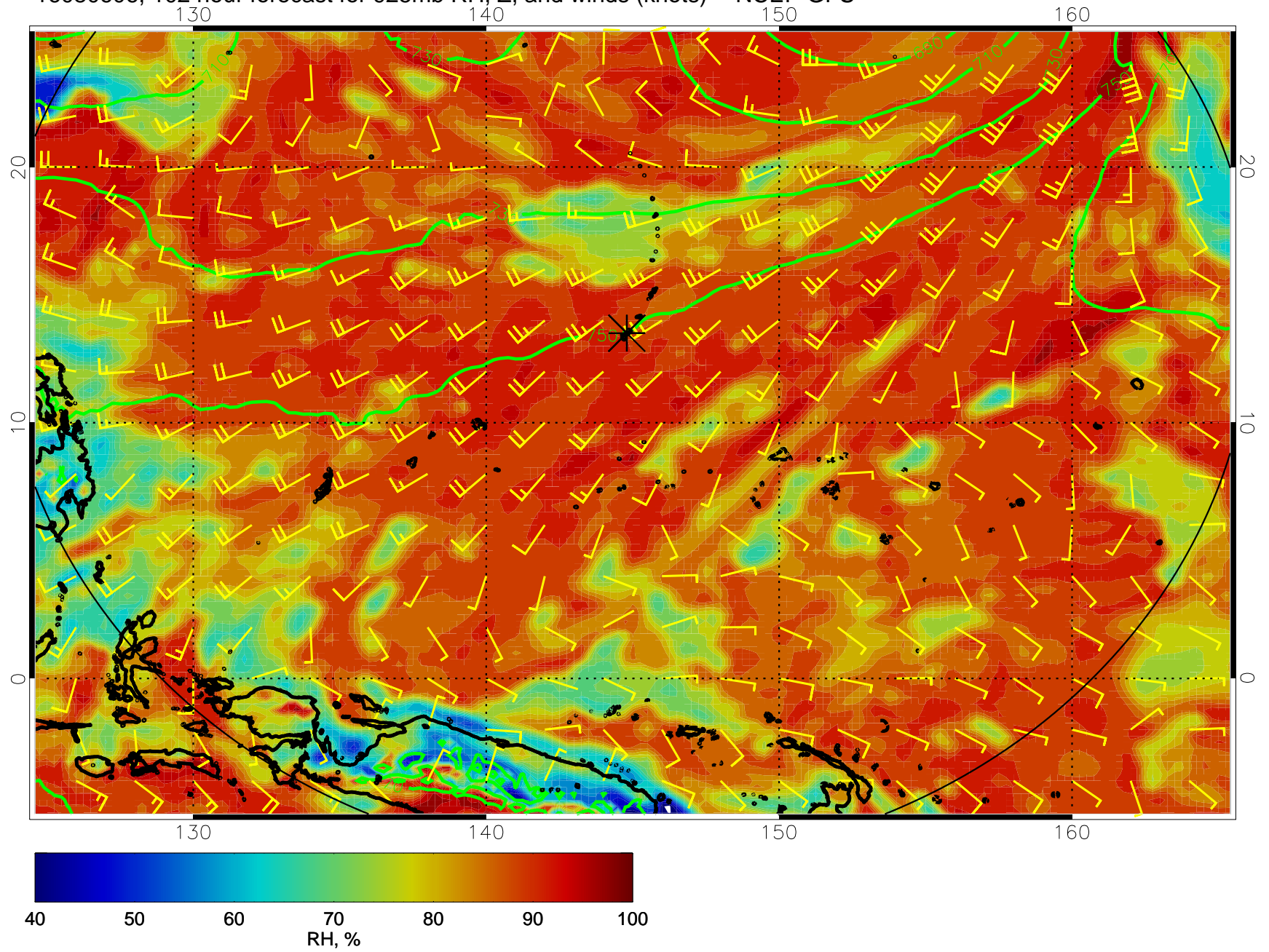
16080606, 102 hour forecast for 925mb RH, Z, and winds (knots) -- NCEP GFS
