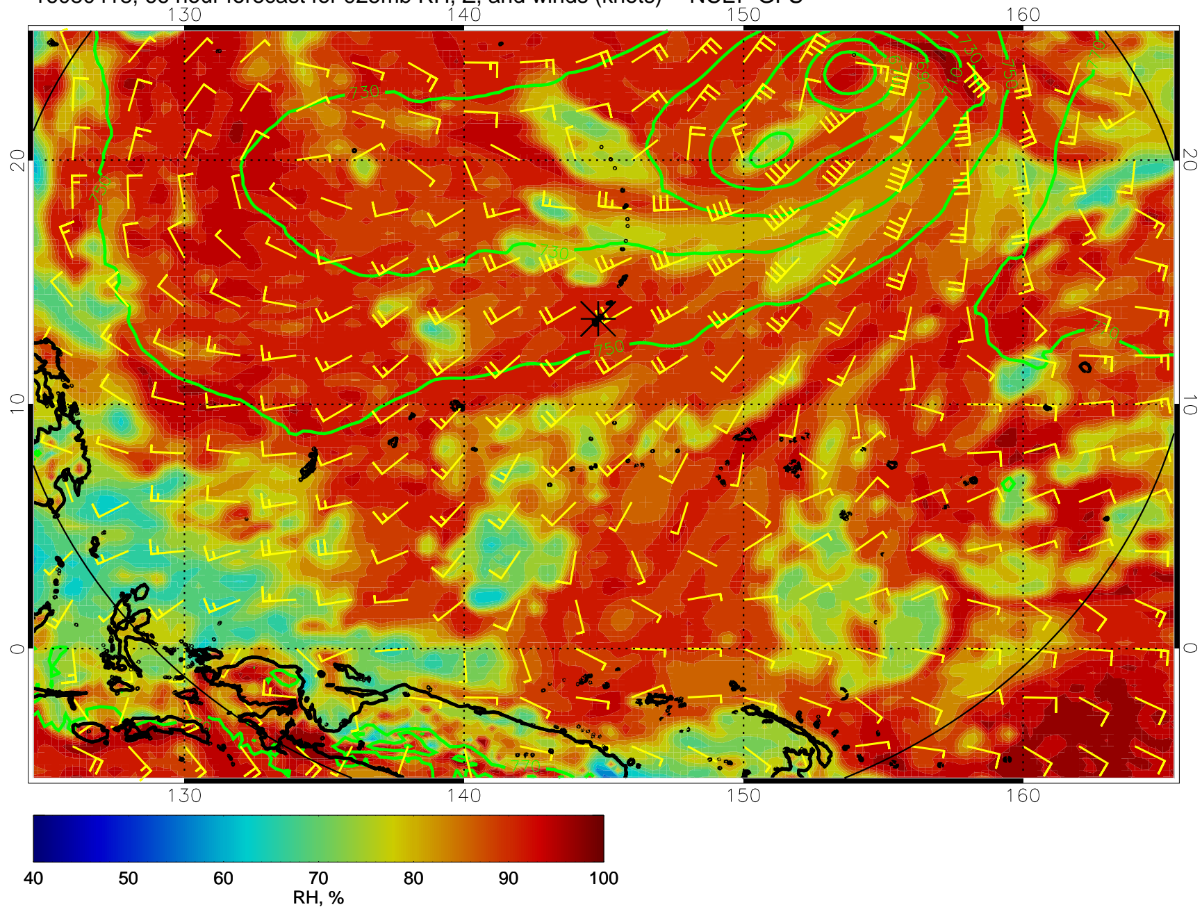
16080418, 66 hour forecast for 925mb RH, Z, and winds (knots) -- NCEP GFS
