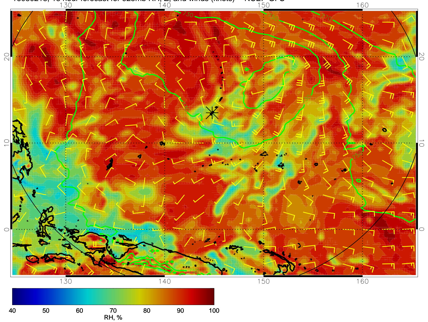
16080218, 18 hour forecast for 925mb RH, Z, and winds (knots) -- NCEP GFS
