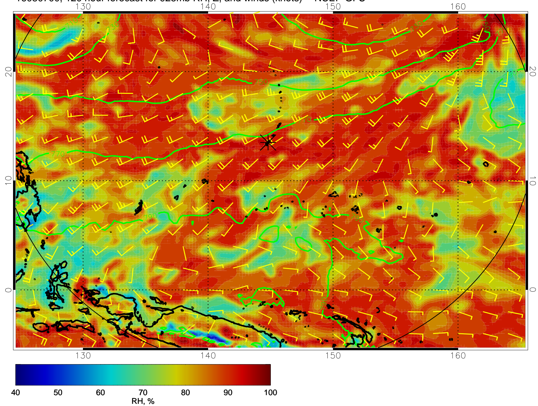
16080700, 120 hour forecast for 925mb RH, Z, and winds (knots) -- NCEP GFS
