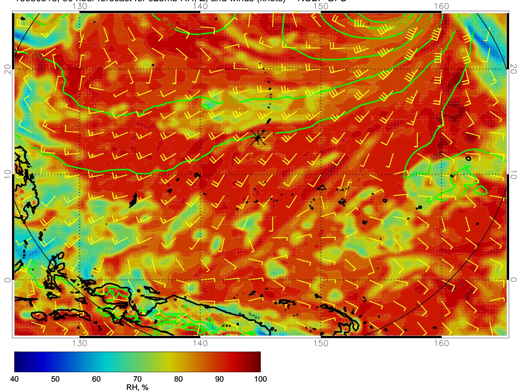
16080518, 90 hour forecast for 925mb RH, Z, and winds (knots) -- NCEP GFS
