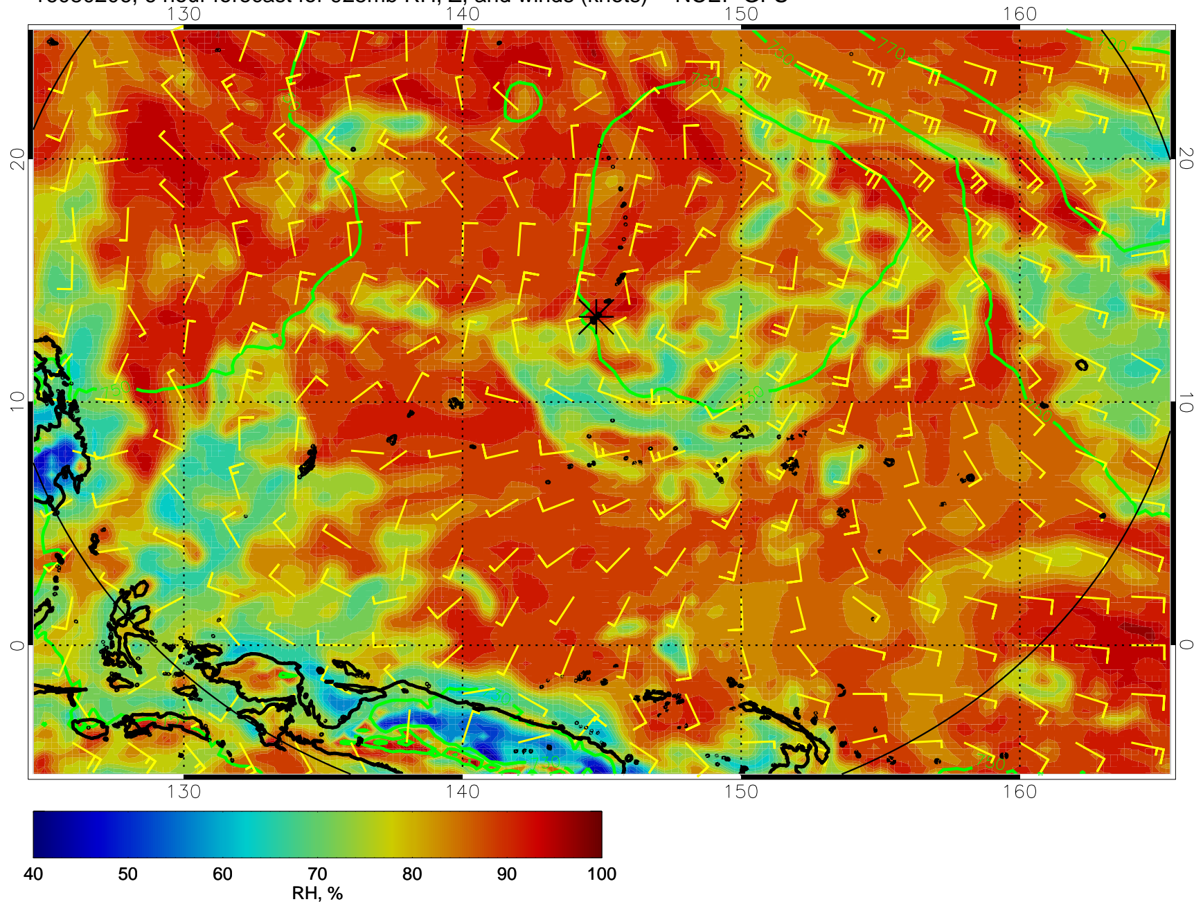
16080206, 6 hour forecast for 925mb RH, Z, and winds (knots) -- NCEP GFS
