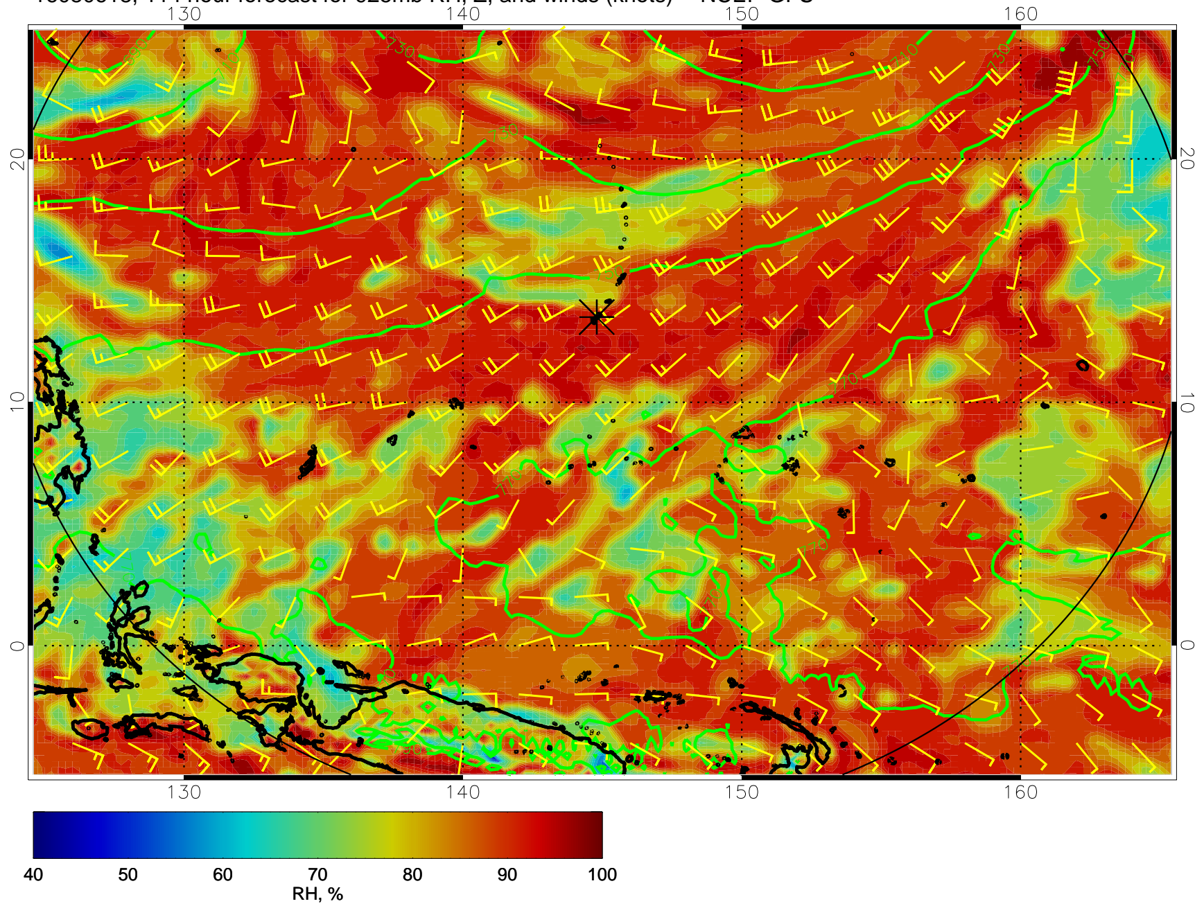
16080618, 114 hour forecast for 925mb RH, Z, and winds (knots) -- NCEP GFS
