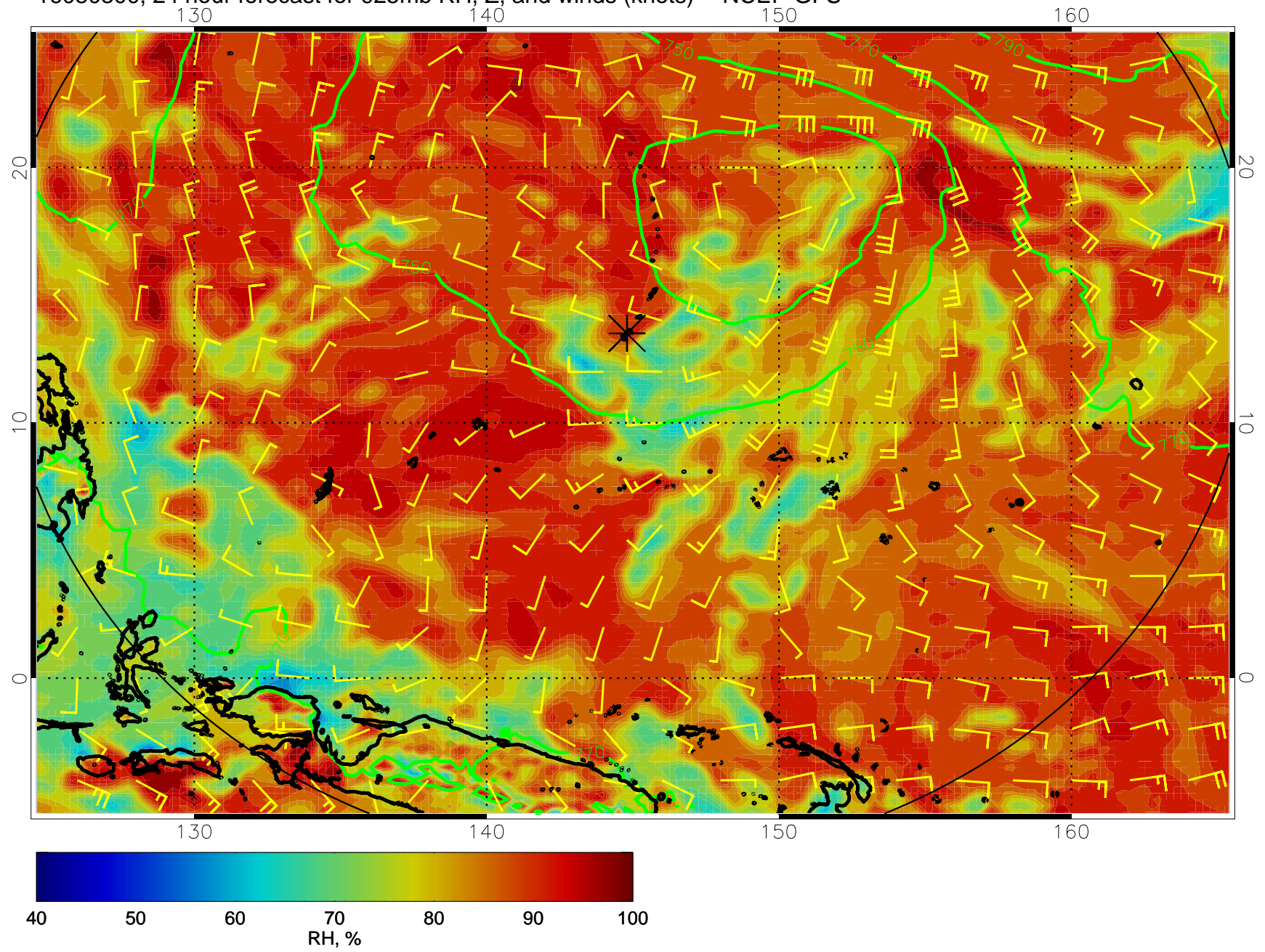
16080300, 24 hour forecast for 925mb RH, Z, and winds (knots) -- NCEP GFS
