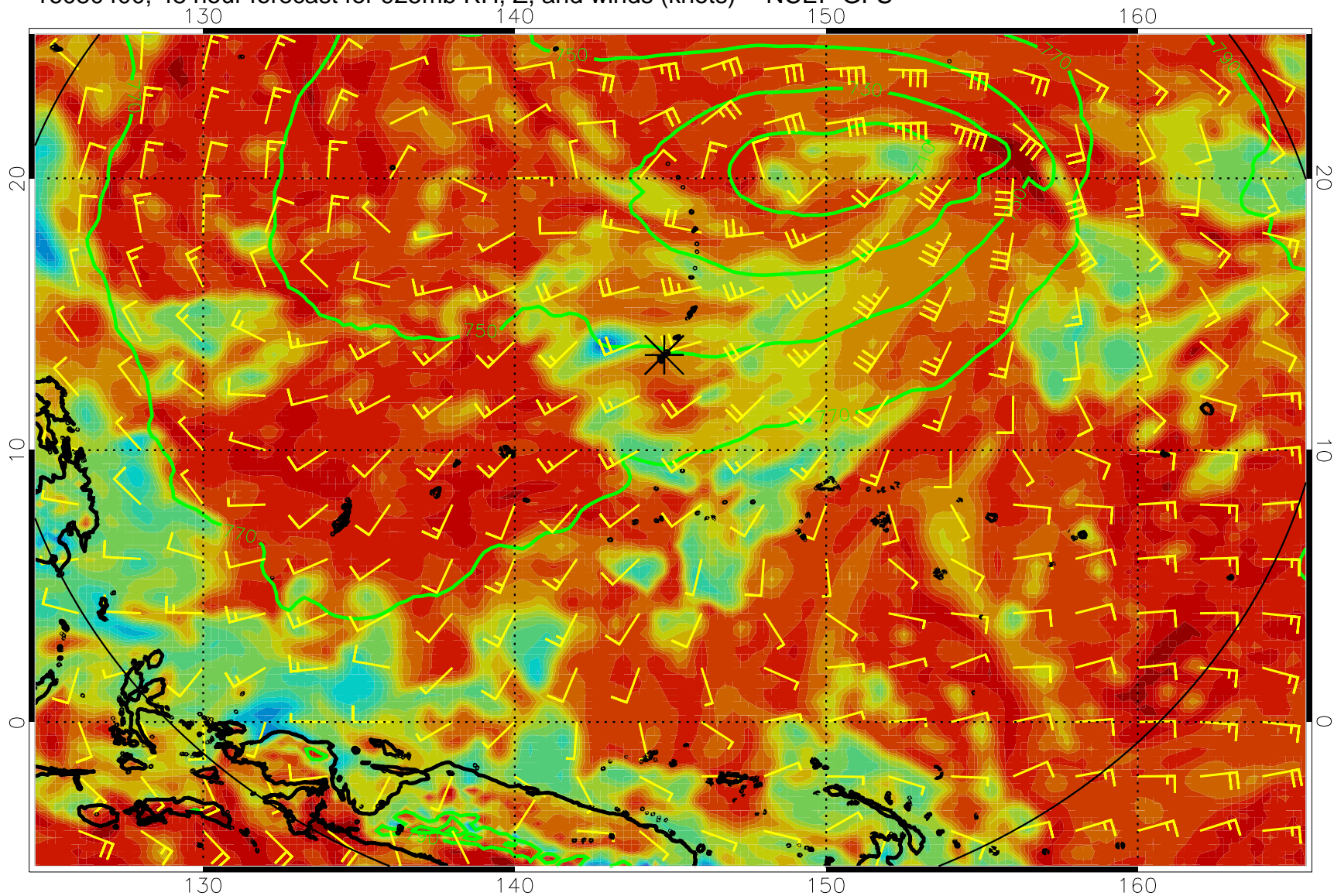
16080400, 48 hour forecast for 925mb RH, Z, and winds (knots) -- NCEP GFS
