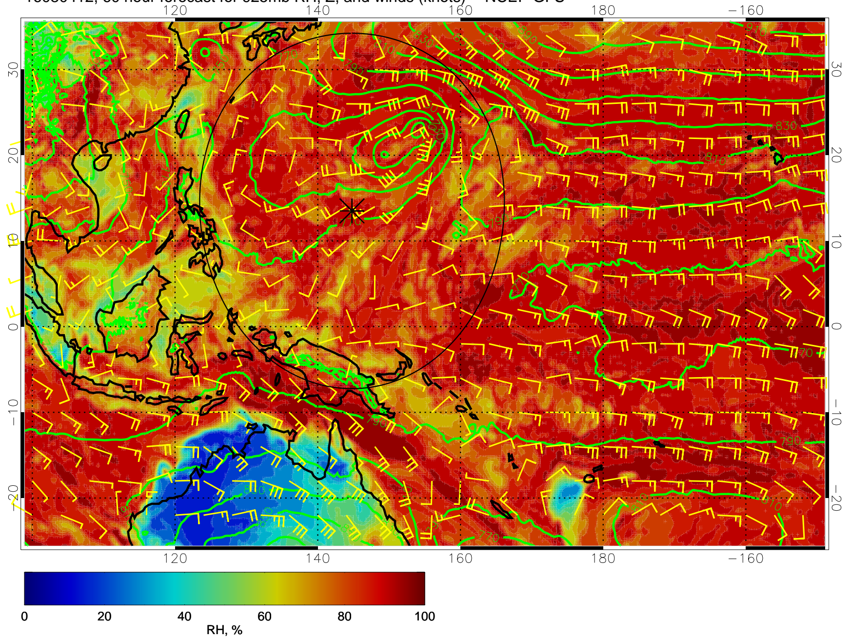
16080412, 60 hour forecast for 925mb RH, Z, and winds (knots) -- NCEP GFS
