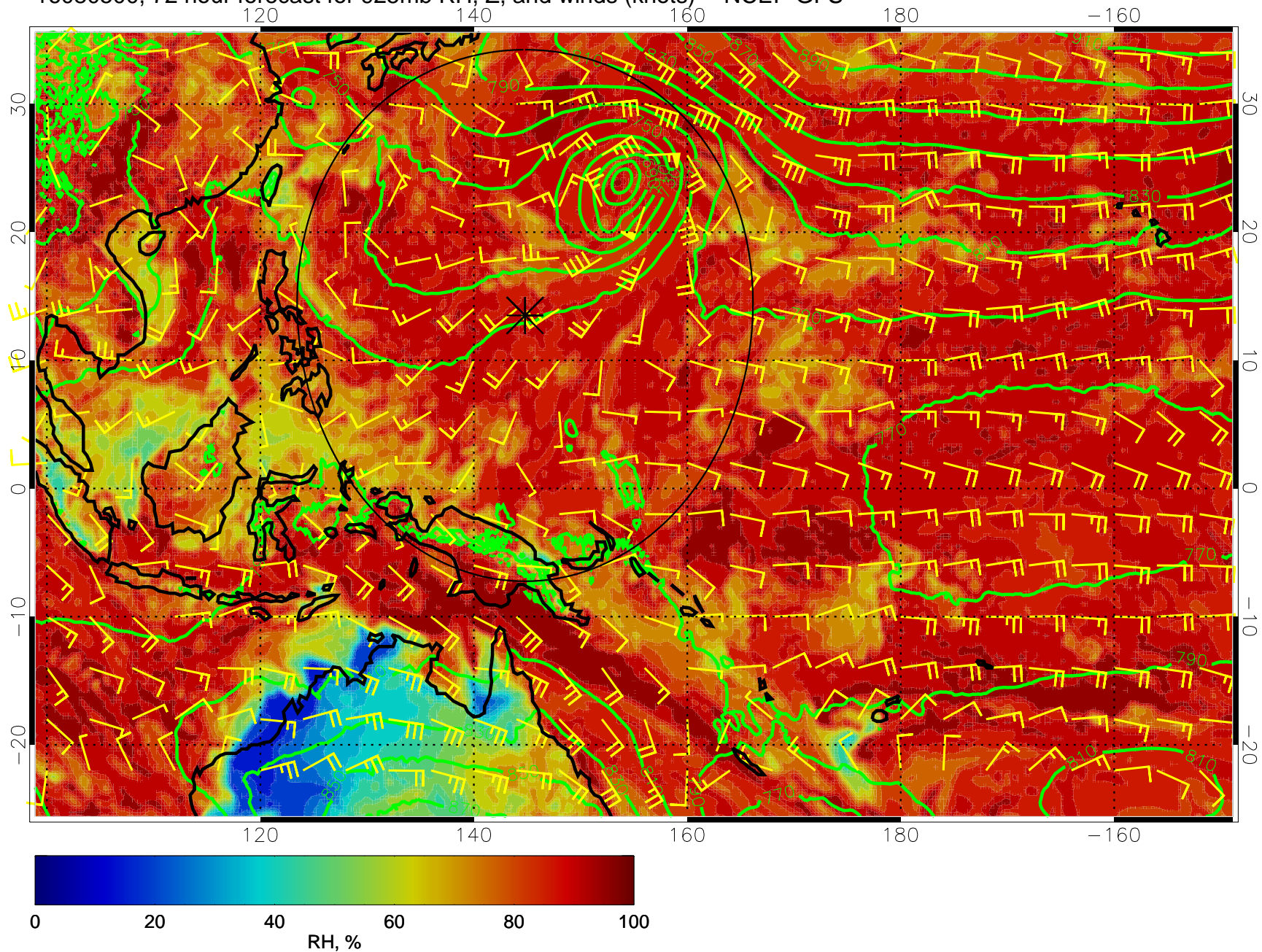
16080500, 72 hour forecast for 925mb RH, Z, and winds (knots) -- NCEP GFS
