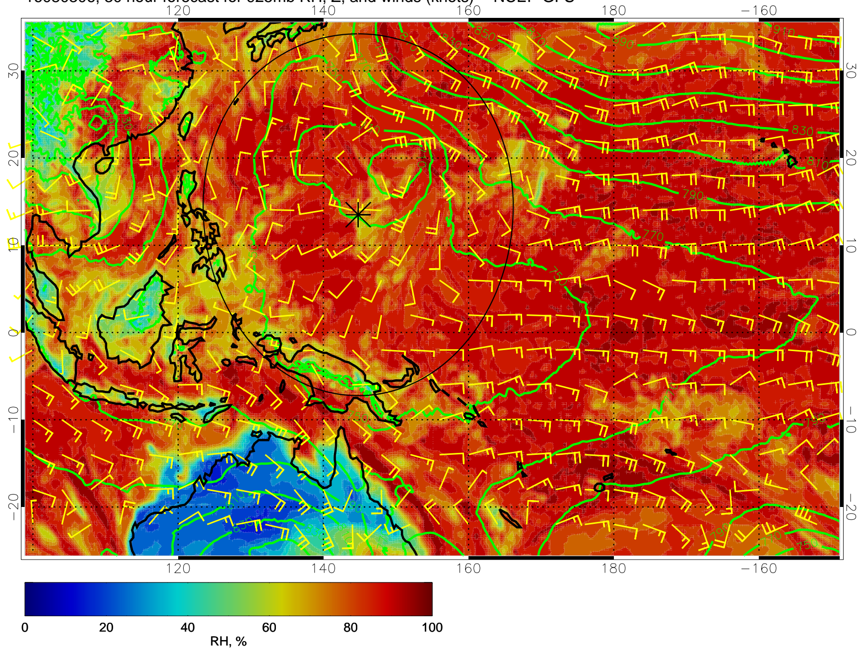
16080306, 30 hour forecast for 925mb RH, Z, and winds (knots) -- NCEP GFS
