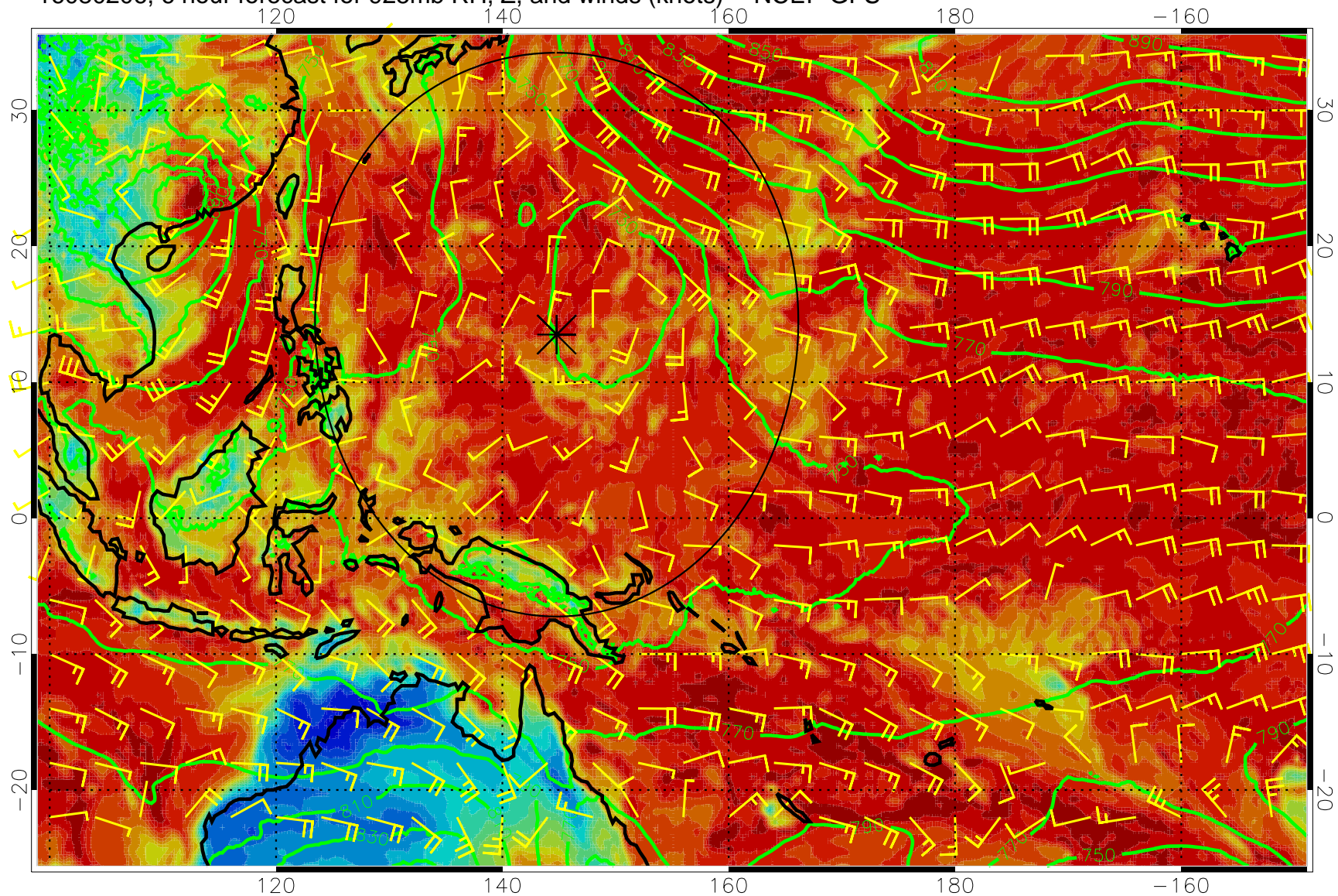
16080206, 6 hour forecast for 925mb RH, Z, and winds (knots) -- NCEP GFS
