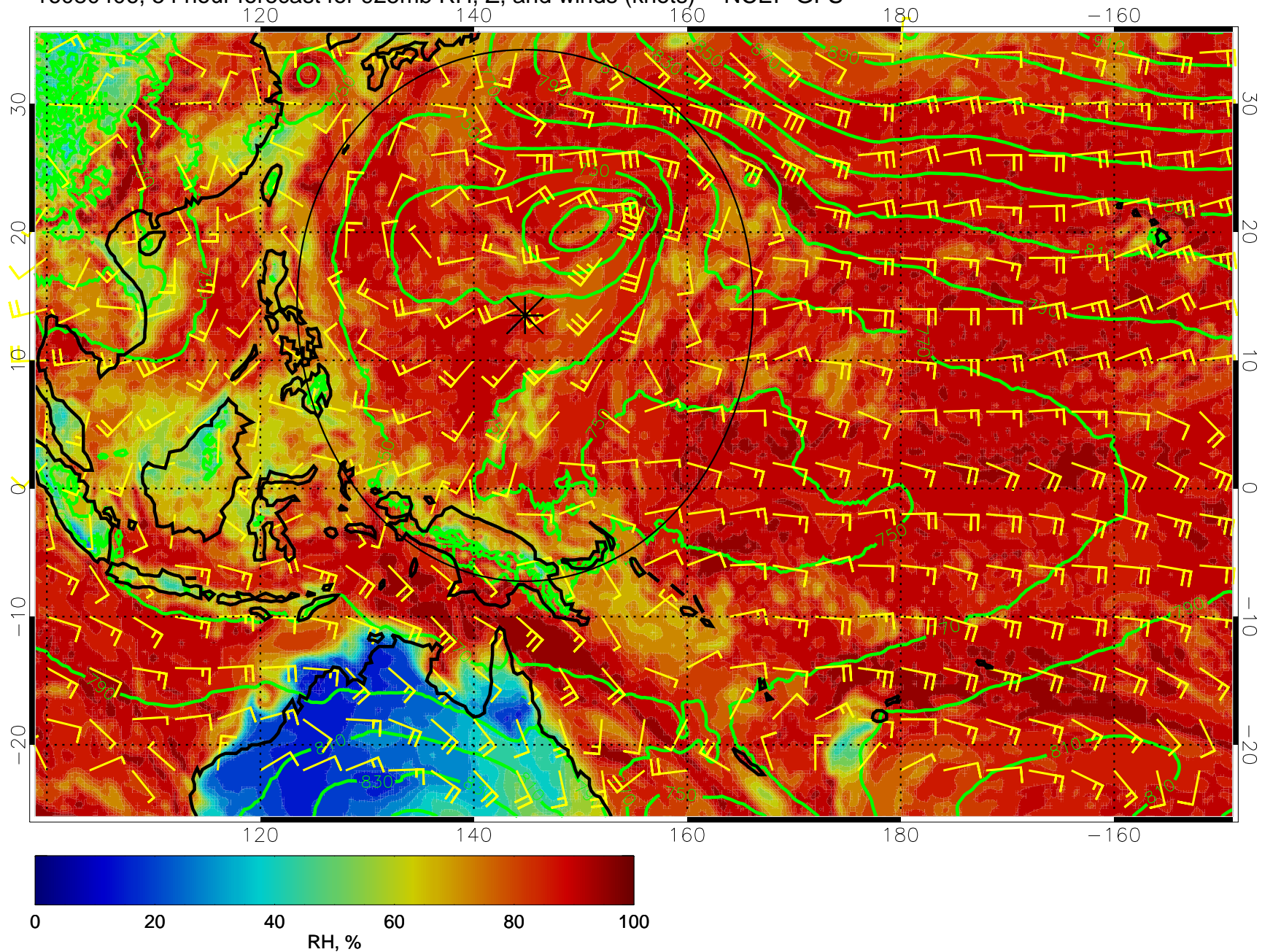
16080406, 54 hour forecast for 925mb RH, Z, and winds (knots) -- NCEP GFS
