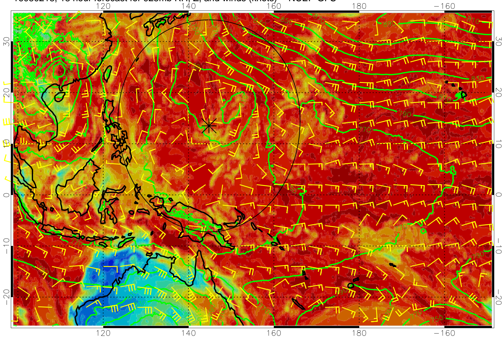
16080218, 18 hour forecast for 925mb RH, Z, and winds (knots) -- NCEP GFS
