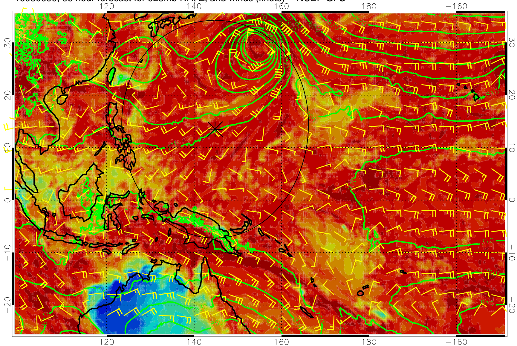
16080600, 96 hour forecast for 925mb RH, Z, and winds (knots) -- NCEP GFS
