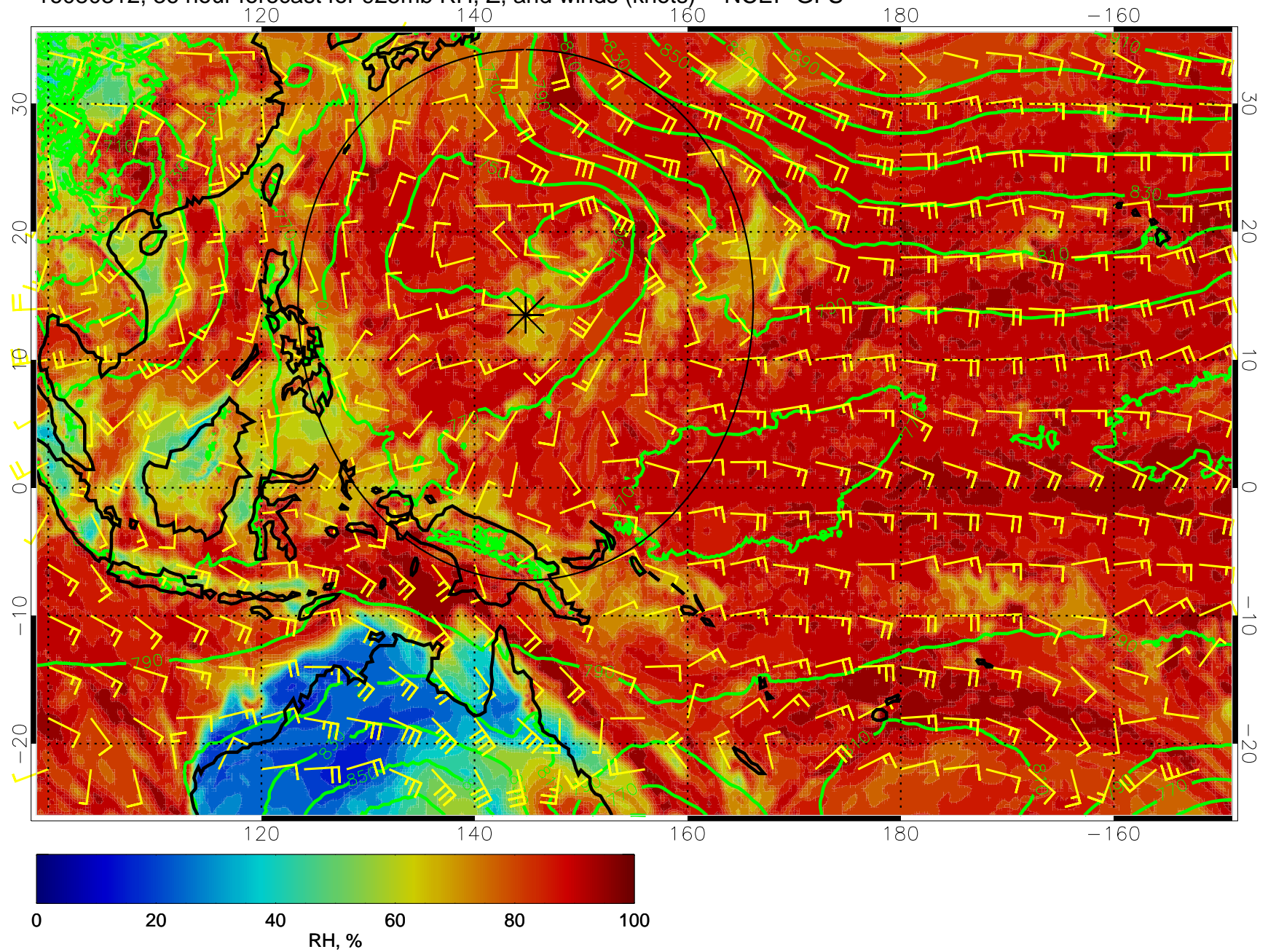
16080312, 36 hour forecast for 925mb RH, Z, and winds (knots) -- NCEP GFS
