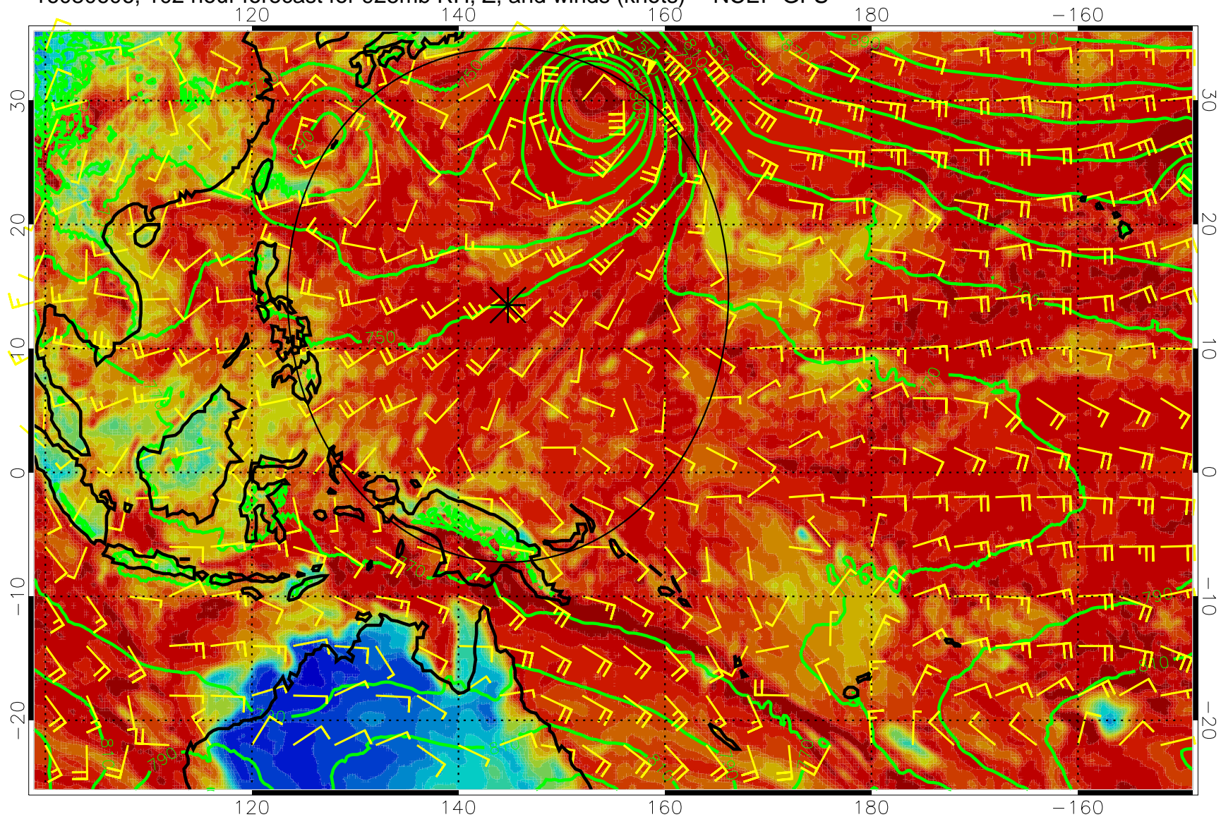
16080606, 102 hour forecast for 925mb RH, Z, and winds (knots) -- NCEP GFS
