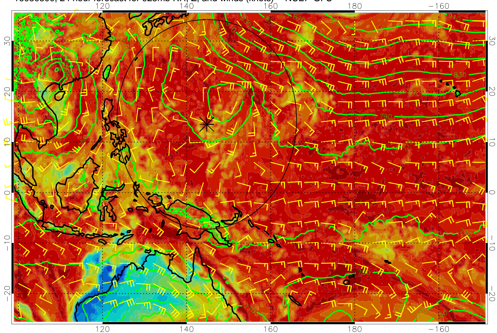
16080300, 24 hour forecast for 925mb RH, Z, and winds (knots) -- NCEP GFS
