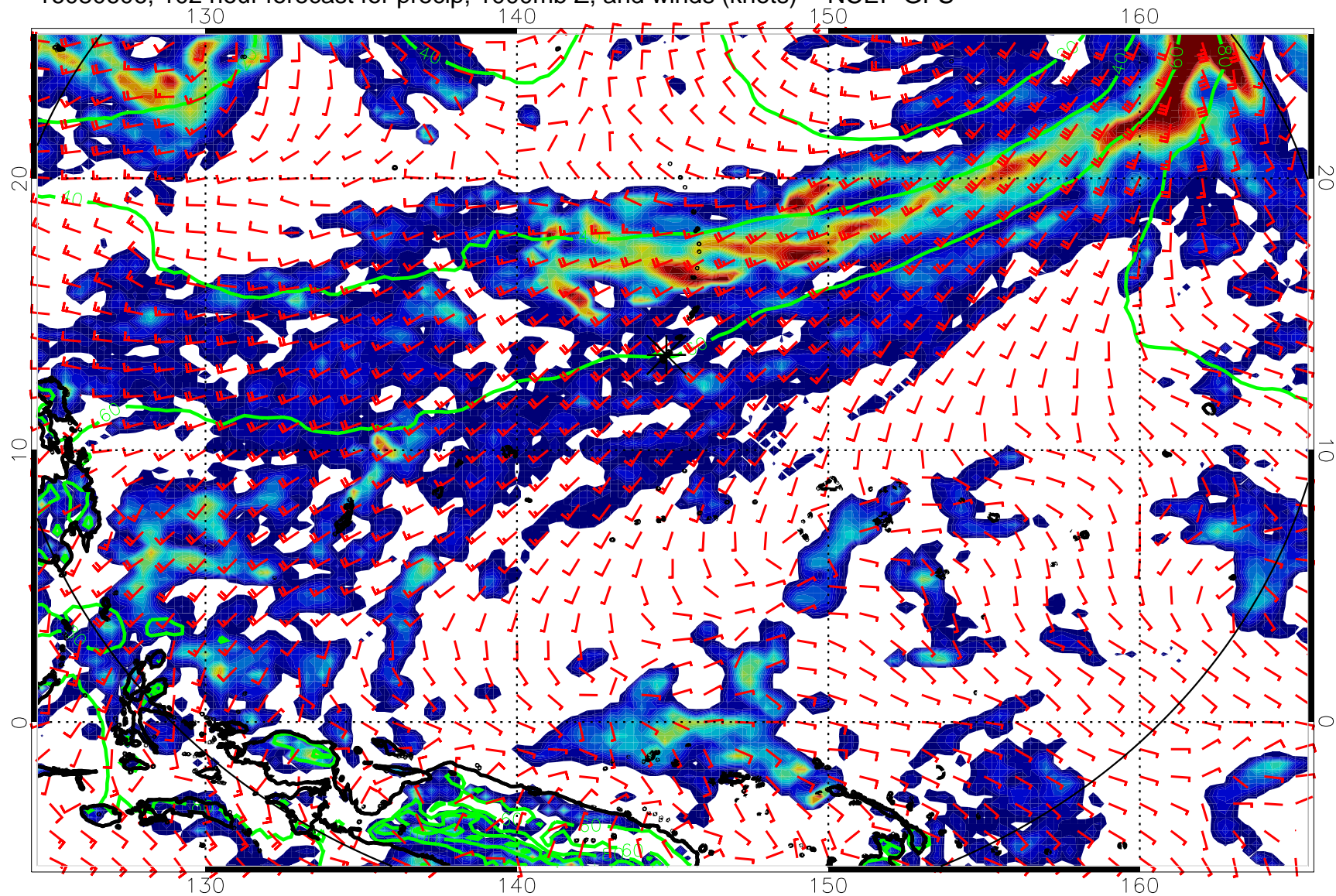
16080606, 102 hour forecast for precip, 1000mb Z, and winds (knots) -- NCEP GFS
