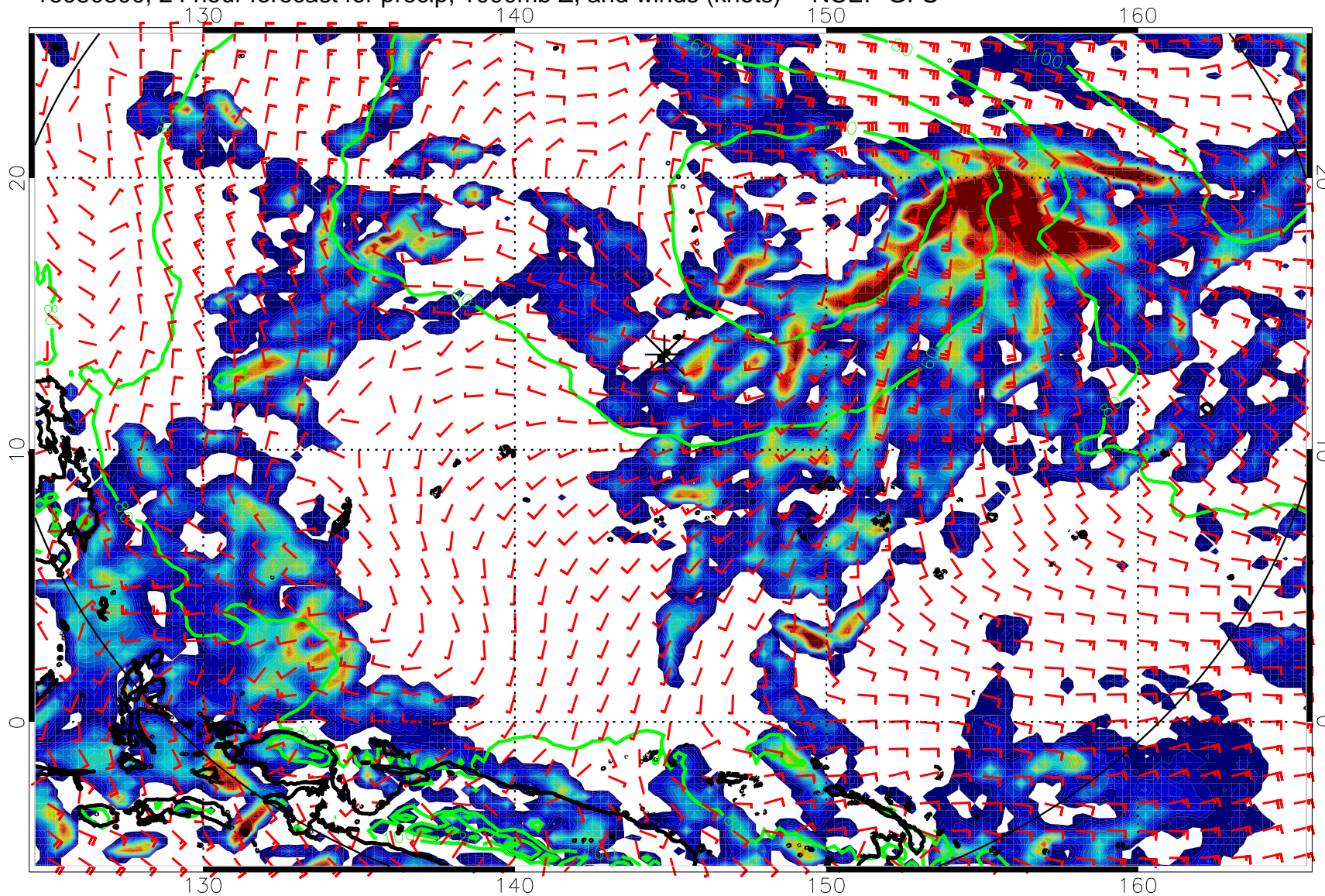
16080300, 24 hour forecast for precip, 1000mb Z, and winds (knots) -- NCEP GFS
