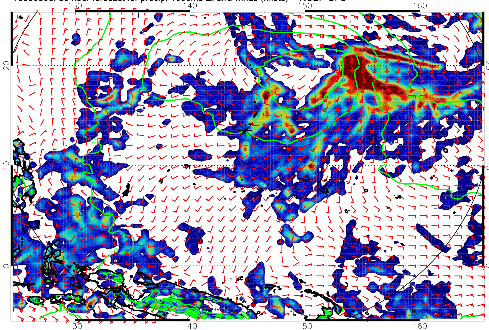
16080306, 30 hour forecast for precip, 1000mb Z, and winds (knots) -- NCEP GFS
