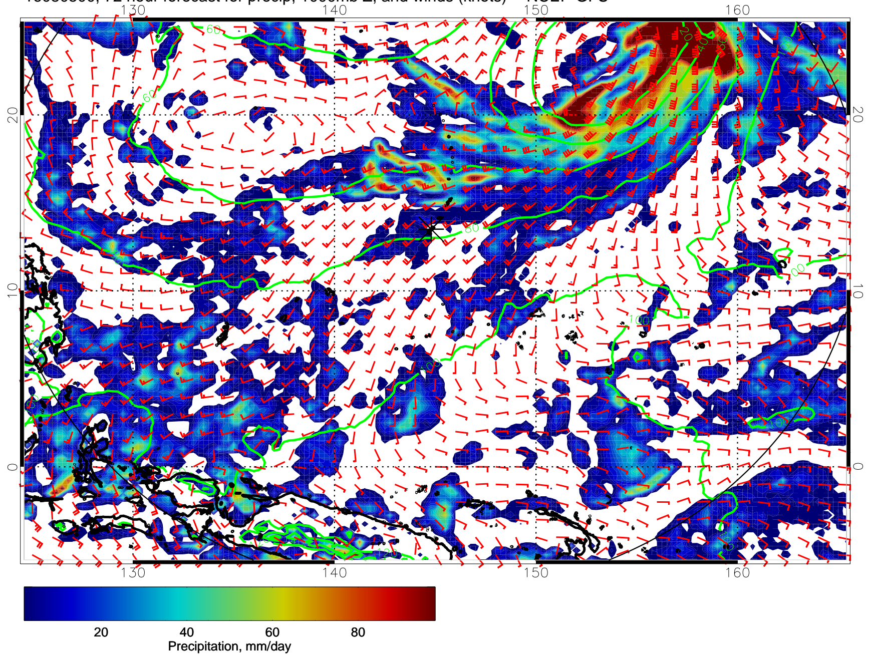
16080500, 72 hour forecast for precip, 1000mb Z, and winds (knots) -- NCEP GFS
