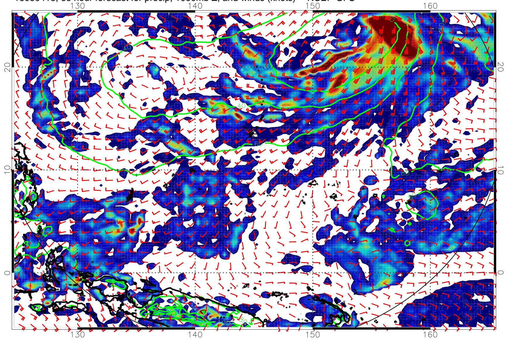
16080418, 66 hour forecast for precip, 1000mb Z, and winds (knots) -- NCEP GFS
