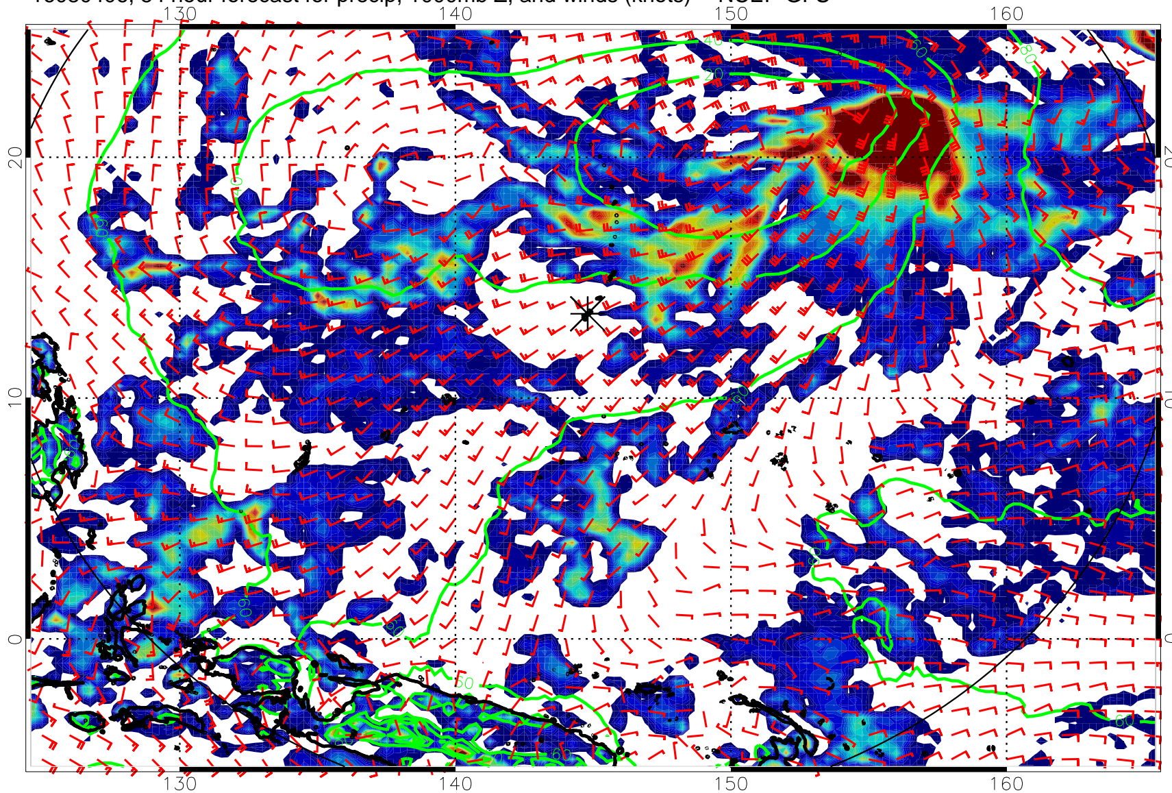
16080406, 54 hour forecast for precip, 1000mb Z, and winds (knots) -- NCEP GFS
