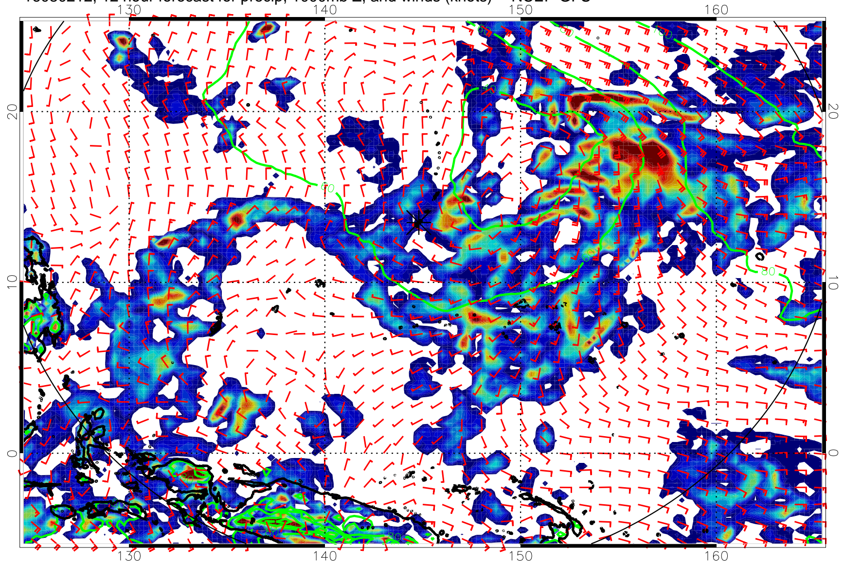
16080212, 12 hour forecast for precip, 1000mb Z, and winds (knots) -- NCEP GFS
