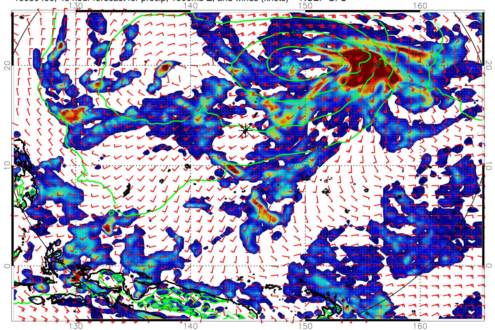
16080400, 48 hour forecast for precip, 1000mb Z, and winds (knots) -- NCEP GFS
