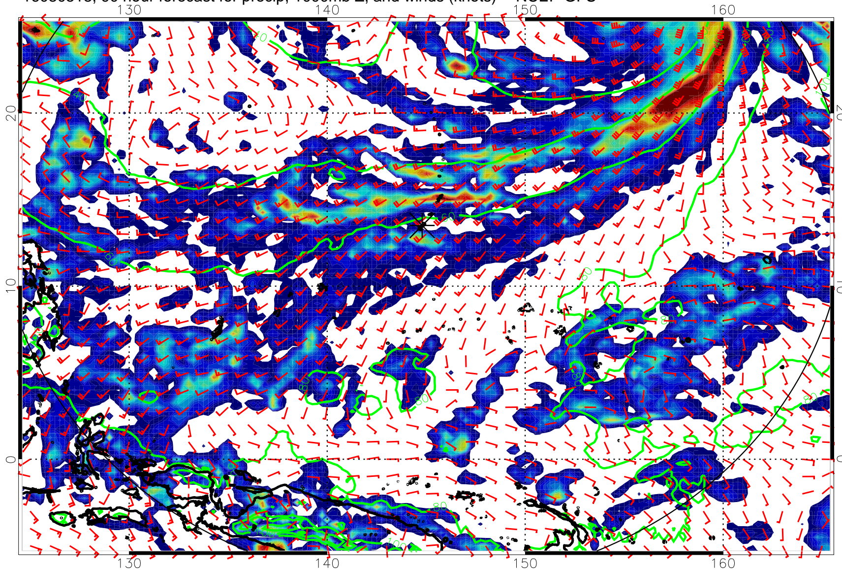
16080518, 90 hour forecast for precip, 1000mb Z, and winds (knots) -- NCEP GFS
