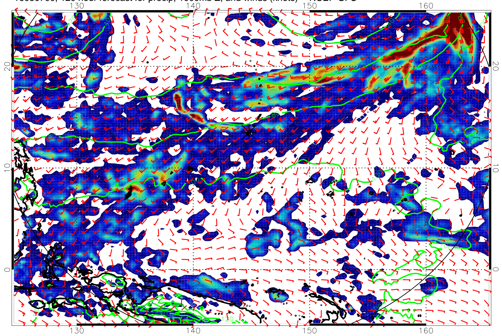
16080700, 120 hour forecast for precip, 1000mb Z, and winds (knots) -- NCEP GFS
