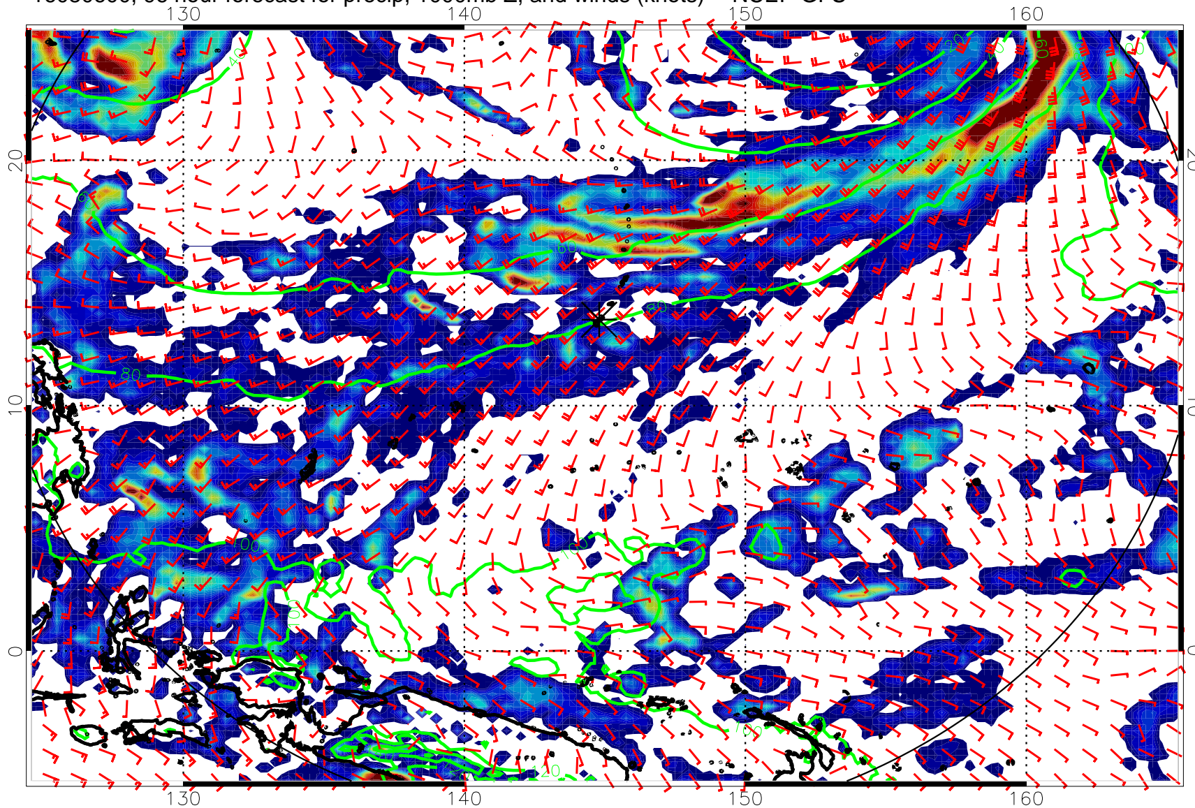
16080600, 96 hour forecast for precip, 1000mb Z, and winds (knots) -- NCEP GFS
