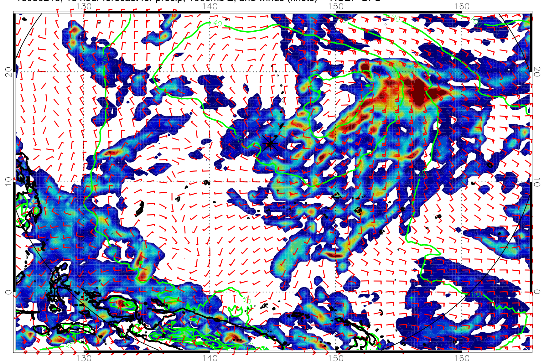
16080218, 18 hour forecast for precip, 1000mb Z, and winds (knots) -- NCEP GFS
