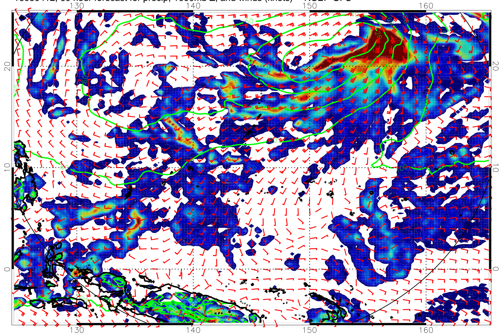
16080412, 60 hour forecast for precip, 1000mb Z, and winds (knots) -- NCEP GFS
