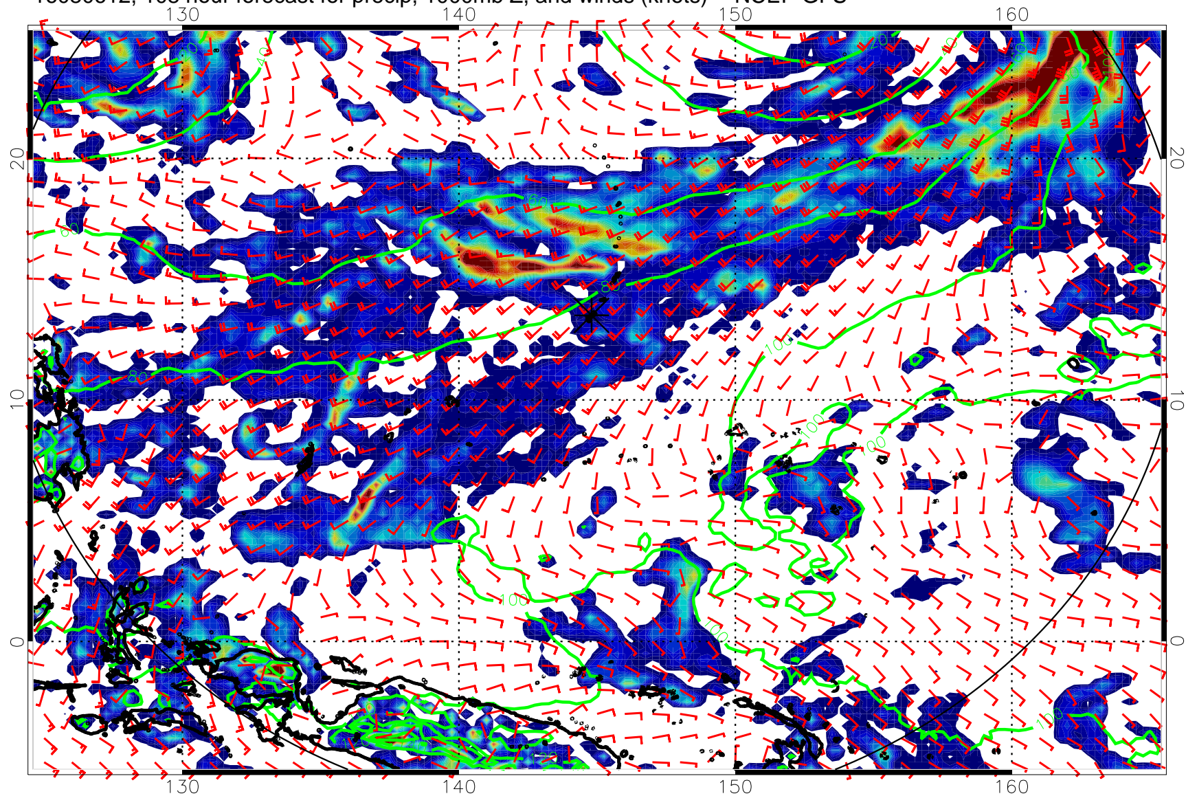
16080612, 108 hour forecast for precip, 1000mb Z, and winds (knots) -- NCEP GFS
