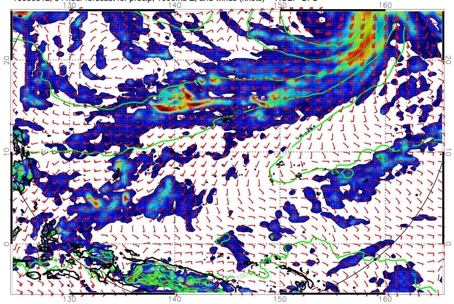
16080512, 84 hour forecast for precip, 1000mb Z, and winds (knots) -- NCEP GFS
