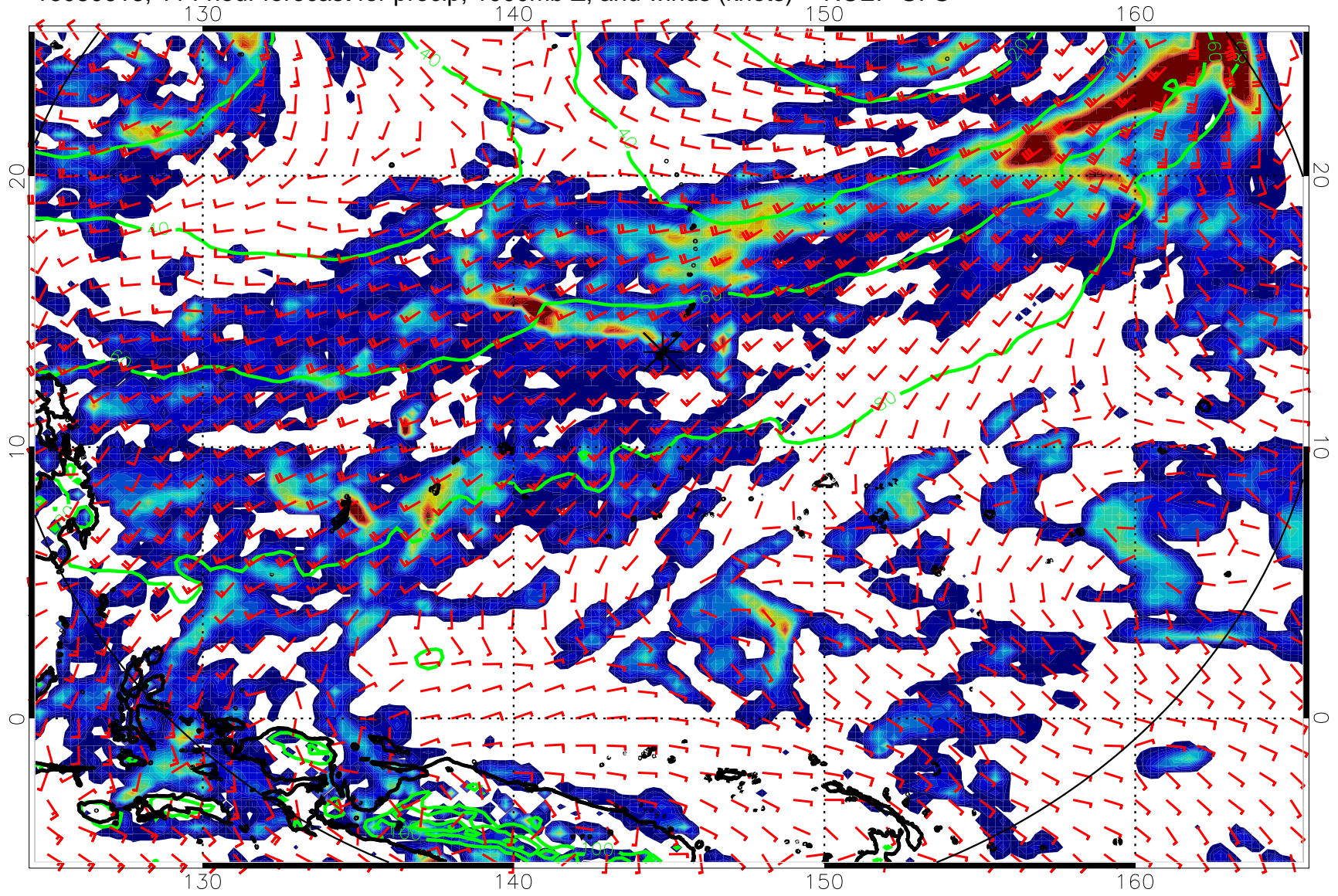
16080618, 114 hour forecast for precip, 1000mb Z, and winds (knots) -- NCEP GFS
