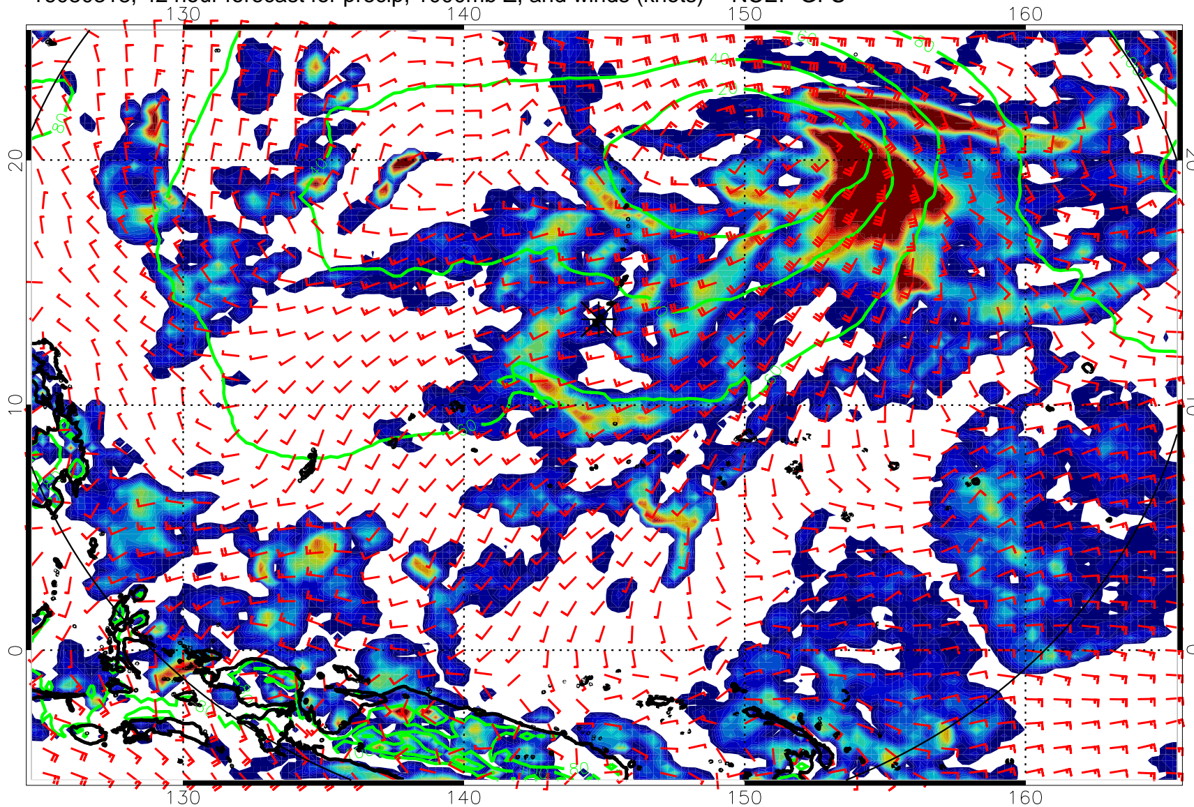
16080318, 42 hour forecast for precip, 1000mb Z, and winds (knots) -- NCEP GFS
