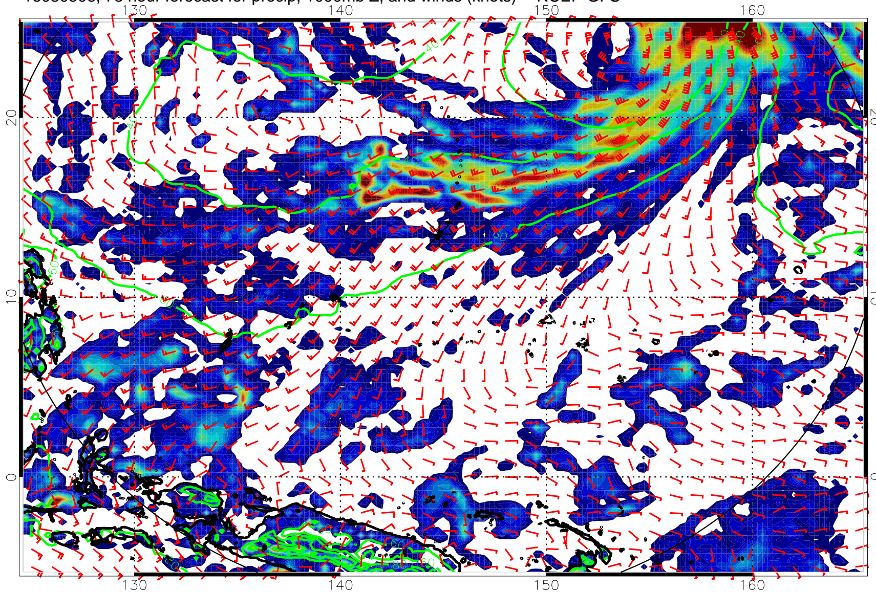
16080506, 78 hour forecast for precip, 1000mb Z, and winds (knots) -- NCEP GFS
