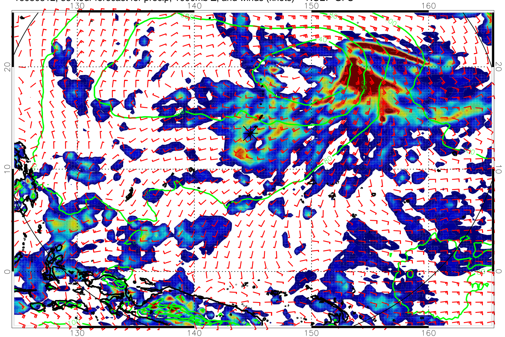
16080312, 36 hour forecast for precip, 1000mb Z, and winds (knots) -- NCEP GFS
