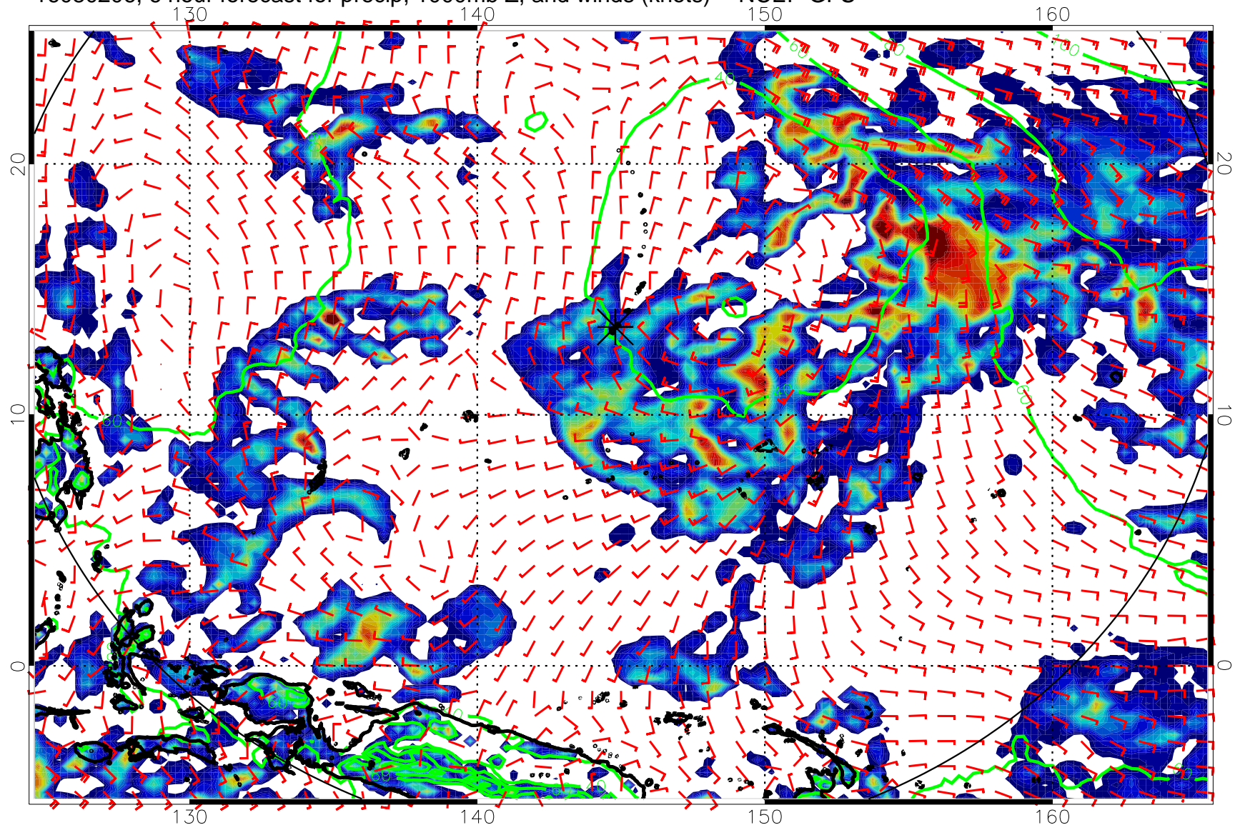
16080206, 6 hour forecast for precip, 1000mb Z, and winds (knots) -- NCEP GFS
