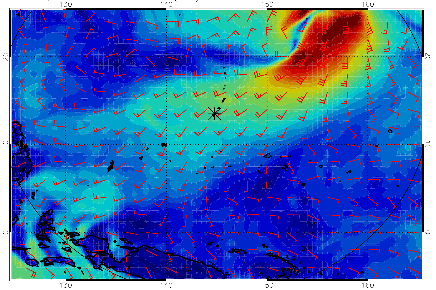
16080500, 72 hour forecast for surface winds (knots) -- NCEP GFS
