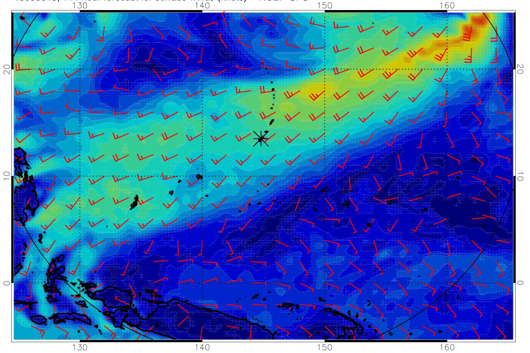
16080618, 114 hour forecast for surface winds (knots) -- NCEP GFS
