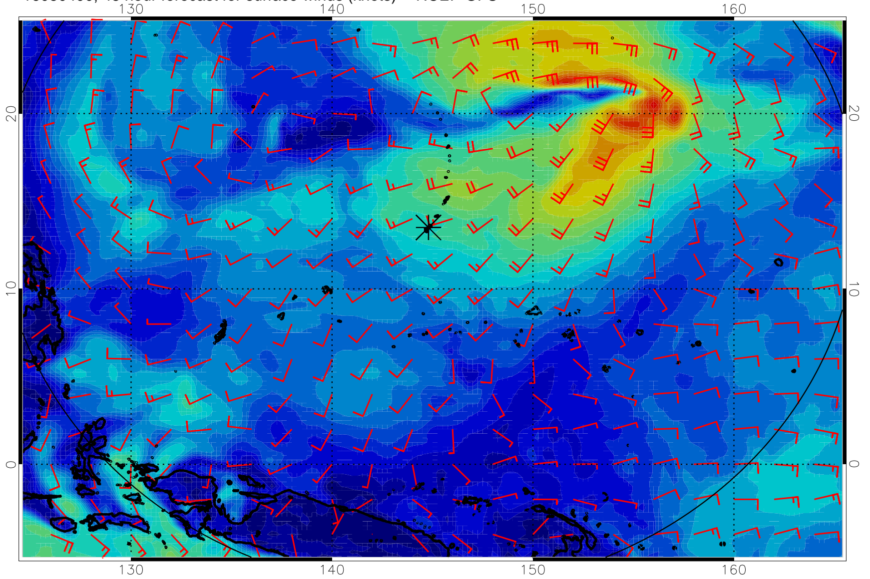
16080400, 48 hour forecast for surface winds (knots) -- NCEP GFS
