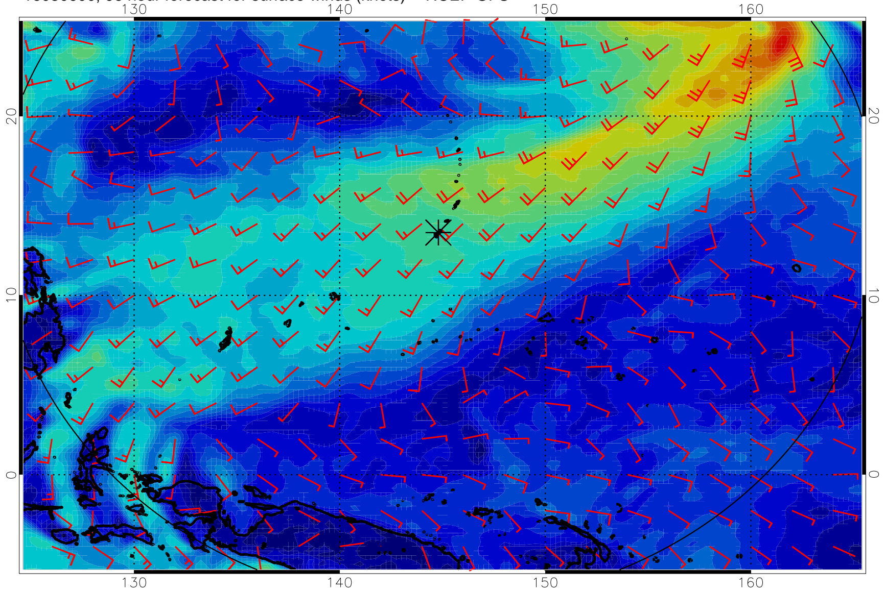
16080600, 96 hour forecast for surface winds (knots) -- NCEP GFS
