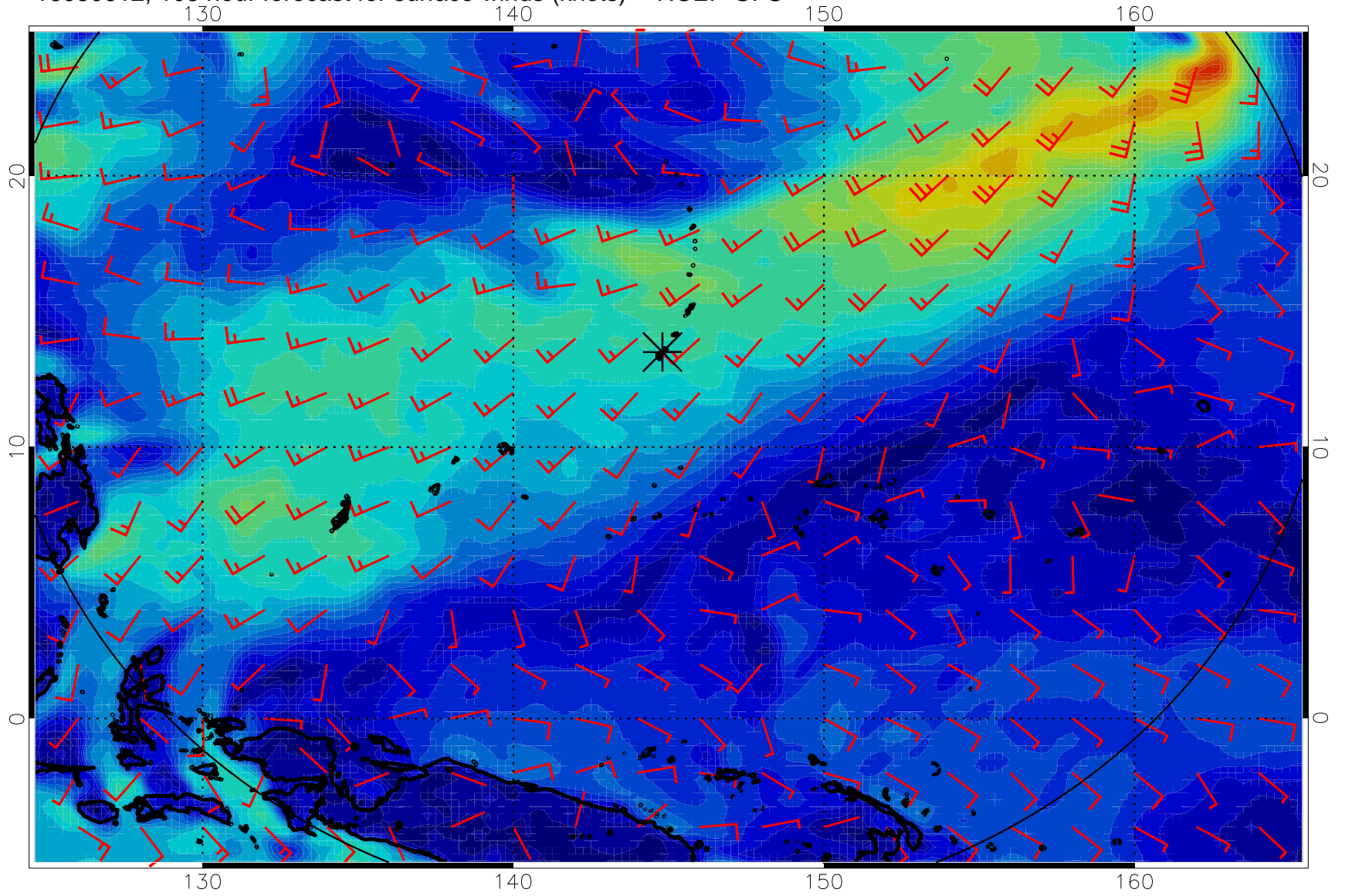
16080612, 108 hour forecast for surface winds (knots) -- NCEP GFS
