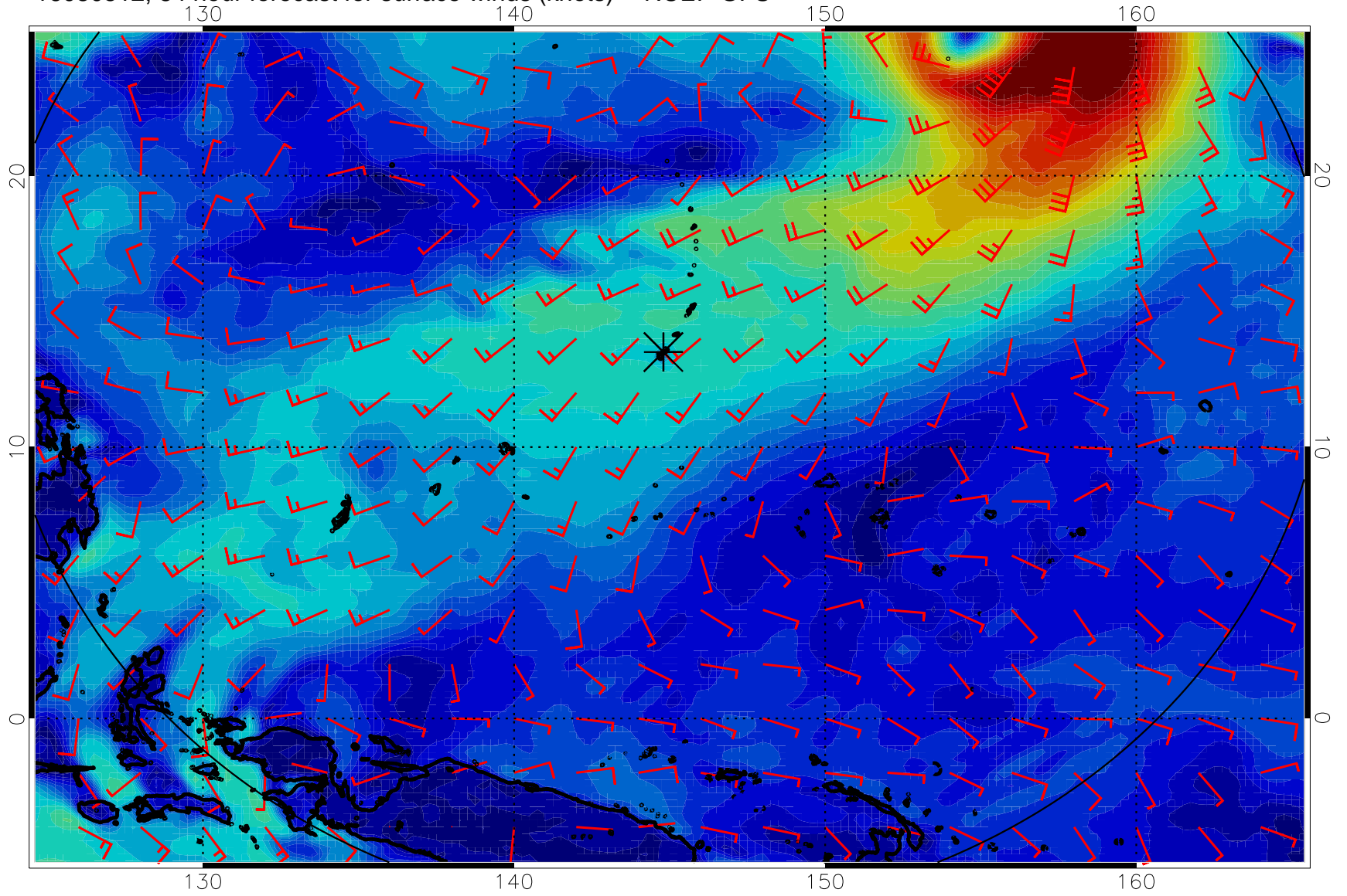
16080512, 84 hour forecast for surface winds (knots) -- NCEP GFS
