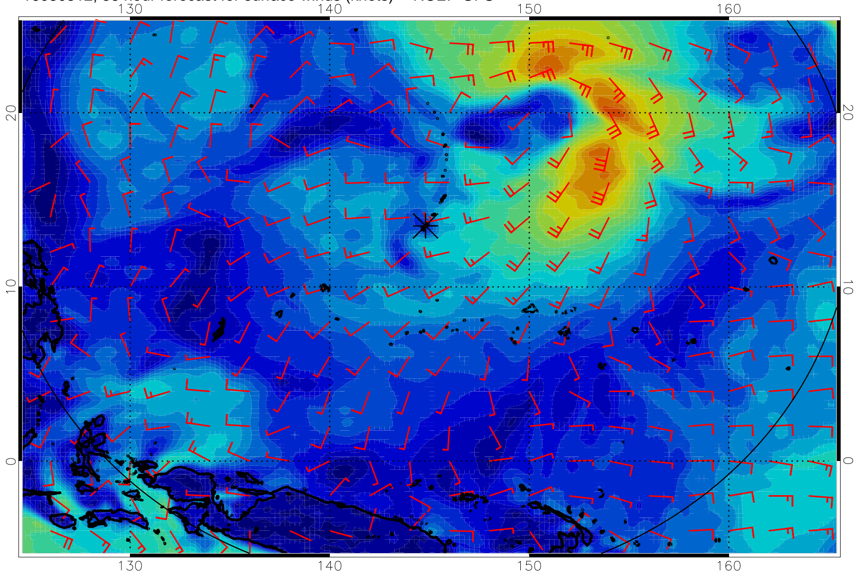
16080312, 36 hour forecast for surface winds (knots) -- NCEP GFS
