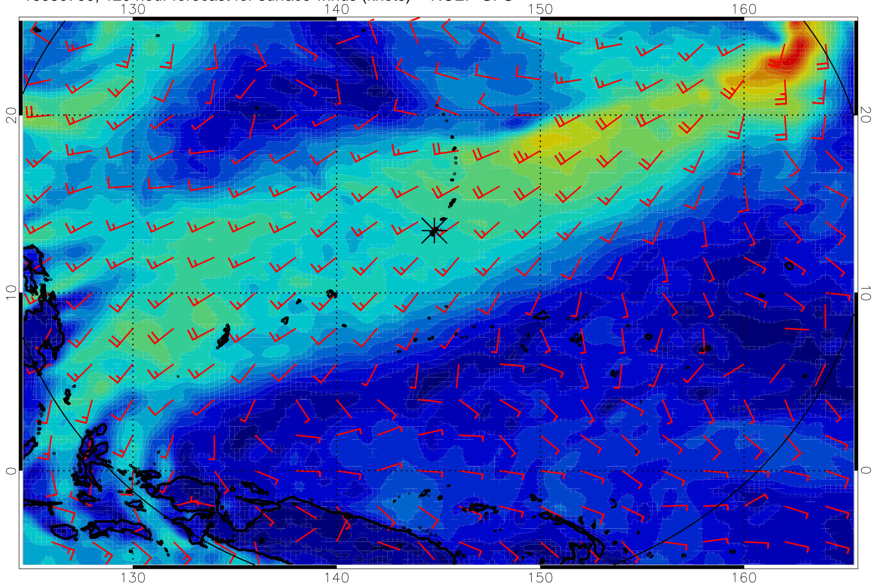
16080700, 120 hour forecast for surface winds (knots) -- NCEP GFS
