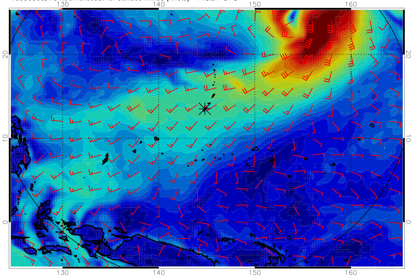
16080506, 78 hour forecast for surface winds (knots) -- NCEP GFS
