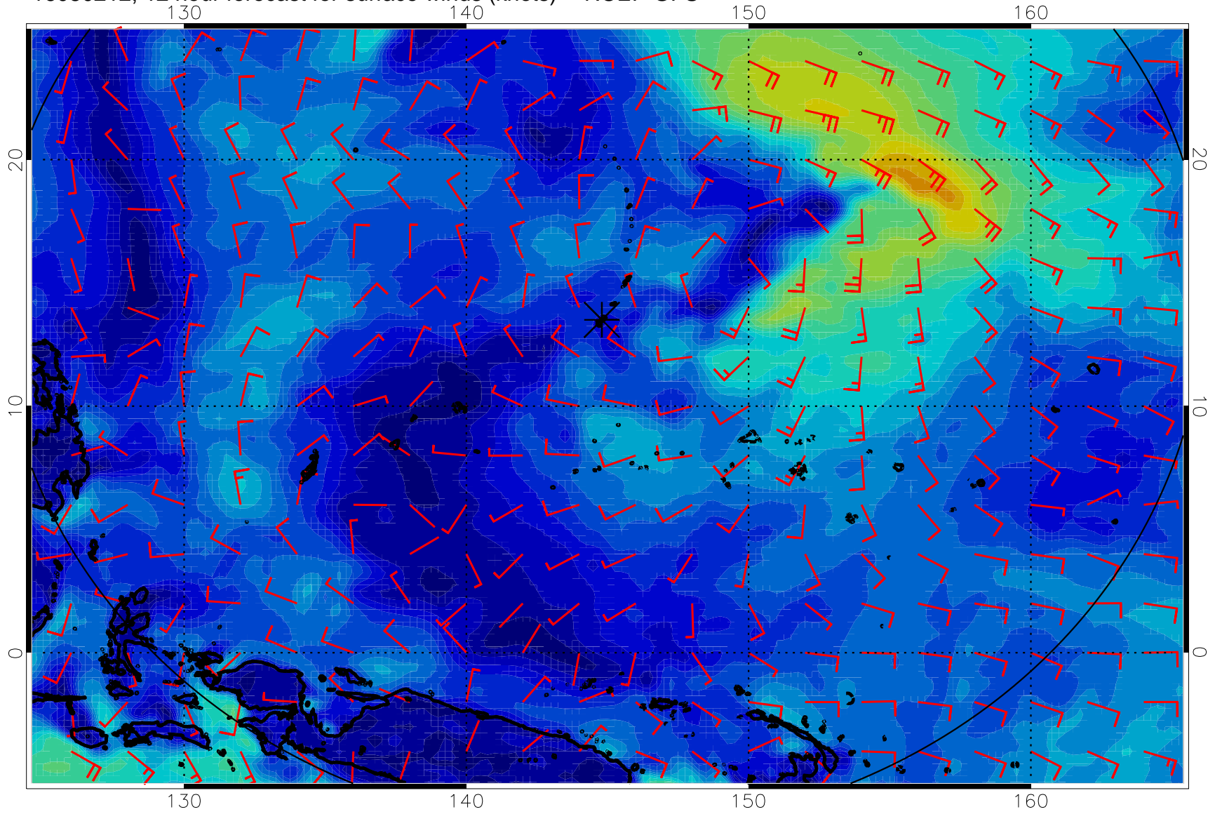
16080212, 12 hour forecast for surface winds (knots) -- NCEP GFS
