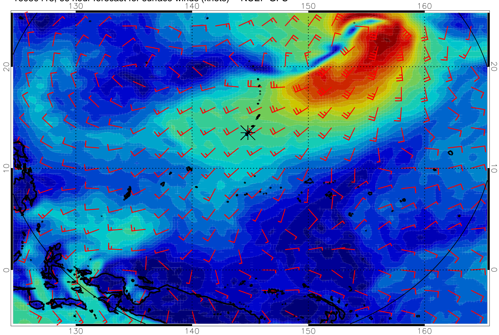
16080418, 66 hour forecast for surface winds (knots) -- NCEP GFS
