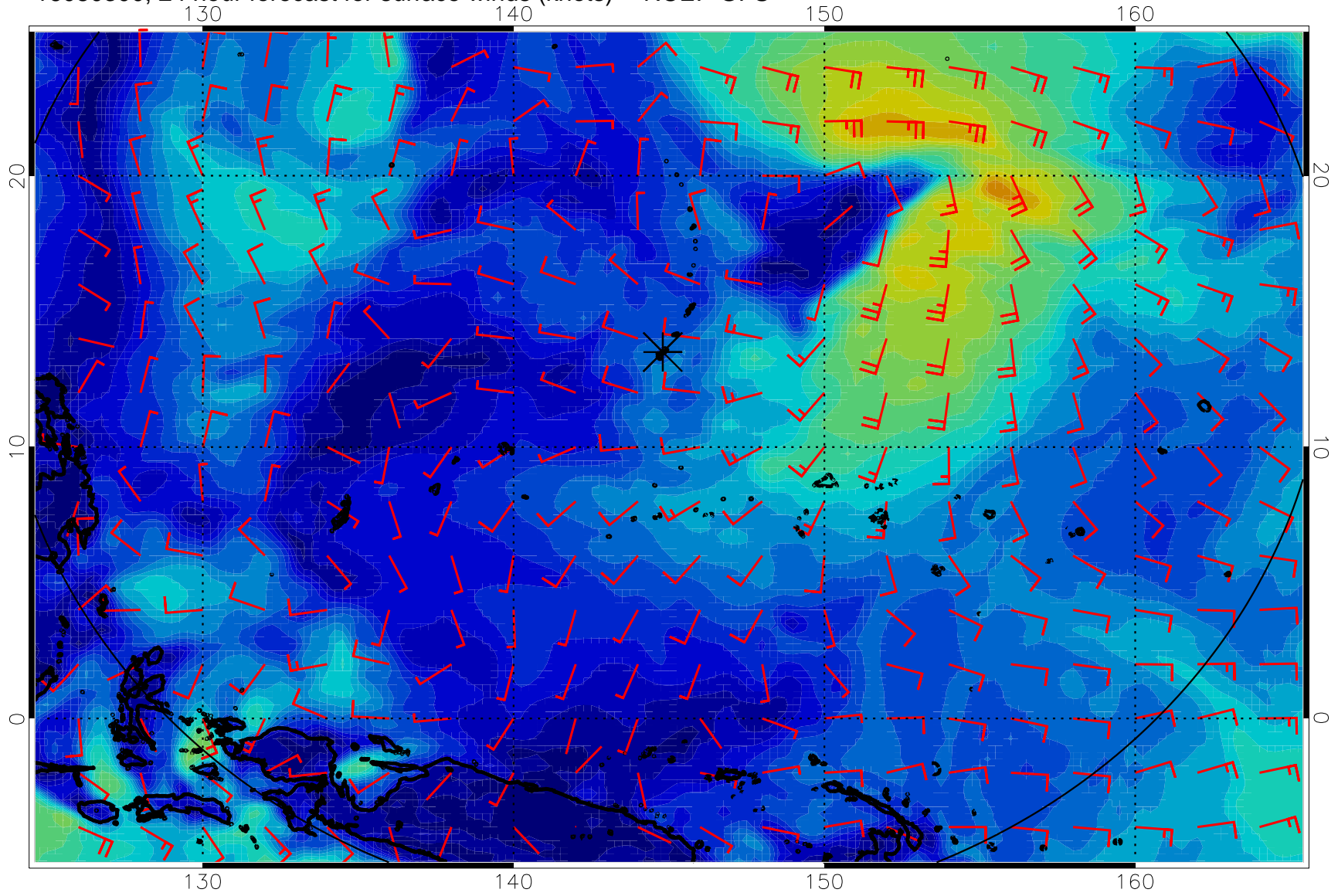
16080300, 24 hour forecast for surface winds (knots) -- NCEP GFS
