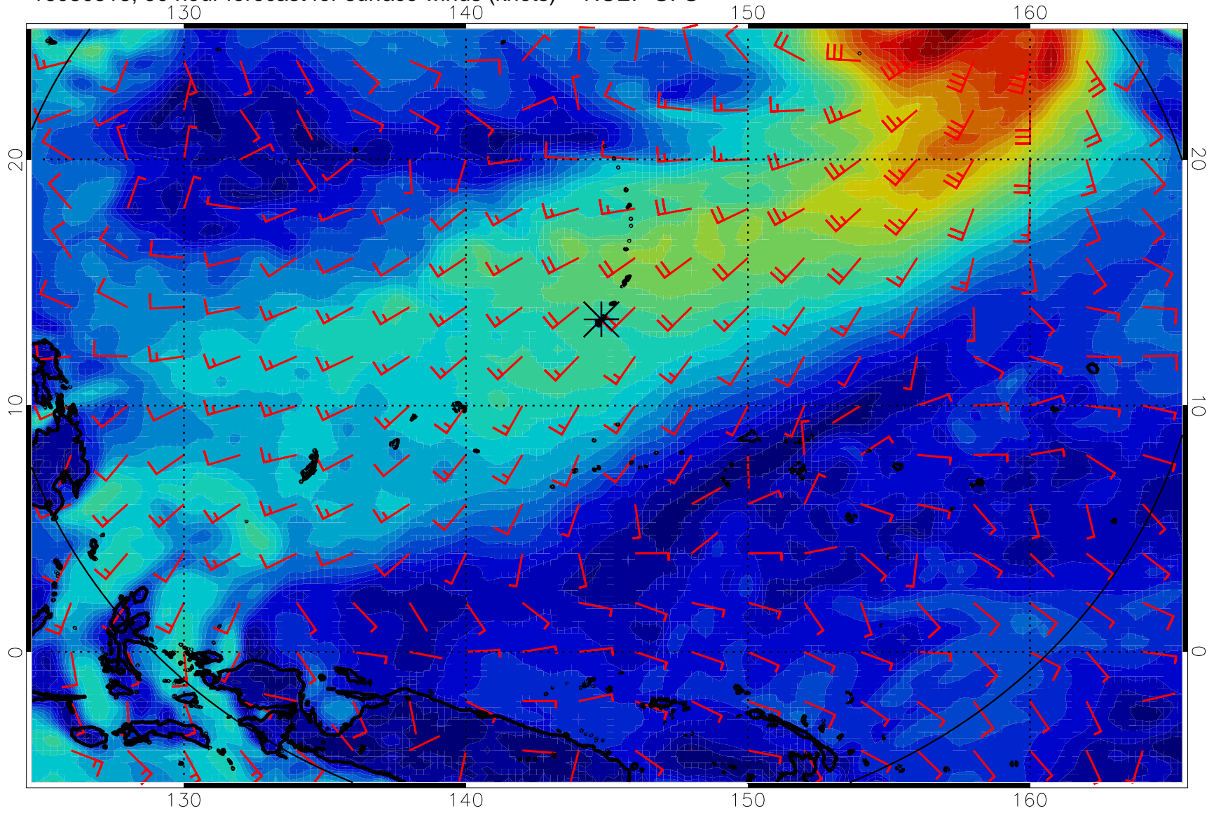
16080518, 90 hour forecast for surface winds (knots) -- NCEP GFS
