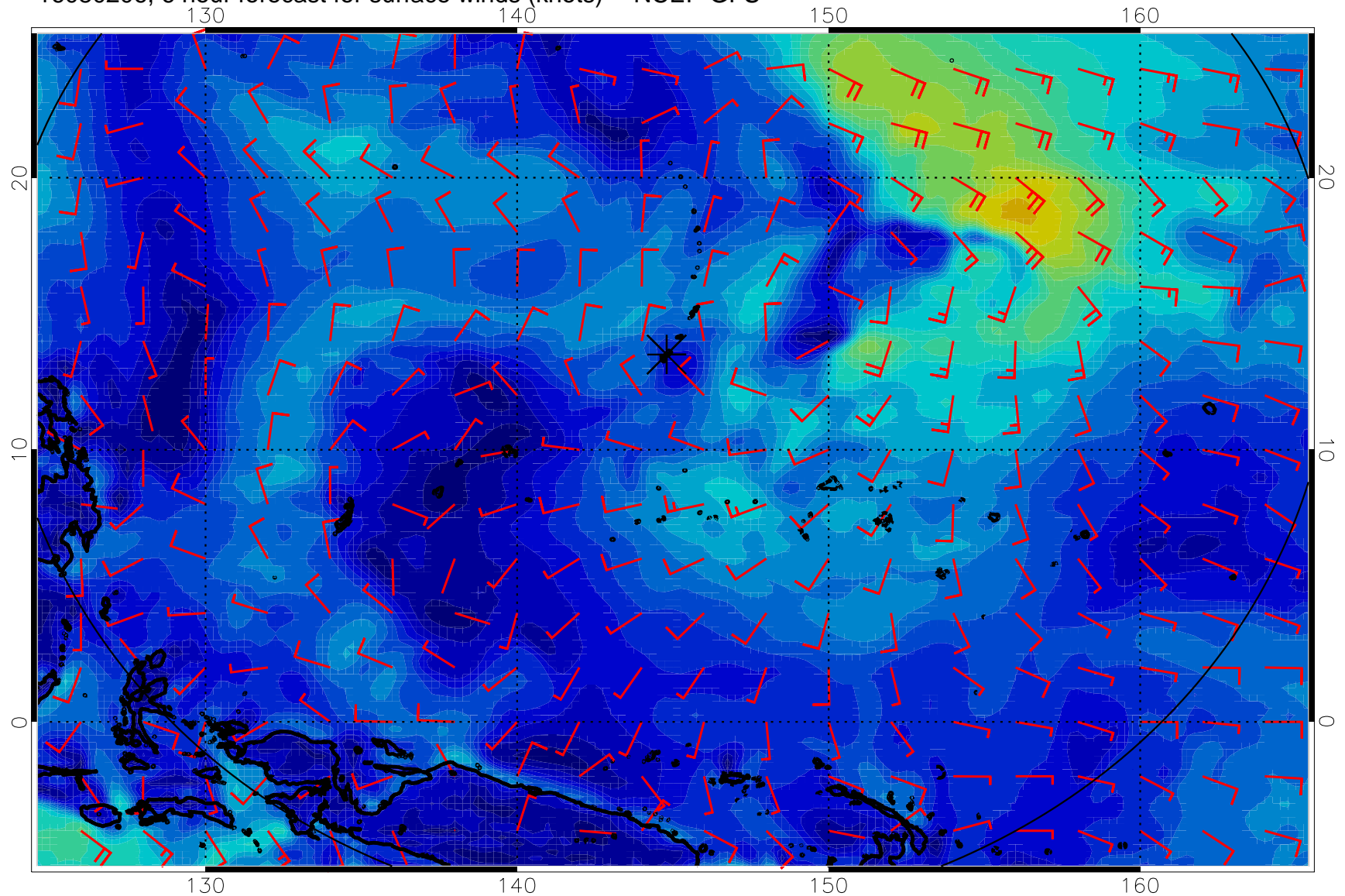
16080206, 6 hour forecast for surface winds (knots) -- NCEP GFS
