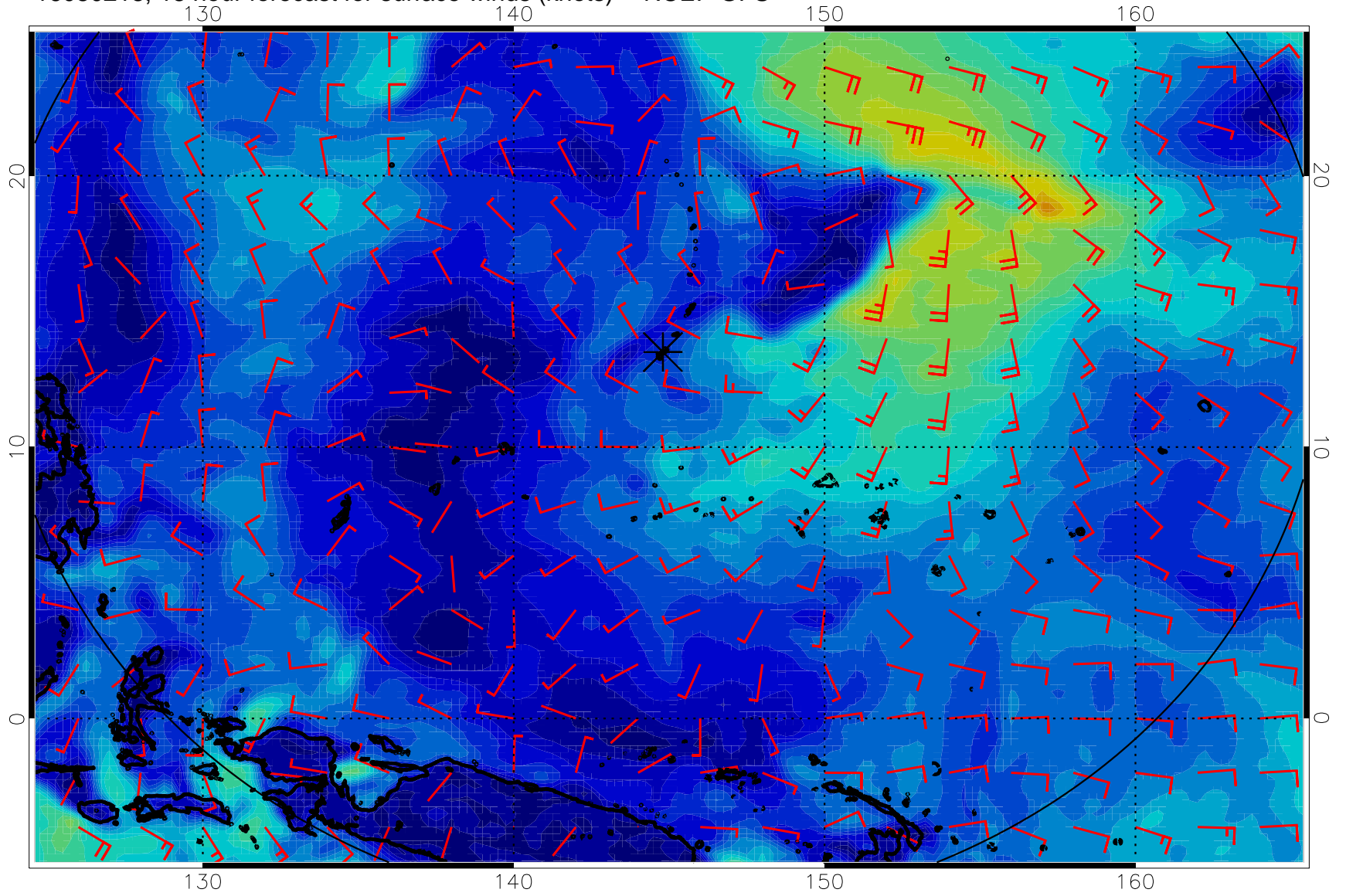
16080218, 18 hour forecast for surface winds (knots) -- NCEP GFS
