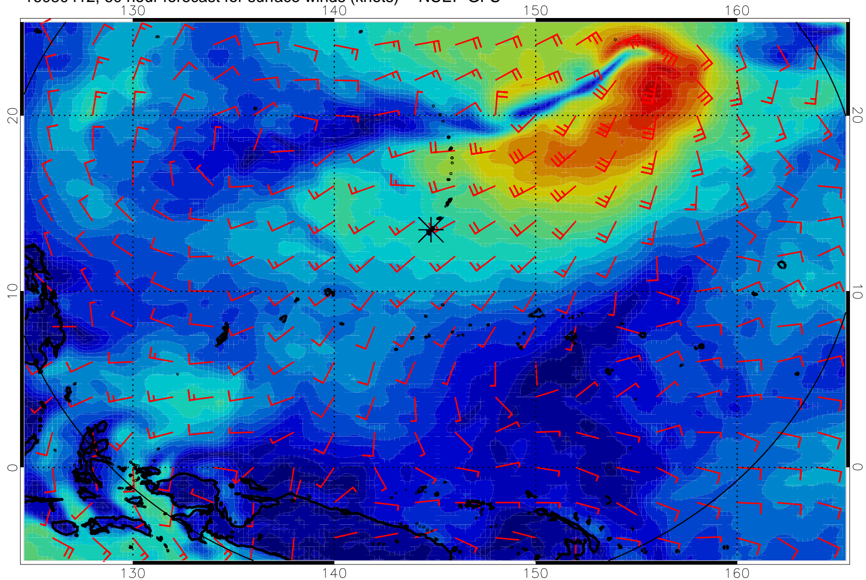
16080412, 60 hour forecast for surface winds (knots) -- NCEP GFS
