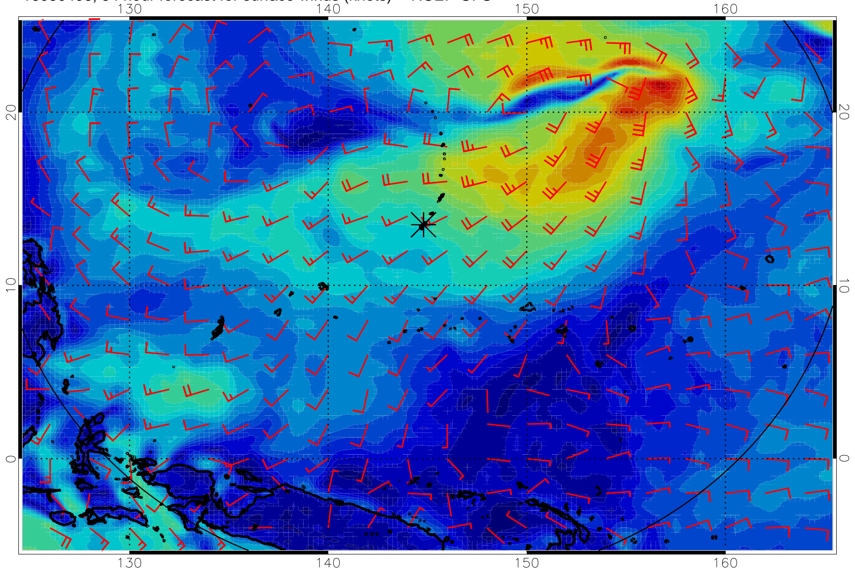
16080406, 54 hour forecast for surface winds (knots) -- NCEP GFS
