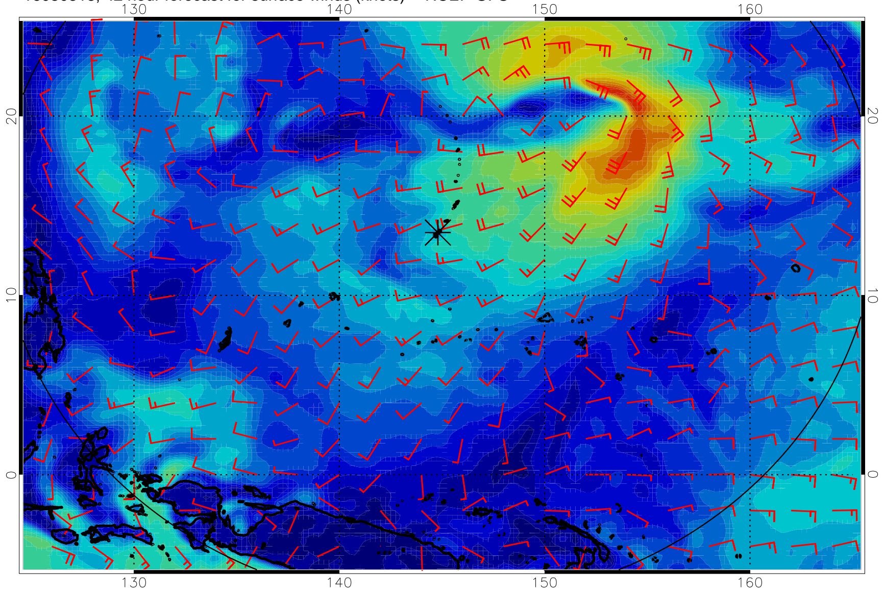
16080318, 42 hour forecast for surface winds (knots) -- NCEP GFS
