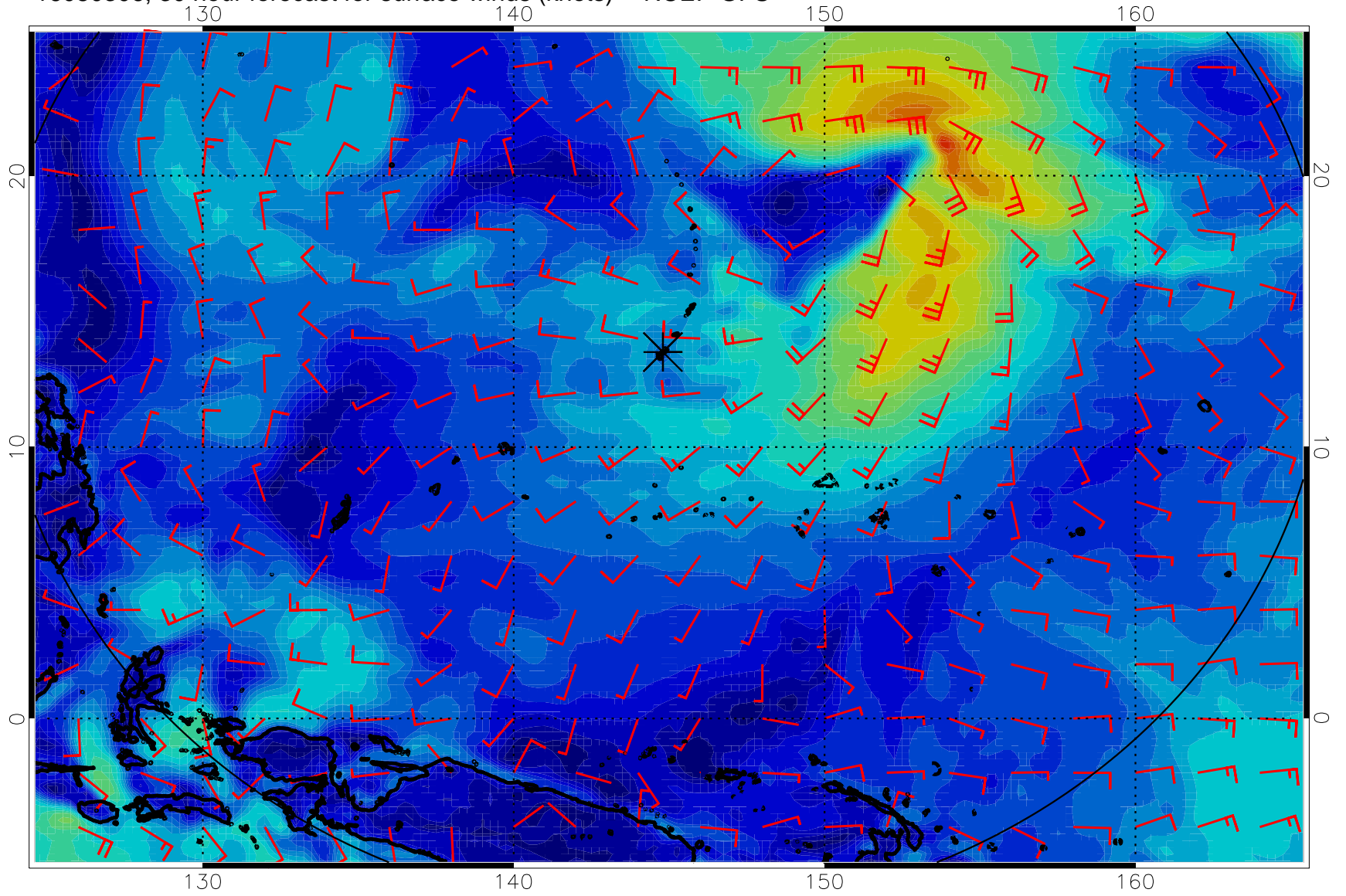
16080306, 30 hour forecast for surface winds (knots) -- NCEP GFS
