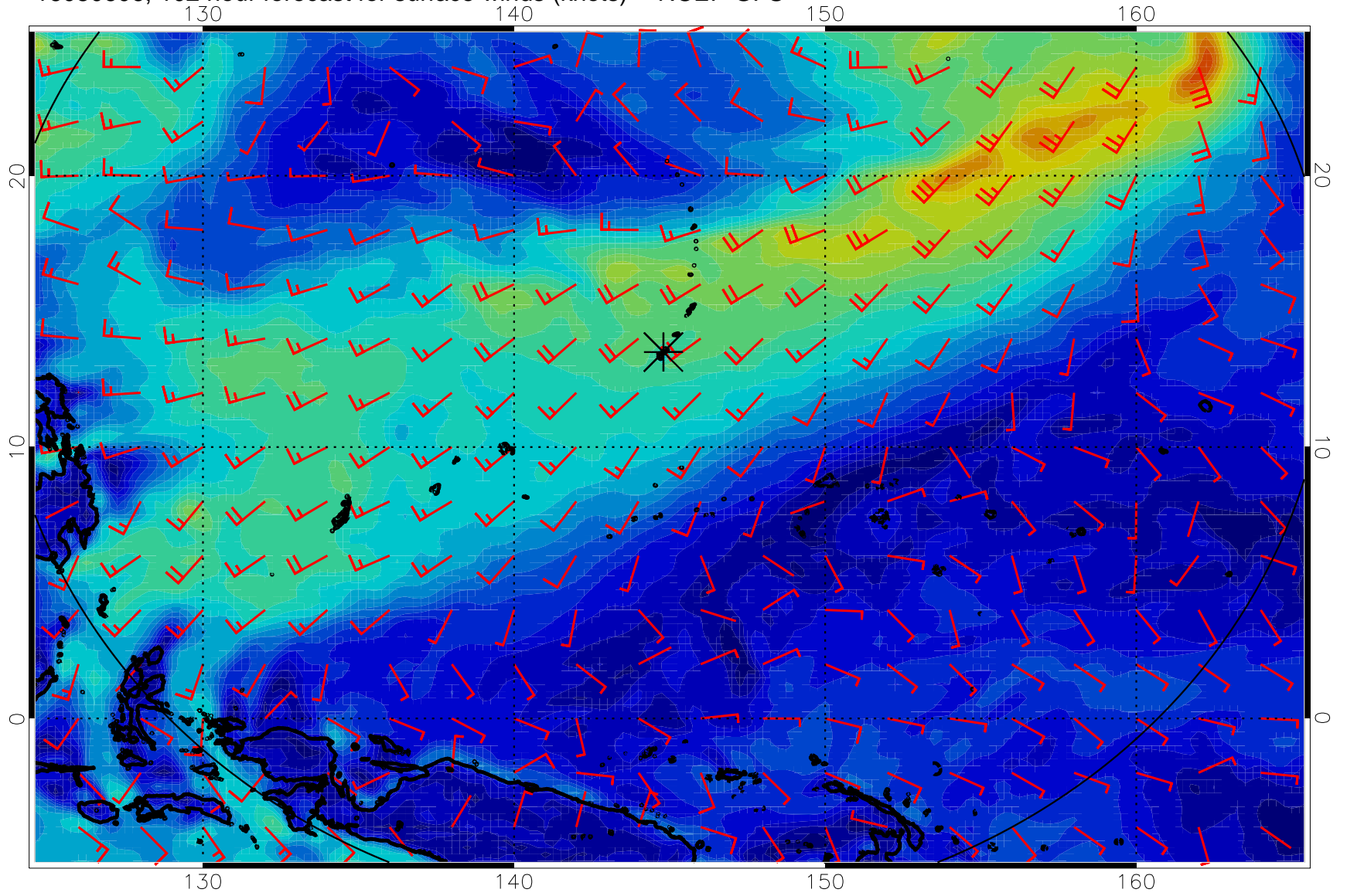
16080606, 102 hour forecast for surface winds (knots) -- NCEP GFS
