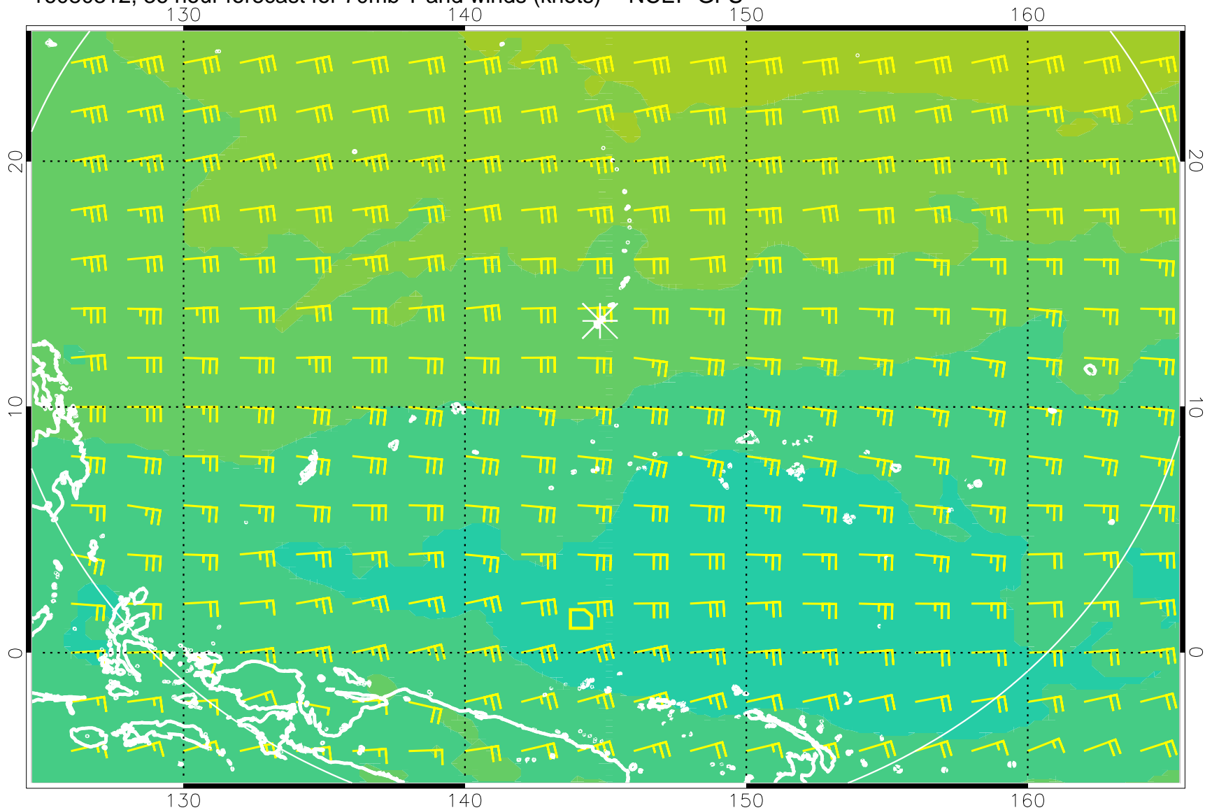
16080312, 36 hour forecast for 70mb T and winds (knots) -- NCEP GFS
