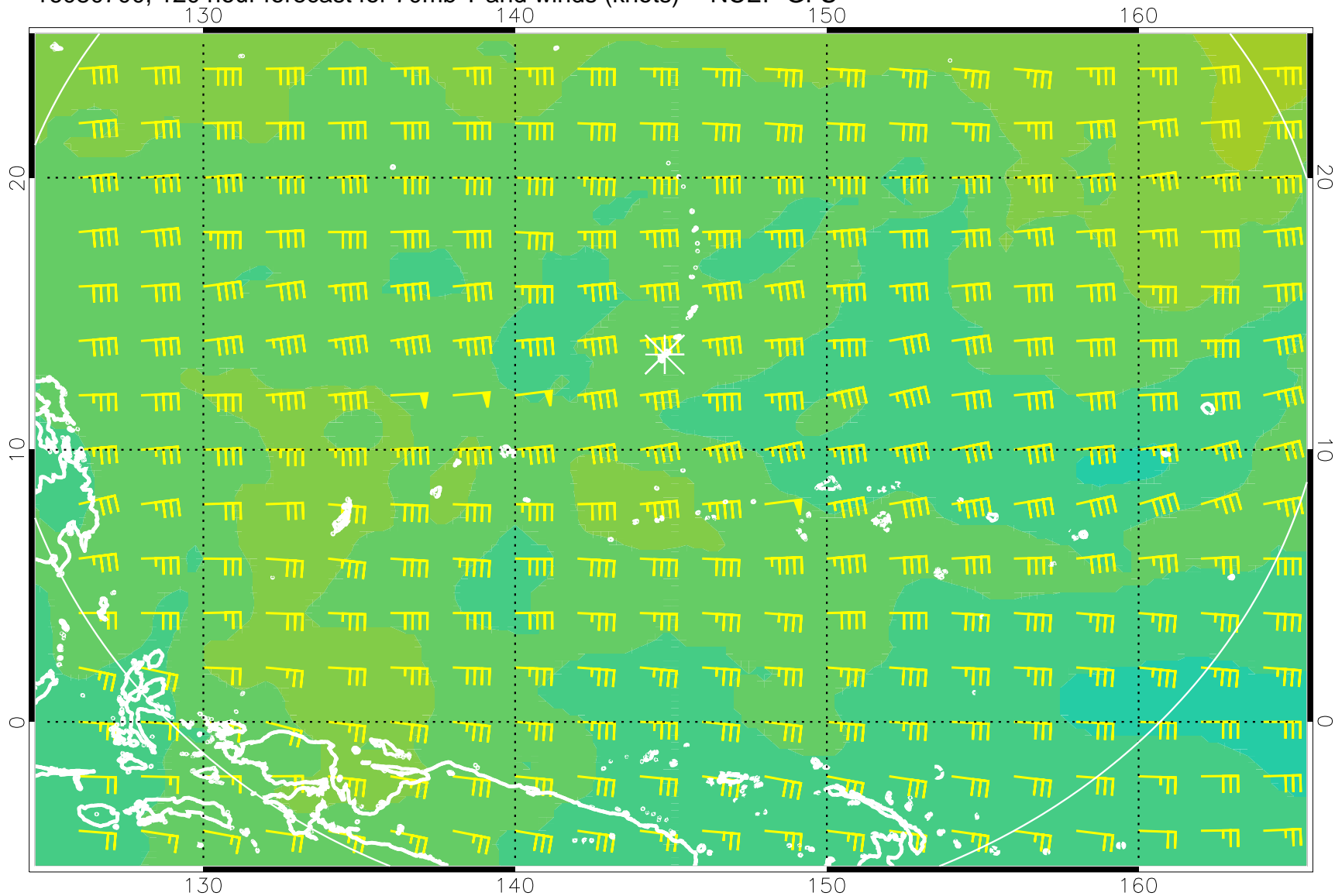
16080700, 120 hour forecast for 70mb T and winds (knots) -- NCEP GFS
