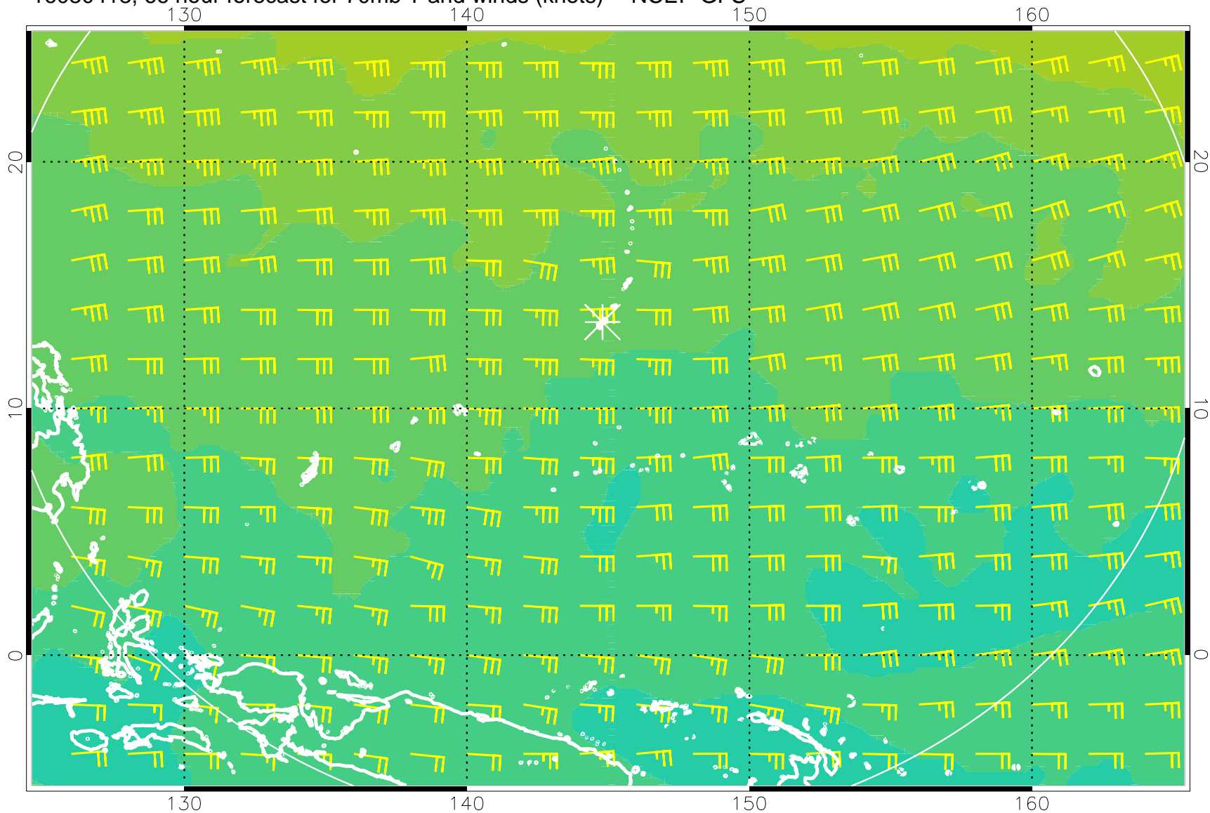
16080418, 66 hour forecast for 70mb T and winds (knots) -- NCEP GFS
