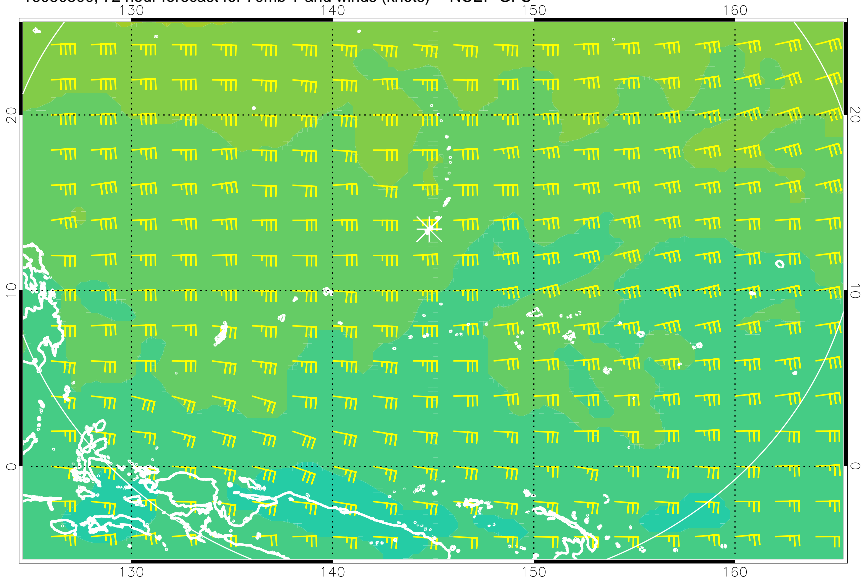
16080500, 72 hour forecast for 70mb T and winds (knots) -- NCEP GFS
