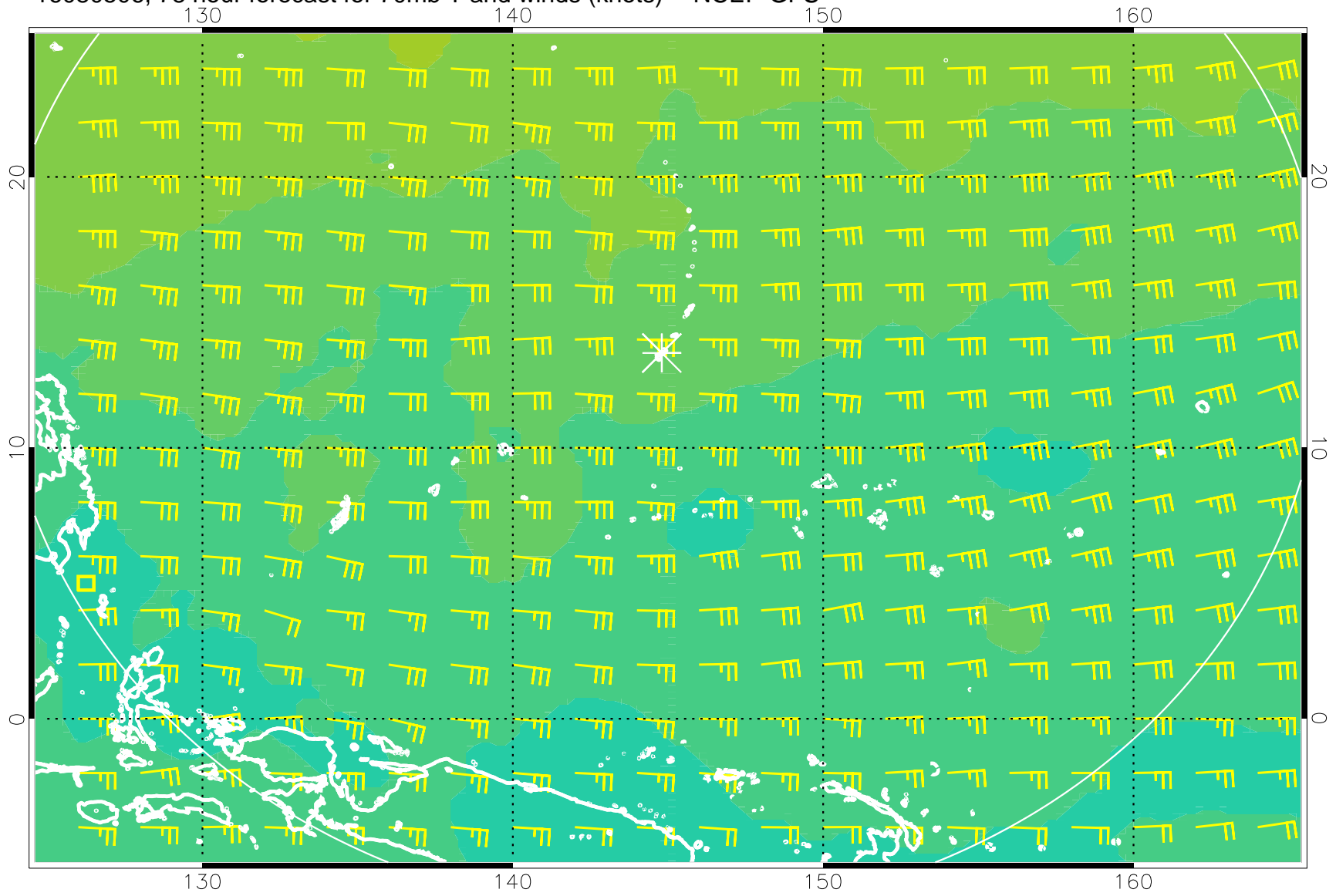
16080506, 78 hour forecast for 70mb T and winds (knots) -- NCEP GFS
