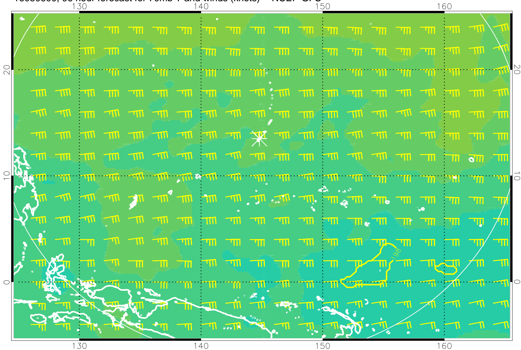
16080600, 96 hour forecast for 70mb T and winds (knots) -- NCEP GFS
