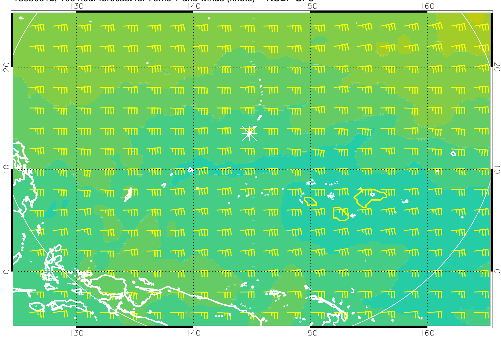
16080612, 108 hour forecast for 70mb T and winds (knots) -- NCEP GFS
