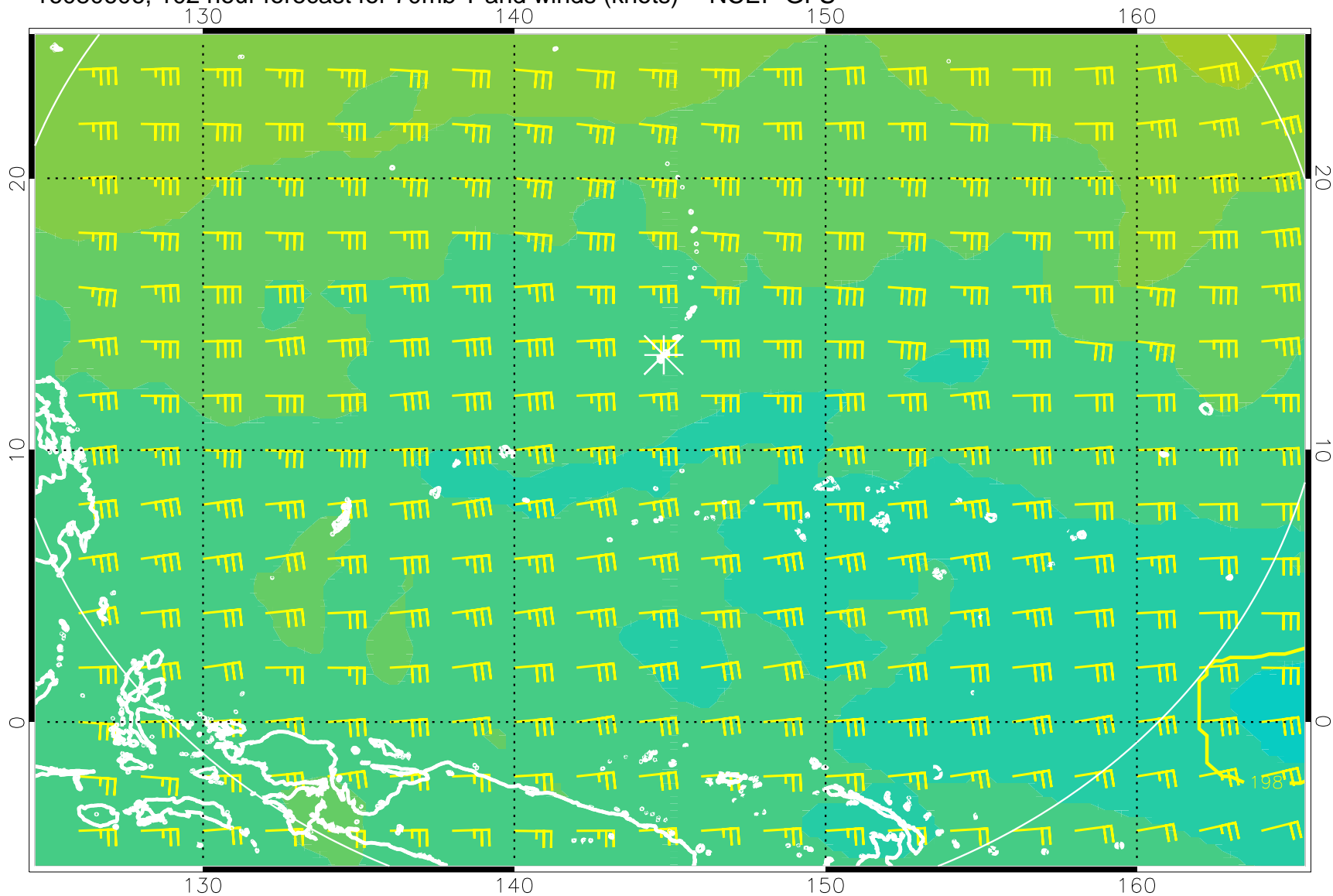
16080606, 102 hour forecast for 70mb T and winds (knots) -- NCEP GFS
