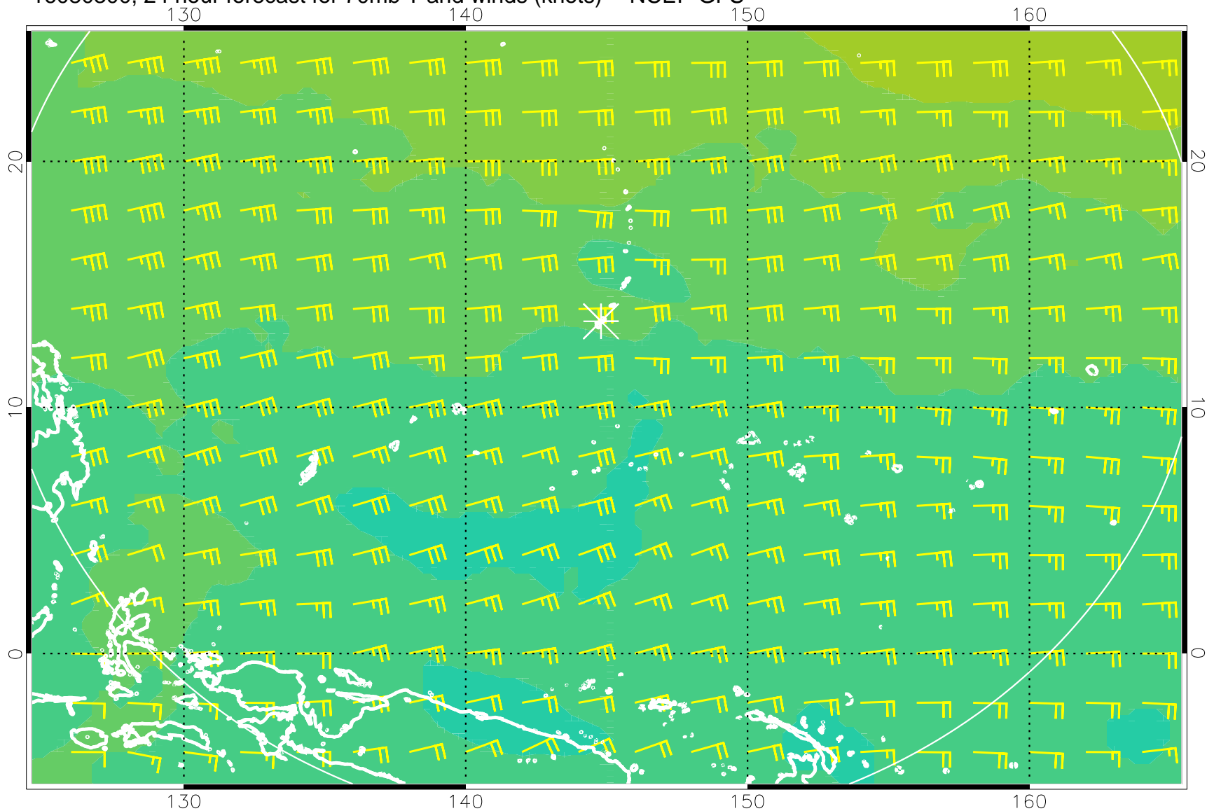
16080300, 24 hour forecast for 70mb T and winds (knots) -- NCEP GFS
