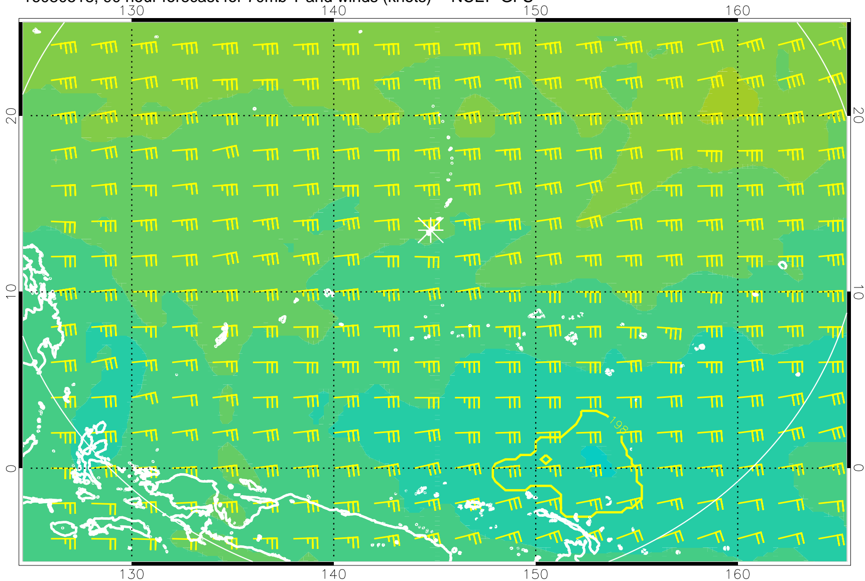
16080518, 90 hour forecast for 70mb T and winds (knots) -- NCEP GFS
