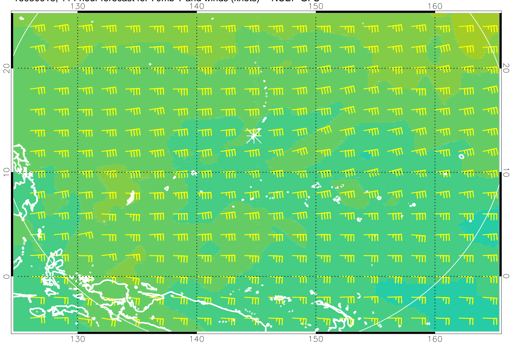
16080618, 114 hour forecast for 70mb T and winds (knots) -- NCEP GFS
