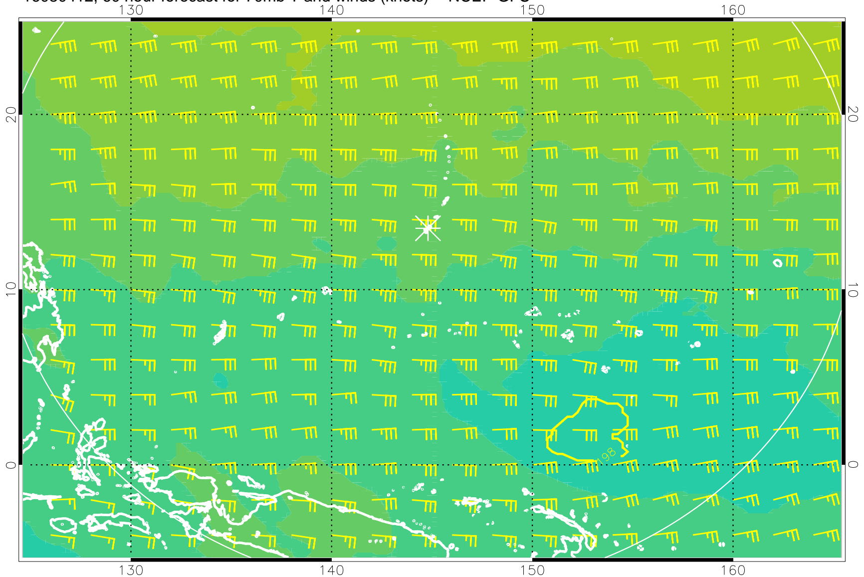
16080412, 60 hour forecast for 70mb T and winds (knots) -- NCEP GFS
