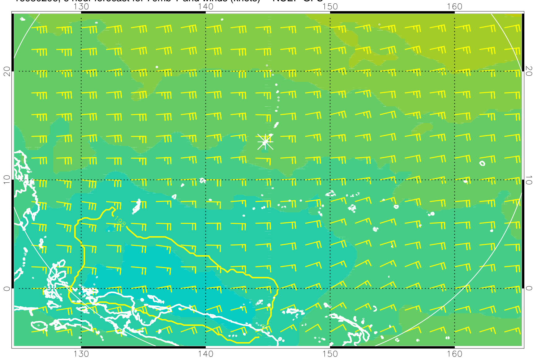
16080206, 6 hour forecast for 70mb T and winds (knots) -- NCEP GFS
