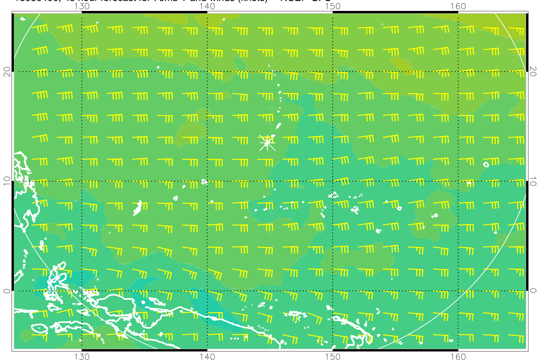
16080400, 48 hour forecast for 70mb T and winds (knots) -- NCEP GFS
