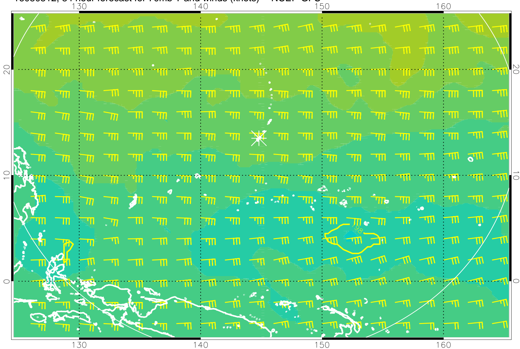
16080512, 84 hour forecast for 70mb T and winds (knots) -- NCEP GFS
