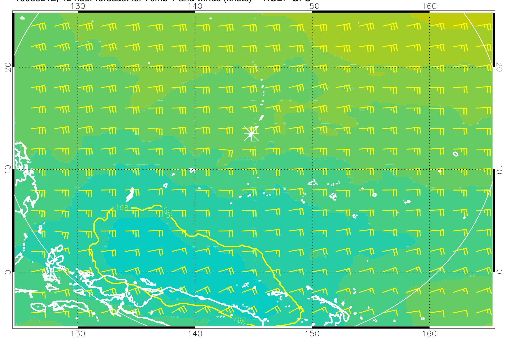
16080212, 12 hour forecast for 70mb T and winds (knots) -- NCEP GFS
