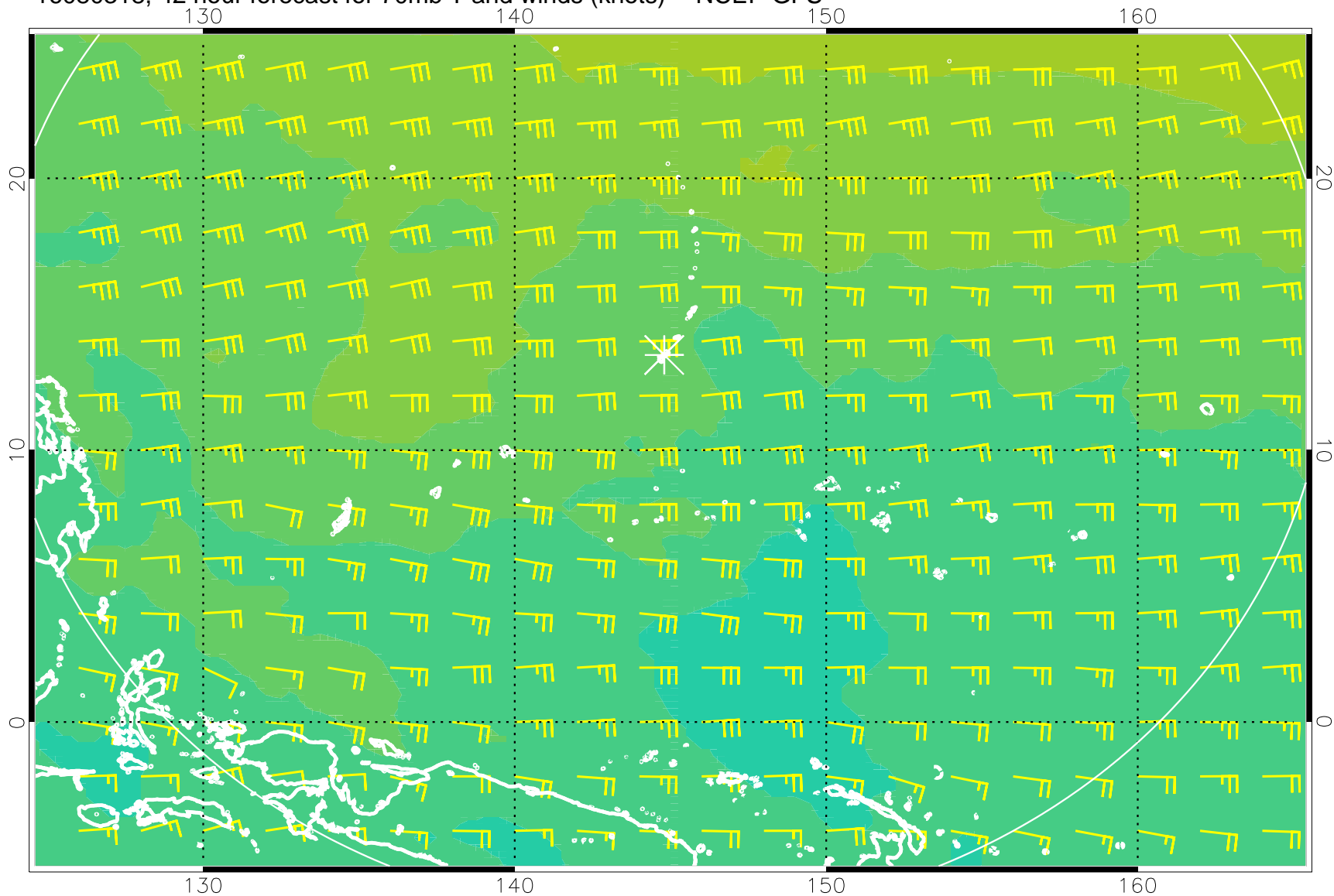
16080318, 42 hour forecast for 70mb T and winds (knots) -- NCEP GFS
