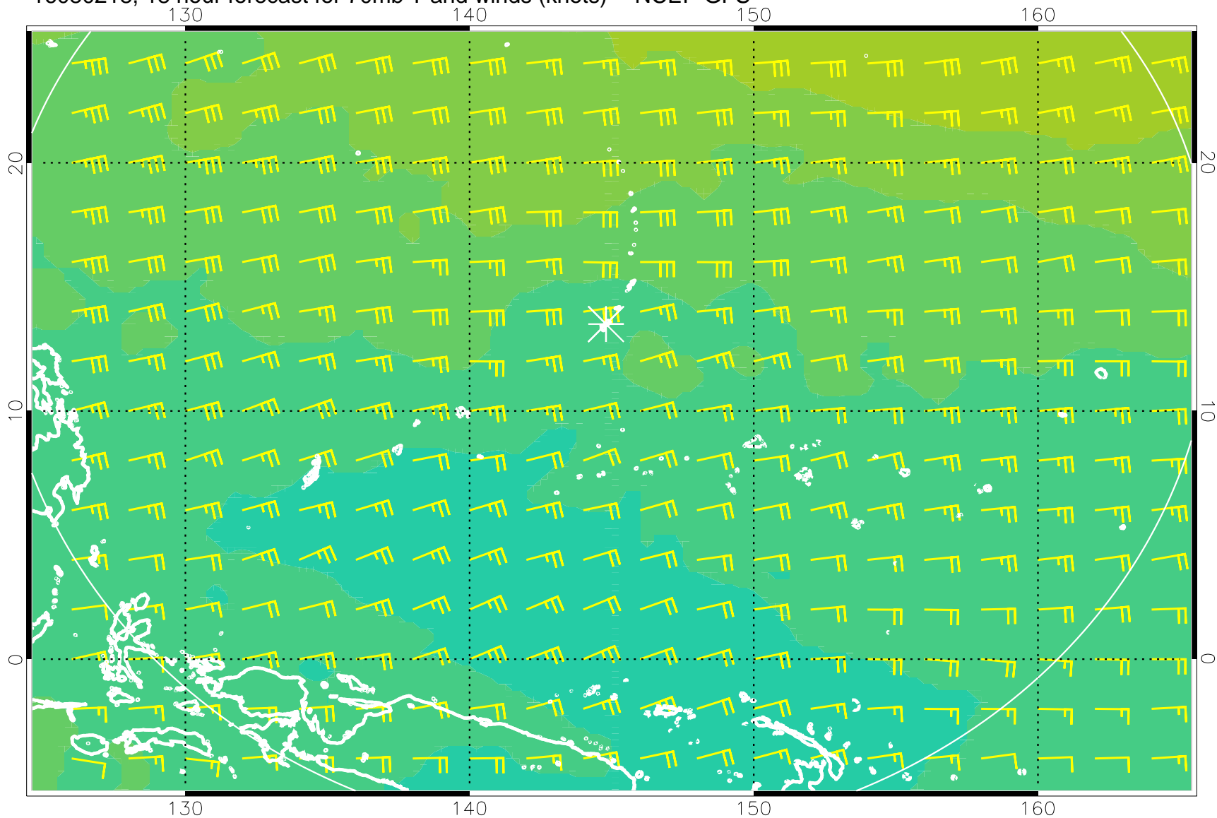
16080218, 18 hour forecast for 70mb T and winds (knots) -- NCEP GFS
