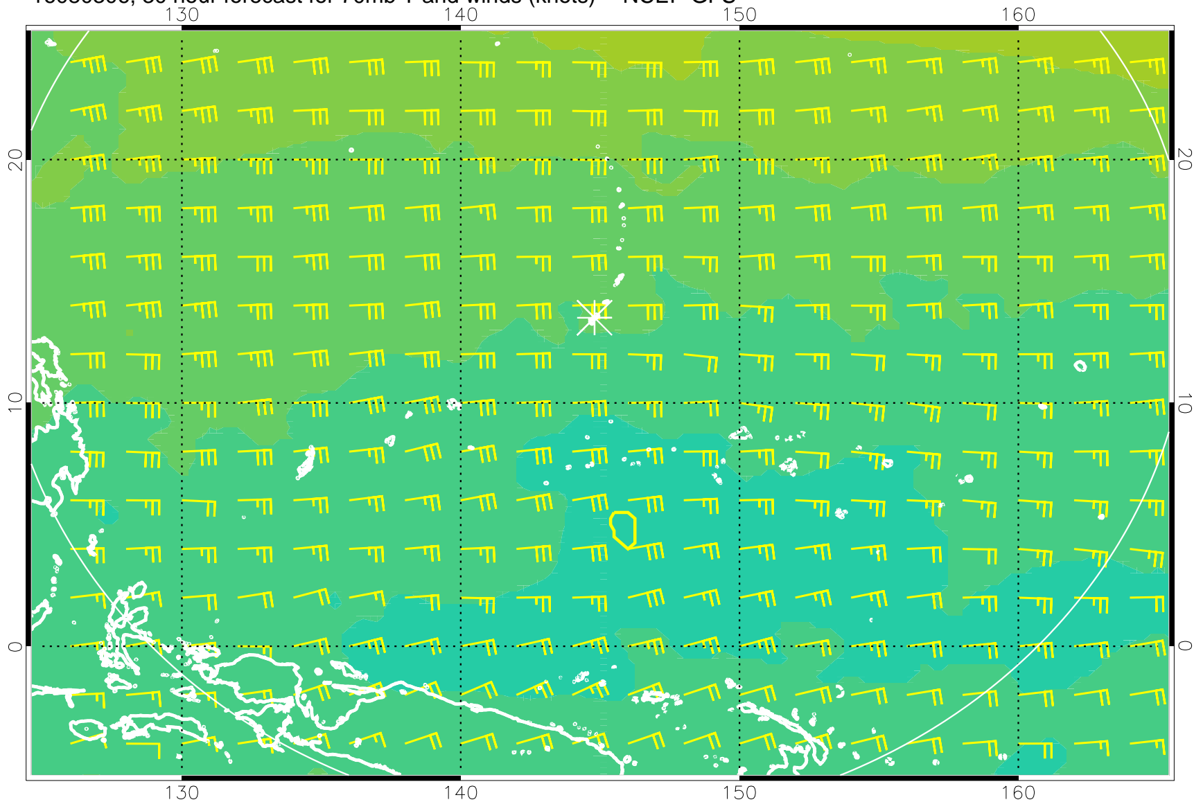
16080306, 30 hour forecast for 70mb T and winds (knots) -- NCEP GFS
