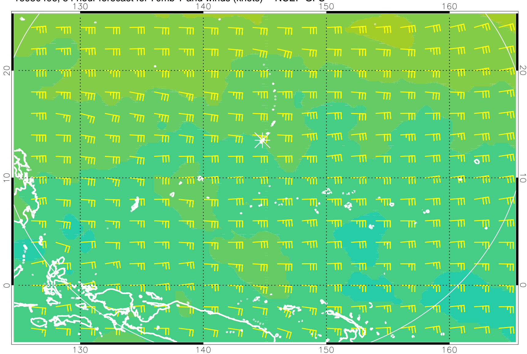
16080406, 54 hour forecast for 70mb T and winds (knots) -- NCEP GFS
