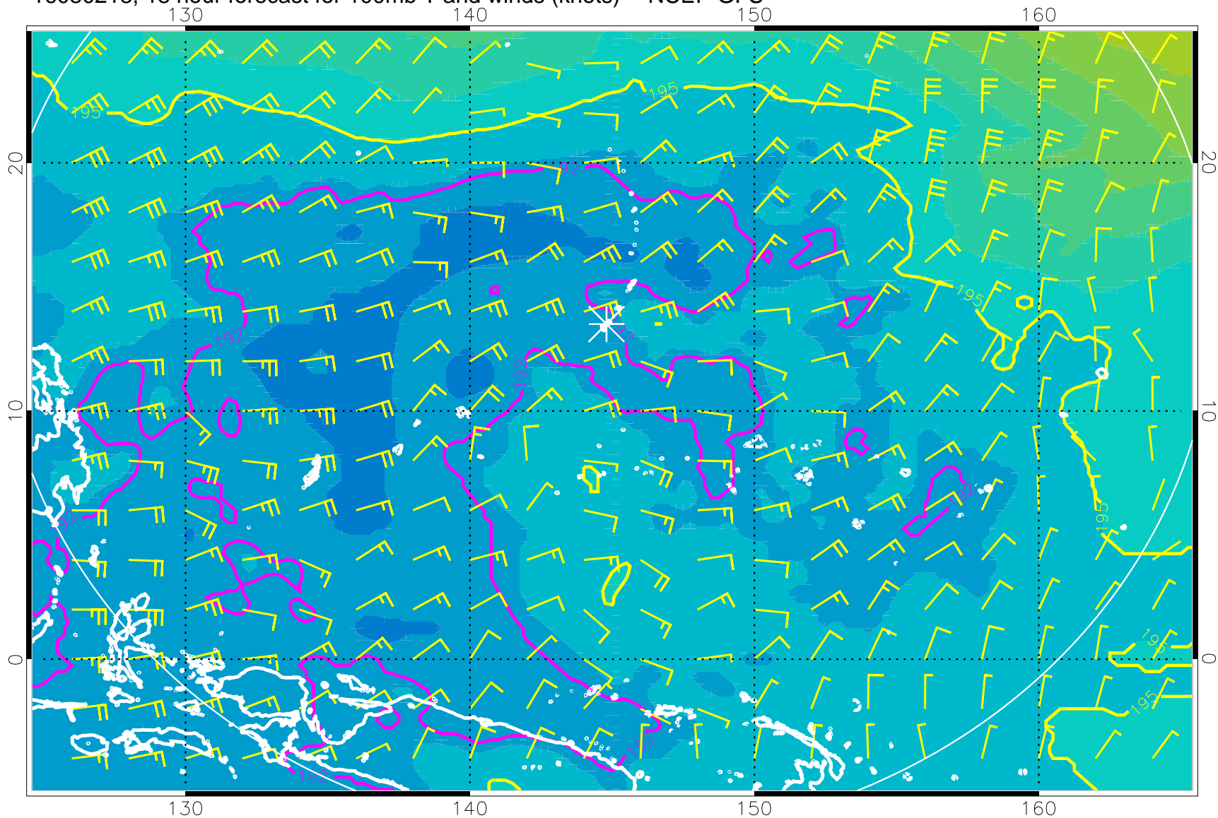
16080218, 18 hour forecast for 100mb T and winds (knots) -- NCEP GFS
