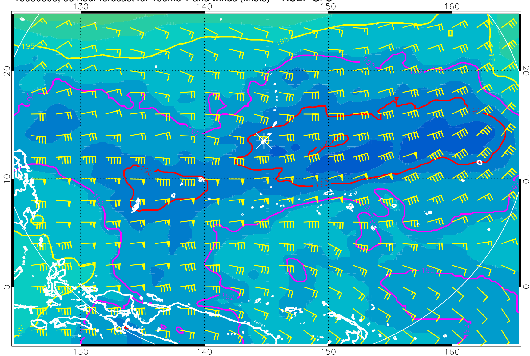
16080600, 96 hour forecast for 100mb T and winds (knots) -- NCEP GFS
