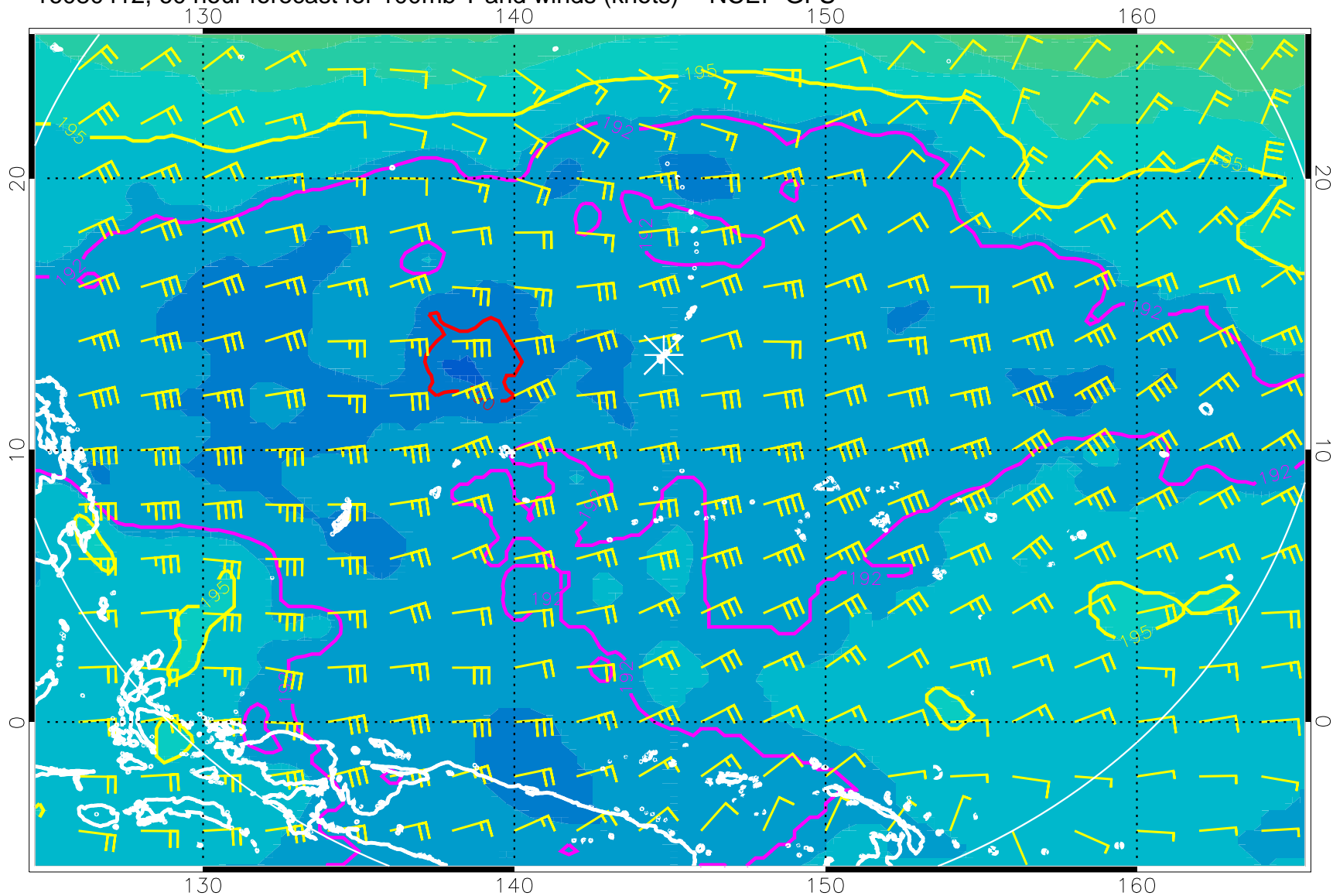
16080412, 60 hour forecast for 100mb T and winds (knots) -- NCEP GFS
