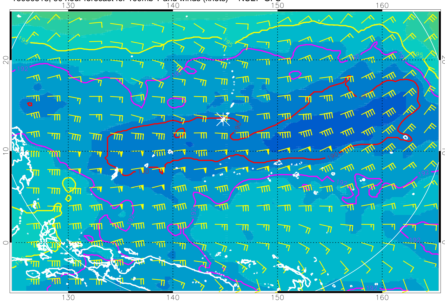
16080518, 90 hour forecast for 100mb T and winds (knots) -- NCEP GFS
