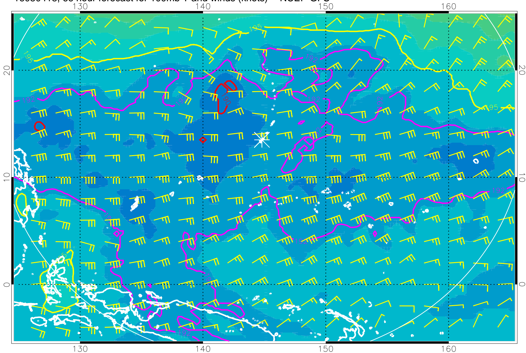
16080418, 66 hour forecast for 100mb T and winds (knots) -- NCEP GFS
