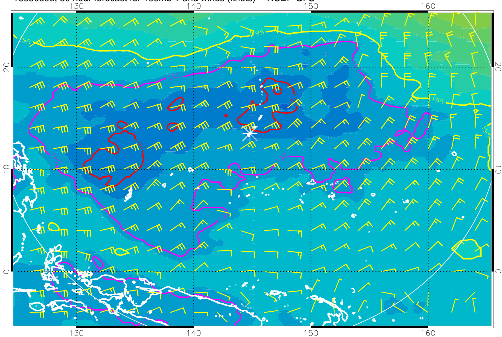
16080306, 30 hour forecast for 100mb T and winds (knots) -- NCEP GFS
