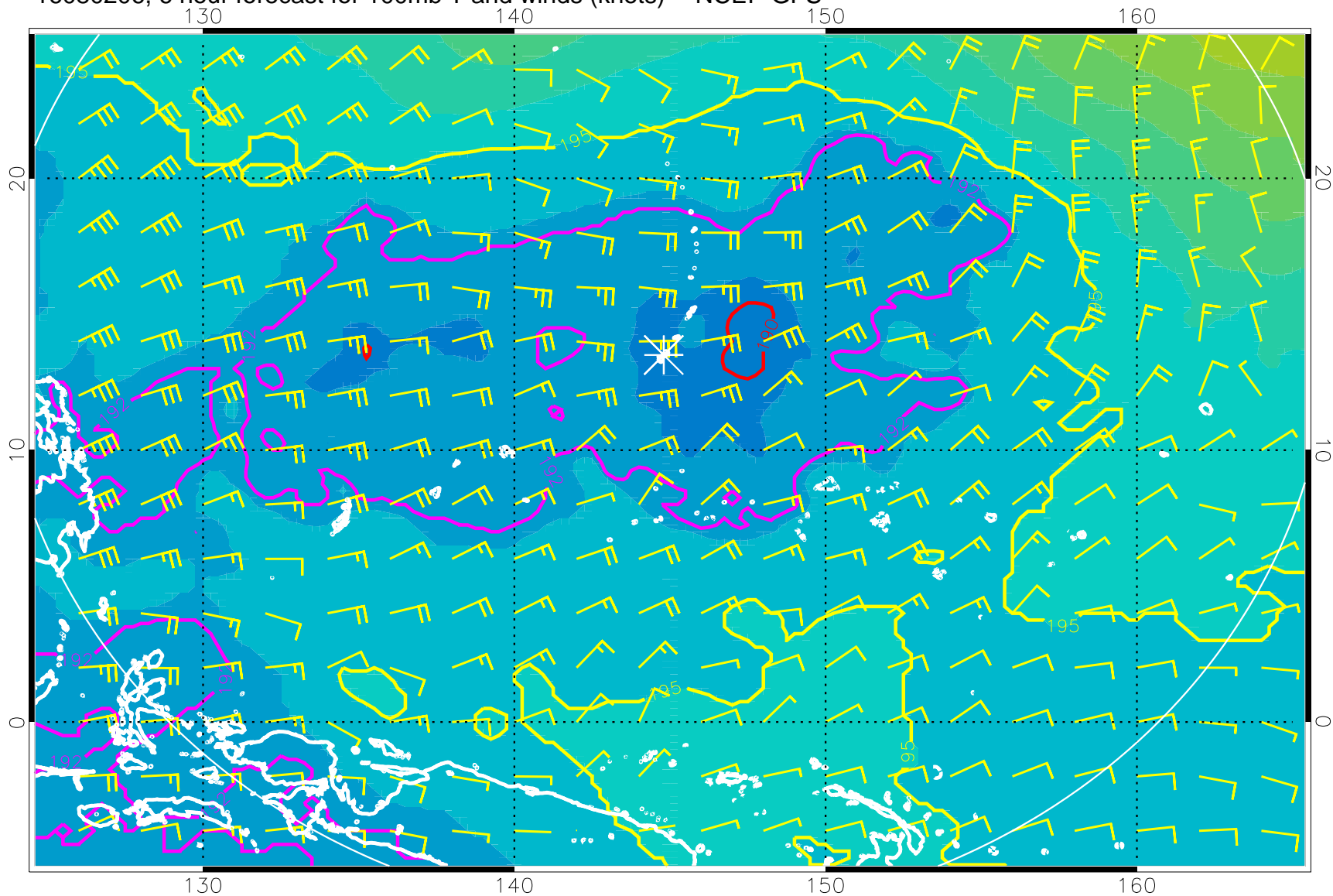
16080206, 6 hour forecast for 100mb T and winds (knots) -- NCEP GFS
