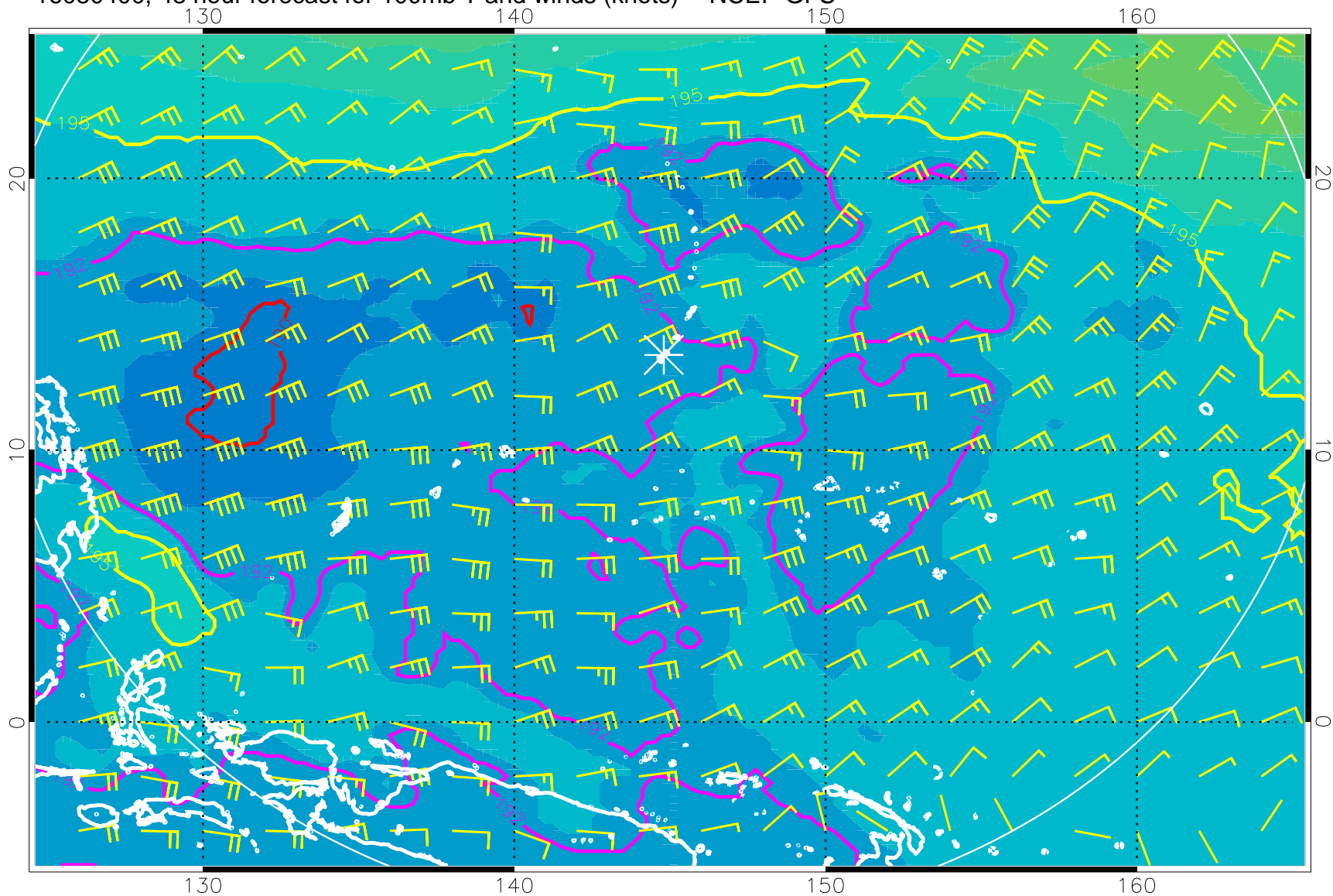
16080400, 48 hour forecast for 100mb T and winds (knots) -- NCEP GFS
