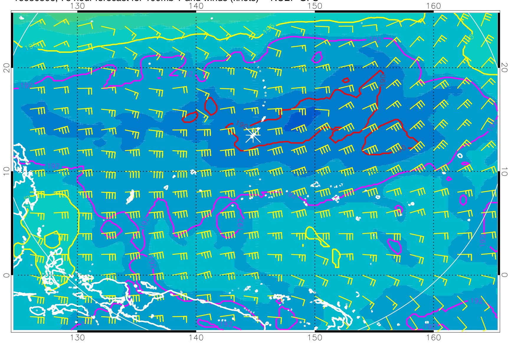
16080506, 78 hour forecast for 100mb T and winds (knots) -- NCEP GFS
