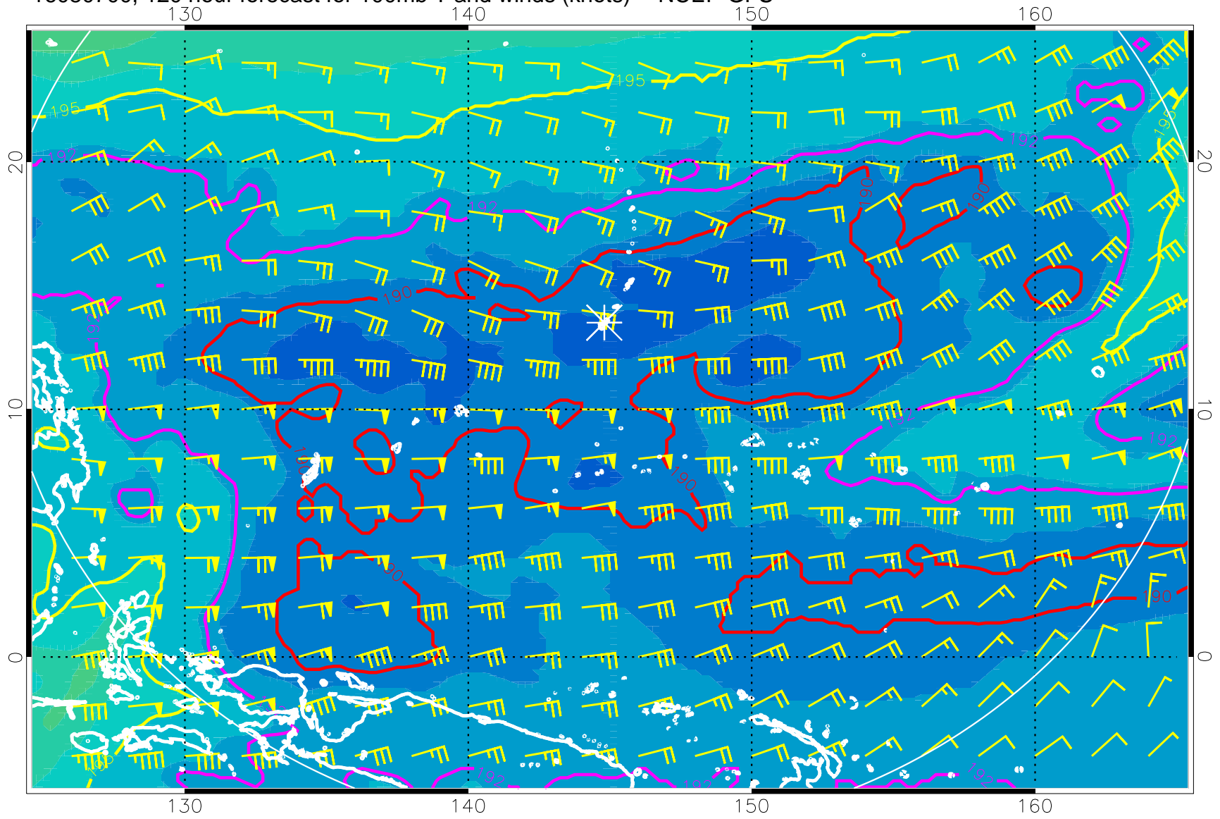
16080700, 120 hour forecast for 100mb T and winds (knots) -- NCEP GFS
