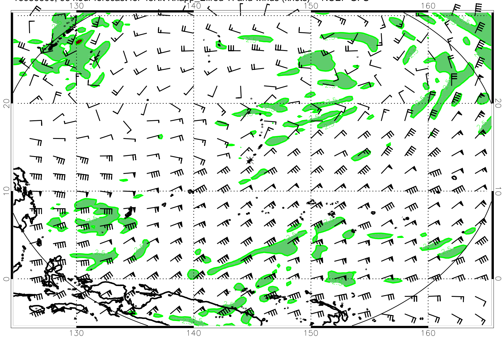
16080600, 96 hour forecast for 45Kft Knapp_Ellrod TI and winds (knots) -- NCEP GFS
