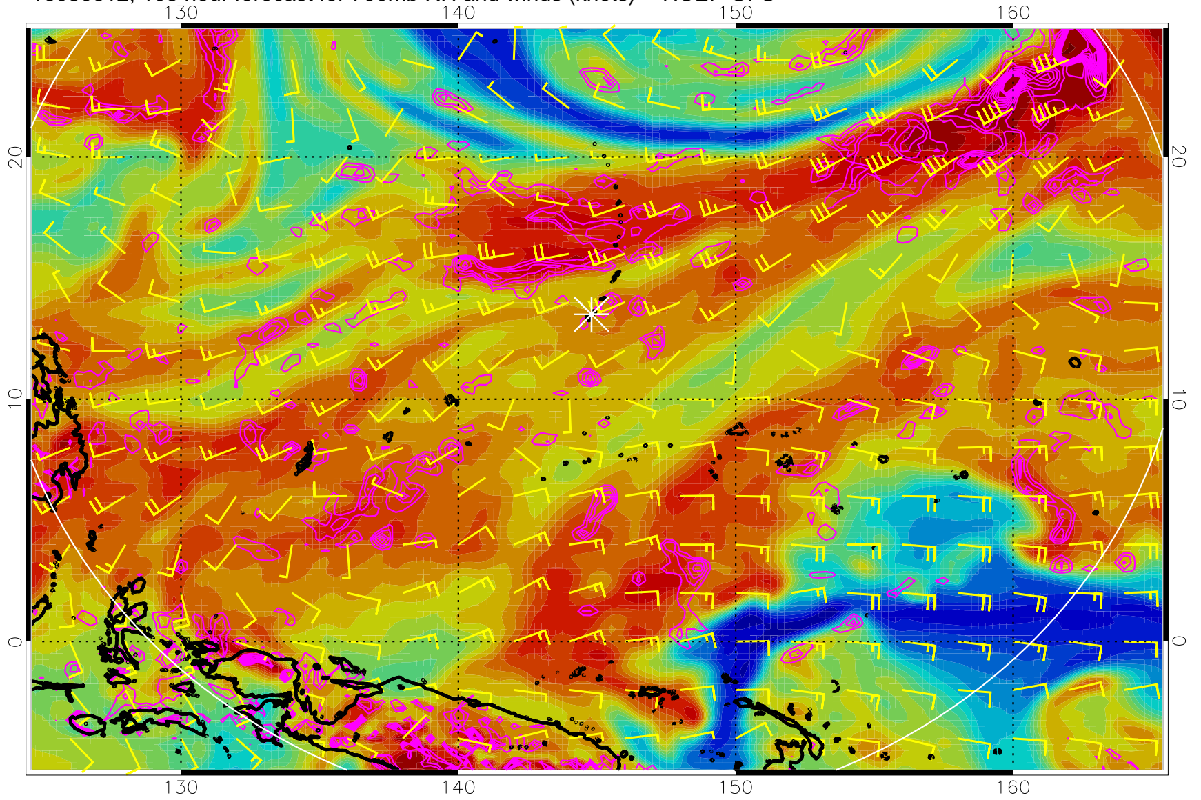
16080612, 108 hour forecast for 700mb RH and winds (knots) -- NCEP GFS
