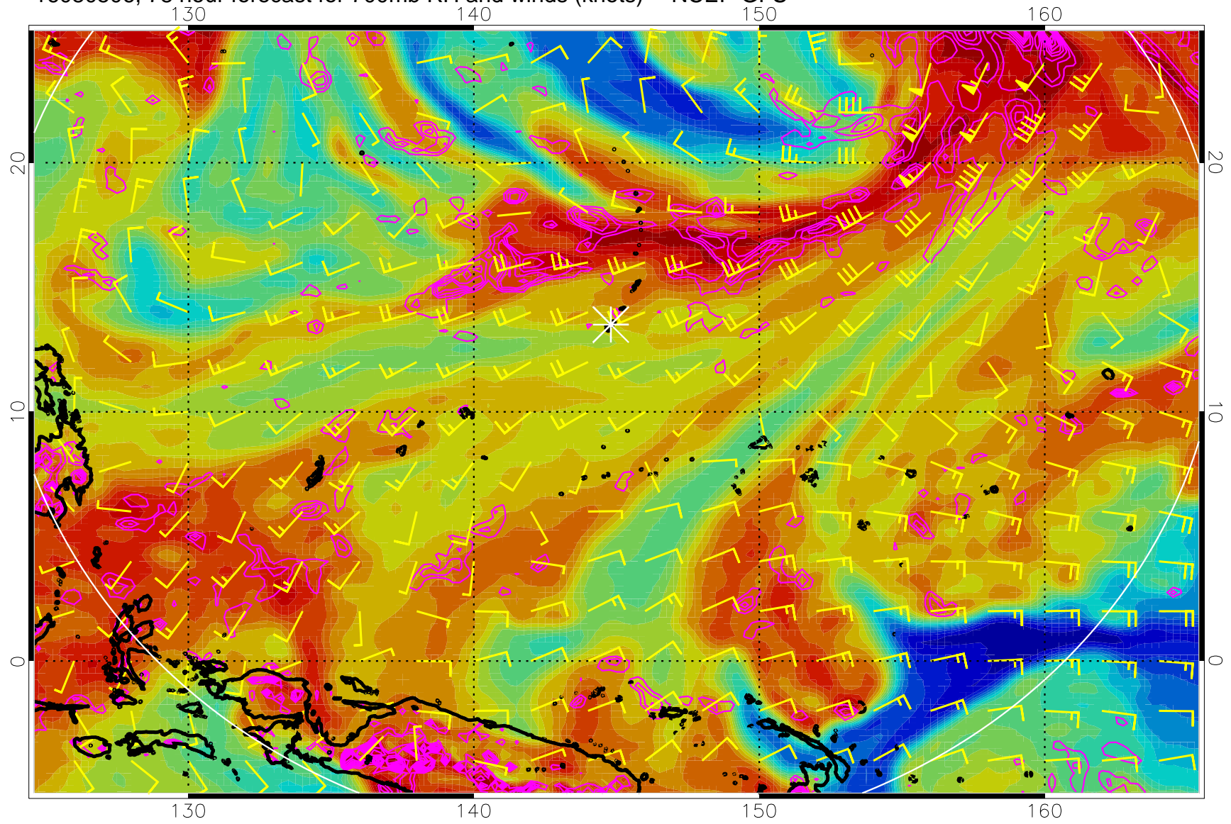
16080506, 78 hour forecast for 700mb RH and winds (knots) -- NCEP GFS
