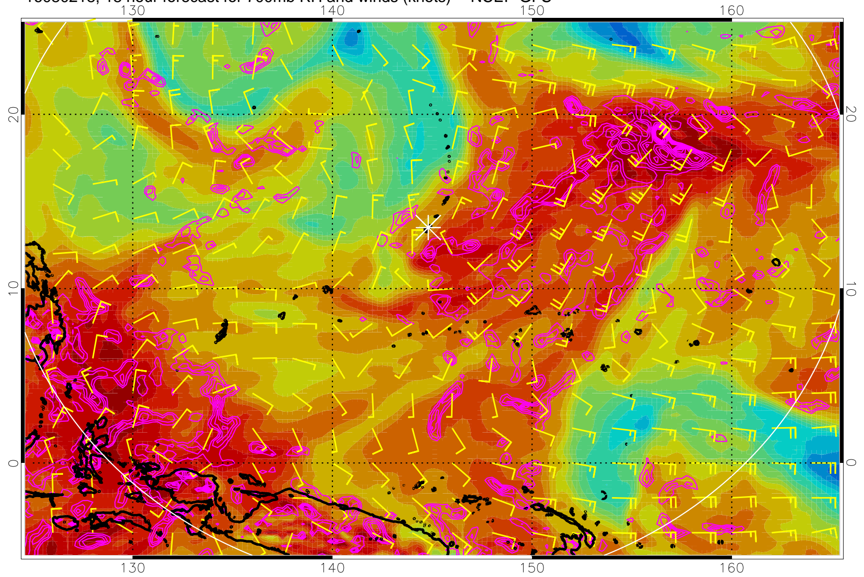
16080218, 18 hour forecast for 700mb RH and winds (knots) -- NCEP GFS
