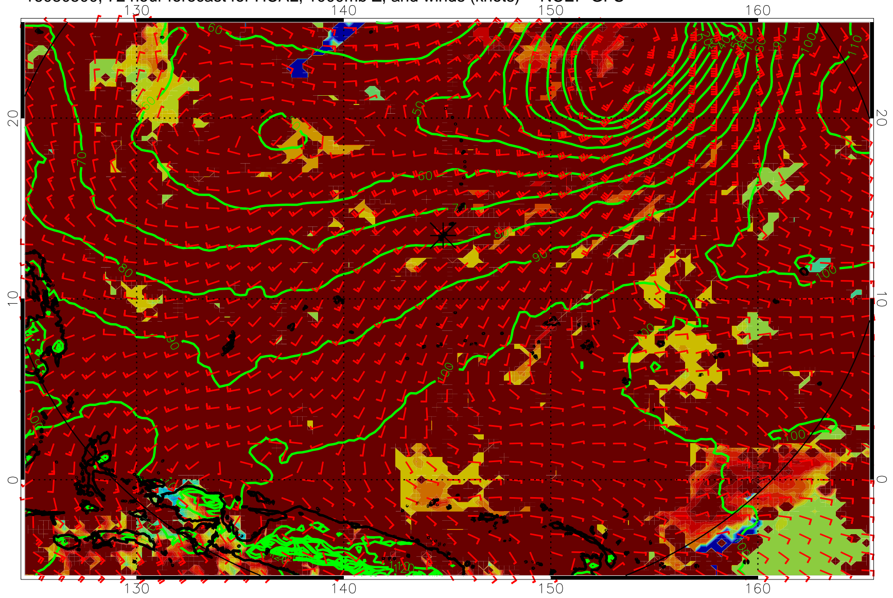
16080500, 72 hour forecast for HCAL, 1000mb Z, and winds (knots) -- NCEP GFS
