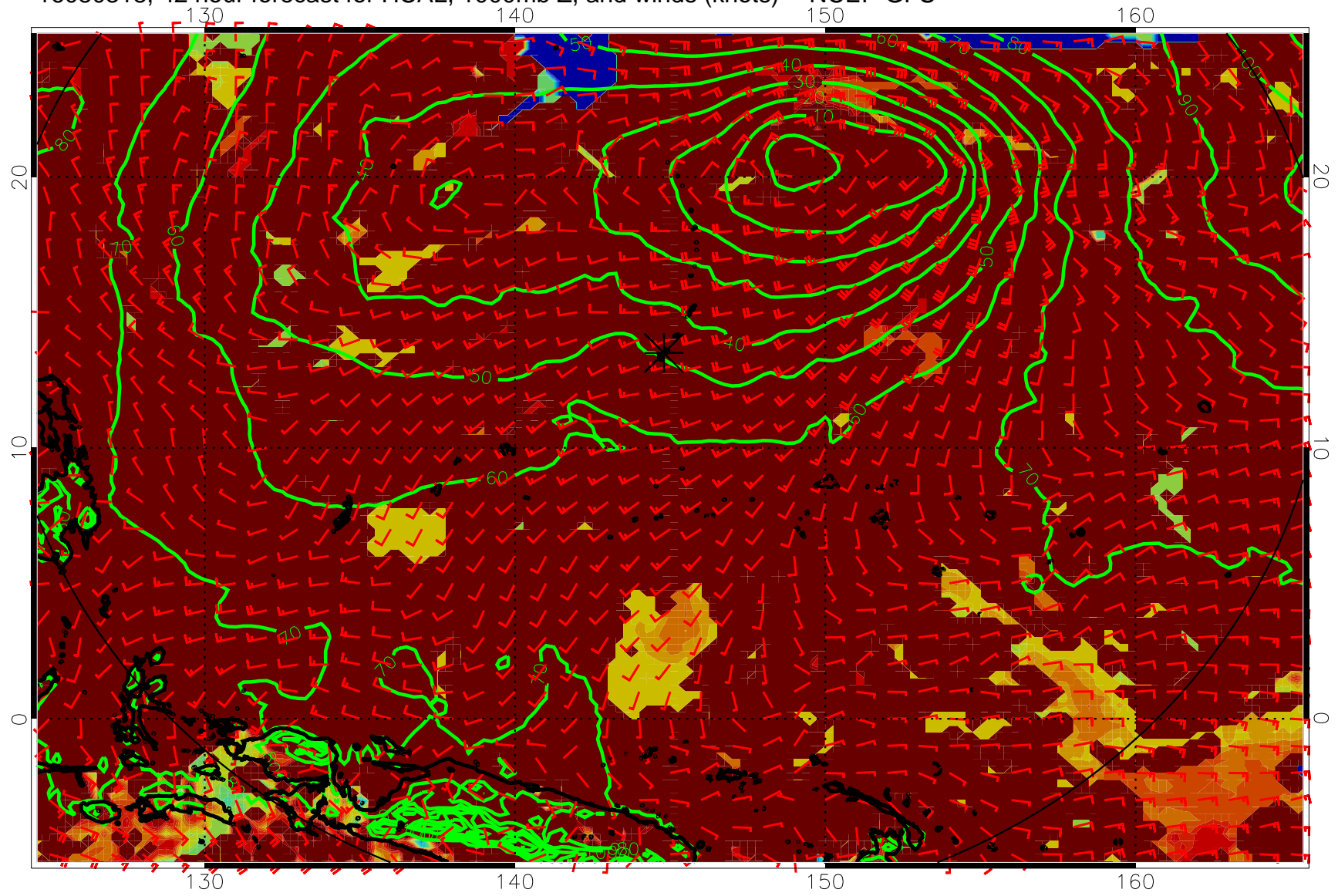
16080318, 42 hour forecast for HCAL, 1000mb Z, and winds (knots) -- NCEP GFS
