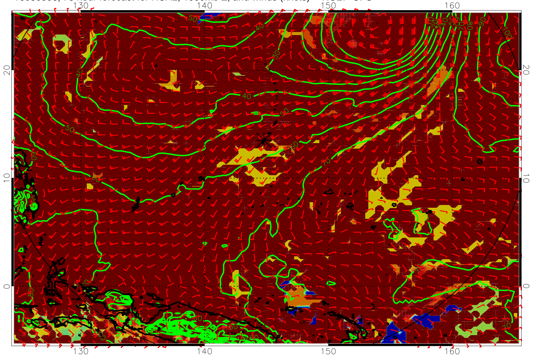
16080506, 78 hour forecast for HCAL, 1000mb Z, and winds (knots) -- NCEP GFS
