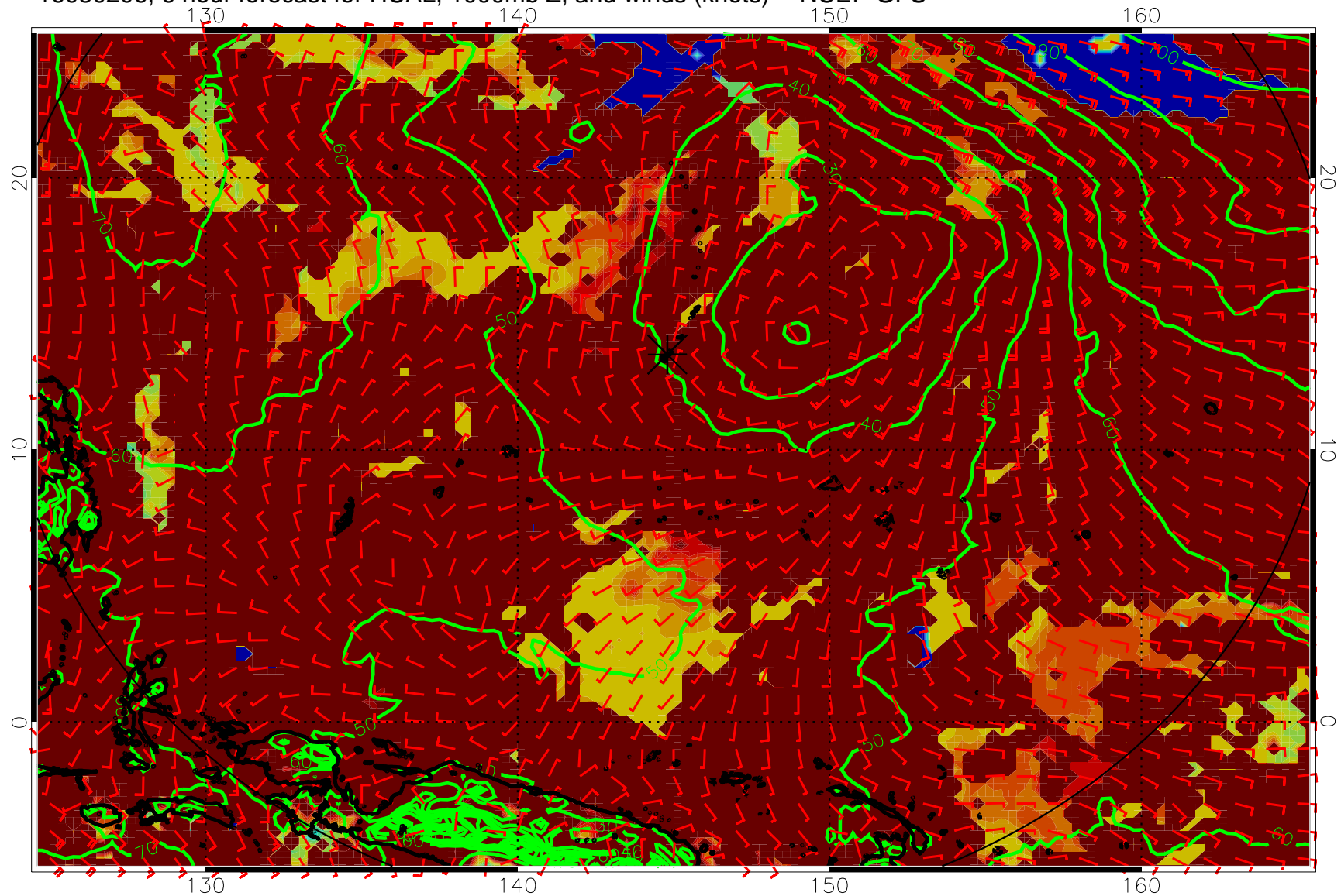
16080206, 6 hour forecast for HCAL, 1000mb Z, and winds (knots) -- NCEP GFS
