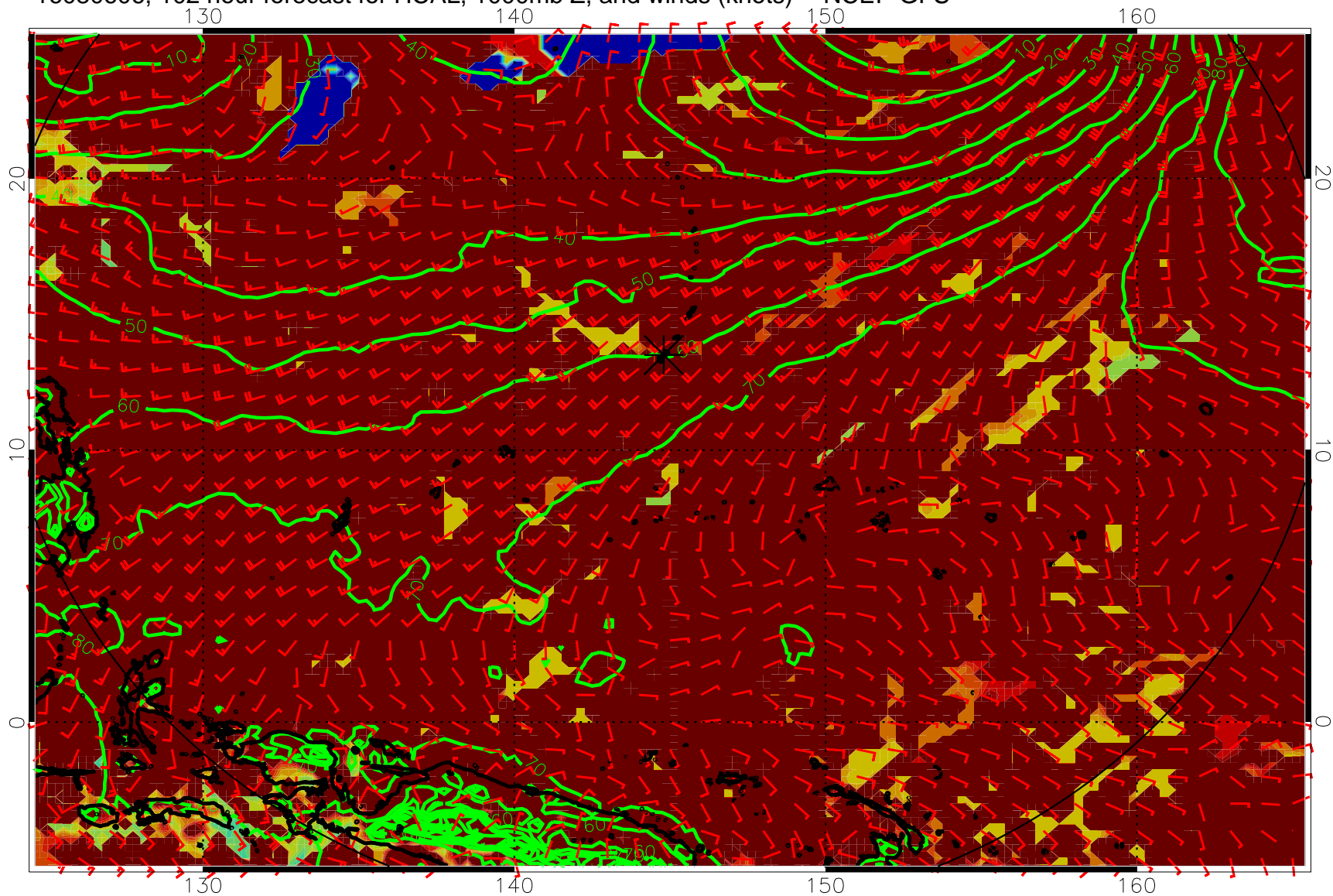
16080606, 102 hour forecast for HCAL, 1000mb Z, and winds (knots) -- NCEP GFS
