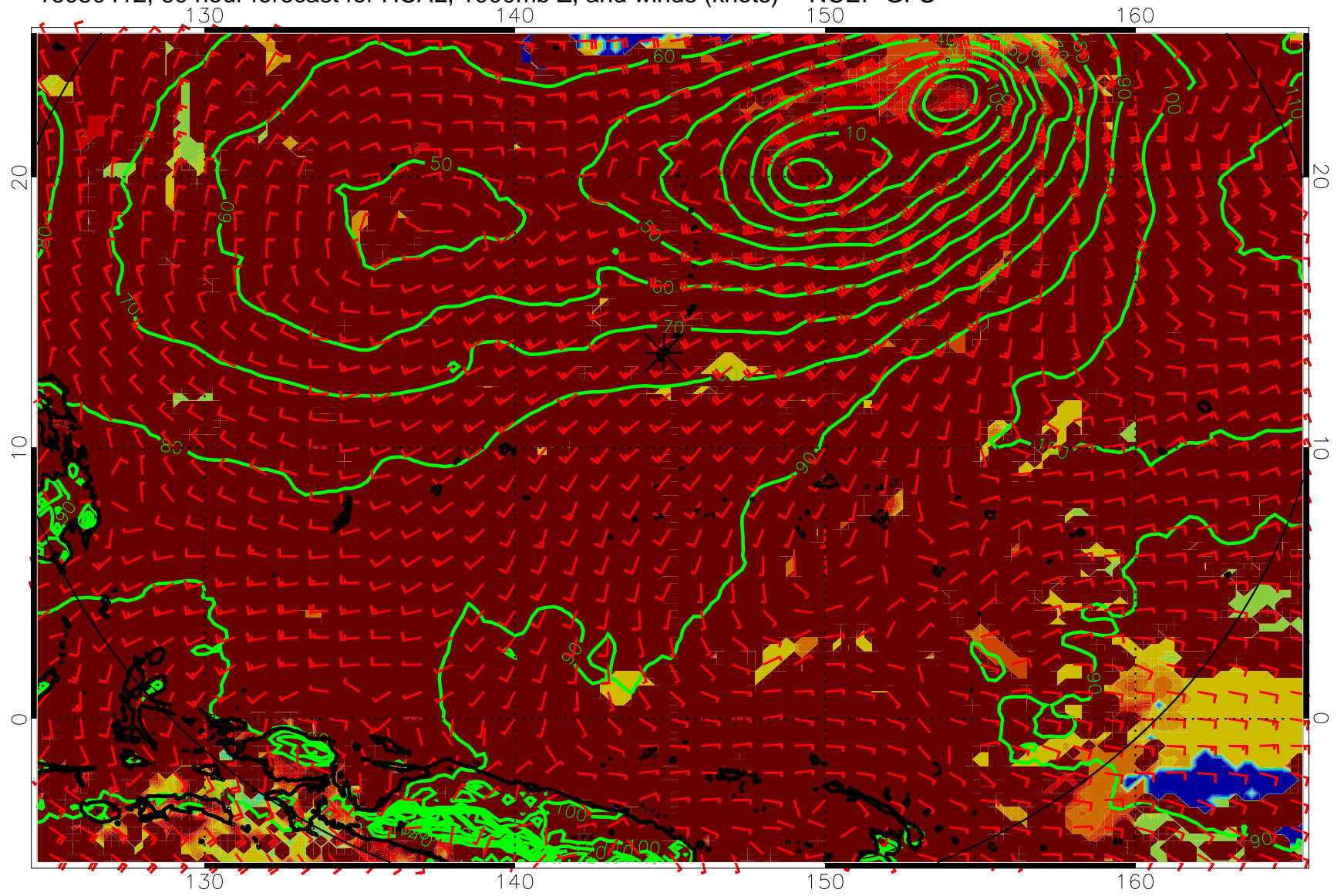
16080412, 60 hour forecast for HCAL, 1000mb Z, and winds (knots) -- NCEP GFS
