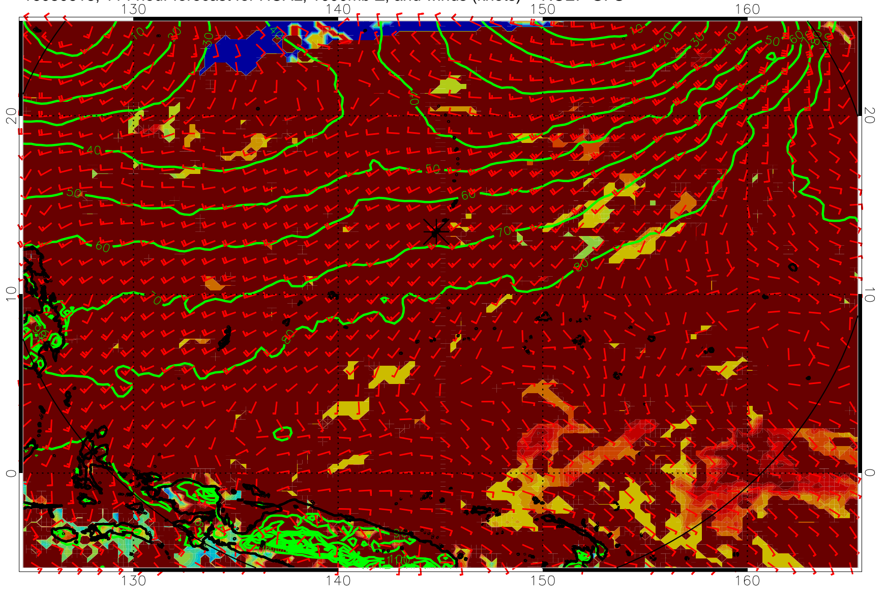
16080618, 114 hour forecast for HCAL, 1000mb Z, and winds (knots) -- NCEP GFS
