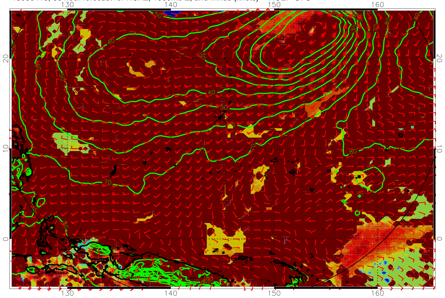
16080418, 66 hour forecast for HCAL, 1000mb Z, and winds (knots) -- NCEP GFS
