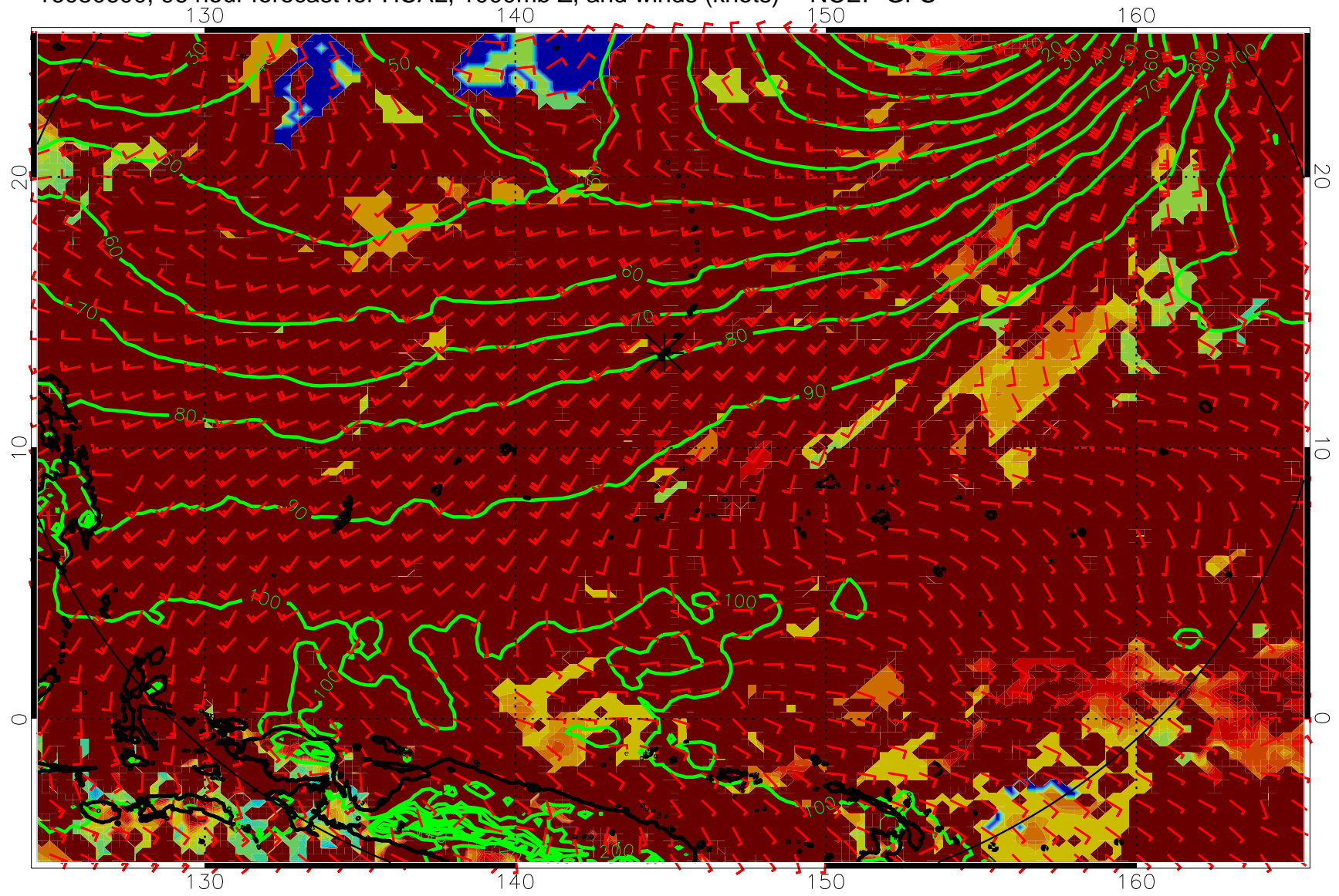
16080600, 96 hour forecast for HCAL, 1000mb Z, and winds (knots) -- NCEP GFS
