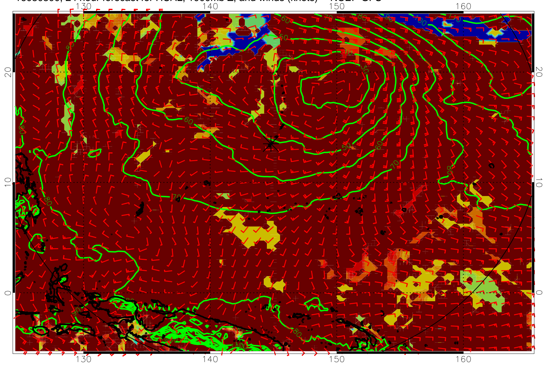
16080300, 24 hour forecast for HCAL, 1000mb Z, and winds (knots) -- NCEP GFS
