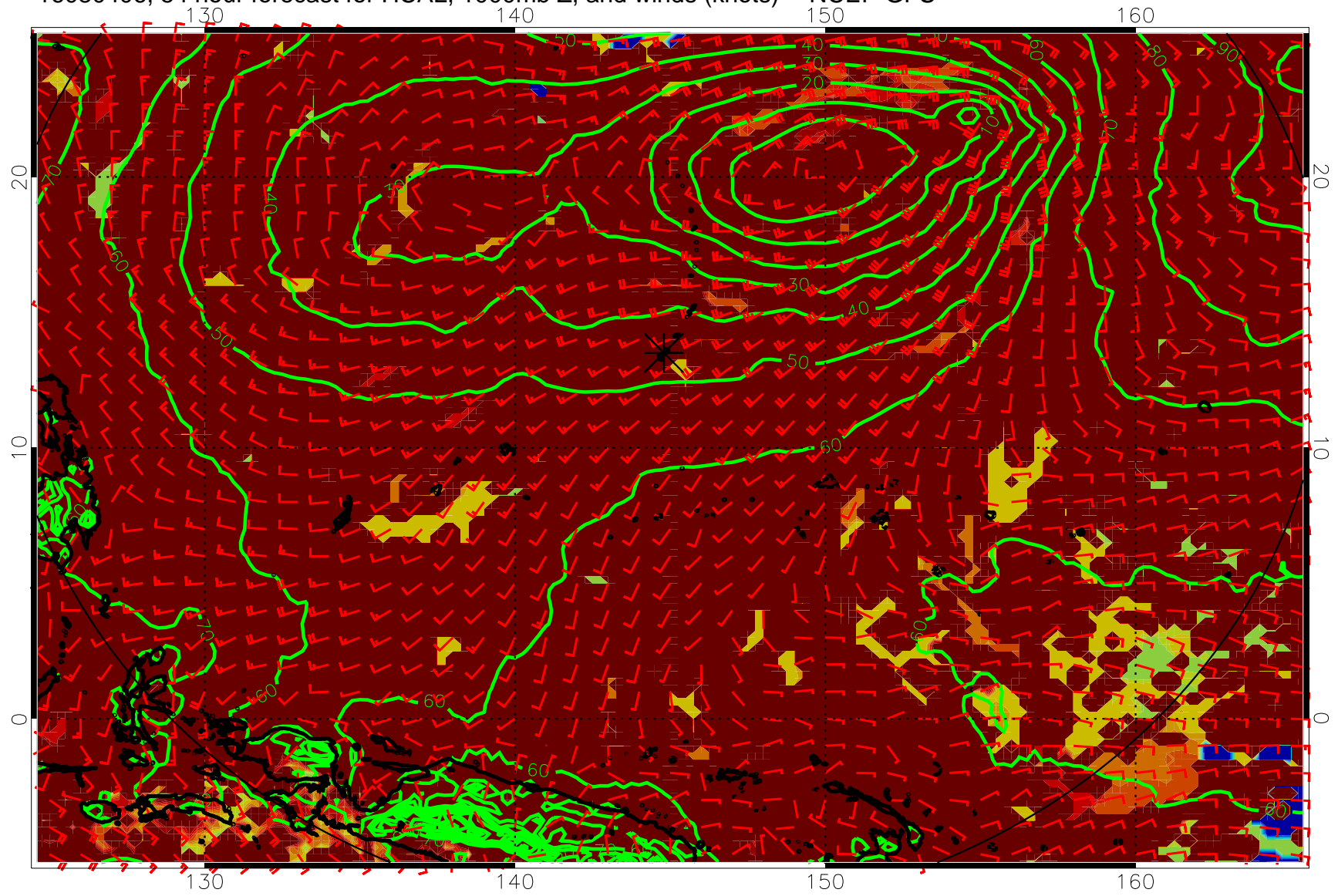
16080406, 54 hour forecast for HCAL, 1000mb Z, and winds (knots) -- NCEP GFS
