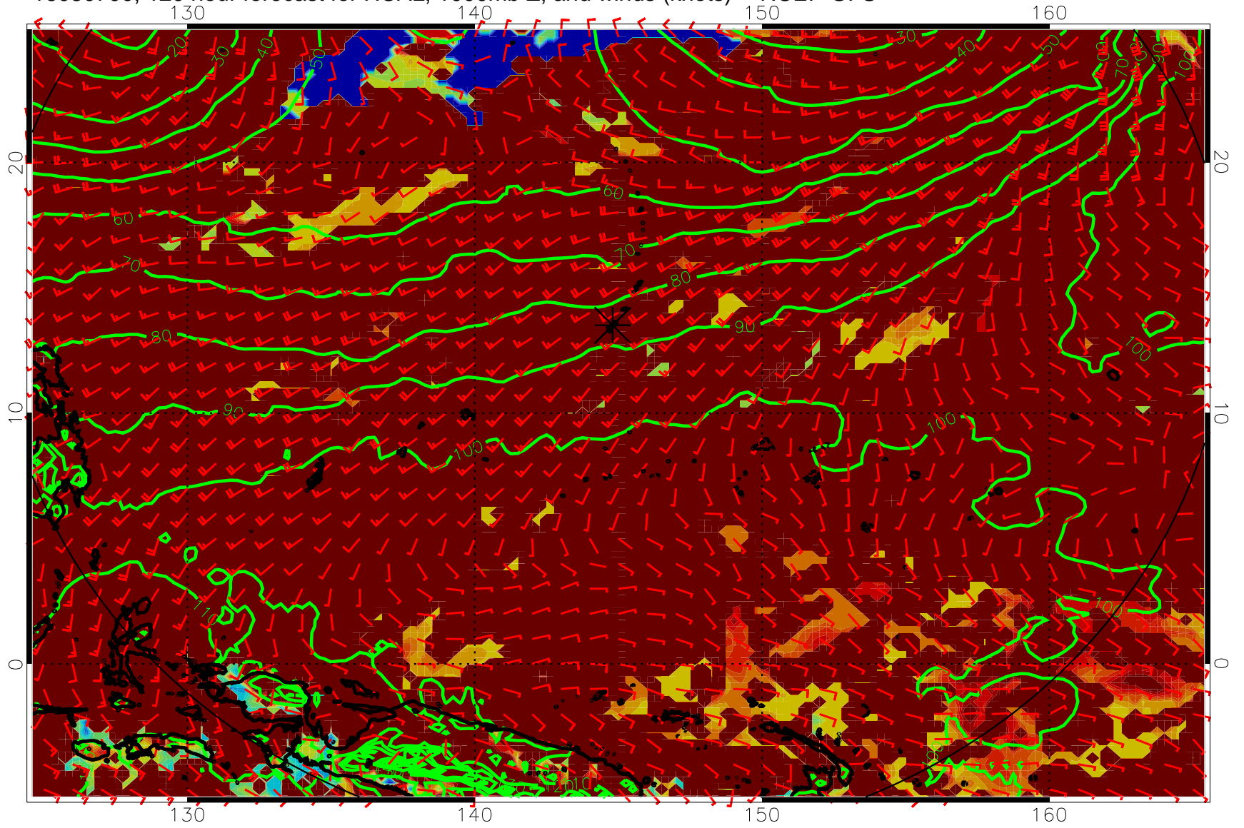
16080700, 120 hour forecast for HCAL, 1000mb Z, and winds (knots) -- NCEP GFS
