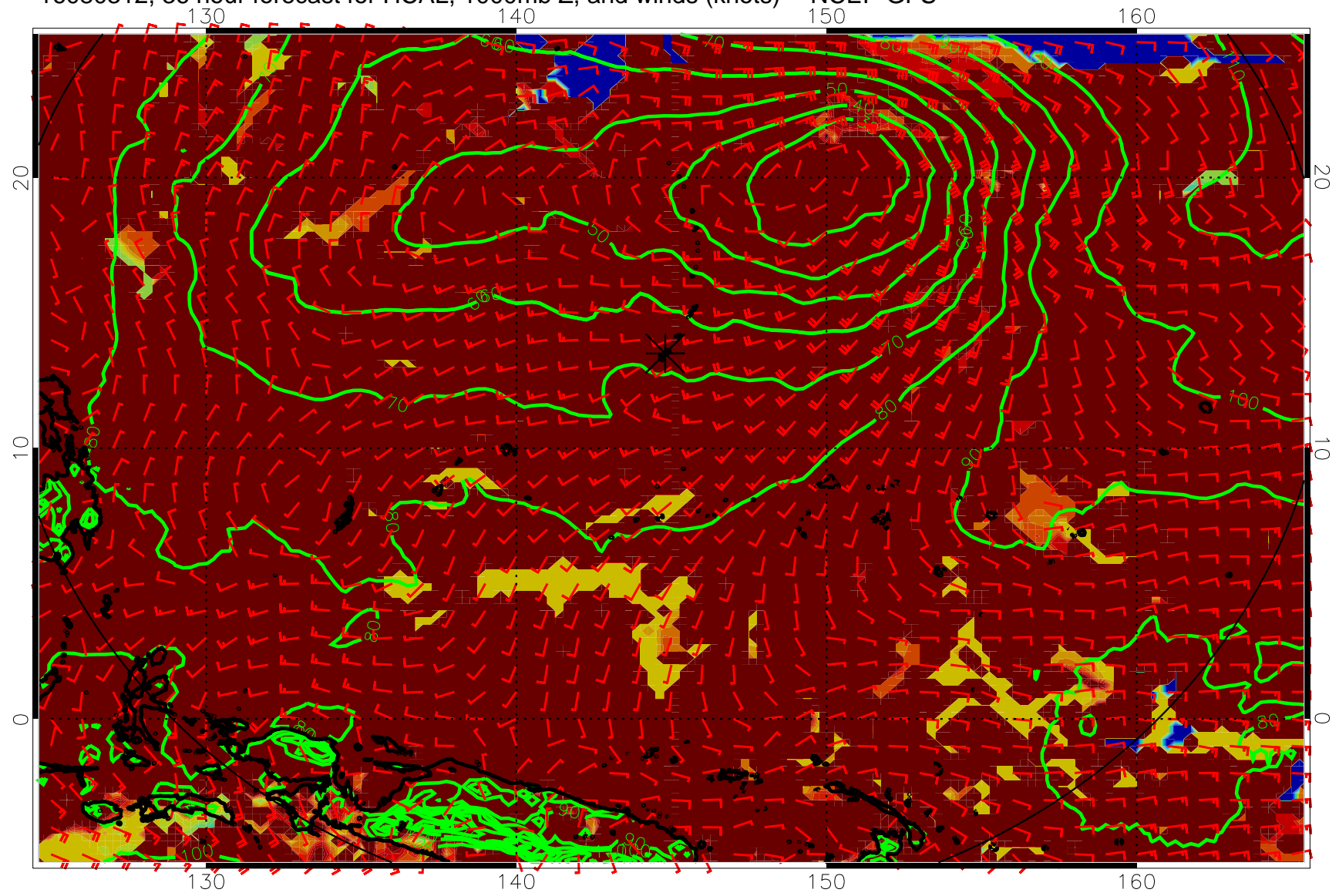
16080312, 36 hour forecast for HCAL, 1000mb Z, and winds (knots) -- NCEP GFS
