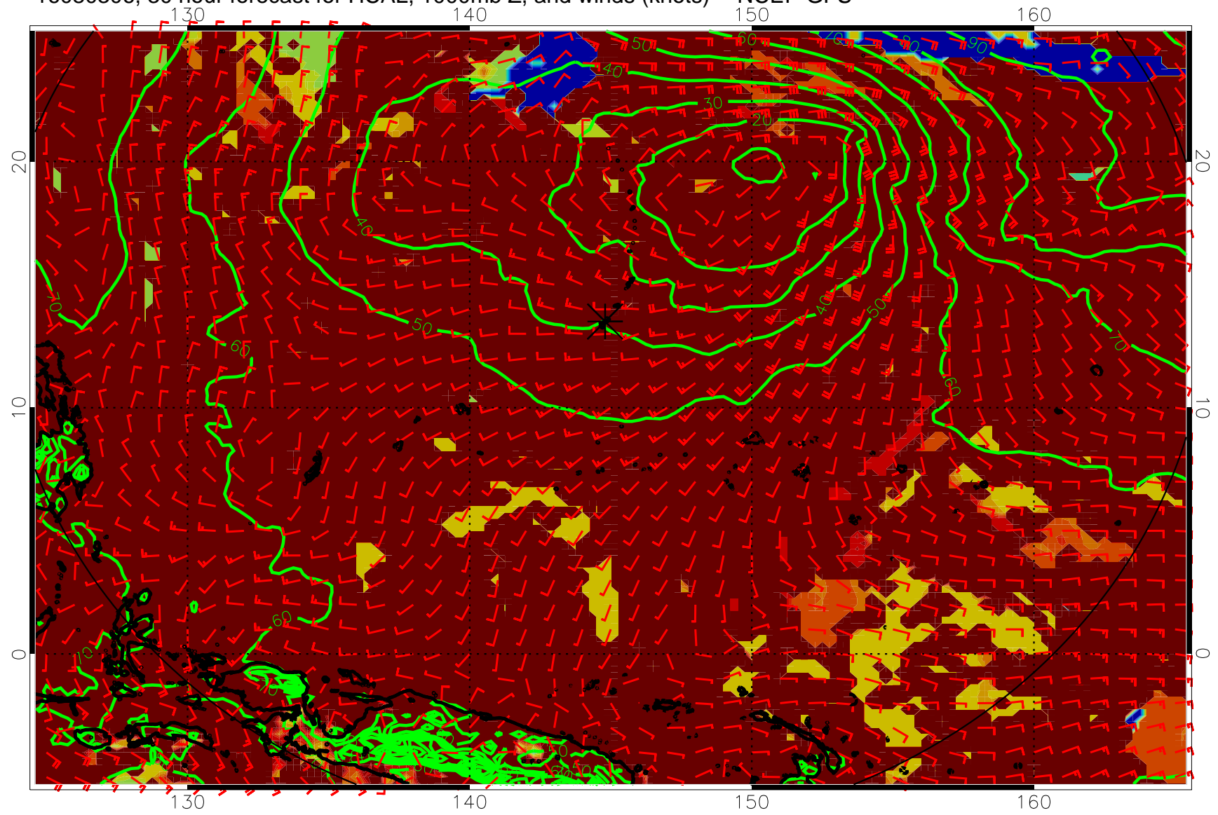
16080306, 30 hour forecast for HCAL, 1000mb Z, and winds (knots) -- NCEP GFS
