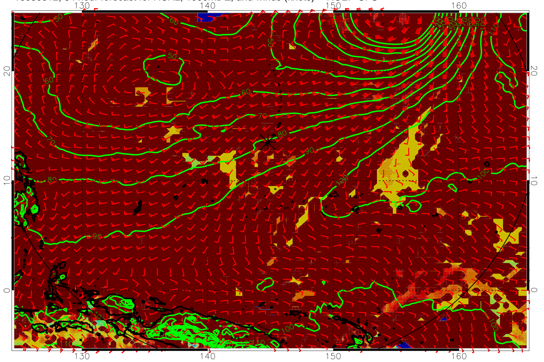
16080512, 84 hour forecast for HCAL, 1000mb Z, and winds (knots) -- NCEP GFS
