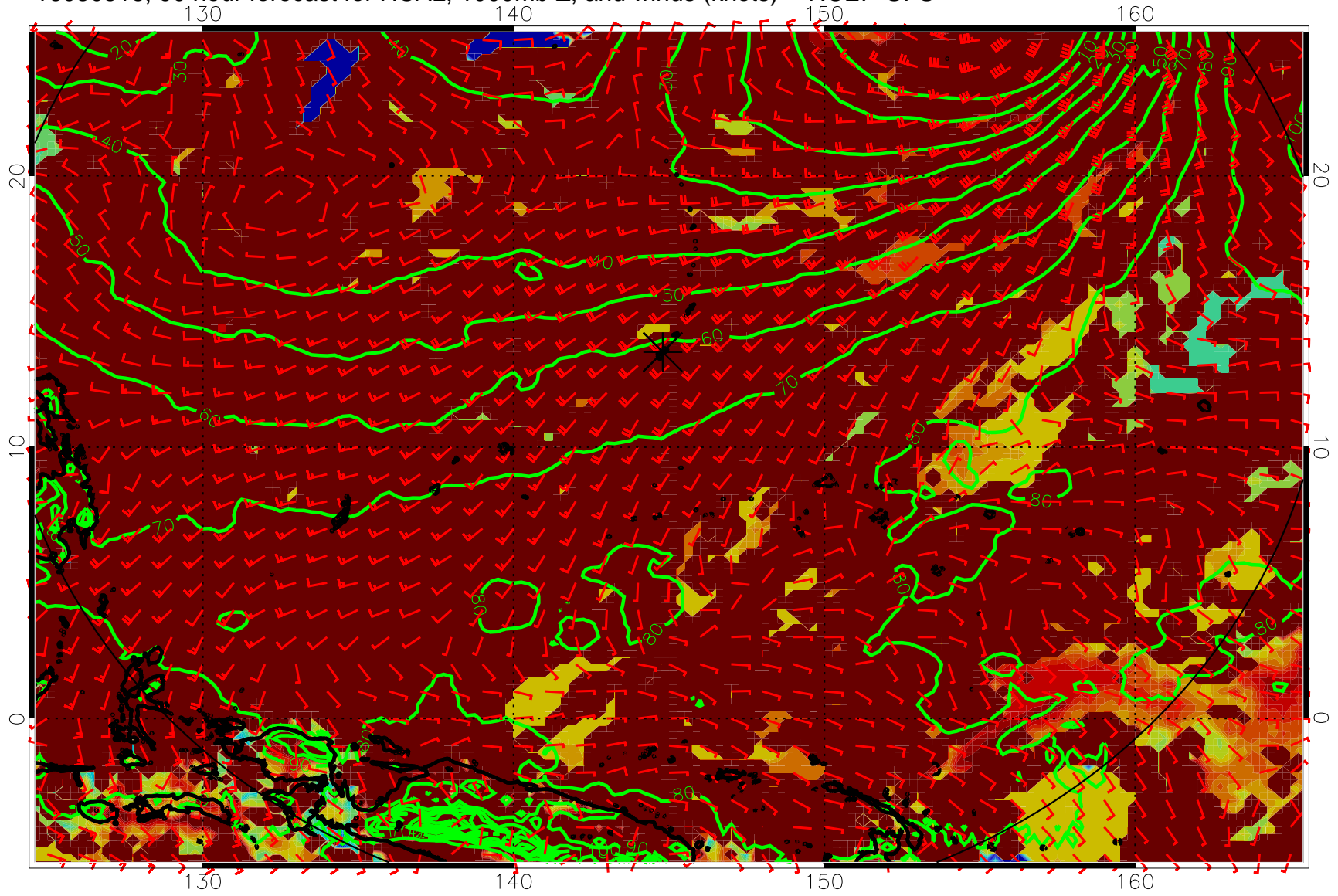
16080518, 90 hour forecast for HCAL, 1000mb Z, and winds (knots) -- NCEP GFS
