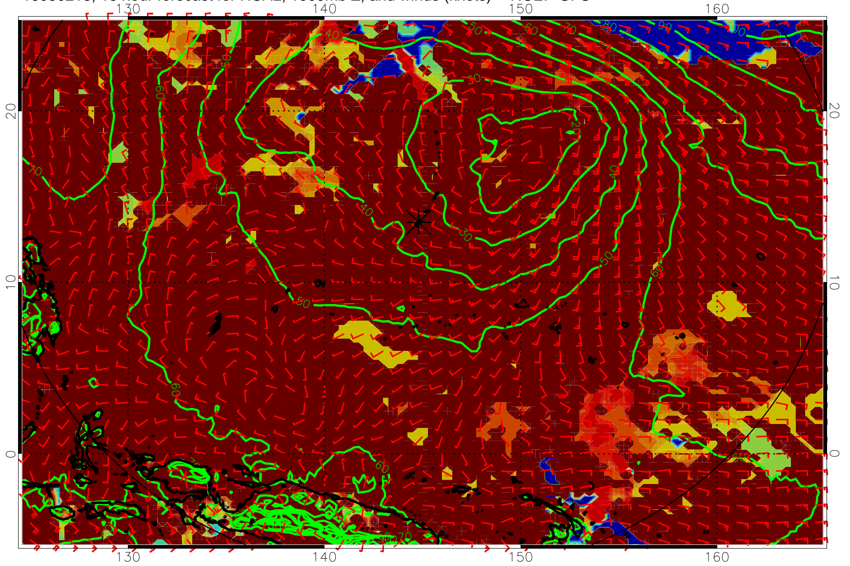
16080218, 18 hour forecast for HCAL, 1000mb Z, and winds (knots) -- NCEP GFS
