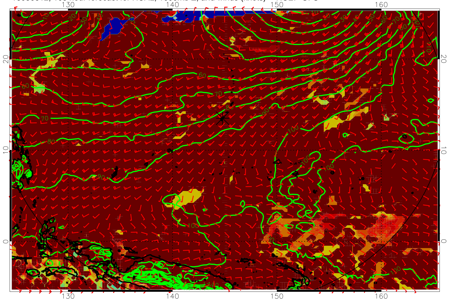
16080612, 108 hour forecast for HCAL, 1000mb Z, and winds (knots) -- NCEP GFS
