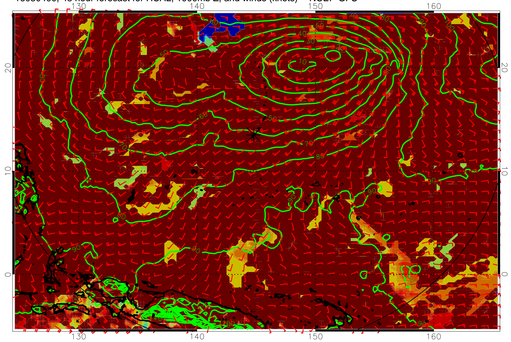
16080400, 48 hour forecast for HCAL, 1000mb Z, and winds (knots) -- NCEP GFS
