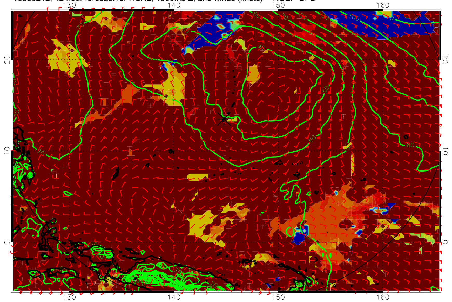
16080212, 12 hour forecast for HCAL, 1000mb Z, and winds (knots) -- NCEP GFS
