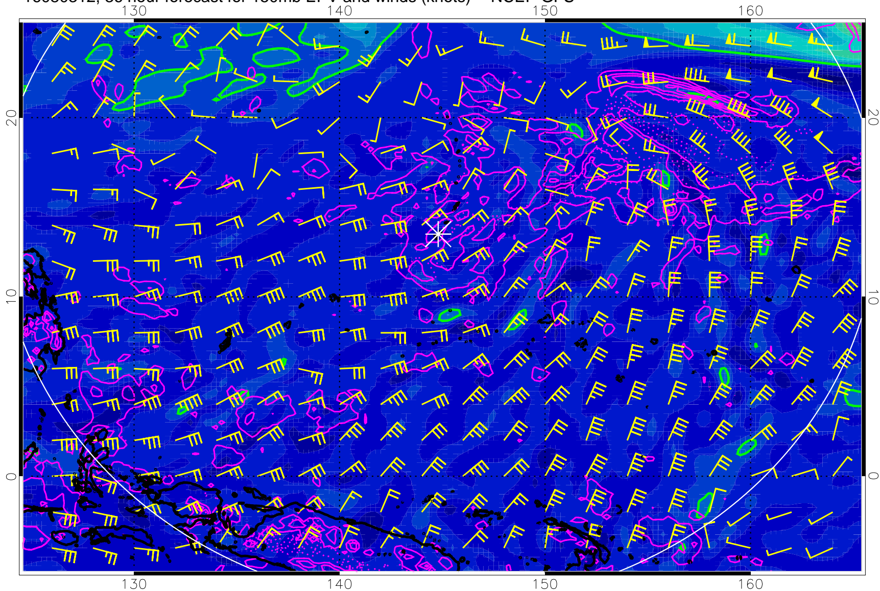
16080312, 36 hour forecast for 150mb EPV and winds (knots) -- NCEP GFS
