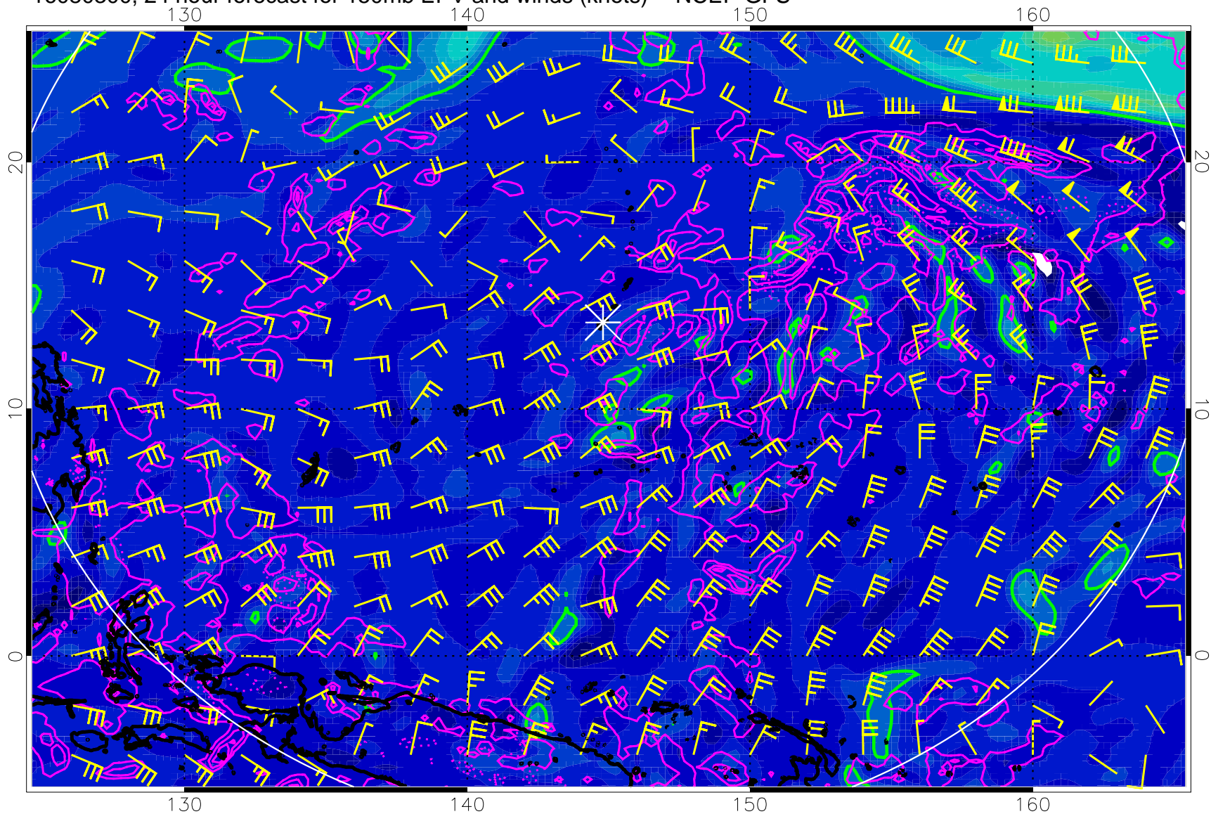
16080300, 24 hour forecast for 150mb EPV and winds (knots) -- NCEP GFS
