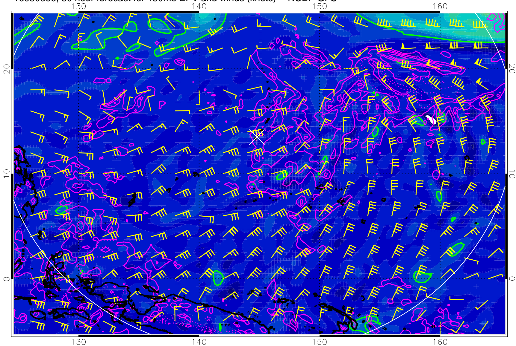
16080306, 30 hour forecast for 150mb EPV and winds (knots) -- NCEP GFS
