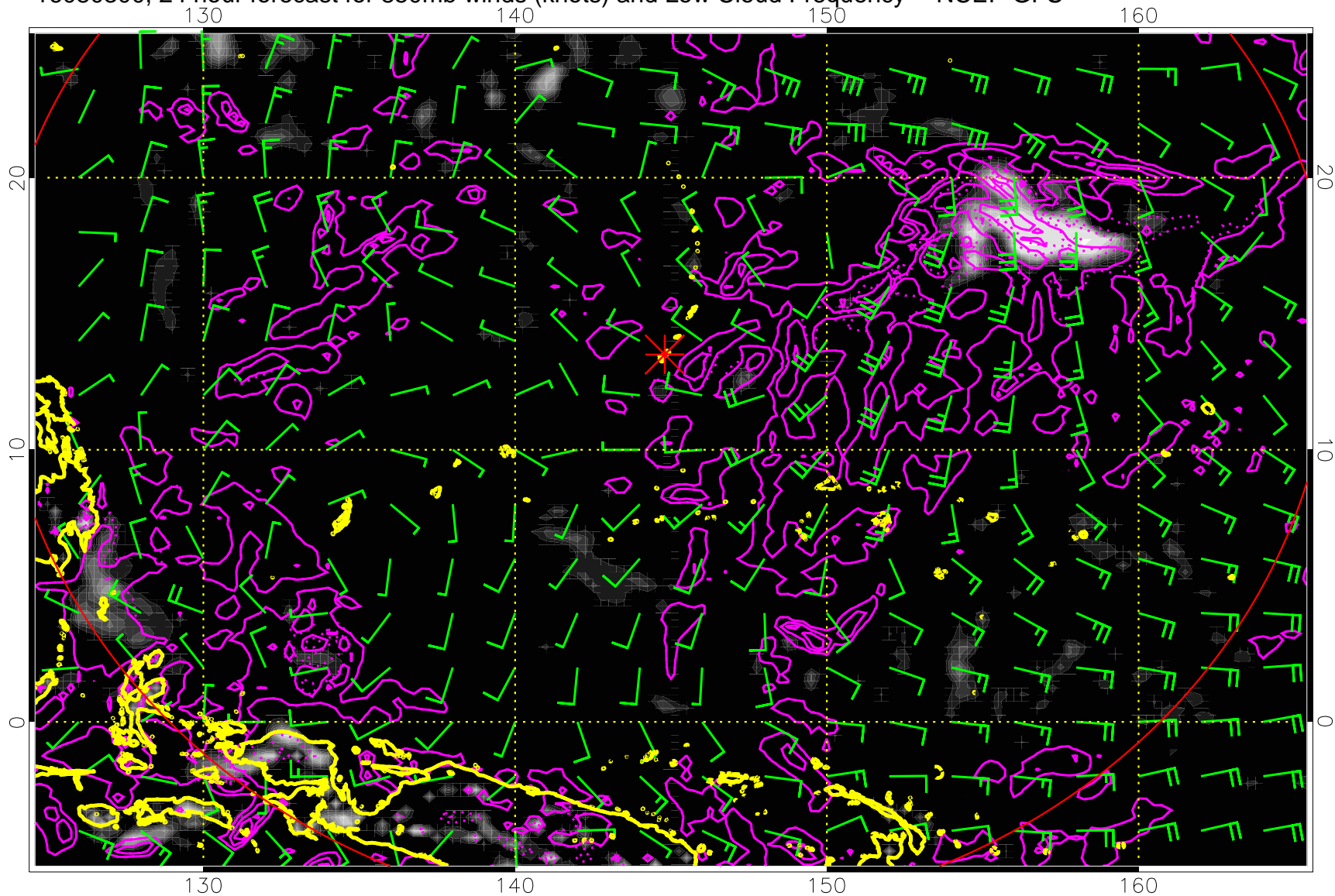
16080300, 24 hour forecast for 850mb winds (knots) and Low Cloud Frequency -- NCEP GFS
