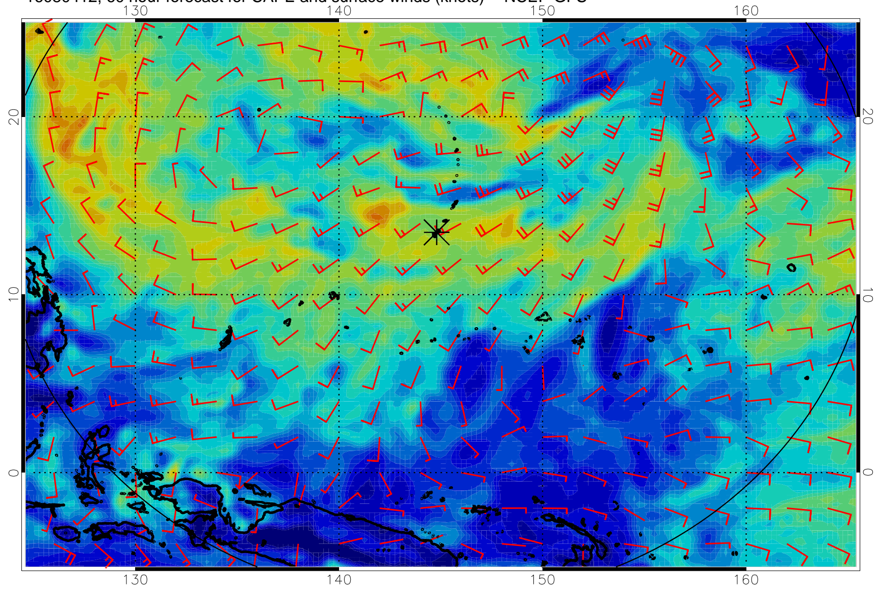
16080412, 60 hour forecast for CAPE and surface winds (knots) -- NCEP GFS
