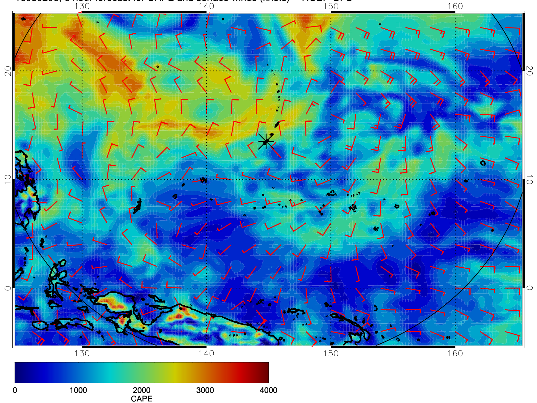
16080206, 6 hour forecast for CAPE and surface winds (knots) -- NCEP GFS
