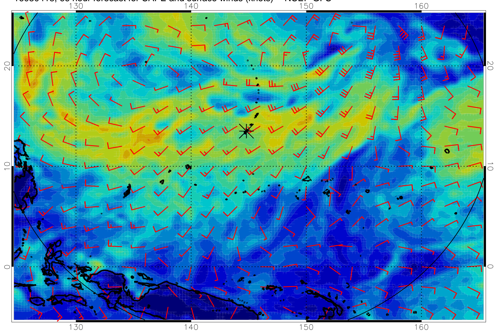
16080418, 66 hour forecast for CAPE and surface winds (knots) -- NCEP GFS
