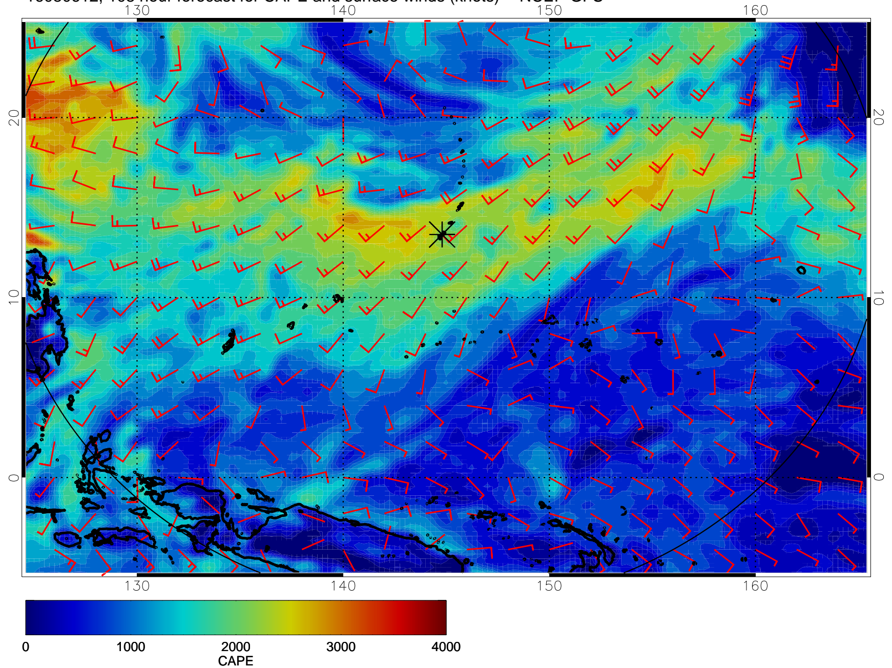
16080612, 108 hour forecast for CAPE and surface winds (knots) -- NCEP GFS
