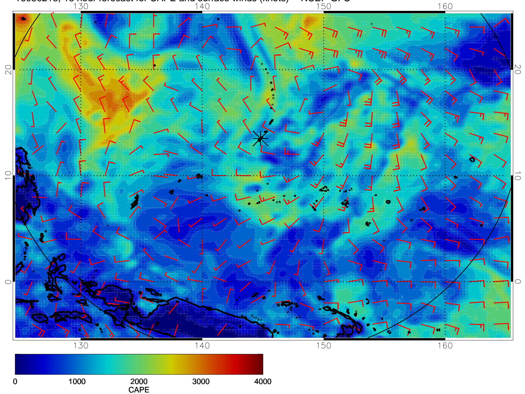
16080218, 18 hour forecast for CAPE and surface winds (knots) -- NCEP GFS
