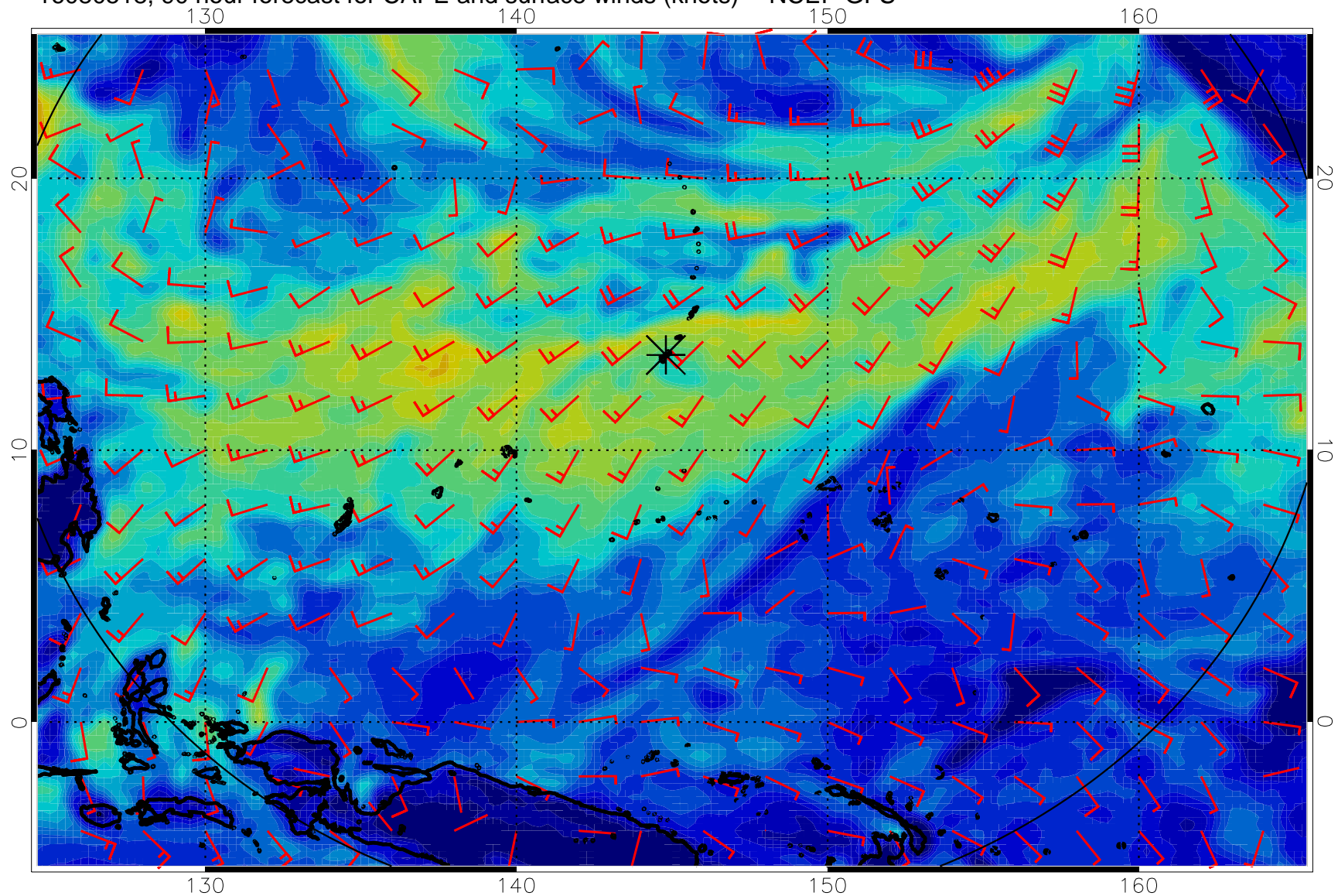
16080518, 90 hour forecast for CAPE and surface winds (knots) -- NCEP GFS
