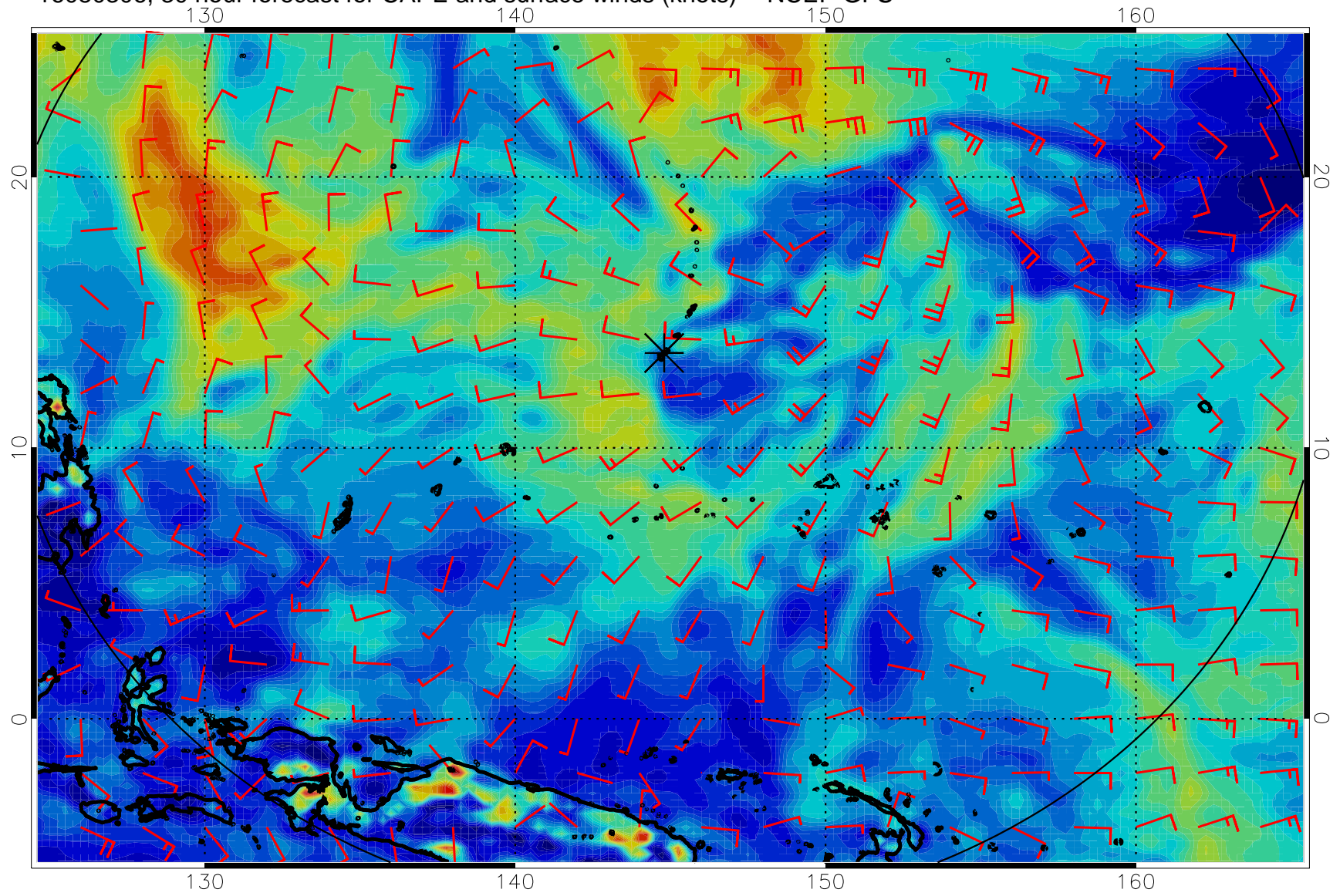
16080306, 30 hour forecast for CAPE and surface winds (knots) -- NCEP GFS
