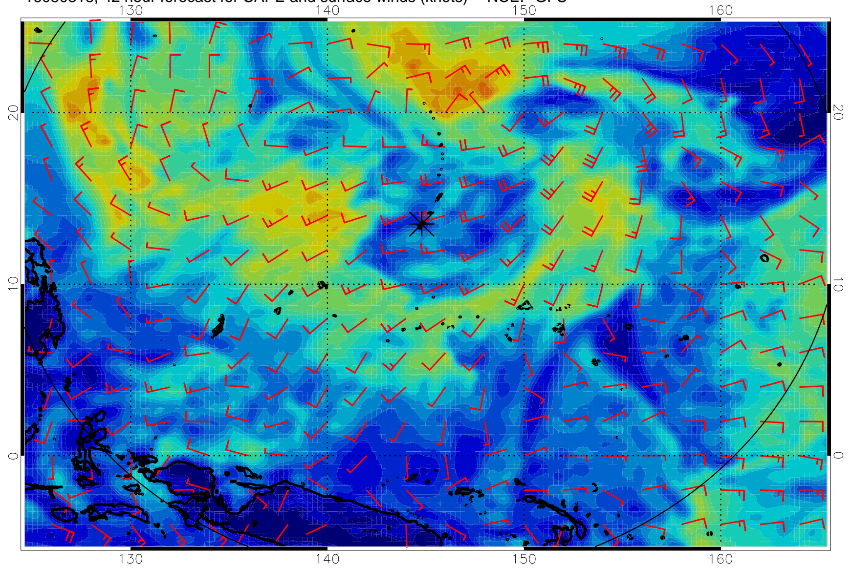
16080318, 42 hour forecast for CAPE and surface winds (knots) -- NCEP GFS
