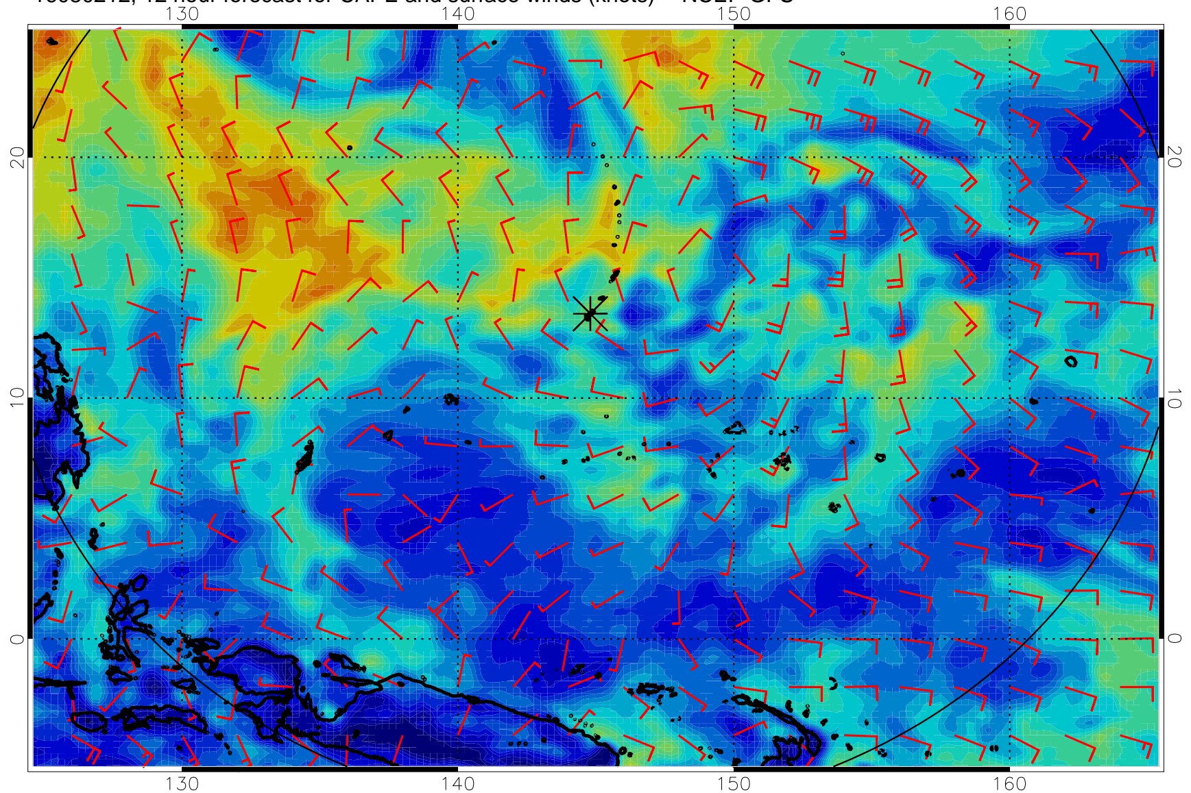
16080212, 12 hour forecast for CAPE and surface winds (knots) -- NCEP GFS
