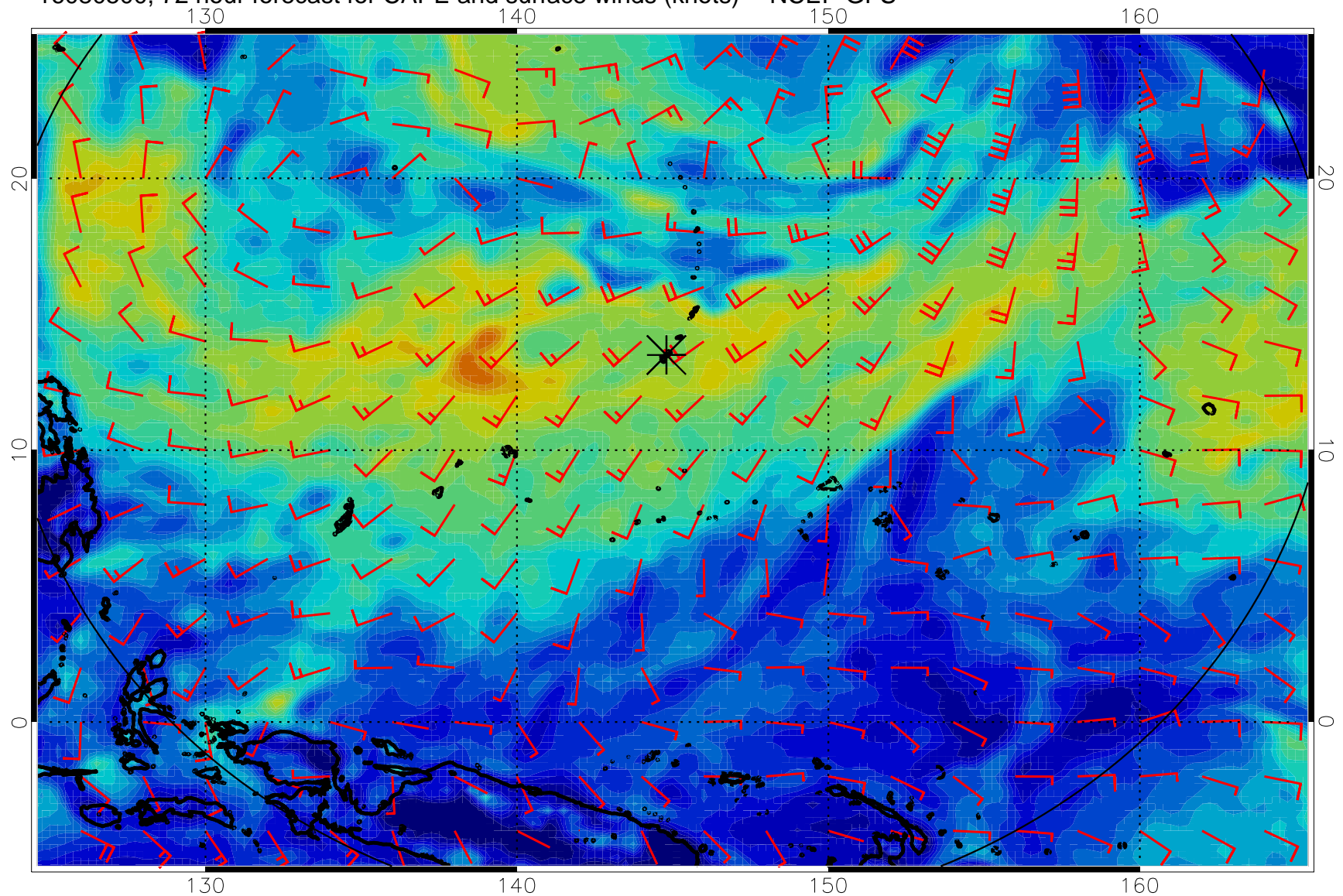
16080500, 72 hour forecast for CAPE and surface winds (knots) -- NCEP GFS
