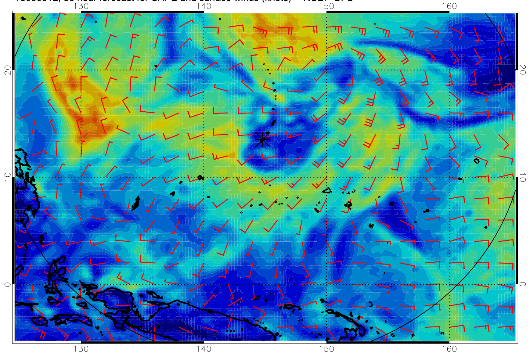
16080312, 36 hour forecast for CAPE and surface winds (knots) -- NCEP GFS
