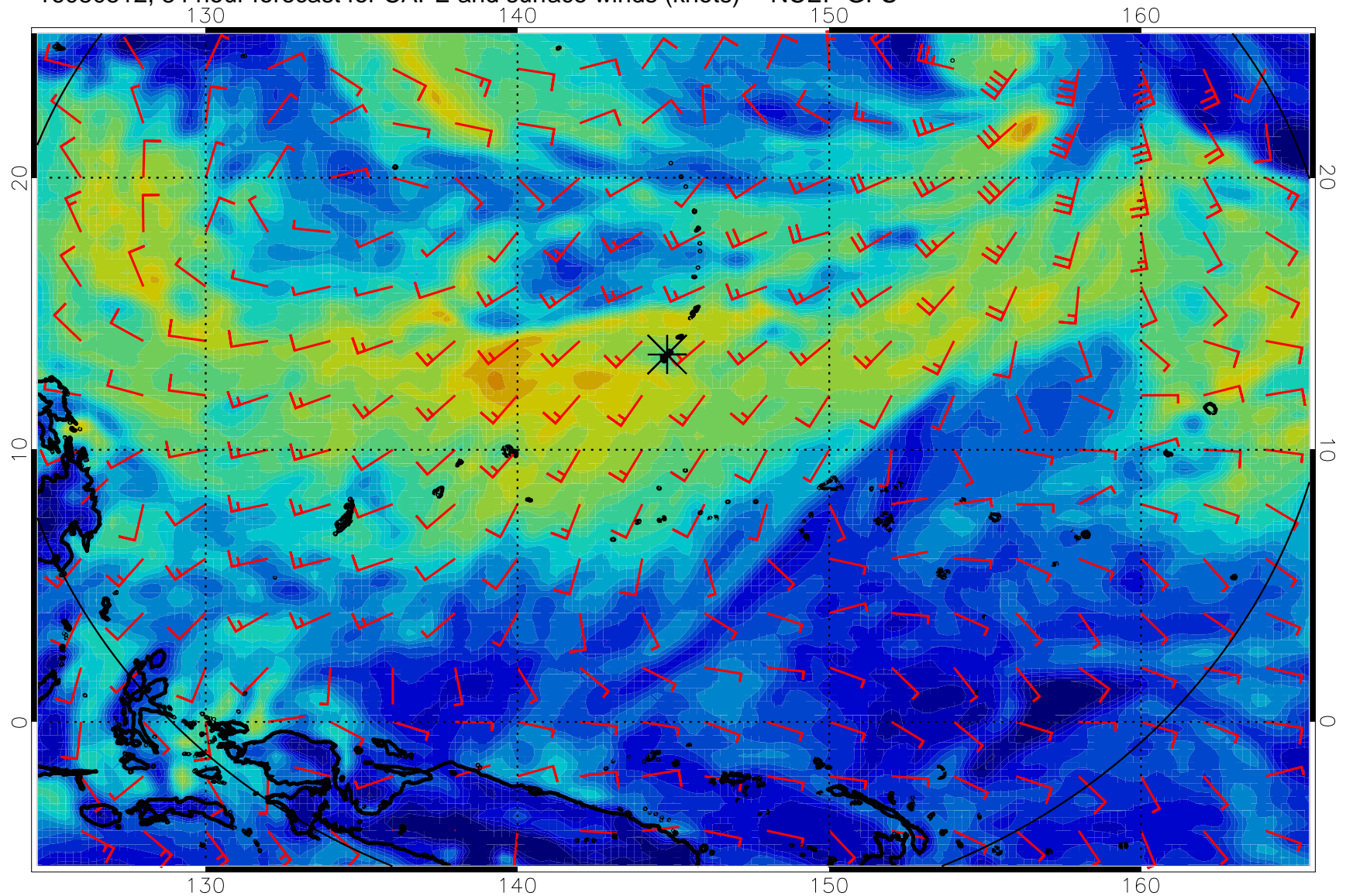
16080512, 84 hour forecast for CAPE and surface winds (knots) -- NCEP GFS
