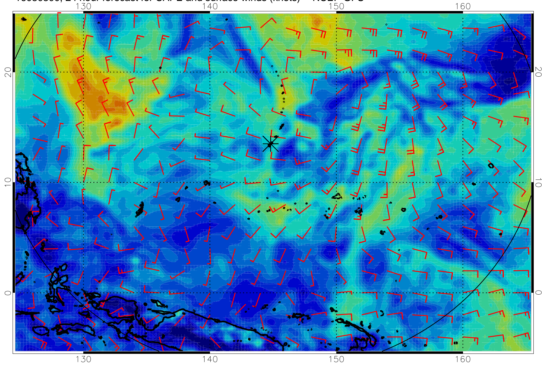
16080300, 24 hour forecast for CAPE and surface winds (knots) -- NCEP GFS
