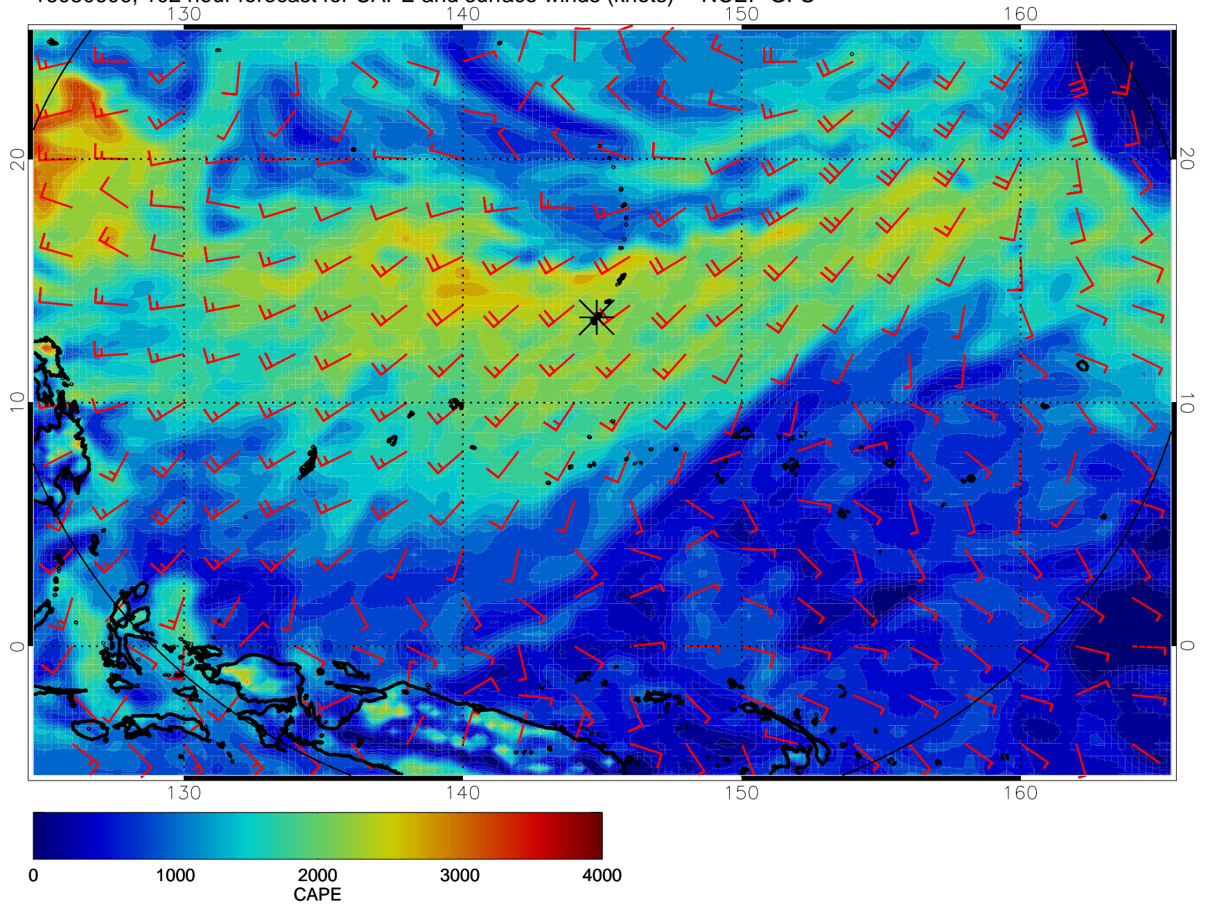
16080606, 102 hour forecast for CAPE and surface winds (knots) -- NCEP GFS
