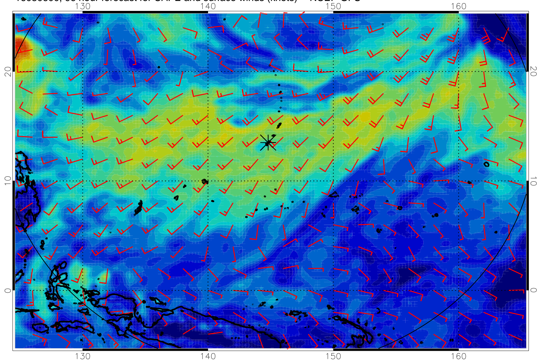
16080600, 96 hour forecast for CAPE and surface winds (knots) -- NCEP GFS
