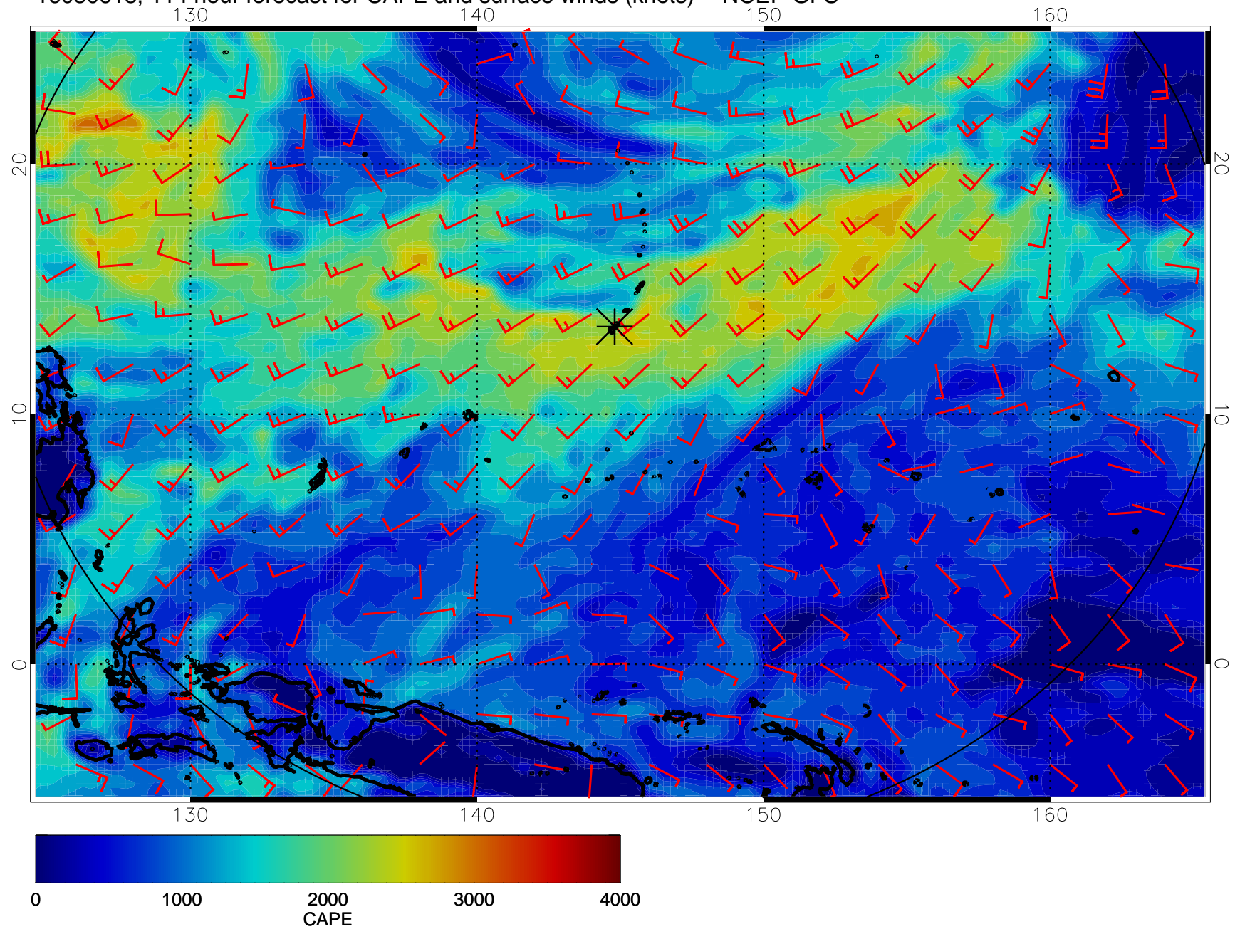
16080618, 114 hour forecast for CAPE and surface winds (knots) -- NCEP GFS
