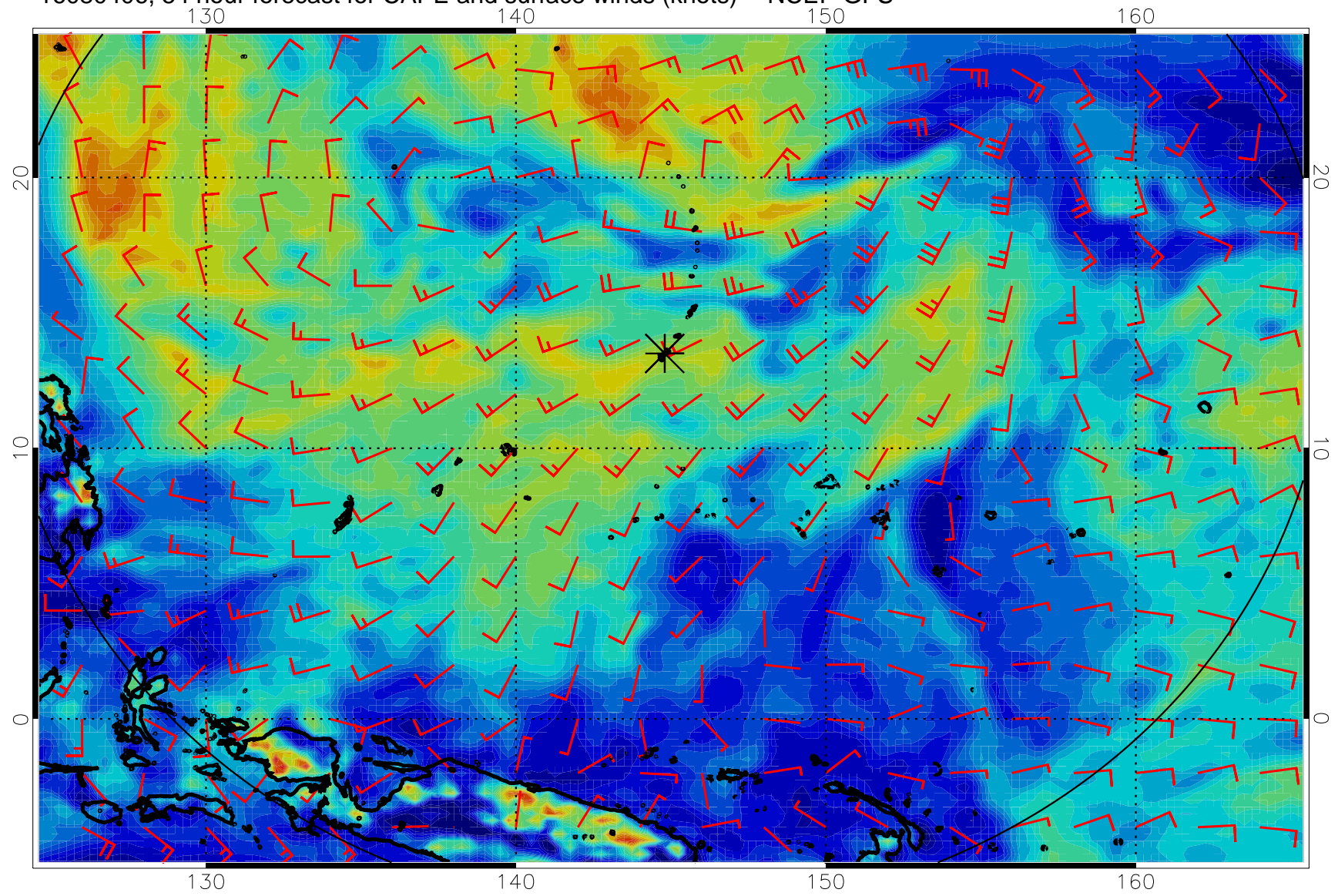
16080406, 54 hour forecast for CAPE and surface winds (knots) -- NCEP GFS
