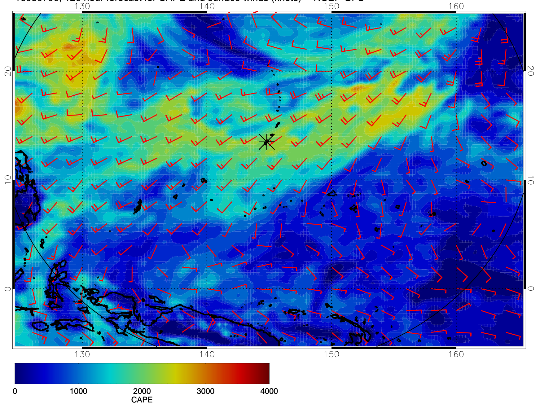
16080700, 120 hour forecast for CAPE and surface winds (knots) -- NCEP GFS
