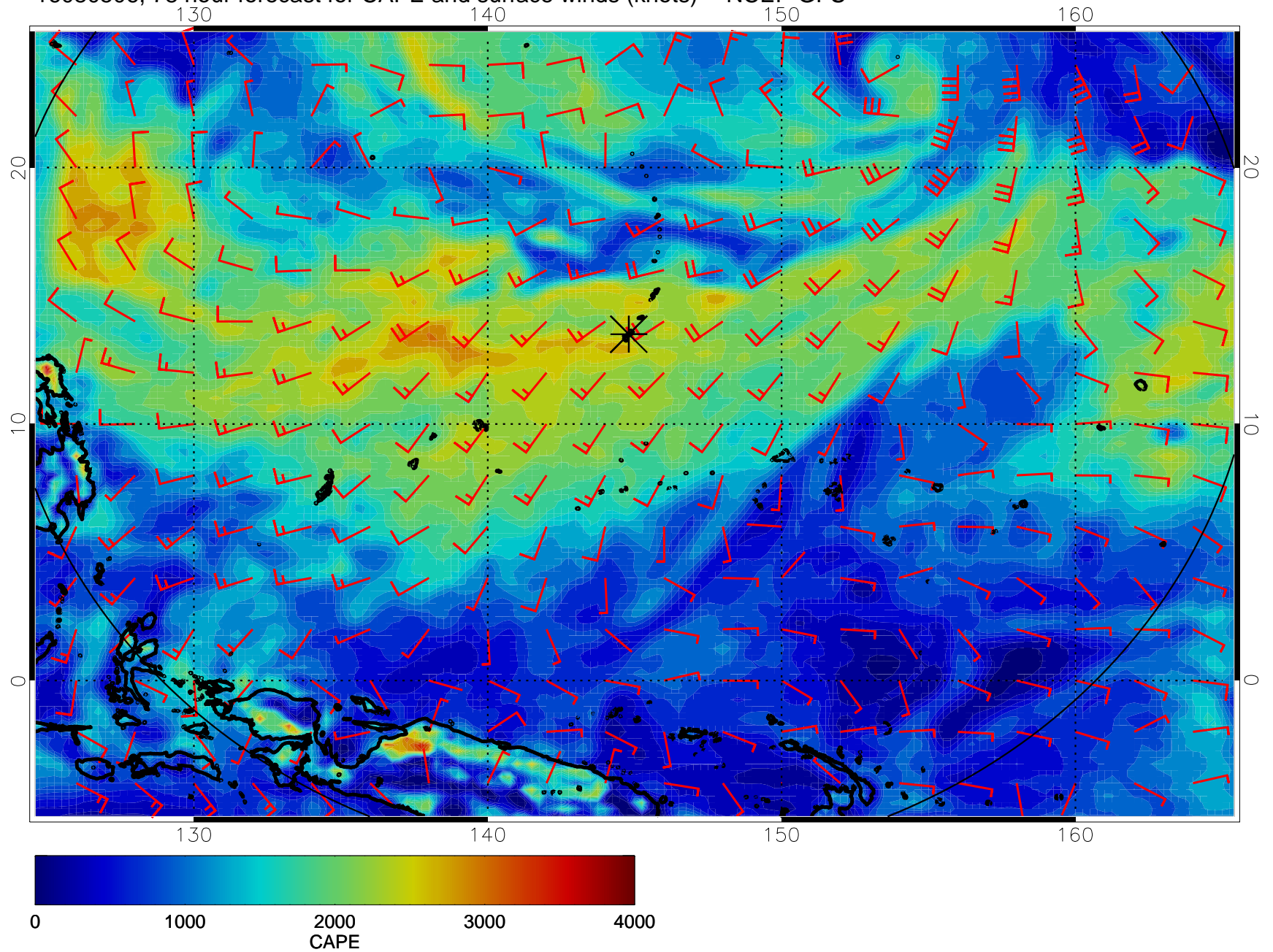
16080506, 78 hour forecast for CAPE and surface winds (knots) -- NCEP GFS
