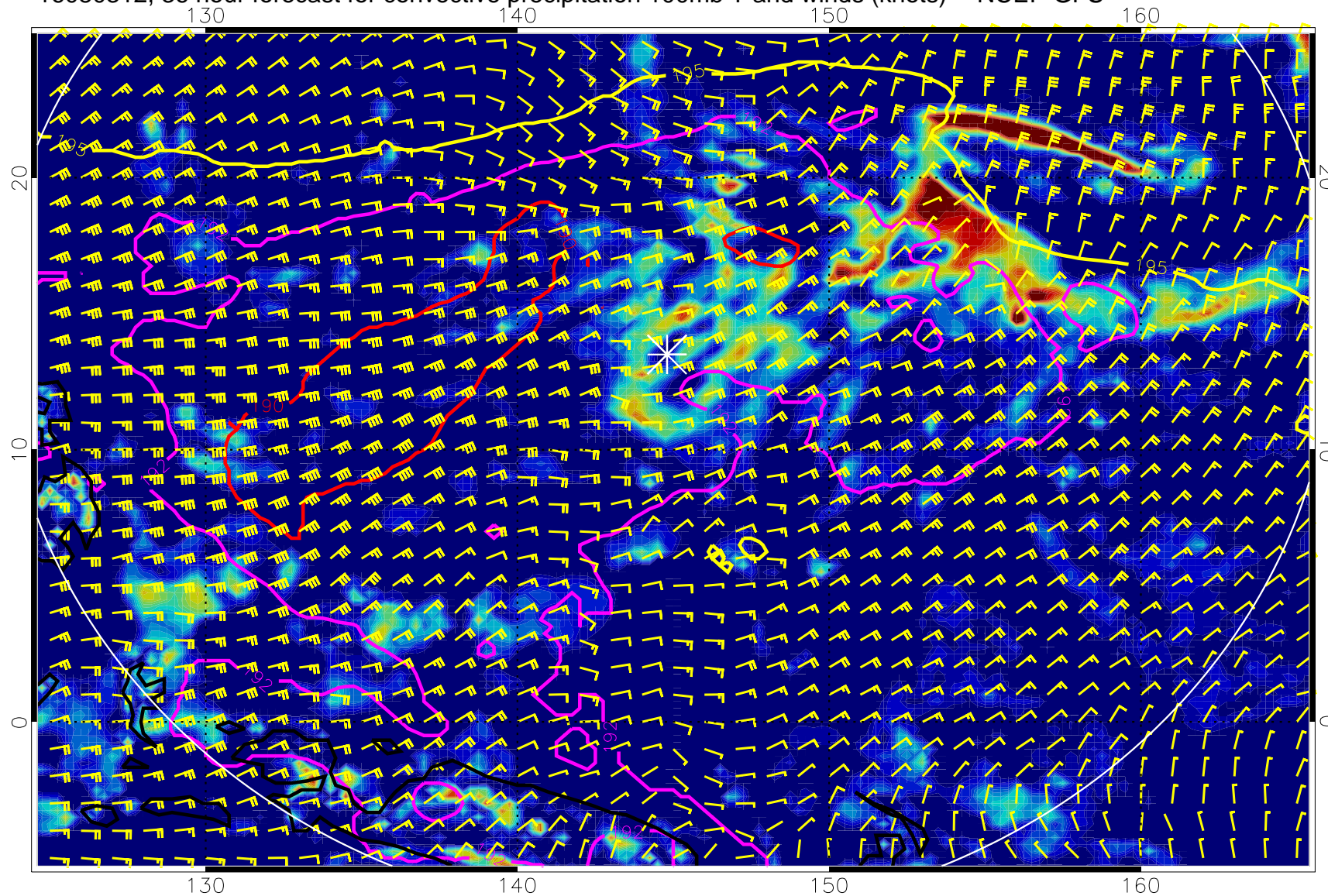
16080312, 36 hour forecast for convective precipitation 100mb T and winds (knots) -- NCEP GFS
