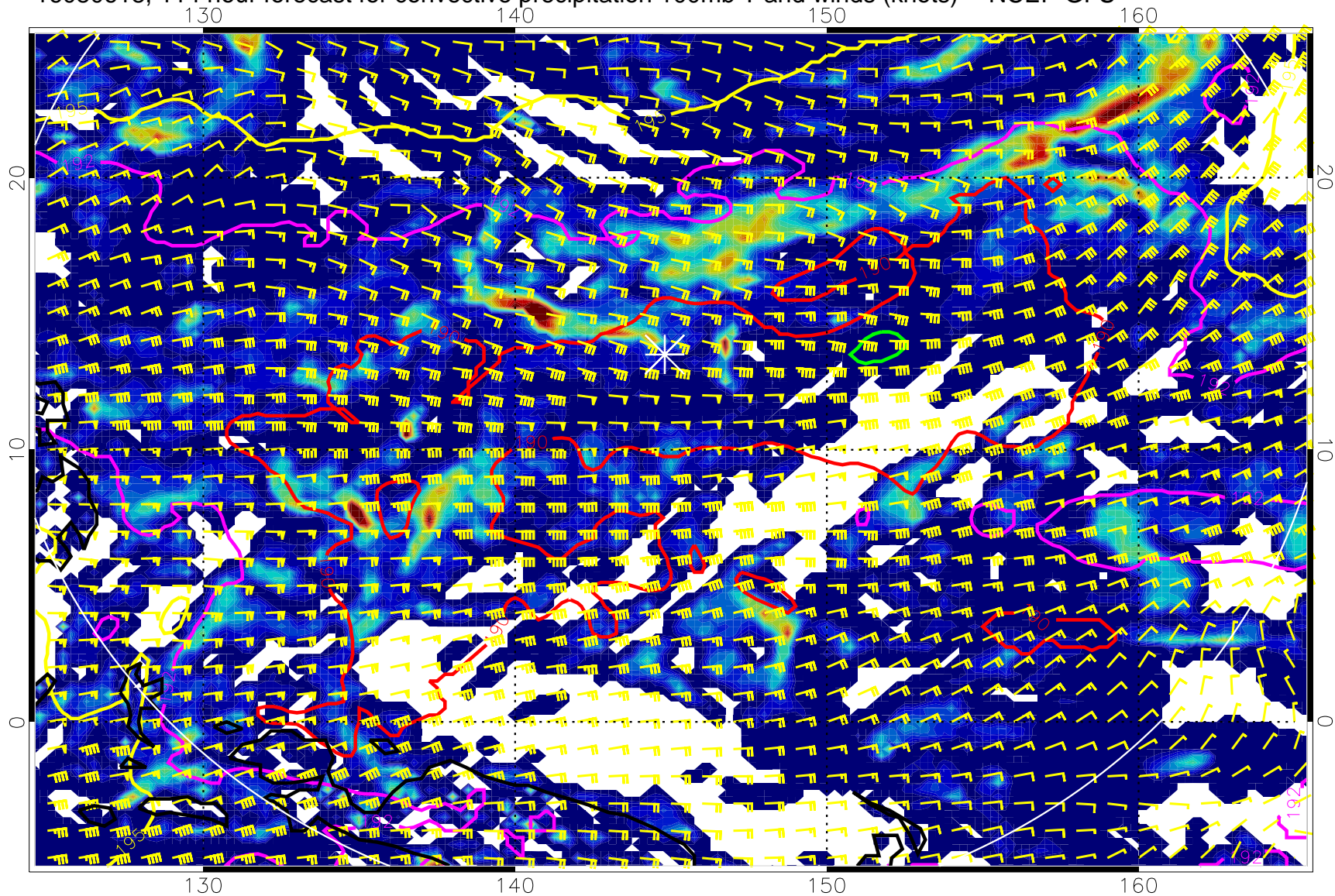
16080618, 114 hour forecast for convective precipitation 100mb T and winds (knots) -- NCEP GFS
