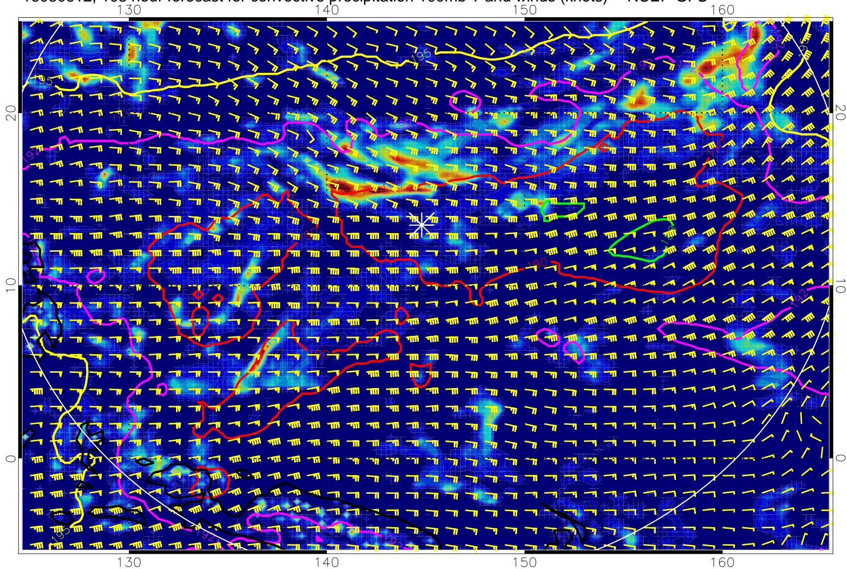
16080612, 108 hour forecast for convective precipitation 100mb T and winds (knots) -- NCEP GFS
