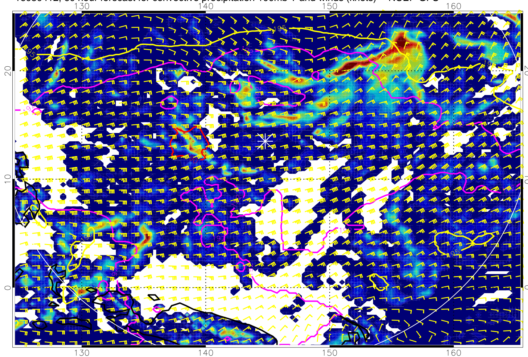
16080412, 60 hour forecast for convective precipitation 100mb T and winds (knots) -- NCEP GFS
