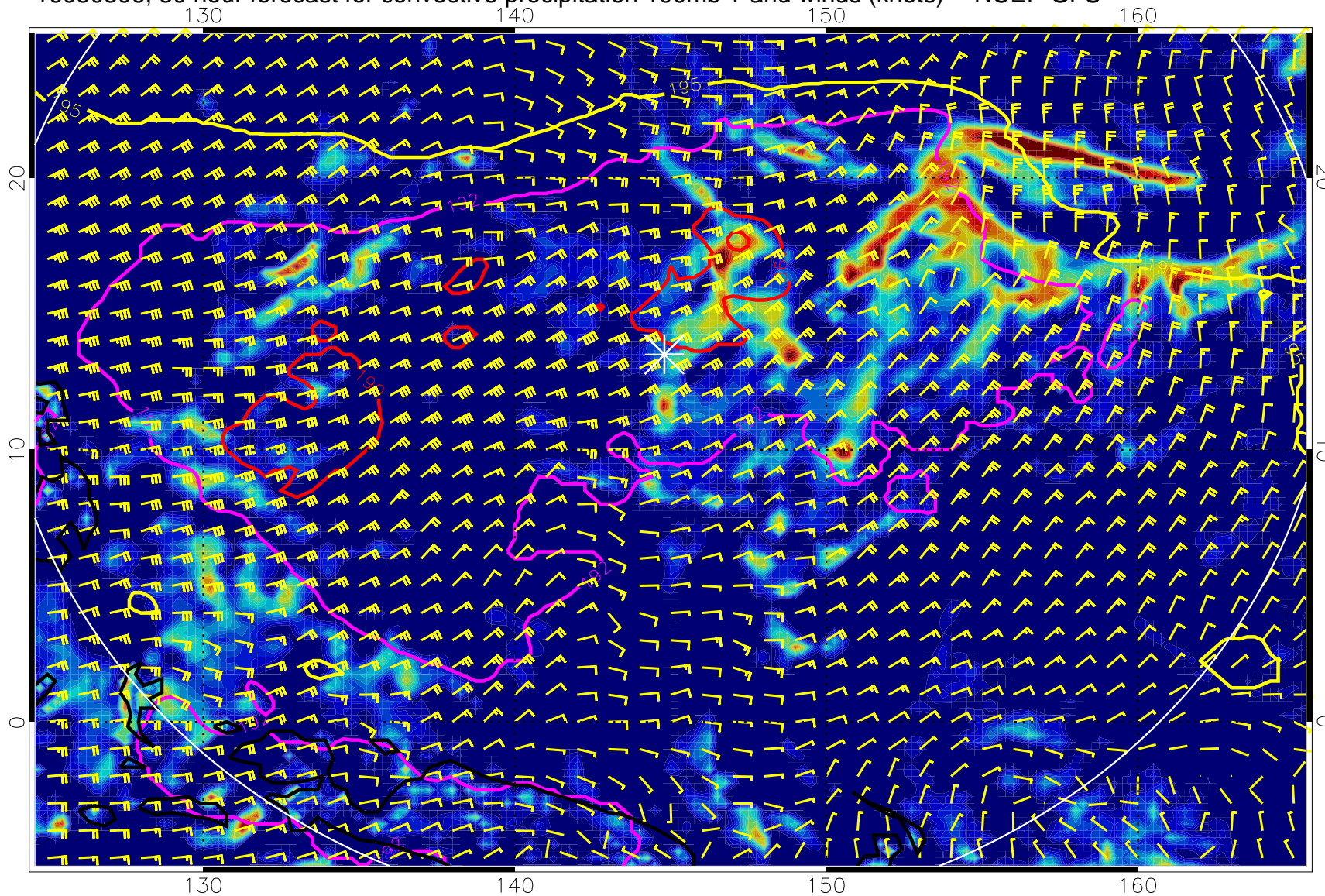
16080306, 30 hour forecast for convective precipitation 100mb T and winds (knots) -- NCEP GFS
