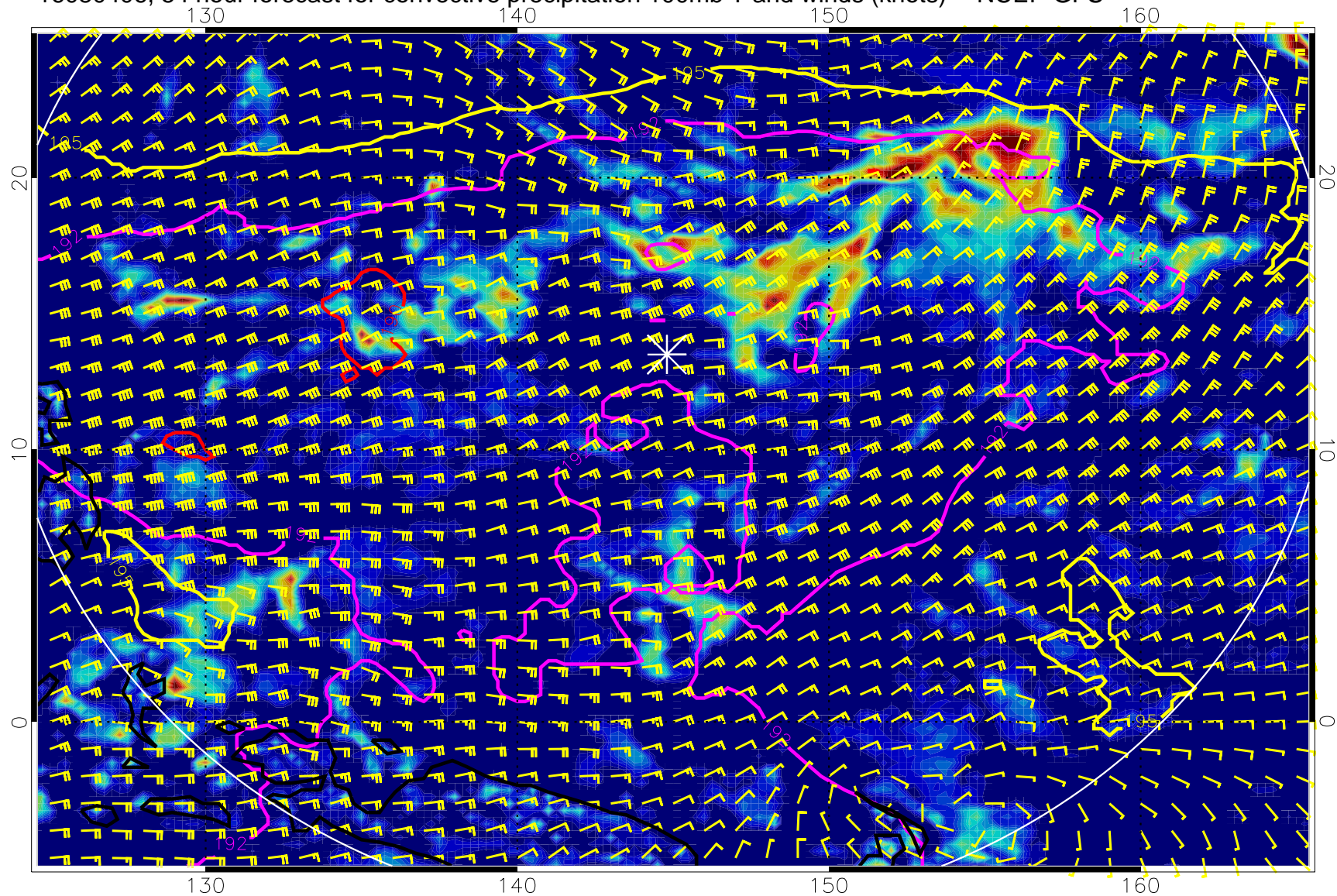
16080406, 54 hour forecast for convective precipitation 100mb T and winds (knots) -- NCEP GFS
