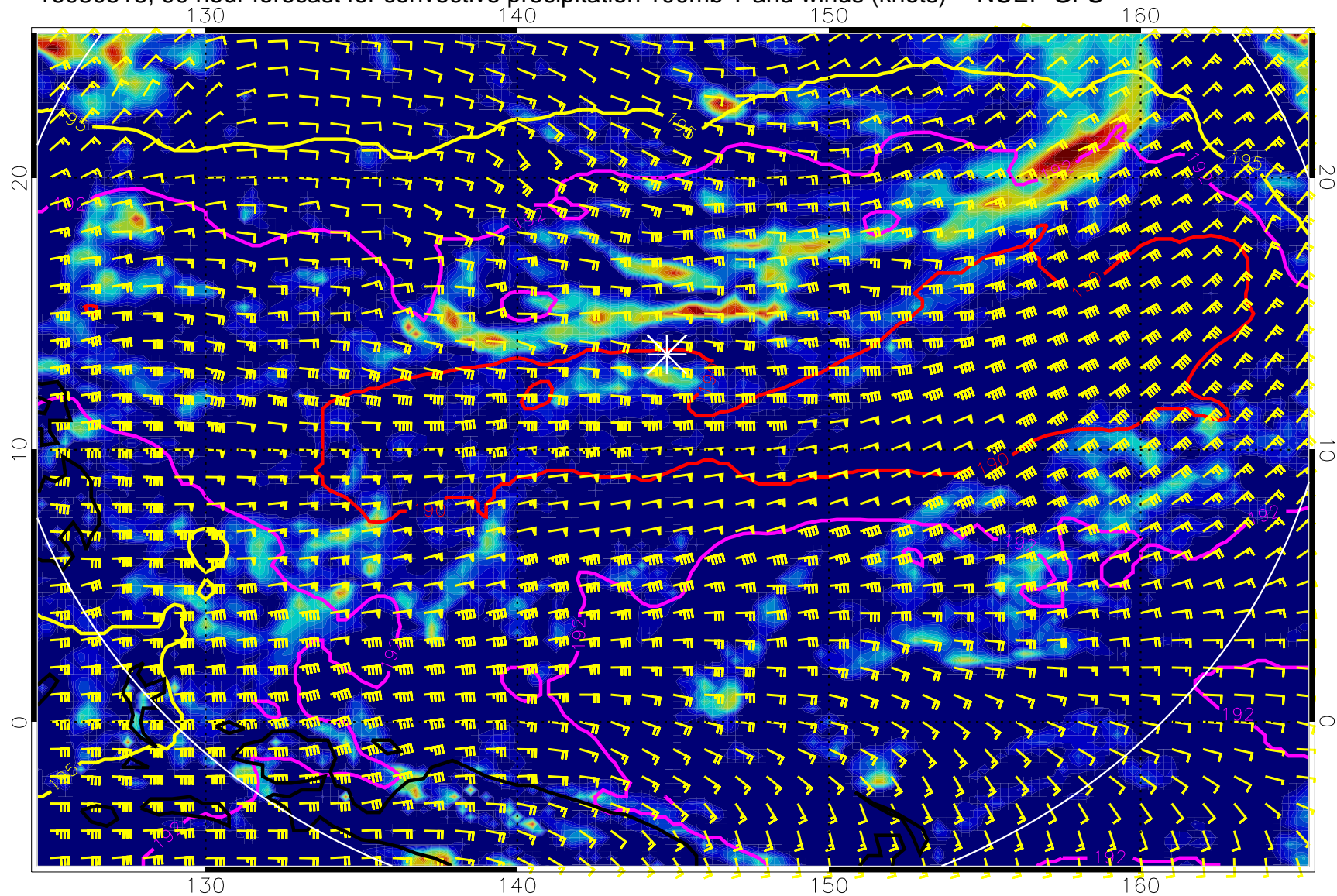
16080518, 90 hour forecast for convective precipitation 100mb T and winds (knots) -- NCEP GFS
