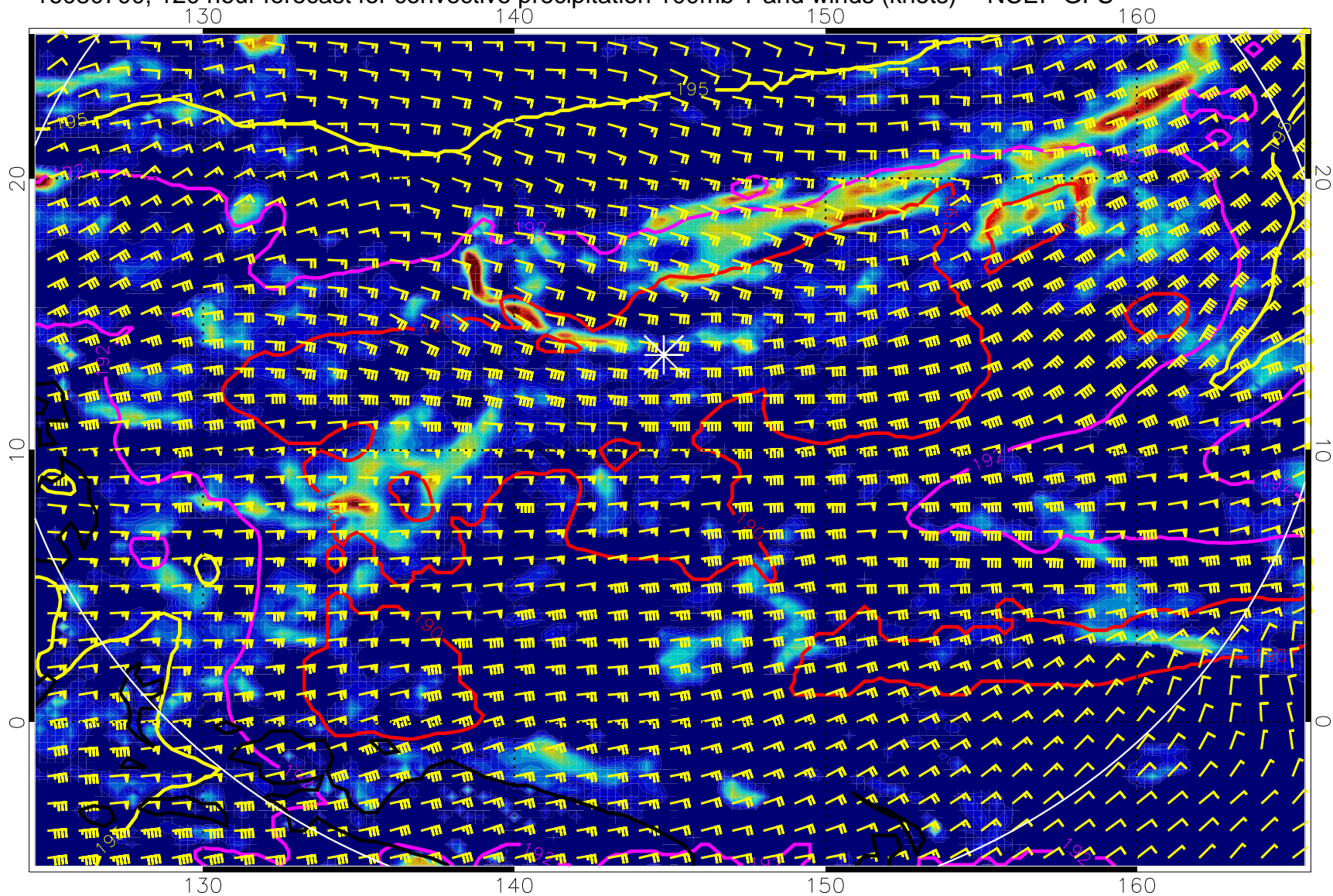
16080700, 120 hour forecast for convective precipitation 100mb T and winds (knots) -- NCEP GFS
