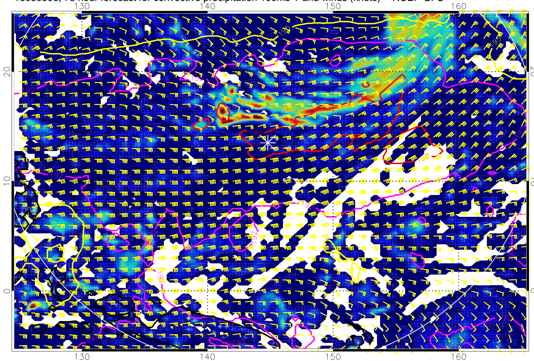
16080506, 78 hour forecast for convective precipitation 100mb T and winds (knots) -- NCEP GFS
