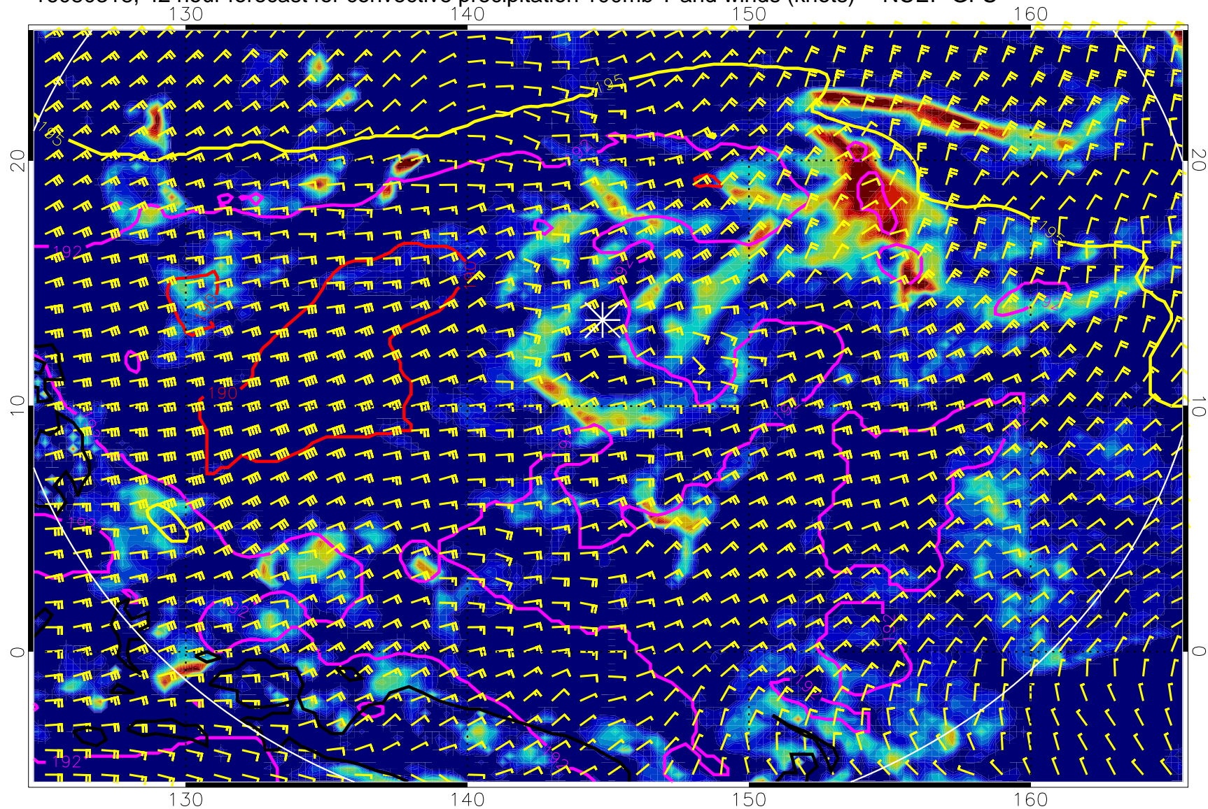
16080318, 42 hour forecast for convective precipitation 100mb T and winds (knots) -- NCEP GFS
