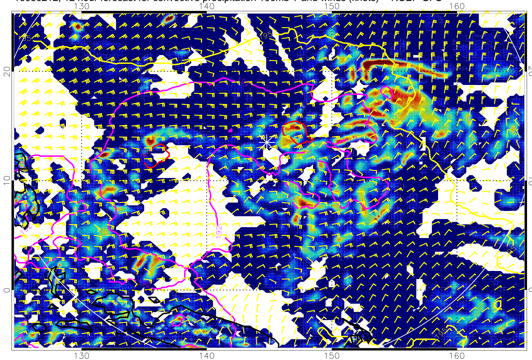
16080212, 12 hour forecast for convective precipitation 100mb T and winds (knots) -- NCEP GFS
