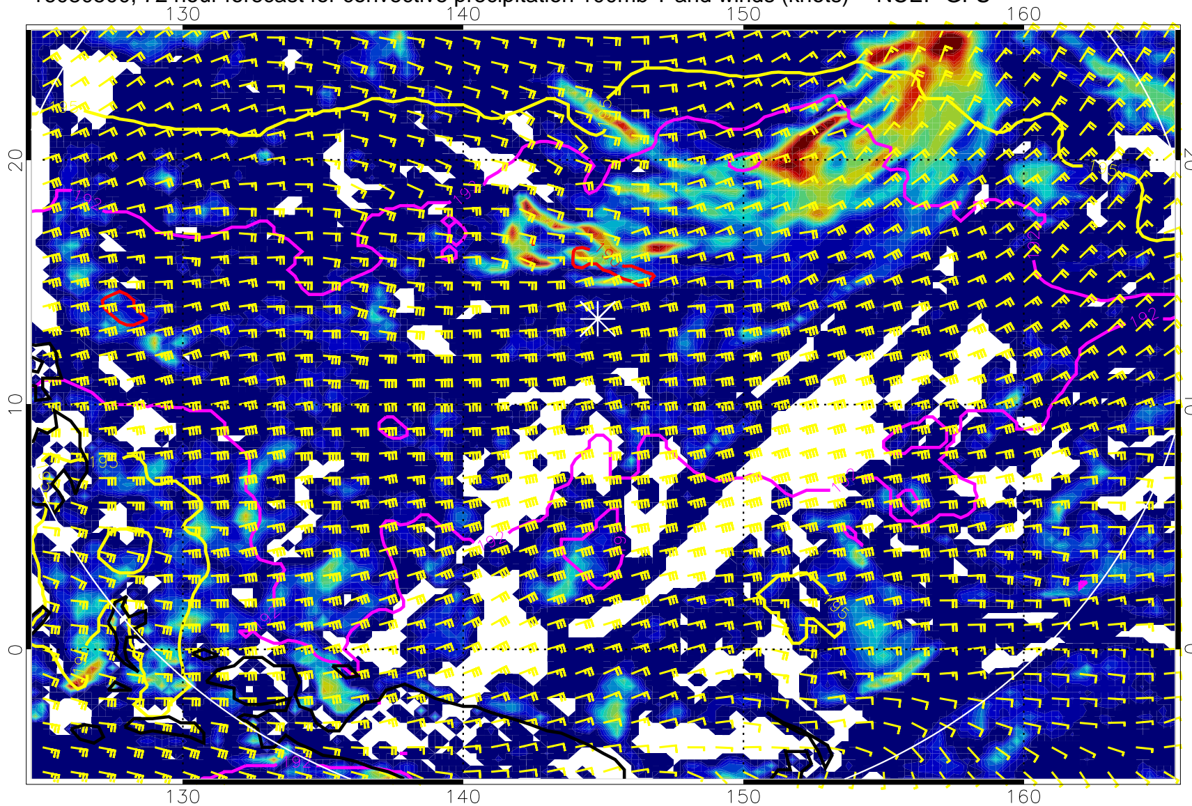
16080500, 72 hour forecast for convective precipitation 100mb T and winds (knots) -- NCEP GFS
