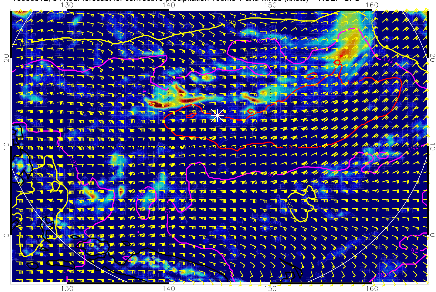
16080512, 84 hour forecast for convective precipitation 100mb T and winds (knots) -- NCEP GFS
