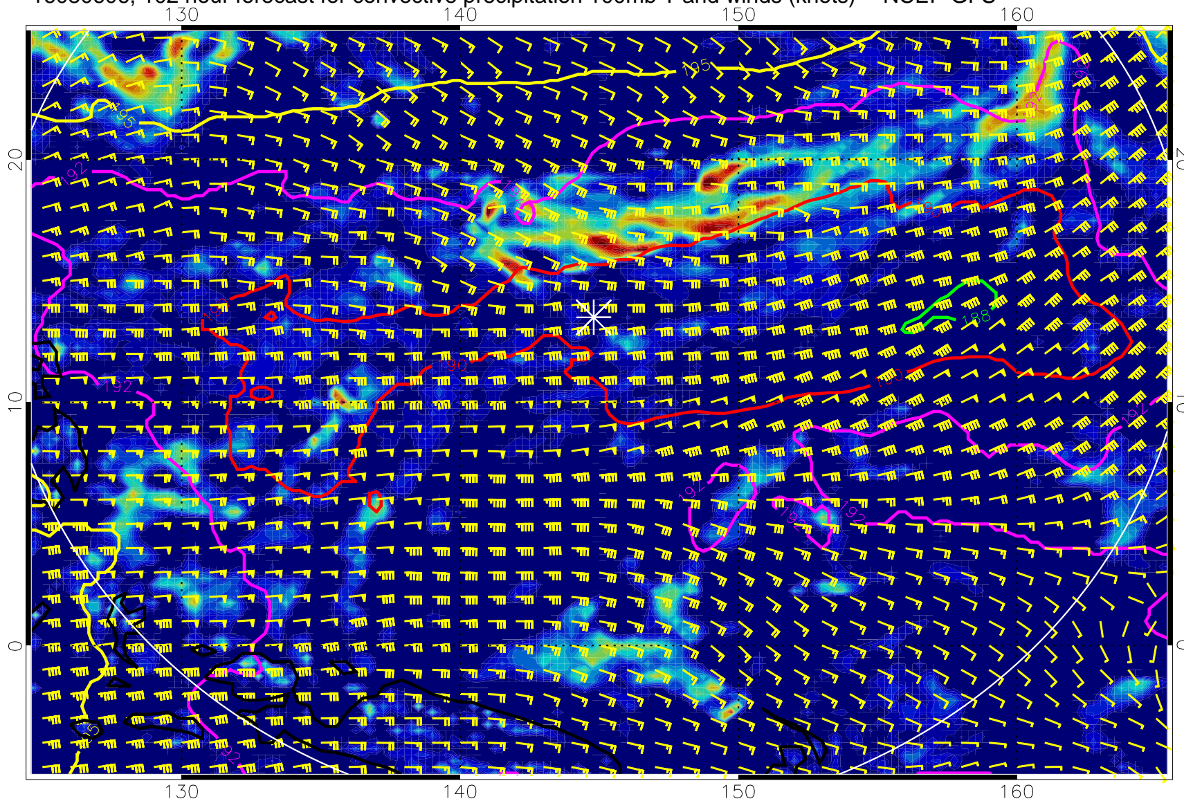
16080606, 102 hour forecast for convective precipitation 100mb T and winds (knots) -- NCEP GFS
