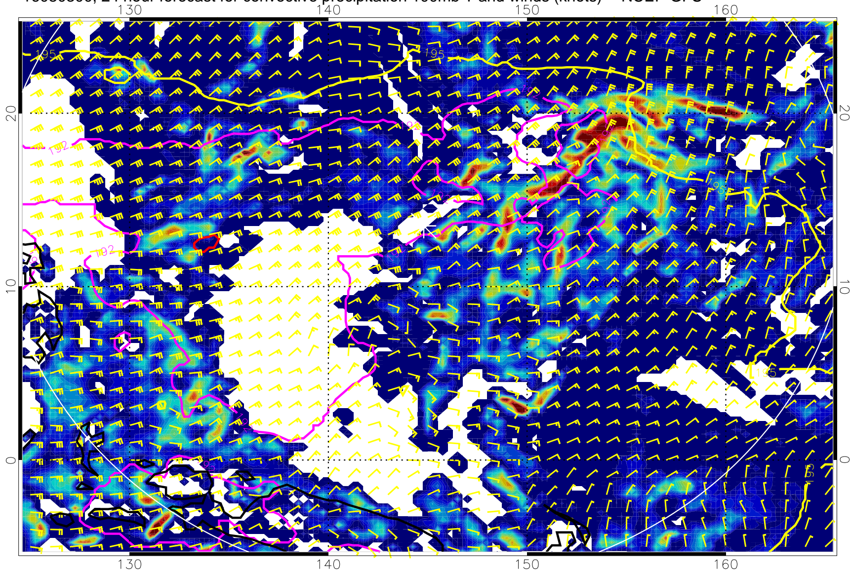
16080300, 24 hour forecast for convective precipitation 100mb T and winds (knots) -- NCEP GFS
