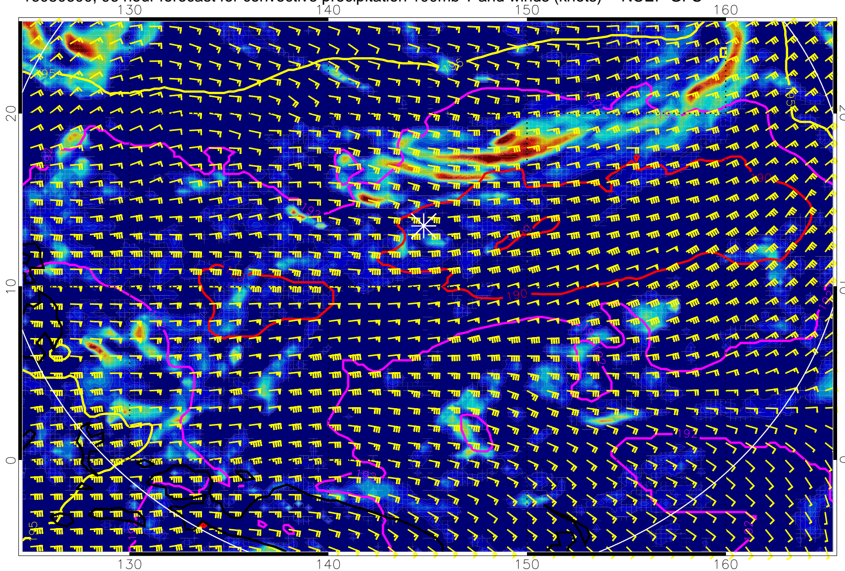
16080600, 96 hour forecast for convective precipitation 100mb T and winds (knots) -- NCEP GFS
