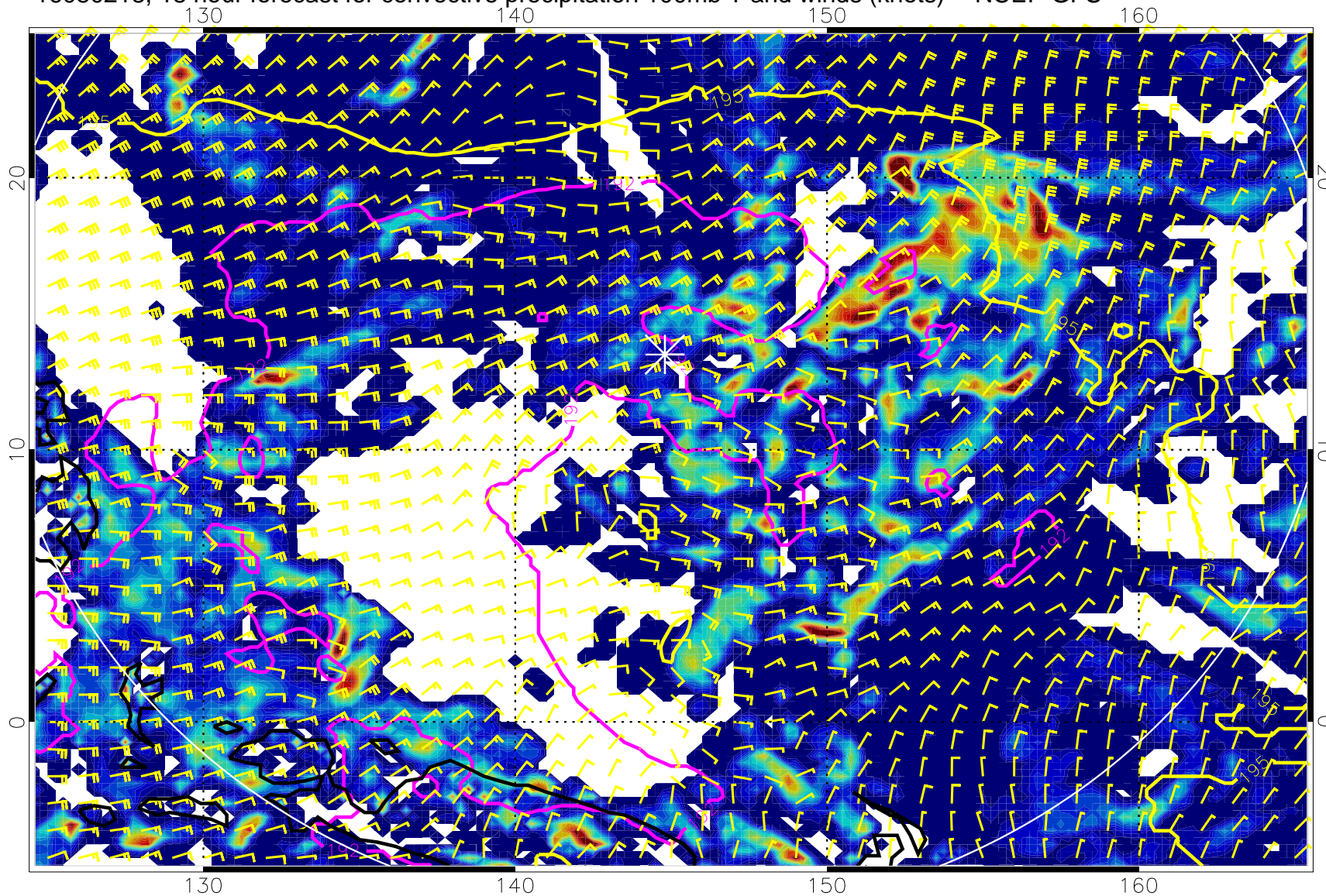
16080218, 18 hour forecast for convective precipitation 100mb T and winds (knots) -- NCEP GFS
