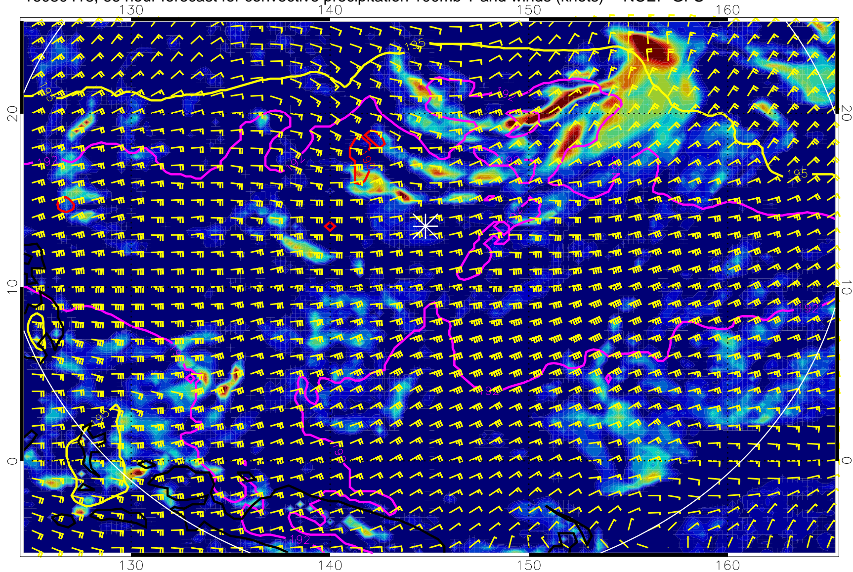
16080418, 66 hour forecast for convective precipitation 100mb T and winds (knots) -- NCEP GFS
