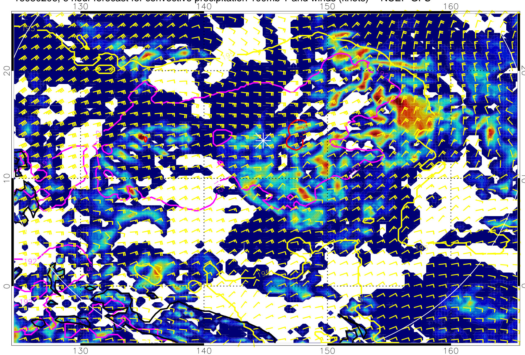
16080206, 6 hour forecast for convective precipitation 100mb T and winds (knots) -- NCEP GFS
