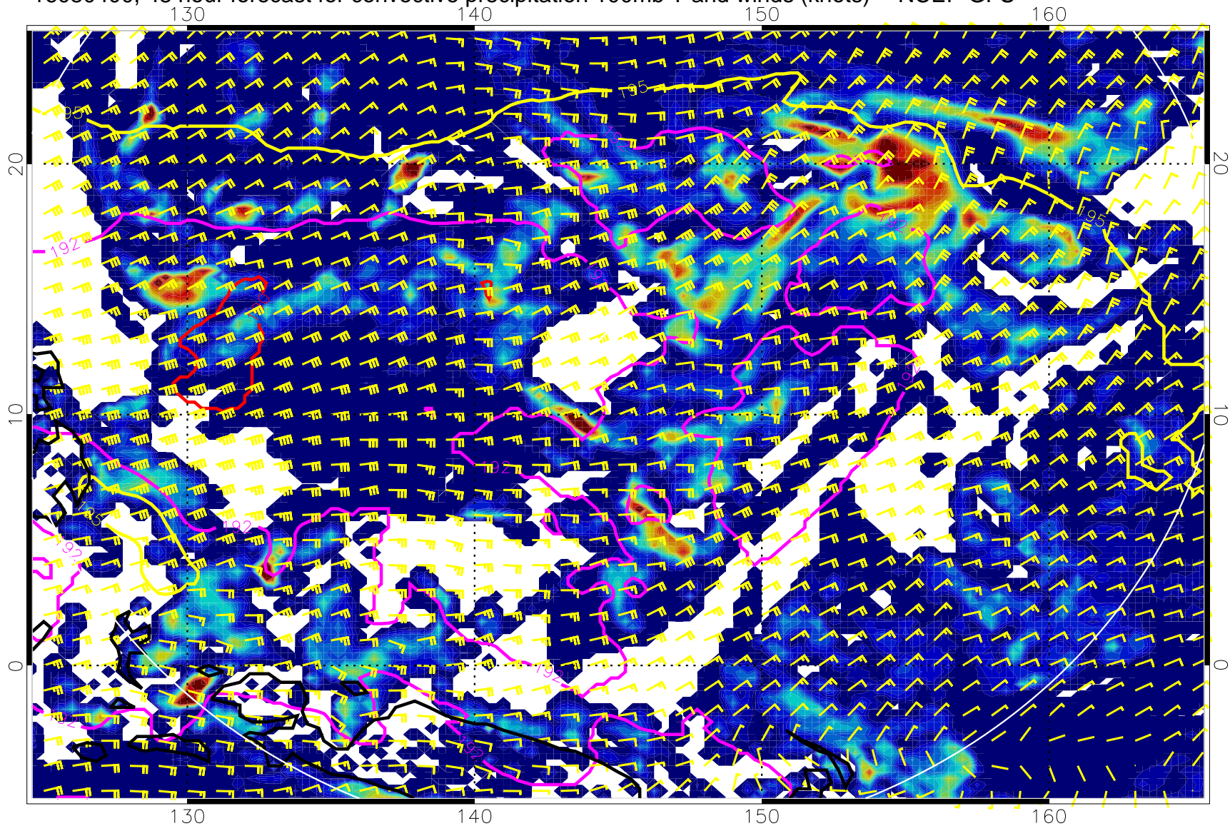
16080400, 48 hour forecast for convective precipitation 100mb T and winds (knots) -- NCEP GFS
