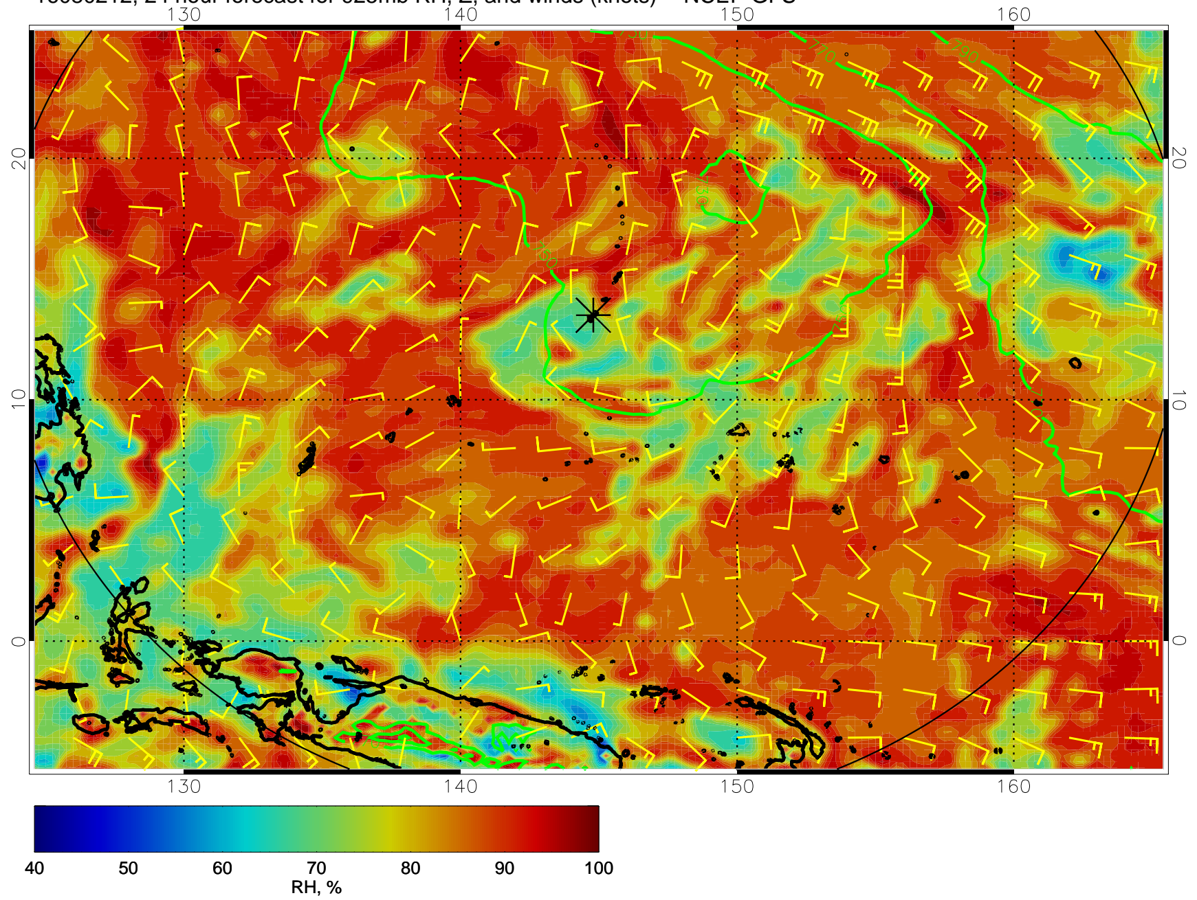
16080212, 24 hour forecast for 925mb RH, Z, and winds (knots) -- NCEP GFS
