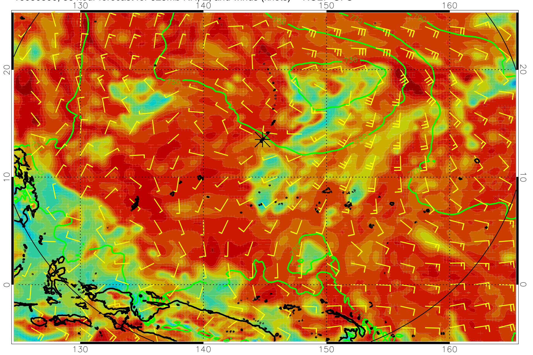
16080300, 36 hour forecast for 925mb RH, Z, and winds (knots) -- NCEP GFS
