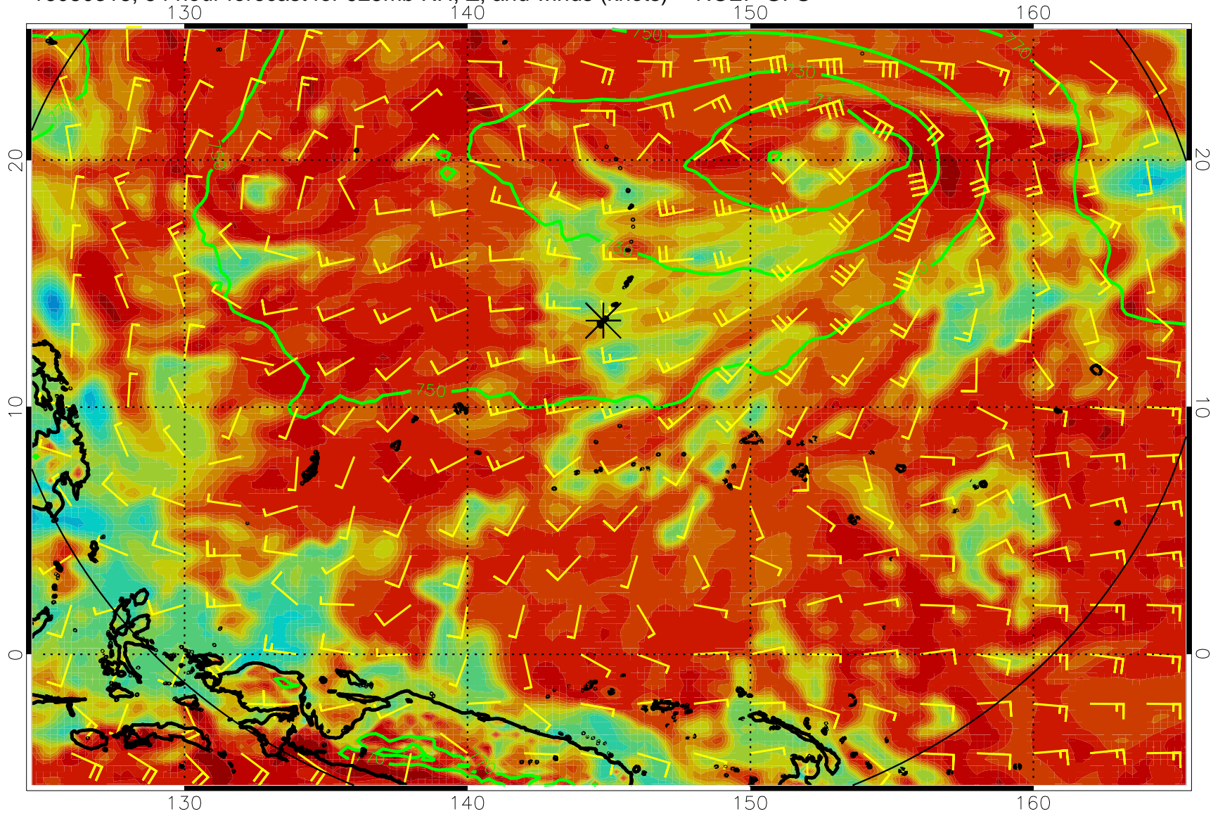
16080318, 54 hour forecast for 925mb RH, Z, and winds (knots) -- NCEP GFS
