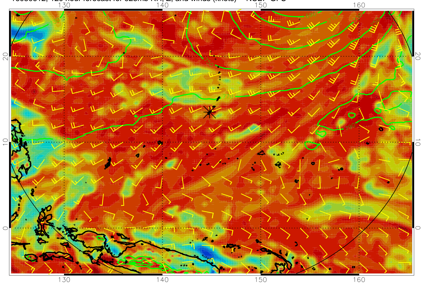
16080612, 120 hour forecast for 925mb RH, Z, and winds (knots) -- NCEP GFS
