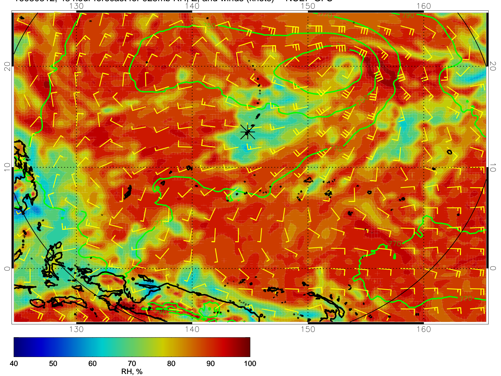
16080312, 48 hour forecast for 925mb RH, Z, and winds (knots) -- NCEP GFS
