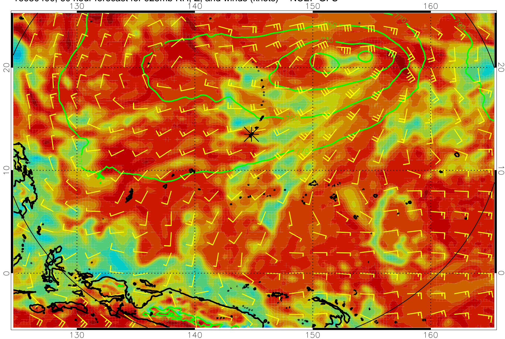
16080400, 60 hour forecast for 925mb RH, Z, and winds (knots) -- NCEP GFS
