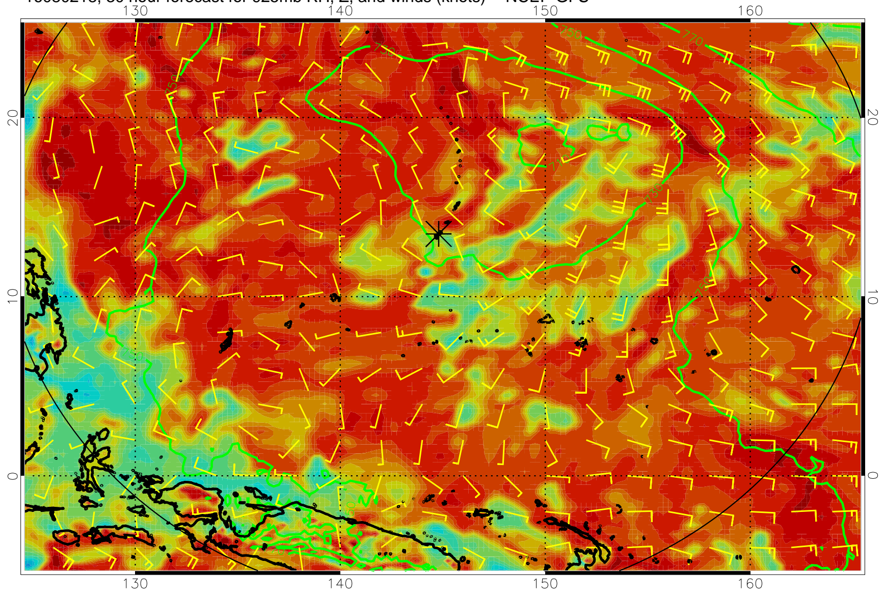
16080218, 30 hour forecast for 925mb RH, Z, and winds (knots) -- NCEP GFS
