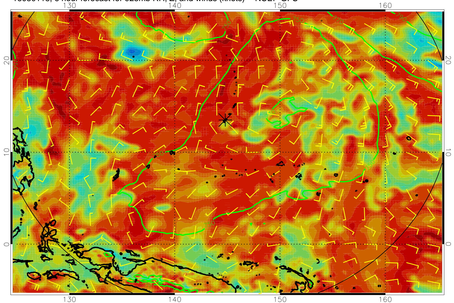
16080118, 6 hour forecast for 925mb RH, Z, and winds (knots) -- NCEP GFS
