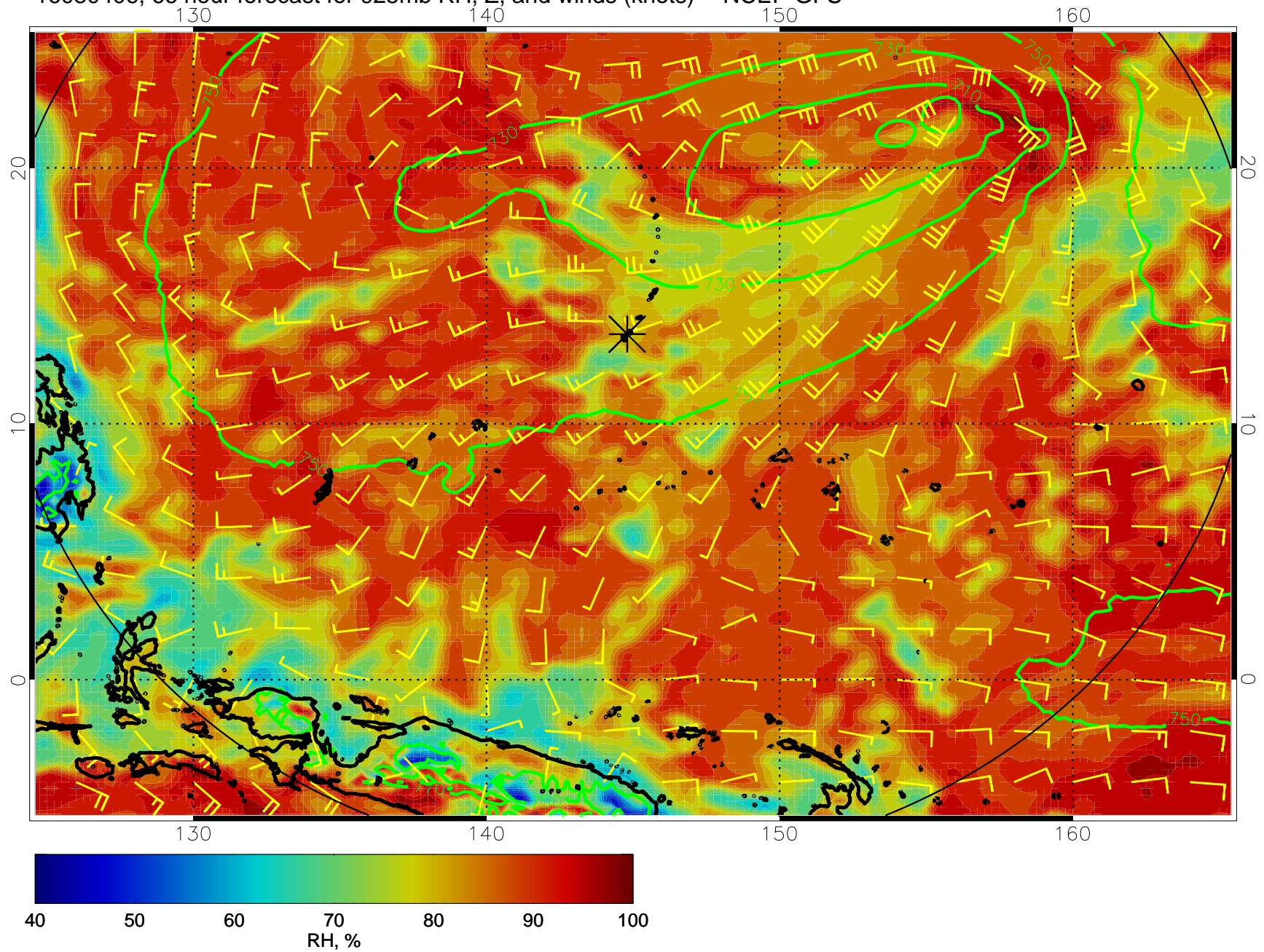
16080406, 66 hour forecast for 925mb RH, Z, and winds (knots) -- NCEP GFS
