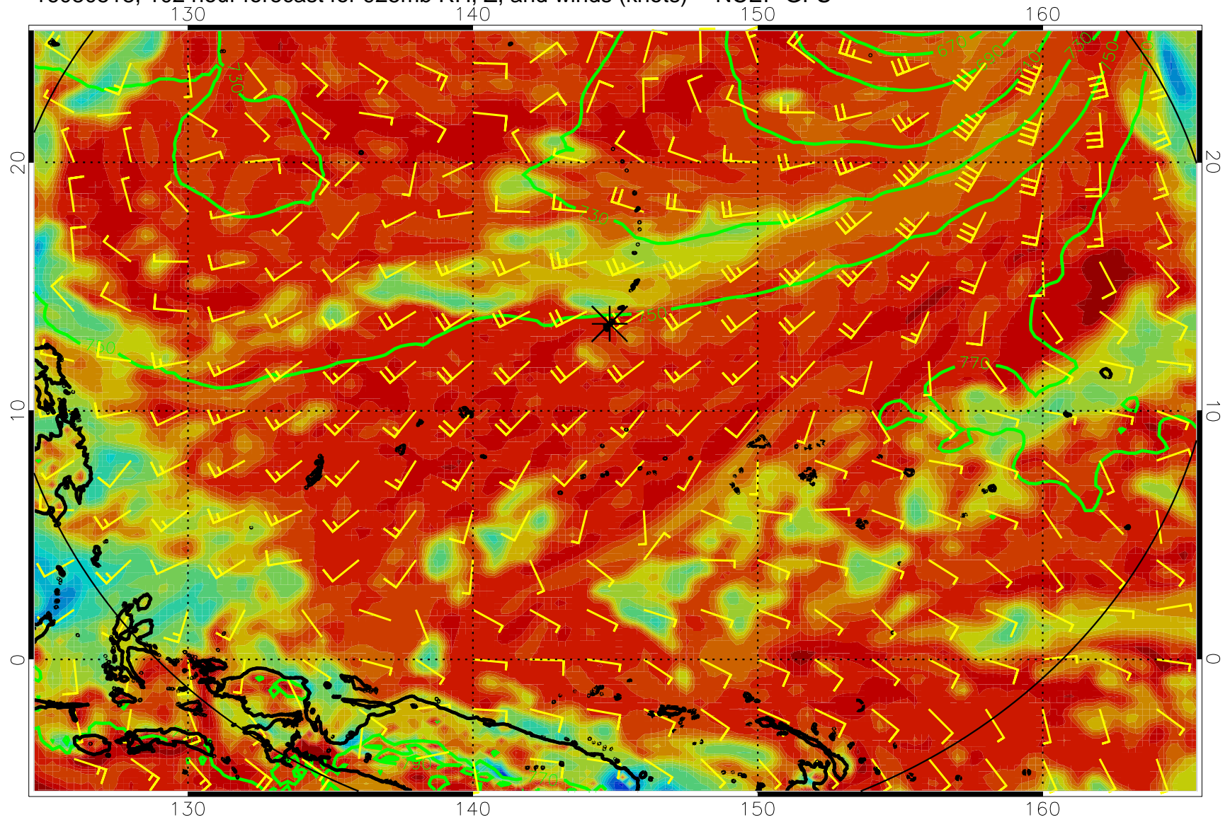
16080518, 102 hour forecast for 925mb RH, Z, and winds (knots) -- NCEP GFS
