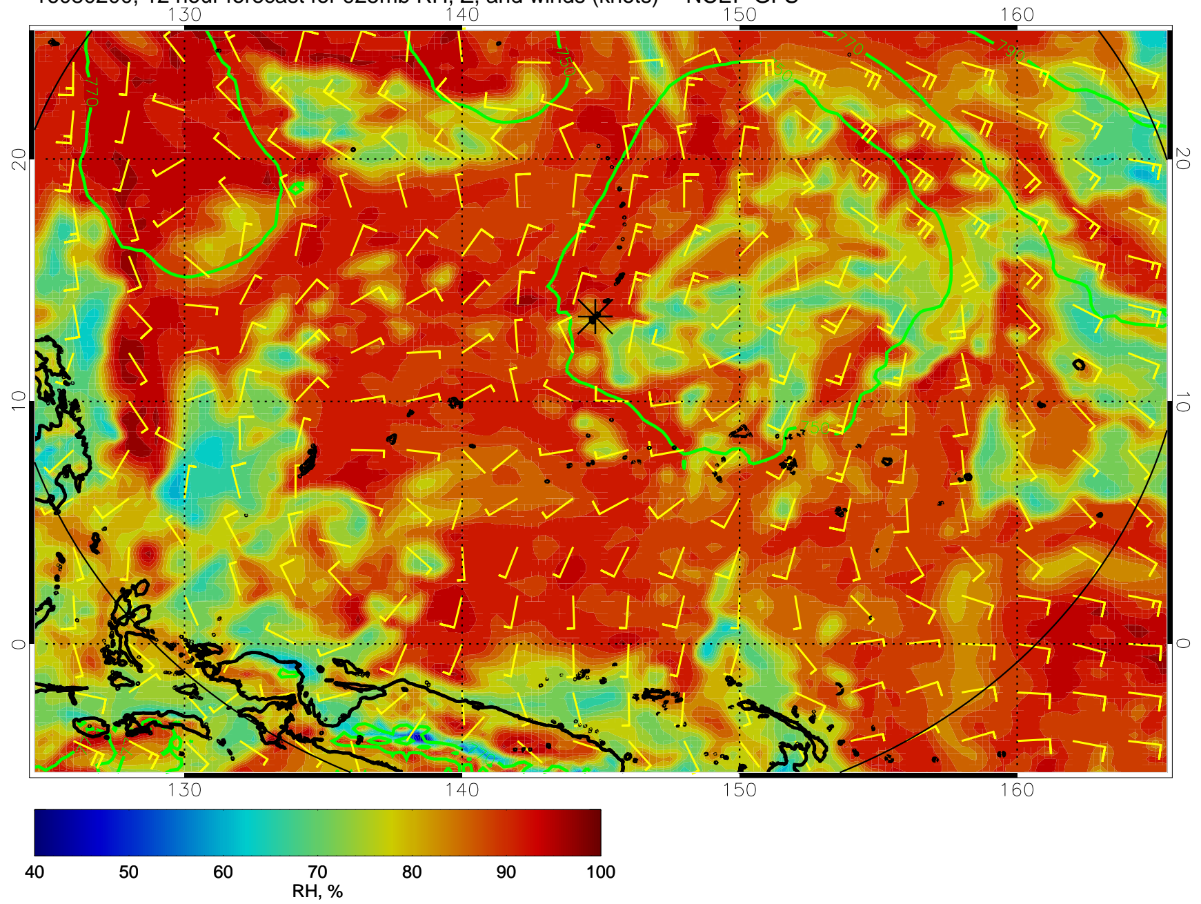
16080200, 12 hour forecast for 925mb RH, Z, and winds (knots) -- NCEP GFS
