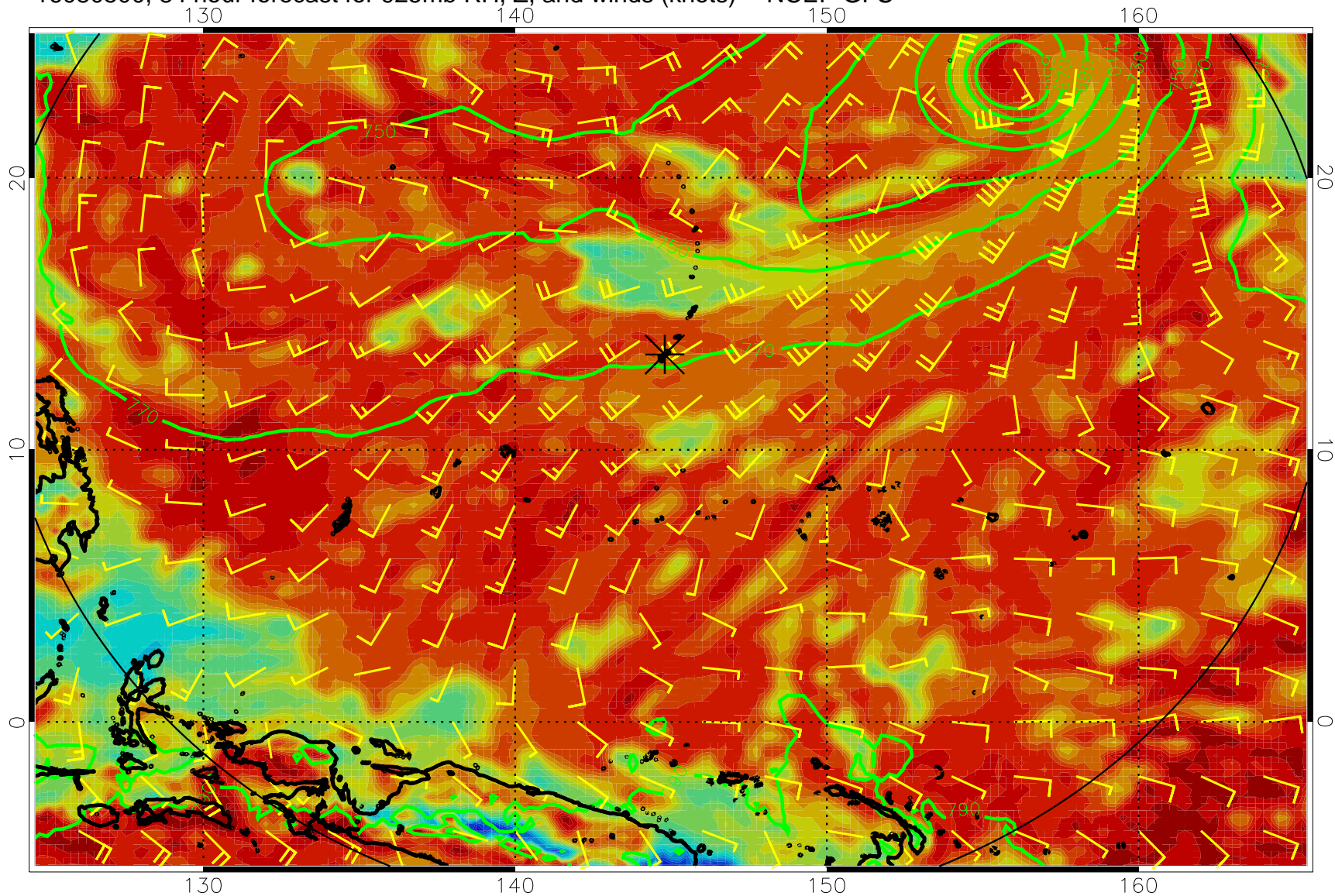
16080500, 84 hour forecast for 925mb RH, Z, and winds (knots) -- NCEP GFS
