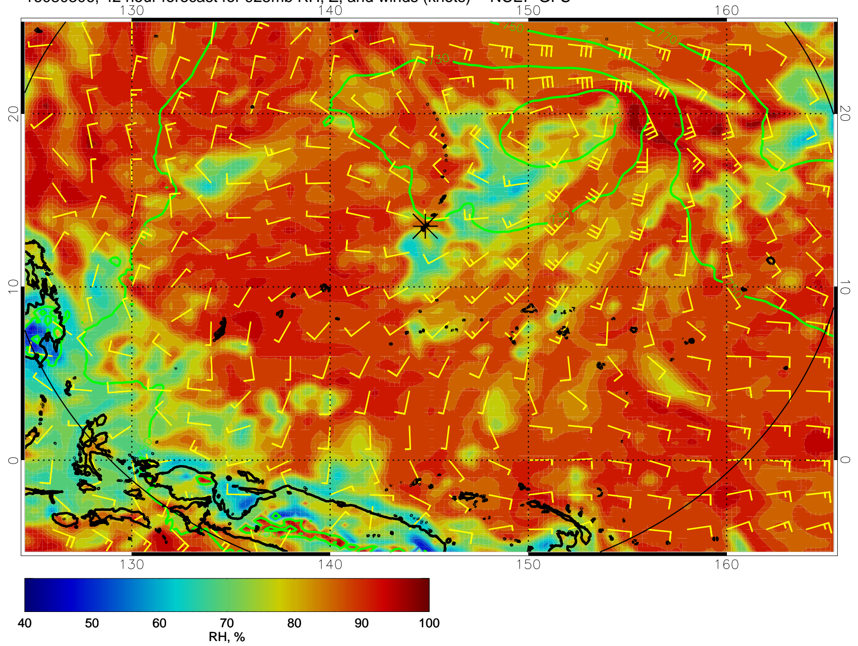
16080306, 42 hour forecast for 925mb RH, Z, and winds (knots) -- NCEP GFS
