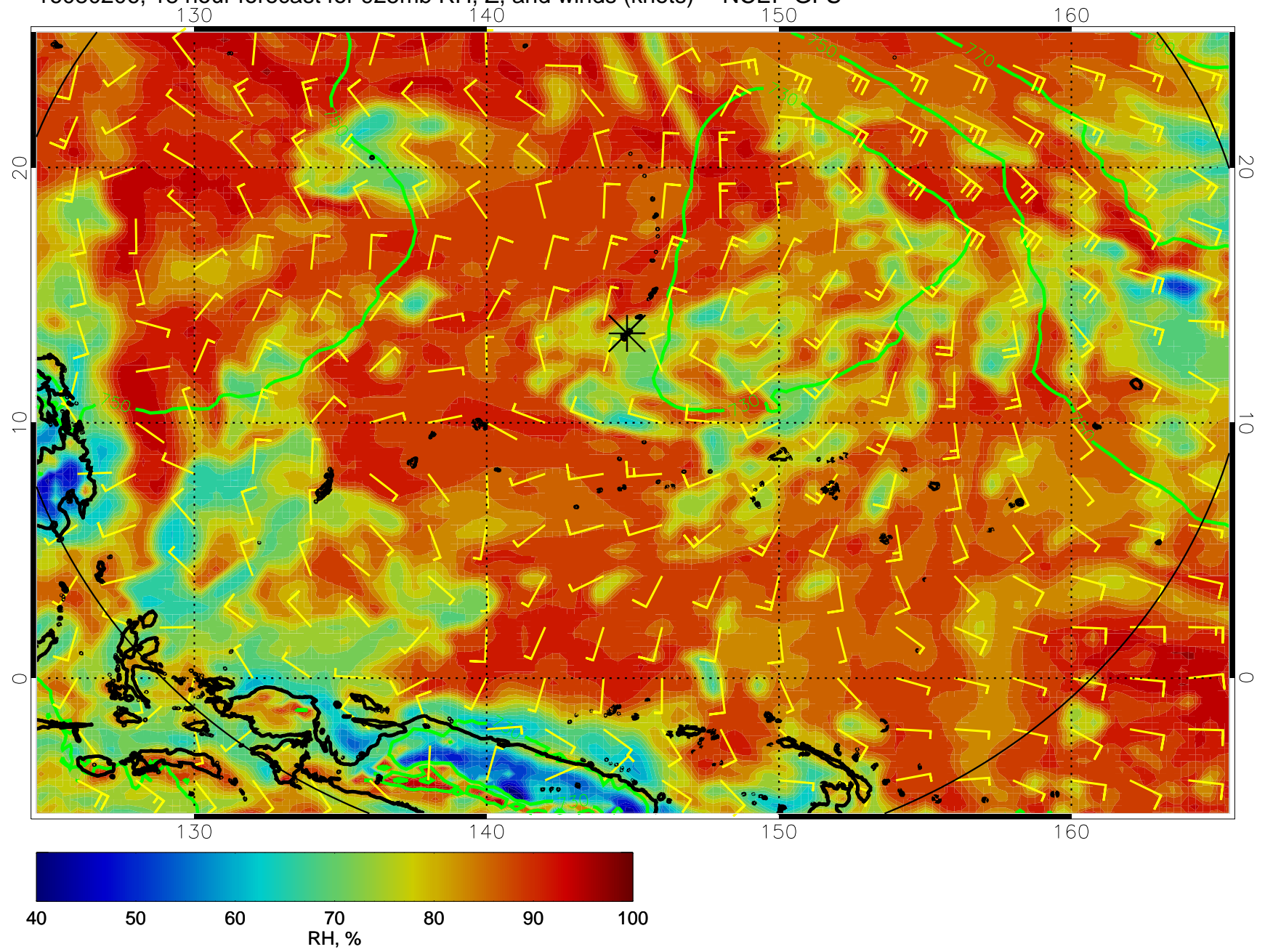
16080206, 18 hour forecast for 925mb RH, Z, and winds (knots) -- NCEP GFS
