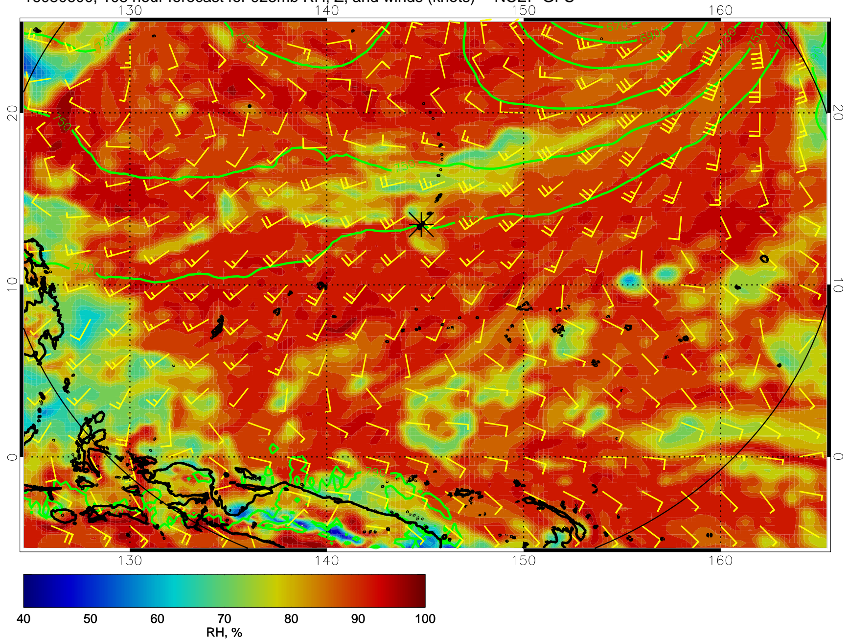
16080600, 108 hour forecast for 925mb RH, Z, and winds (knots) -- NCEP GFS
