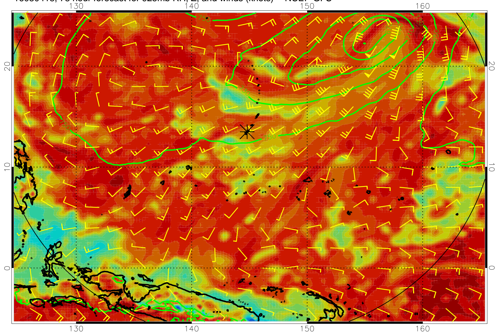
16080418, 78 hour forecast for 925mb RH, Z, and winds (knots) -- NCEP GFS
