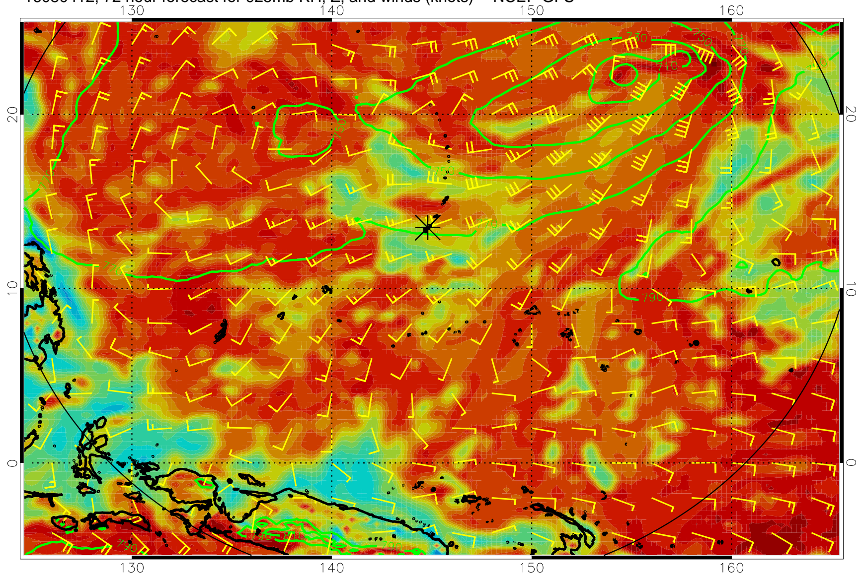
16080412, 72 hour forecast for 925mb RH, Z, and winds (knots) -- NCEP GFS
