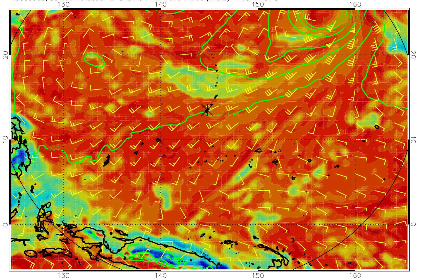
16080506, 90 hour forecast for 925mb RH, Z, and winds (knots) -- NCEP GFS
