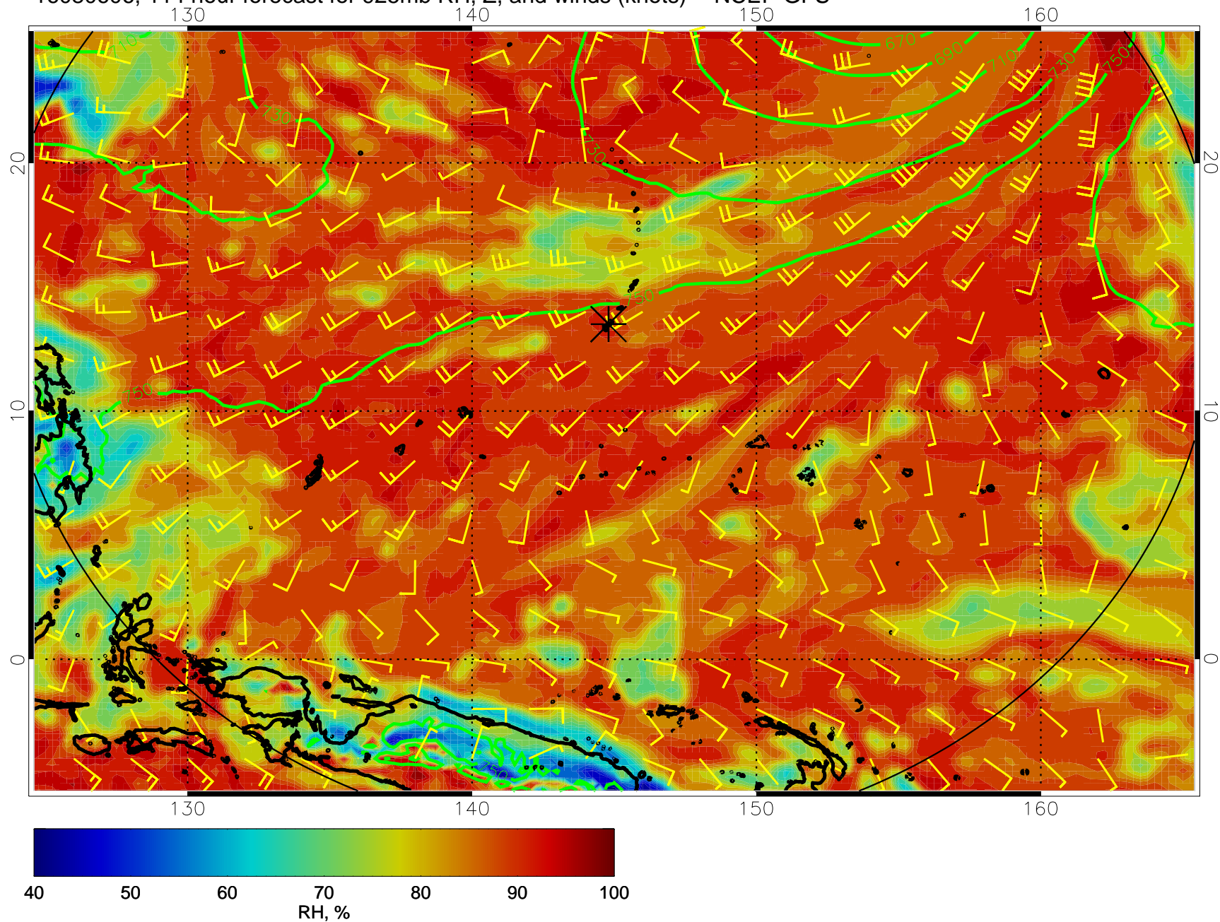
16080606, 114 hour forecast for 925mb RH, Z, and winds (knots) -- NCEP GFS
