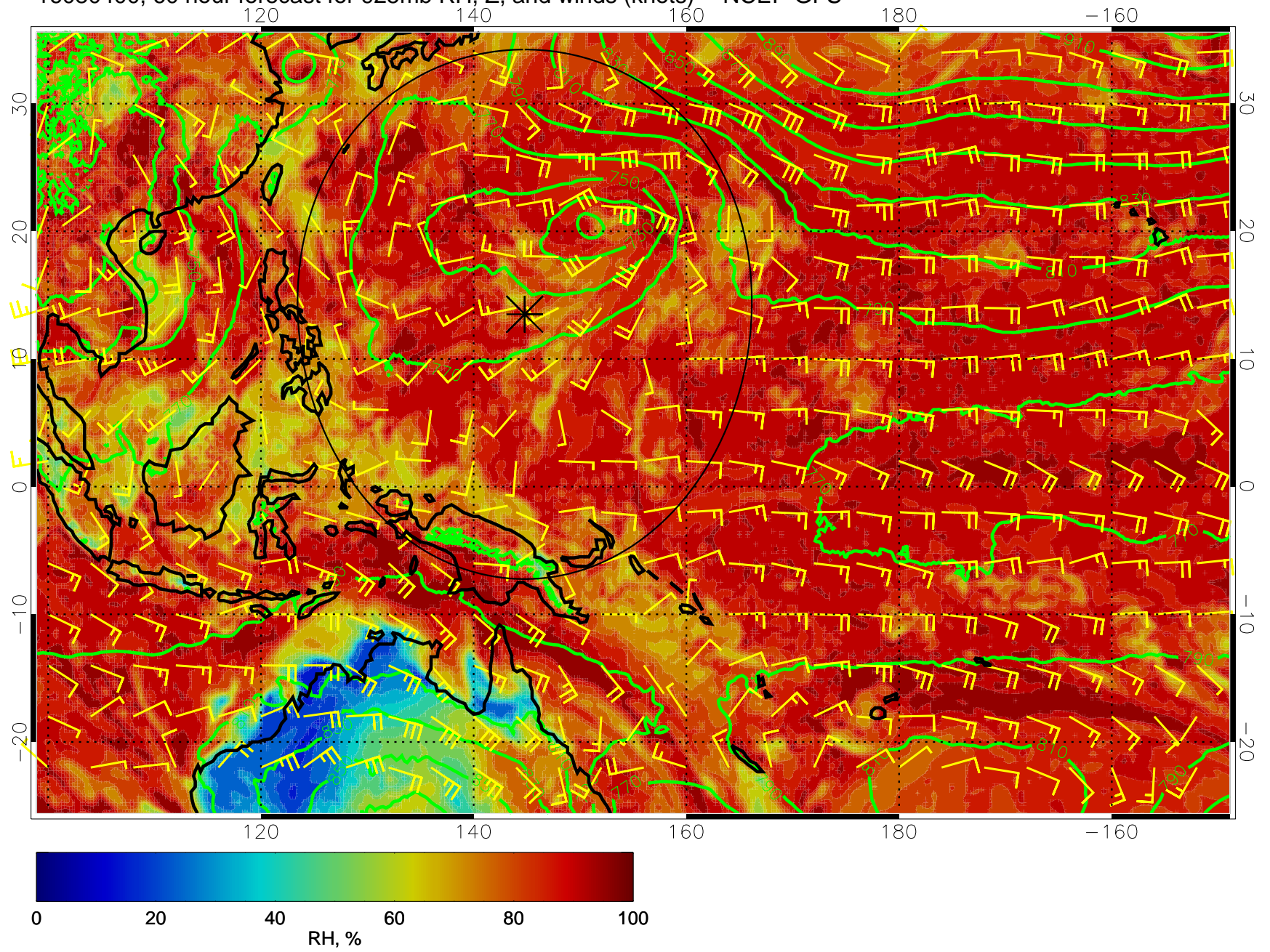
16080400, 60 hour forecast for 925mb RH, Z, and winds (knots) -- NCEP GFS
