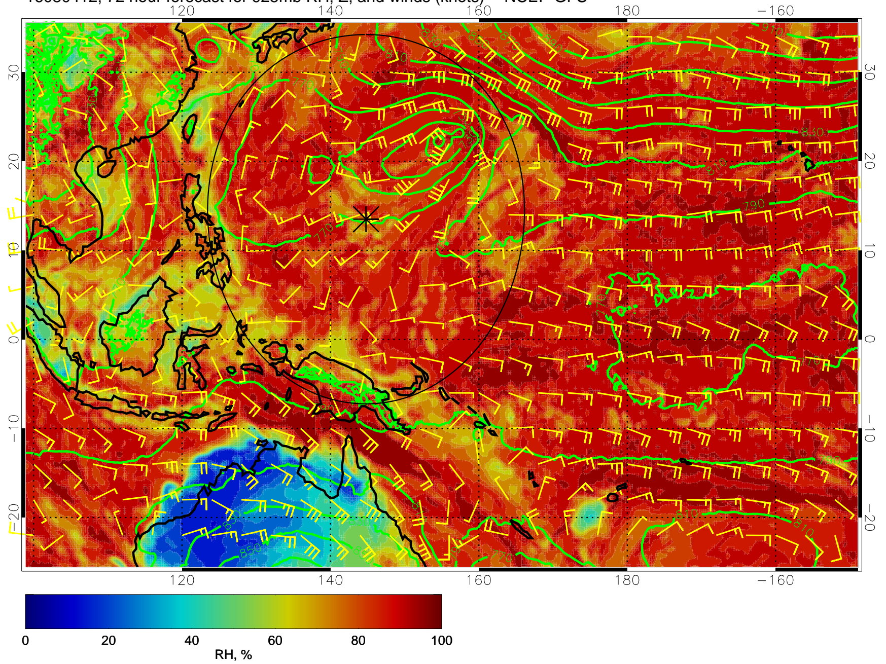
16080412, 72 hour forecast for 925mb RH, Z, and winds (knots) -- NCEP GFS
