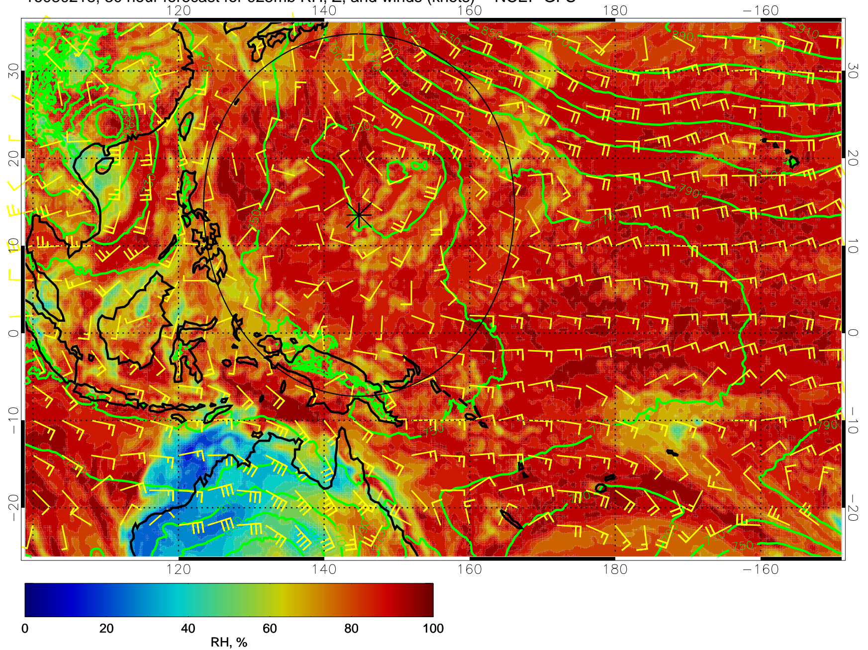
16080218, 30 hour forecast for 925mb RH, Z, and winds (knots) -- NCEP GFS
