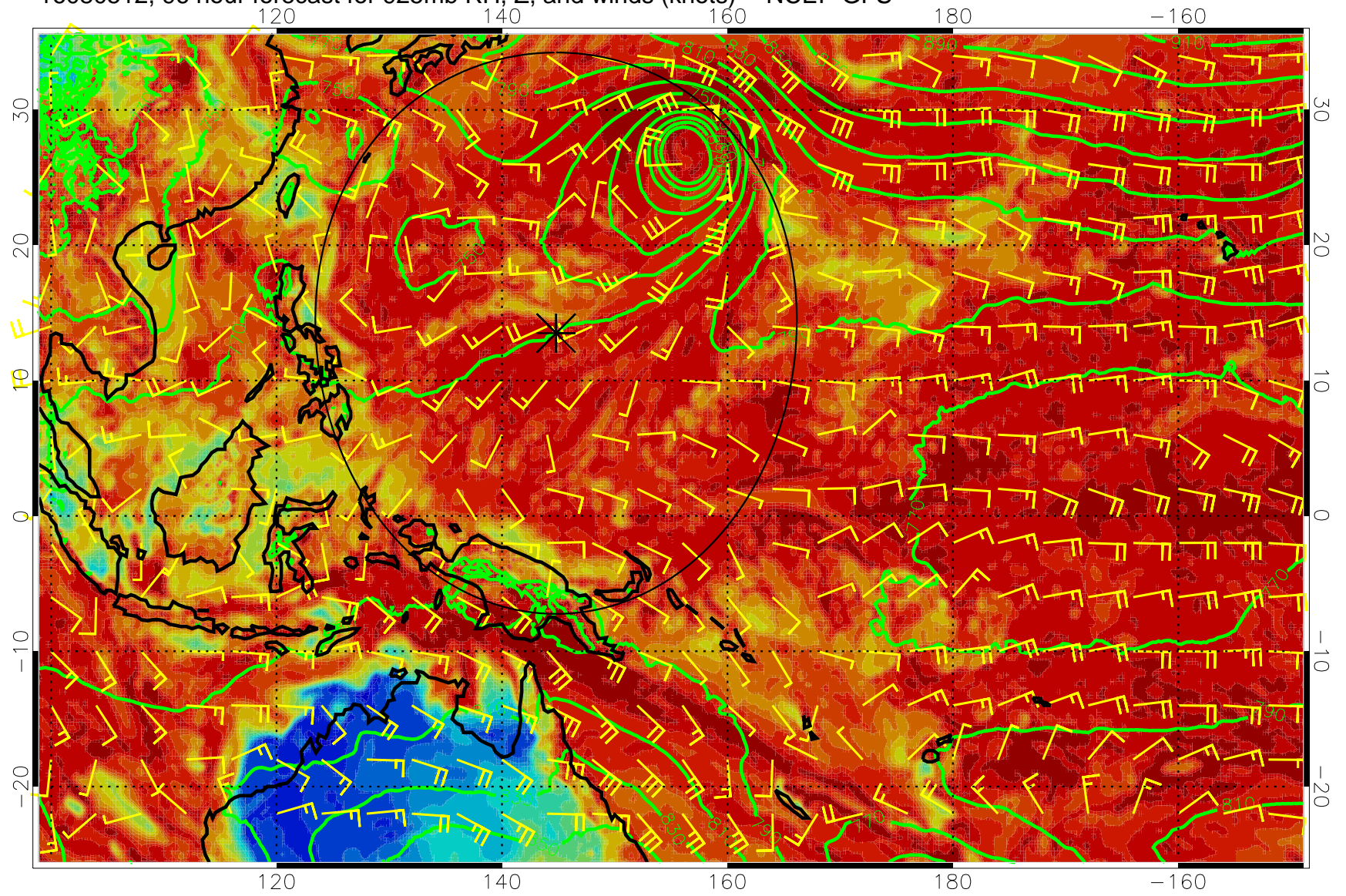
16080512, 96 hour forecast for 925mb RH, Z, and winds (knots) -- NCEP GFS
