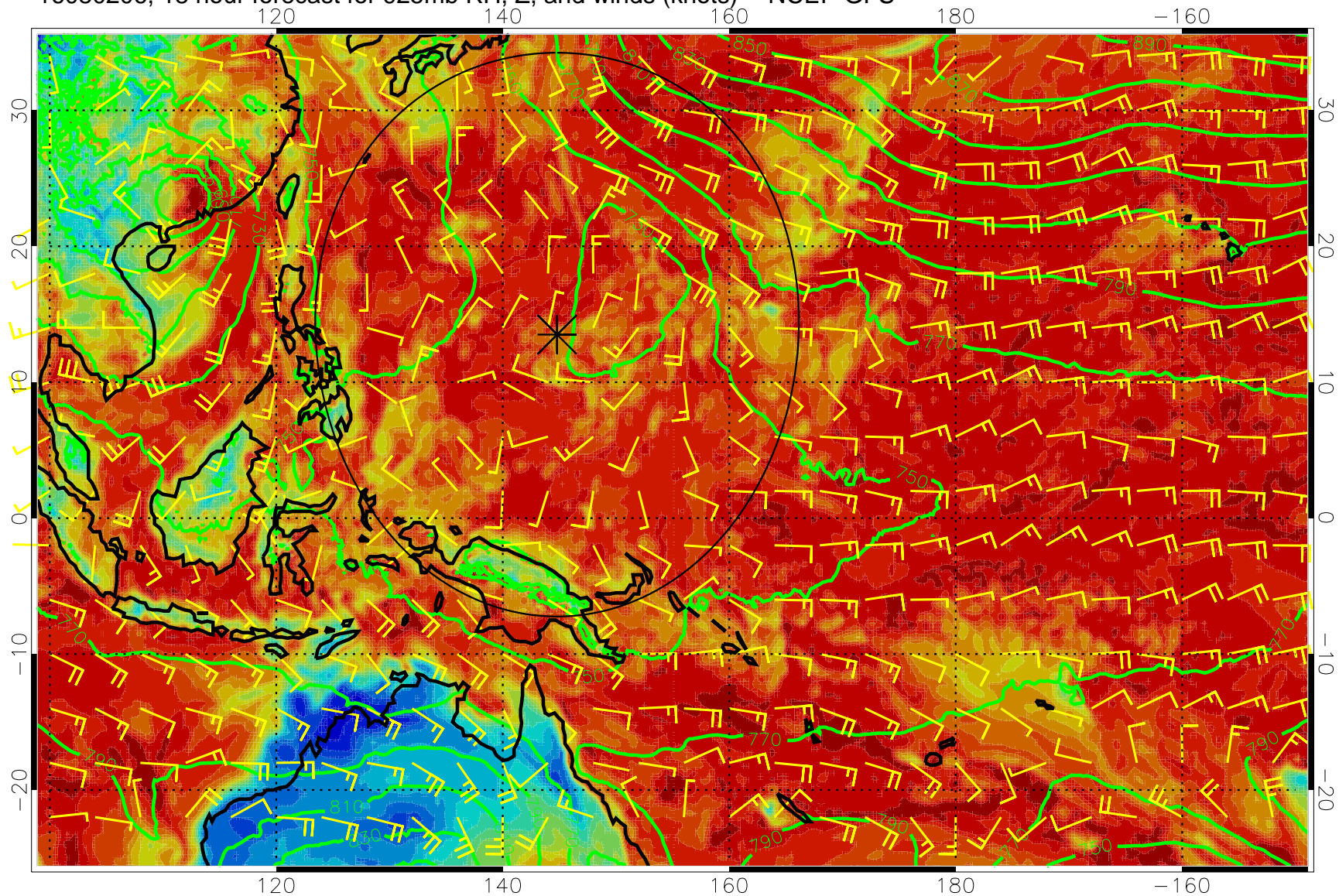
16080206, 18 hour forecast for 925mb RH, Z, and winds (knots) -- NCEP GFS
