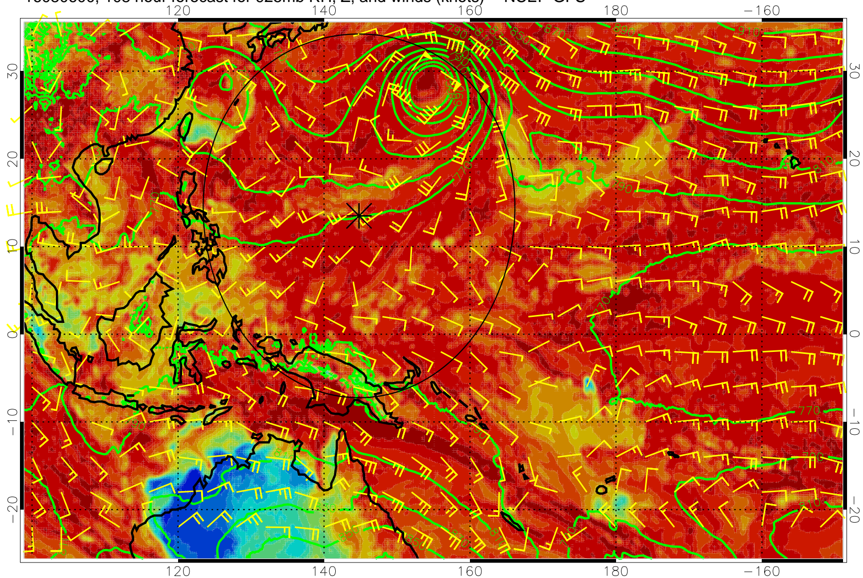
16080600, 108 hour forecast for 925mb RH, Z, and winds (knots) -- NCEP GFS
