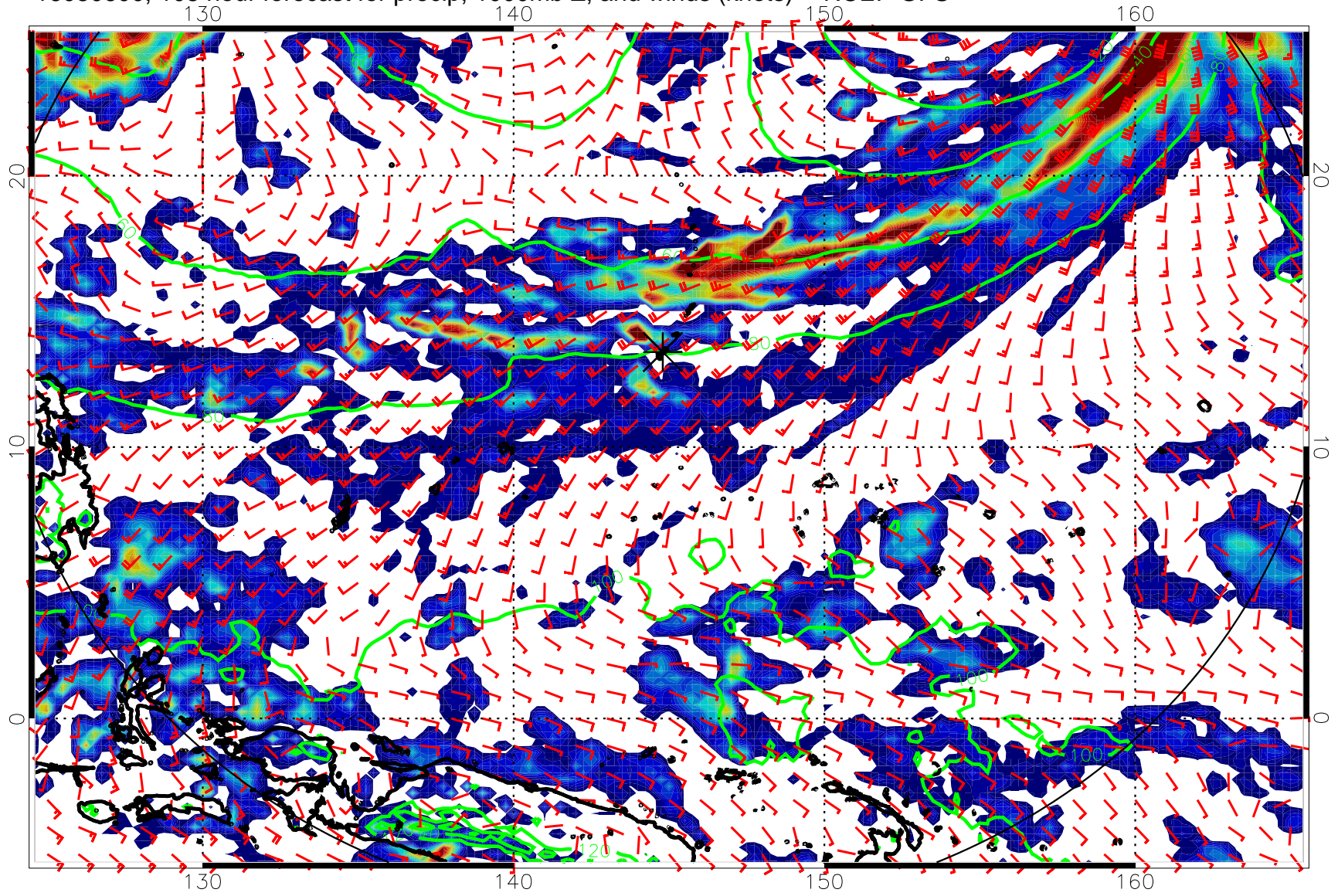
16080600, 108 hour forecast for precip, 1000mb Z, and winds (knots) -- NCEP GFS
