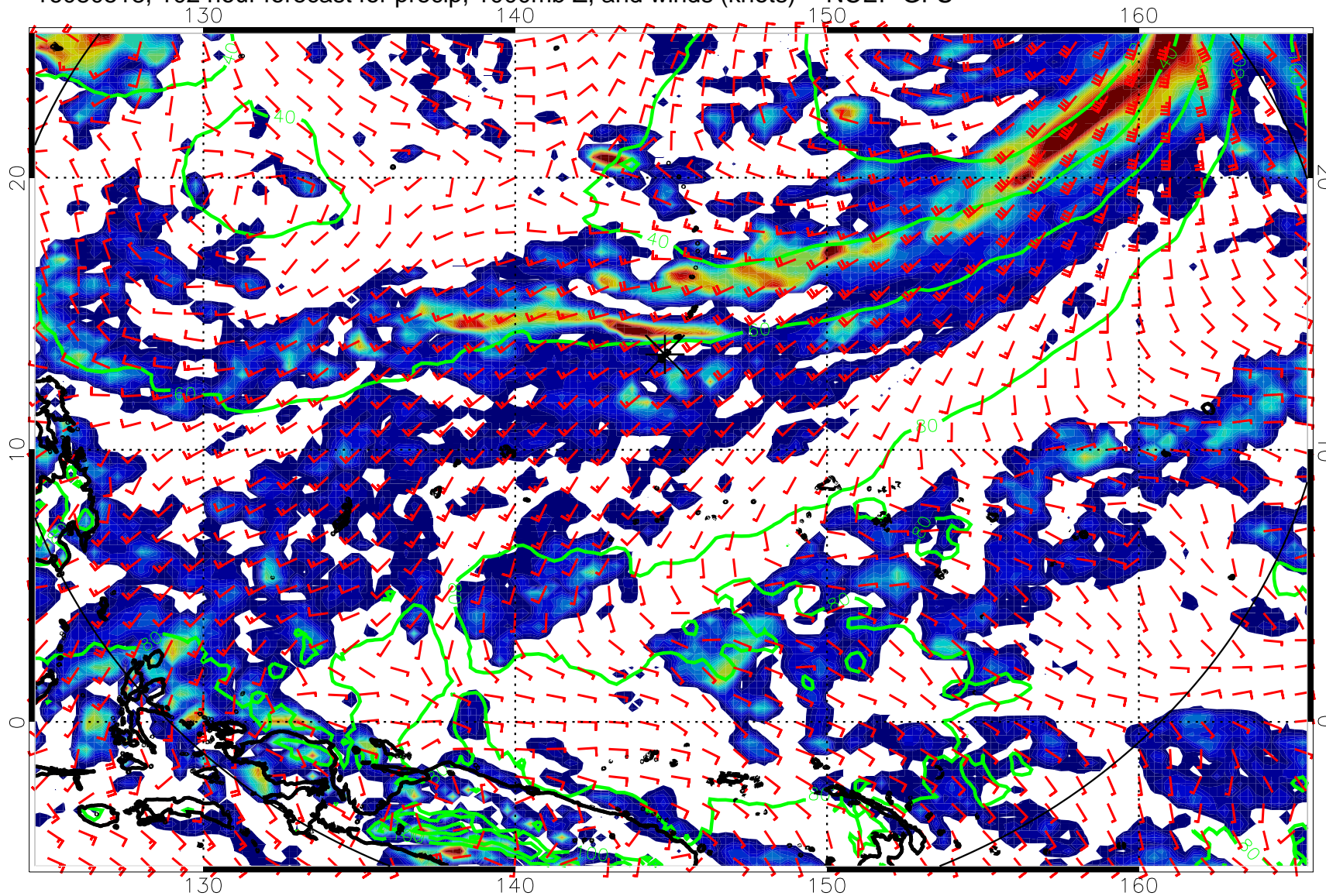
16080518, 102 hour forecast for precip, 1000mb Z, and winds (knots) -- NCEP GFS
