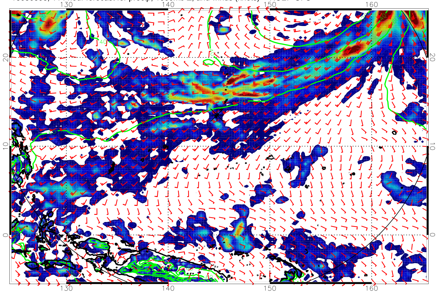
16080606, 114 hour forecast for precip, 1000mb Z, and winds (knots) -- NCEP GFS
