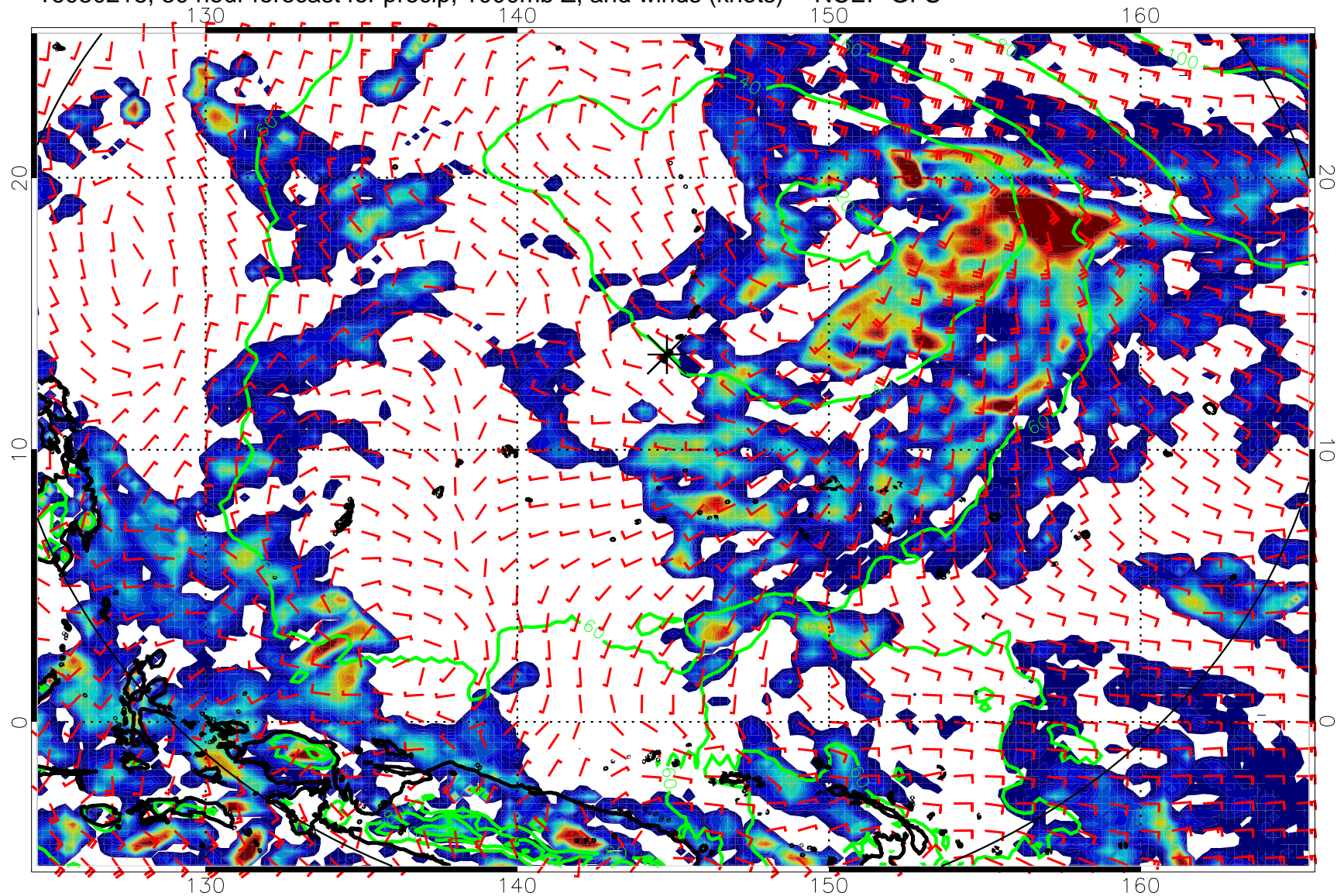
16080218, 30 hour forecast for precip, 1000mb Z, and winds (knots) -- NCEP GFS
