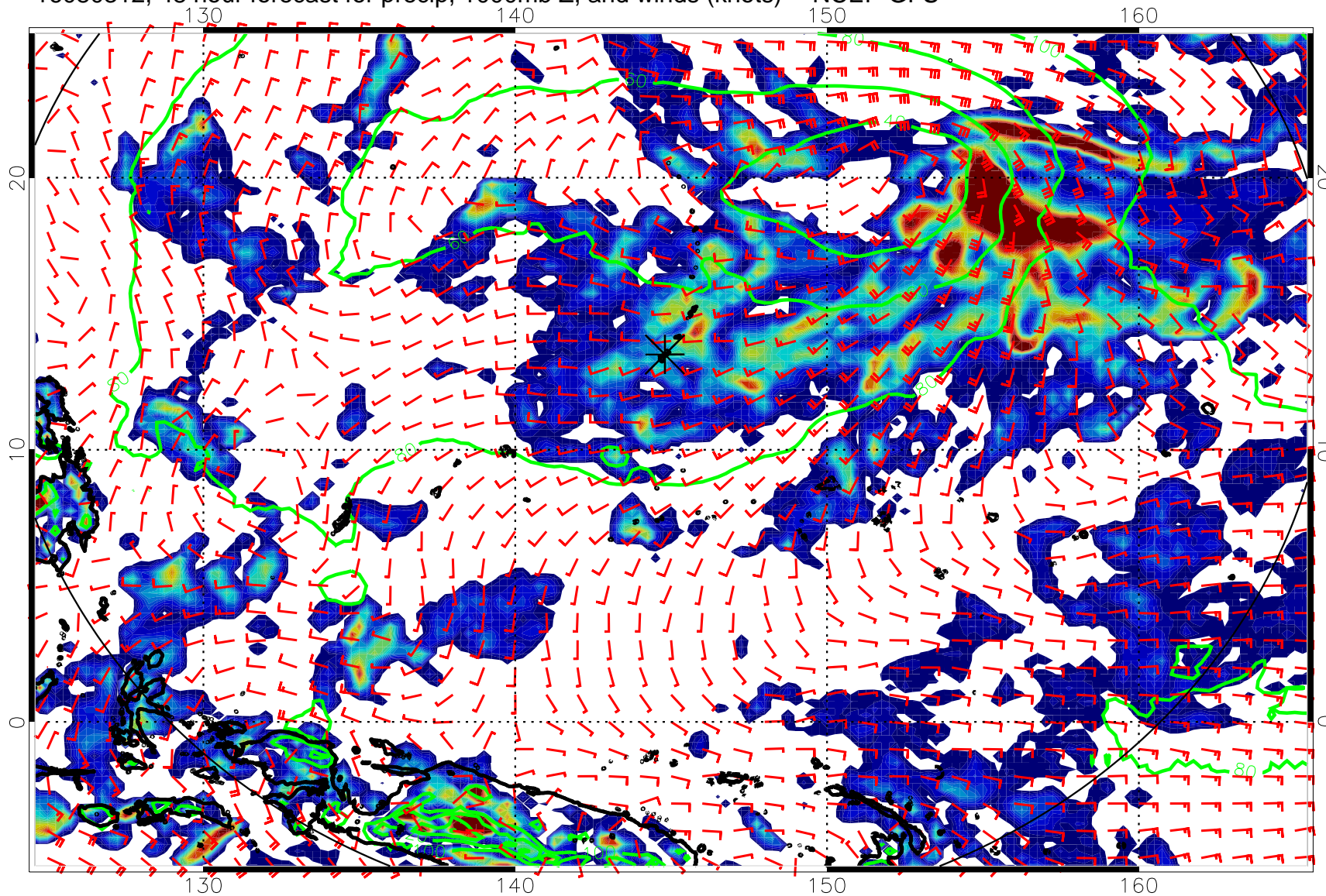
16080312, 48 hour forecast for precip, 1000mb Z, and winds (knots) -- NCEP GFS
