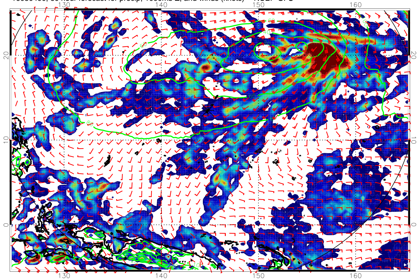
16080400, 60 hour forecast for precip, 1000mb Z, and winds (knots) -- NCEP GFS
