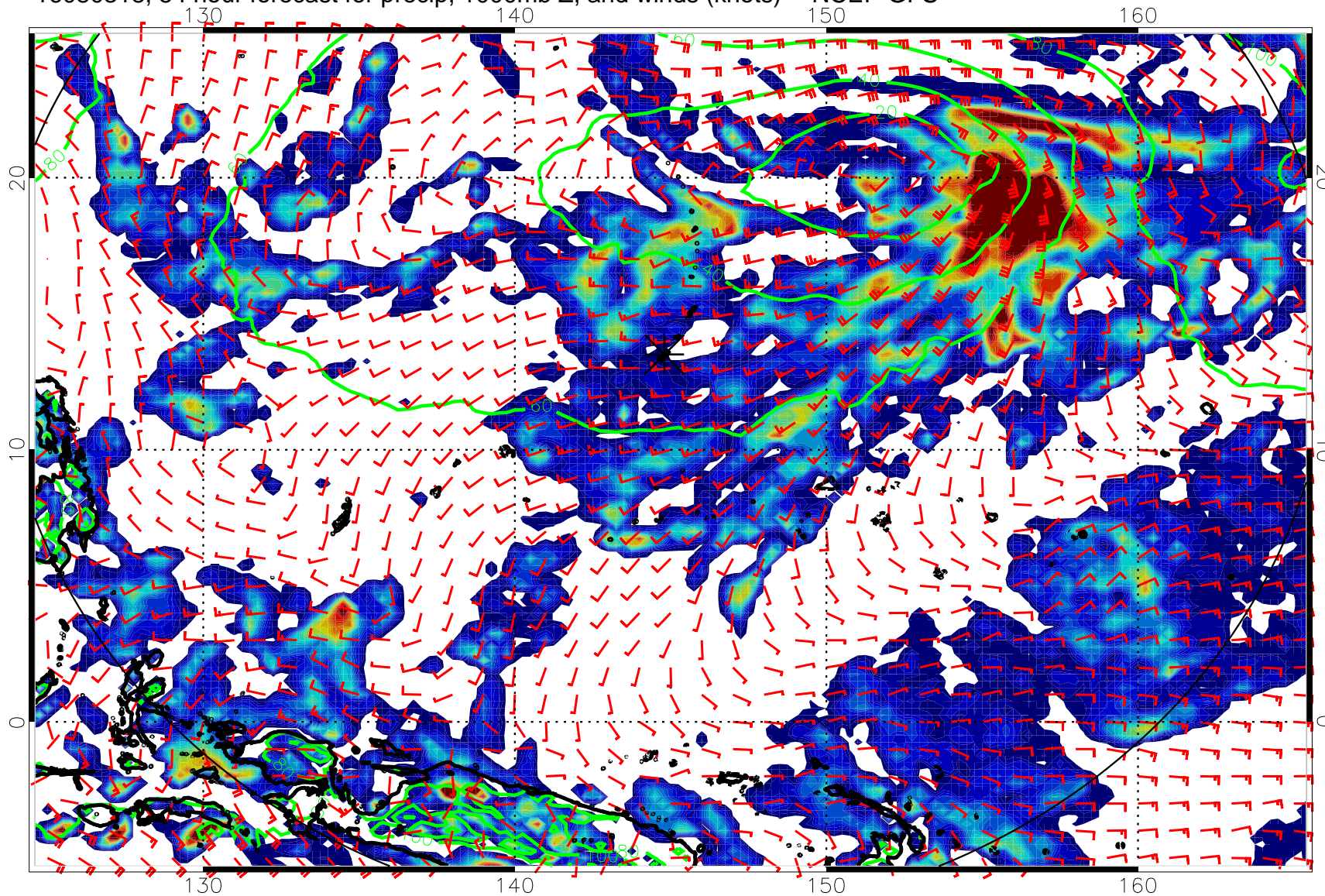
16080318, 54 hour forecast for precip, 1000mb Z, and winds (knots) -- NCEP GFS
