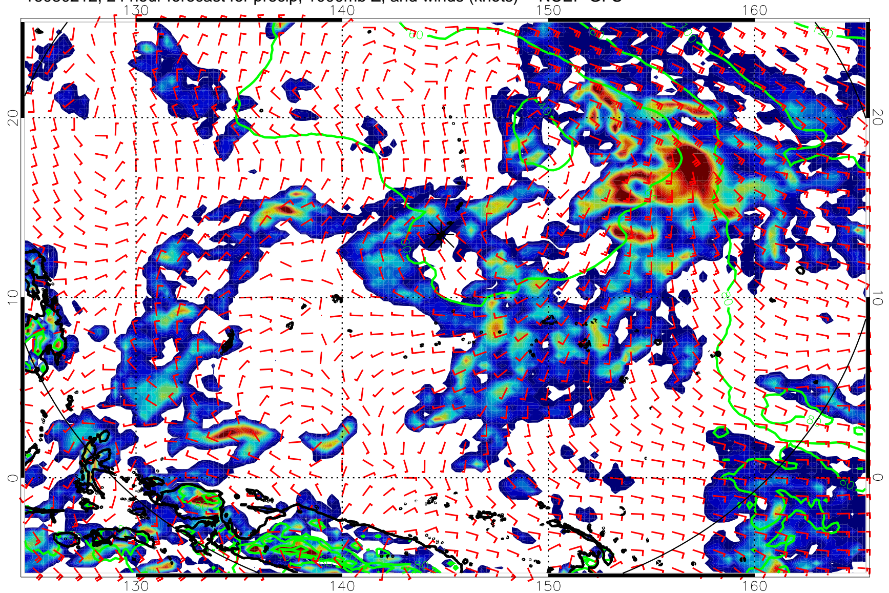
16080212, 24 hour forecast for precip, 1000mb Z, and winds (knots) -- NCEP GFS
