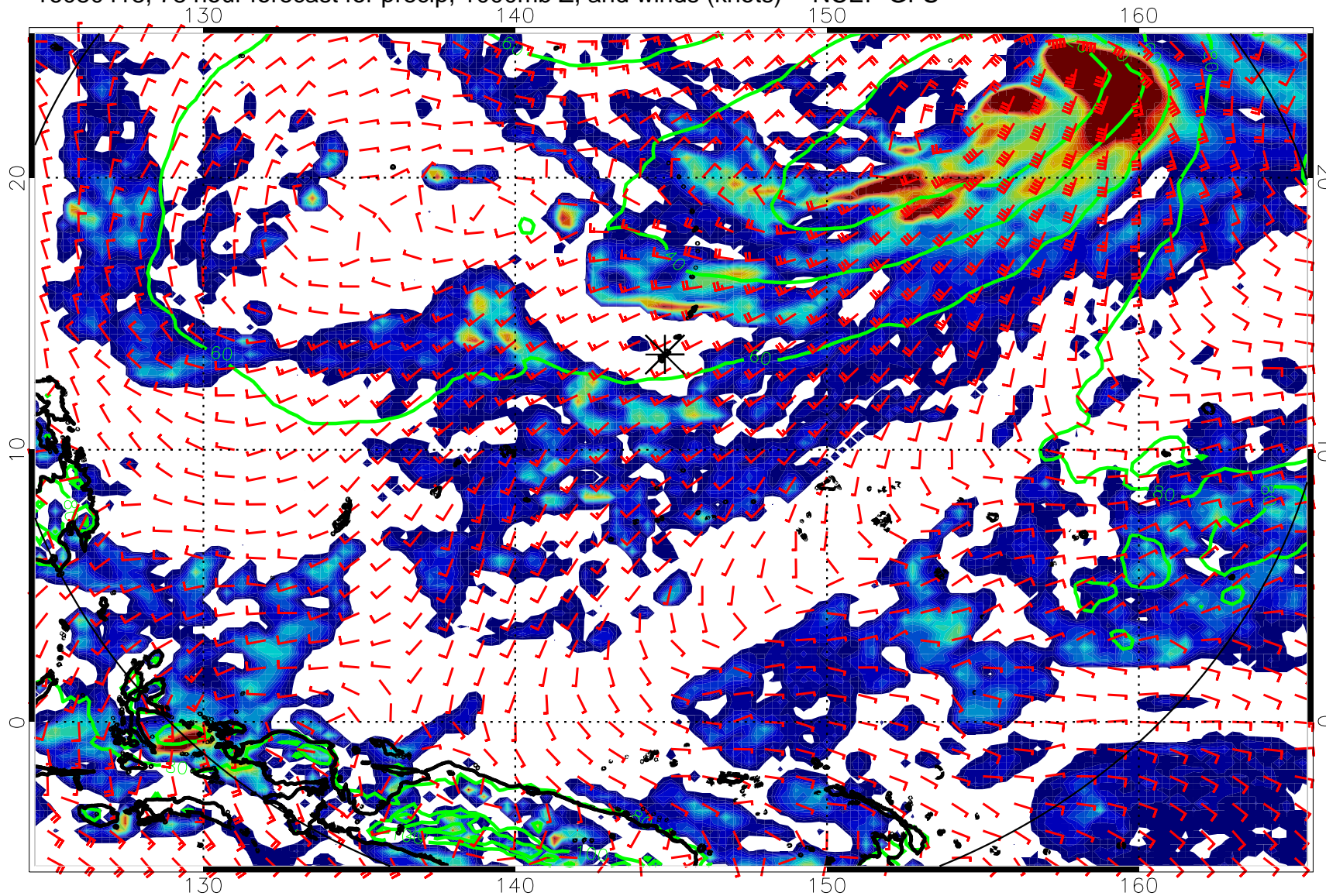
16080418, 78 hour forecast for precip, 1000mb Z, and winds (knots) -- NCEP GFS
