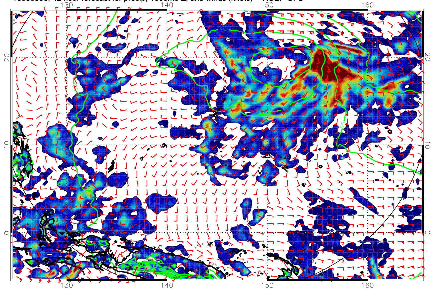
16080306, 42 hour forecast for precip, 1000mb Z, and winds (knots) -- NCEP GFS
