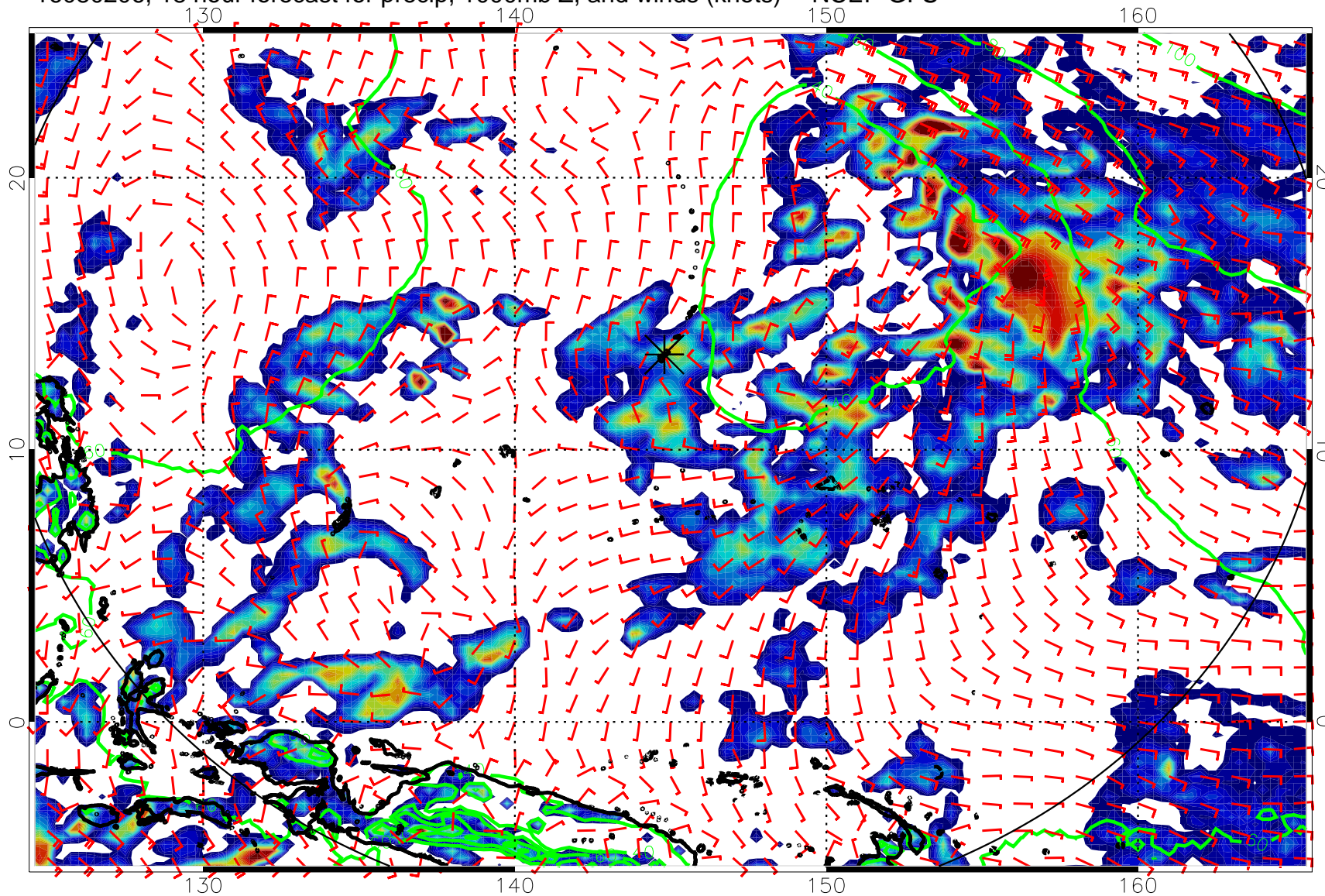
16080206, 18 hour forecast for precip, 1000mb Z, and winds (knots) -- NCEP GFS
