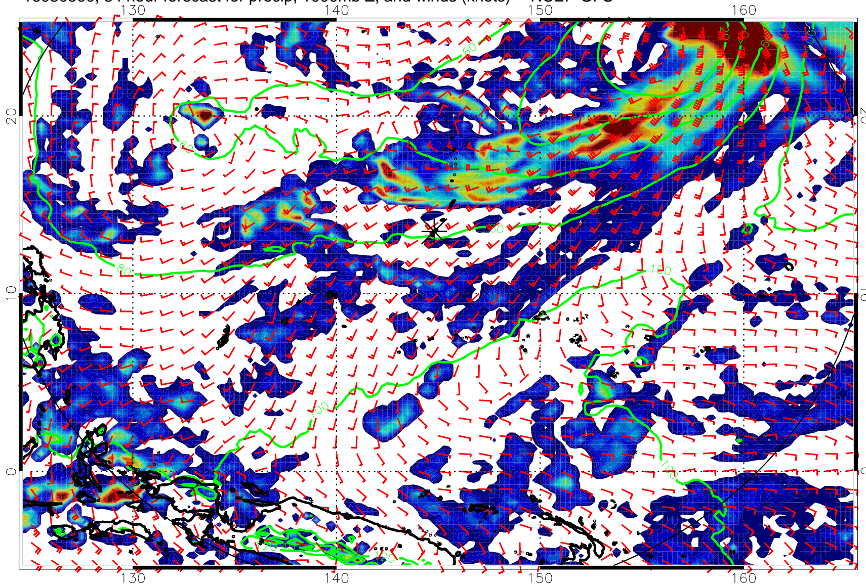
16080500, 84 hour forecast for precip, 1000mb Z, and winds (knots) -- NCEP GFS
