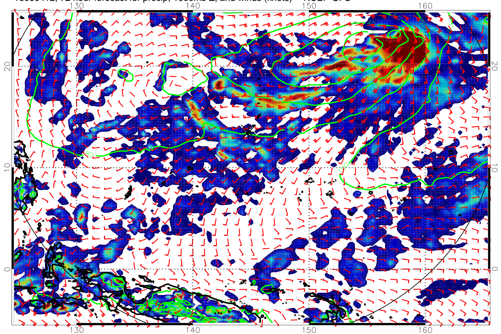
16080412, 72 hour forecast for precip, 1000mb Z, and winds (knots) -- NCEP GFS
