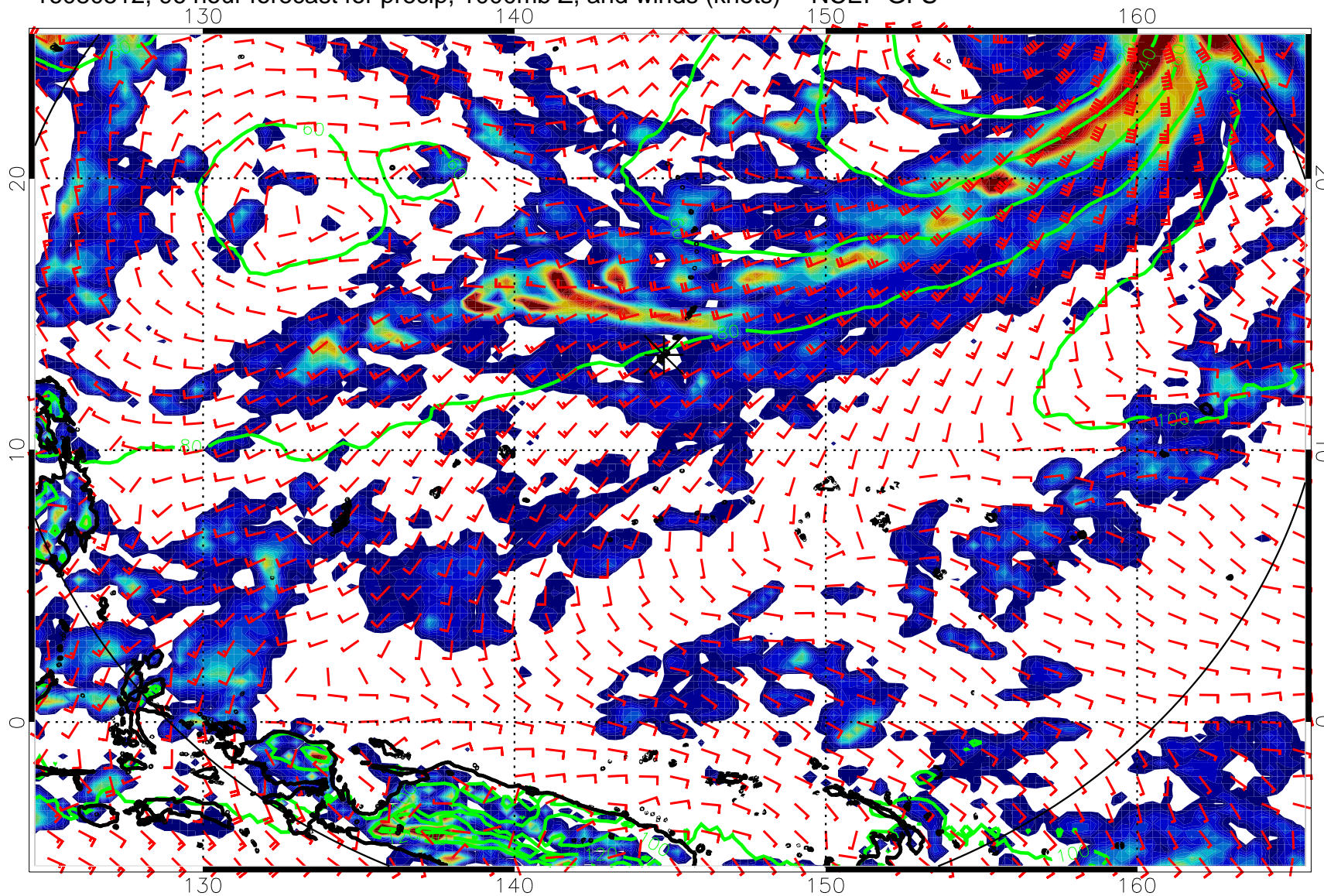
16080512, 96 hour forecast for precip, 1000mb Z, and winds (knots) -- NCEP GFS
