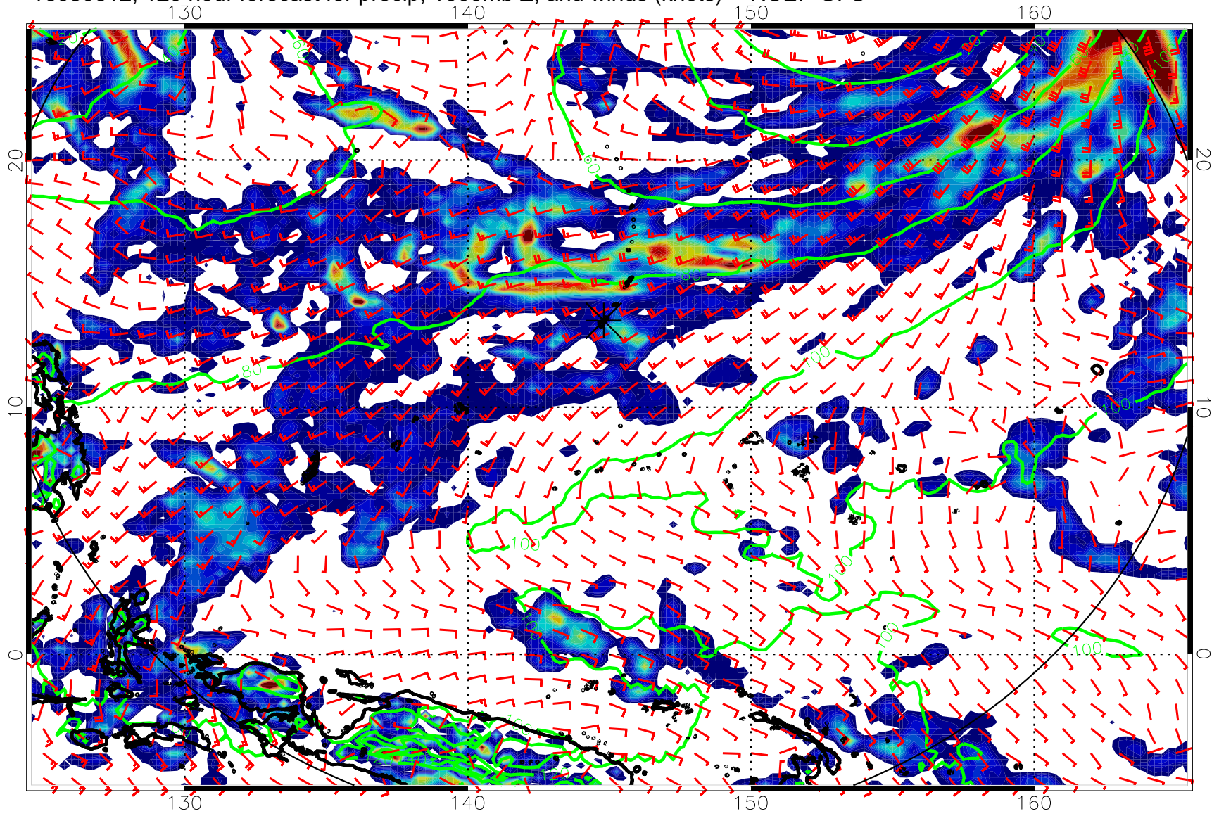
16080612, 120 hour forecast for precip, 1000mb Z, and winds (knots) -- NCEP GFS
