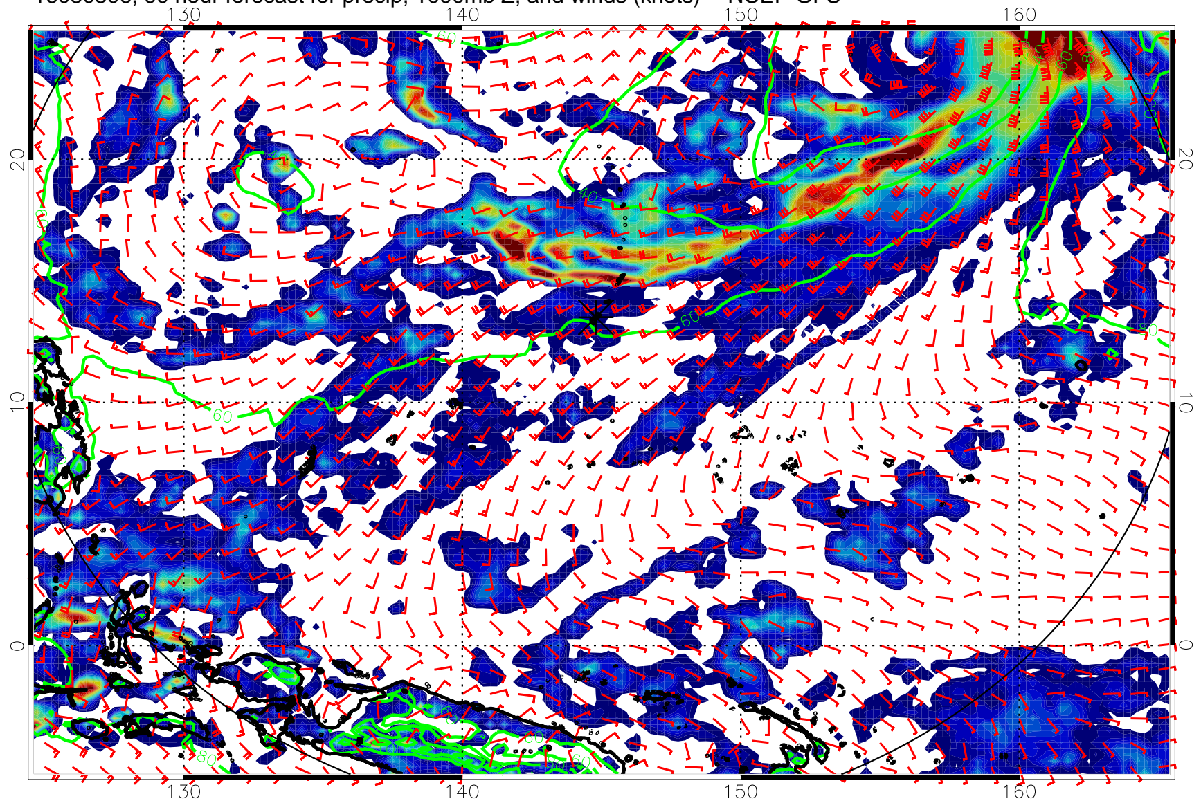
16080506, 90 hour forecast for precip, 1000mb Z, and winds (knots) -- NCEP GFS
