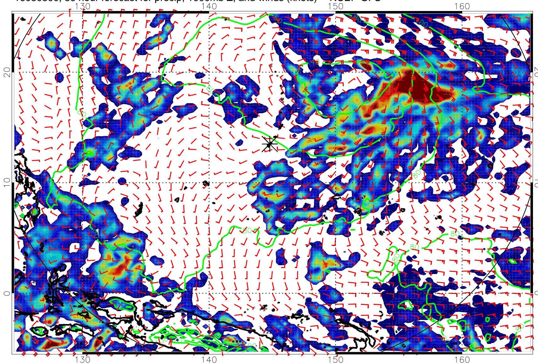
16080300, 36 hour forecast for precip, 1000mb Z, and winds (knots) -- NCEP GFS
