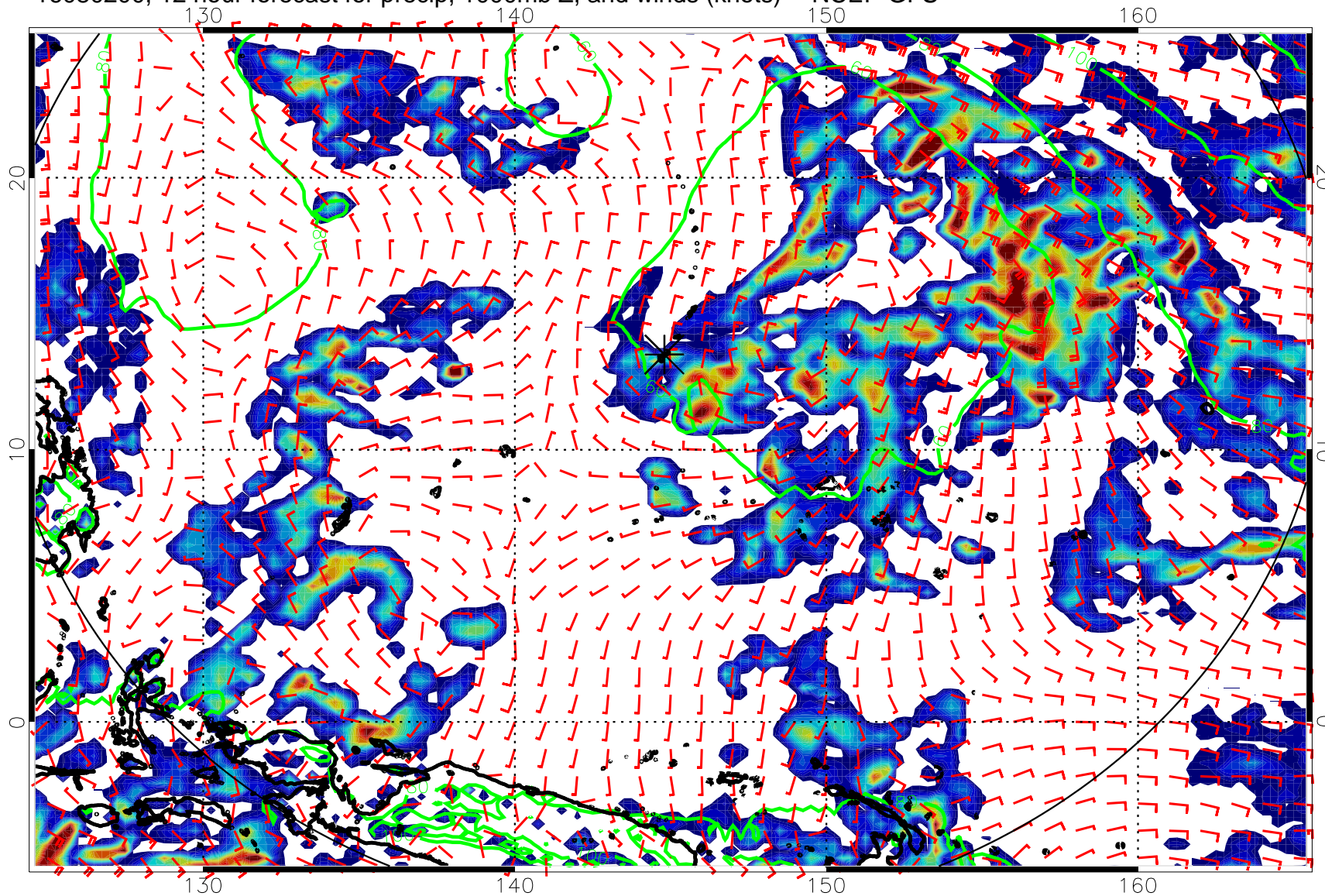
16080200, 12 hour forecast for precip, 1000mb Z, and winds (knots) -- NCEP GFS
