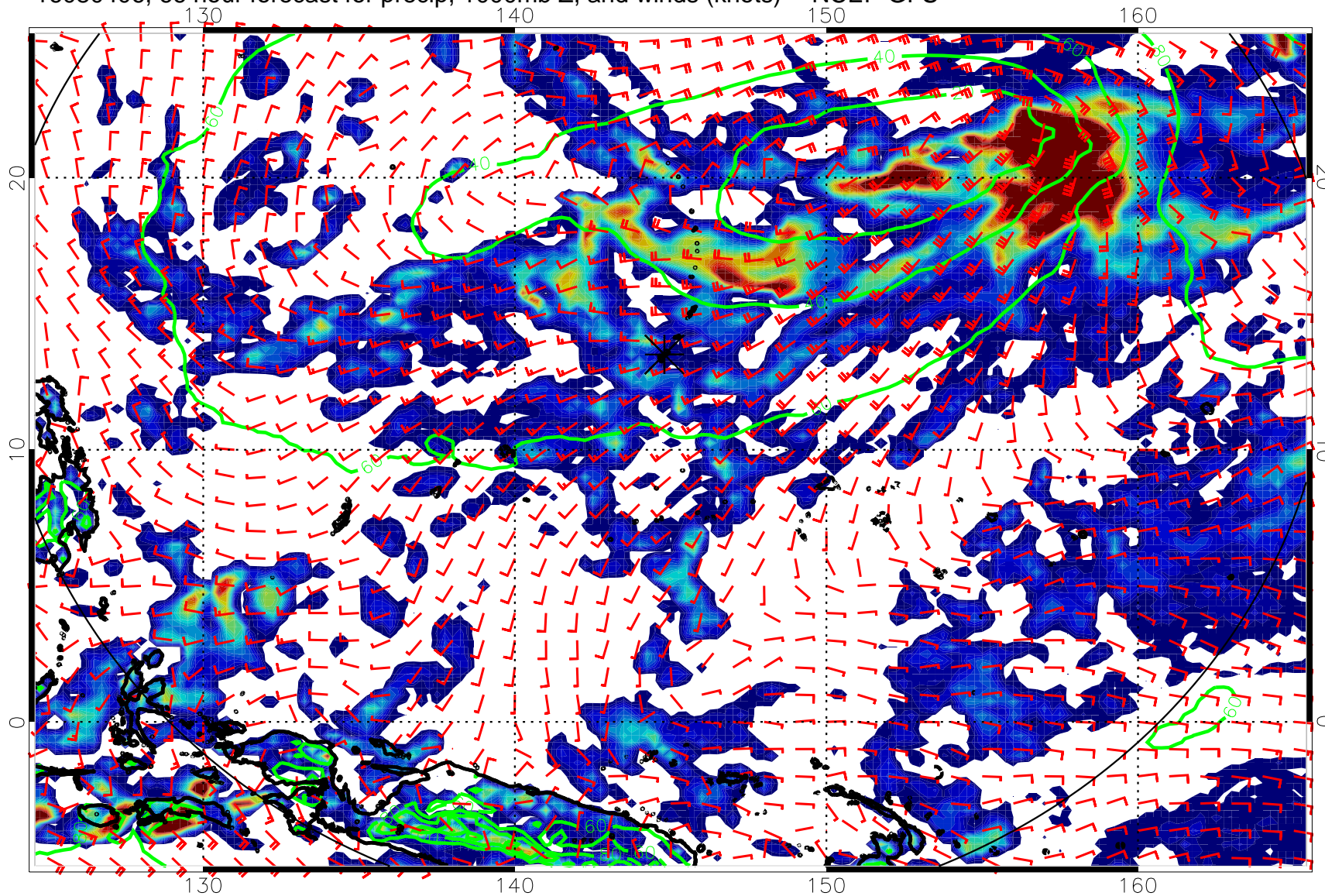
16080406, 66 hour forecast for precip, 1000mb Z, and winds (knots) -- NCEP GFS
