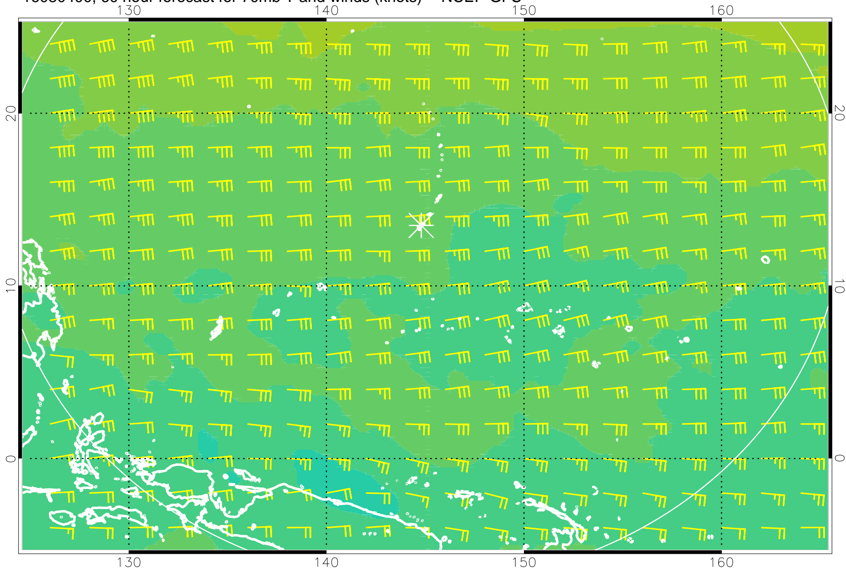
16080400, 60 hour forecast for 70mb T and winds (knots) -- NCEP GFS
