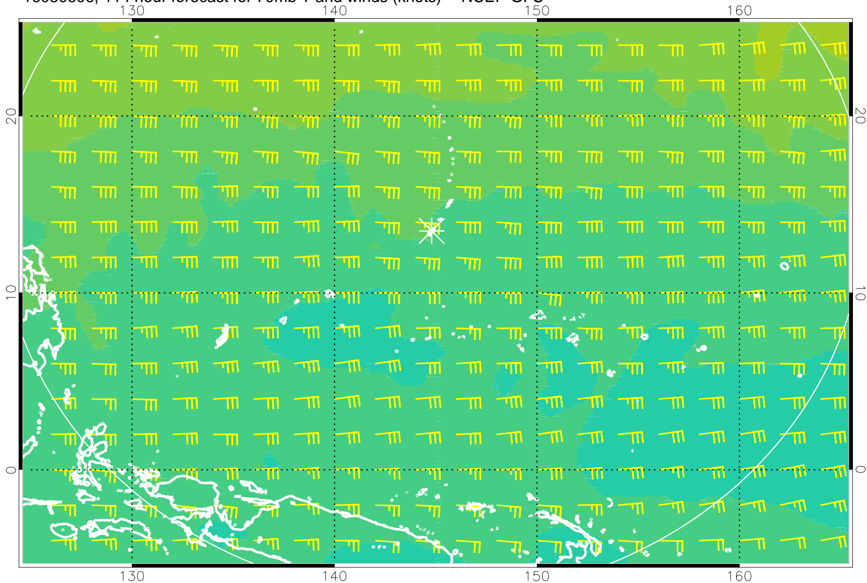
16080606, 114 hour forecast for 70mb T and winds (knots) -- NCEP GFS
