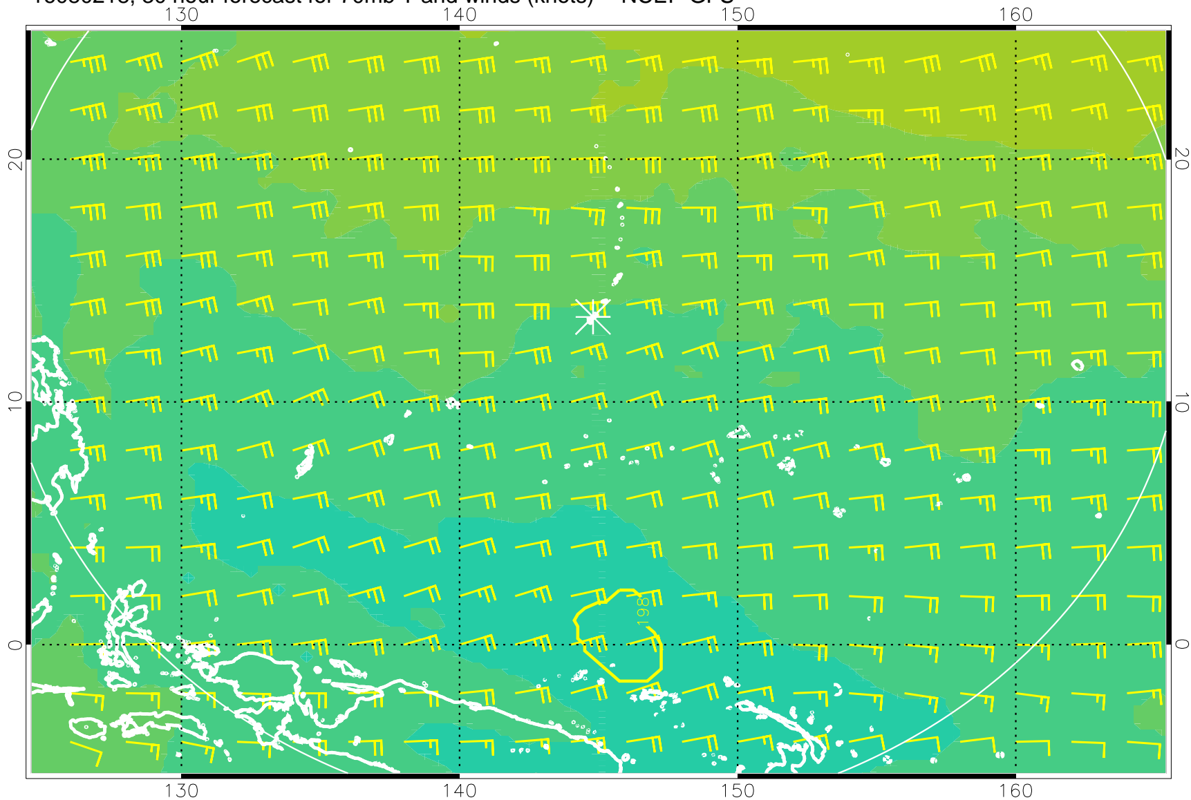
16080218, 30 hour forecast for 70mb T and winds (knots) -- NCEP GFS
