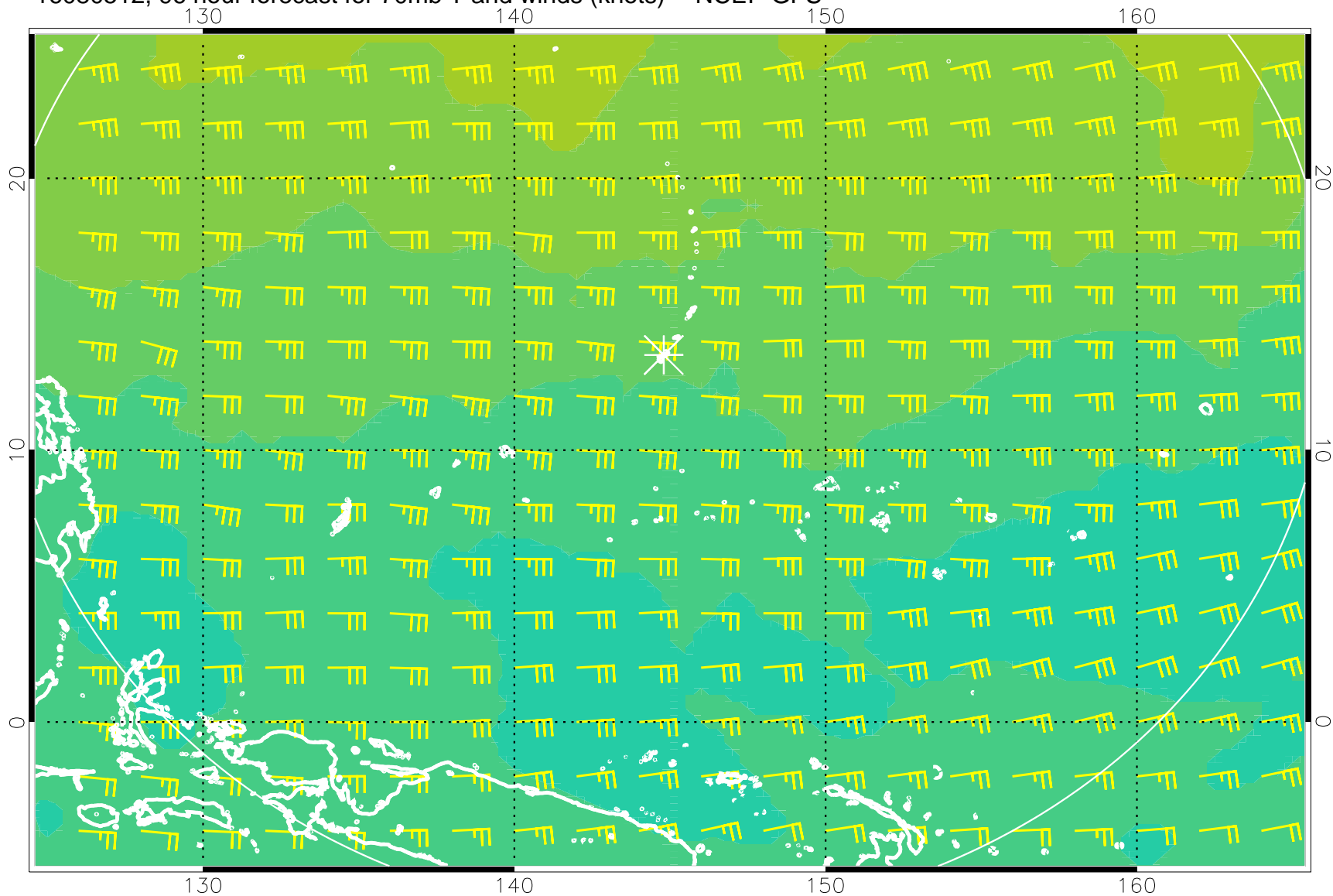
16080512, 96 hour forecast for 70mb T and winds (knots) -- NCEP GFS
