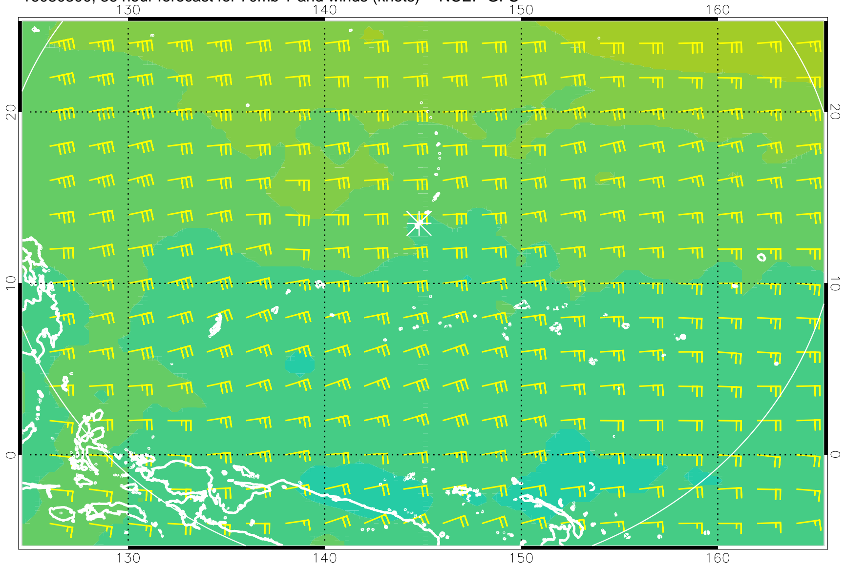
16080300, 36 hour forecast for 70mb T and winds (knots) -- NCEP GFS
