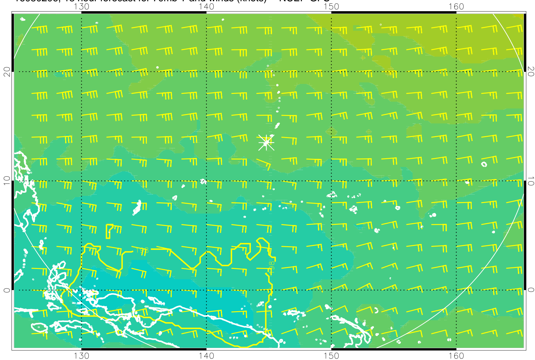
16080206, 18 hour forecast for 70mb T and winds (knots) -- NCEP GFS
