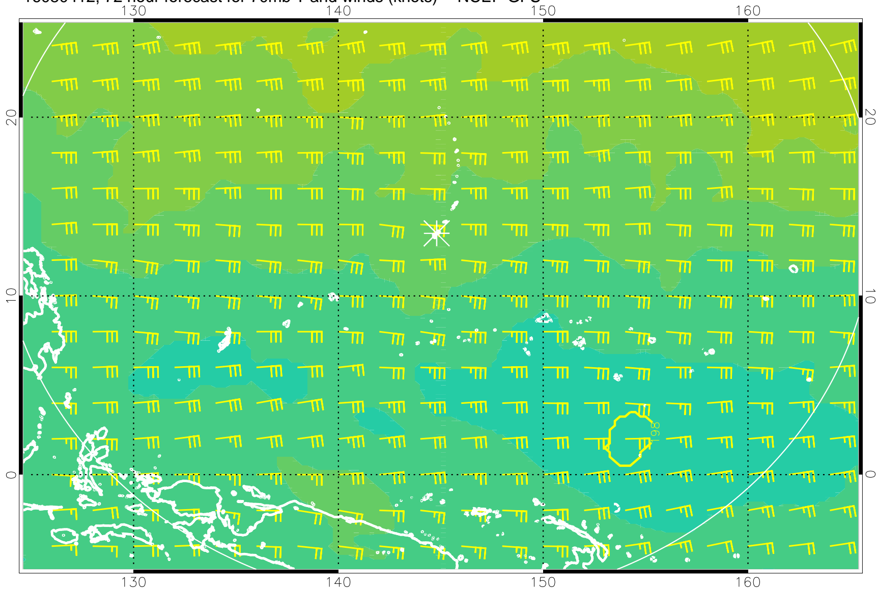
16080412, 72 hour forecast for 70mb T and winds (knots) -- NCEP GFS
