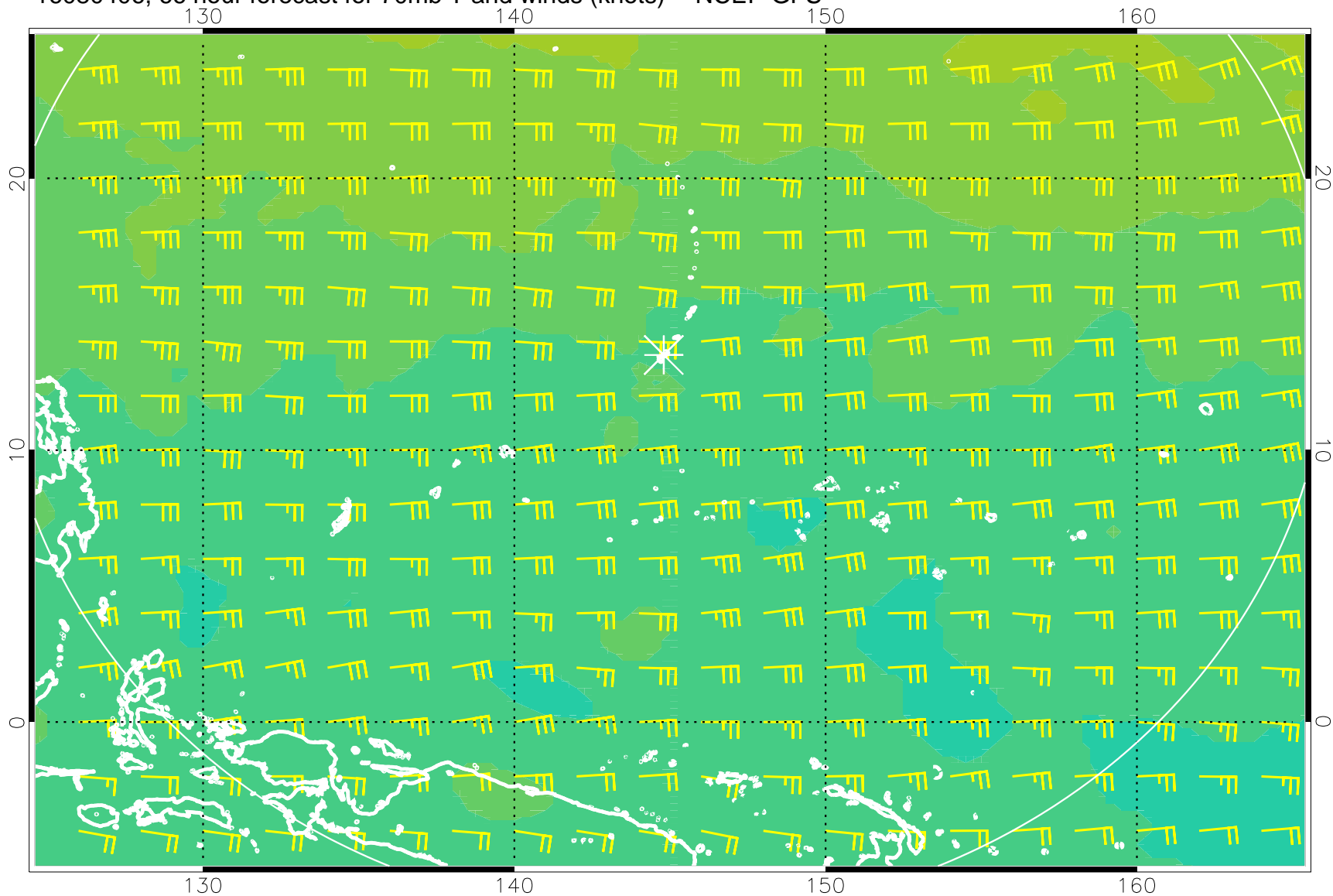
16080406, 66 hour forecast for 70mb T and winds (knots) -- NCEP GFS
