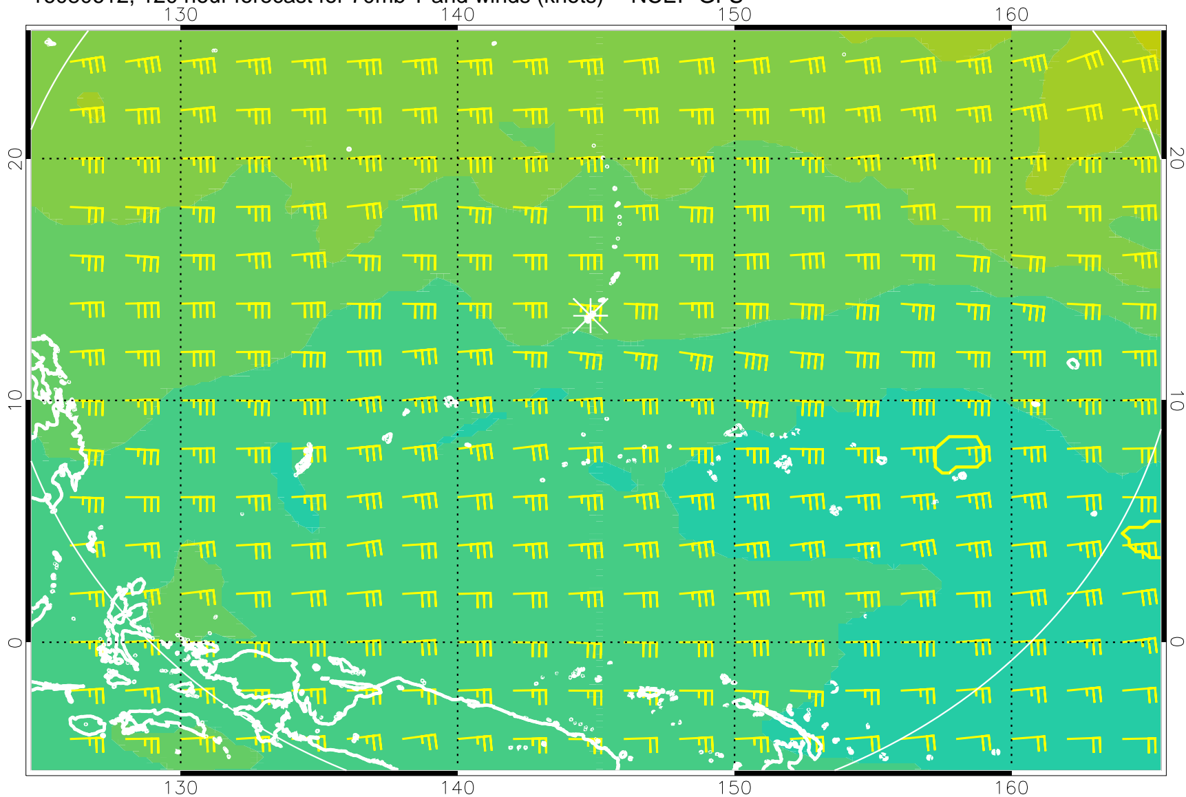
16080612, 120 hour forecast for 70mb T and winds (knots) -- NCEP GFS
