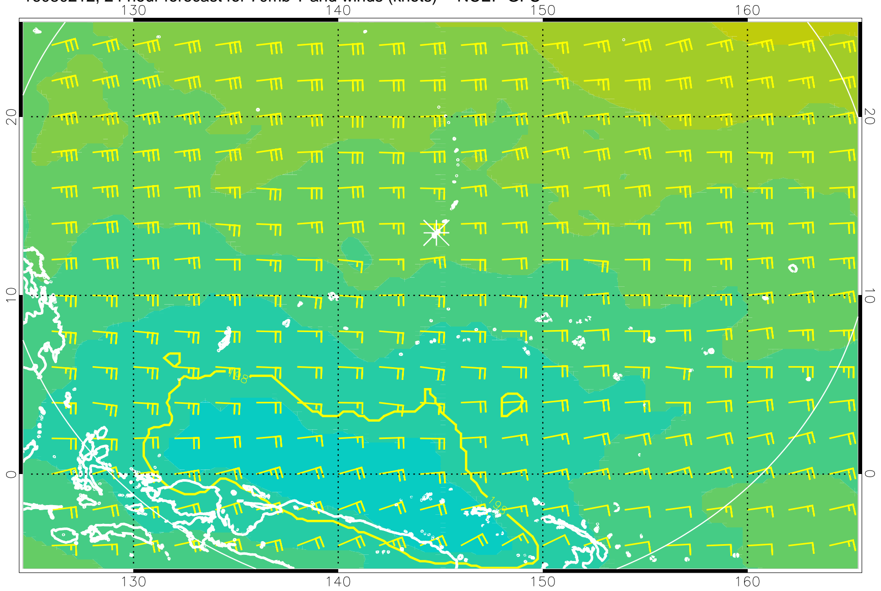
16080212, 24 hour forecast for 70mb T and winds (knots) -- NCEP GFS
