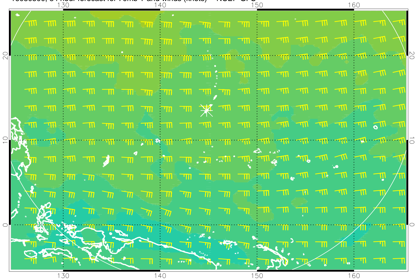
16080500, 84 hour forecast for 70mb T and winds (knots) -- NCEP GFS
