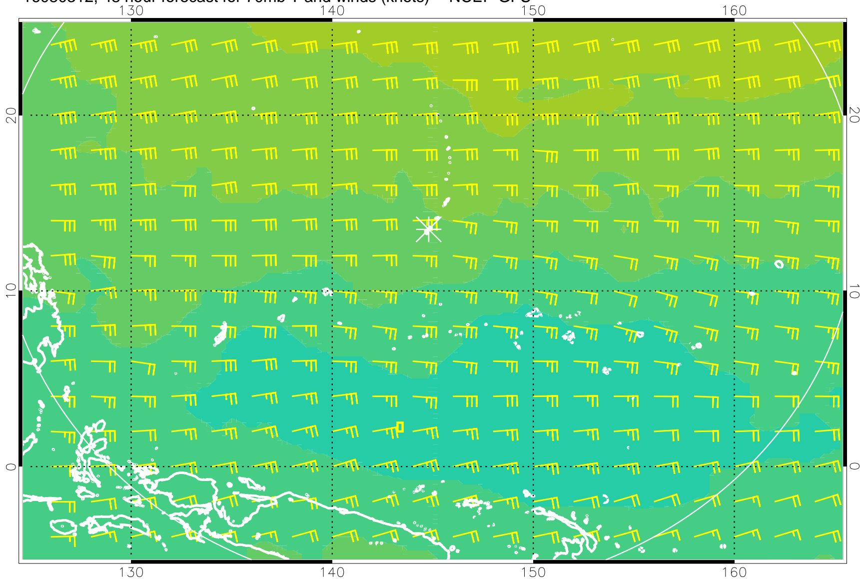
16080312, 48 hour forecast for 70mb T and winds (knots) -- NCEP GFS
