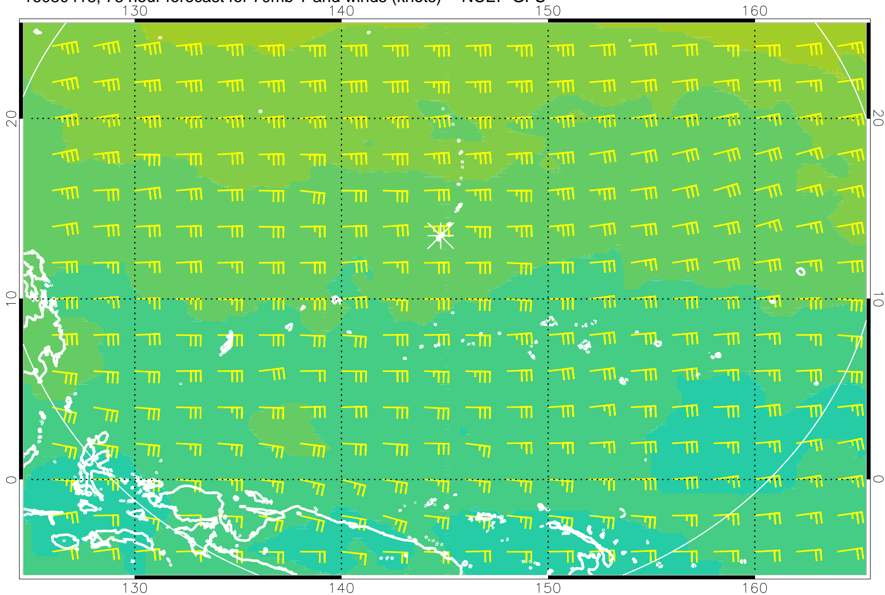
16080418, 78 hour forecast for 70mb T and winds (knots) -- NCEP GFS
