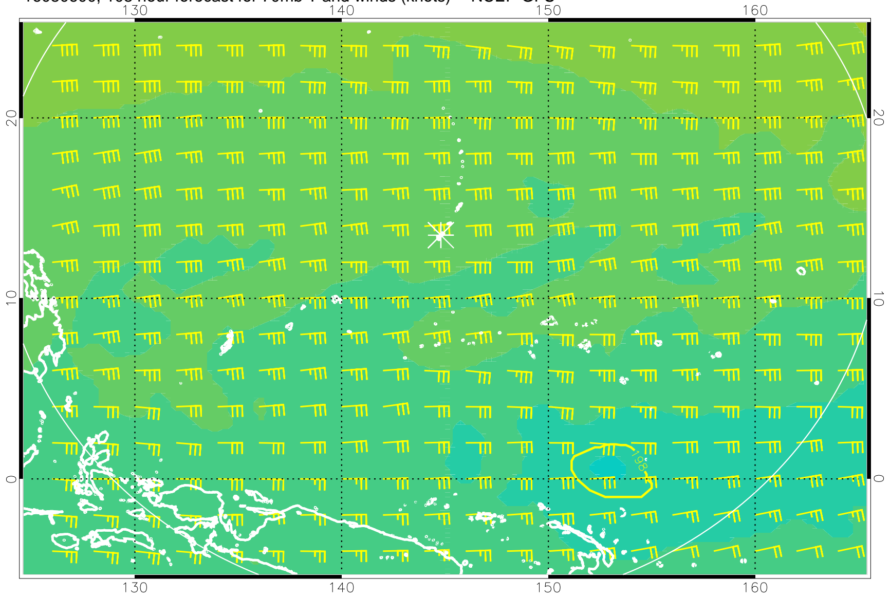
16080600, 108 hour forecast for 70mb T and winds (knots) -- NCEP GFS
