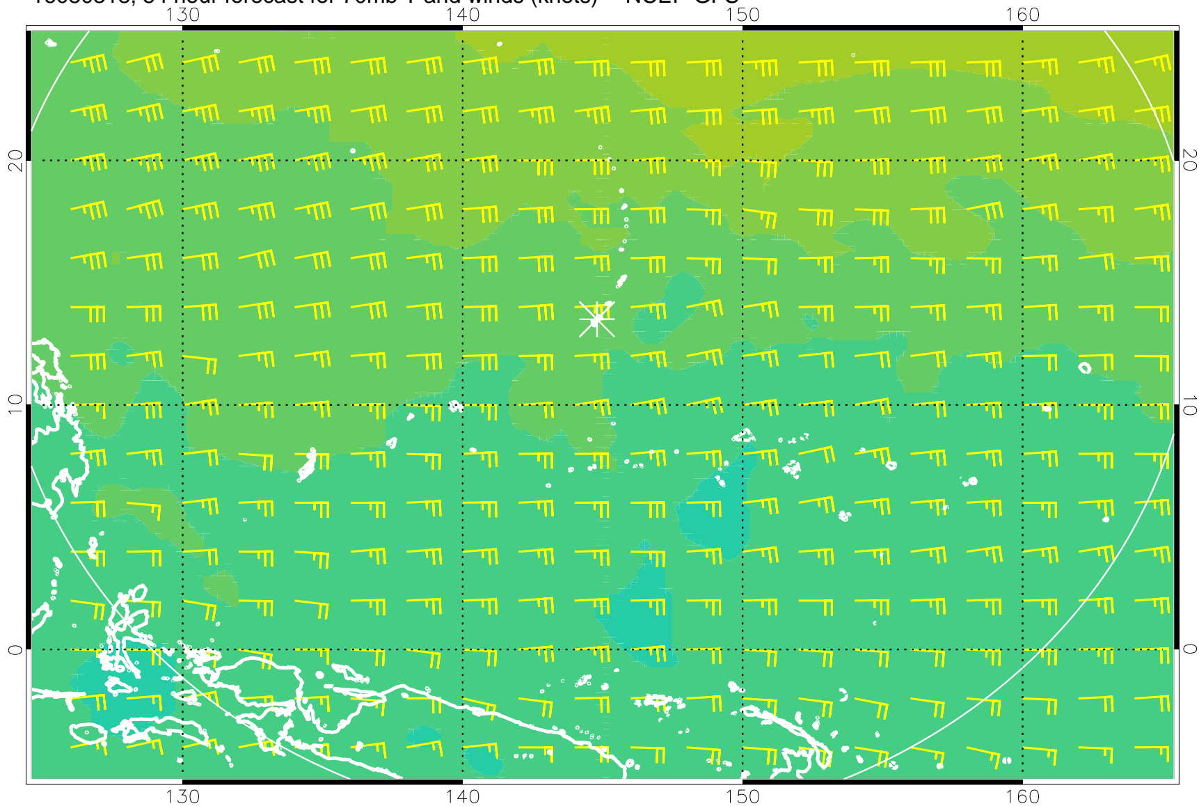
16080318, 54 hour forecast for 70mb T and winds (knots) -- NCEP GFS
