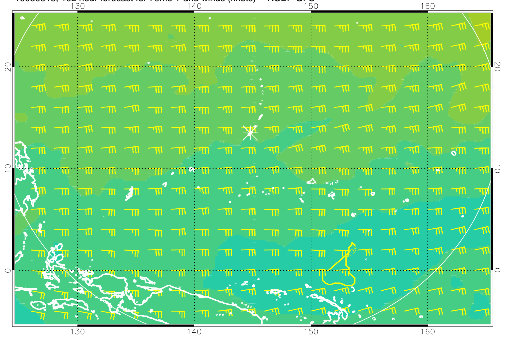
16080518, 102 hour forecast for 70mb T and winds (knots) -- NCEP GFS
