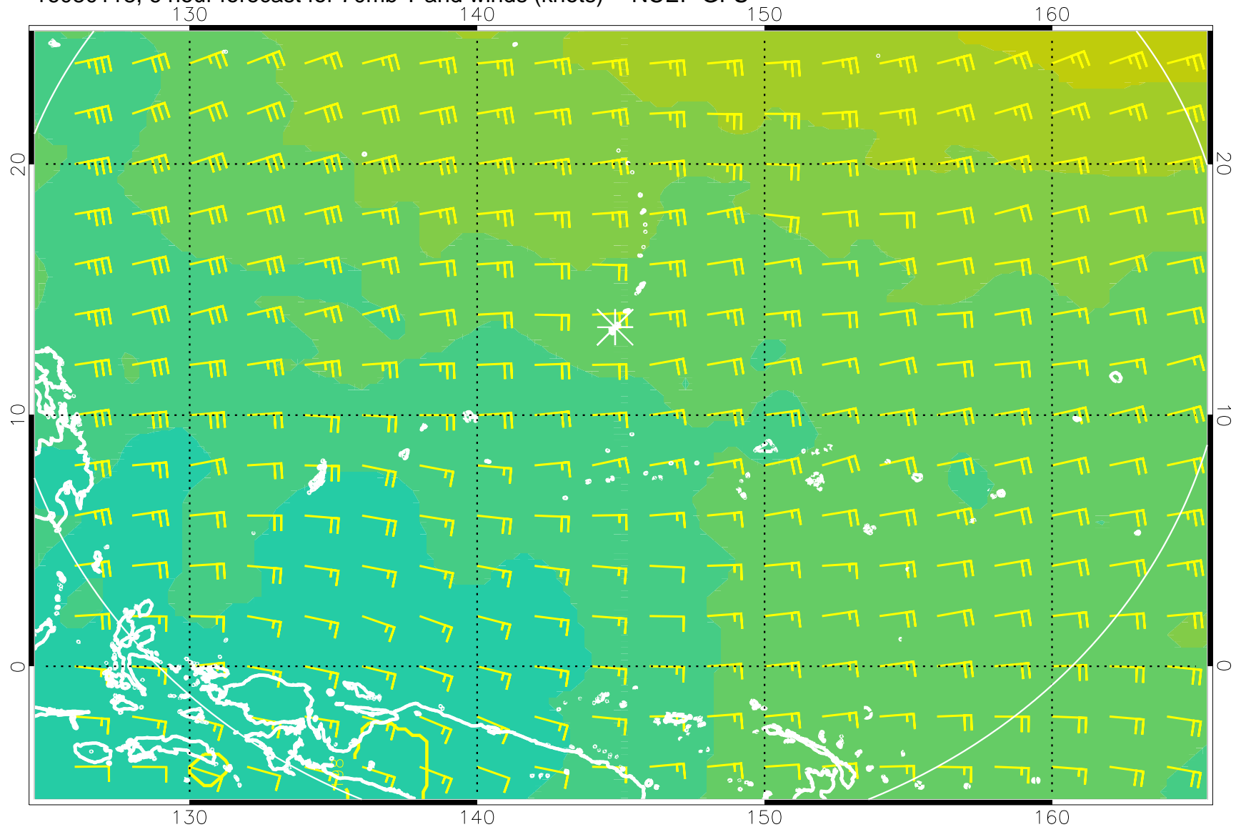
16080118, 6 hour forecast for 70mb T and winds (knots) -- NCEP GFS
