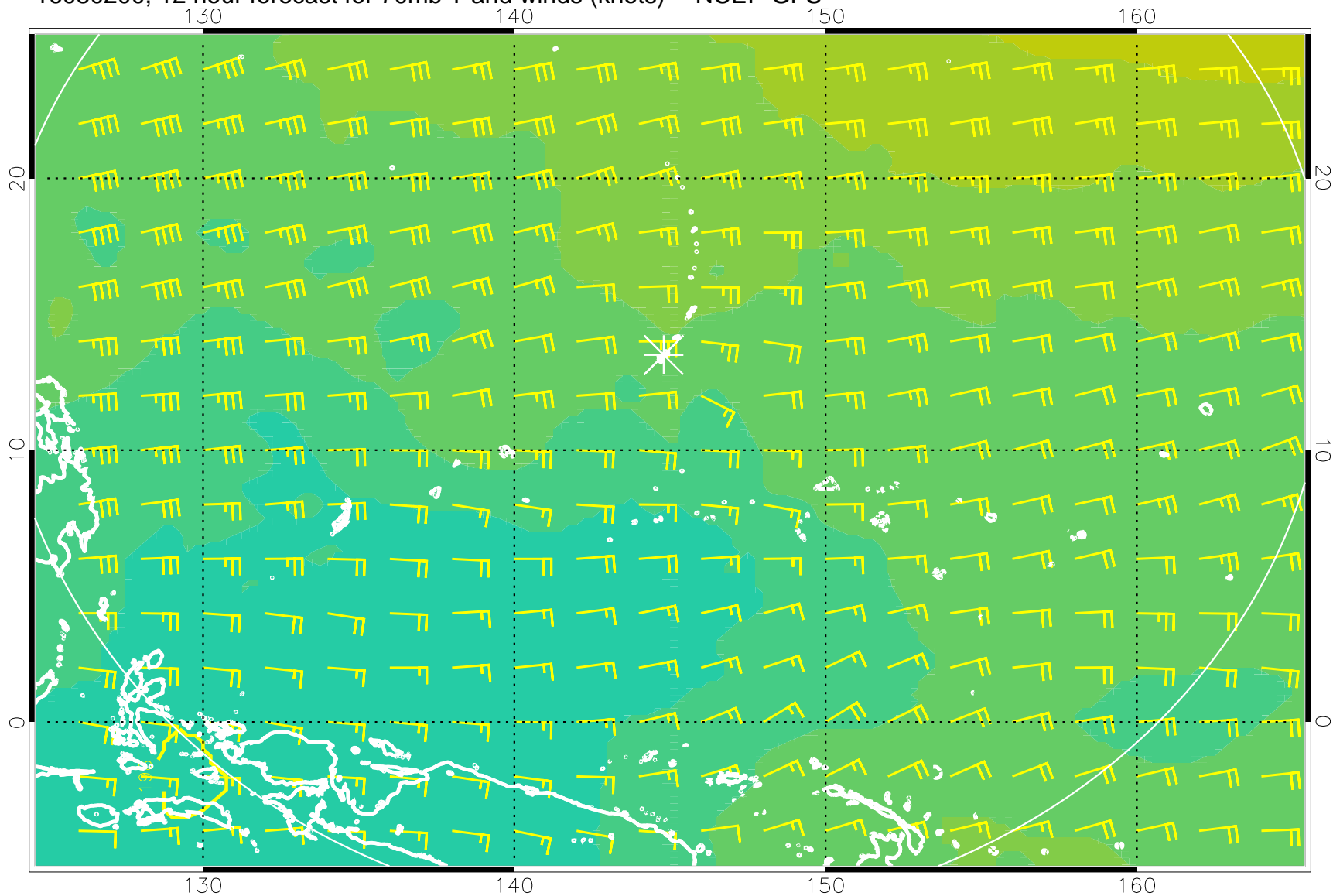
16080200, 12 hour forecast for 70mb T and winds (knots) -- NCEP GFS
