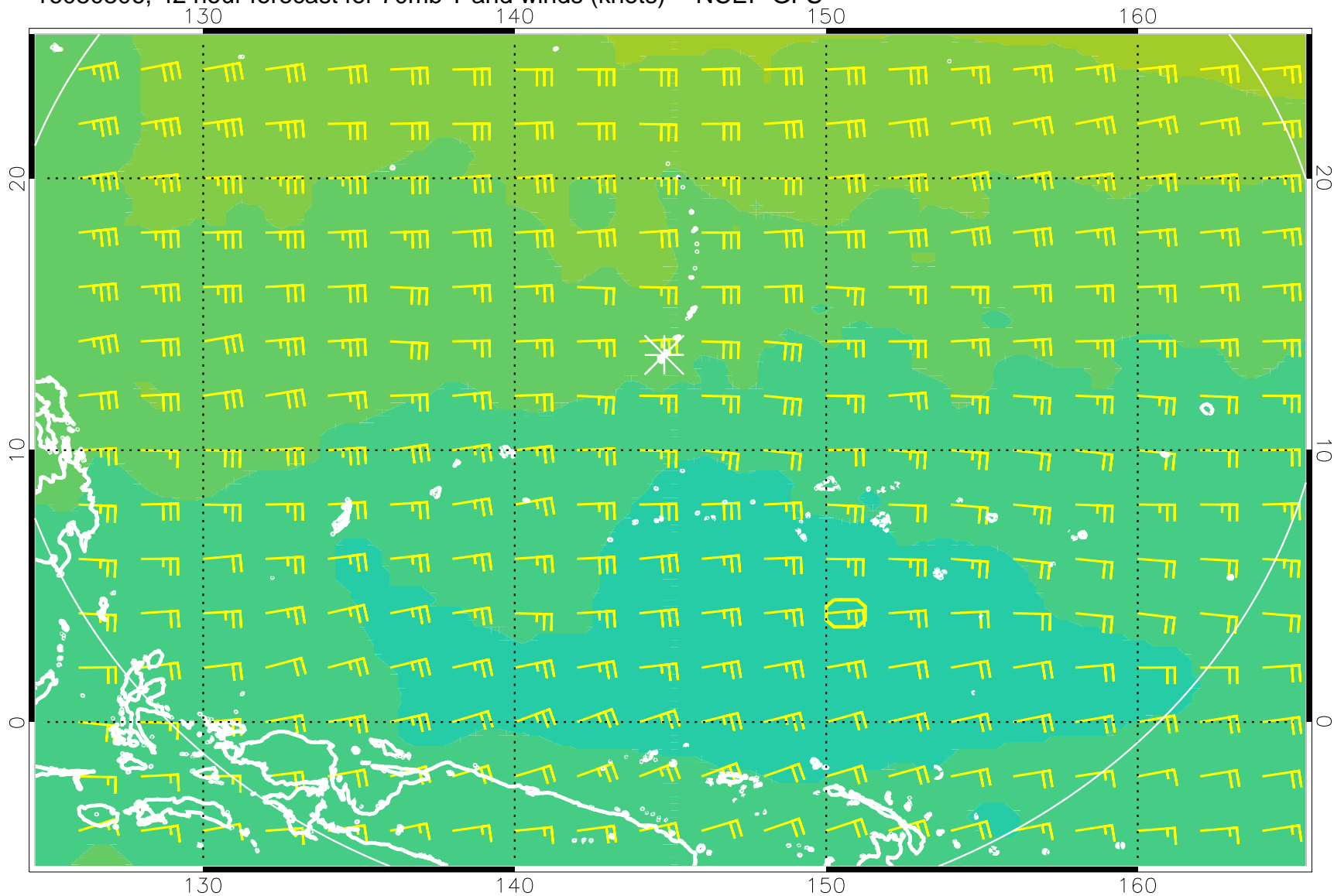
16080306, 42 hour forecast for 70mb T and winds (knots) -- NCEP GFS
