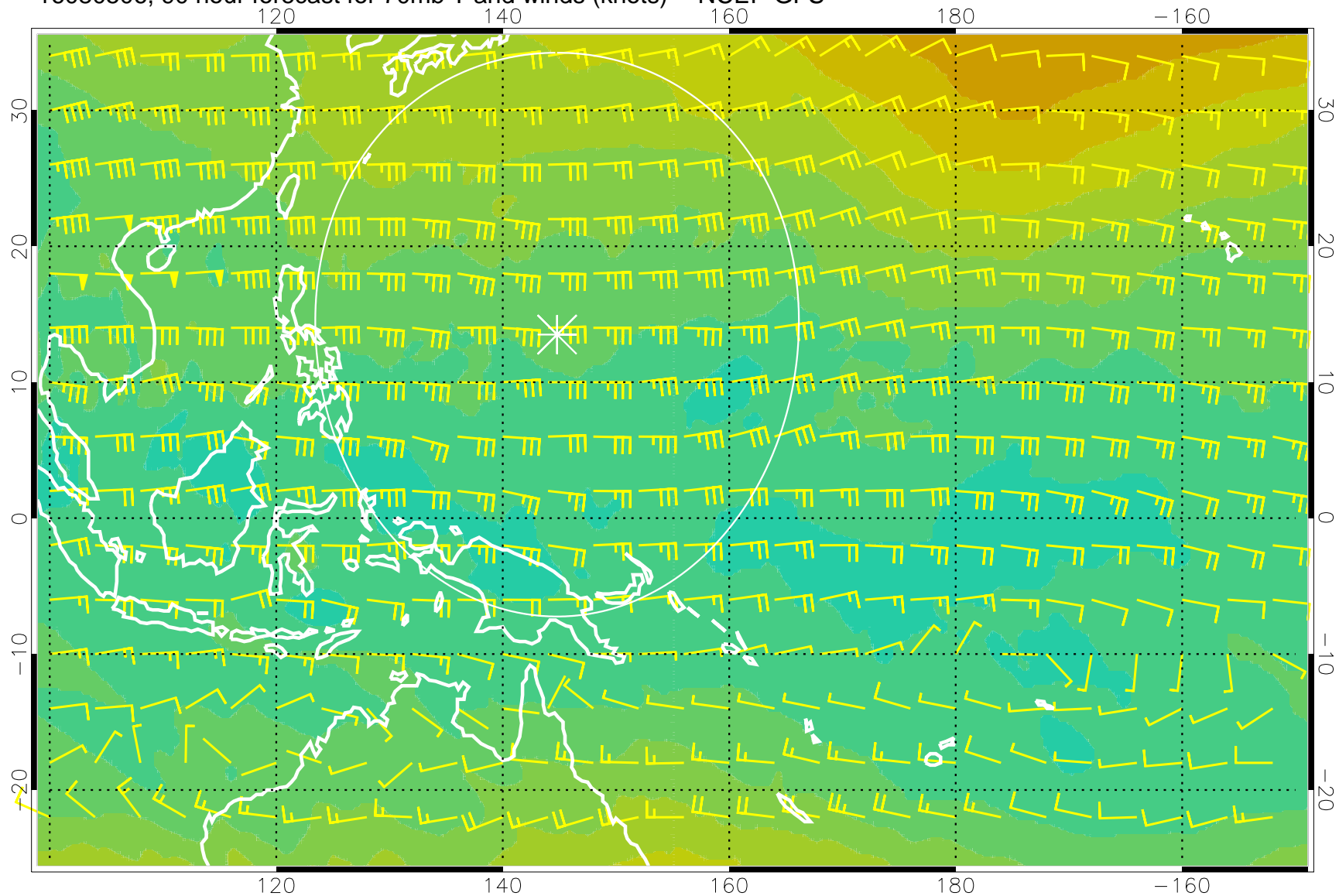
16080506, 90 hour forecast for 70mb T and winds (knots) -- NCEP GFS
