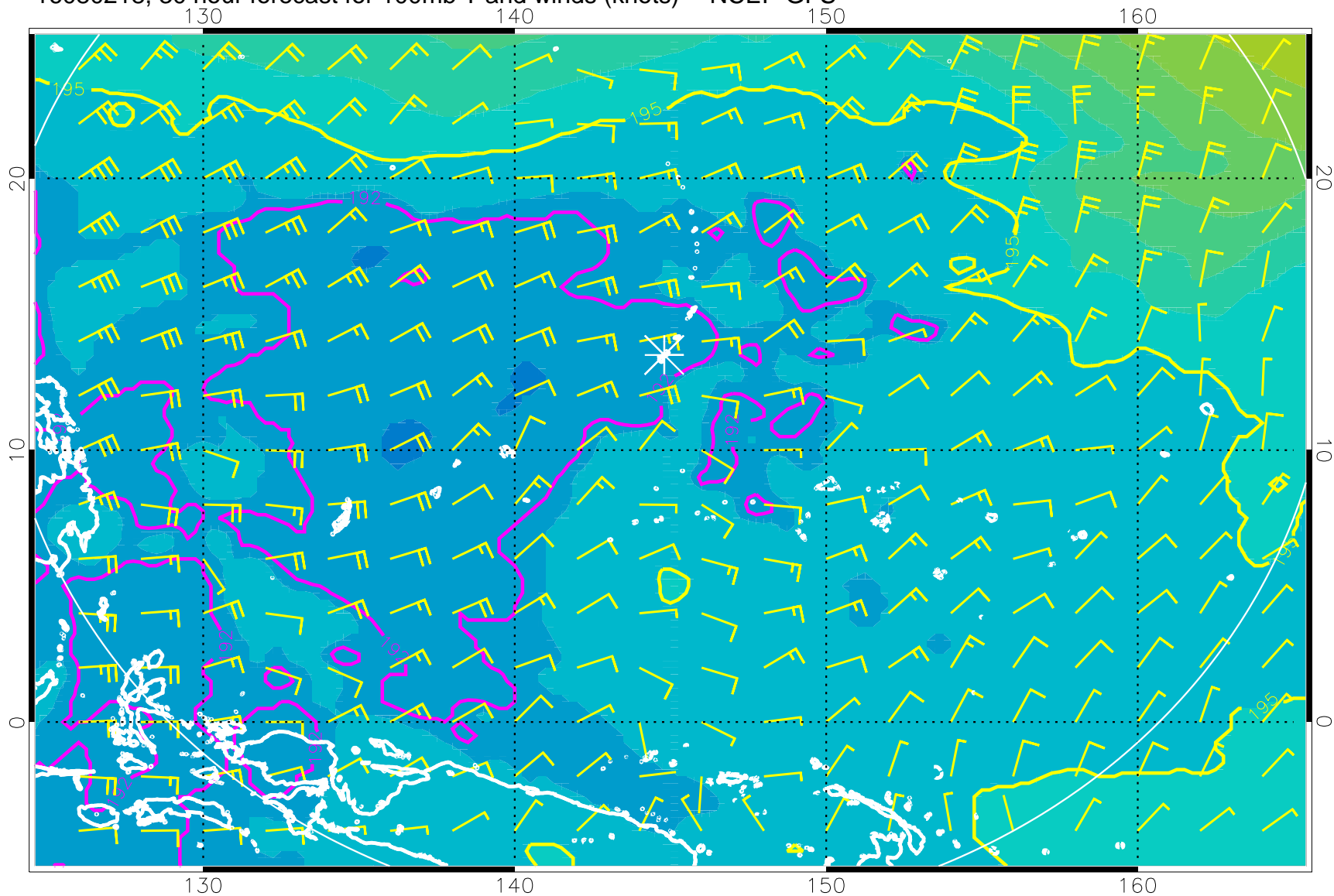
16080218, 30 hour forecast for 100mb T and winds (knots) -- NCEP GFS
