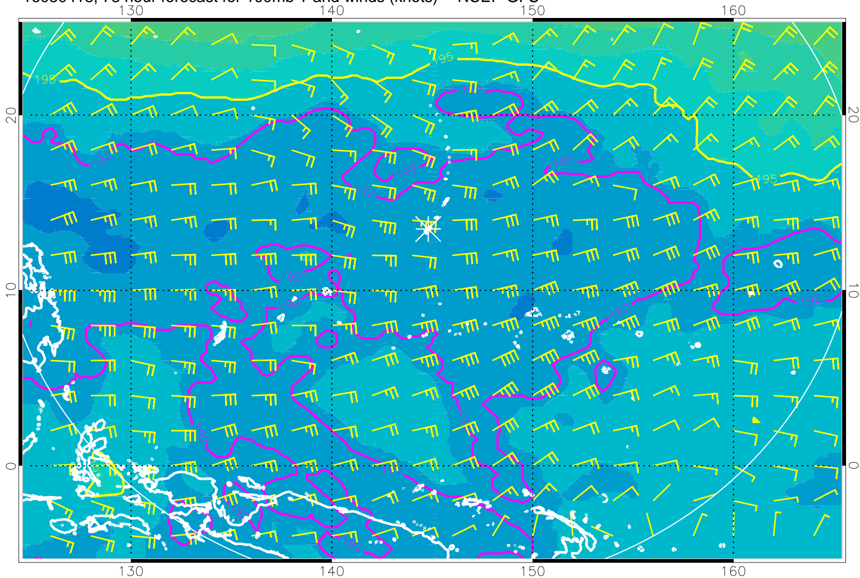
16080418, 78 hour forecast for 100mb T and winds (knots) -- NCEP GFS
