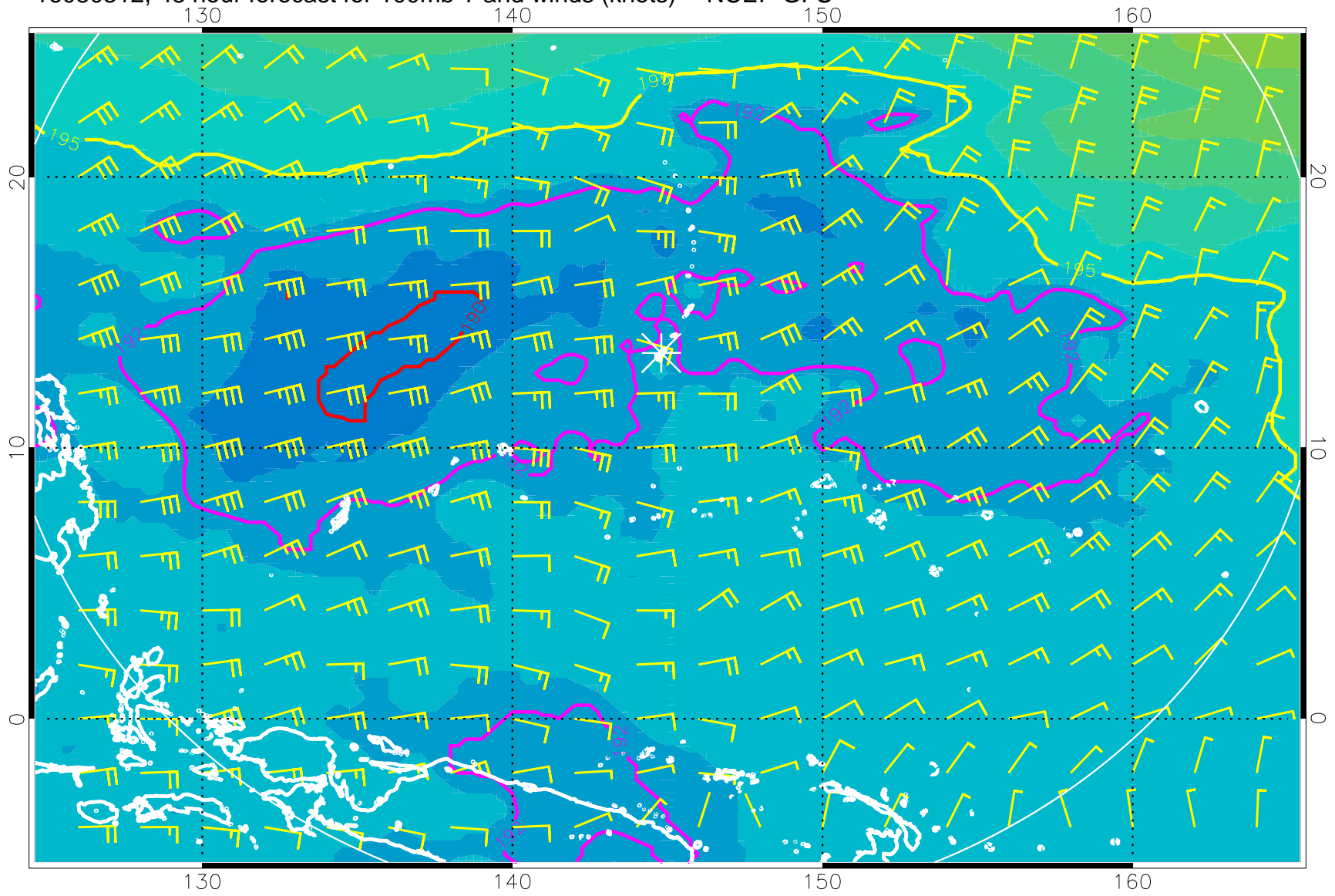
16080312, 48 hour forecast for 100mb T and winds (knots) -- NCEP GFS
