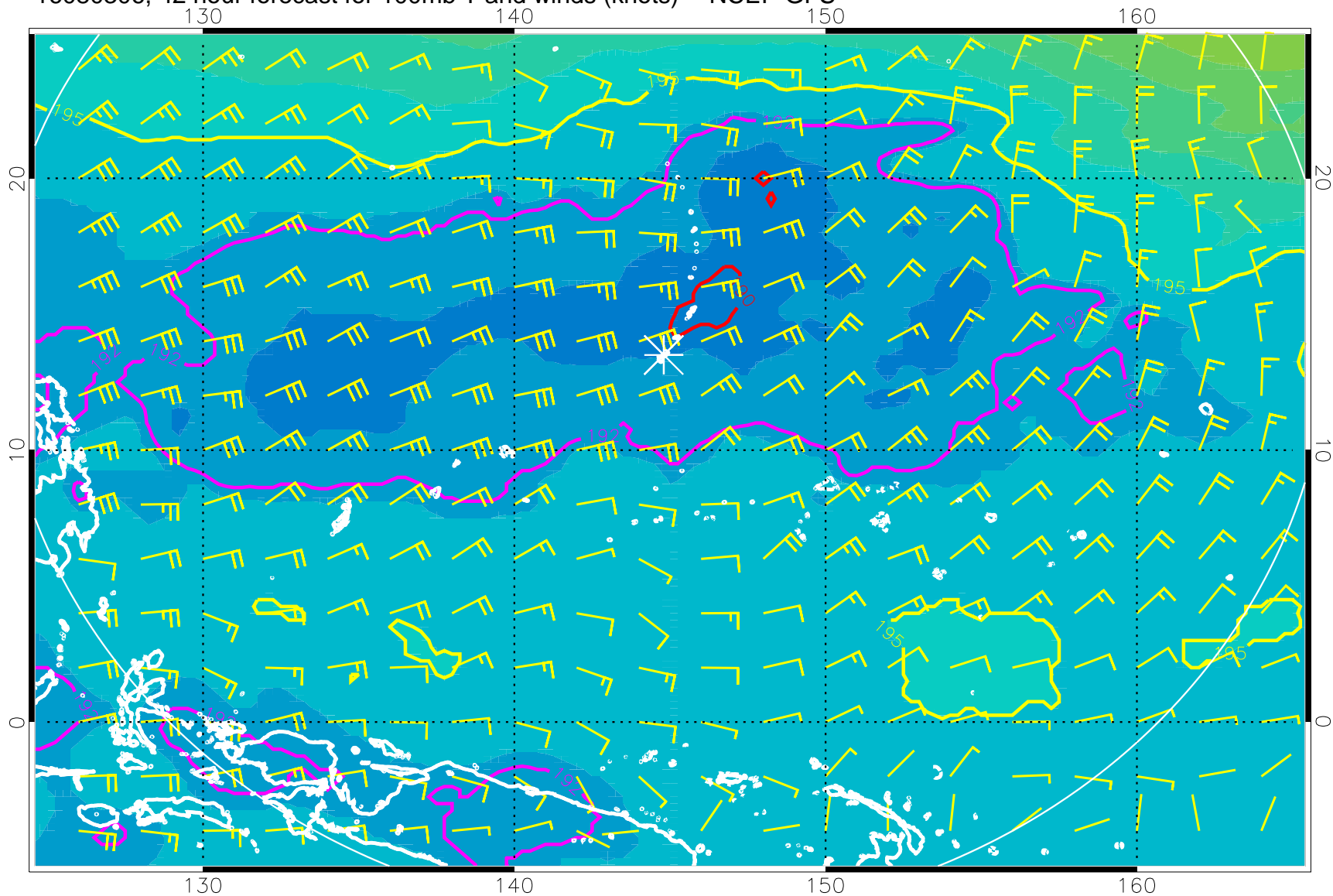
16080306, 42 hour forecast for 100mb T and winds (knots) -- NCEP GFS
