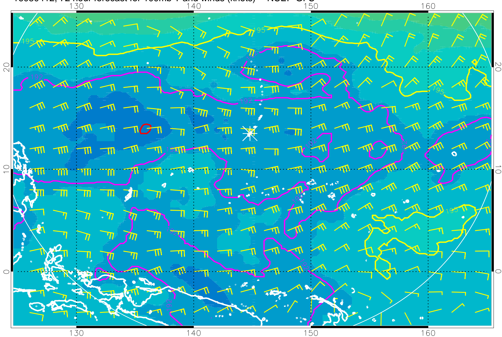
16080412, 72 hour forecast for 100mb T and winds (knots) -- NCEP GFS
