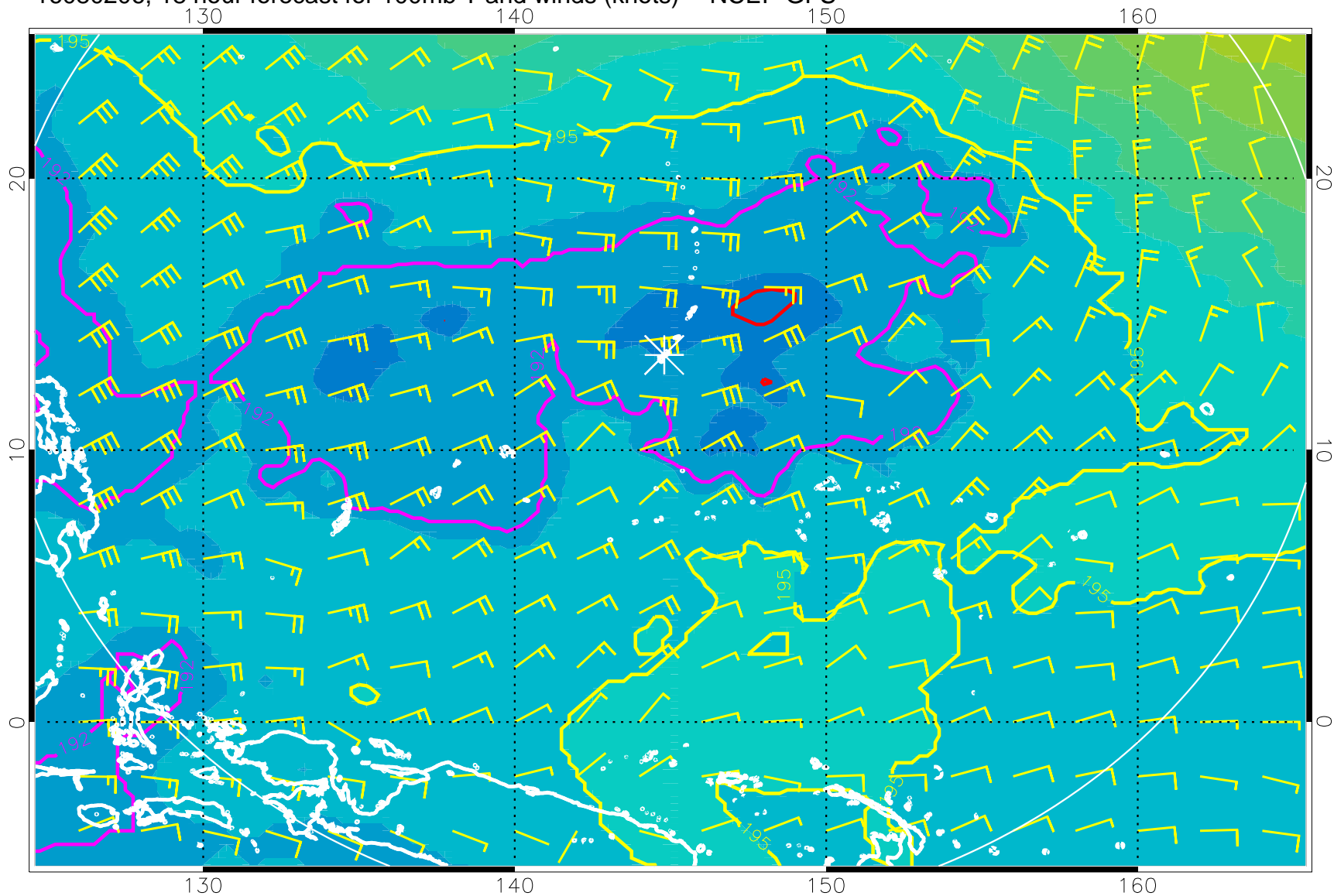
16080206, 18 hour forecast for 100mb T and winds (knots) -- NCEP GFS
