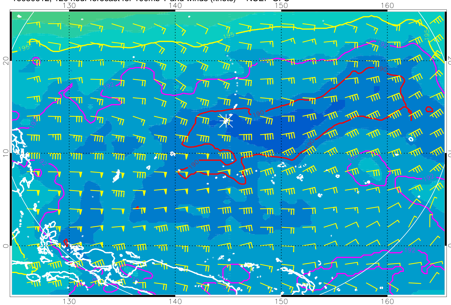
16080612, 120 hour forecast for 100mb T and winds (knots) -- NCEP GFS
