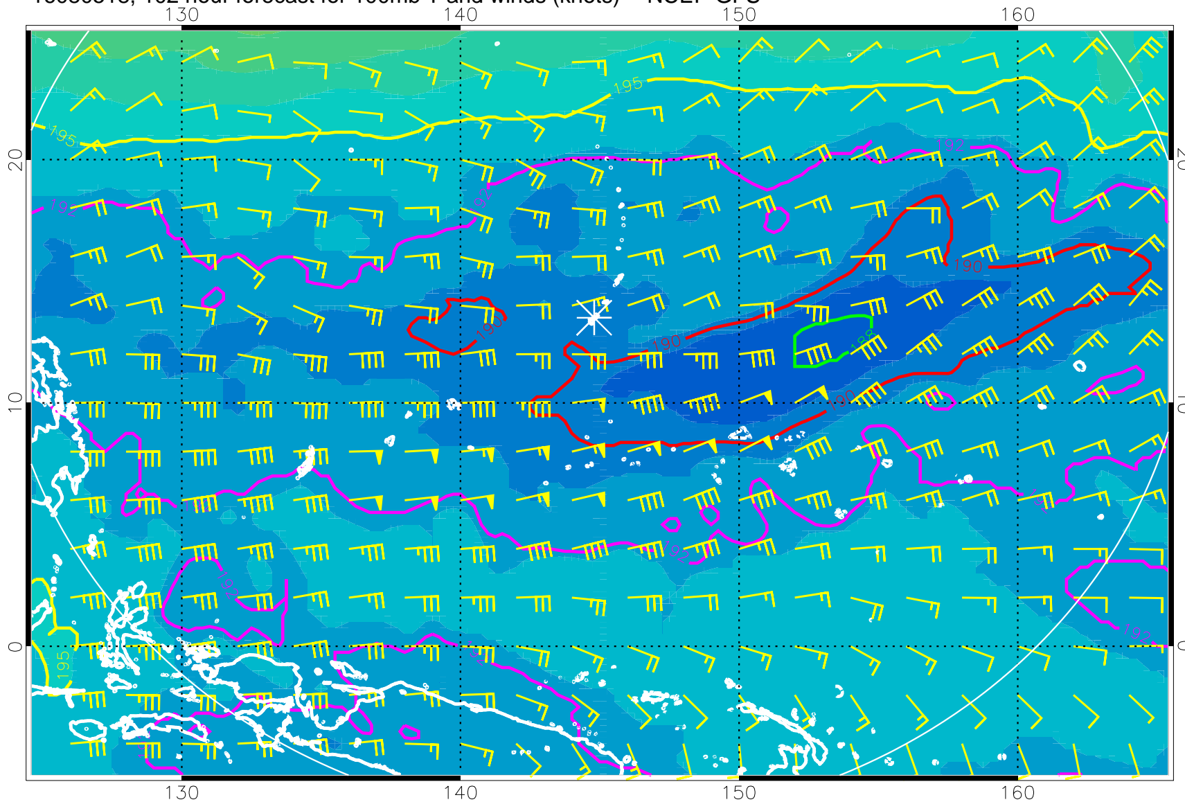
16080518, 102 hour forecast for 100mb T and winds (knots) -- NCEP GFS
