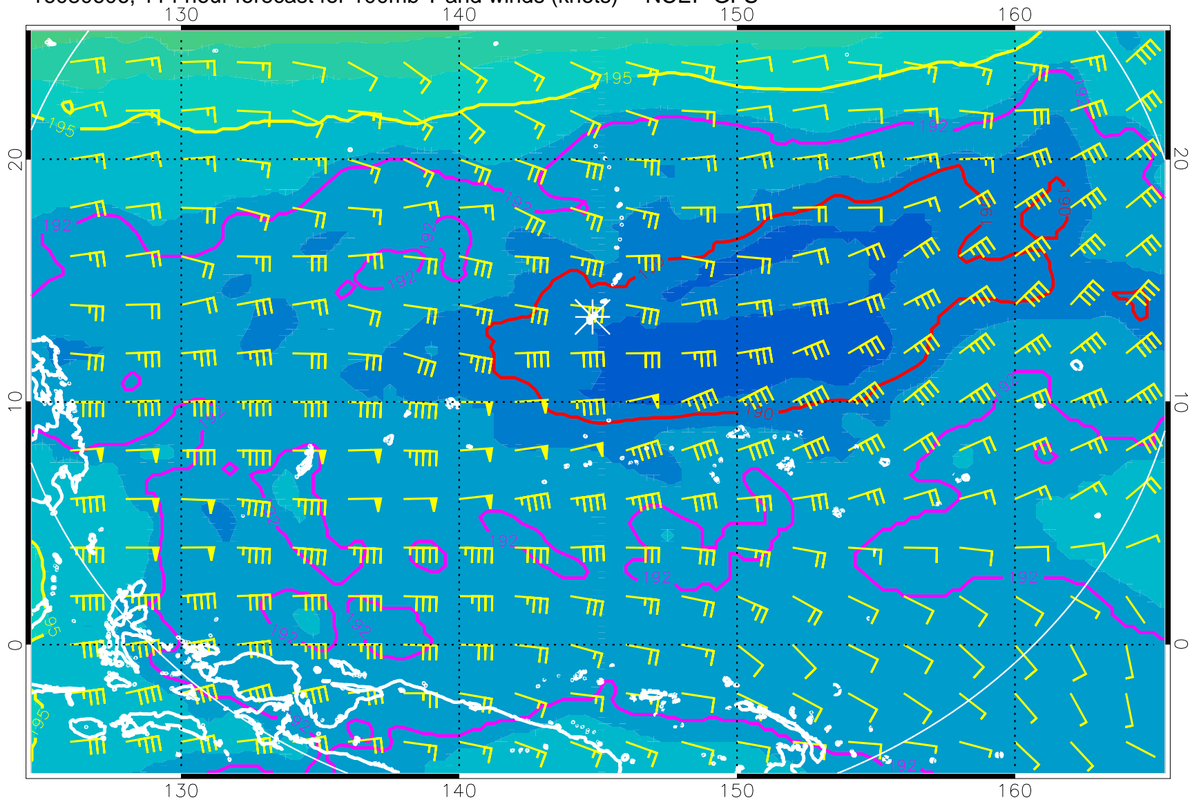
16080606, 114 hour forecast for 100mb T and winds (knots) -- NCEP GFS
