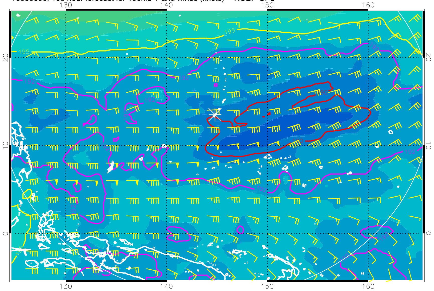
16080600, 108 hour forecast for 100mb T and winds (knots) -- NCEP GFS
