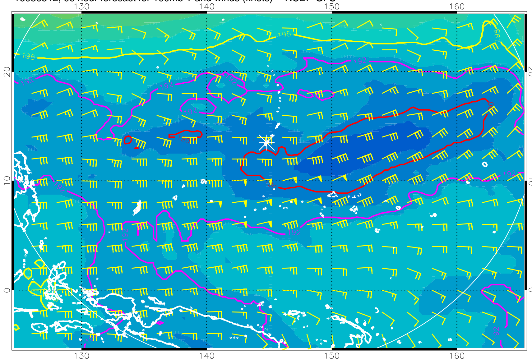
16080512, 96 hour forecast for 100mb T and winds (knots) -- NCEP GFS
