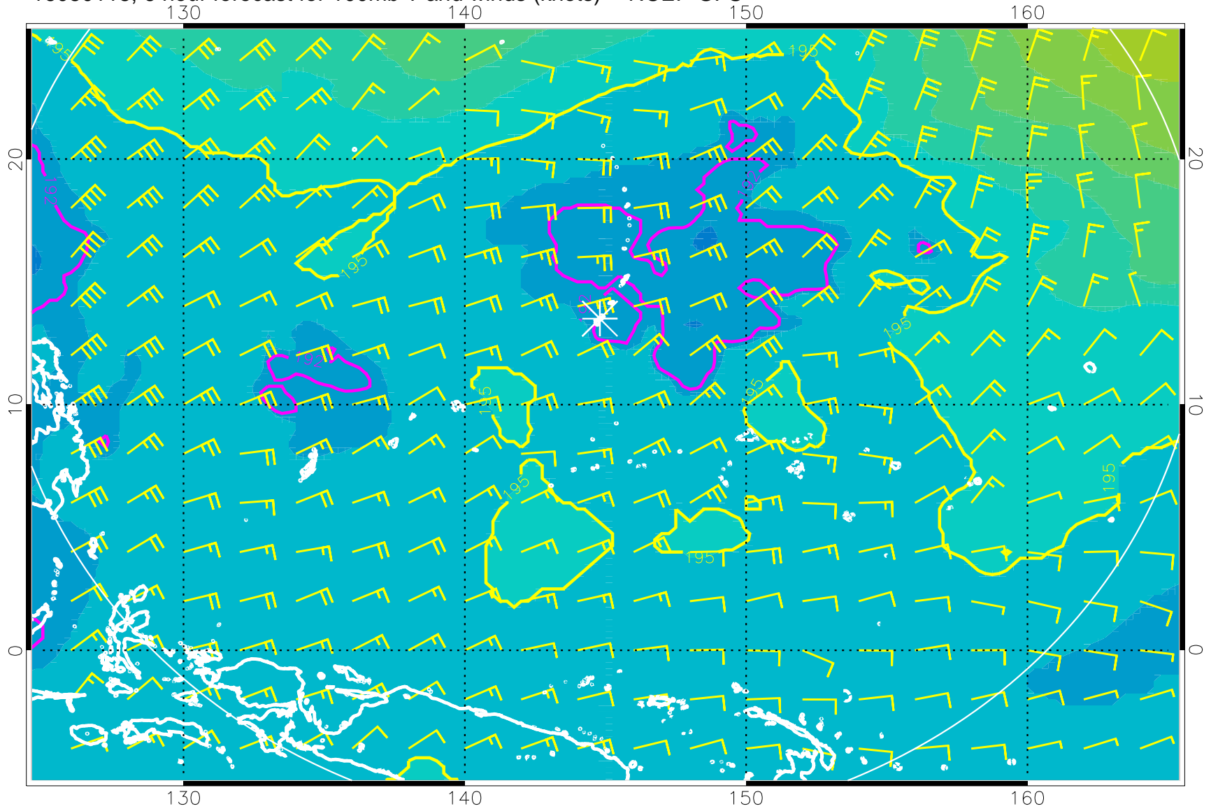
16080118, 6 hour forecast for 100mb T and winds (knots) -- NCEP GFS
