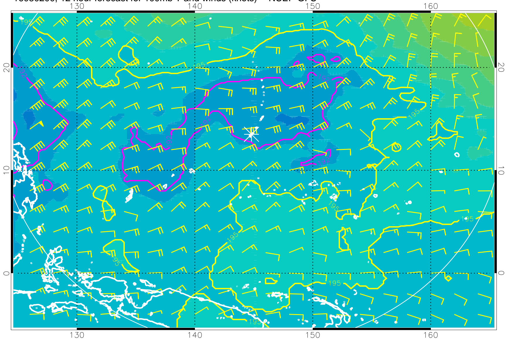
16080200, 12 hour forecast for 100mb T and winds (knots) -- NCEP GFS
