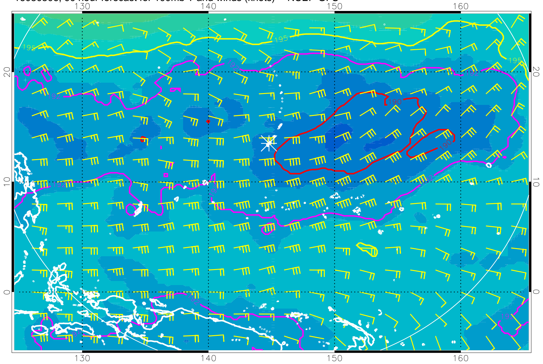
16080506, 90 hour forecast for 100mb T and winds (knots) -- NCEP GFS
