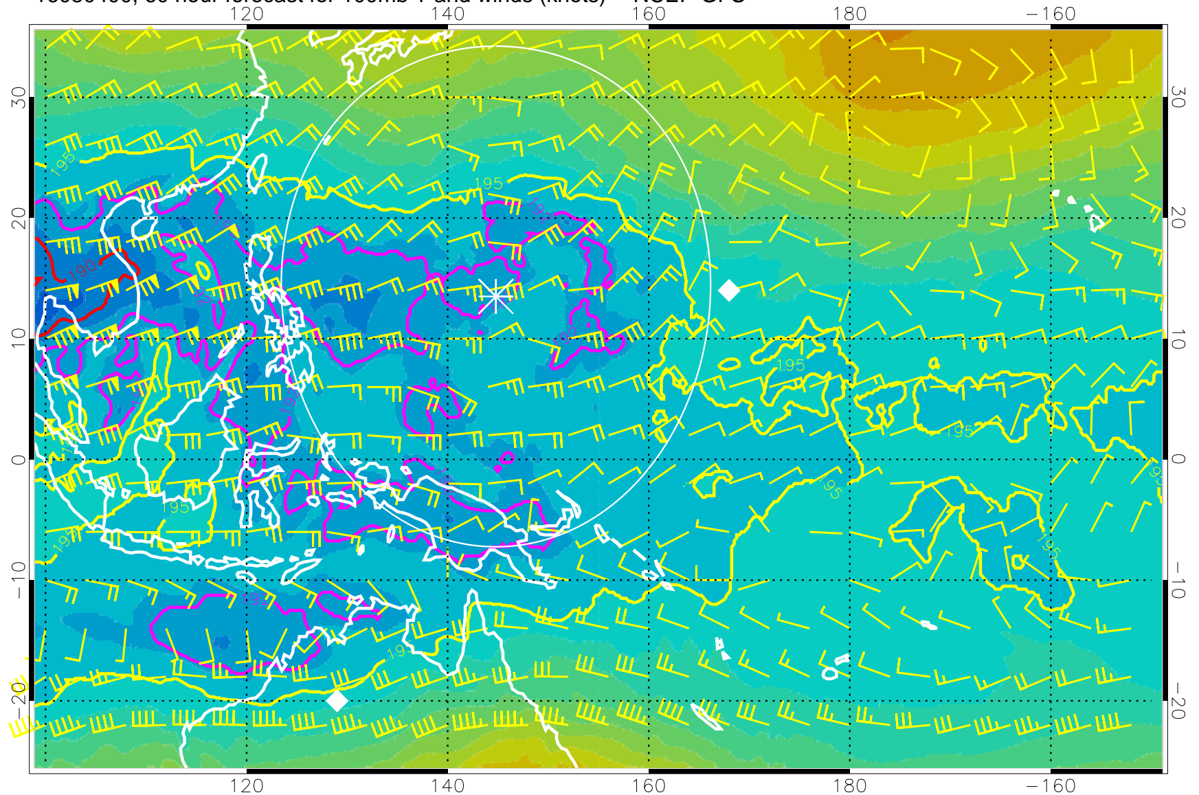
16080400, 60 hour forecast for 100mb T and winds (knots) -- NCEP GFS
