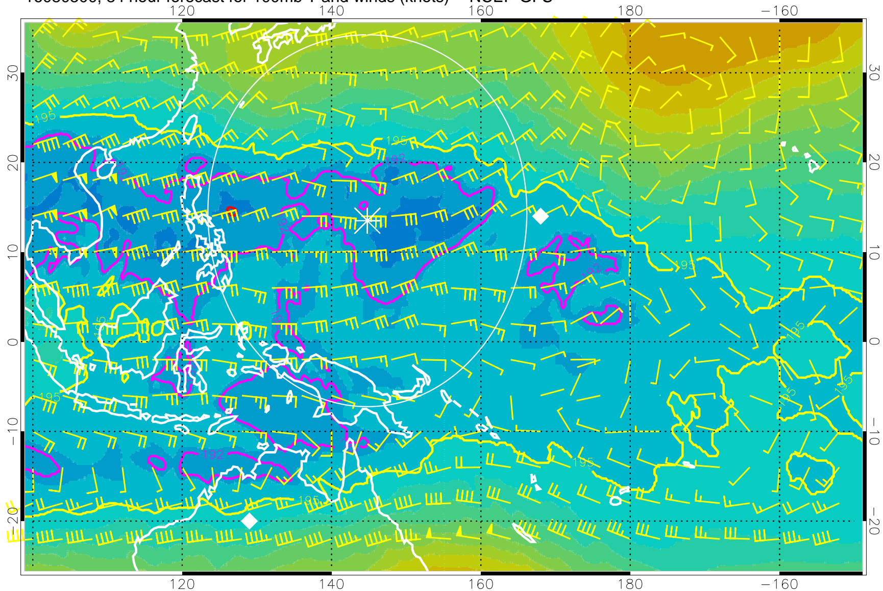
16080500, 84 hour forecast for 100mb T and winds (knots) -- NCEP GFS
