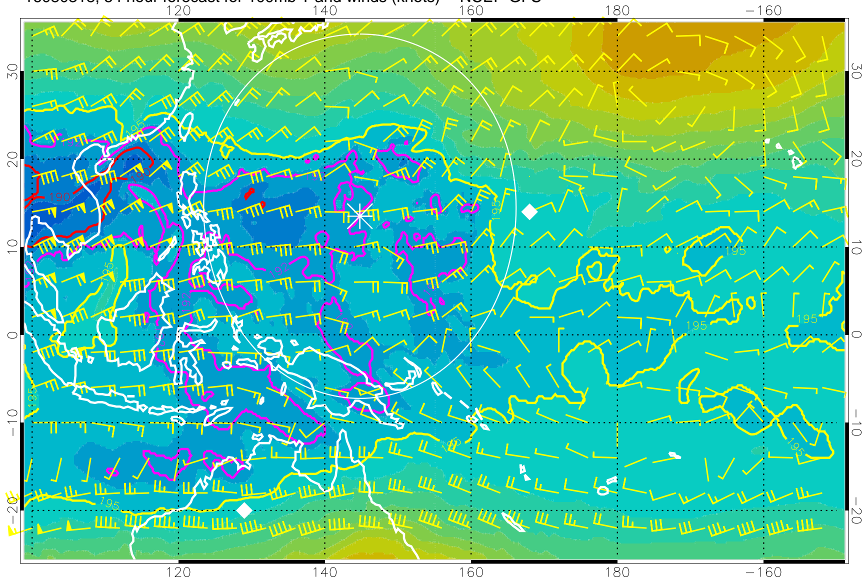
16080318, 54 hour forecast for 100mb T and winds (knots) -- NCEP GFS
