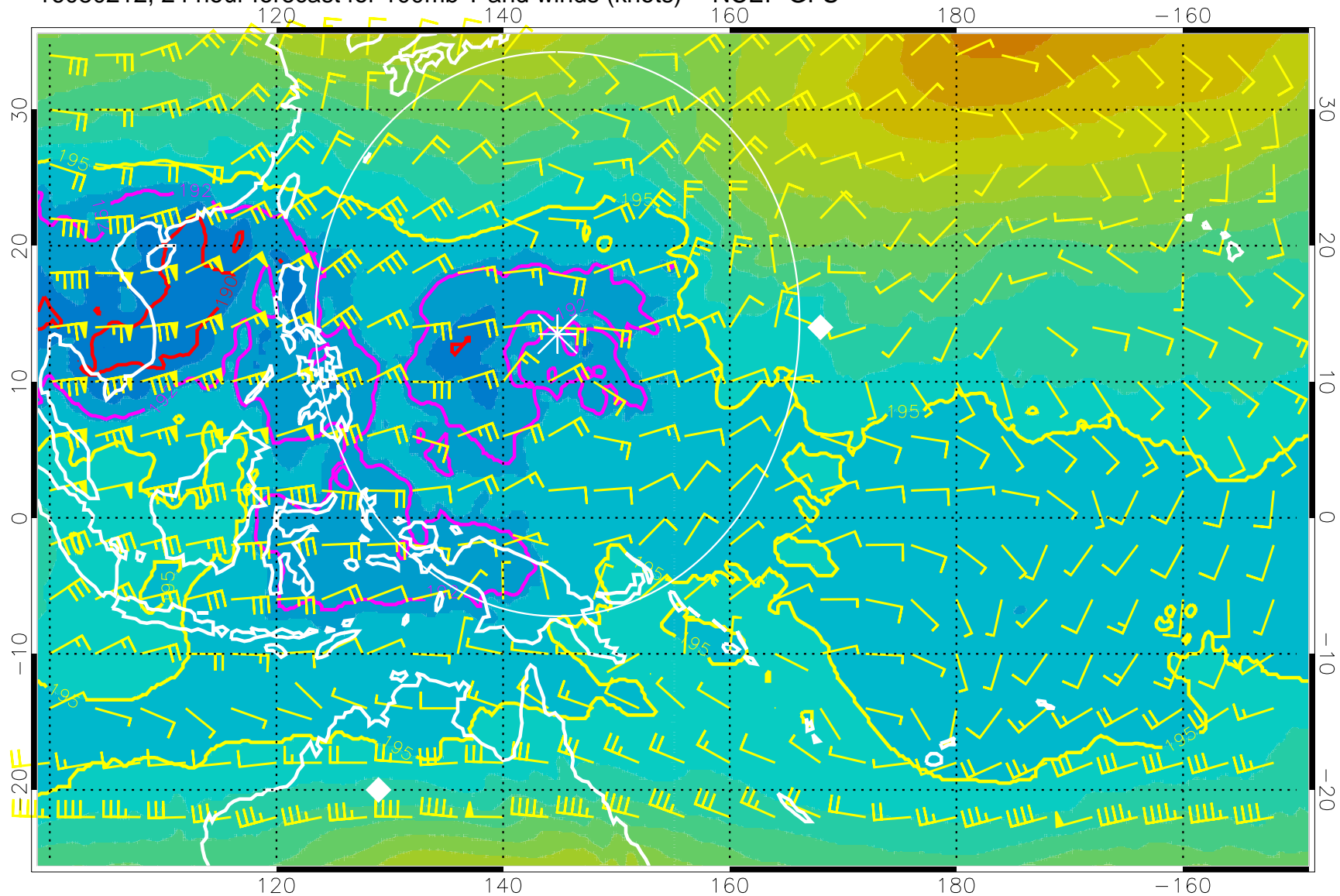
16080212, 24 hour forecast for 100mb T and winds (knots) -- NCEP GFS
