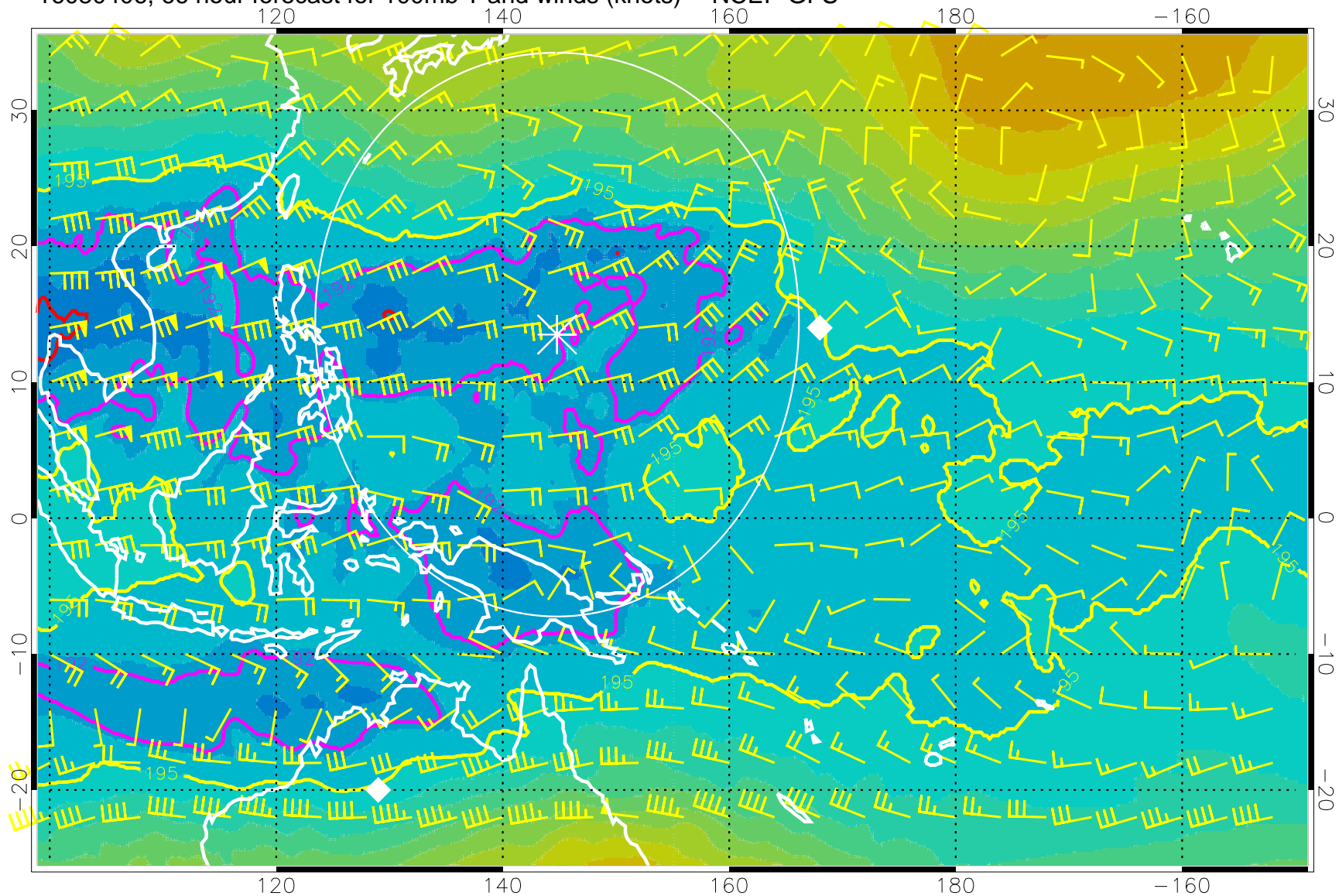
16080406, 66 hour forecast for 100mb T and winds (knots) -- NCEP GFS
