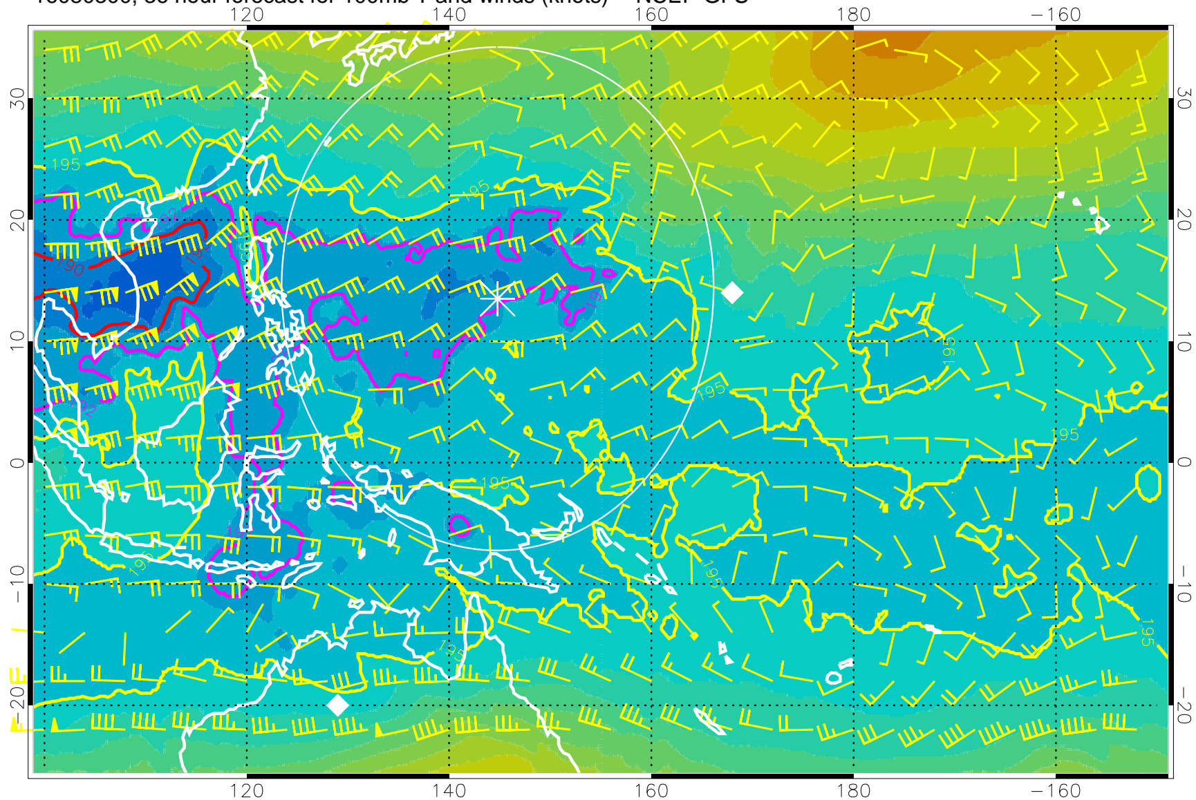
16080300, 36 hour forecast for 100mb T and winds (knots) -- NCEP GFS
