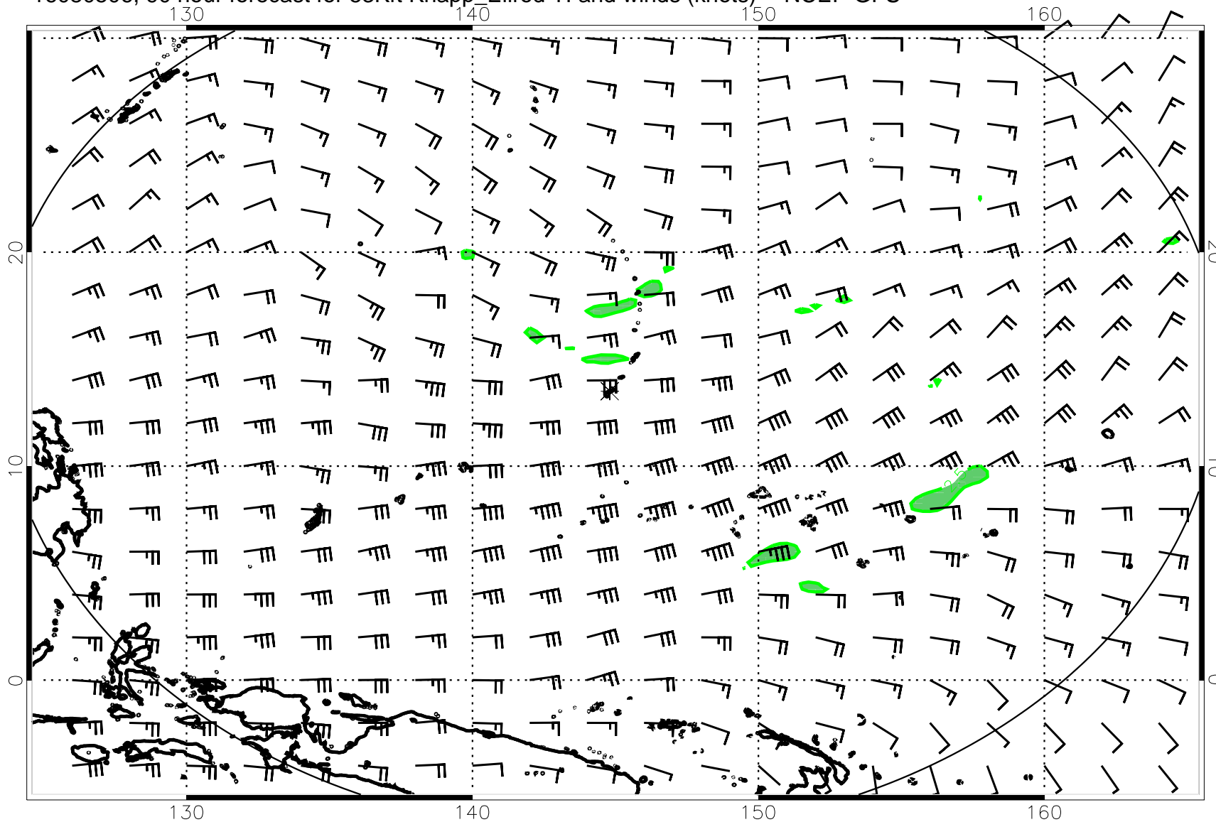
16080506, 90 hour forecast for 53Kft Knapp_Ellrod TI and winds (knots) -- NCEP GFS
