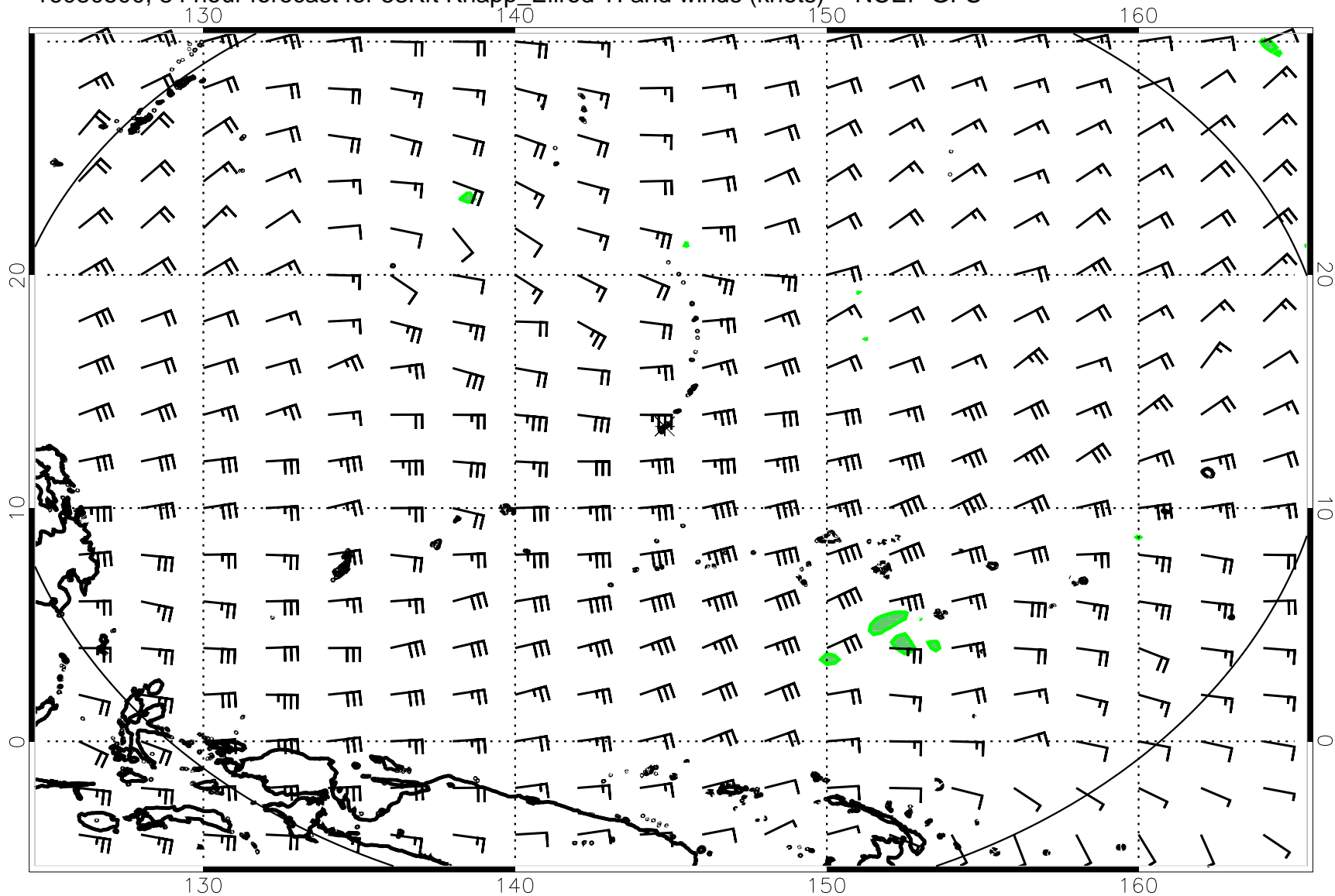
16080500, 84 hour forecast for 53Kft Knapp_Ellrod TI and winds (knots) -- NCEP GFS
