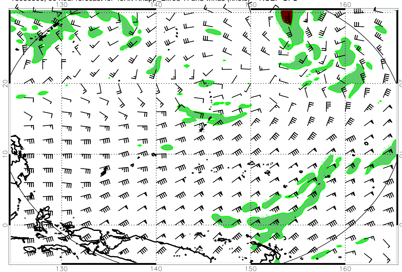
16080506, 90 hour forecast for 45Kft Knapp_Ellrod TI and winds (knots) -- NCEP GFS
