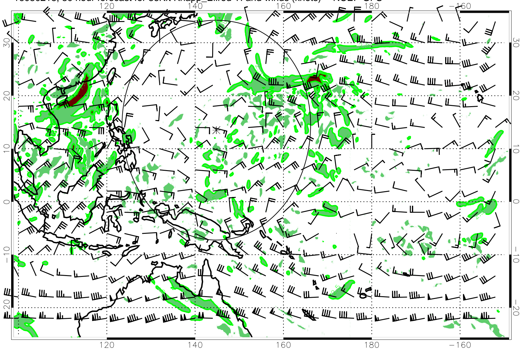
16080218, 30 hour forecast for 36Kft Knapp_Ellrod TI and winds (knots) -- NCEP GFS
