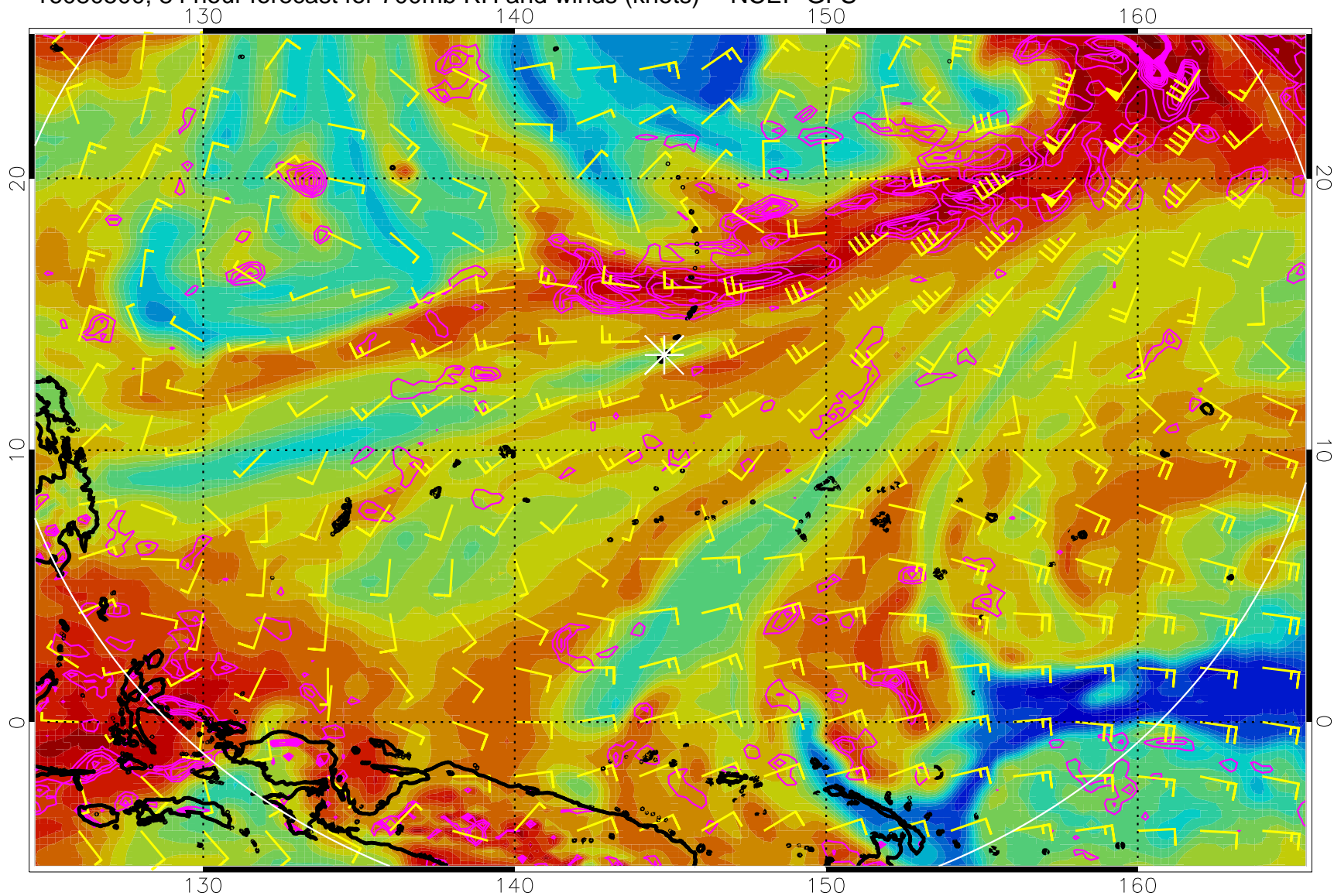
16080500, 84 hour forecast for 700mb RH and winds (knots) -- NCEP GFS
