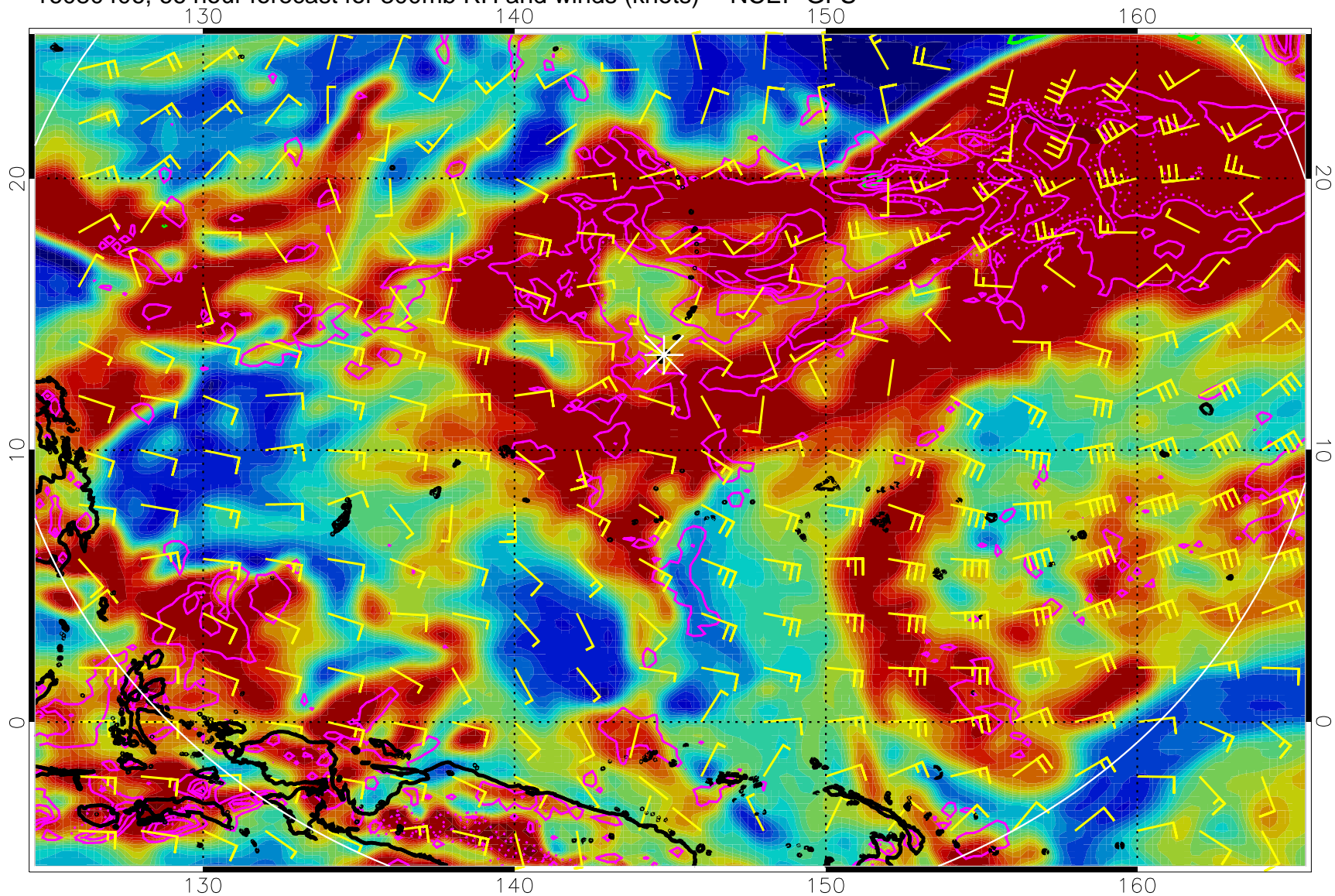
16080406, 66 hour forecast for 300mb RH and winds (knots) -- NCEP GFS
