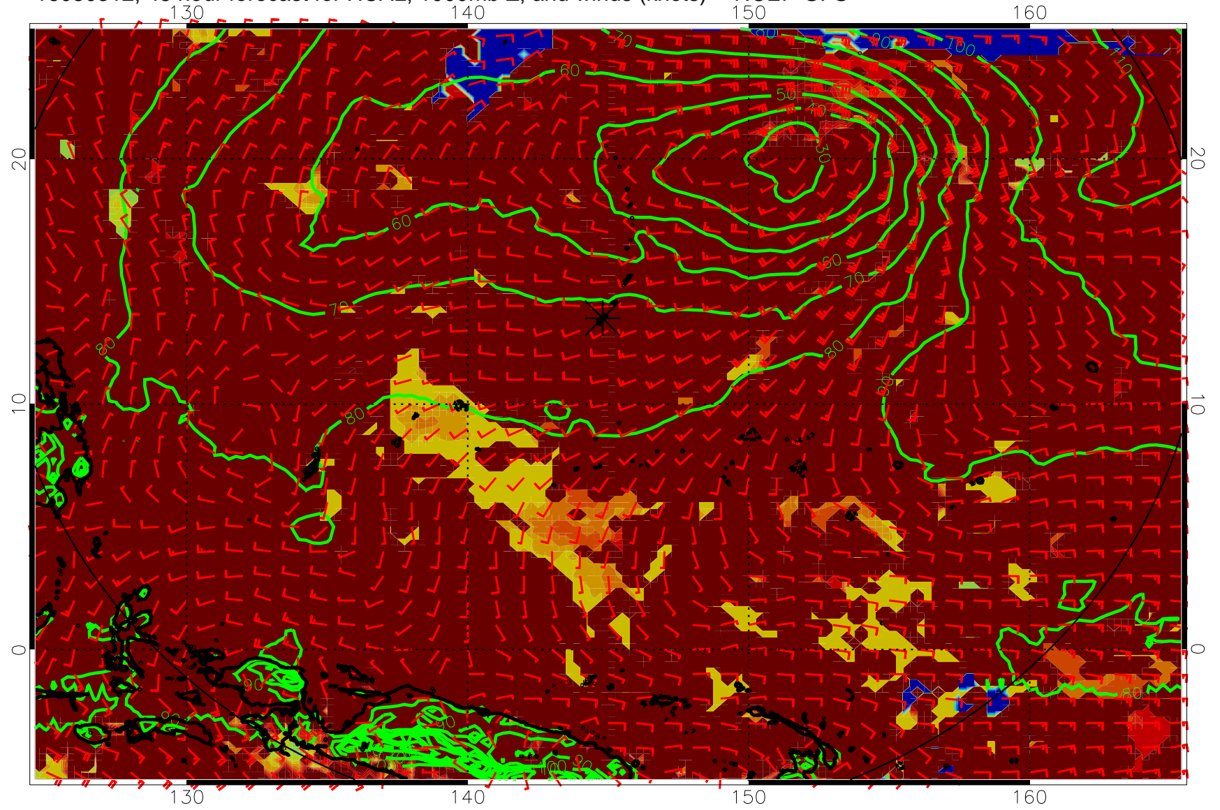
16080312, 48 hour forecast for HCAL, 1000mb Z, and winds (knots) -- NCEP GFS
