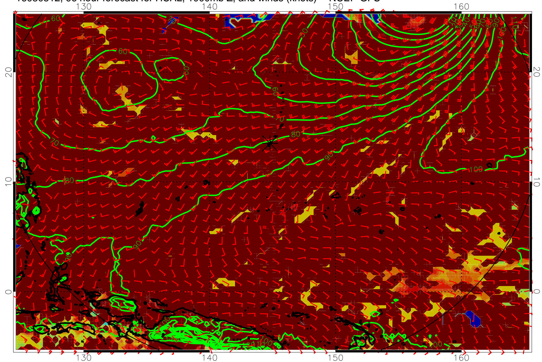
16080512, 96 hour forecast for HCAL, 1000mb Z, and winds (knots) -- NCEP GFS
