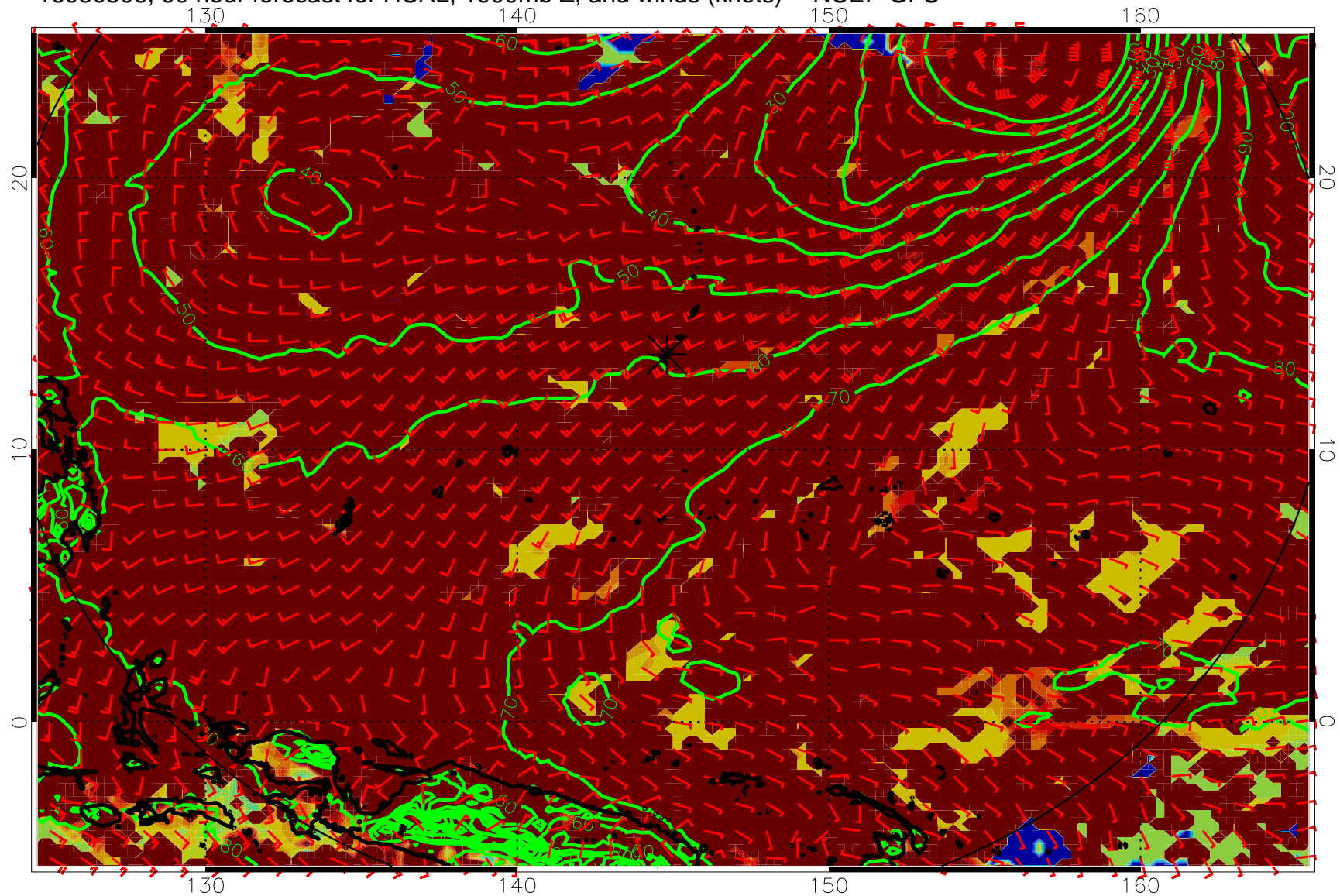
16080506, 90 hour forecast for HCAL, 1000mb Z, and winds (knots) -- NCEP GFS
