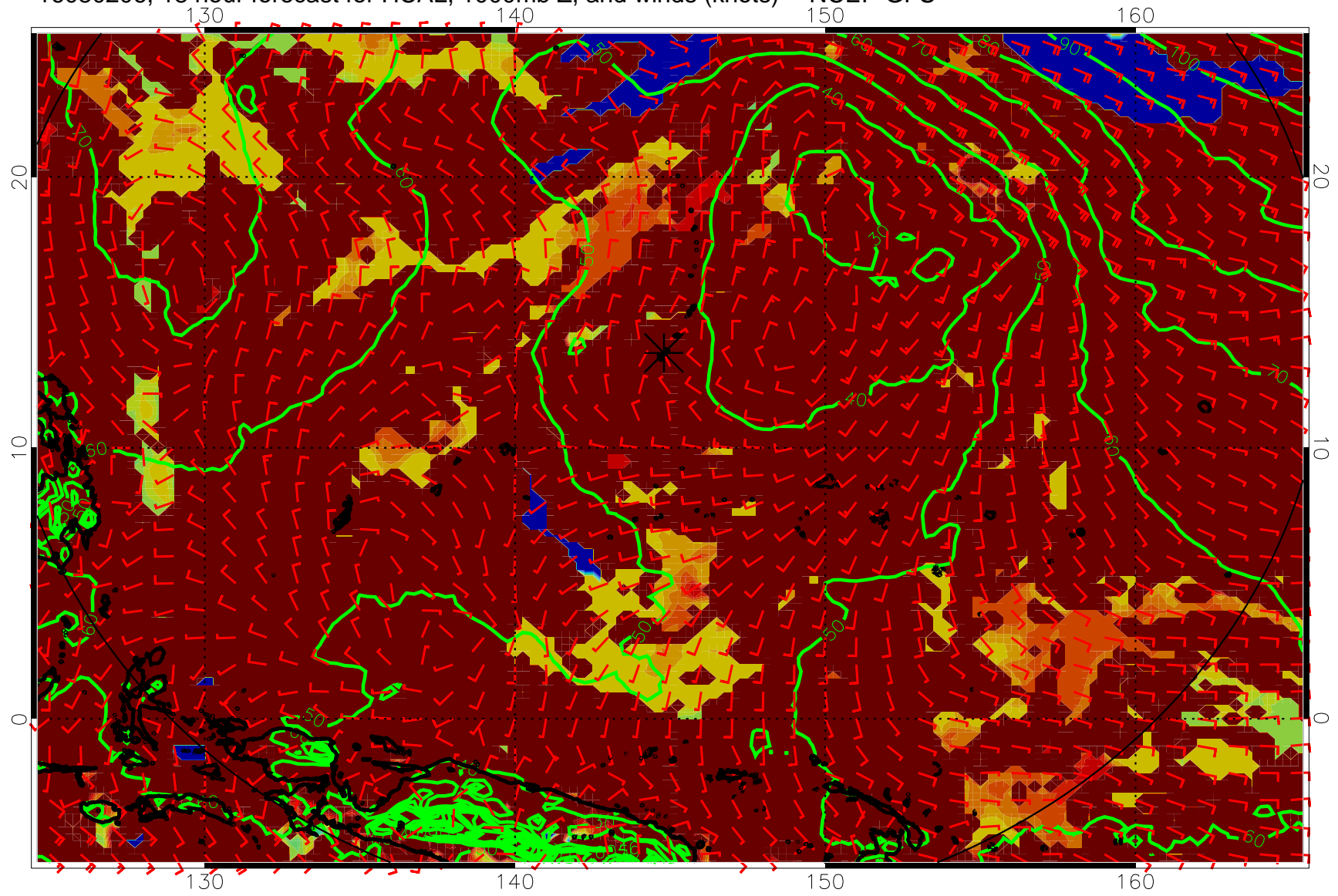
16080206, 18 hour forecast for HCAL, 1000mb Z, and winds (knots) -- NCEP GFS
