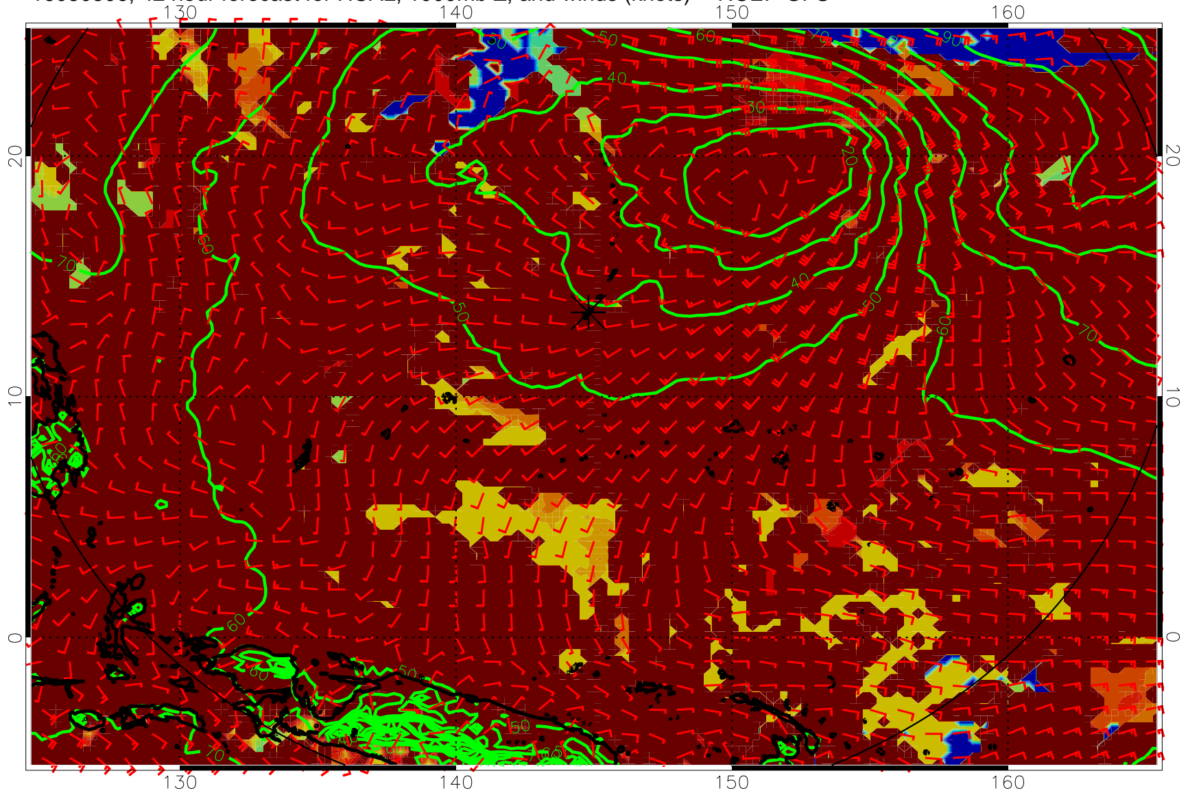
16080306, 42 hour forecast for HCAL, 1000mb Z, and winds (knots) -- NCEP GFS
