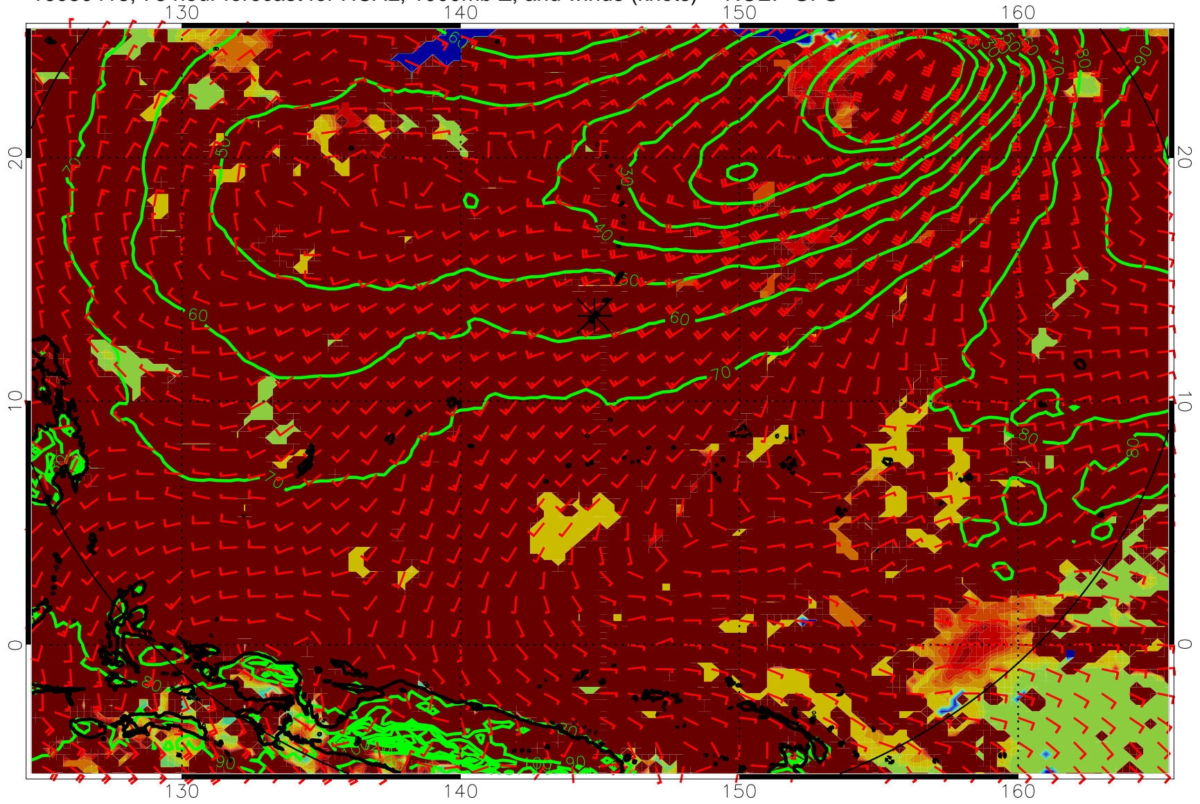
16080418, 78 hour forecast for HCAL, 1000mb Z, and winds (knots) -- NCEP GFS
