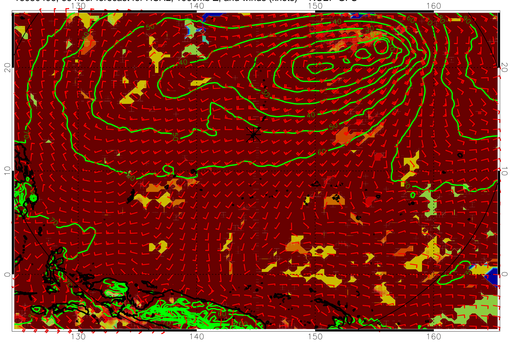
16080406, 66 hour forecast for HCAL, 1000mb Z, and winds (knots) -- NCEP GFS
