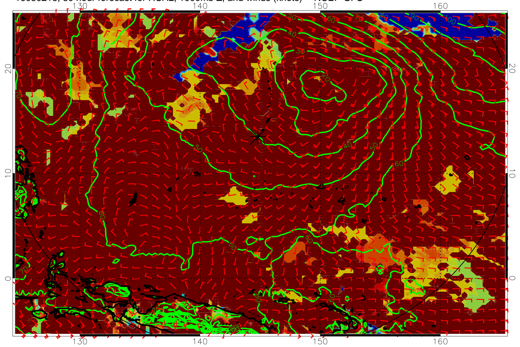
16080218, 30 hour forecast for HCAL, 1000mb Z, and winds (knots) -- NCEP GFS
