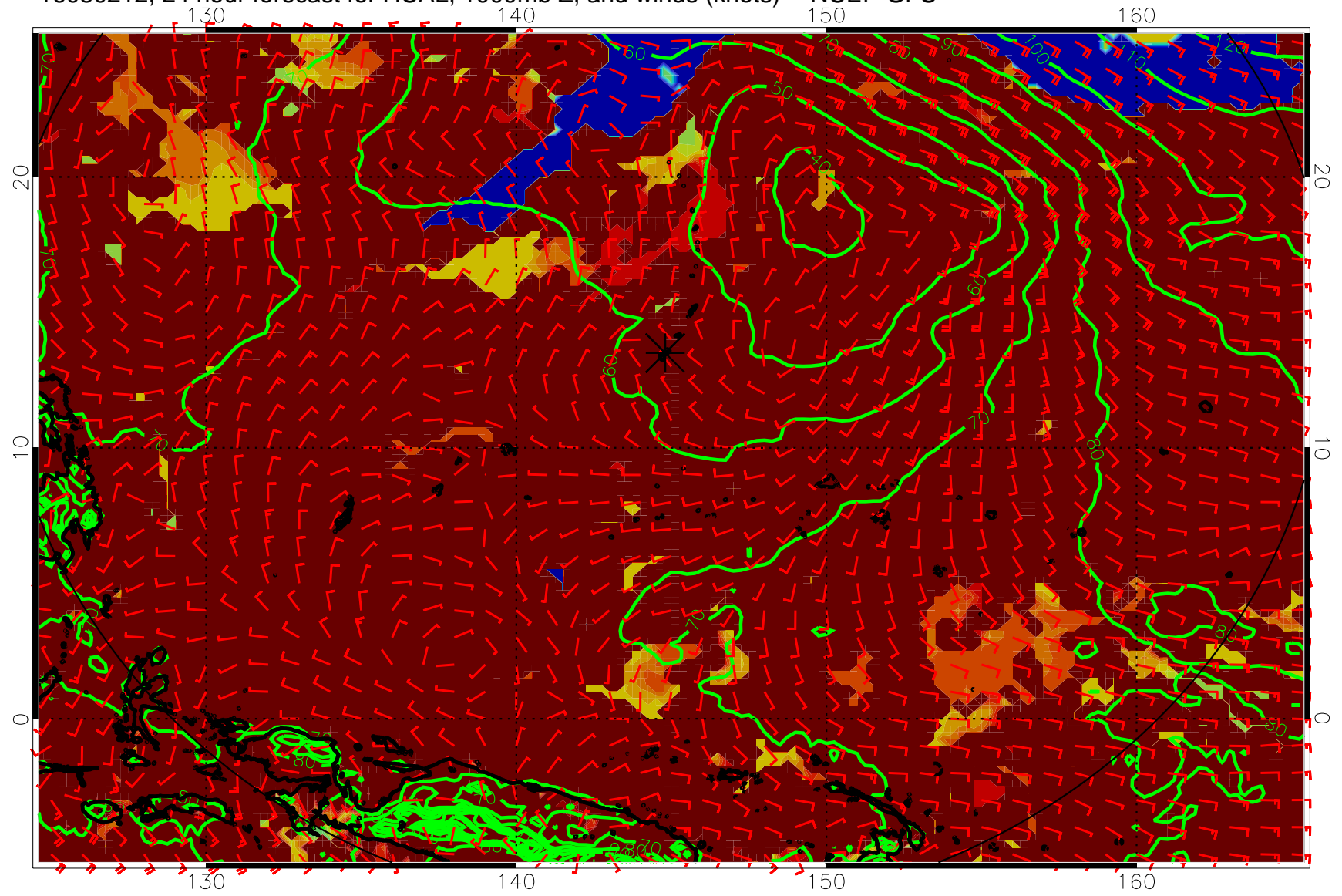
16080212, 24 hour forecast for HCAL, 1000mb Z, and winds (knots) -- NCEP GFS
