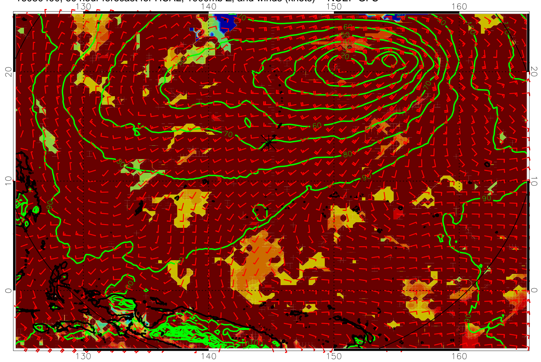
16080400, 60 hour forecast for HCAL, 1000mb Z, and winds (knots) -- NCEP GFS
