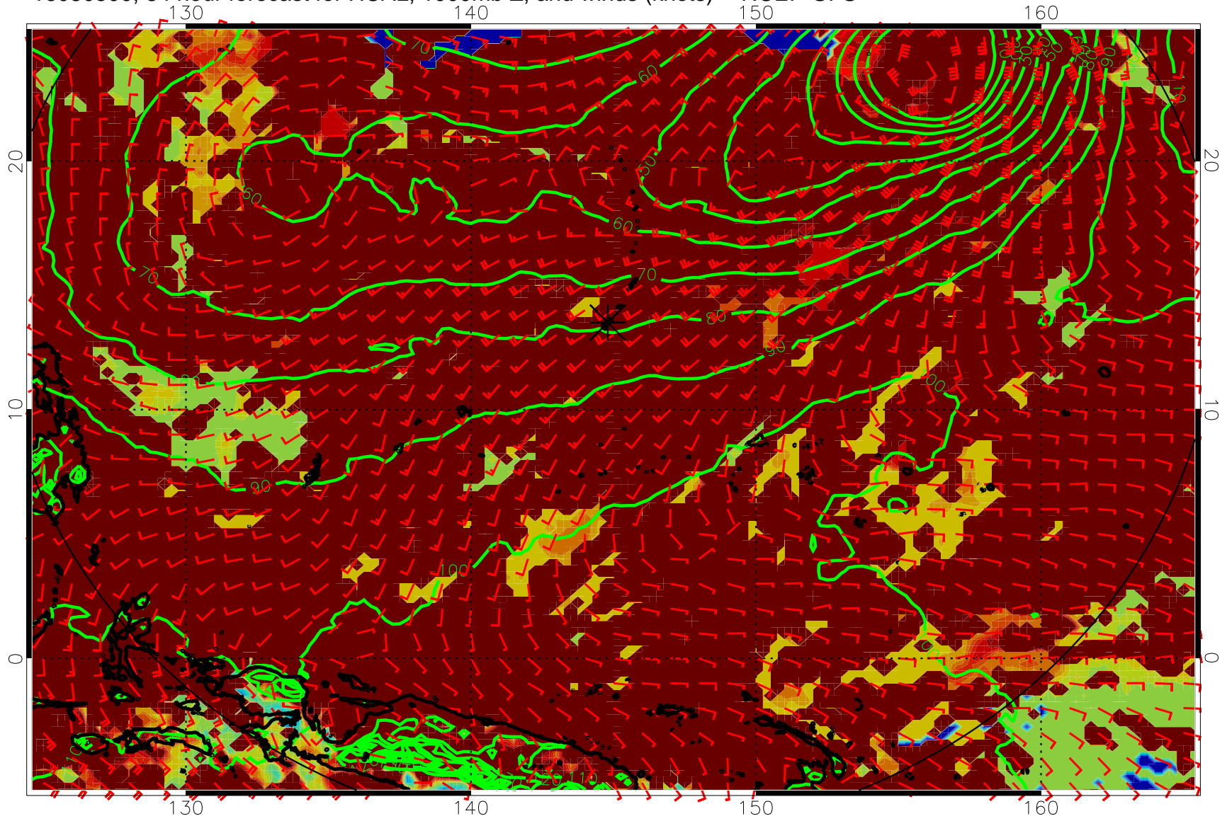
16080500, 84 hour forecast for HCAL, 1000mb Z, and winds (knots) -- NCEP GFS
