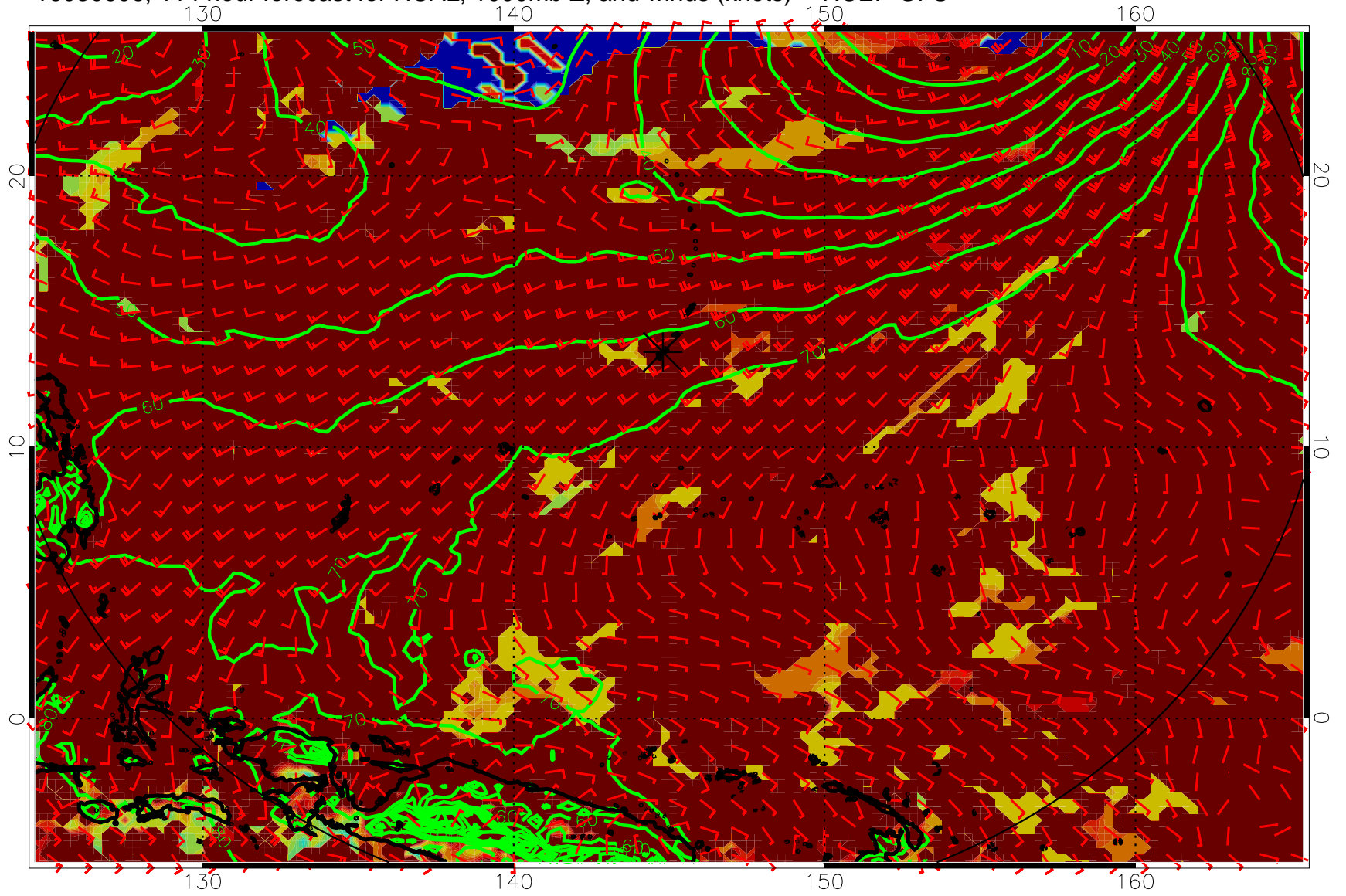
16080606, 114 hour forecast for HCAL, 1000mb Z, and winds (knots) -- NCEP GFS
