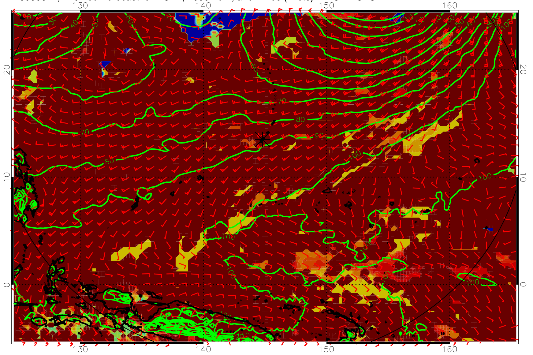
16080612, 120 hour forecast for HCAL, 1000mb Z, and winds (knots) -- NCEP GFS
