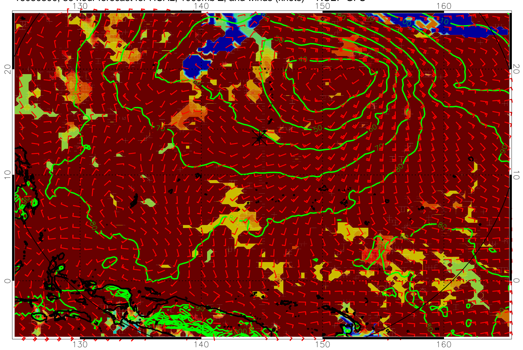
16080300, 36 hour forecast for HCAL, 1000mb Z, and winds (knots) -- NCEP GFS
