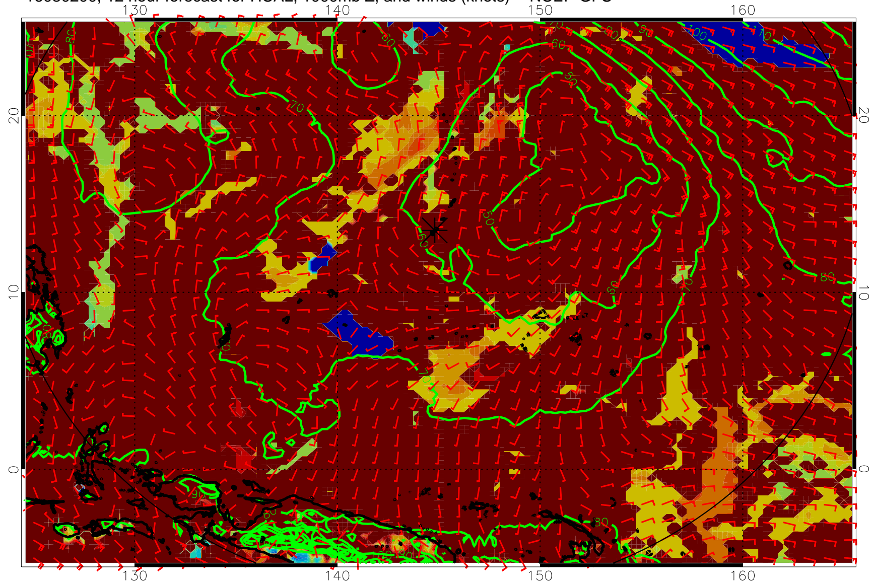
16080200, 12 hour forecast for HCAL, 1000mb Z, and winds (knots) -- NCEP GFS
