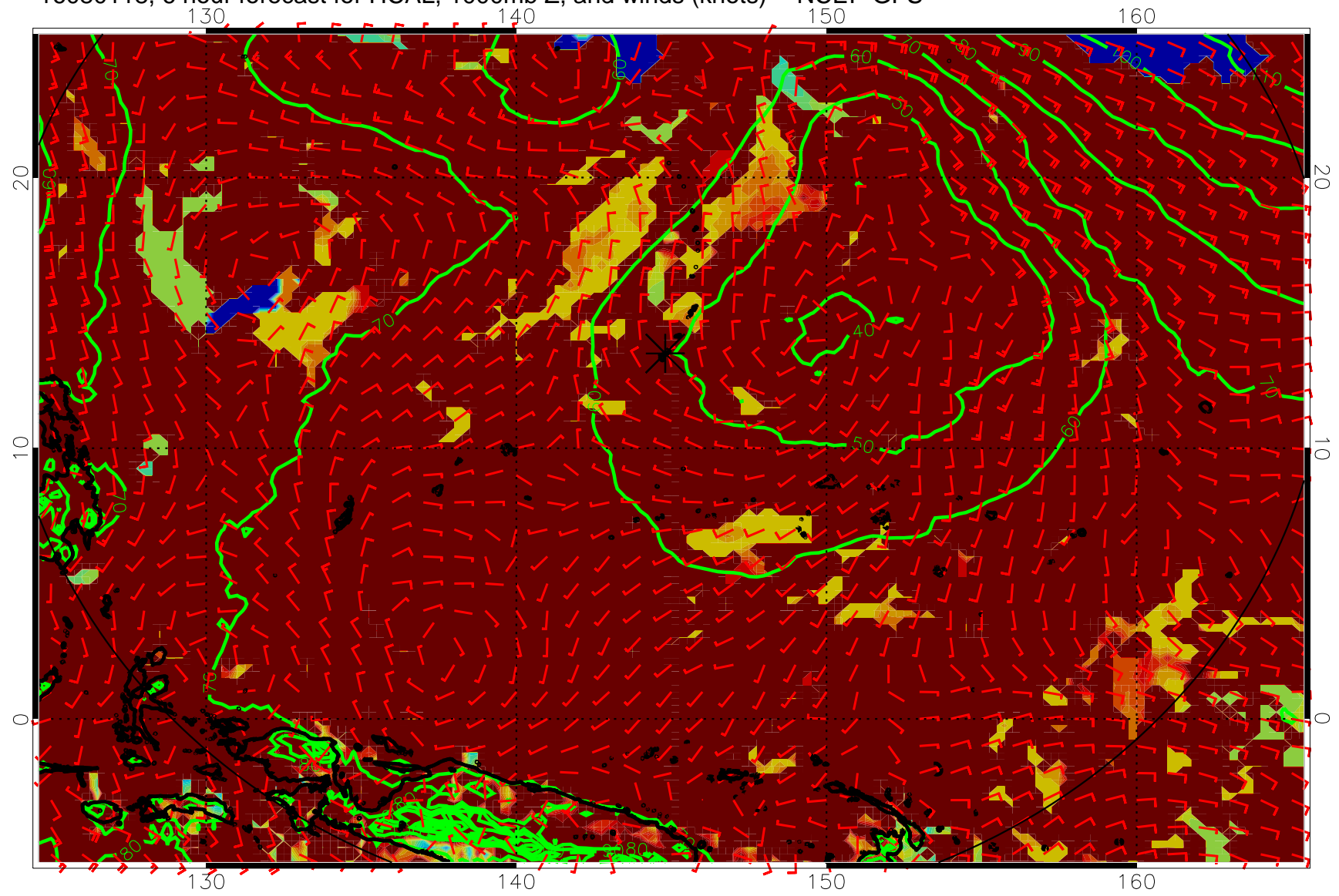
16080118, 6 hour forecast for HCAL, 1000mb Z, and winds (knots) -- NCEP GFS
