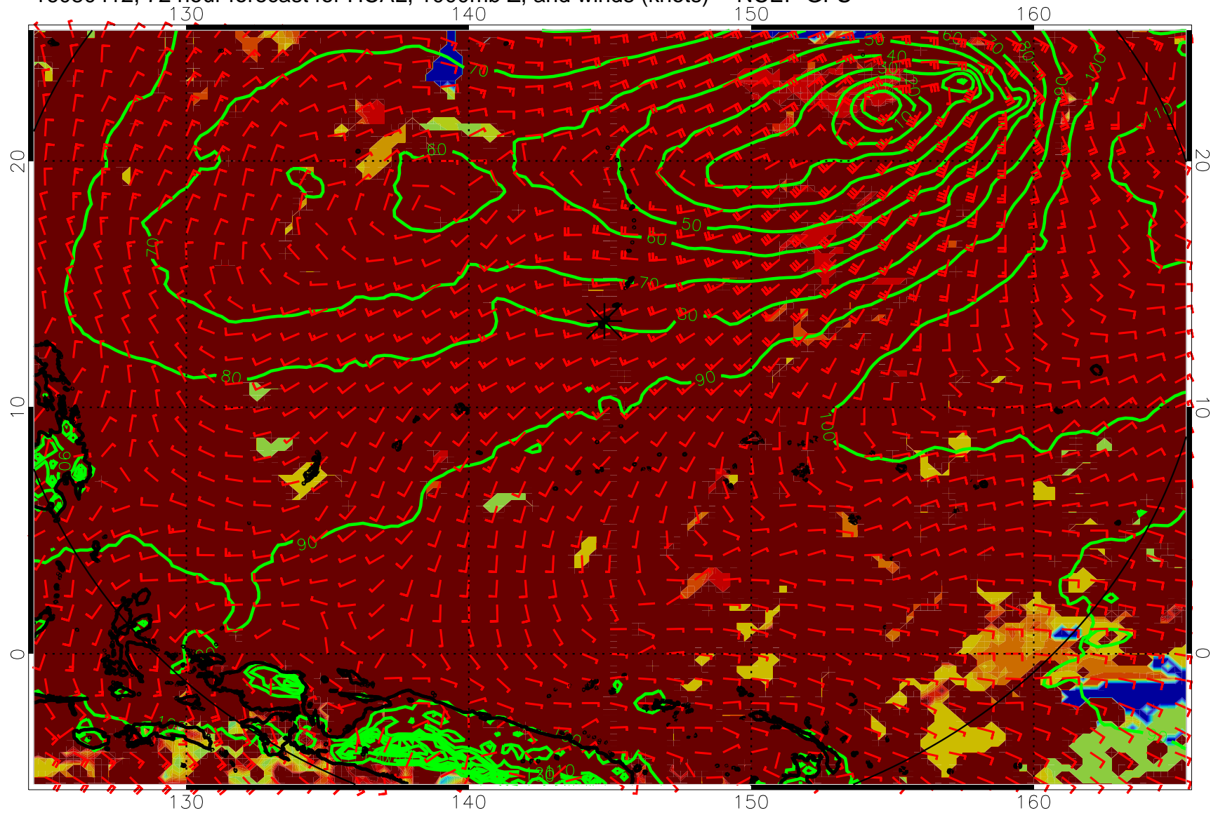
16080412, 72 hour forecast for HCAL, 1000mb Z, and winds (knots) -- NCEP GFS
