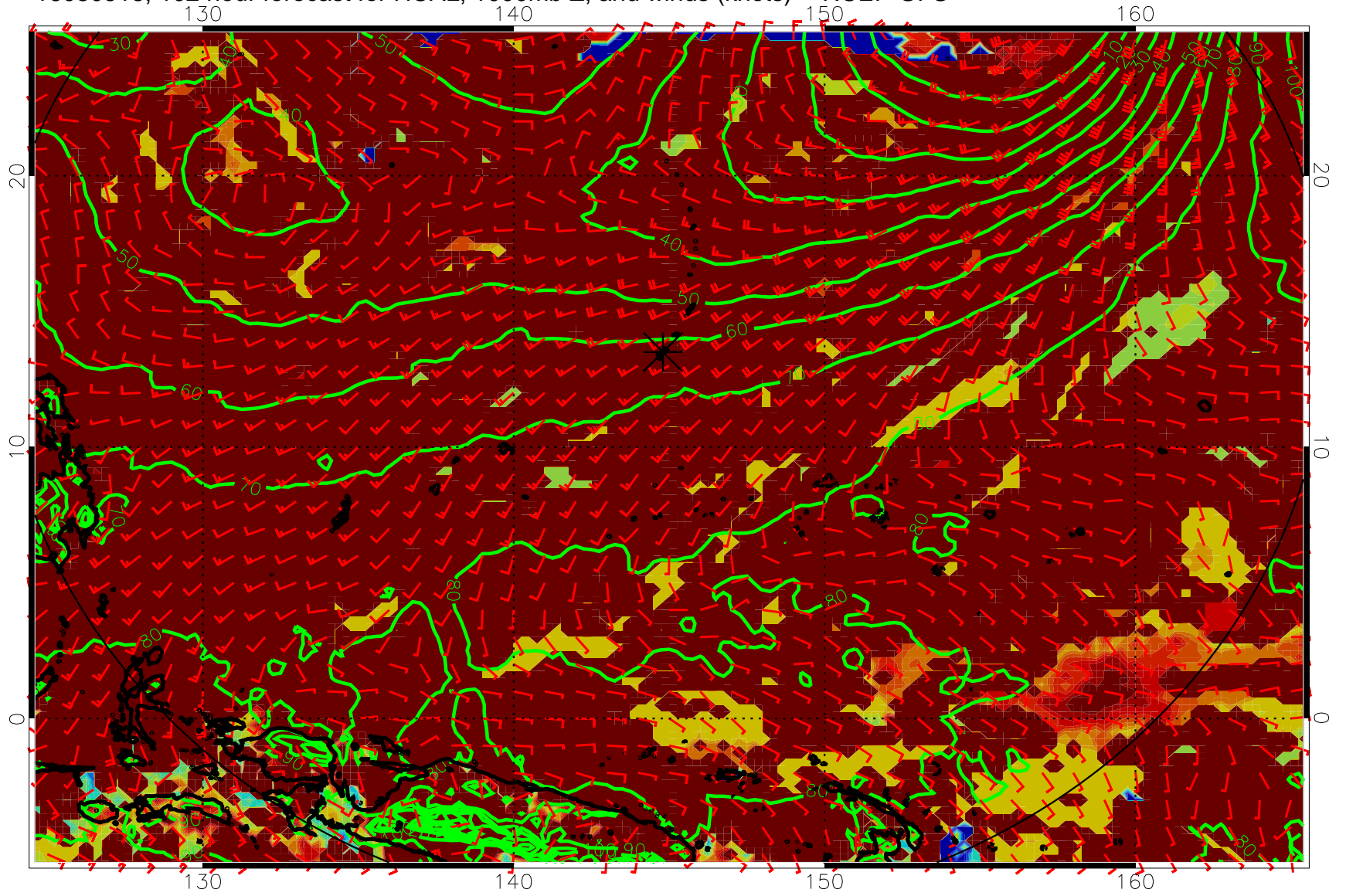
16080518, 102 hour forecast for HCAL, 1000mb Z, and winds (knots) -- NCEP GFS
