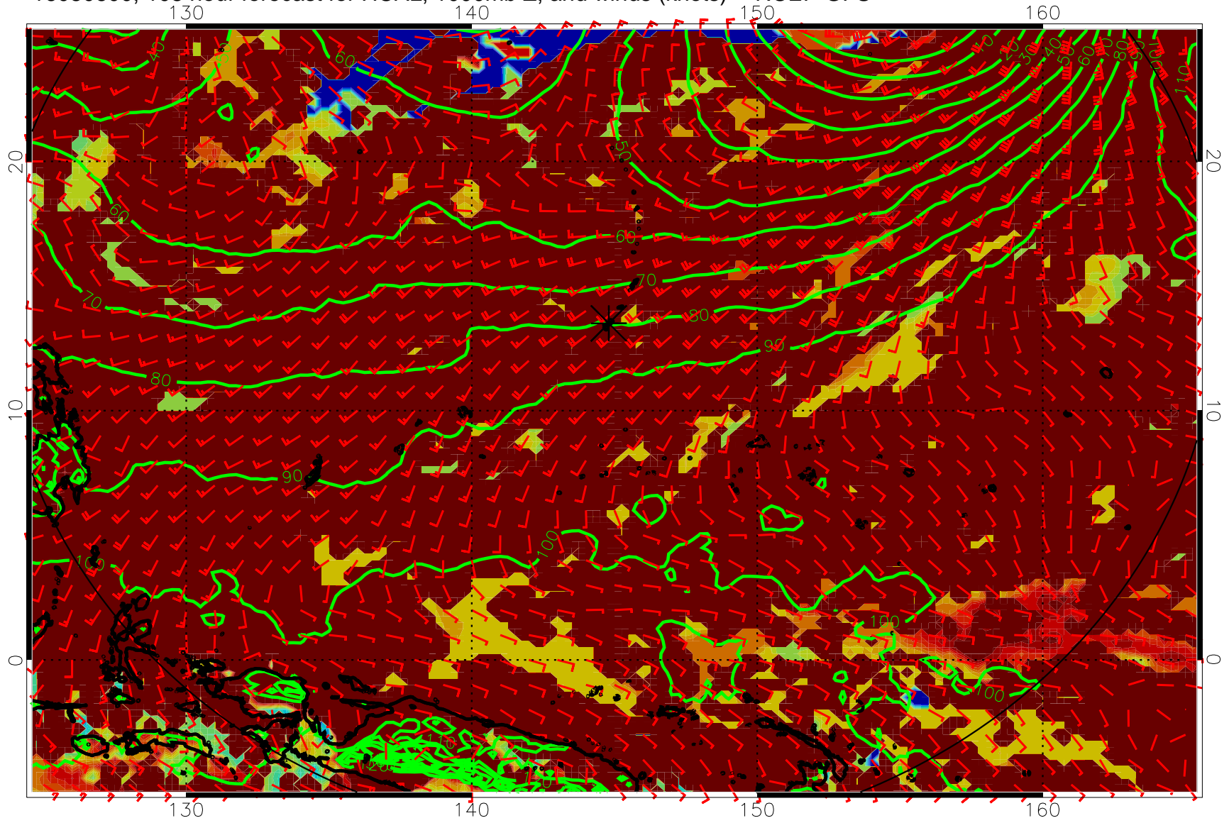
16080600, 108 hour forecast for HCAL, 1000mb Z, and winds (knots) -- NCEP GFS
