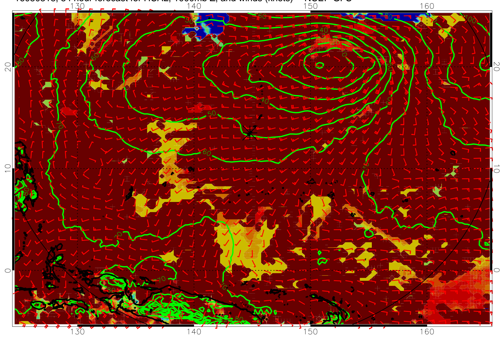
16080318, 54 hour forecast for HCAL, 1000mb Z, and winds (knots) -- NCEP GFS
