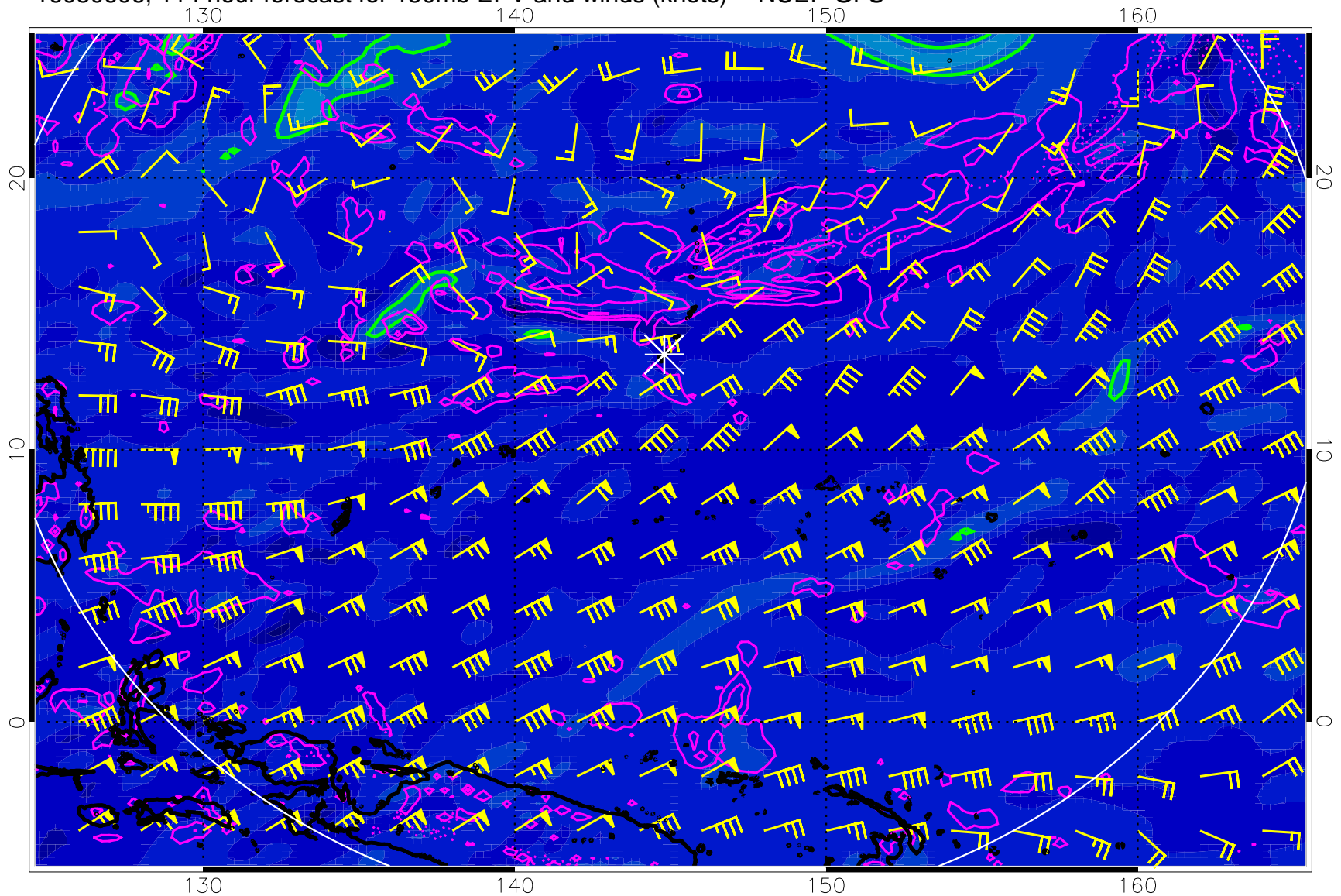
16080606, 114 hour forecast for 150mb EPV and winds (knots) -- NCEP GFS
