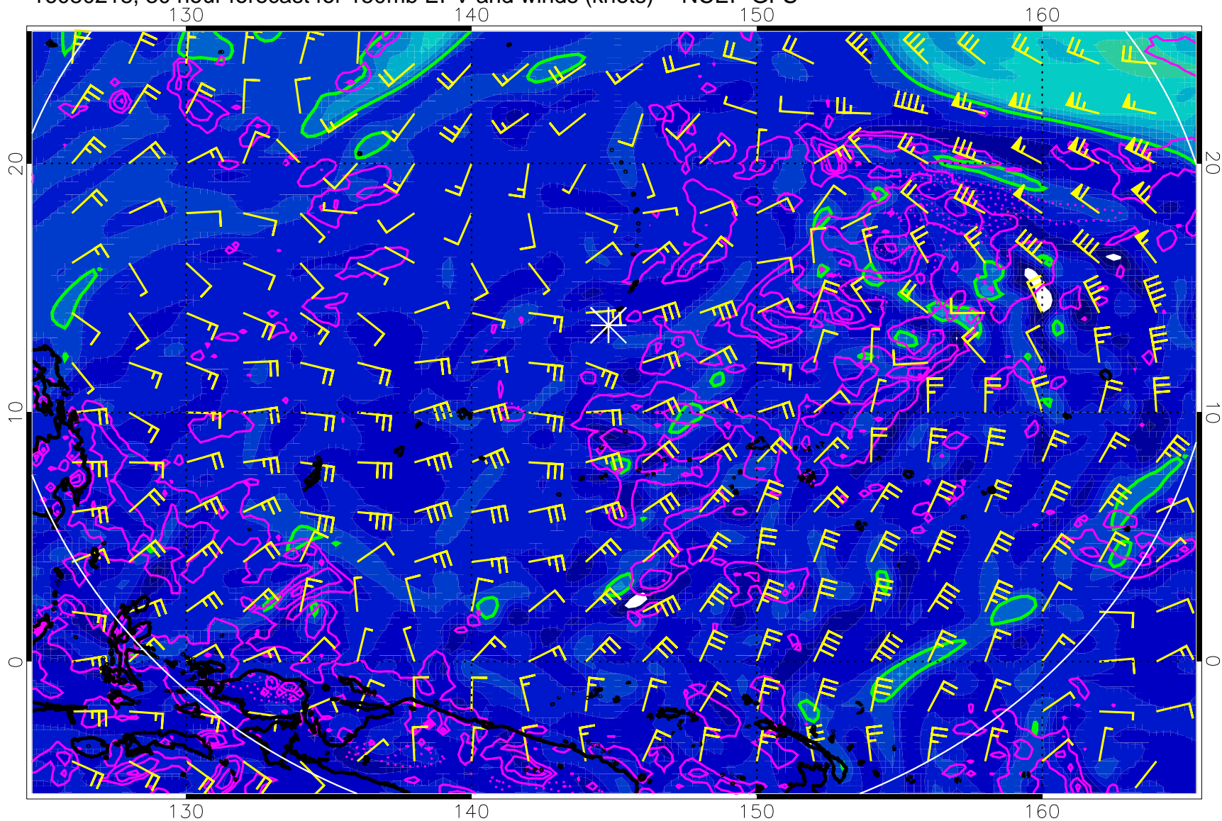
16080218, 30 hour forecast for 150mb EPV and winds (knots) -- NCEP GFS
