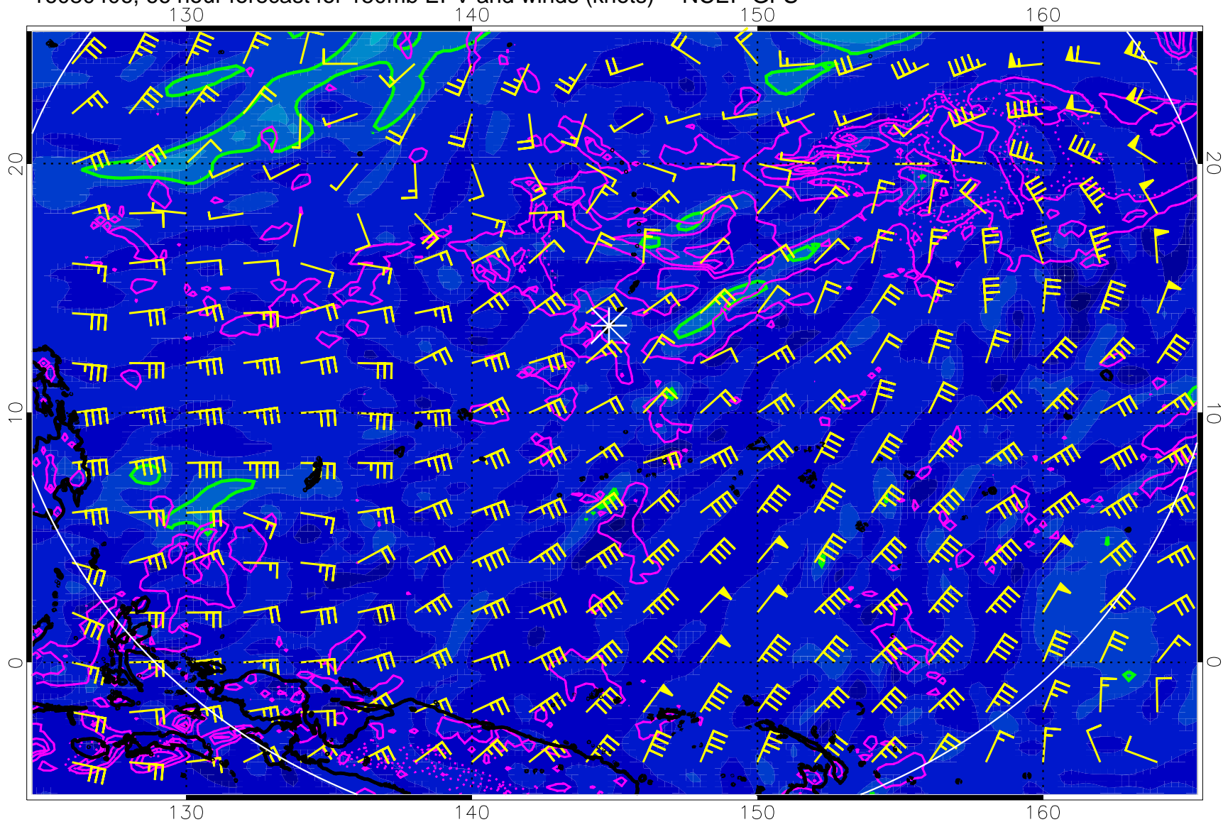
16080406, 66 hour forecast for 150mb EPV and winds (knots) -- NCEP GFS
