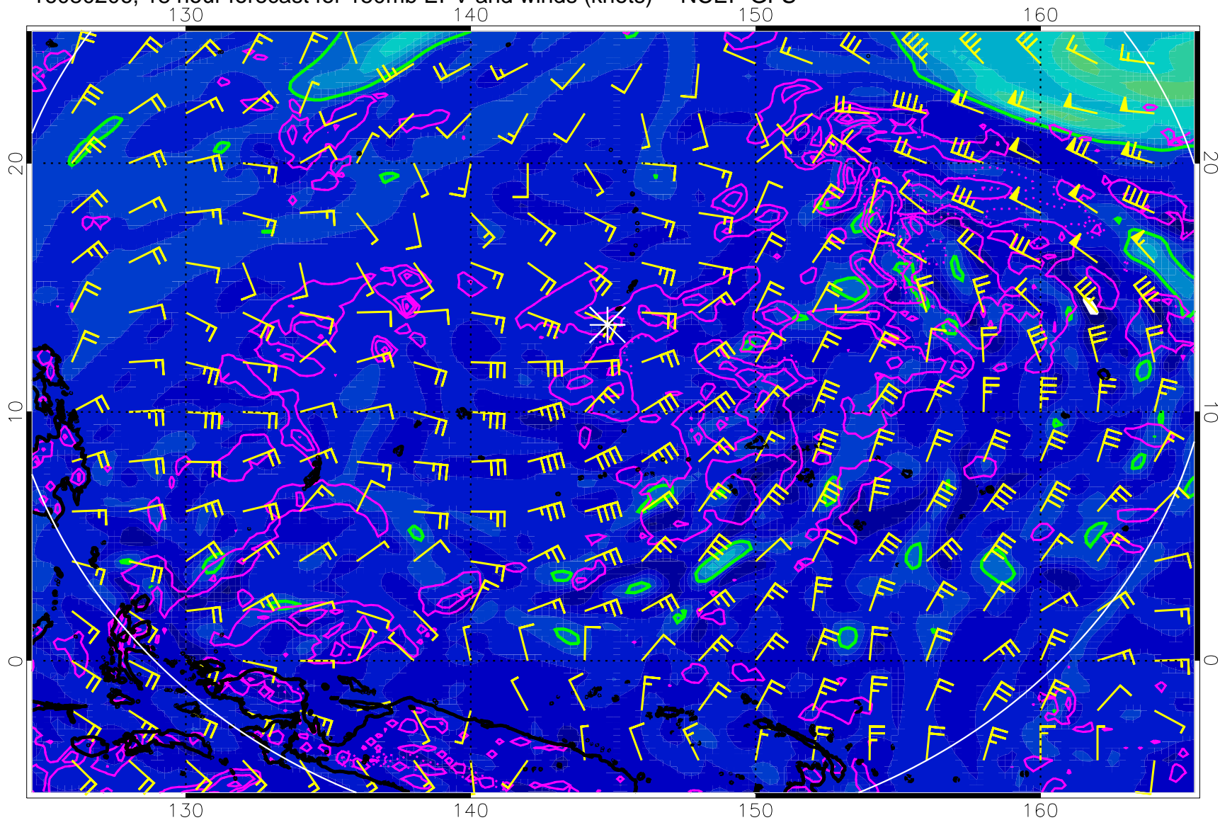
16080206, 18 hour forecast for 150mb EPV and winds (knots) -- NCEP GFS
