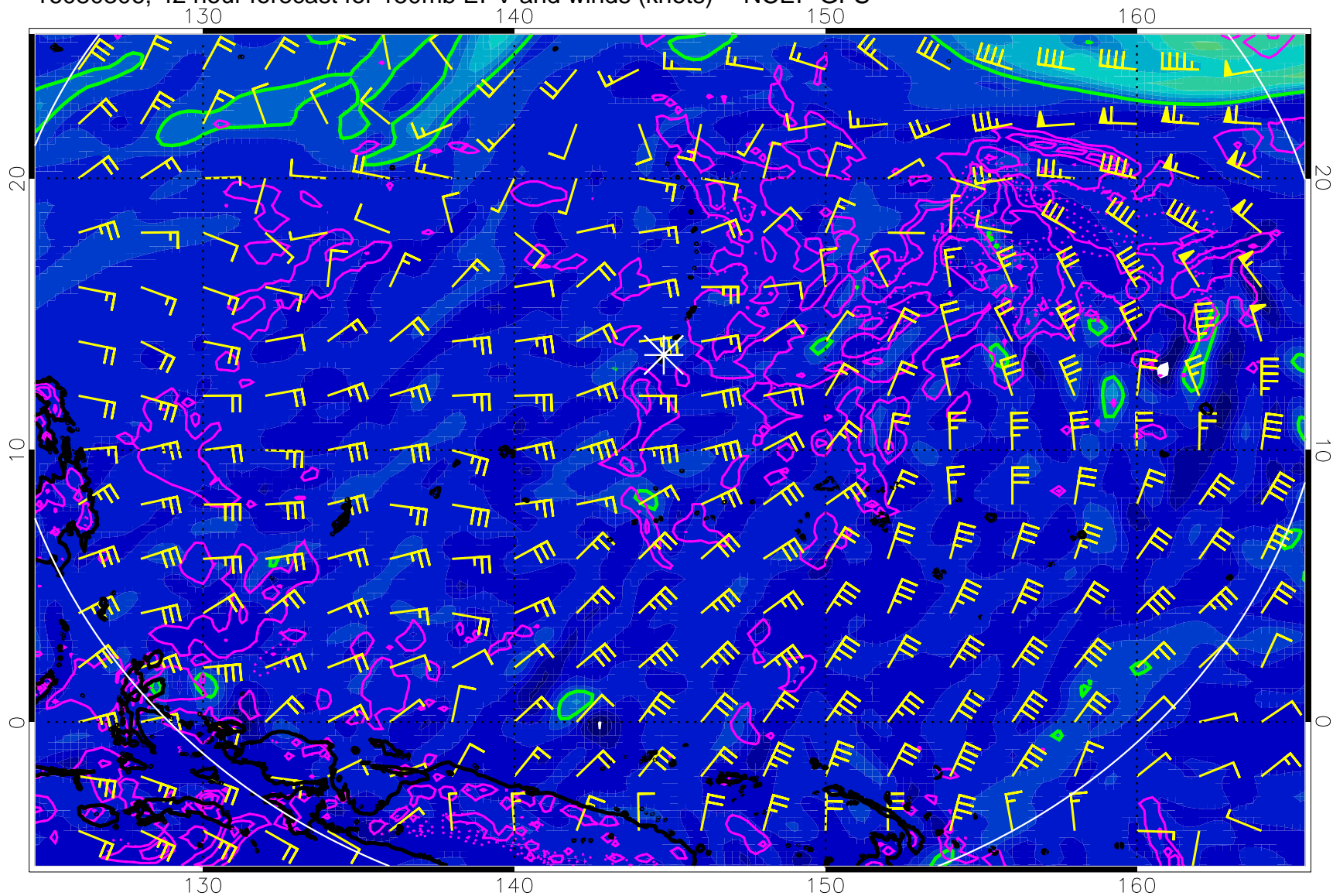
16080306, 42 hour forecast for 150mb EPV and winds (knots) -- NCEP GFS
