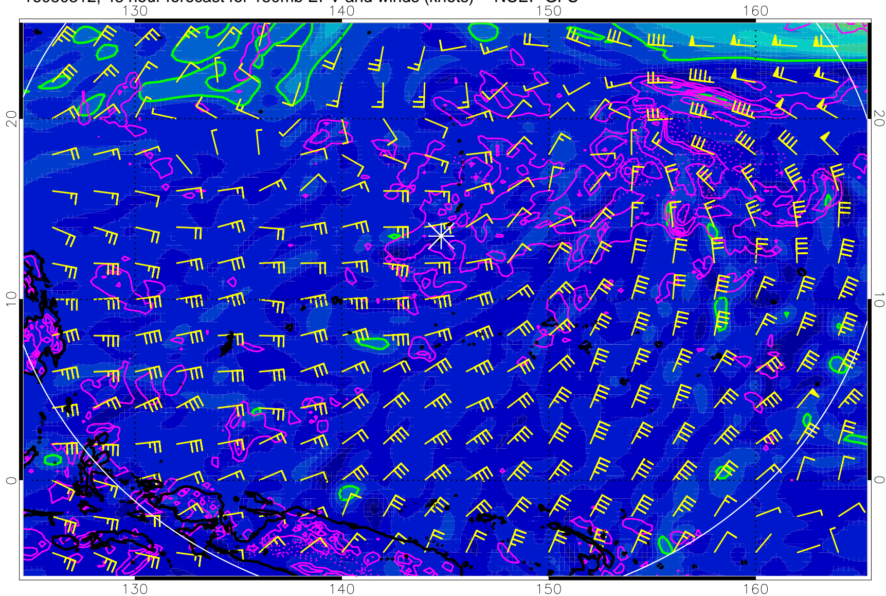
16080312, 48 hour forecast for 150mb EPV and winds (knots) -- NCEP GFS
