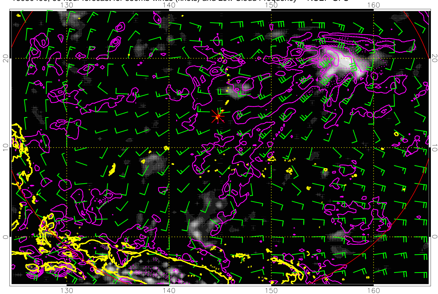
16080400, 60 hour forecast for 850mb winds (knots) and Low Cloud Frequency -- NCEP GFS
