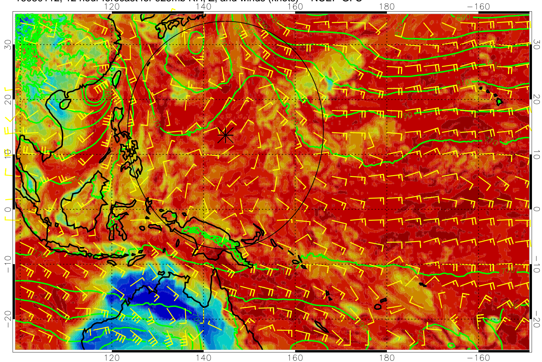
16080112, 12 hour forecast for 925mb RH, Z, and winds (knots) -- NCEP GFS
