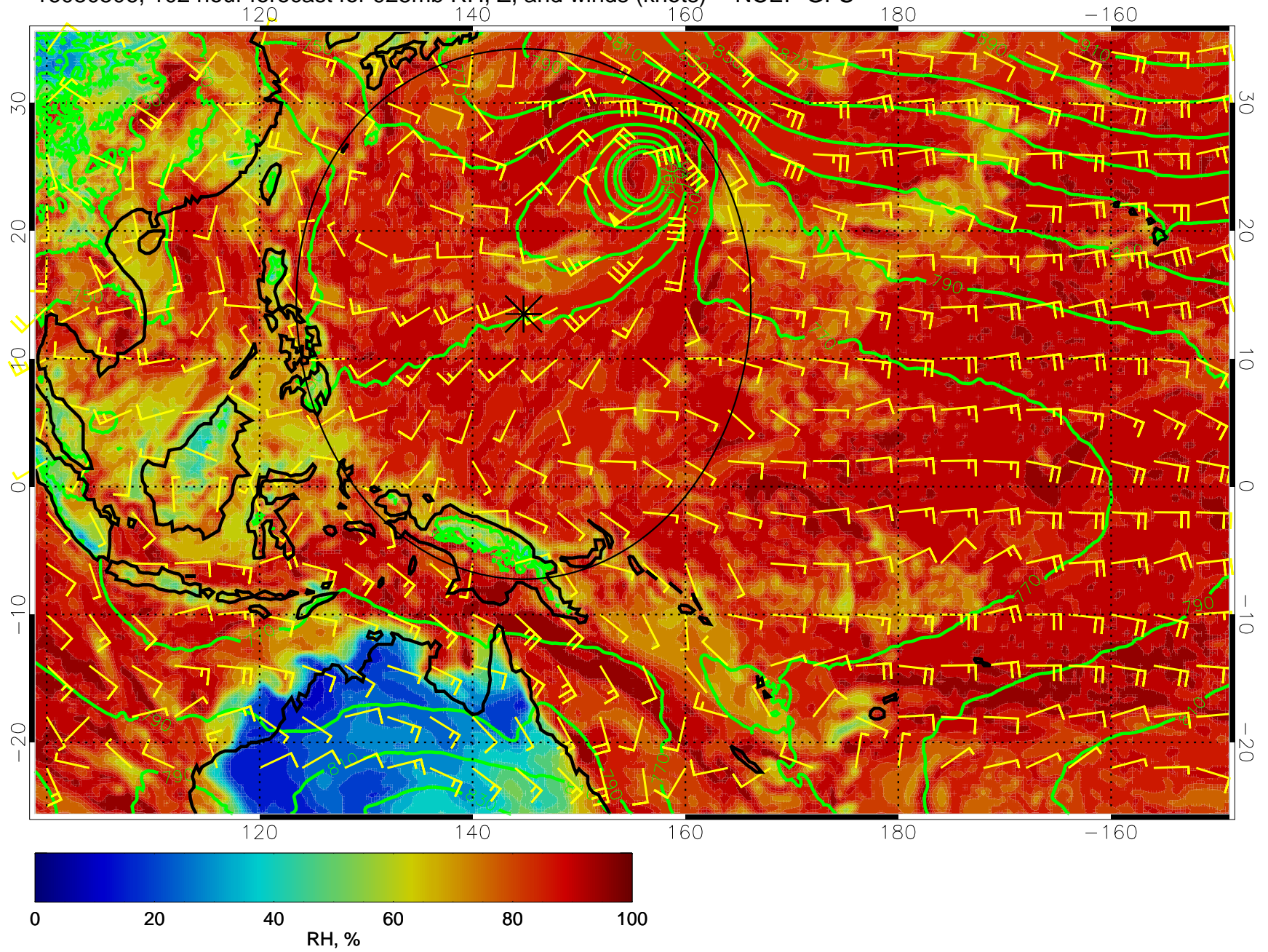
16080506, 102 hour forecast for 925mb RH, Z, and winds (knots) -- NCEP GFS
