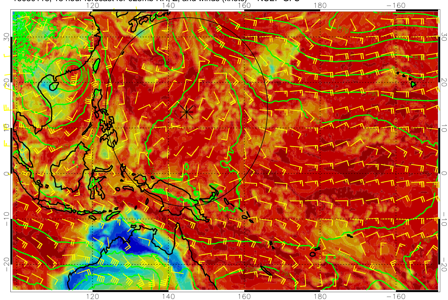
16080118, 18 hour forecast for 925mb RH, Z, and winds (knots) -- NCEP GFS
