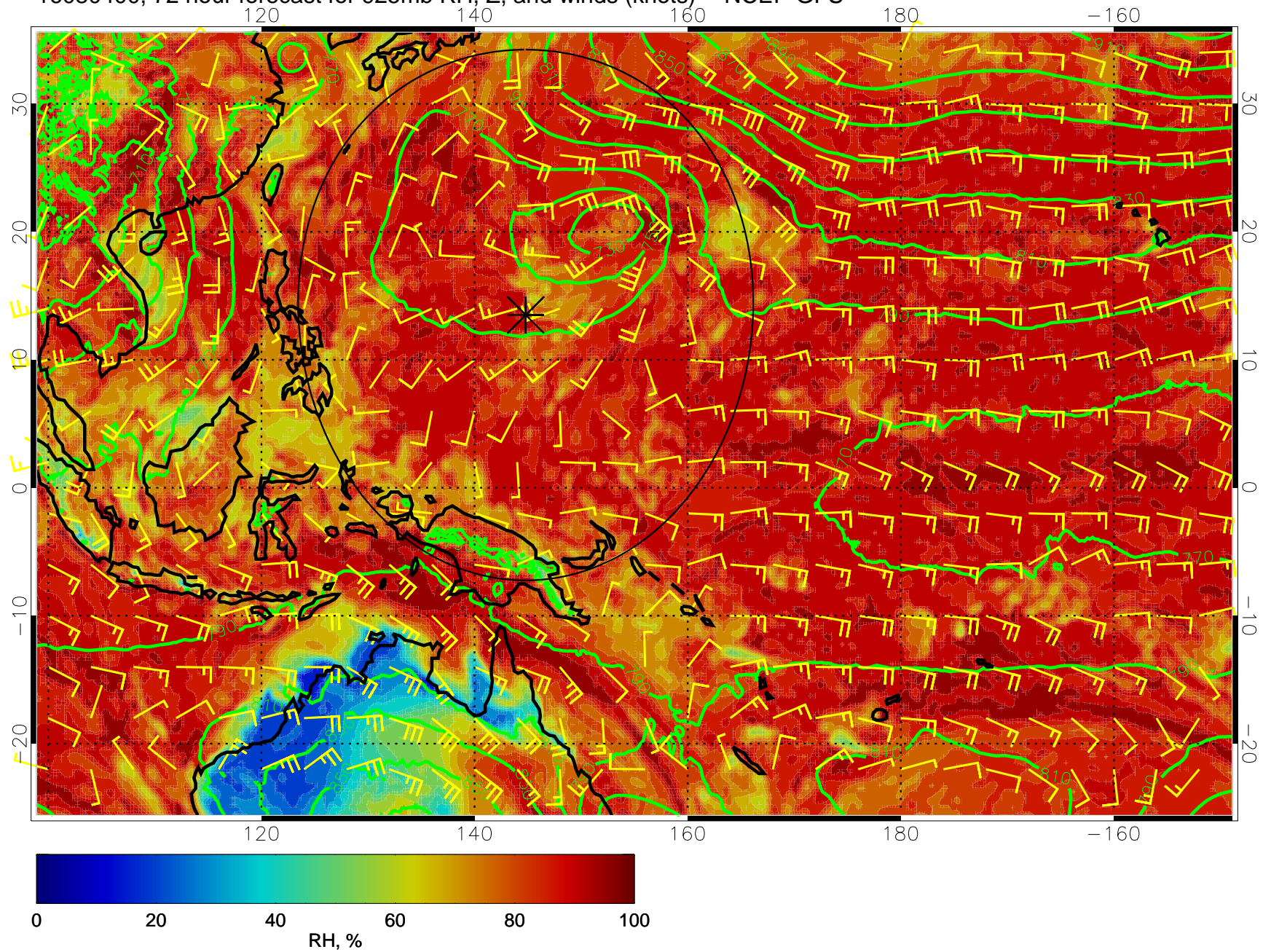
16080400, 72 hour forecast for 925mb RH, Z, and winds (knots) -- NCEP GFS
