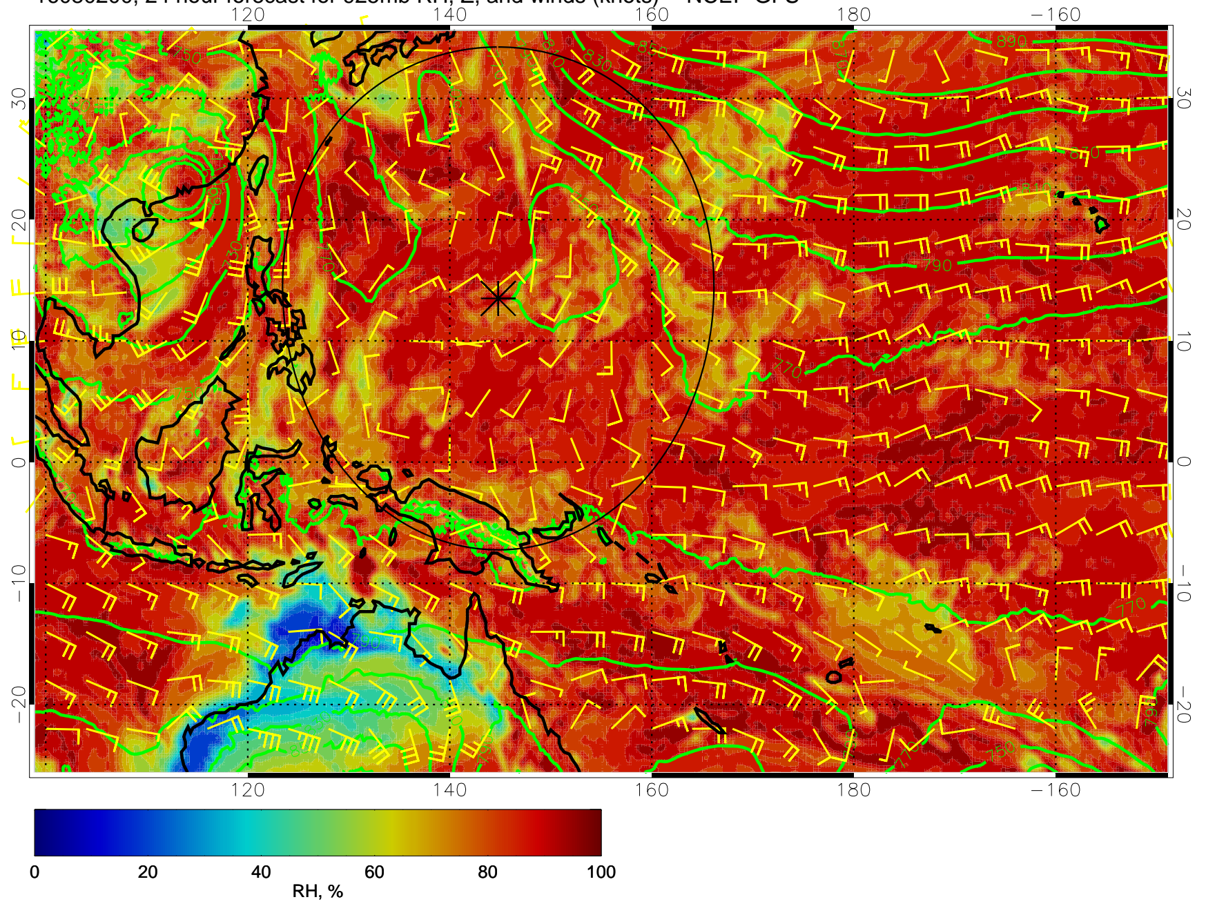
16080200, 24 hour forecast for 925mb RH, Z, and winds (knots) -- NCEP GFS
