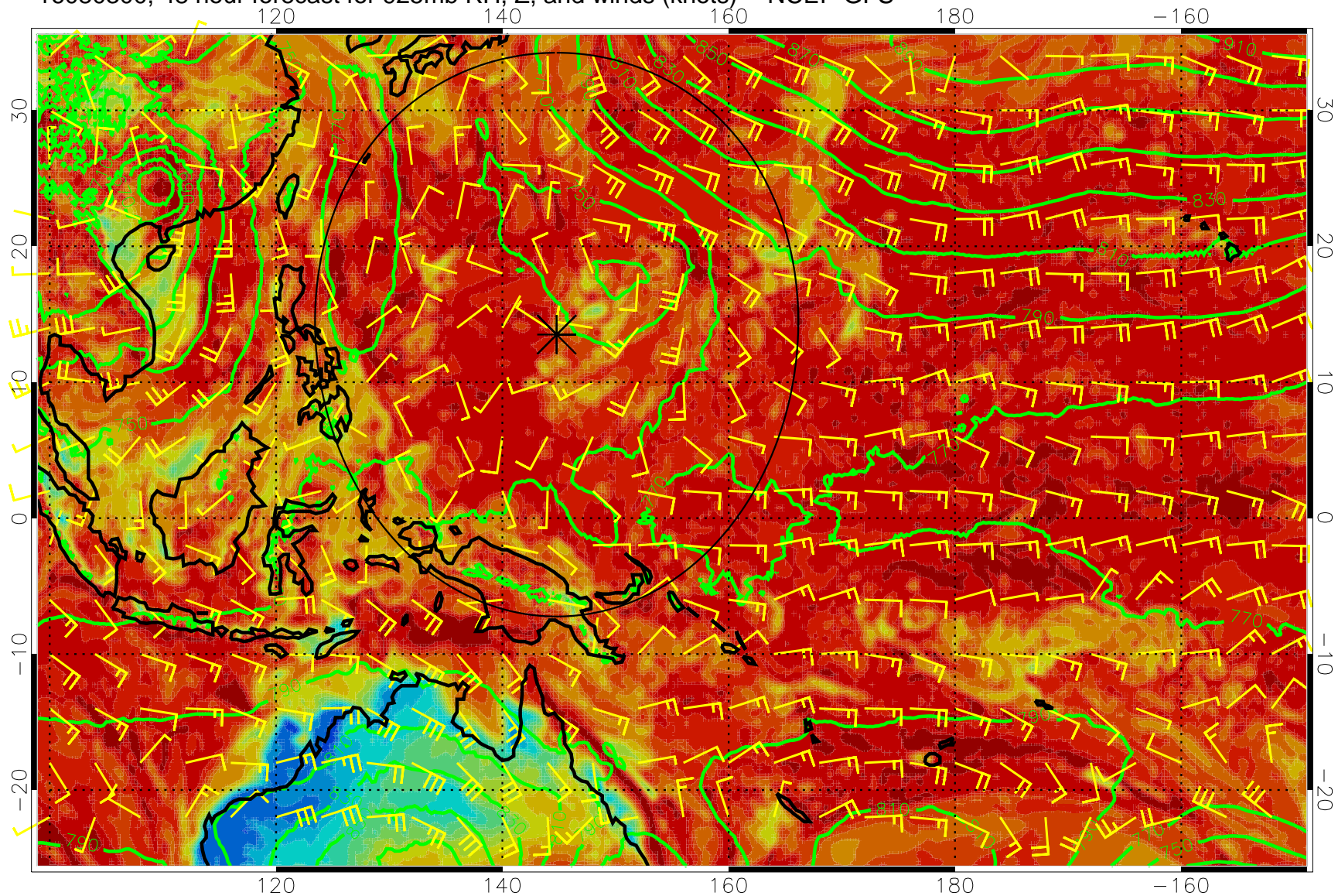
16080300, 48 hour forecast for 925mb RH, Z, and winds (knots) -- NCEP GFS
