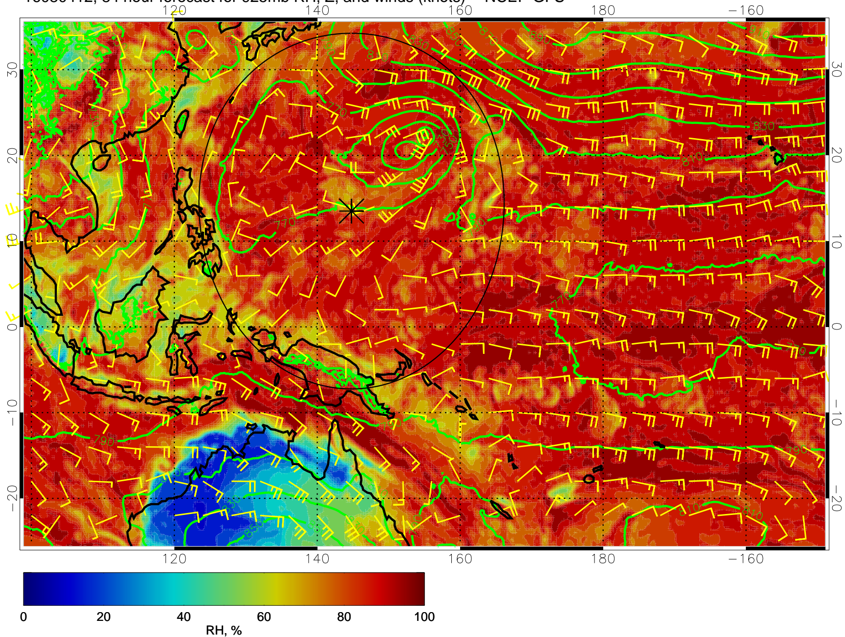
16080412, 84 hour forecast for 925mb RH, Z, and winds (knots) -- NCEP GFS
