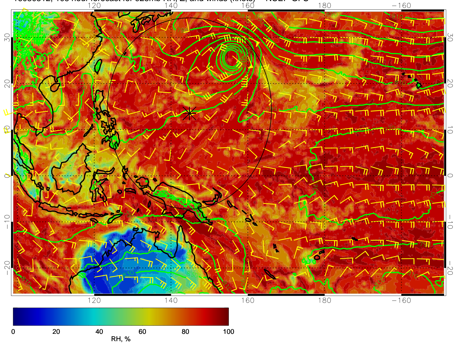
16080512, 108 hour forecast for 925mb RH, Z, and winds (knots) -- NCEP GFS
