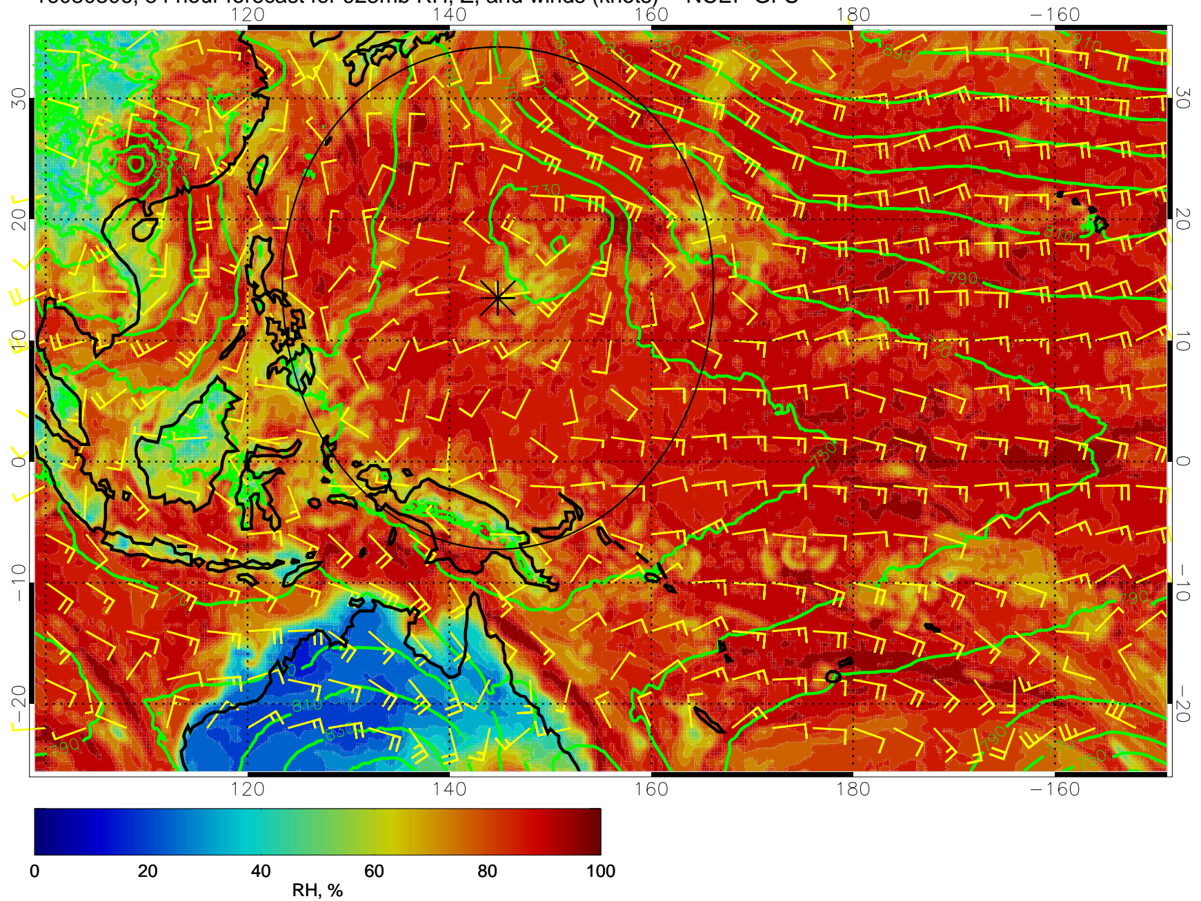
16080306, 54 hour forecast for 925mb RH, Z, and winds (knots) -- NCEP GFS
