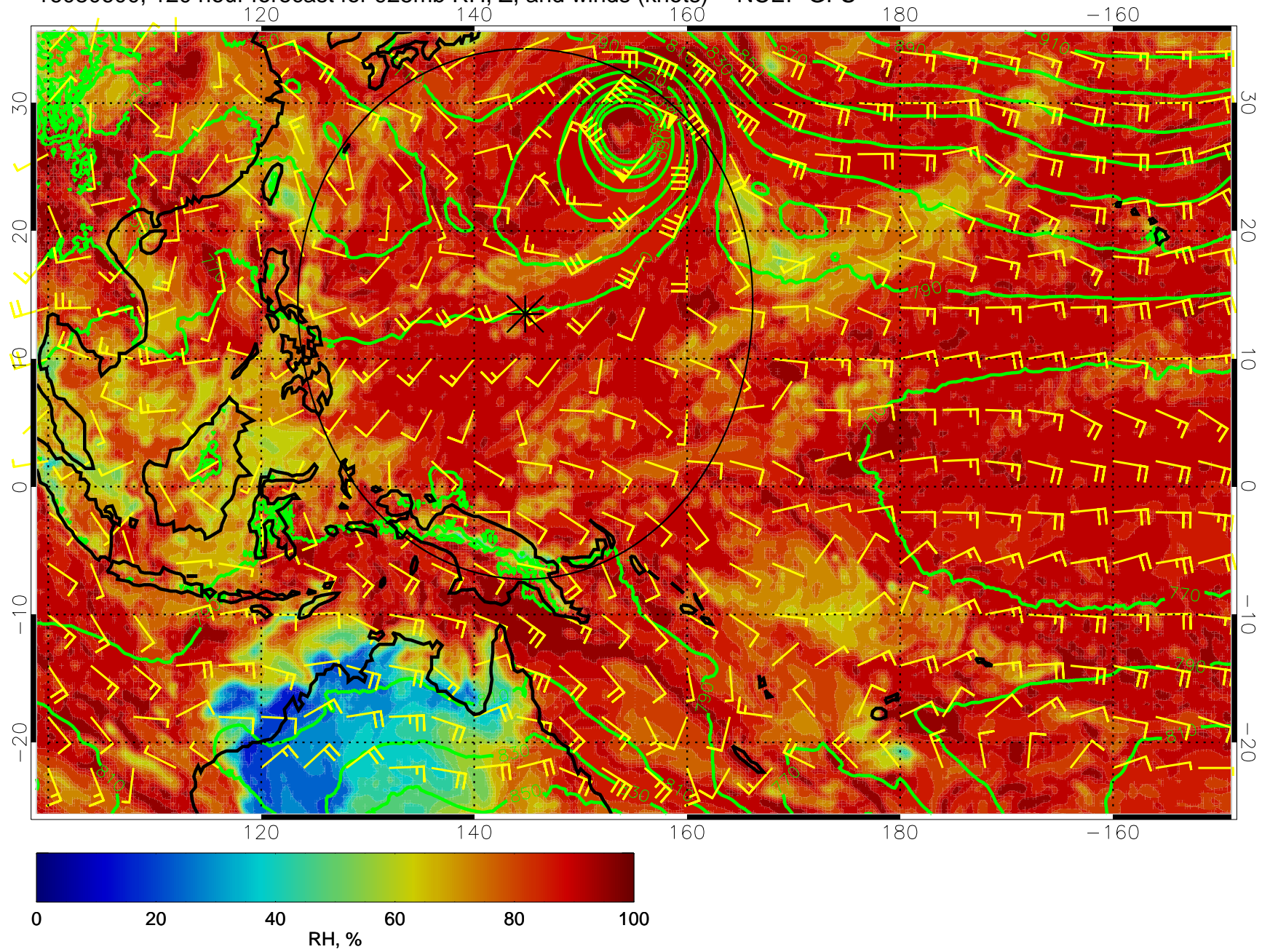
16080600, 120 hour forecast for 925mb RH, Z, and winds (knots) -- NCEP GFS
