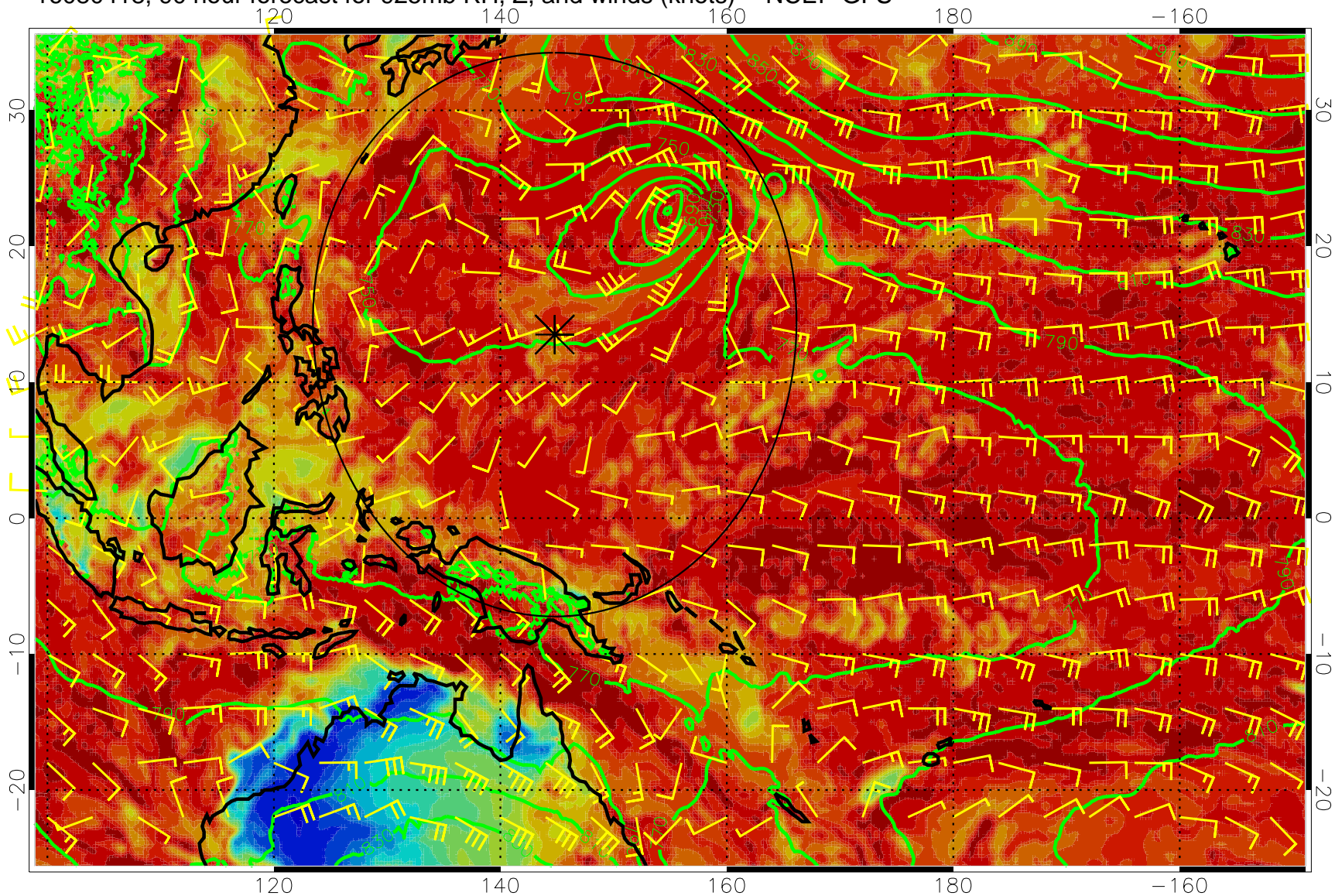
16080418, 90 hour forecast for 925mb RH, Z, and winds (knots) -- NCEP GFS
