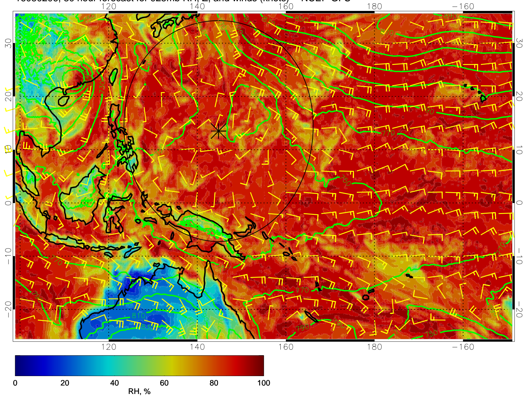
16080206, 30 hour forecast for 925mb RH, Z, and winds (knots) -- NCEP GFS
