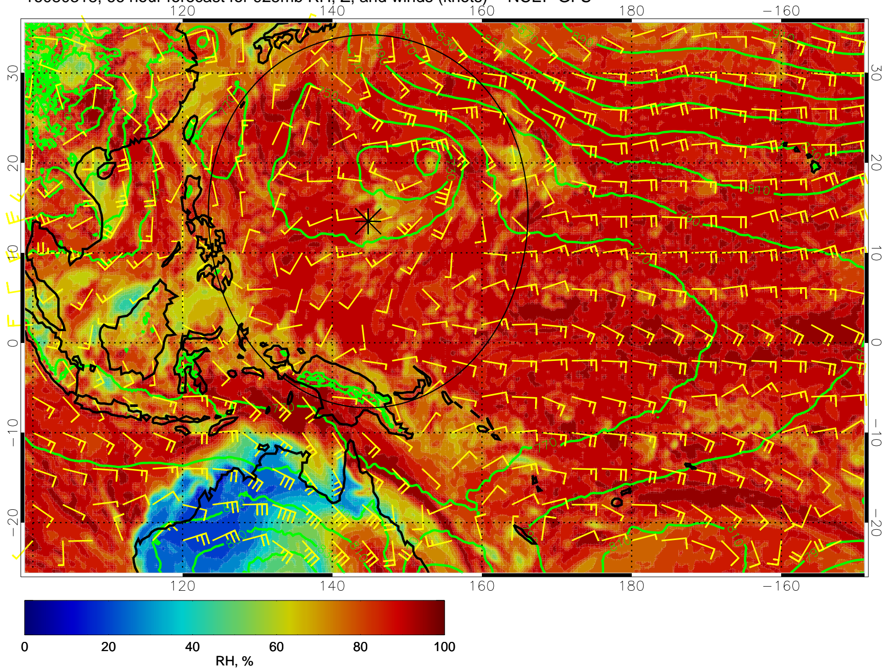
16080318, 66 hour forecast for 925mb RH, Z, and winds (knots) -- NCEP GFS
